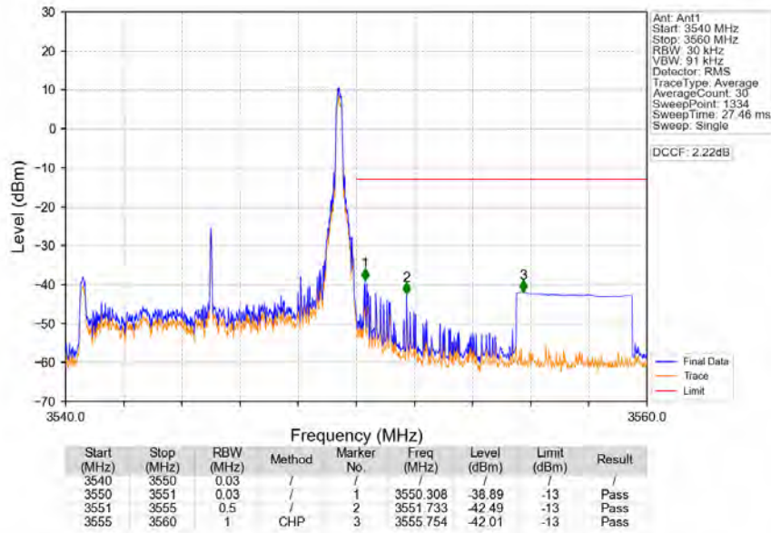
Band42a_10MHz_256QAM_HCH_3545MHz_RB_50_0_NTNV
