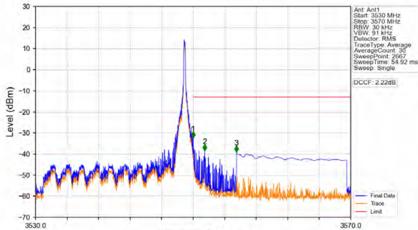
Band42a_20MHz_16QAM_HCH_3540MHz_RB_1_99_NTNV
