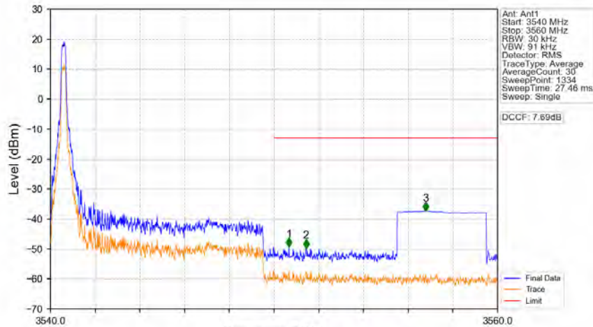
Band42a_10MHz_16QAM_HCH_3545MHz_RB_1_49_NTNV
