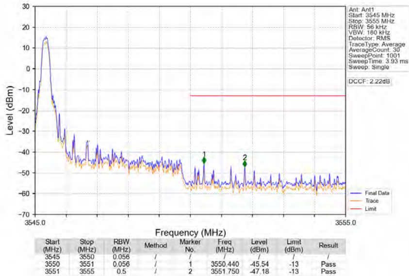
Band42a_5MHz_64QAM_HCH_3547.5MHz_RB_25_0_NTNV
