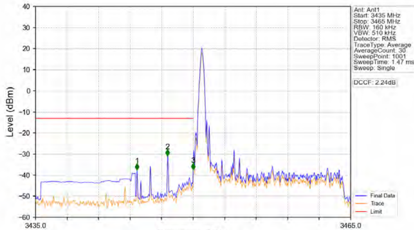
Band42a_15MHz_64QAM_LCH_3457.5MHz_RB_75_0_NTNV
