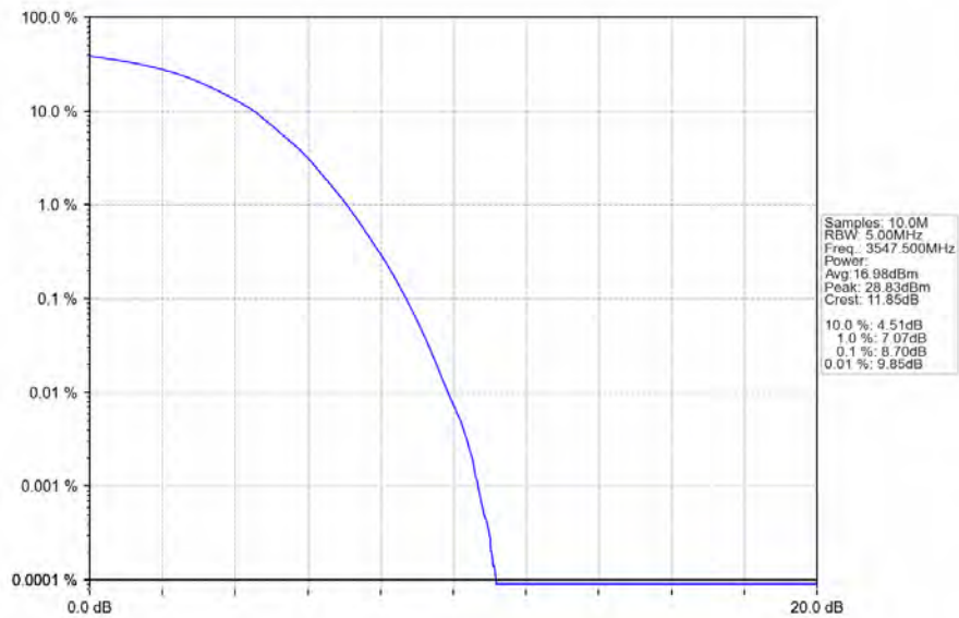
Band42a_5MHz_64QAM_HCH_3547.5MHz_RB_25_0_NTNV
