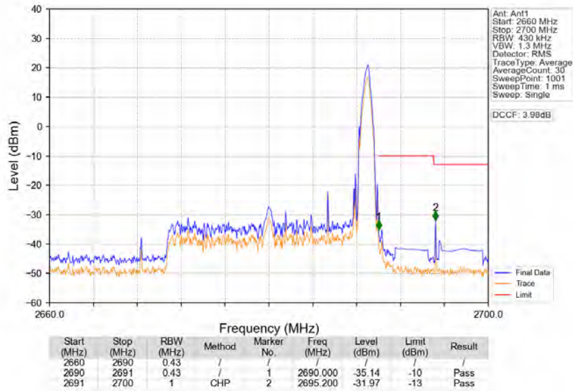
Band41_20MHz_256QAM_HCH_2680MHz_RB_1_99_NTNV
