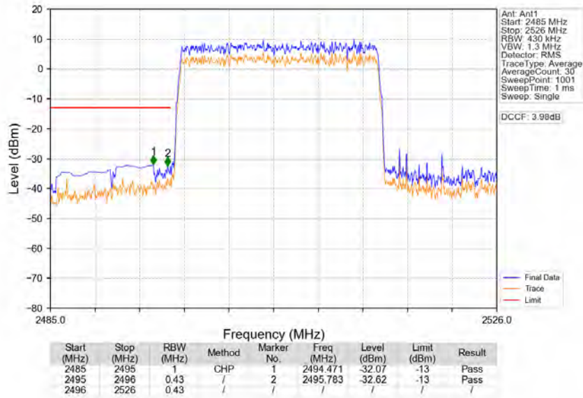
Band41_20MHz_64QAM_LCH_2506MHz_RB_100_0_NTNV
