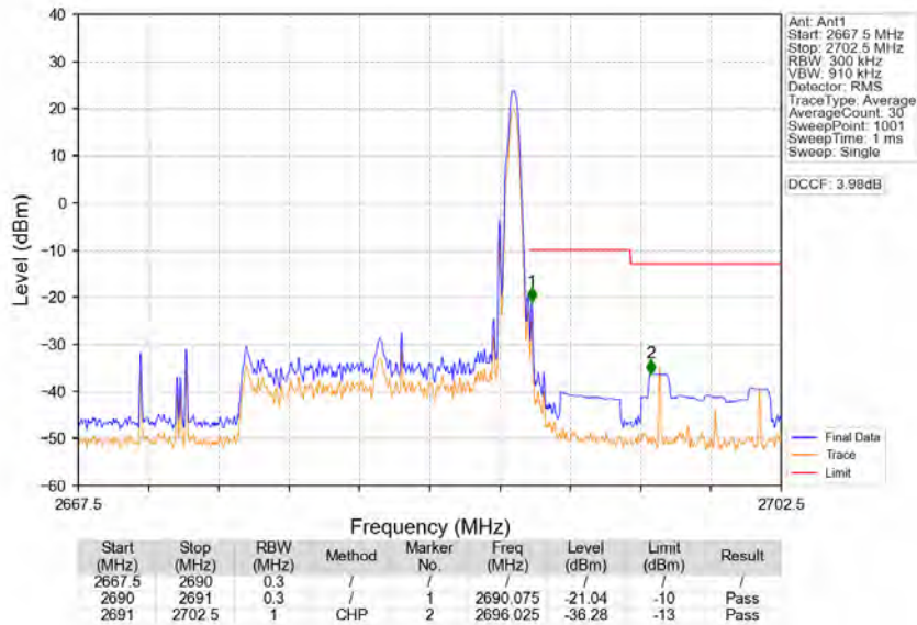
Band41_15MHz_16QAM_HCH_2682.5MHz_RB_1_74_NTNV
