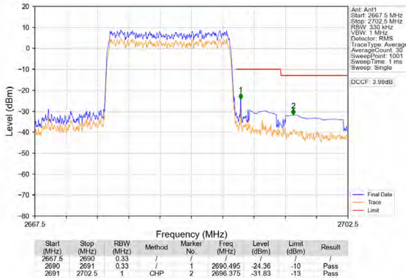
Band41_15MHz_64QAM_HCH_2682.5MHz_RB_75_0_NTNV
