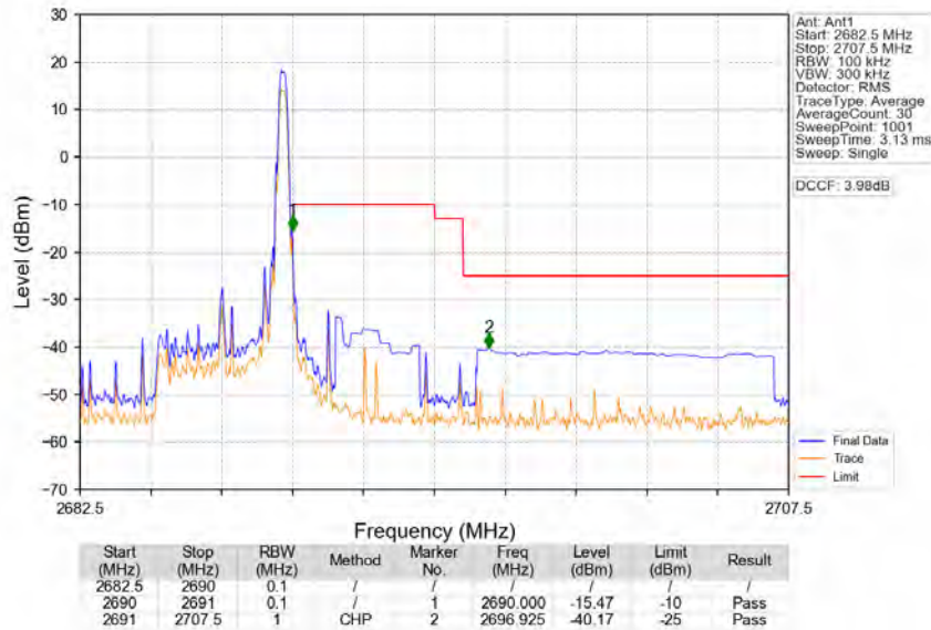
Band41_5MHz_256QAM_HCH_2687.5MHz_RB_1_24_NTNV
