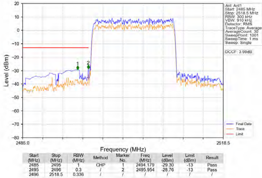
Band41_15MHz_64QAM_LCH_2503.5MHz_RB_75_0_NTNV
