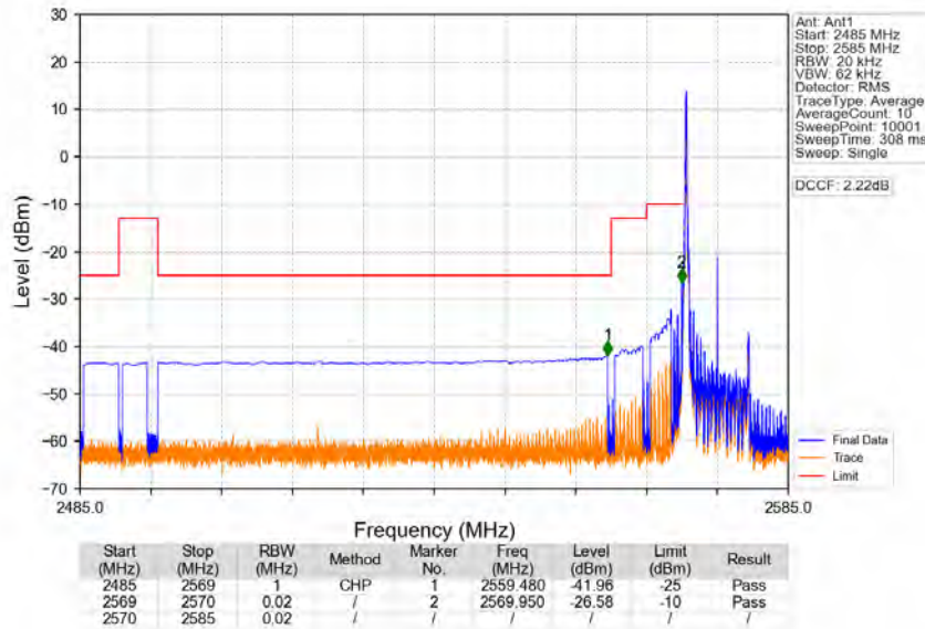
Band38_10MHz_64QAM_LCH_2575MHz_RB_1_0_NTNV
