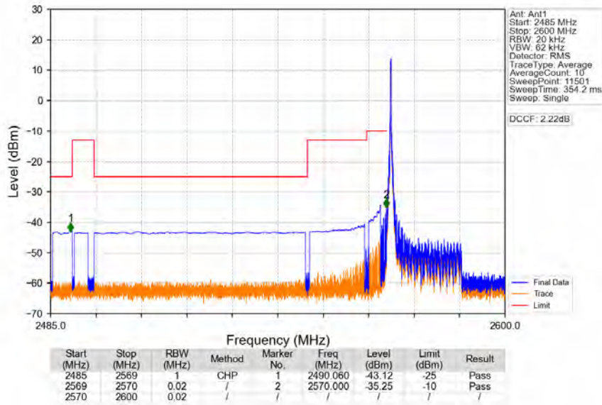
Band38_20MHz_64QAM_LCH_2580MHz_RB_1_0_NTNV
