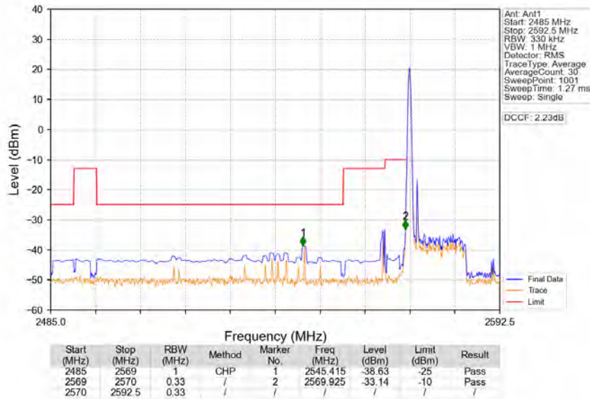
Band38_15MHz_64QAM_LCH_2577.5MHz_RB_75_0_NTNV
