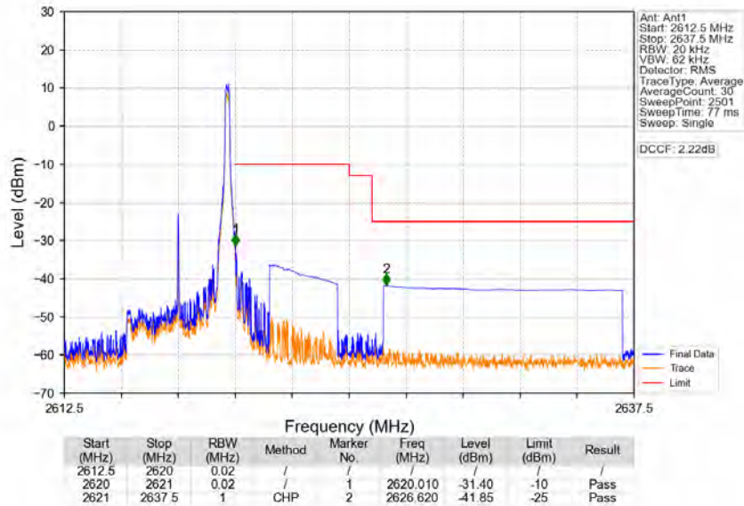
Band38_5MHz_256QAM_HCH_2617.5MHz_RB_1_24_NTNV
