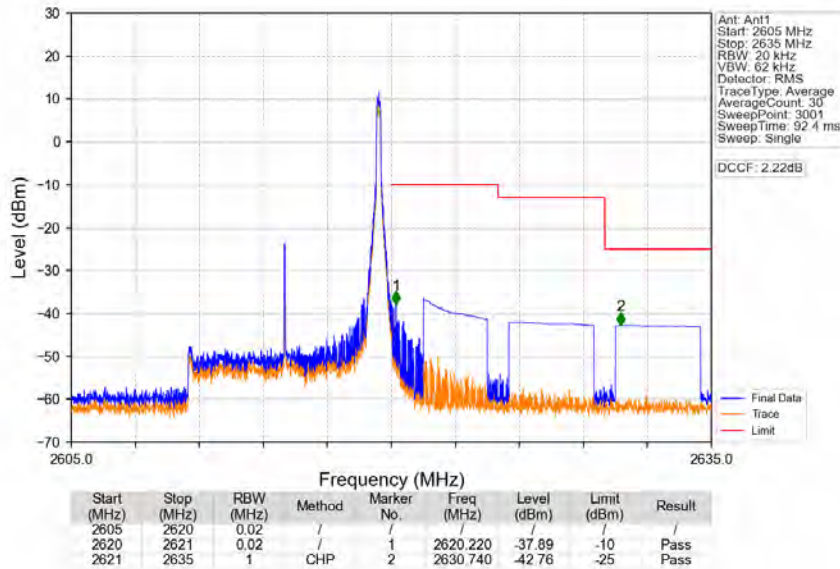
Band38_10MHz_256QAM_HCH_2615MHz_RB_1_49_NTNV
