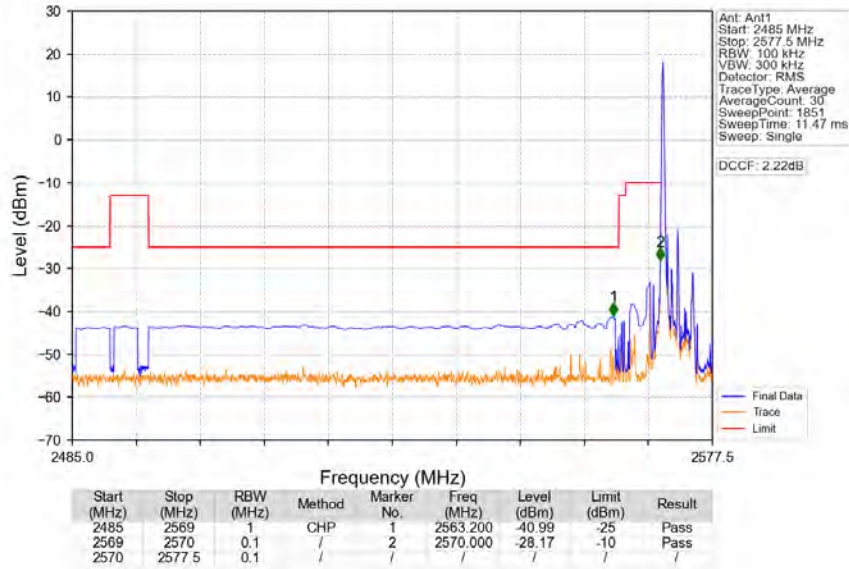
Band38_5MHz_QPSK_LCH_2572.5MHz_RB_25_0_NTNV
