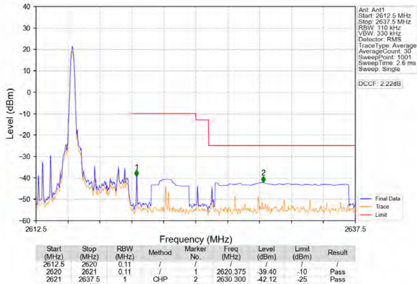
Band38_5MHz_QPSK_HCH_2617.5MHz_RB_25_0_NTNV
