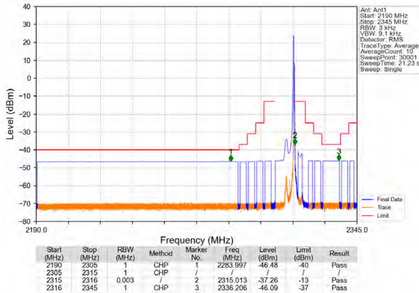
Band30_5MHz_QPSK_HCH_2312.5MHz_RB_25_0_NTNV
