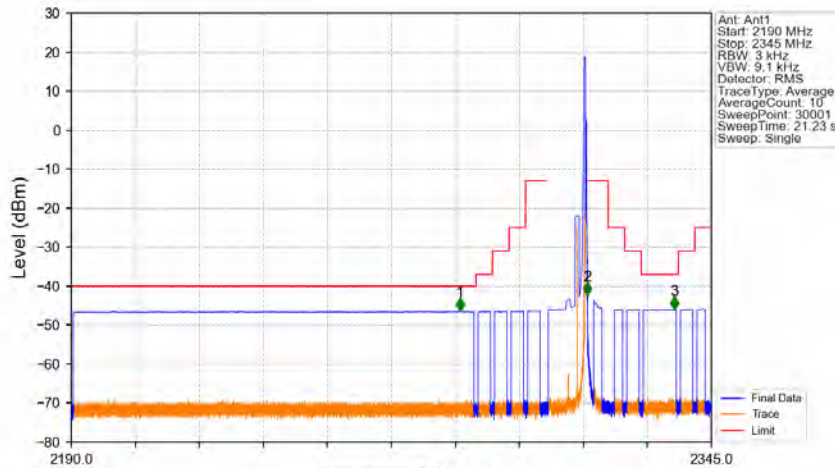
Band30_5MHz_256QAM_HCH_2312.5MHz_RB_1_24_NTNV
