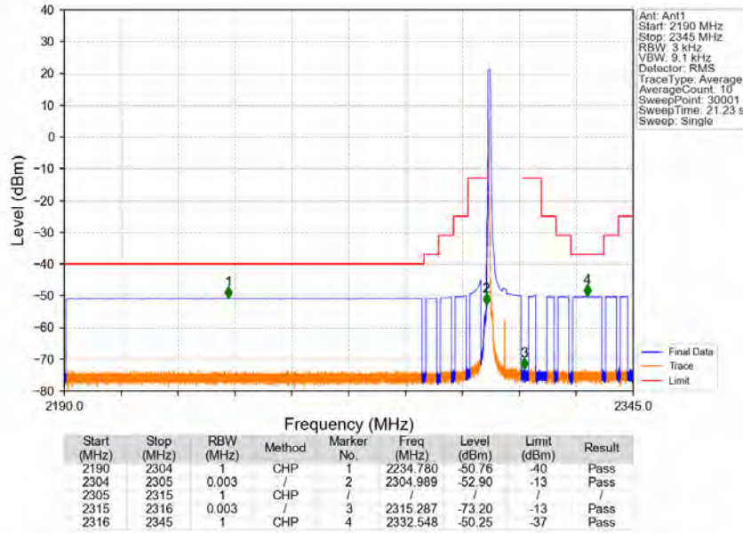
Band30_10MHz_64QAM_LCH_2310MHz_RB_1_0_NTNV
