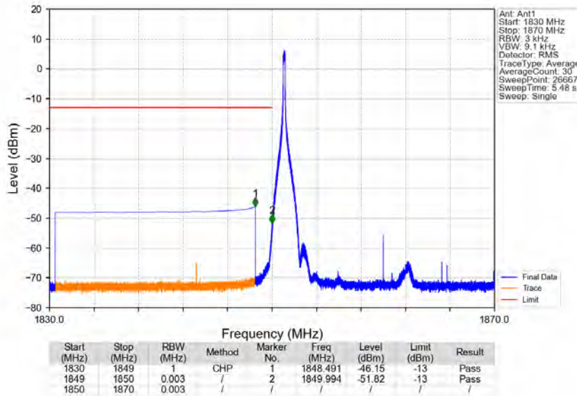
Band25_20MHz_16QAM_LCH_1860MHz_RB_1_0_NTNV
