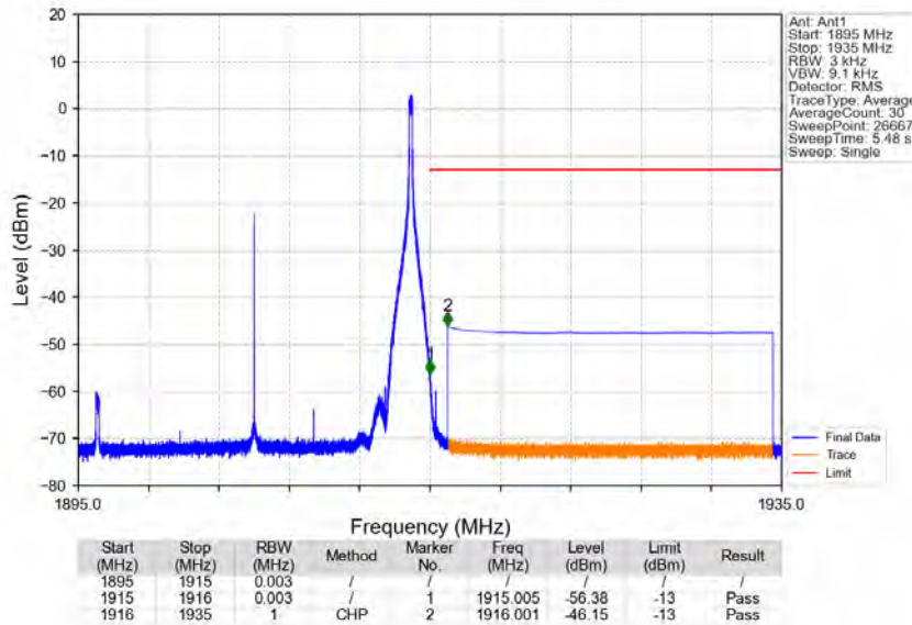
Band25_20MHz_256QAM_HCH_1905MHz_RB_1_99_NTNV
