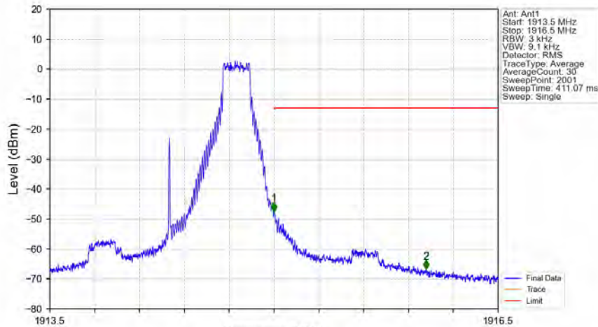
Band25_1.4MHz_256QAM_HCH_1914.3MHz_RB_1_5_NTNV
