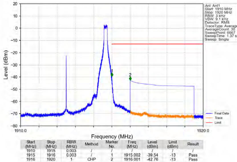
Band25_5MHz_256QAM_HCH_1912.5MHz_RB_1_24_NTNV
