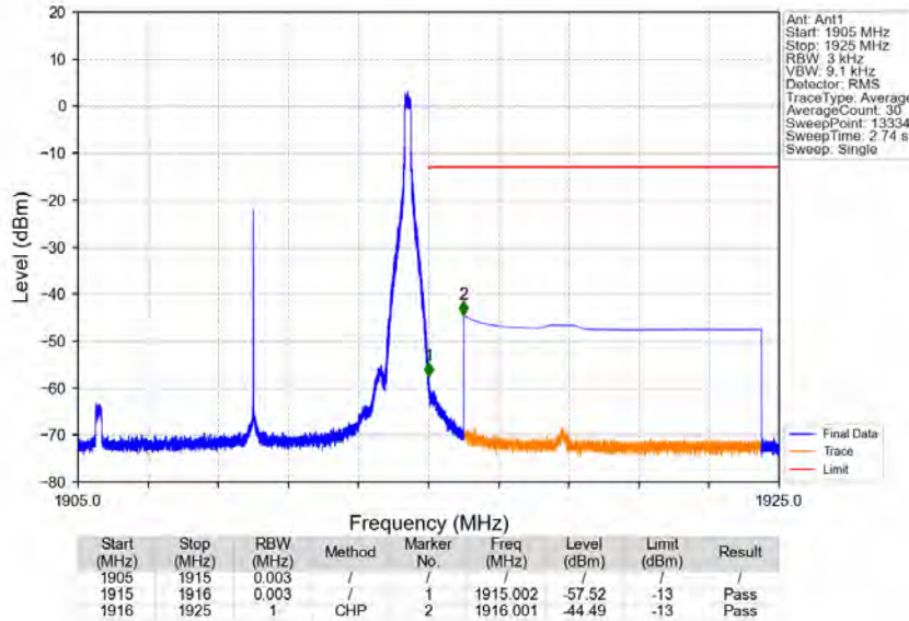
Band25_10MHz_256QAM_HCH_1910MHz_RB_1_49_NTNV
