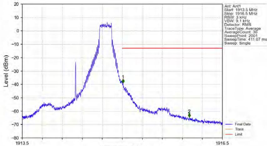
Band25 1.4MHz 16QAM HCH 1914.3MHz RB 1 5 NTV
