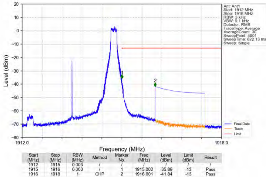
Band25_3MHz_256QAM_HCH_1913.5MHz_RB_1_14_NTNV
