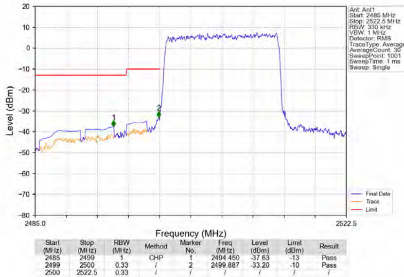
Band7_15MHz_QPSK_LCH_2507.5MHz_RB_75_0_NTNV
