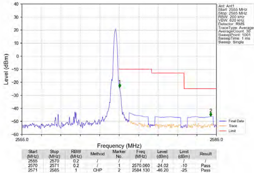
Band7_10MHz_16QAM_HCH_2565MHz_RB_1_49_NTV
