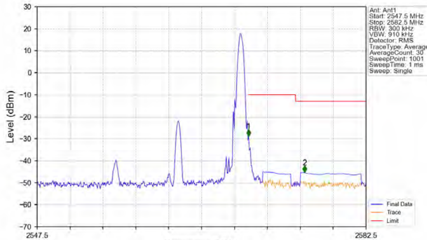
Band7_15MHz_256QAM_HCH_2562.5MHz_RB_1_74_NTNV
