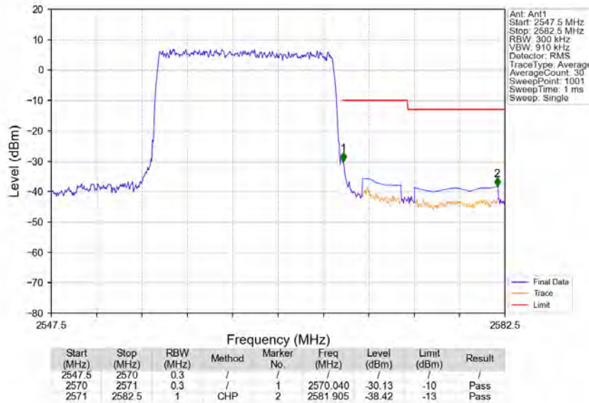
Band7_15MHz_QPSK_HCH_2562.5MHz_RB_75_0_NTV
