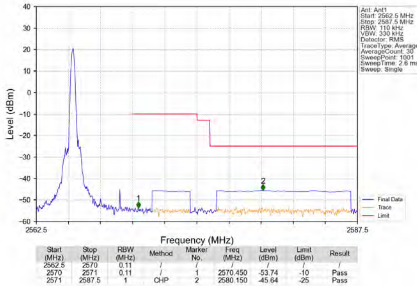
Band7_5MHz_64QAM_HCH_2567.5MHz_RB_25_0_NTNV
