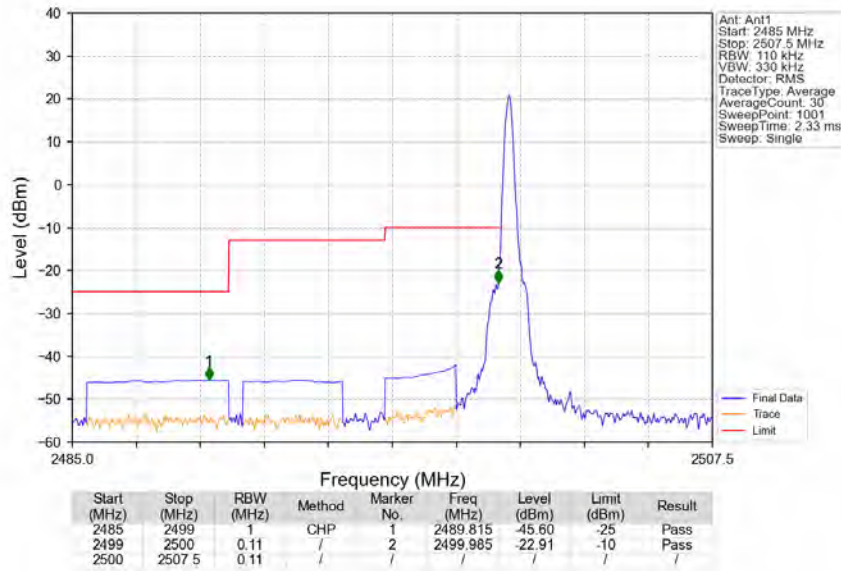
Band7_5MHz_64QAM_LCH_2502.5MHz_RB_25_0_NTNV
