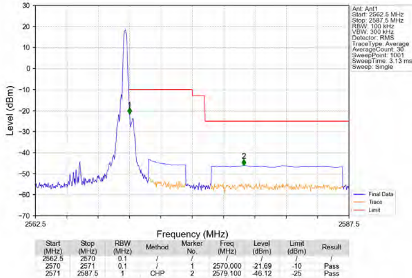
Band7_5MHz_16QAM_HCH_2567.5MHz_RB_1_24_NTNV
