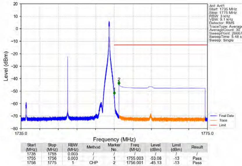
Band4_20MHz_64QAM_HCH_1745MHz_RB_1_99_NTNV
