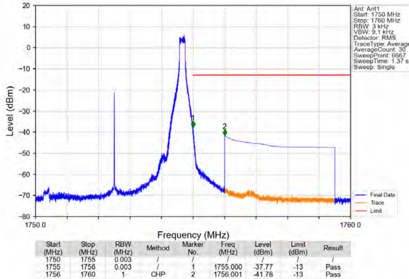
Band4_5MHz_64QAM_HCH_1752.5MHz_RB_1_24_NTNV
