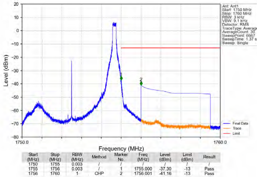
Band4 5MHz QPSK HCH 1752.5MHz RB 1 24_NTNV
