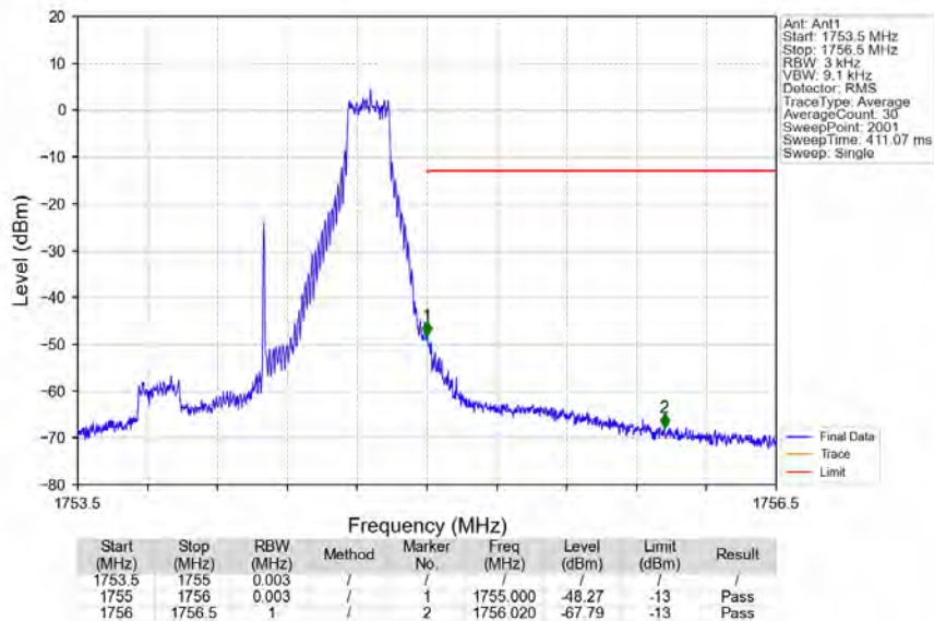
Band4 1.4MHz 256QAM HCH 1754.3MHz RB 1 5 NTV
