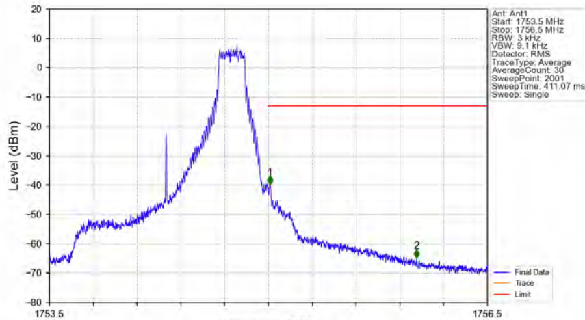
Band4 1.4MHz QPSK HCH 1754.3MHz RB 1 5 NTV
