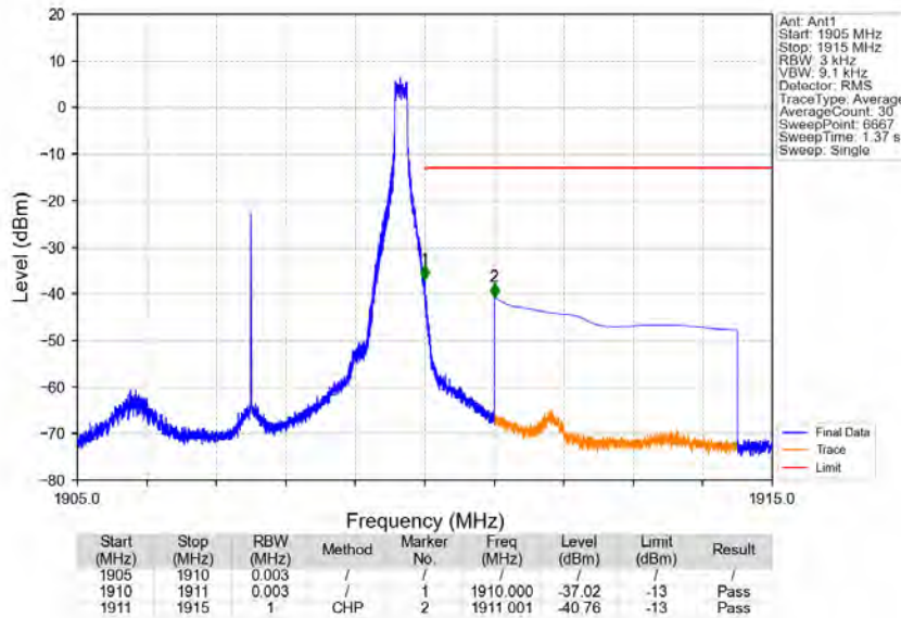
Band2_5MHz_16QAM_HCH_1907.5MHz_RB_1_24_NTNV
