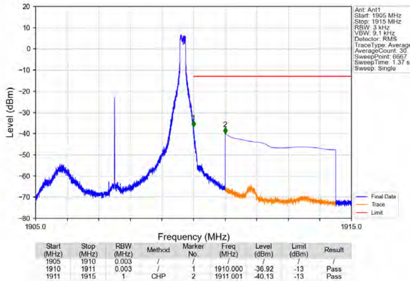
Band2 5MHz QPSK HCH 1907.5MHz RB 1 24_NTNV
