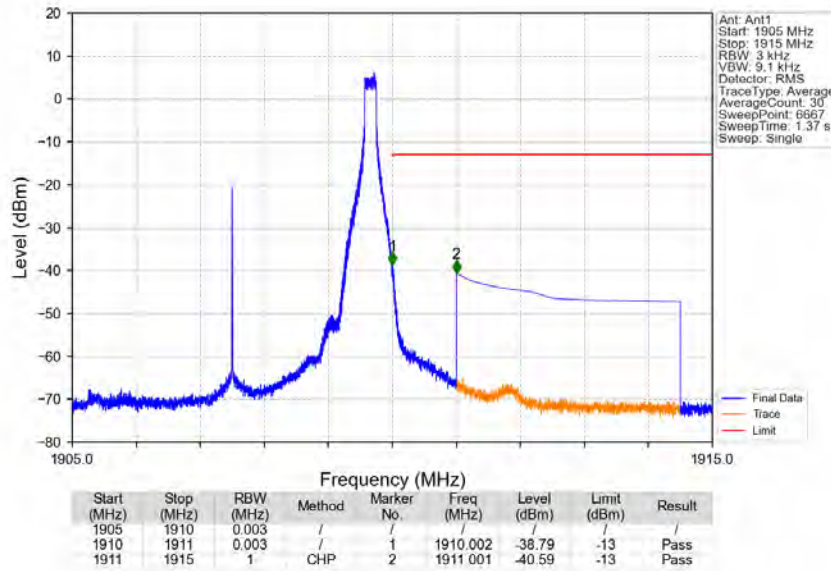
Band2_5MHz_64QAM_HCH_1907.5MHz_RB_1_24_NTNV
