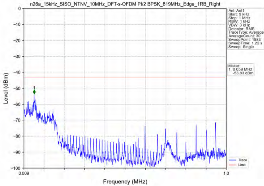
n26a_15kHz_SISO_NTNV_10MHz_DFT-s-OFDM PI/2 BPSK_819MHz_Edge_1RB_Right
