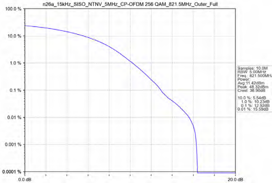
n26a_15kHz_SISO_NTNV_5MHz_CP-OFDM 256 QAM 821.5MHz_Outer_Full
