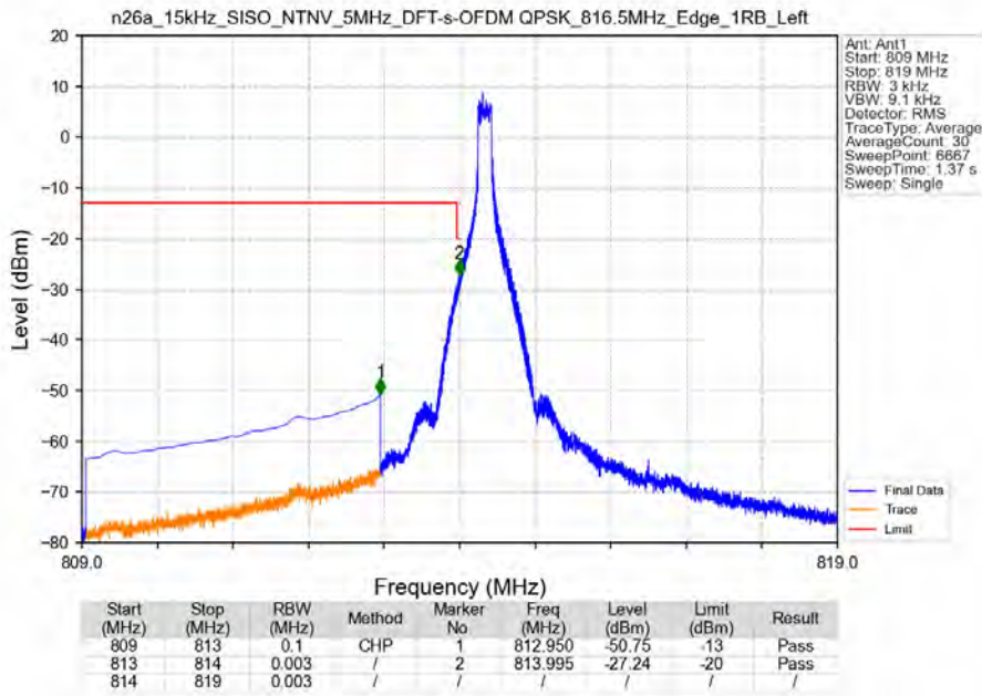
n26a_15kHz_SISO_NTNV_5MHz_DFT-s-OFDM_QPSK_816.5MHz_Edge_1RB_Left
