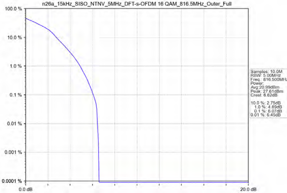
n26a_15kHz_SISO_NTNV_5MHz_DFT-s-OFDM_16 QAM_816.5MHz_Outer_Full
