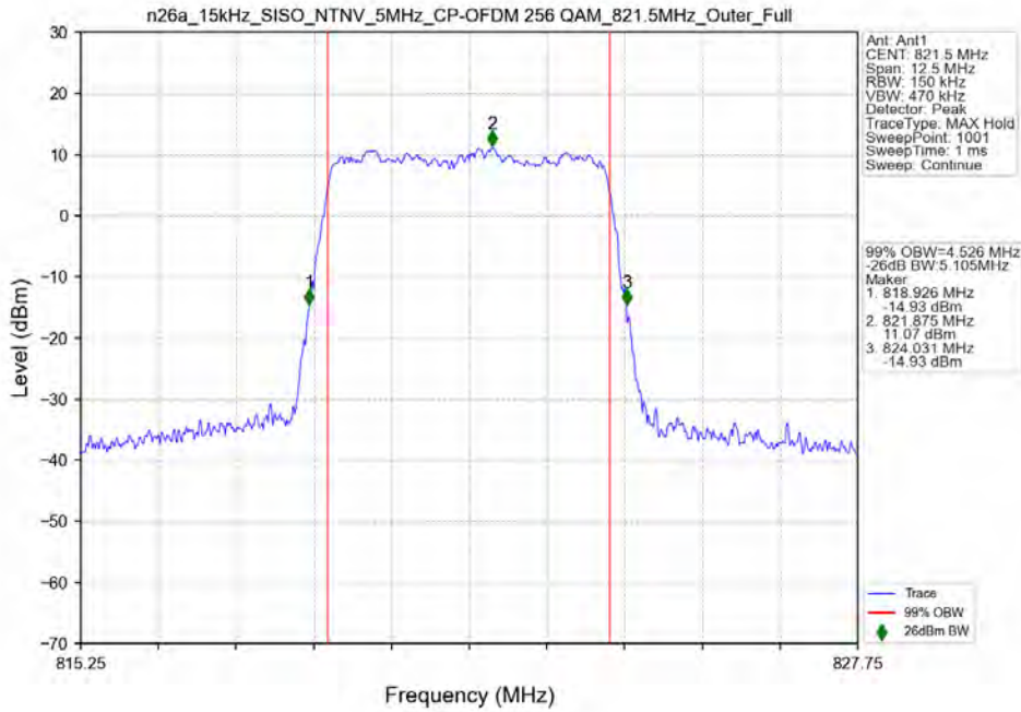
n26a_15kHz_SISO_NTNV_5MHz_CP-OFDM 256 QAM 821.5MHz_Outer_Full
