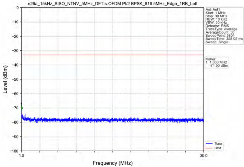
n26a_15kHz_SISO_NTNV_5MHz_DFT-s-OFDM PI/2 BPSK_816.5MHz_Edge_1RB_Left
