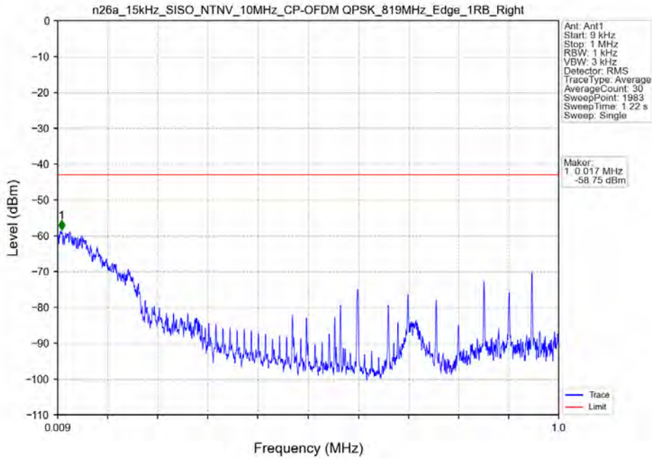
n26a_15kHz_SISO_NTNV_10MHz_CP-OFDM QPSK_819MHz_Edge_1RB_Right
