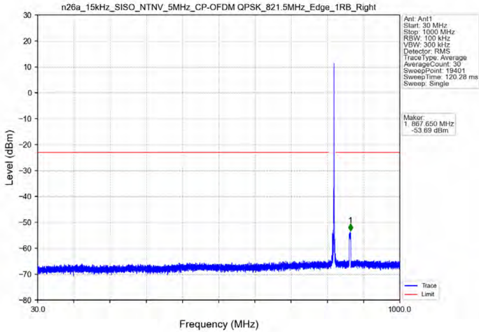
n26a_15kHz_SISO_NTNV_5MHz_CP-OFDM QPSK_821.5MHz_Edge_1RB_Right
