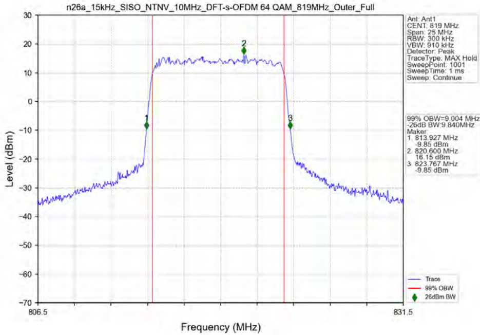
n26a_15kHz_SISO_NTNV_10MHz_DFT-s-OFDM 64 QAM_819MHz_Outer_Full
