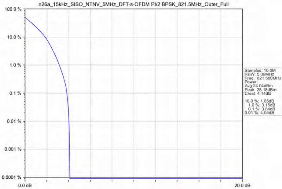
n26a_15kHz_SISO_NTNV_5MHz_DFT-s-OFDM PI/2 BPSK_821.5MHz_Outer_Full
