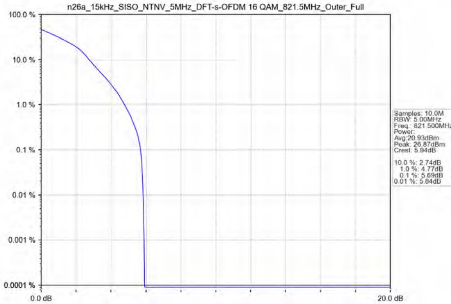
n26a_15kHz_SISO_NTNV_5MHz_DFT-s-OFDM 16 QAM_821.5MHz_Outer_Full
