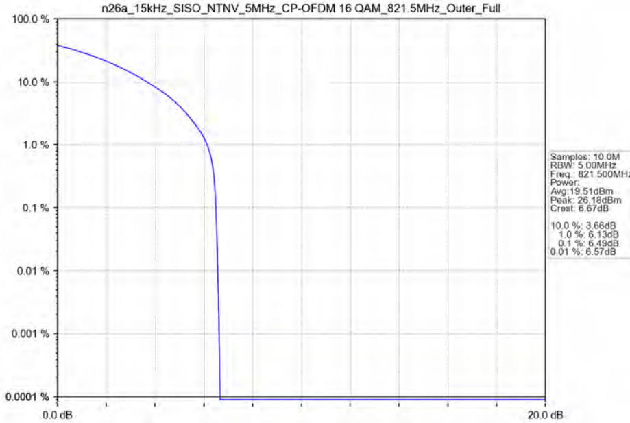
n26a_15kHz_SISO_NTNV_5MHz_CP-OFDM 16 QAM_ 821.5MHz_ Outer_Full
