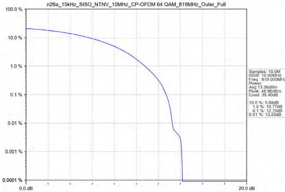
n26a_15kHz_SISO_NTNV_10MHz_CP-OFDM 64 QAM_819MHz_Outer_Full
