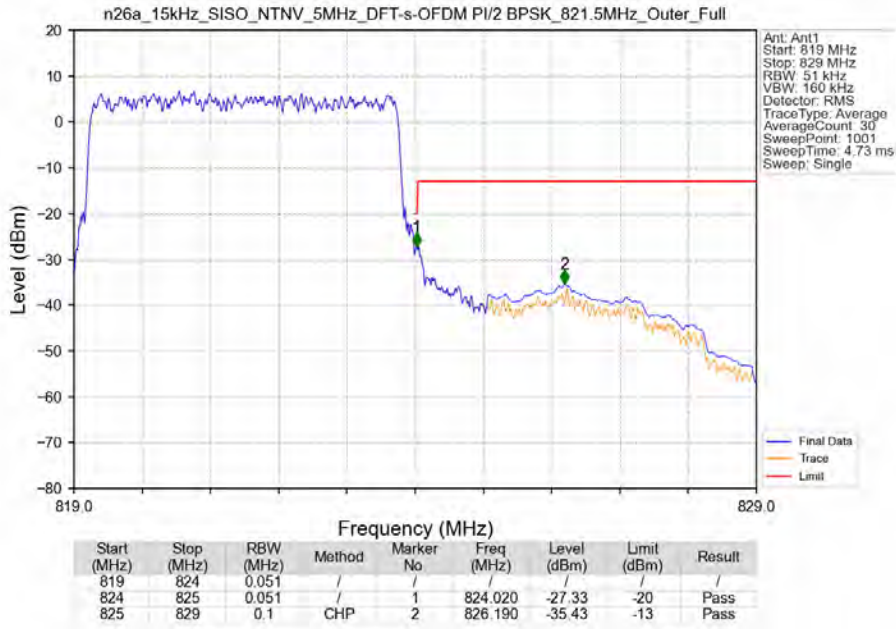
n26a_15kHz_SISO_NTNV_5MHz_DFT-s-OFDM PI/2 BPSK_821.5MHz_Outer_Full
