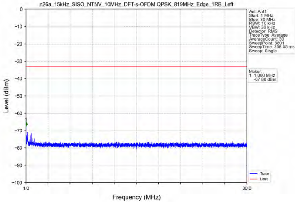
n26a_15kHz_SISO_NTNV_10MHz_DFT-s-OFDM QPSK_819MHz_Edge_1RB_Left
