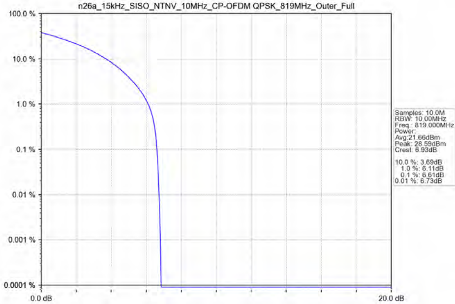
n26a_15kHz_SISO_NTNV_10MHz_CP-OFDM QPSK_819MHz_Outer_Full
