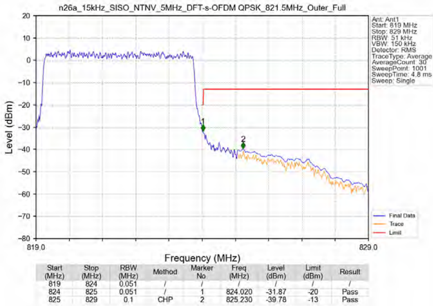
n26a_15kHz_SISO_NTNV_5MHz_DFT-s-OFDM QPSK_821.5MHz_Outer_Full
