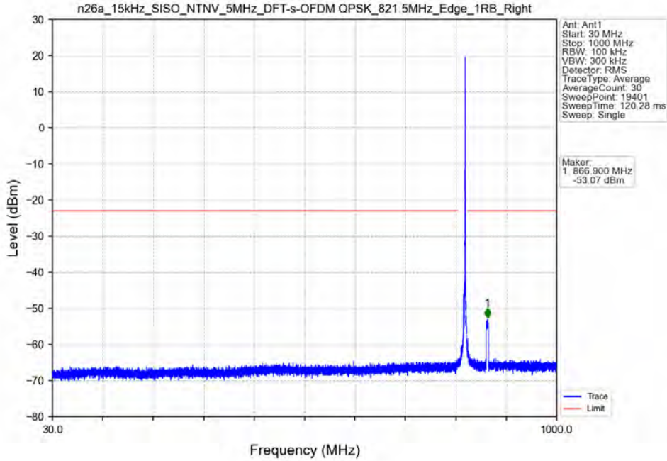
n26a_15kHz_SISO_NTNV_5MHz_DFT-s-OFDM QPSK_821.5MHz_Edge_1RB_Right
