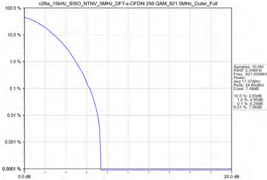
n26a_15kHz_SISO_NTNV_5MHz_DFT-s-OFDM_256_QAM_821.5MHz_Outer_Full
