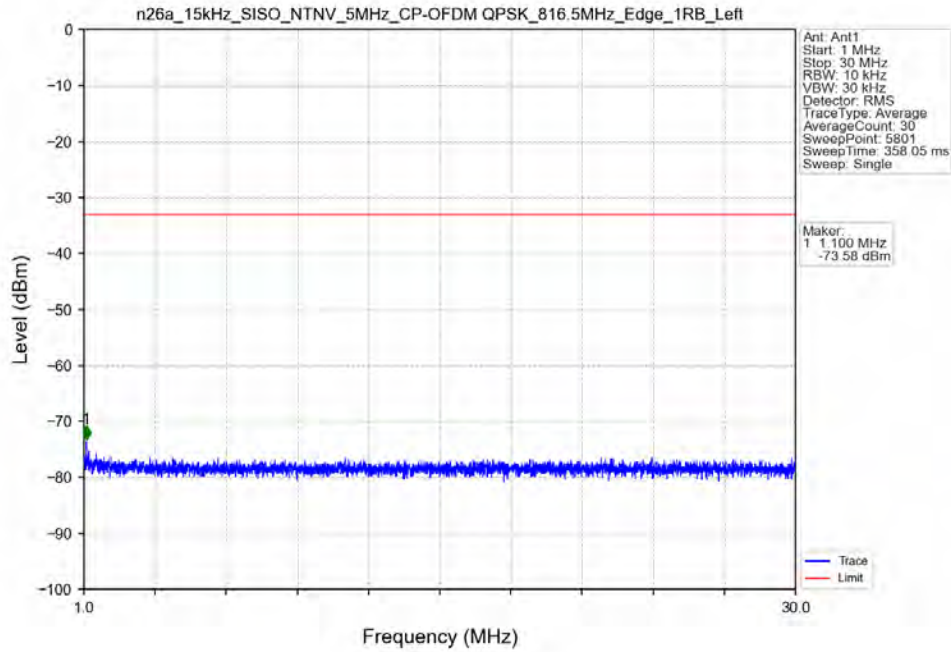
n26a_15kHz_SISO_NTNV_5MHz_CP-OFDM QPSK_816.5MHz_Edge_1RB_Left
