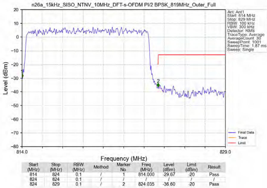
n26a_15kHz_SISO_NTNV_10MHz_DFT-s-OFDM PI/2 BPSK_819MHz_Outer_Full
