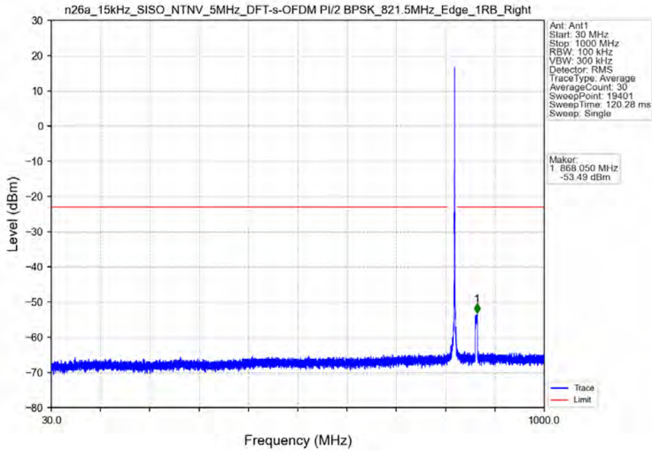
n26a_15kHz_SISO_NTNV_5MHz_DFT-s-OFDM PI/2 BPSK_821.5MHz_Edge_1RB_Right
