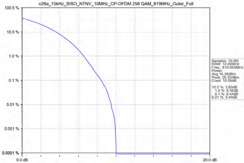
n26a_15kHz_SISO_NTNV_10MHz_CP-OFDM_256_QAM_819MHz_Outer_Full
