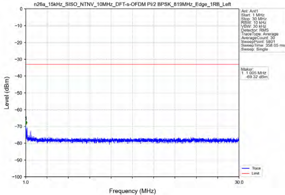
n26a_15kHz_SISO_NTNV_10MHz_DFT-s-OFDM PI/2 BPSK_819MHz_Edge_1RB_Left
