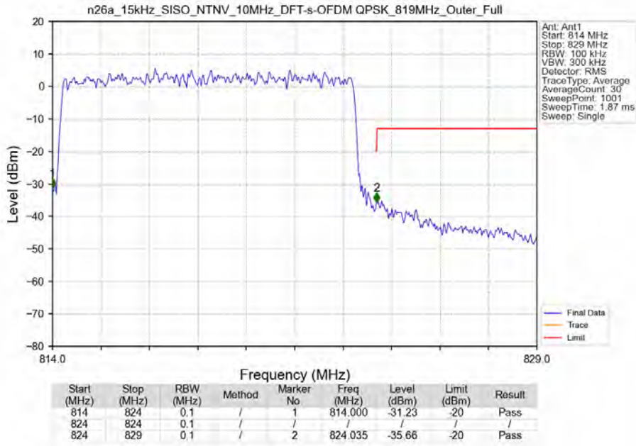
n26a_15kHz_SISO_NTNV_10MHz_DFT-s-OFDM_QPSK_819MHz_Outer_Full
