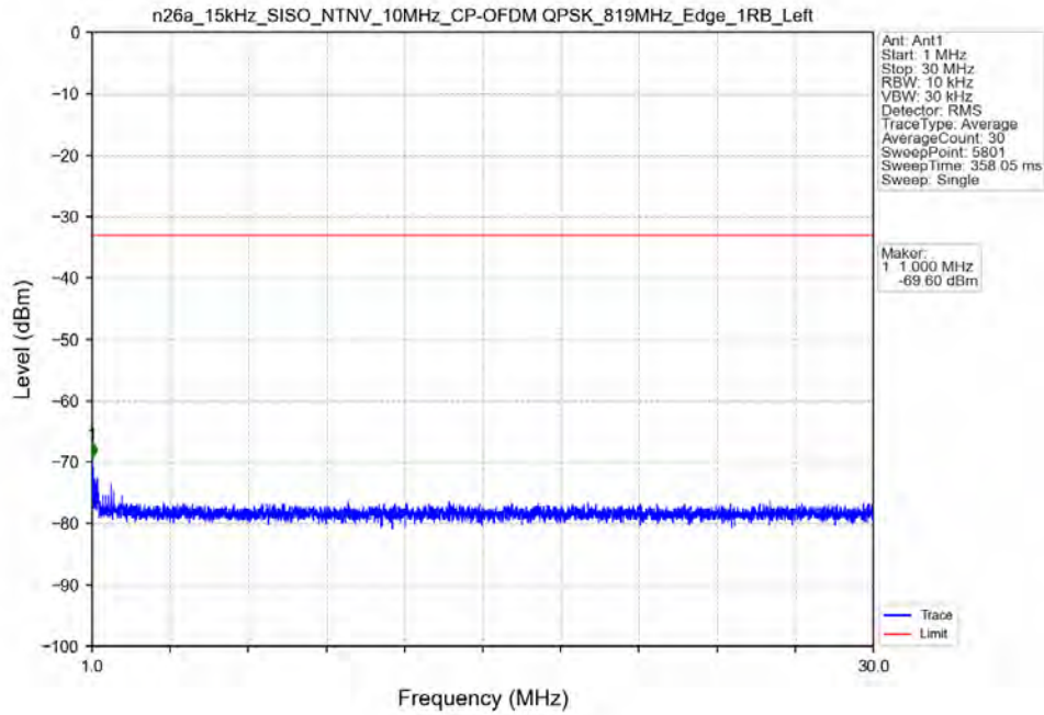
n26a_15kHz_SISO_NTNV_10MHz_CP-OFDM QPSK_819MHz_Edge_1RB_Left
