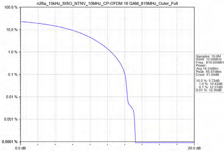
n26a_15kHz_SISO_NTNV_10MHz_CP-OFDM 16 QAM_819MHz_Outer_Full
