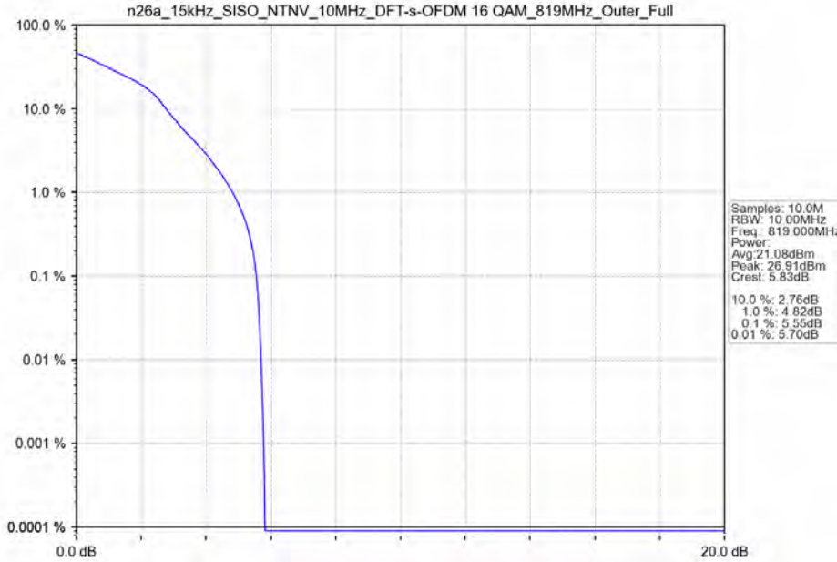
n26a_15kHz_SISO_NTNV_10MHz_DFT-s-OFDM 16 QAM_819MHz_Outer_Full
