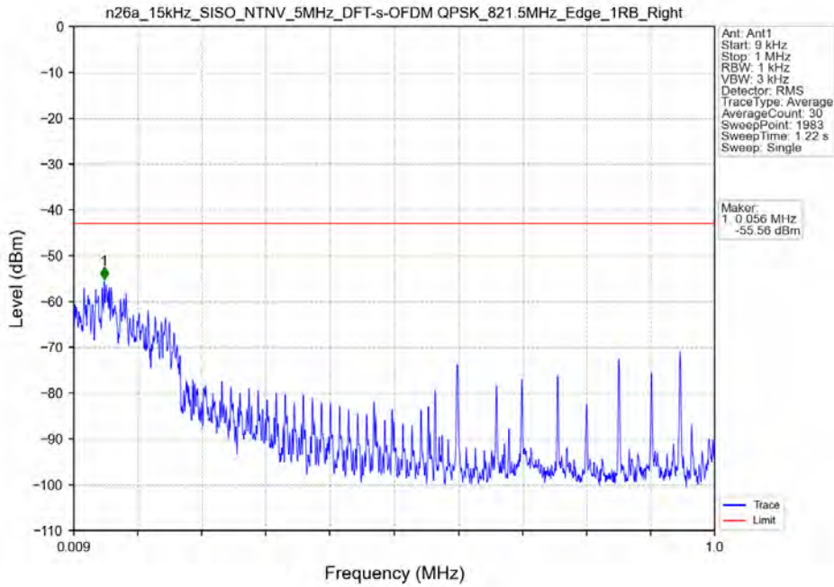
n26a_15kHz_SISO_NTNV_5MHz_DFT-s-OFDM QPSK_821.5MHz_Edge_1RB_Right
