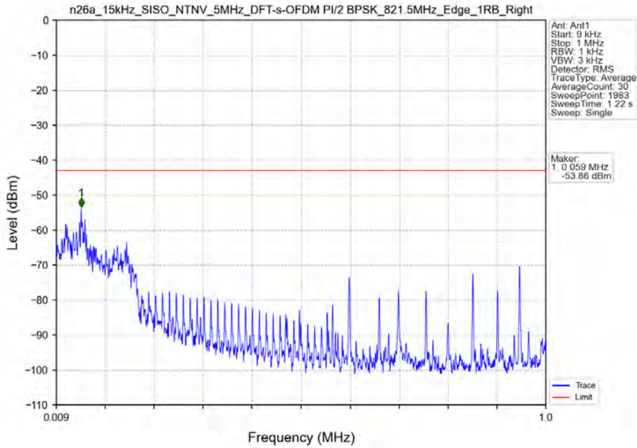
n26a_15kHz_SISO_NTNV_5MHz_DFT-s-OFDM PI/2 BPSK_821.5MHz_Edge_1RB_Right
