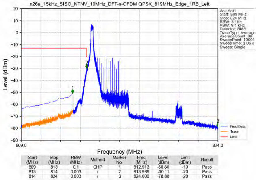
n26a_15kHz_SISO_NTNV_10MHz_DFT-s-OFDM QPSK_819MHz_Edge_1RB_Left
