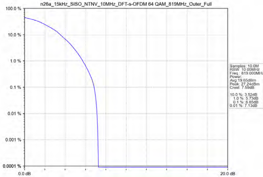
n26a_15kHz_SISO_NTNV_10MHz_DFT-s-OFDM 64 QAM_819MHz_Outer_Full
