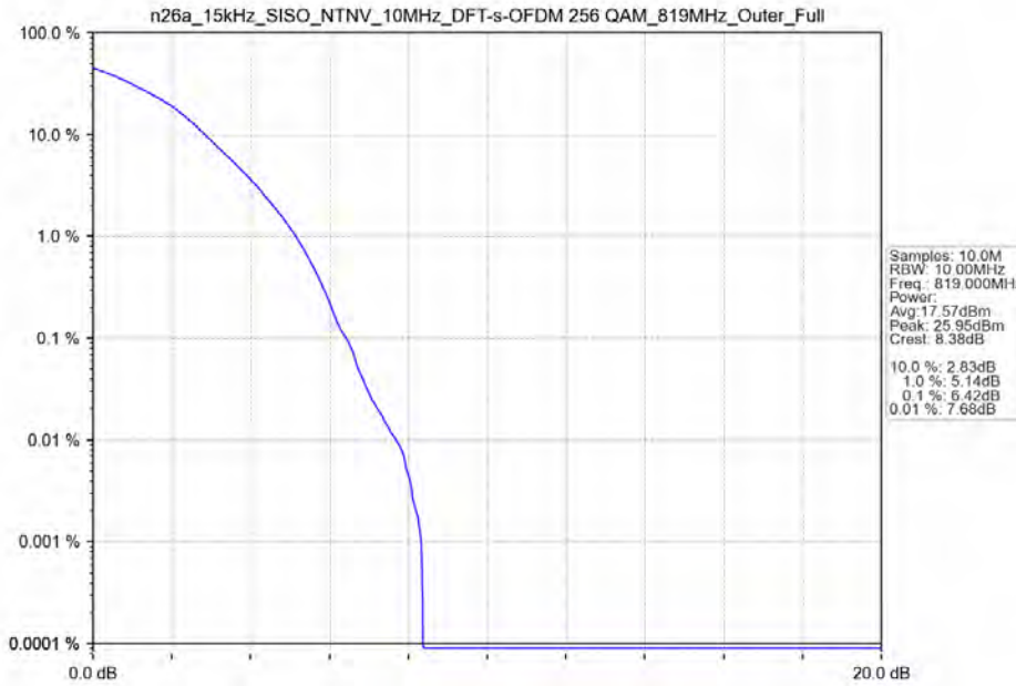
n26a_15kHz_SISO_NTNV_10MHz_DFT-s-OFDM 256 QAM_819MHz_Outer_Full
