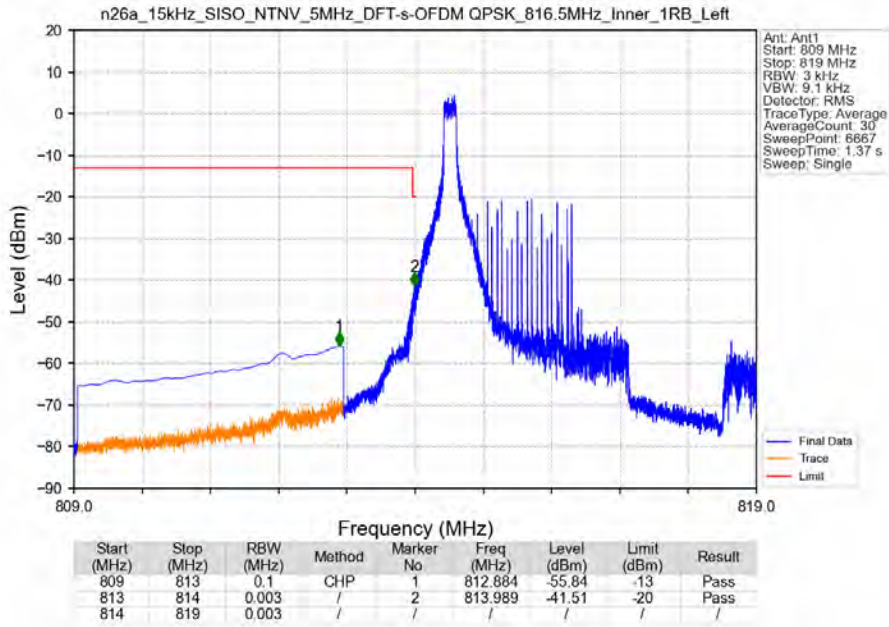
n26a_15kHz_SISO_NTNV_5MHz_DFT-s-OFDM QPSK_816.5MHz_Inner_1RB_Left
