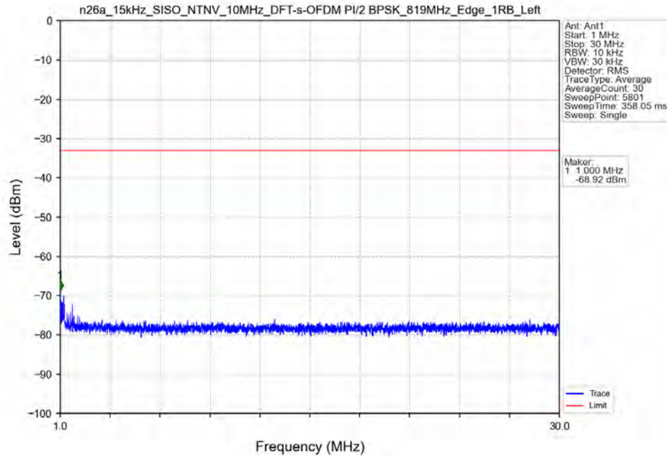
n26a_15kHz_SISO_NTNV_10MHz_DFT-s-OFDM_PI/2_BPSK_819MHz_Edge_1RB_Left
