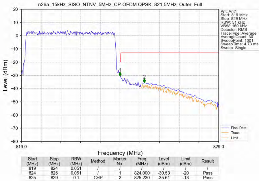
n26a_15kHz_SISO_NTNV_5MHz_CP-OFDM QPSK_821.5MHz_Outer_Full
