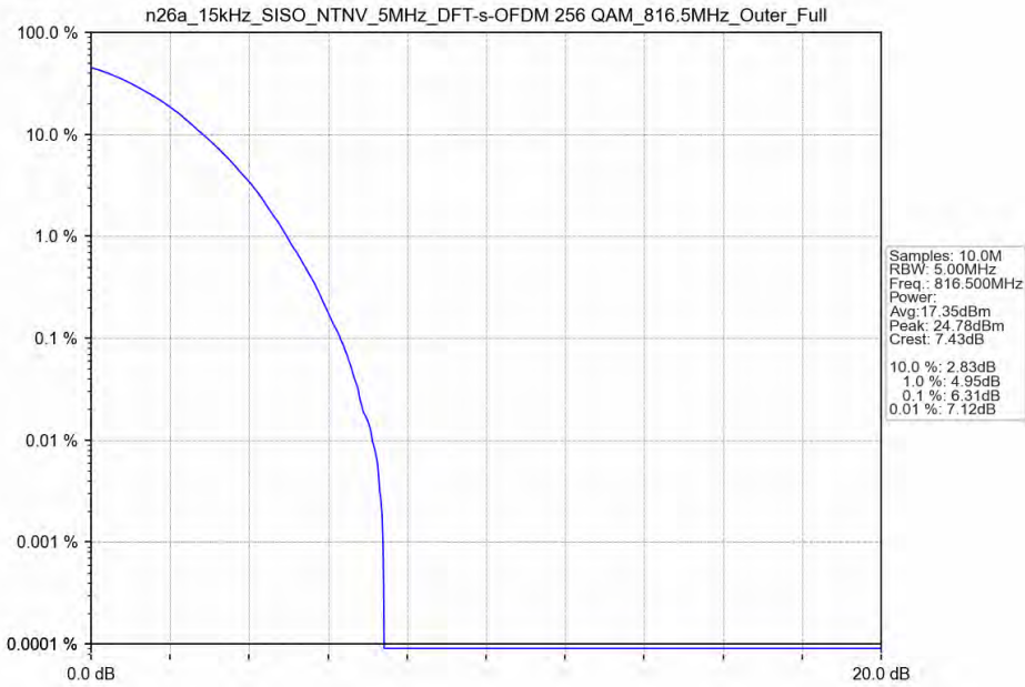
n26a_15kHz_SISO_NTNV_5MHz_DFT-s-OFDM_256_QAM_816.5MHz_Outer_Full
