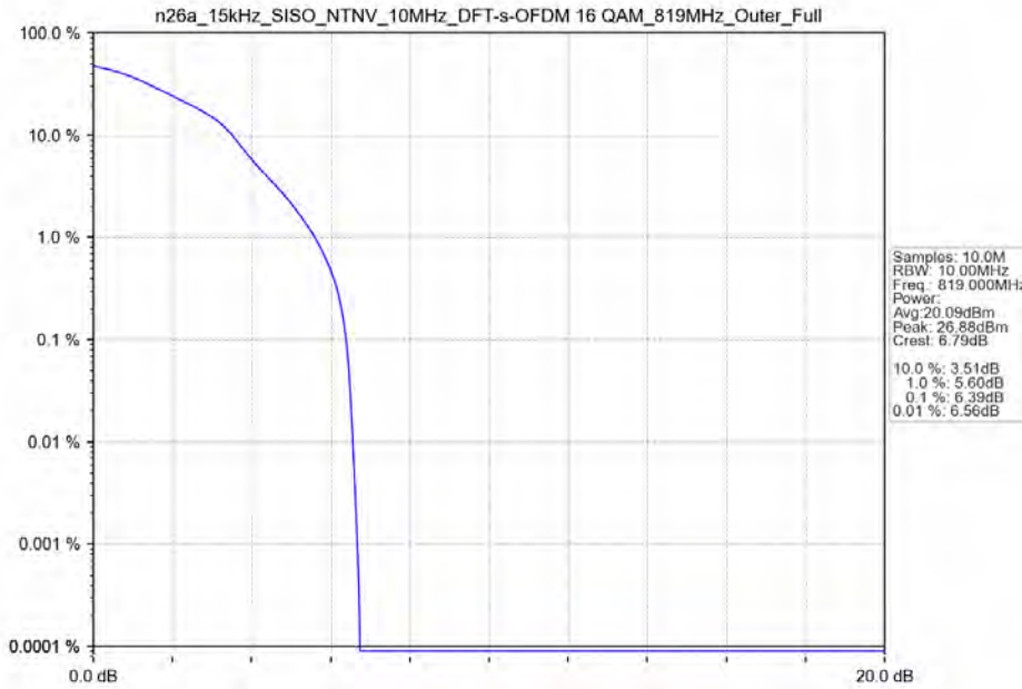
n26a_15kHz_SISO_NTNV_10MHz_DFT-s-OFDM_16_QAM_819MHz_Outer_Full
