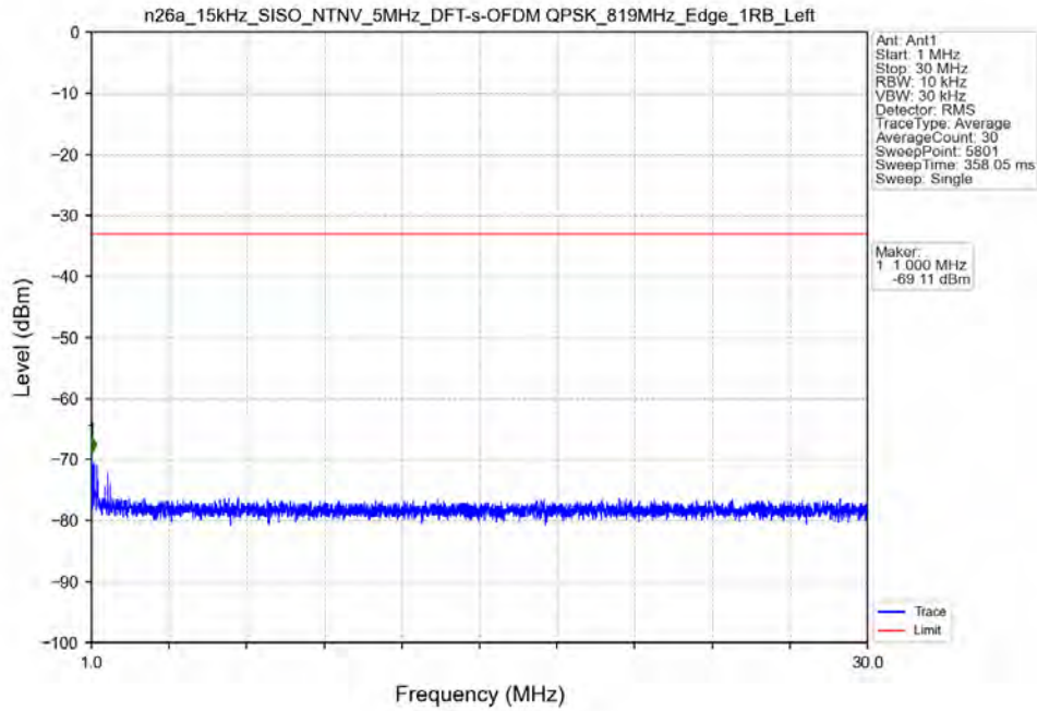
n26a_15kHz_SISO_NTNV_5MHz_DFT-s-OFDM_QPSK_819MHz_Edge_1RB_Left
