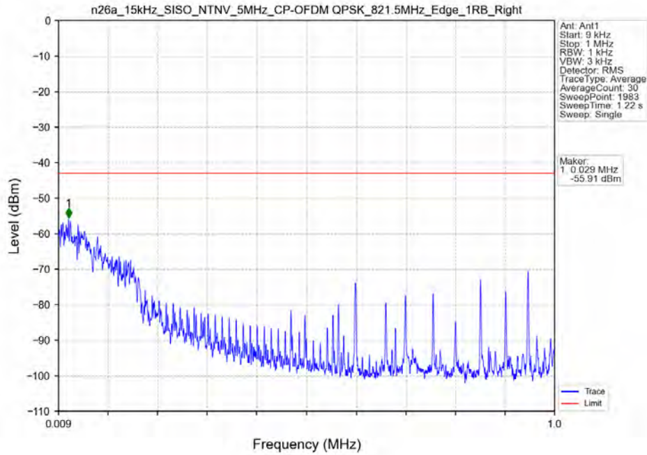
n26a_15kHz_SISO_NTNV_5MHz_CP-OFDM QPSK_821.5MHz_Edge_1RB_Right
