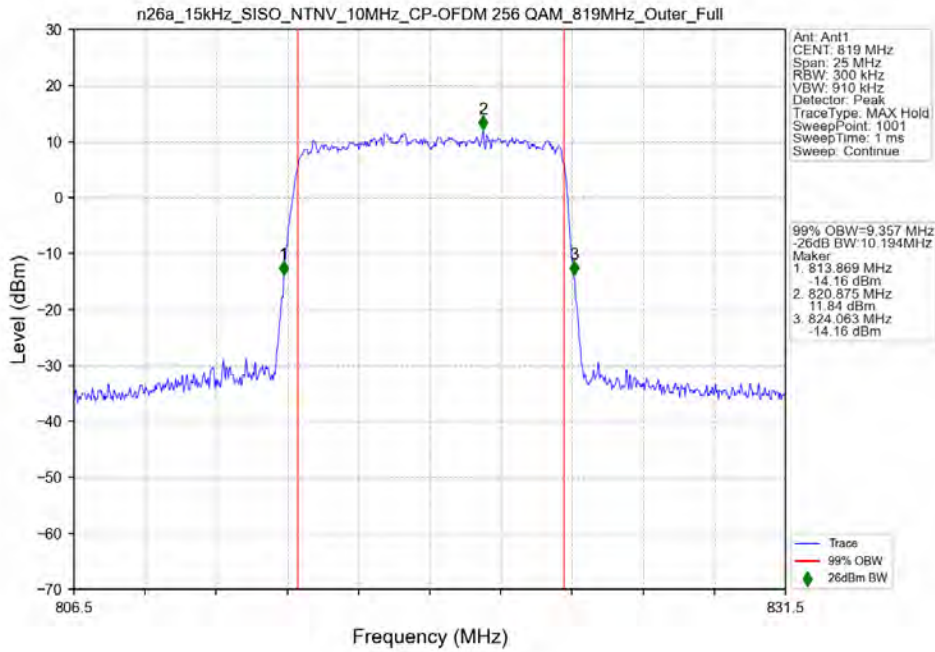
n26a_15kHz_SISO_NTNV_10MHz_CP-OFDM 256 QAM_819MHz_Outer_Full
