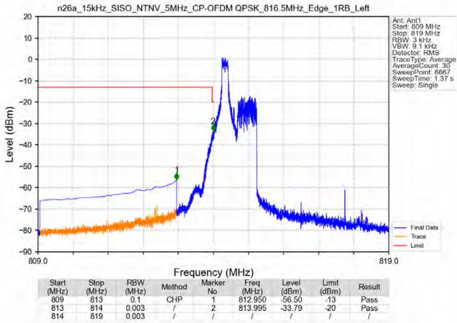
n26a_15kHz_SISO_NTNV_5MHz_CP-OFDM QPSK_816.5MHz_Edge_1RB_Left
