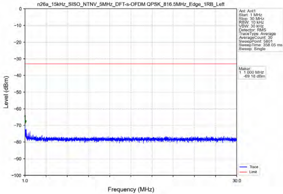
n26a_15kHz_SISO_NTNV_5MHz_DFT-s-OFDM_QPSK_816.5MHz_Edge_1RB_Left
