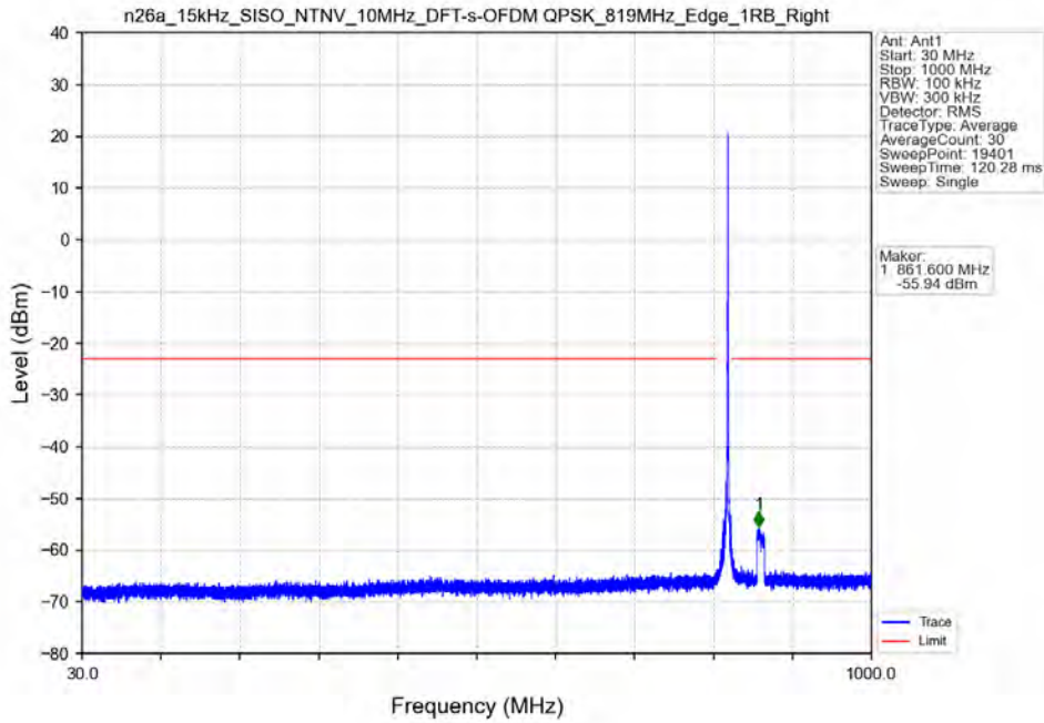
n26a_15kHz_SISO_NTNV_10MHz_DFT-s-OFDM_QPSK_819MHz_Edge_1RB_Right
