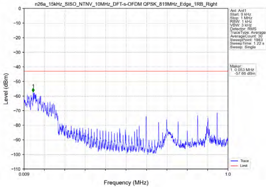
n26a_15kHz_SISO_NTNV_10MHz_DFT-s-OFDM_QPSK_819MHz_Edge_1RB_Right
