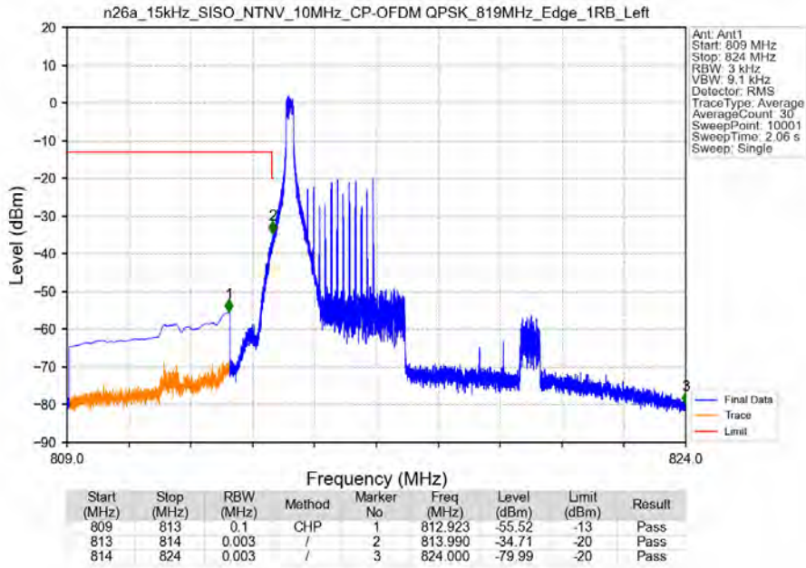
n26a_15kHz_SISO_NTNV_10MHz_CP-OFDM QPSK_819MHz_Edge_1RB_Left
