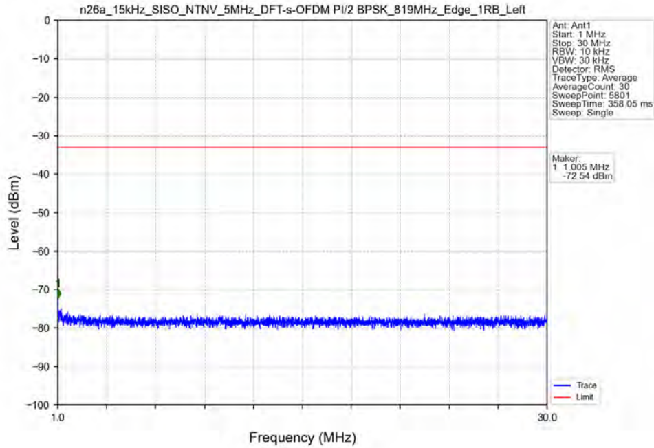
n26a_15kHz_SISO_NTNV_5MHz_DFT-s-OFDM PI/2 BPSK_819MHz_Edge_1RB_Left
