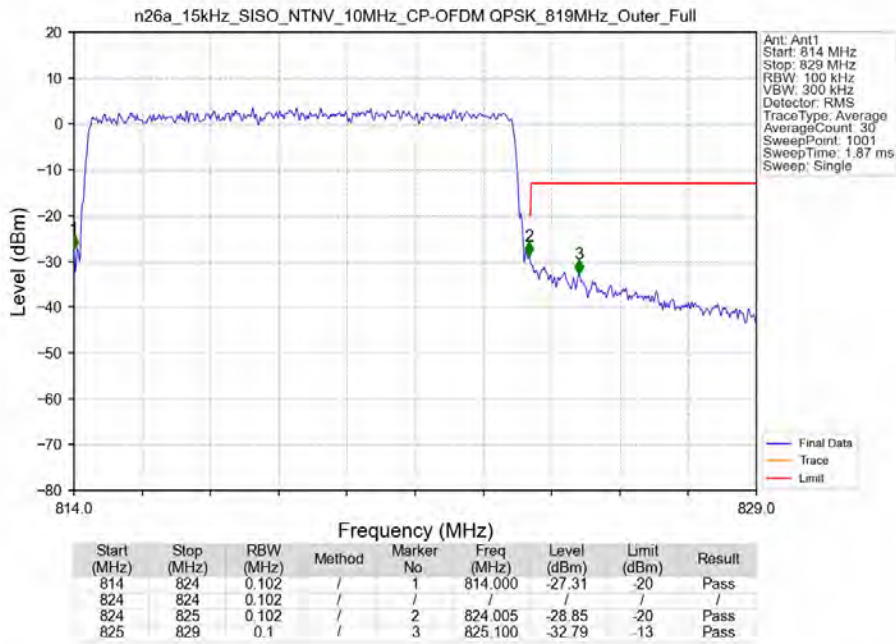
n26a_15kHz_SISO_NTNV_10MHz_CP-OFDM_QPSK_819MHz_Outer_Full
