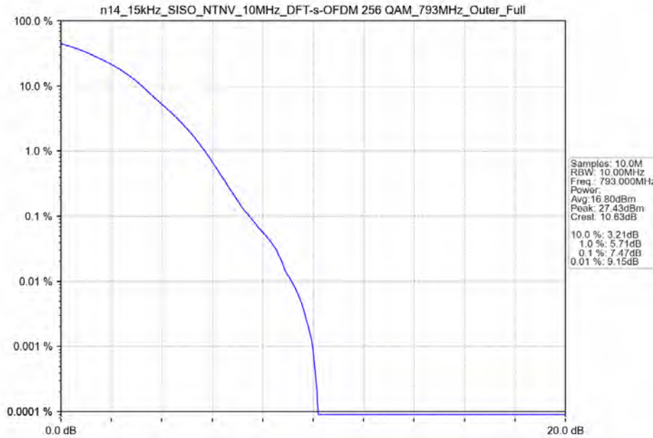
n14_15kHz_SISO_NTNV_10MHz_DFT-s-OFDM 256 QAM_793MHz_Outer_Full
