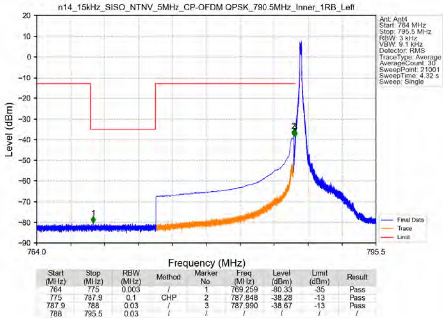
n14_15kHz_SISO_NTNV_5MHz_CP-OFDM QPSK_790.5MHz_Inner_1RB_Left
