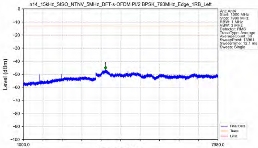
n14_15kHz_SISO_NTNV_5MHz_DFT-s-OFDM PI/2 BPSK_793MHz_Edge_1RB_Left
