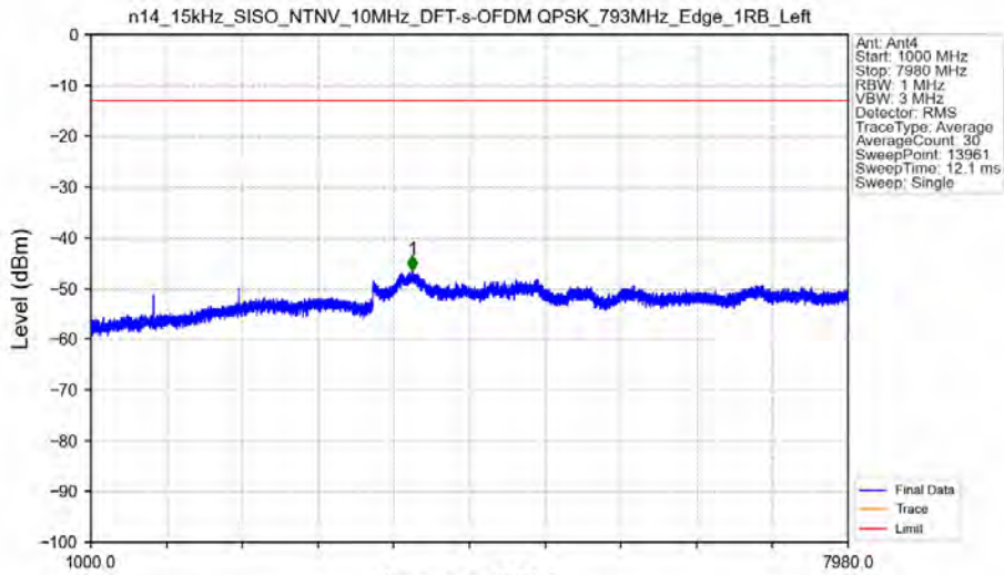
n14_15kHz_SISO_NTNV_10MHz_DFT-s-OFDM_QPSK_793MHz_Edge_1RB_Left
