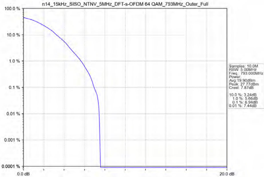
n14_15kHz_SISO_NTNV_5MHz_DFT-s-OFDM 64 QAM_793MHz_Outer_Full
