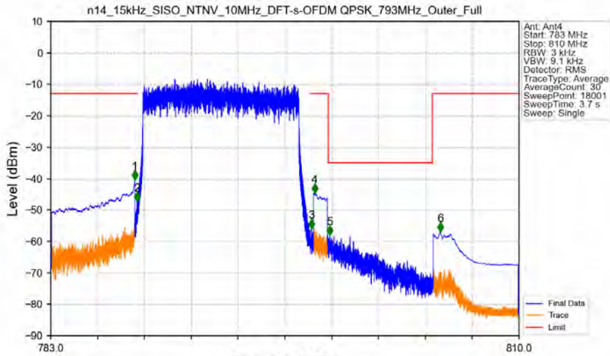
n14_15kHz_SISO_NTNV_10MHz_DFT-s-OFDM QPSK_793MHz_Outer_Full
