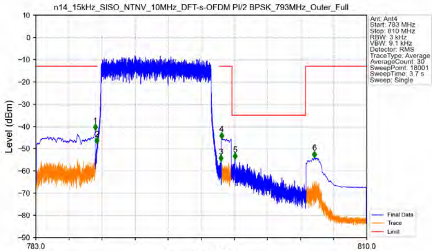
n14_15kHz_SISO_NTNV_10MHz_DFT-s-OFDM PI/2 BPSK_793MHz_Outer_Full
