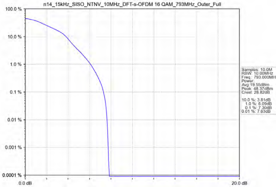
n14_15kHz_SISO_NTNV_10MHz_DFT-s-OFDM 16 QAM_793MHz_Outer_Full
