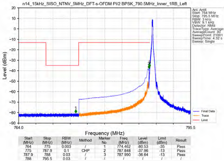
n14_15kHz_SISO_NTNV_5MHz_DFT-s-OFDM PI/2 BPSK_790.5MHz_Inner_1RB_Left
