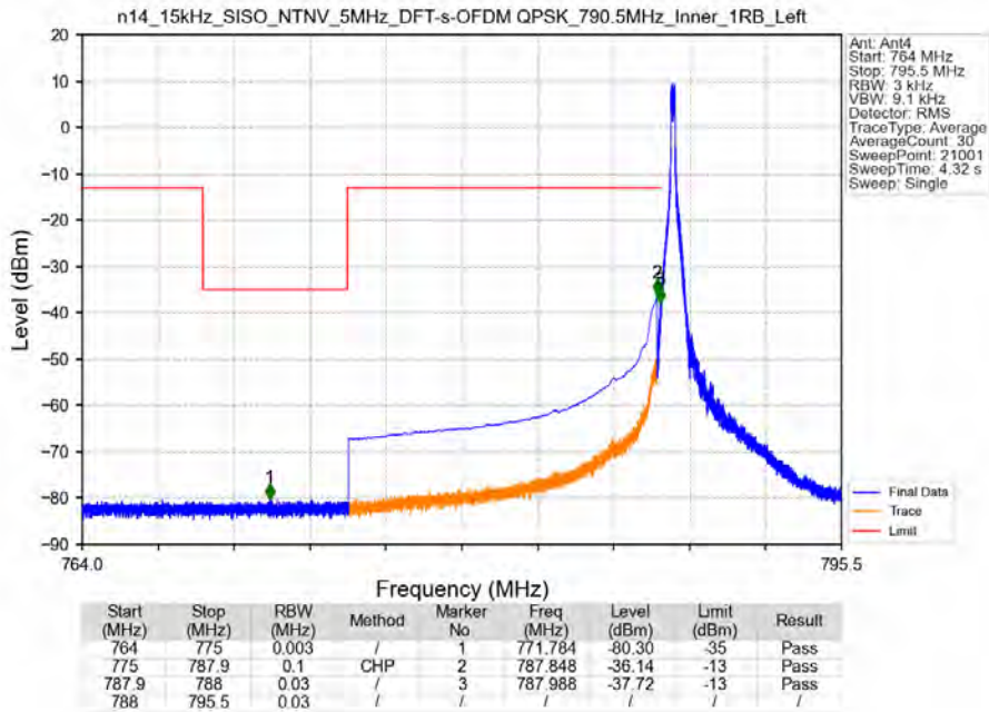
n14_15kHz_SISO_NTNV_5MHz_DFT-s-OFDM QPSK_790.5MHz_Inner_1RB_Left
