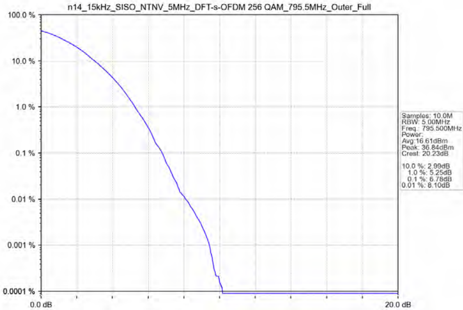
n14_15kHz_SISO_NTNV_5MHz_DFT-s-OFDM 256 QAM_795.5MHz_Outer_Full
