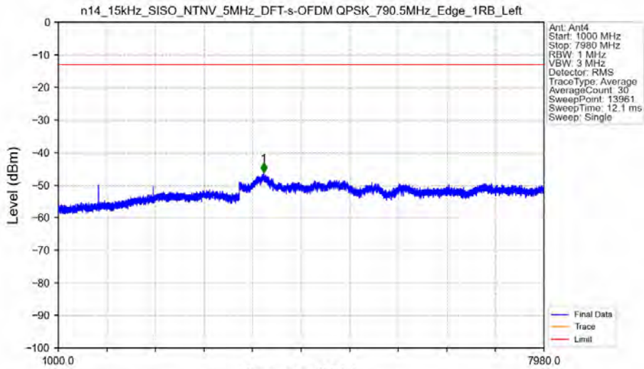
n14_15kHz_SISO_NTNV_5MHz_DFT-s-OFDM QPSK_790.5MHz_Edge_1RB_Left
