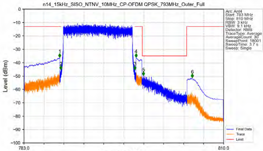
n14_15kHz_SISO_NTNV_10MHz_CP-OFDM QPSK_793MHz_Outer_Full
