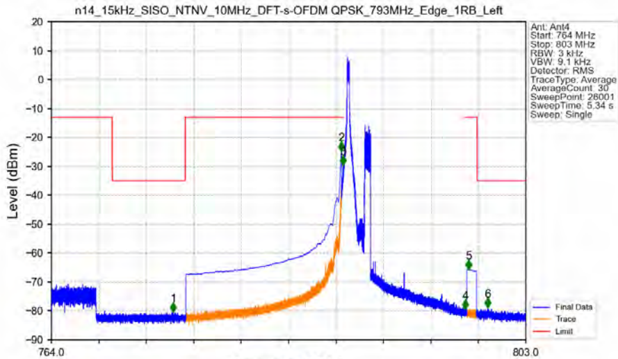
n14_15kHz_SISO_NTNV_10MHz_DFT-s-OFDM_QPSK_793MHz_Edge_1RB_Left
