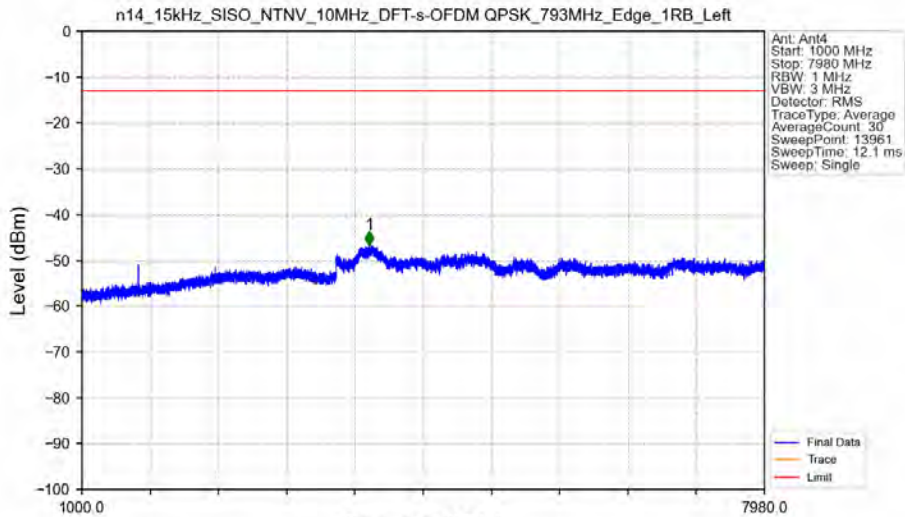
n14_15kHz_SISO_NTNV_10MHz_DFT-s-OFDM_QPSK_793MHz_Edge_1RB_Left
