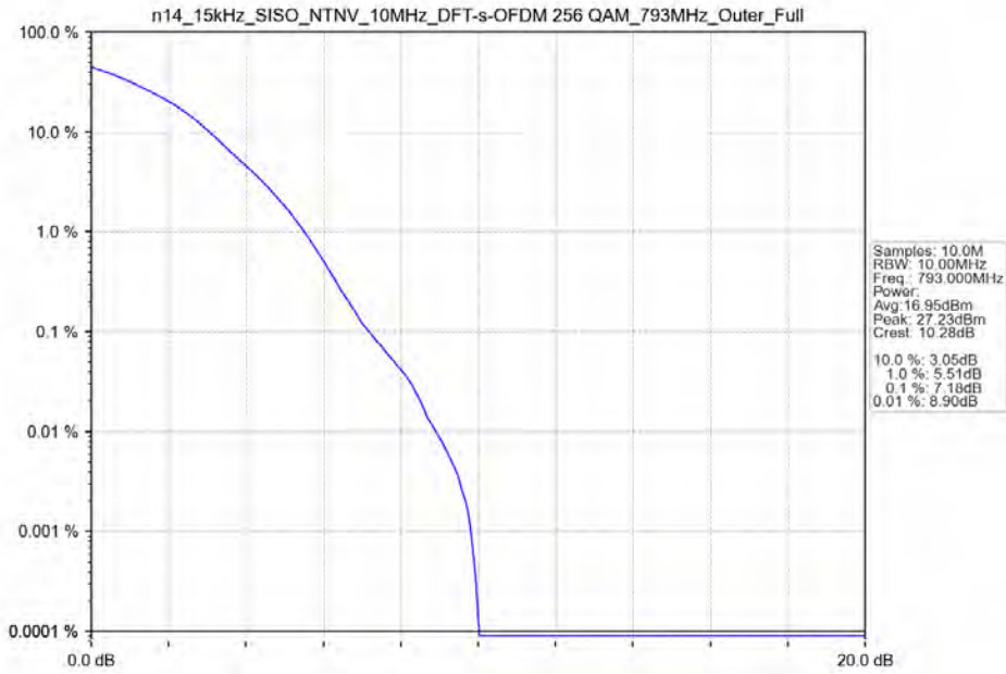
n14_15kHz_SISO_NTNV_10MHz_DFT-s-OFDM 256 QAM_793MHz_Outer_Full
