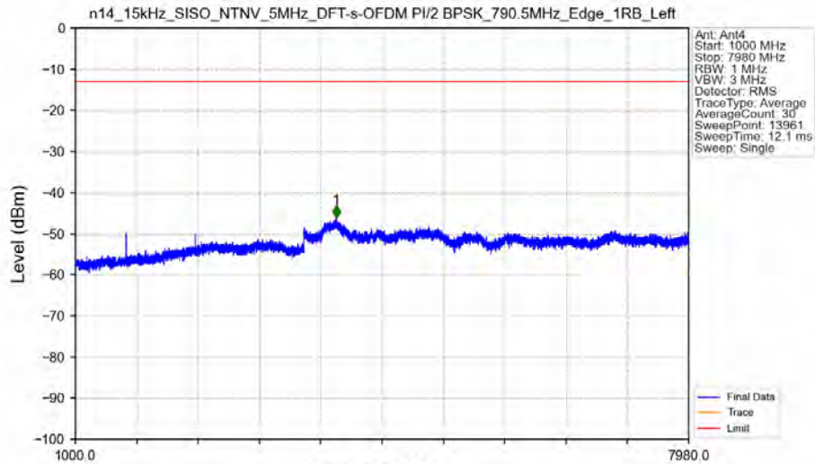
n14_15kHz_SISO_NTNV_5MHz_DFT-s-OFDM PI/2 BPSK_790.5MHz_Edge_1RB_Left
