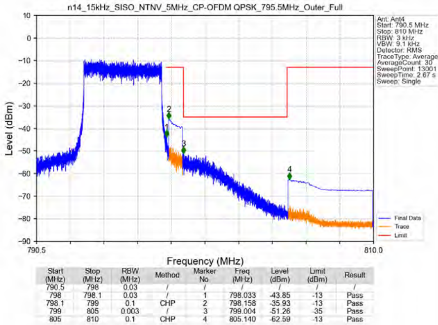
n14_15kHz_SISO_NTNV_5MHz_CP-OFDM QPSK_795.5MHz_Outer_Full
