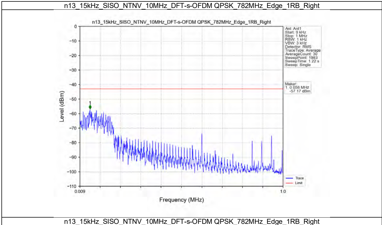
n13_15kHz_SISO_NTNV_10MHz_DFT-s-OFDM_QPSK_782MHz_Edge_1RB_Right
