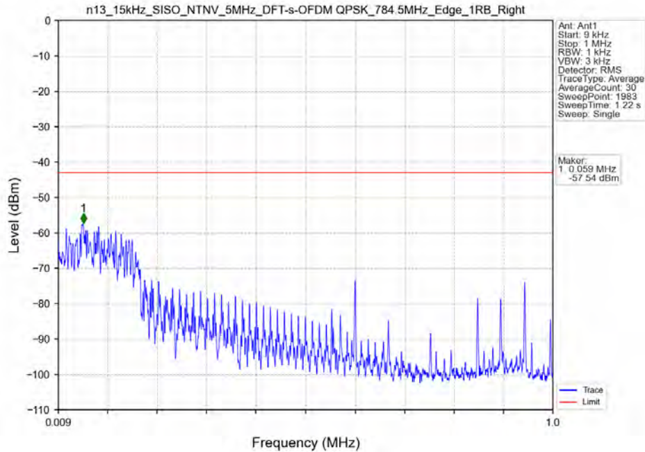
n13_15kHz_SISO_NTNV_5MHz_DFT-s-OFDM_QPSK_784.5MHz_Edge_1RB_Right
