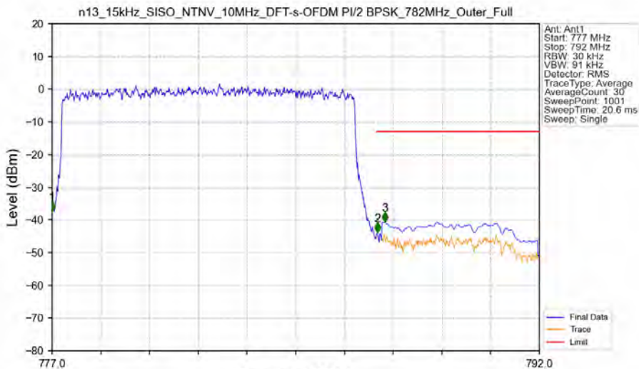
n13_15kHz_SISO_NTNV_10MHz_DFT-s-OFDM_PI/2_BPSK_782MHz_Outer_Full
