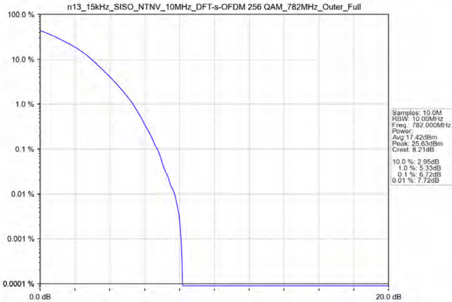
n13_15kHz_SISO_NTNV_10MHz_DFT-s-OFDM_256_QAM_782MHz_Outer_Full
