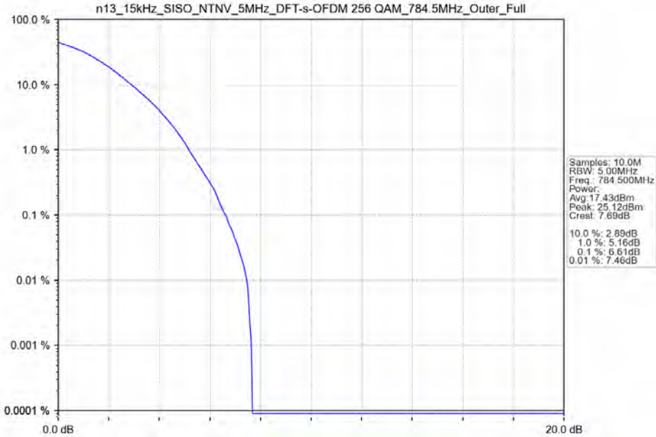
n13_15kHz_SISO_NTNV_5MHz_DFT-s-OFDM_256_QAM_784.5MHz_Outer_Full
