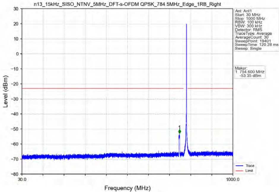
n13_15kHz_SISO_NTNV_5MHz_DFT-s-OFDM QPSK_784.5MHz_Edge_1RB_Right
