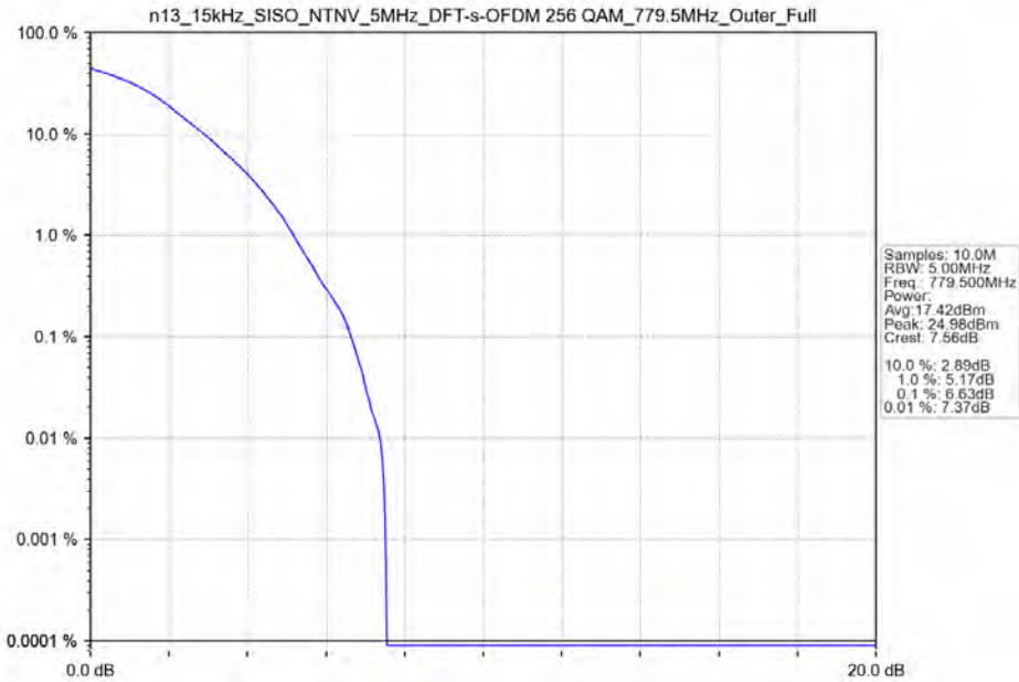
n13_15kHz_SISO_NTNV_5MHz_DFT-s-OFDM_256_QAM_779.5MHz_Outer_Full
