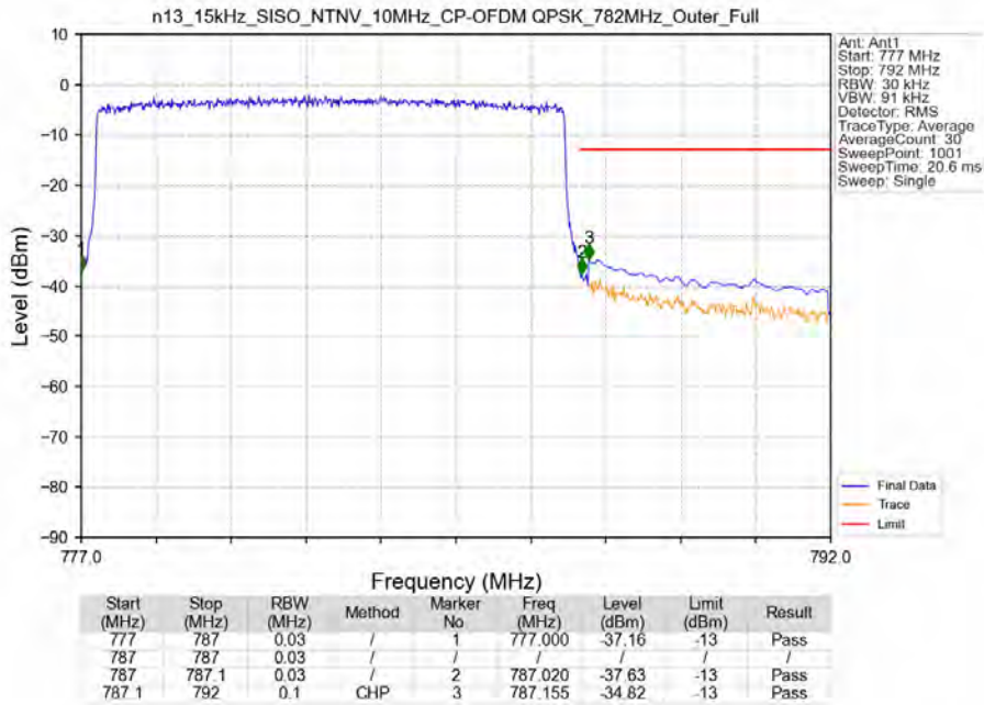
n13_15kHz_SISO_NTNV_10MHz_CP-OFDM_QPSK_782MHz_Outer_Full
