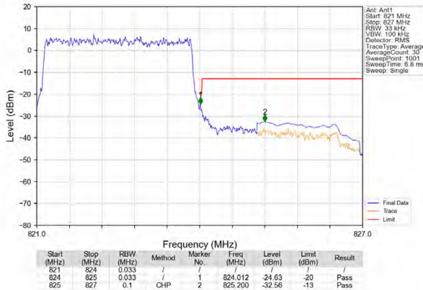
Band26a_3MHz_QPSK_HCH_822.5MHz_RB_15_0_NTV
