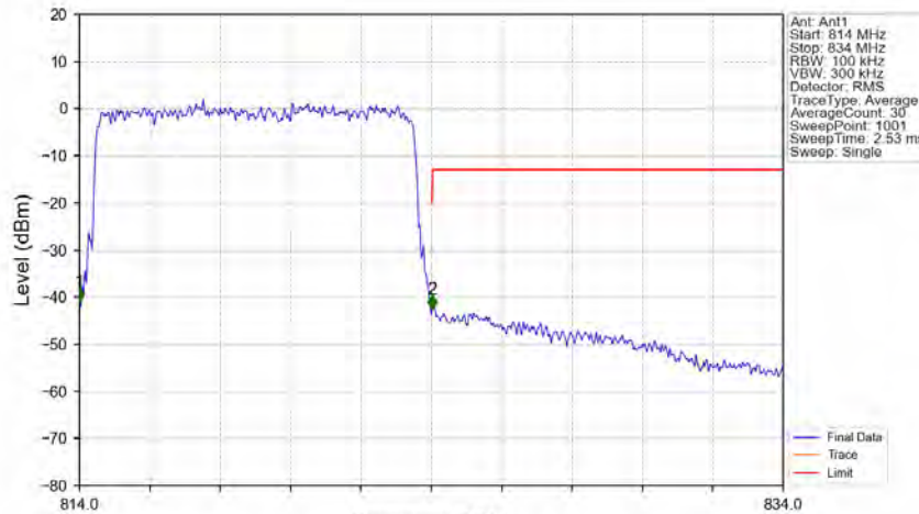
Band26a_10MHz_256QAM_MCH_819MHz_RB_50_0_NTNV
