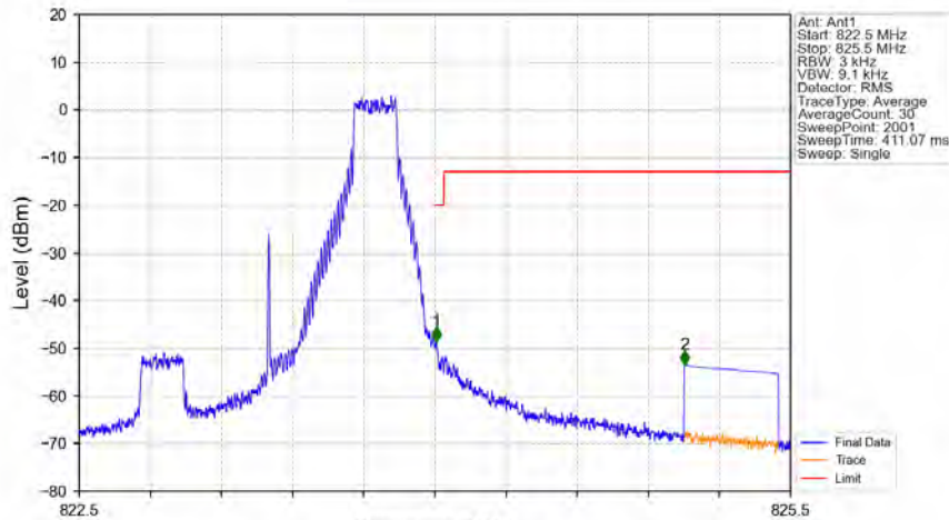
Band26a_1.4MHz_256QAM_HCH_823.3MHz_RB_1_5_NTNV
