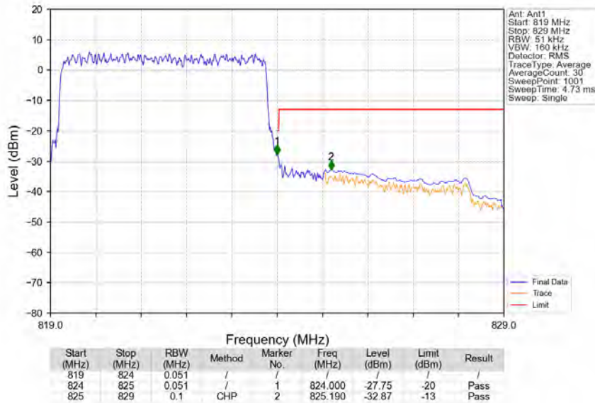
Band26a_5MHz_QPSK_HCH_821.5MHz_RB_25_0_NTNV
