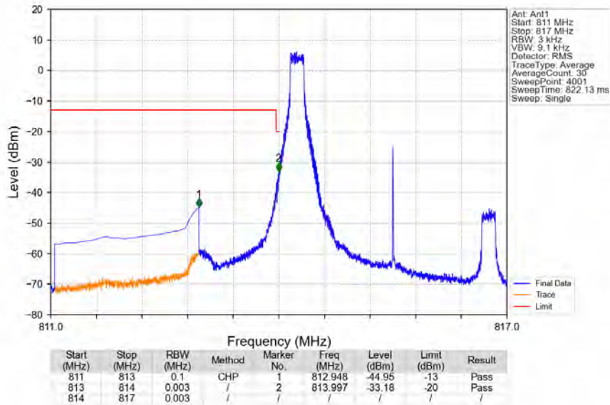
Band26a_3MHz_64QAM_LCH_815.5MHz_RB_1_0_NTNV
