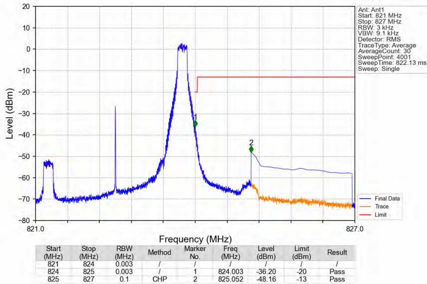
Band26a_3MHz_256QAM_HCH_822.5MHz_RB_1_14_NTNV
