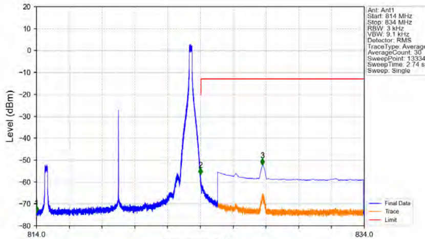
Band26a_10MHz_256QAM_HCH_819MHz_RB_1_49_NTNV
