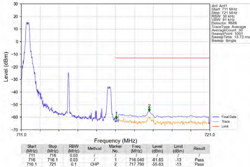
Band17 5MHz 64QAM HCH 713.5MHz RB 25 0 NTV
