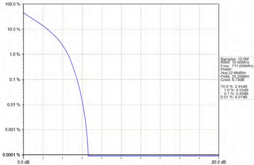
Band17 10MHz QPSK HCH 711MHz RB 50 0 NTV
