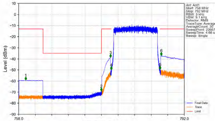
Band13_10MHz_64QAM_LCH_782MHz_RB_50_0_NTNV
