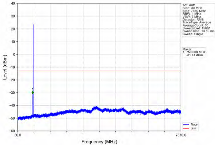
Band13_5MHz_16QAM_LCH_779.5MHz_RB_1_0_NTNV
