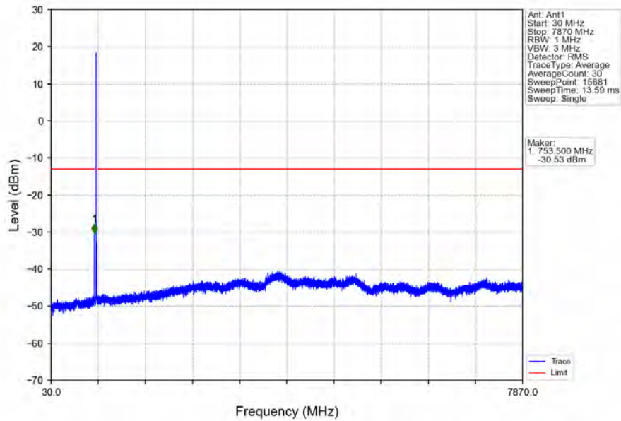
Band13_10MHz_256QAM_MCH_782MHz_RB_1_0_NTNV
