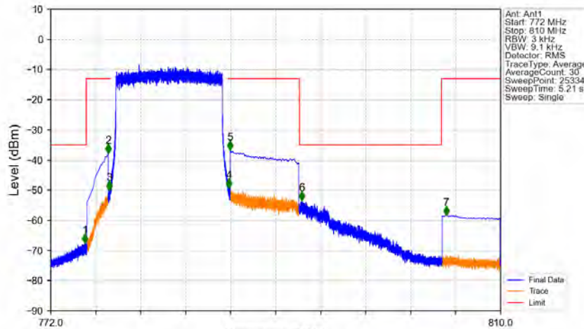
Band13_10MHz_16QAM_MCH_782MHz_RB_50_0_NTNV
