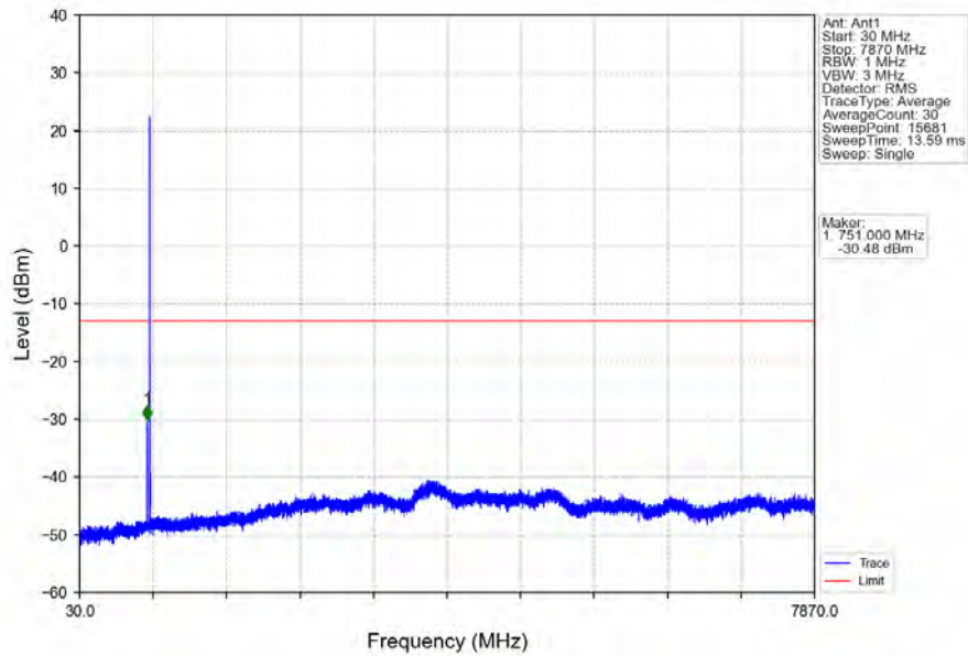
Band13_10MHz_16QAM_MCH_782MHz_RB_1_0_NTNV
