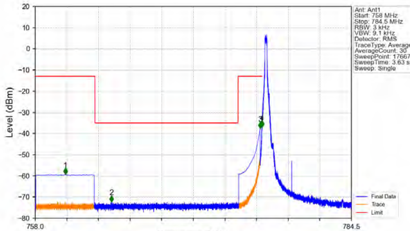
Band13_5MHz_64QAM_LCH_779.5MHz_RB_25_0_NTNV
