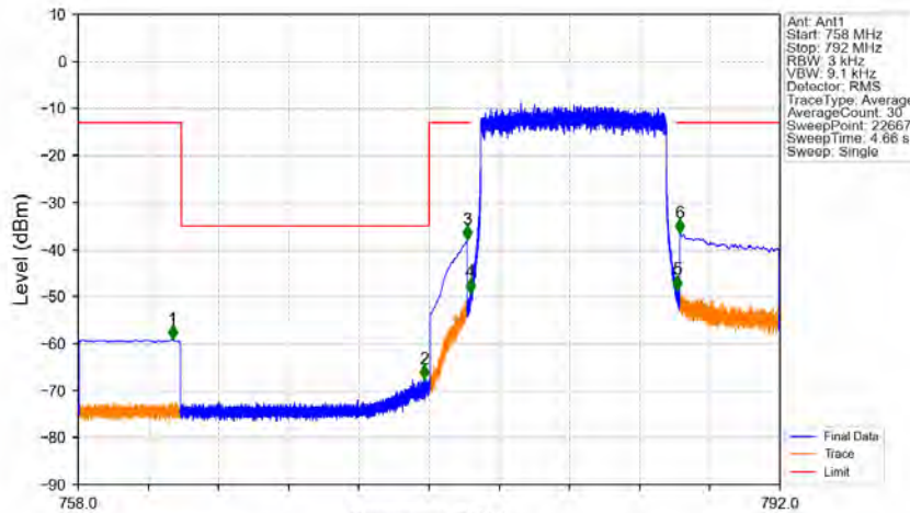
Band13_10MHz_16QAM_LCH_782MHz_RB_50_0_NTNV
