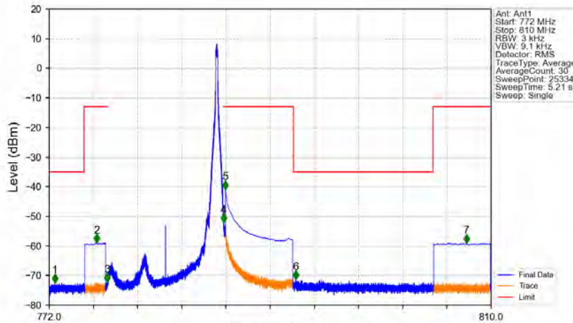
Band13_10MHz_16QAM_HCH_782MHz_RB_1_49_NTV
