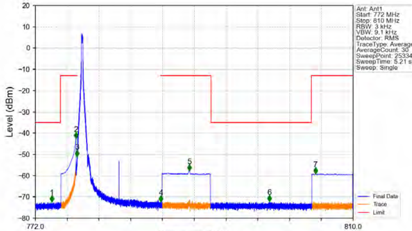
Band13_10MHz_64QAM_MCH_782MHz_RB_50_0_NTNV
