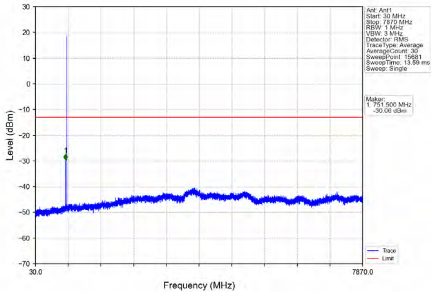
Band13_5MHz_256QAM_MCH_782MHz_RB_1_0_NTNV
