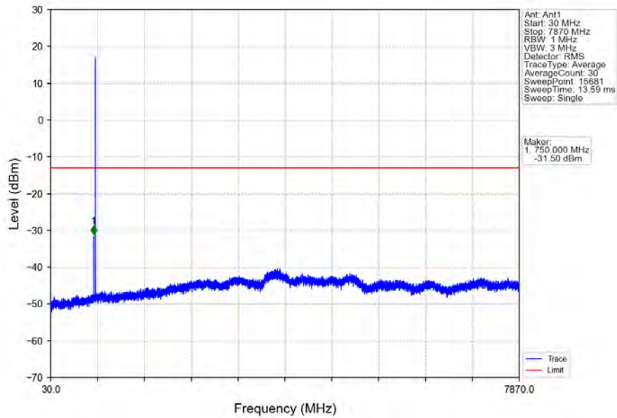
Band13_5MHz_256QAM_LCH_779.5MHz_RB_1_0_NTNV
