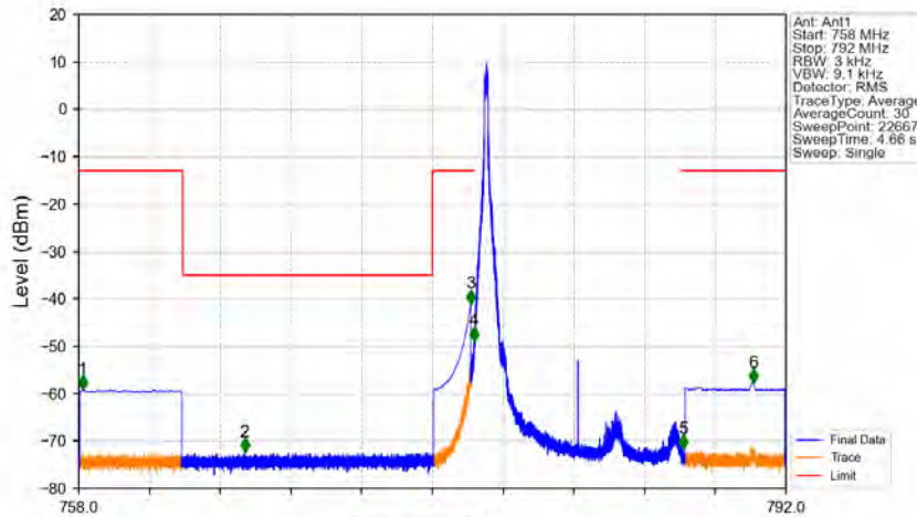
Band13 10MHz 16QAM LCH 782MHz RB 1 0 NTN
