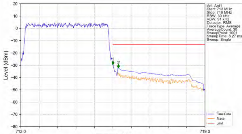
Band12_3MHz_QPSK_HCH_714.5MHz_RB_15_0_NTNV
