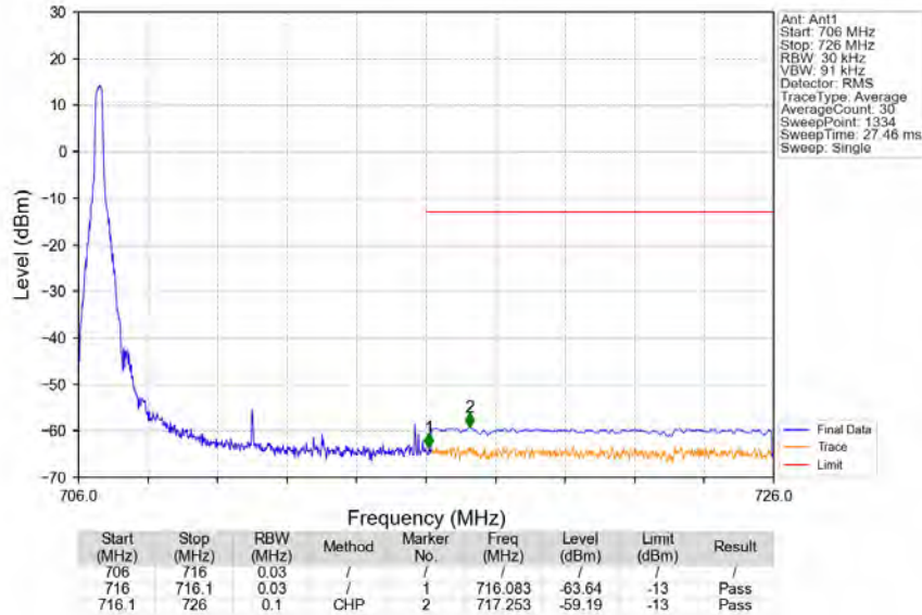
Band12_10MHz_64QAM_HCH_711MHz_RB_50_0_NTV
