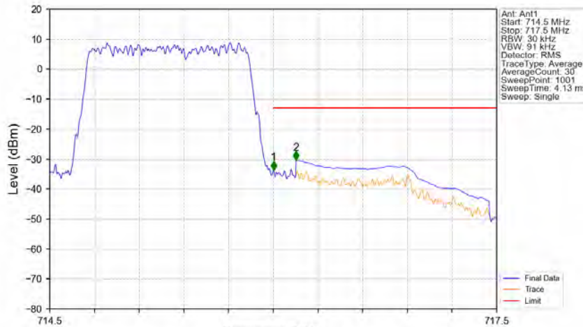
Band12_1.4MHz_QPSK_HCH_715.3MHz_RB_6_0_NTNV
