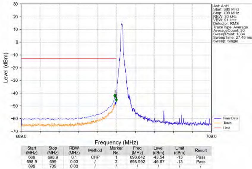
Band12_10MHz_64QAM_LCH_704MHz_RB_50_0_NTNV
