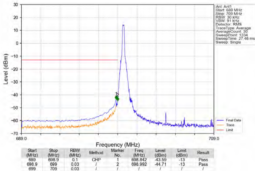
Band12_10MHz_64QAM_LCH_704MHz_RB_1_0_NTNV
