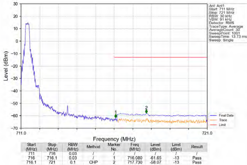
Band12_5MHz_64QAM_HCH_713.5MHz_RB_25_0_NTV
