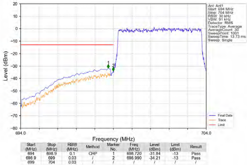
Band12_5MHz_64QAM_LCH_701.5MHz_RB_25_0_NTNV
