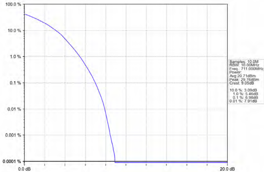
Band12_10MHz_64QAM_HCH_711MHz_RB_50_0_NTNV
