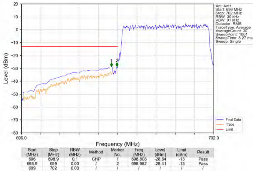
Band12_3MHz_QPSK_LCH_700.5MHz_RB_15_0_NTNV
