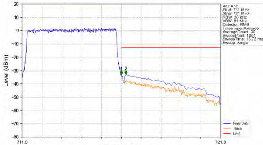
Band12_5MHz_QPSK_HCH_713.5MHz_RB_25_0_NTNV
