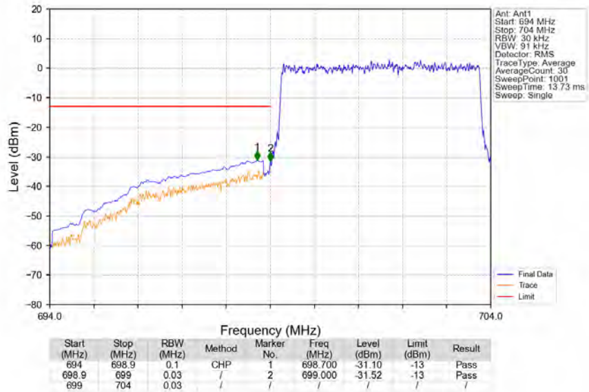
Band12_5MHz_QPSK_LCH_701.5MHz_RB_25_0_NTNV
