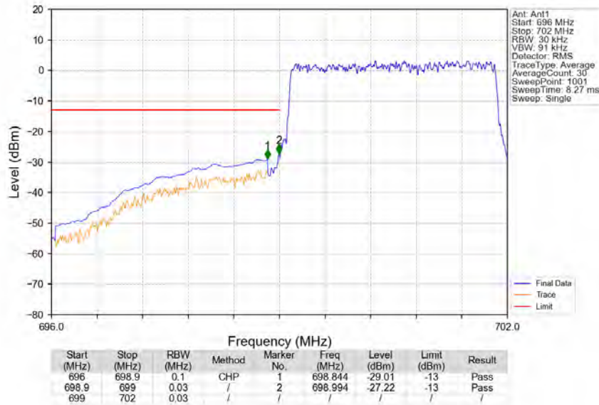
Band12_3MHz_64QAM_LCH_700.5MHz_RB_15_0_NTNV
