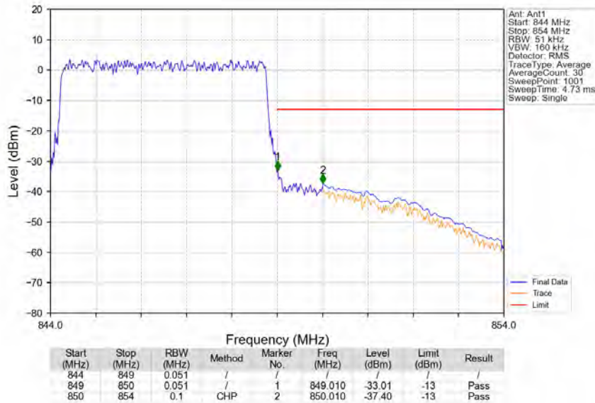
Band5_5MHz_64QAM_HCH_846.5MHz_RB_25_0_NTNV
