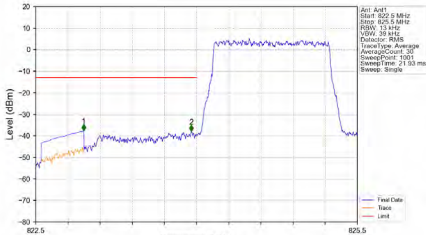
Band5 1.4MHz QPSK LCH 824.7MHz RB 6 0 NTN
