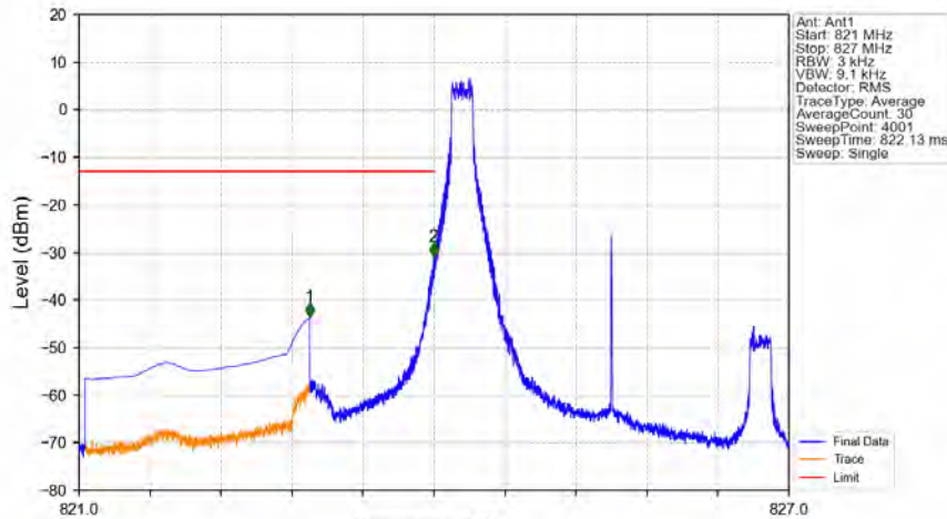
Band5_3MHz_64QAM_LCH_825.5MHz_RB_1_0_NTNV
