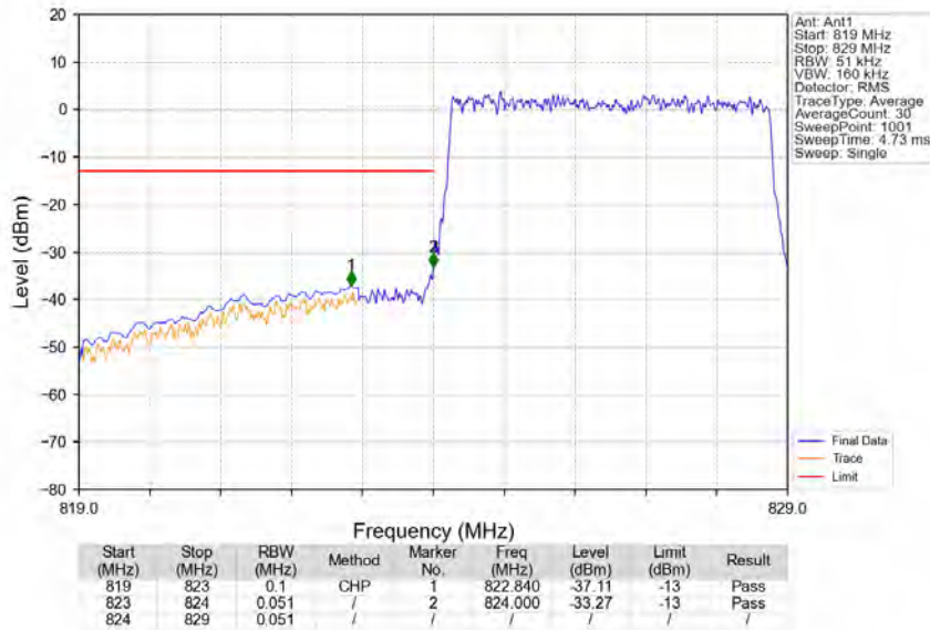
Band5_5MHz_64QAM_LCH_826.5MHz_RB_25_0_NTNV
