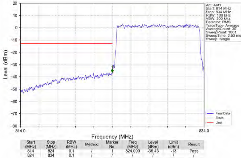
Band5_10MHz_64QAM_LCH_829MHz_RB_50_0_NTNV
