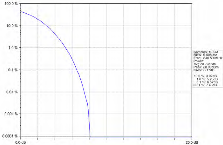
Band5_5MHz_64QAM_HCH_846.5MHz_RB_25_0_NTNV
