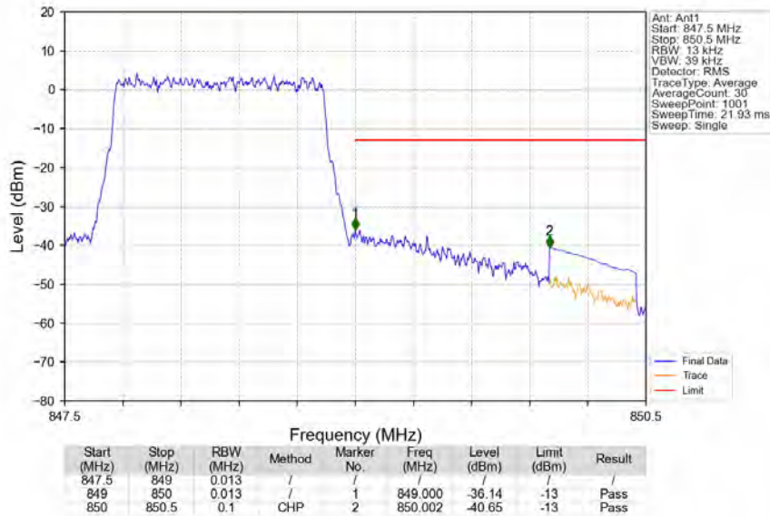
Band5 1.4MHz 64QAM HCH 848.3MHz RB 6 0 NTV
