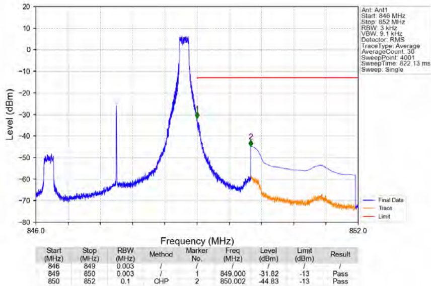
Band5_3MHz_16QAM_HCH_847.5MHz_RB_1_14_NTNV
