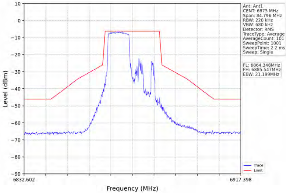
802.11ax(HE20)_HCH_6875MHz_RU106_Right_Ant1_NTNV
