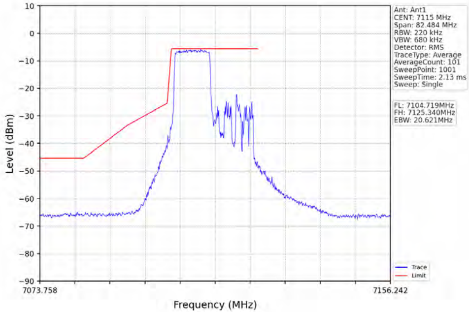
802.11ax(HE20)_HCH_7115MHz_RU106_Right_Ant1_NTNV
