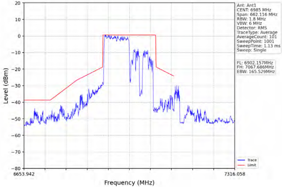
802.11ax(HE160)_MCH_6985MHz_RU996_Right_Ant1_NTNV
