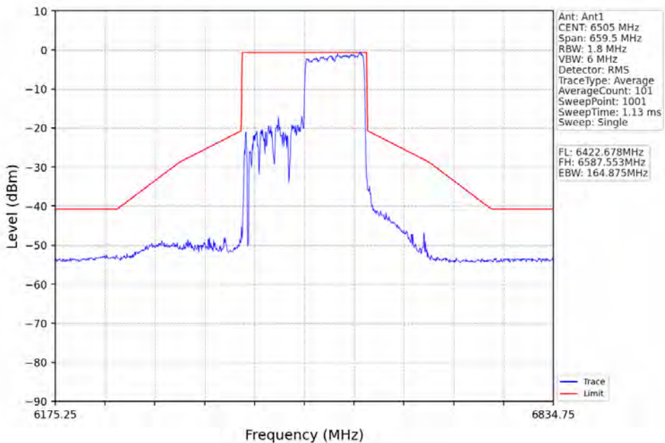
802.11ax(HE160)_HCH_6505MHz_RU996_Right_Ant1_NTNV
