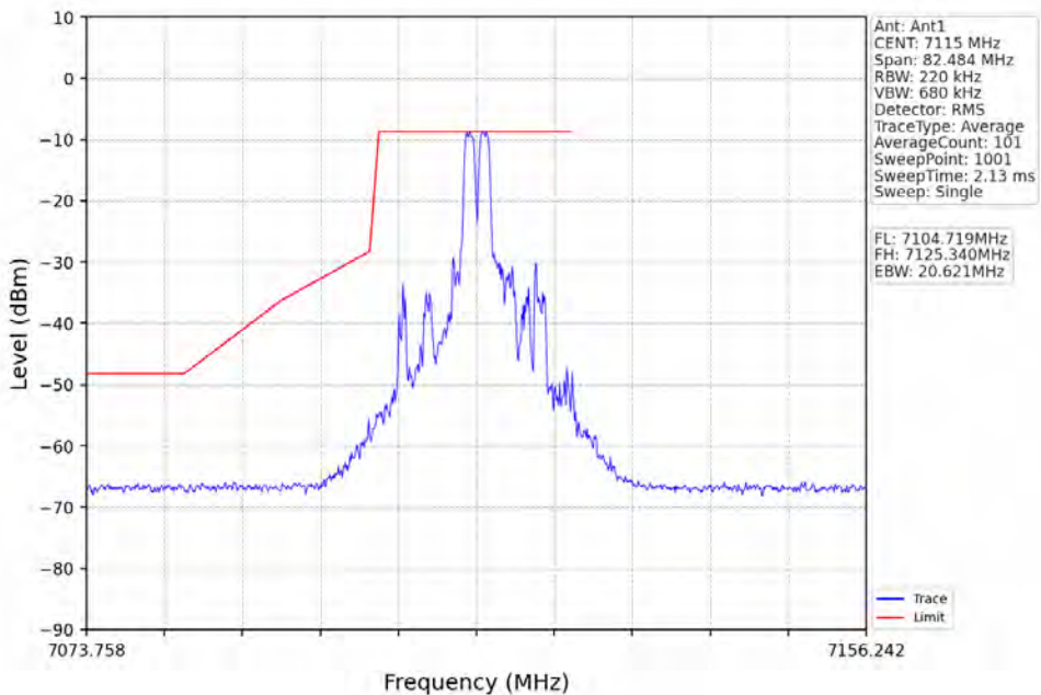
802.11ax(HE20)_HCH_7115MHz_RU26_Mid_Ant1_NTNV
