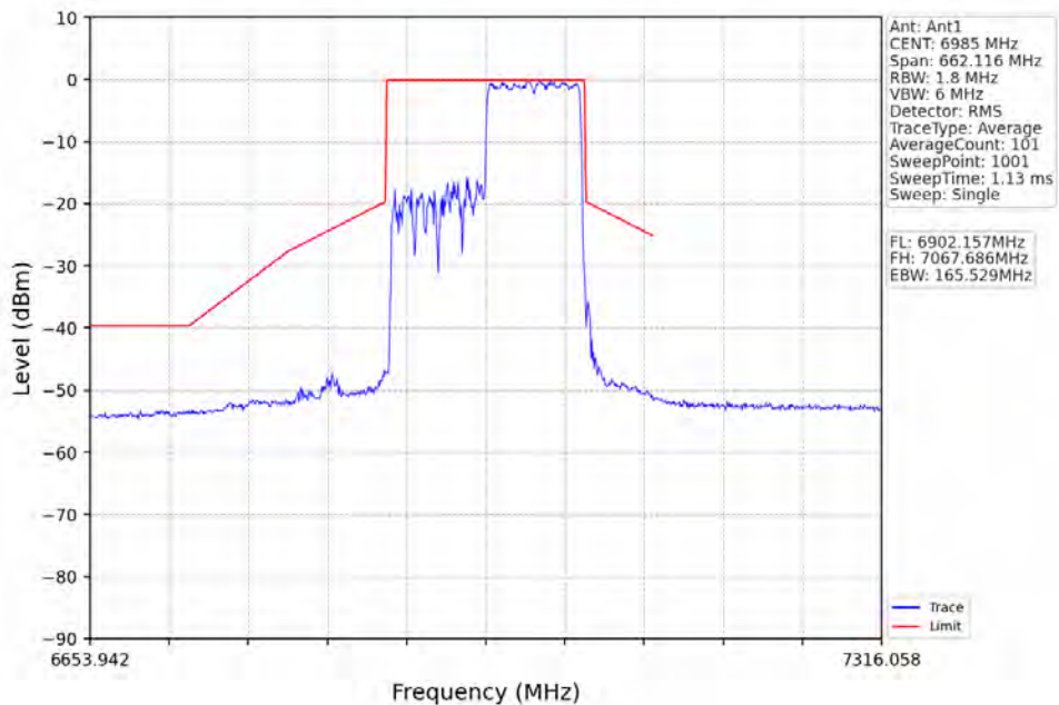
802.11ax(HE160)_MCH_6985MHz_RU996_Right_Ant1_NTNV
