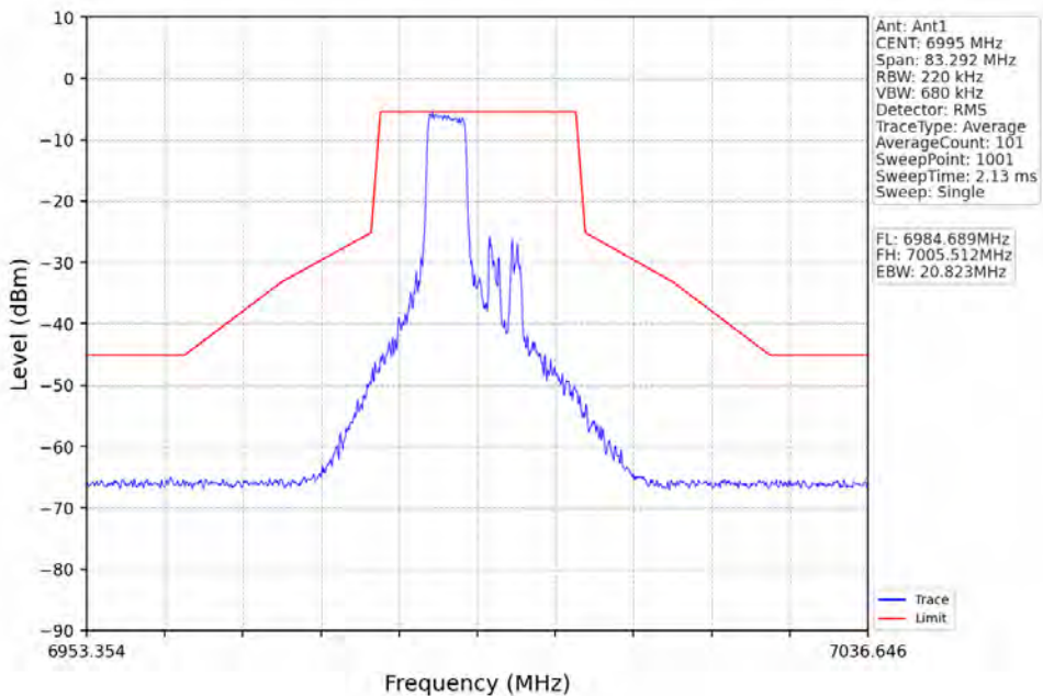
802.11ax(HE20)_MCH_6995MHz_RU52_Mid_Ant1_NTNV
