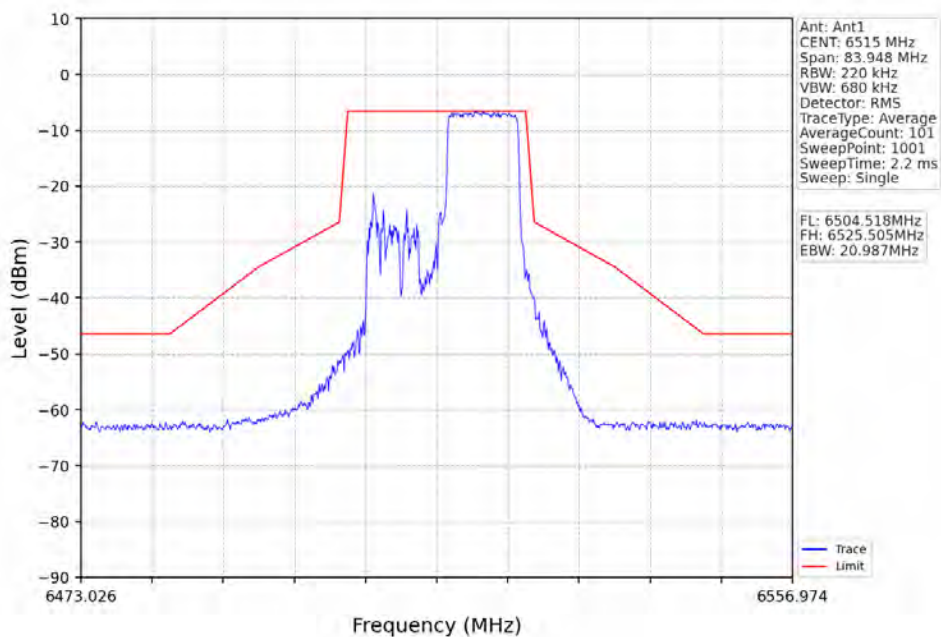
802.11ax(HE20)_HCH_6515MHz_RU106_Right_Ant1_NTNV
