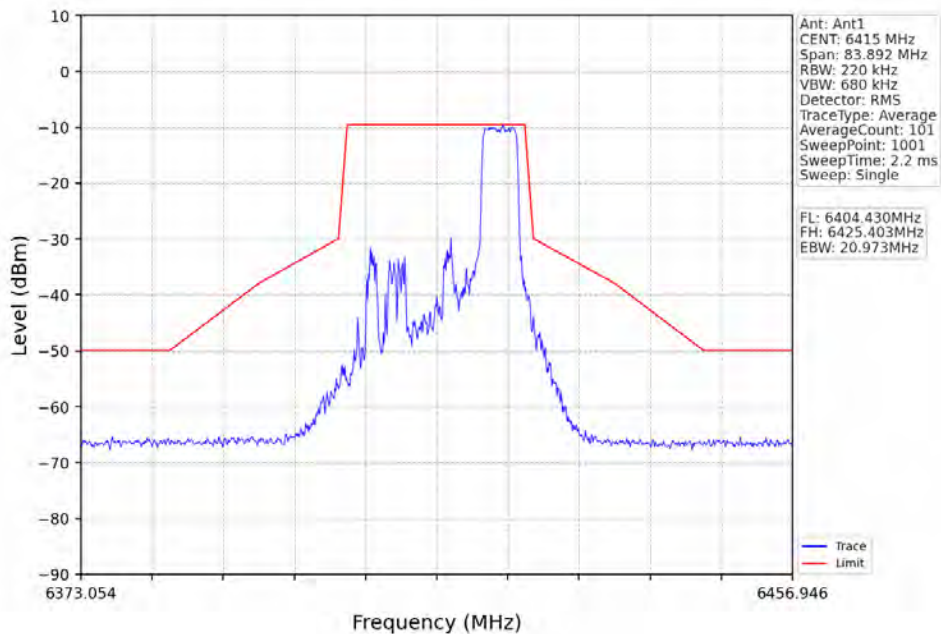
802.11ax(HE20)_HCH_6415MHz_RU52_Right_Ant1_NTNV
