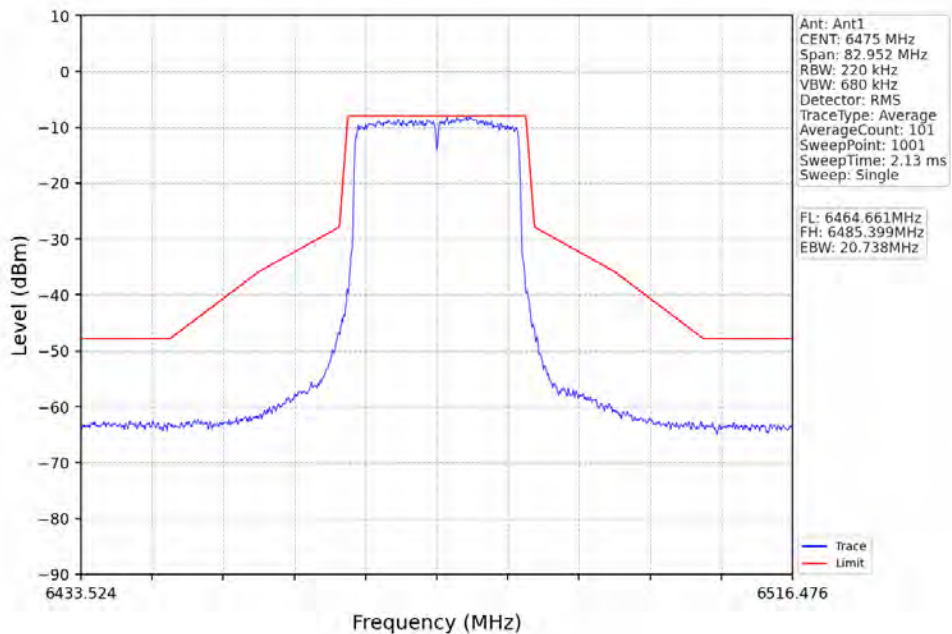
802.11ax(HE20)_MCH_6475MHz_RU242_Left_Ant1_NTNV
