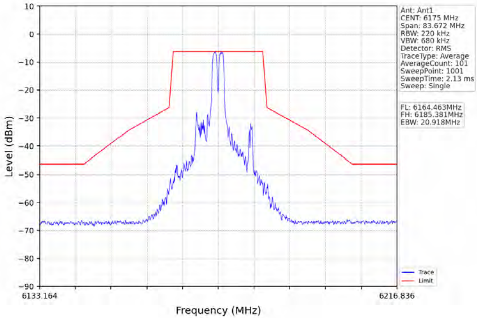
802.11ax(HE20)_MCH_6175MHz_RU26_Right_Ant1_NTNV
