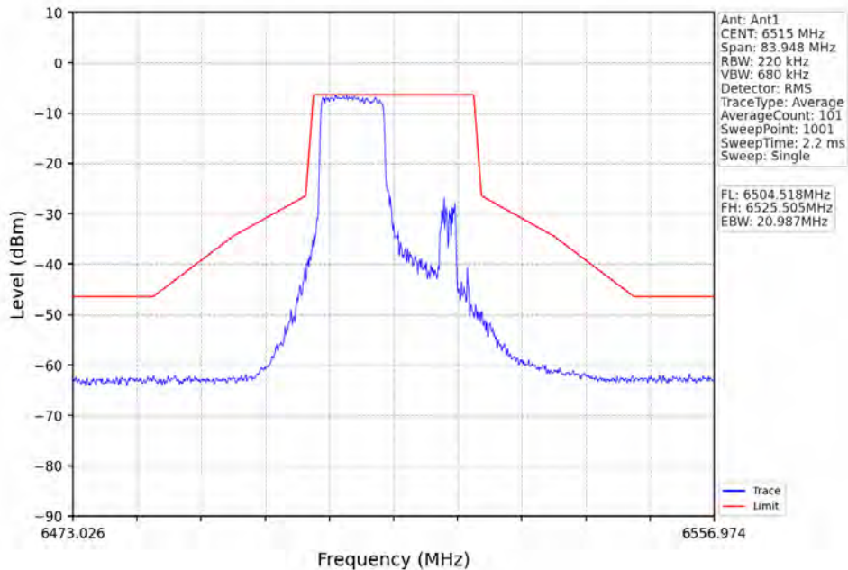
802.11ax(HE20)_HCH_6515MHz_RU106_Right_Ant1_NTNV
