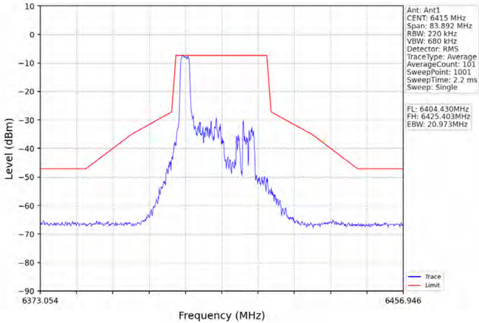
802.11ax(HE20)_HCH_6415MHz_RU26_Mid_Ant1_NTNV
