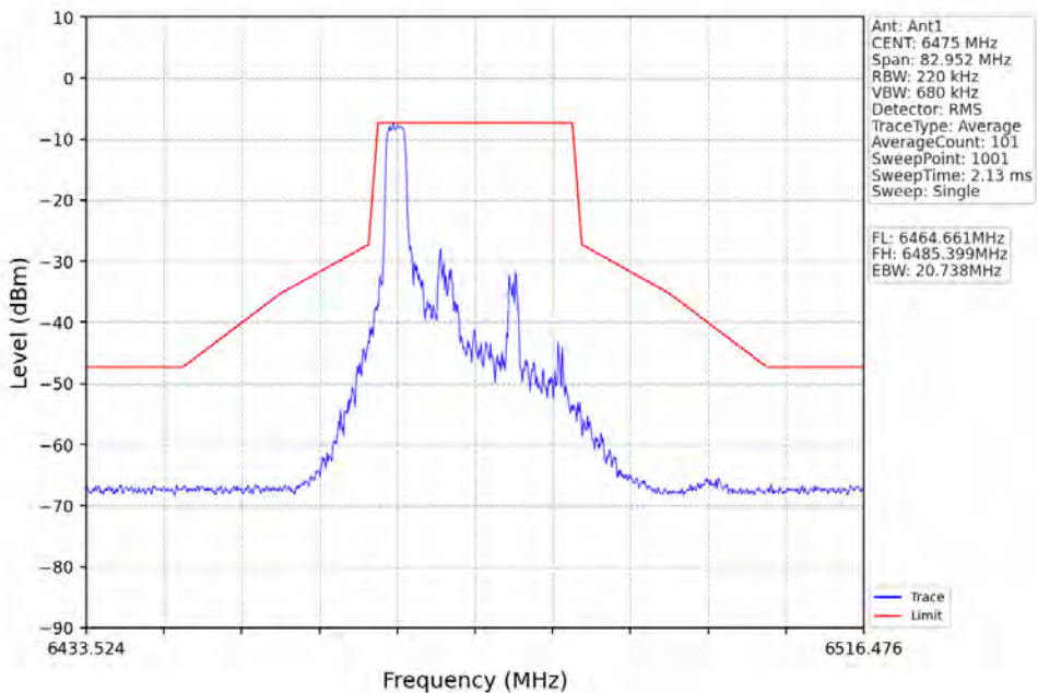
802.11ax(HE20)_MCH_6475MHz_RU26_Left_Ant1_NTNV
