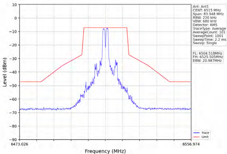
802.11ax(HE20)_HCH_6515MHz_RU26_Mid_Ant1_NTNV
