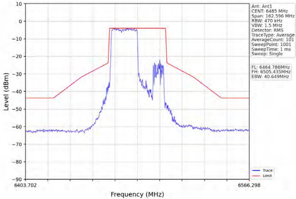
802.11ax(HE40)_MCH_6485MHz_RU242_Right_Ant1_NTNV
