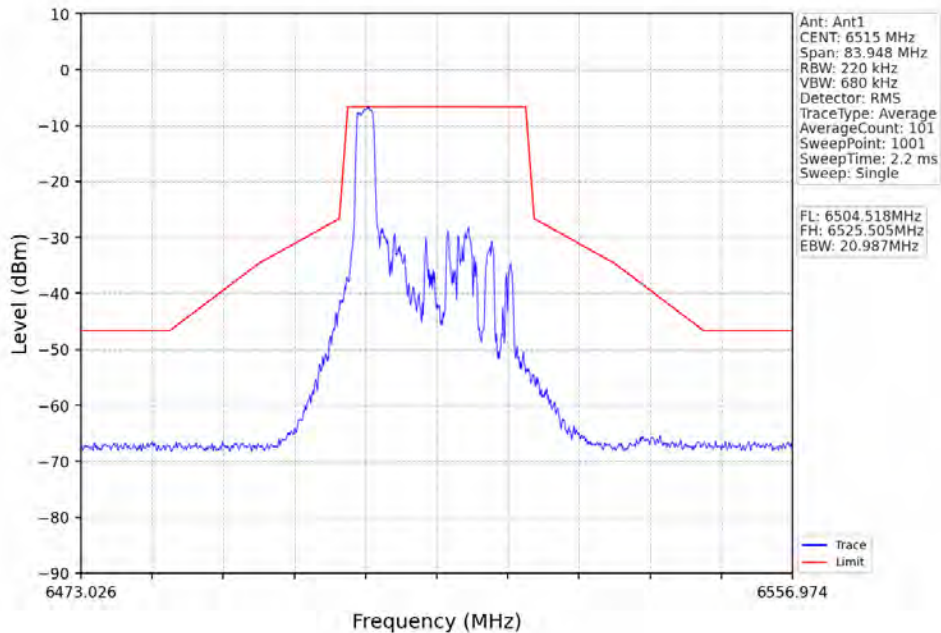
802.11ax(HE20)_HCH_6515MHz_RU26_Mid_Ant1_NTNV
