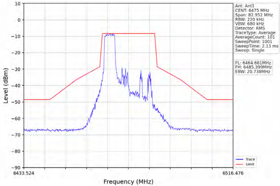
802.11ax(HE20)_MCH_6475MHz_RU52_Mid_Ant1_NTNV
