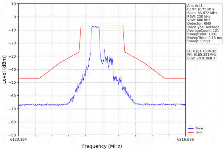
802.11ax(HE20)_MCH_6175MHz_RU52_Mid_Ant1_NTNV
