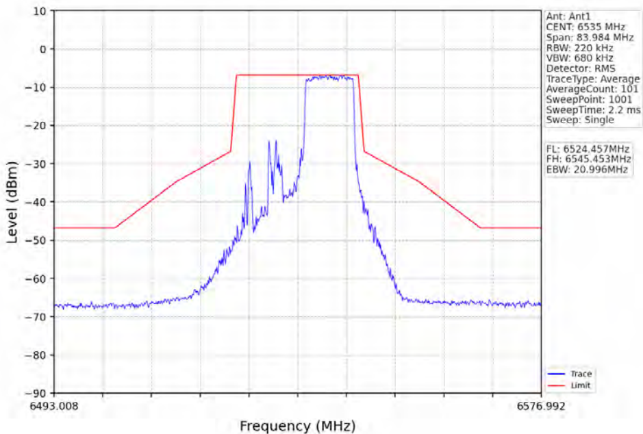
802.11ax(HE20)_LCH_6535MHz_RU106_Right_Ant1_NTNV
