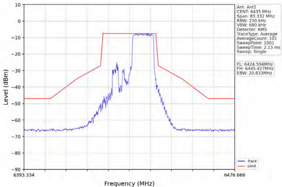
802.11ax(HE20)_LCH_6435MHz_RU106_Right_Ant1_NTNV
