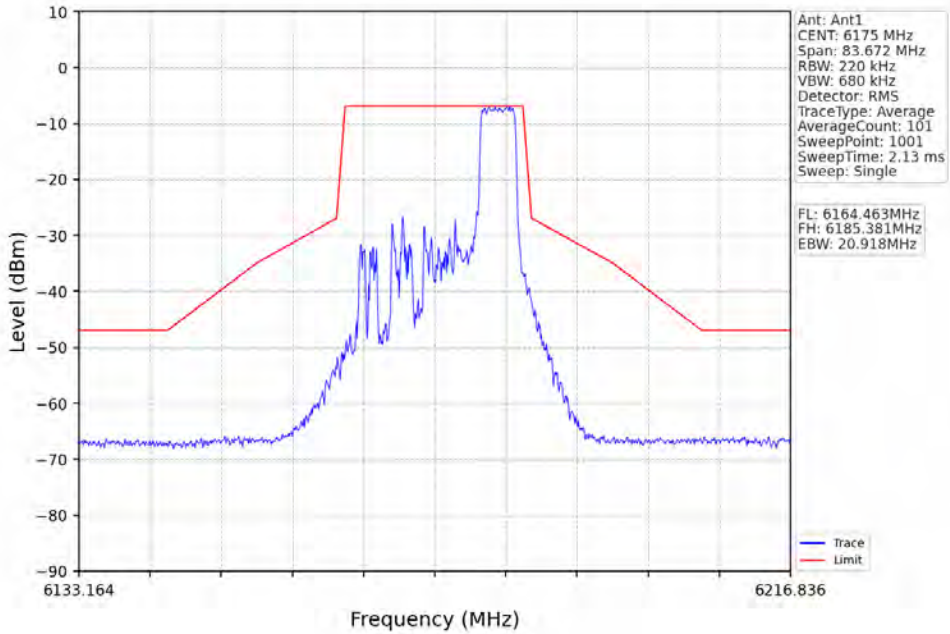
802.11ax(HE20)_MCH_6175MHz_RU106_Left_Ant1_NTNV
