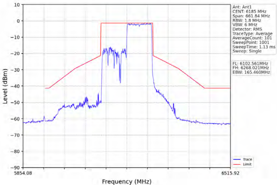
802.11ax(HE160)_MCH_6185MHz_RU996_Right_Ant1_NTNV
