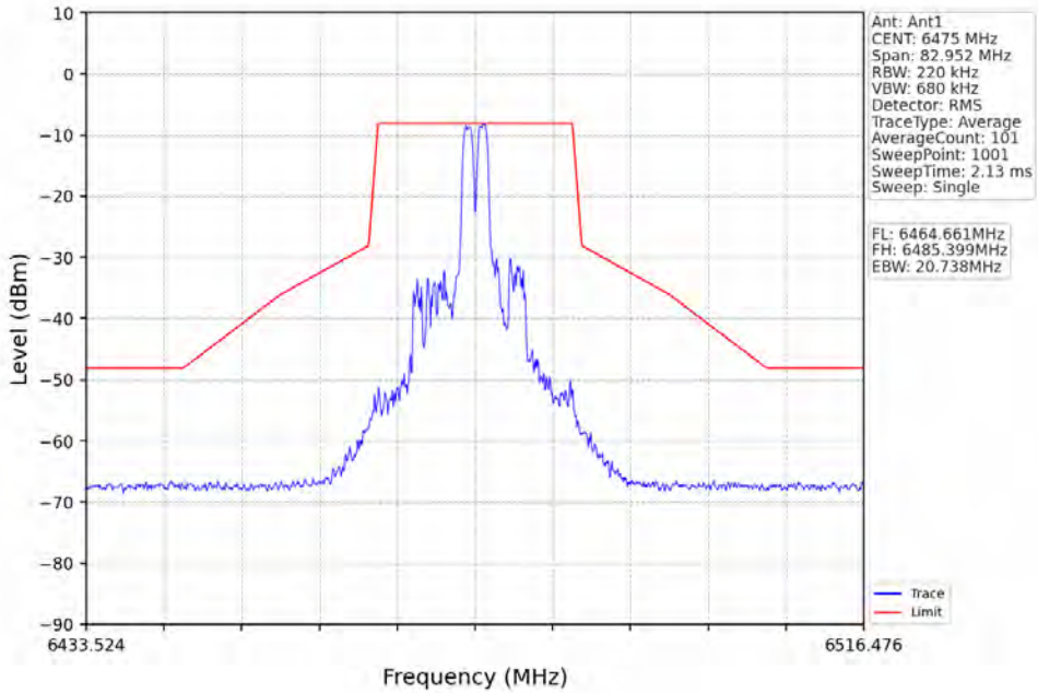
802.11ax(HE20)_MCH_6475MHz_RU26_Right_Ant1_NTNV
