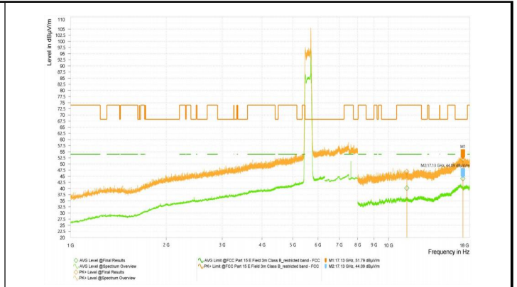
Wi-Fi 5G-11AC80_5290_High
