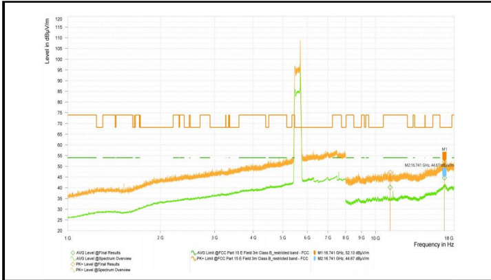
Wi-Fi 5G-11AC20_5180_High
