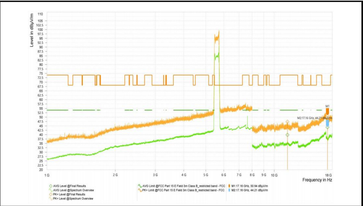
Wi-Fi 5G-11AC20_5220_High
