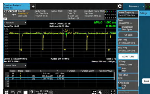
NTNV-11N40SISO-Ant1-2452
