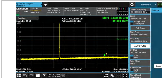
Band66-5MHz-QPSK-131997-1RB#24-1000~3000-PASS
