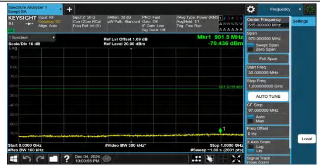
Band66-5MHz-QPSK-131997-1RB#24-30~1000-PASS
