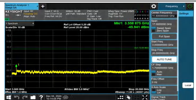
Band66-10MHz-QPSK-132622-1RB#49-3000~20000-PASS
