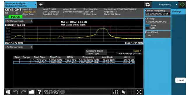
Band66-3MHz-QPSK-132657-1RB#14-PASS
