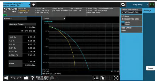
Band66-20MHz-16QAM-132322-100RB#0-PASS
