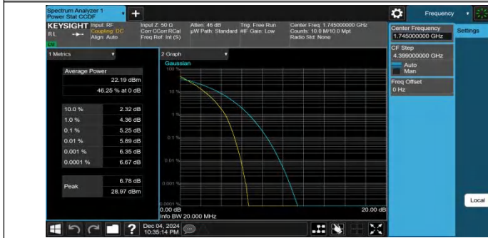
Band66-20MHz-QPSK-132322-100RB#0-PASS
