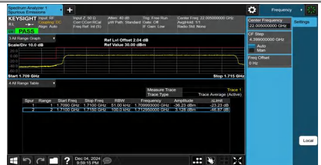
Band66-5MHz-QPSK-132657-1RB#14-PASS
