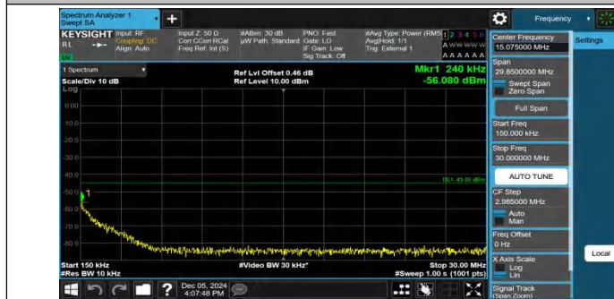
Band41-5MHz-QPSK-41565-1RB#24-0.15~30-PASS
