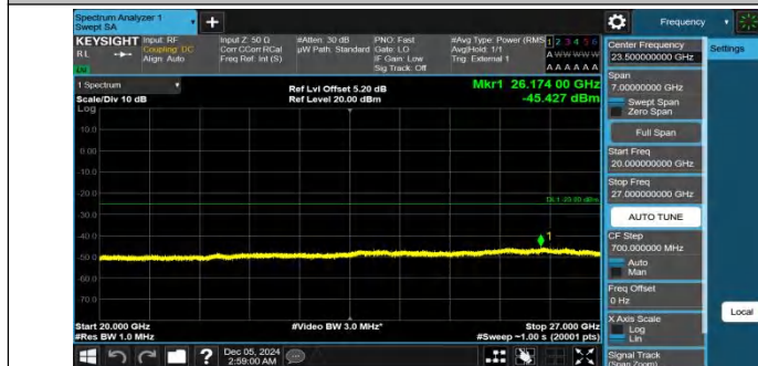
Band41-10MHz-QPSK-40620-1RB#0-20000~27000-PASS
