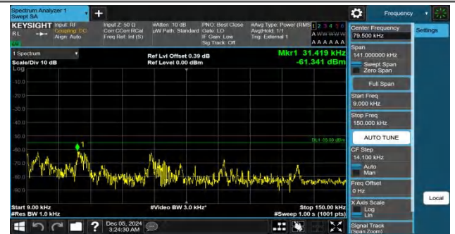
Band41-15MHz-QPSK-40620-1RB#74-0.009~0.15-PASS
