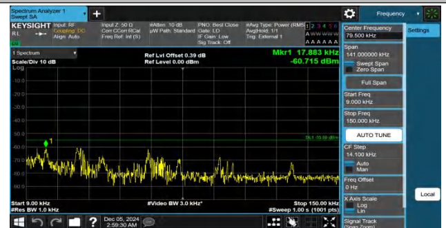
Band41-10MHz-QPSK-40620-1RB#49-0.009~0.15-PASS
