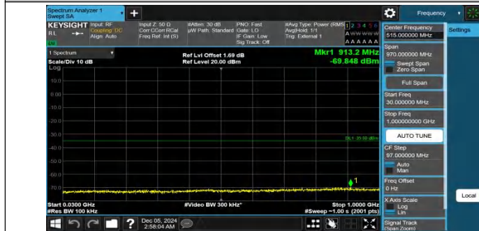
Band41-10MHz-QPSK-40620-1RB#0-30~1000-PASS
