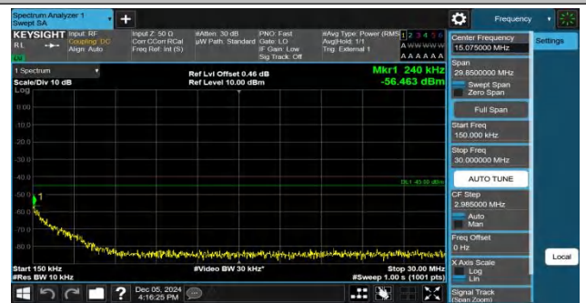
Band41-20MHz-QPSK-41490-1RB#0-0.15~30-PASS
