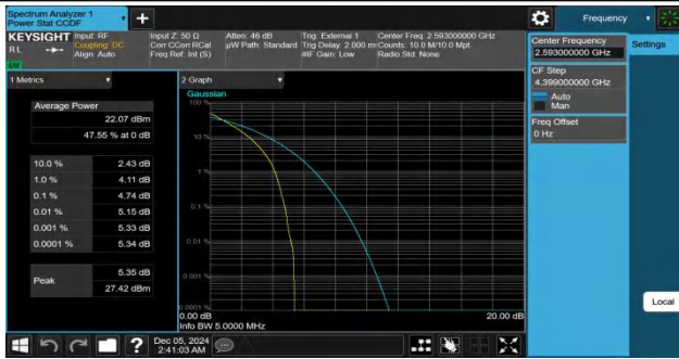
Band41-5MHz-QPSK-40620-25RB#0-PASS
