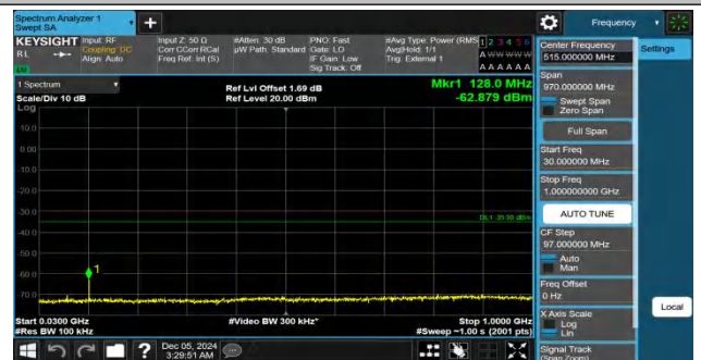
Band41-15MHz-QPSK-41515-1RB#74-30~1000-PASS
