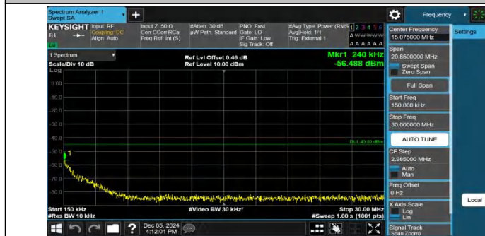
Band41-15MHz-QPSK-39725-1RB#74-0.15~30-PASS
