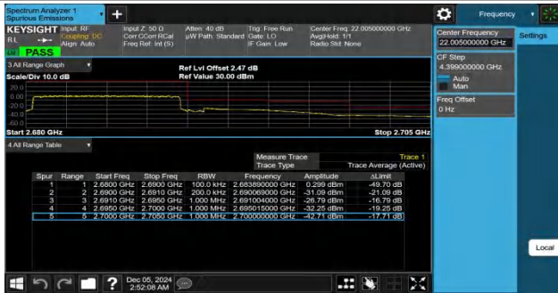
Band41-10MHz-QPSK-41540-50RB#0-PASS
