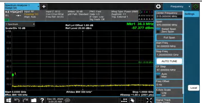
Band41-10MHz-QPSK-40620-1RB#49-30~1000-PASS
