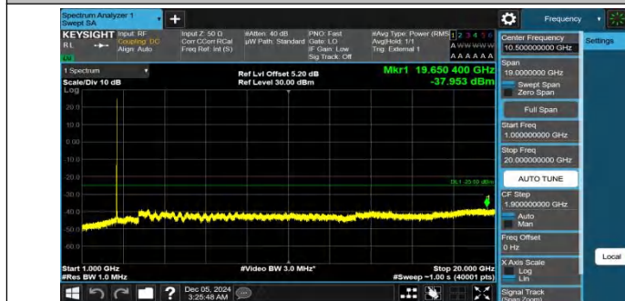
Band41-15MHz-QPSK-40620-1RB#74-1000~20000-PASS
