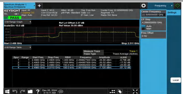
Band41-15MHz-QPSK-39725-75RB#0-PASS
