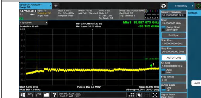
Band41-20MHz-QPSK-40620-1RB#99-1000~20000-PASS
