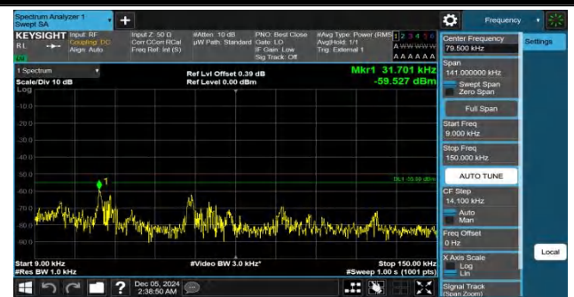
Band41-5MHz-QPSK-41565-1RB#24-0.009~0.15-PASS
