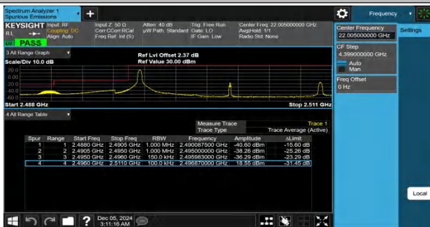
Band41-15MHz-QPSK-39725-1RB#0-PASS
