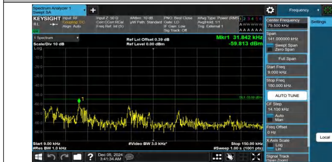
Band41-20MHz-QPSK-39750-1RB#0-0.009~0.15-PASS
