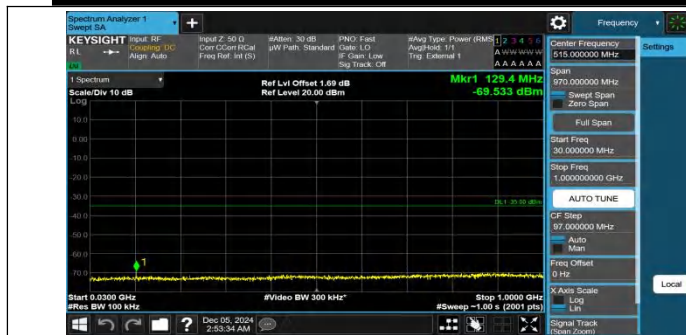
Band41-10MHz-QPSK-39700-1RB#0-30~1000-PASS
