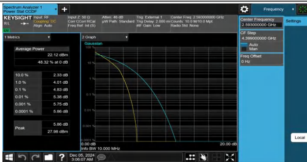
Band41-10MHz-QPSK-40620-50RB#0-PASS
