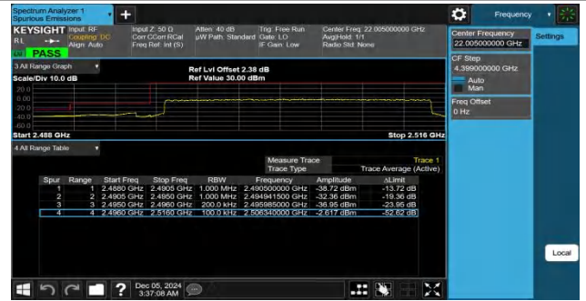
Band41-20MHz-QPSK-39750-100RB#0-PASS
