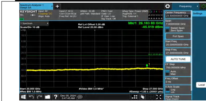
Band41-20MHz-QPSK-40620-1RB#0-20000~27000-PASS
