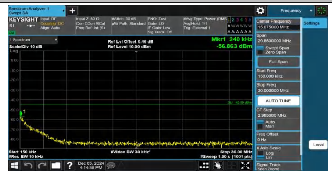
Band41-20MHz-QPSK-39750-1RB#0-0.15~30-PASS
