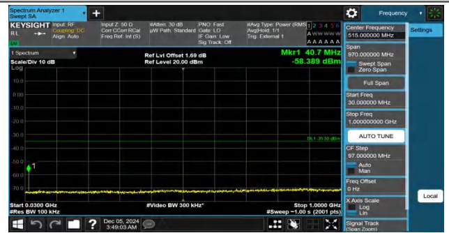
Band41-20MHz-QPSK-40620-1RB#99-30~1000-PASS
