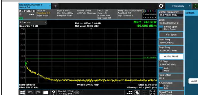
Band41-15MHz-QPSK-41515-1RB#74-0.15~30-PASS
