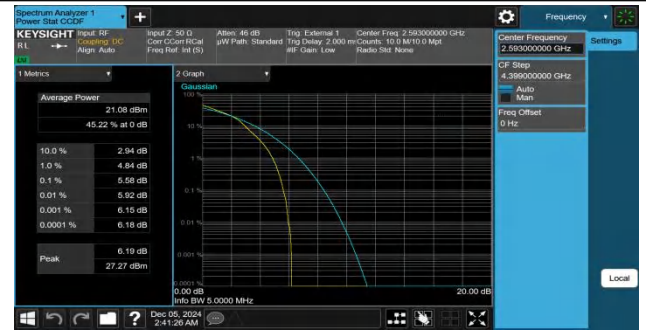
Band41-5MHz-16QAM-40620-25RB#0-PASS
