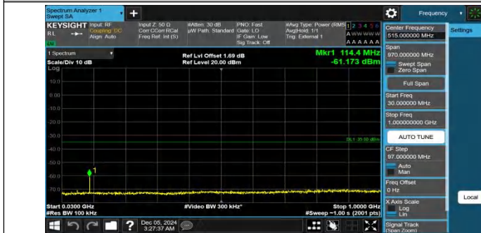
Band41-15MHz-QPSK-41515-1RB#0-30~1000-PASS
