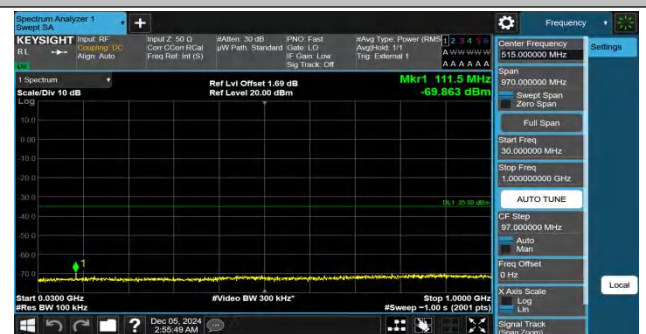
Band41-10MHz-QPSK-39700-1RB#49-30~1000-PASS
