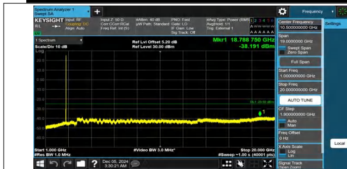
Band41-15MHz-QPSK-41515-1RB#74-1000~20000-PASS
