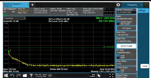
Band41-15MHz-QPSK-41515-1RB#0-0.15~30-PASS
