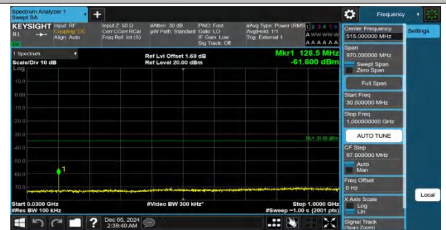
Band41-5MHz-QPSK-41565-1RB#24-30~1000-PASS
