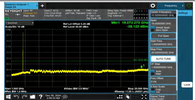
Band41-10MHz-QPSK-40620-1RB#0-1000~20000-PASS
