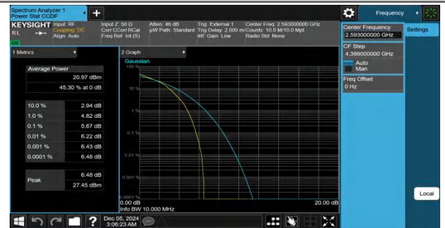
Band41-10MHz-16QAM-40620-50RB#0-PASS
