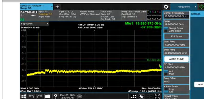
Band41-5MHz-QPSK-41565-1RB#24-1000~20000-PASS
