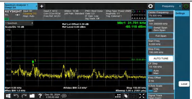
Band41-10MHz-QPSK-39700-1RB#49-0.009~0.15-PASS
