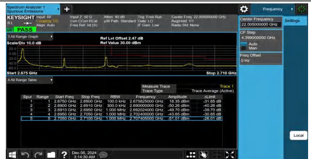
Band41-15MHz-QPSK-41515-1RB#0-PASS
