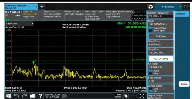
Band41-15MHz-QPSK-39725-1RB#74-0.009~0.15-PASS
