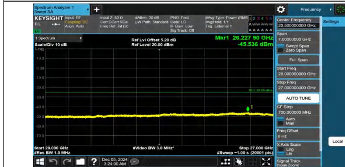
Band41-15MHz-QPSK-40620-1RB#0-20000~27000-PASS
