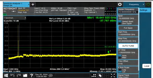
Band41-15MHz-QPSK-41515-1RB#0-1000~20000-PASS
