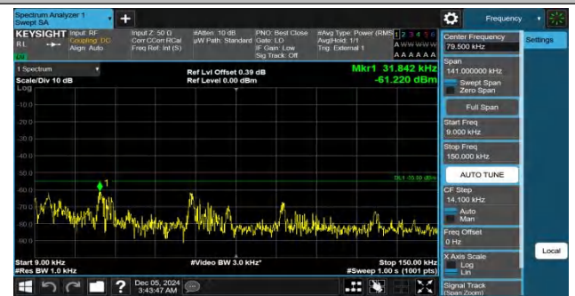
Band41-20MHz-QPSK-39750-1RB#99-0.009~0.15-PASS
