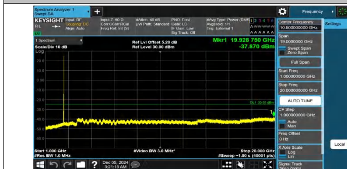
Band41-15MHz-QPSK-39725-1RB#74-1000~20000-PASS
