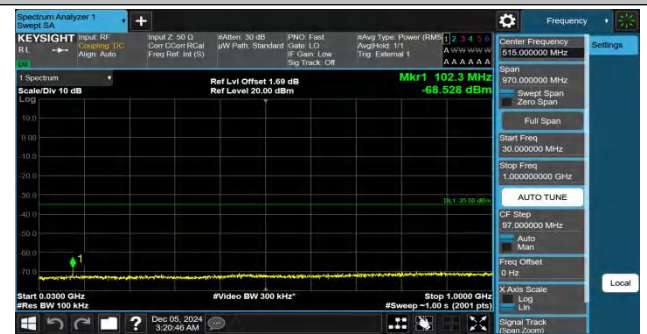
Band41-15MHz-QPSK-39725-1RB#74-30~1000-PASS
