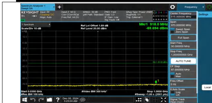
Band41-15MHz-QPSK-40620-1RB#0-30~1000-PASS
