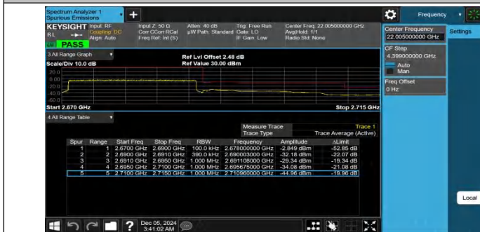
Band41-20MHz-QPSK-41490-100RB#0-PASS
