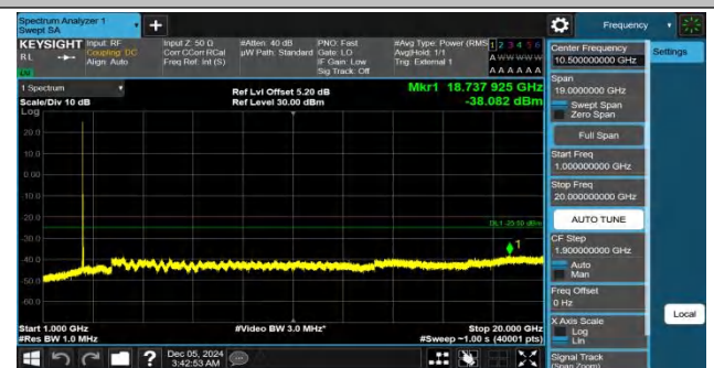
Band41-20MHz-QPSK-39750-1RB#0-1000~20000-PASS
