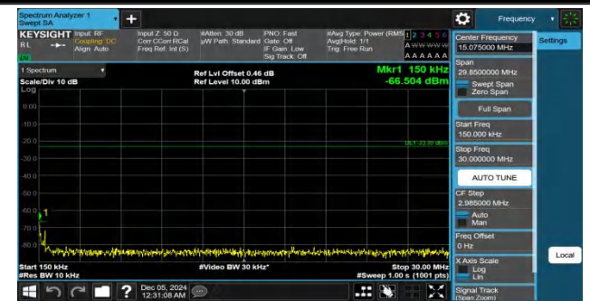
Band26(824-849)-3MHz-QPSK-26915-1RB#0-0.15~30-PASS
