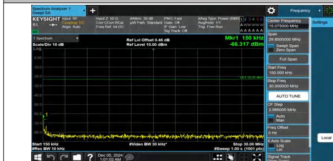
Band26(824-849)-15MHz-QPSK-26865-1RB#74-0.15~30-PASS
