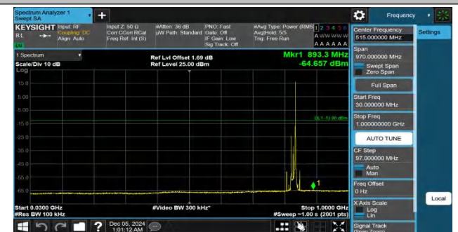
Band26(824-849)-15MHz-QPSK-26865-1RB#74-30~1000-PASS
