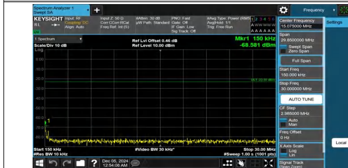
Band26(824-849)-10MHz-QPSK-26990-1RB#49-0.15~30-PASS
