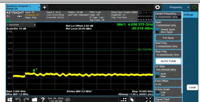
Band26(824-849)-15MHz-QPSK-26965-1RB#74-3000~10000-PAS
