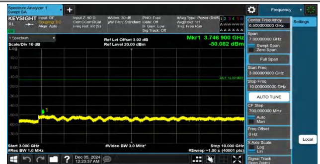
Band26(824-849)-1.4MHz-QPSK-27033-1RB#5-3000~10000-PAS S
