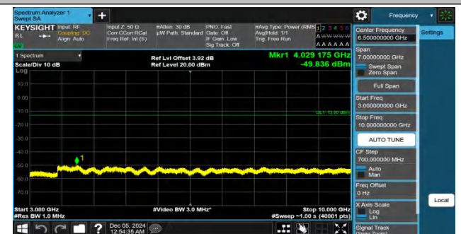
Band26(824-849)-10MHz-QPSK-26990-1RB#49-3000~10000-PAS
