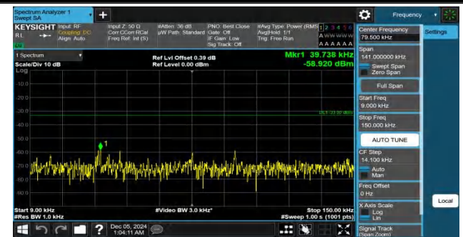
Band26(824-849)-15MHz-QPSK-26965-1RB#74-0.009~0.15-PASS
