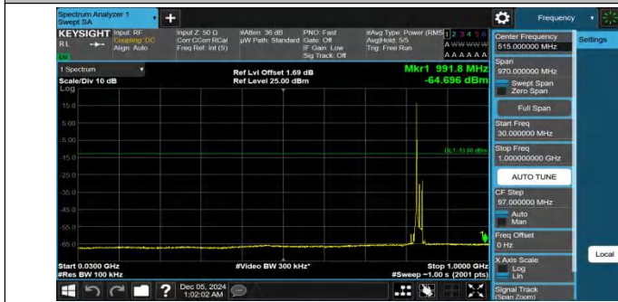
Band26(824-849)-15MHz-QPSK-26915-1RB#0-30~1000-PASS
