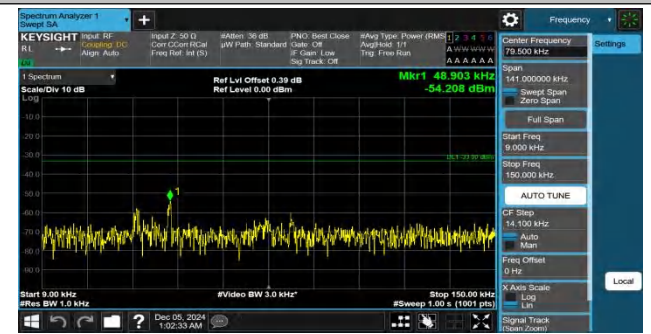
Band26(824-849)-15MHz-QPSK-26915-1RB#74-0.009~0.15-PASS
