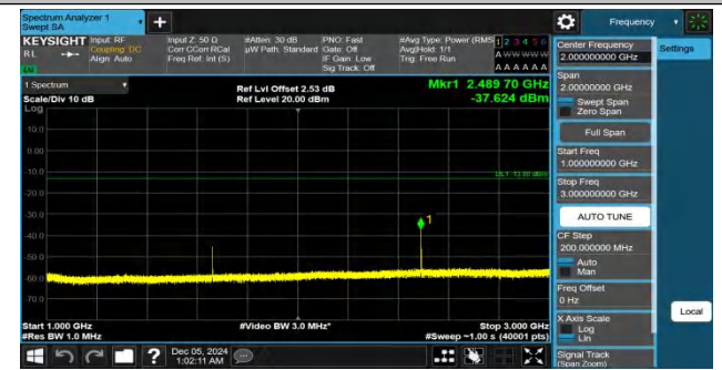
Band26(824-849)-15MHz-QPSK-26915-1RB#0-1000~3000-PASS
