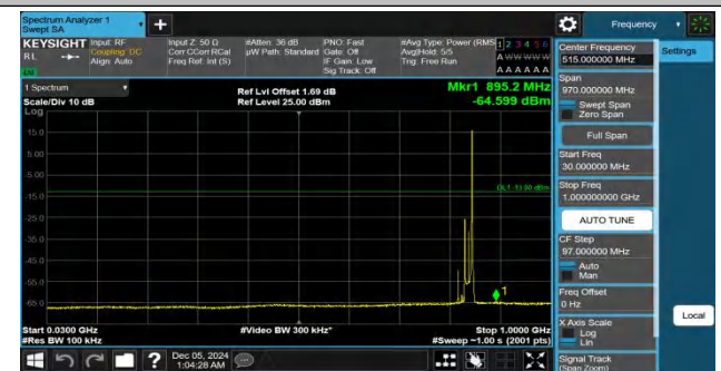
Band26(824-849)-15MHz-QPSK-26965-1RB#74-30~1000-PASS
