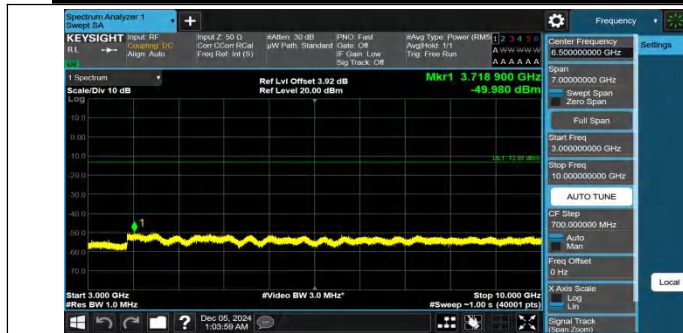
Band26(824-849)-15MHz-QPSK-26965-1RB#0-3000~10000-PAS
