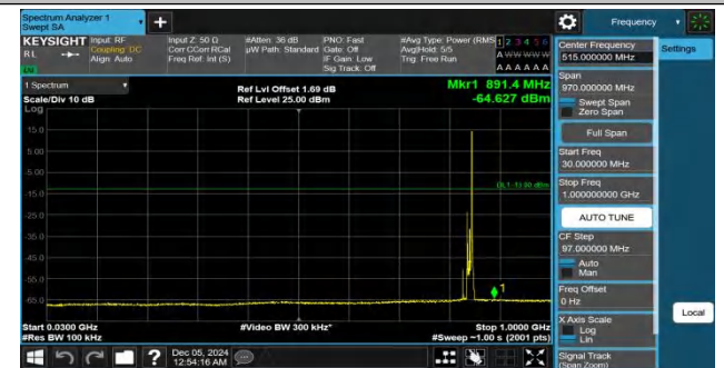
Band26(824-849)-10MHz-QPSK-26990-1RB#49-30~1000-PASS
