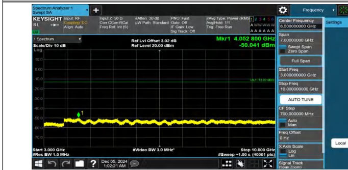
Band26(824-849)-15MHz-QPSK-26915-1RB#0-3000~10000-PAS
