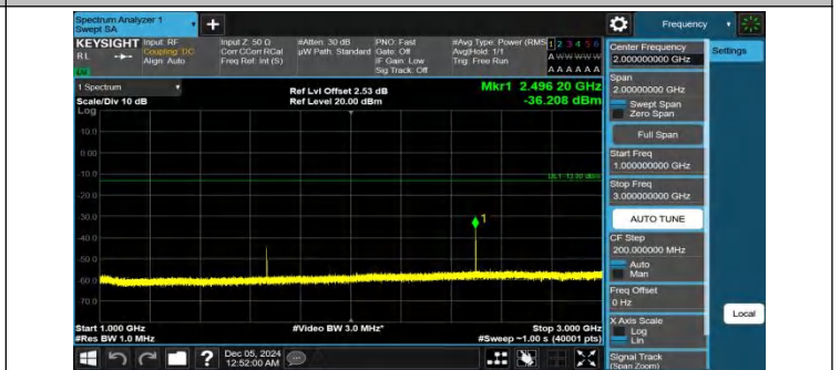
Band26(824-849)-10MHz-QPSK-26915-1RB#0-1000~3000-PASS
