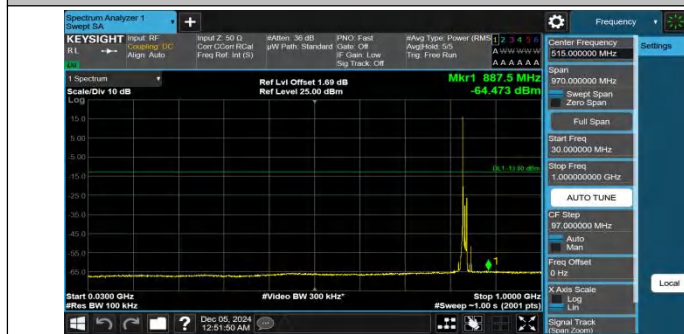
Band26(824-849)-10MHz-QPSK-26915-1RB#0-30~1000-PASS
