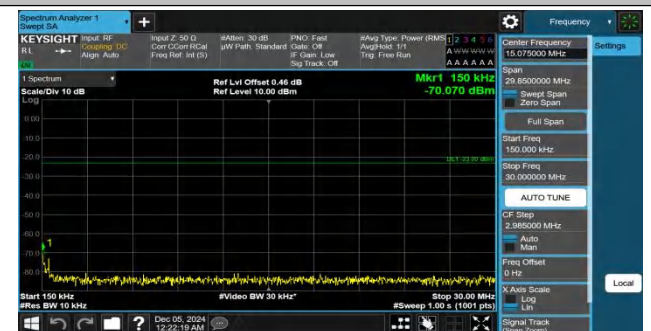
Band26(824-849)-1.4MHz-QPSK-27033-1RB#0-0.15~30-PASS
