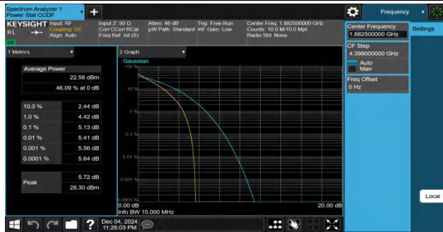
Band25-15MHz-QPSK-26365-75RB#0-PASS
