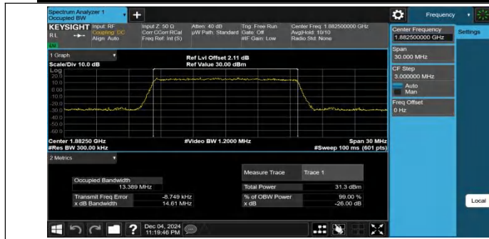
Band25-15MHz-QPSK-26365-75RB#0-PASS
