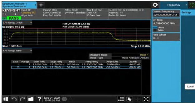
Band25-3MHz-QPSK-26675-15RB#0-PASS
