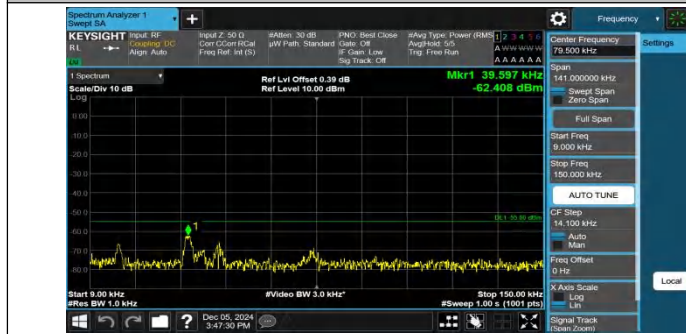
Band7-5MHz-QPSK-21100-1RB#0-0.009~0.15-PASS
