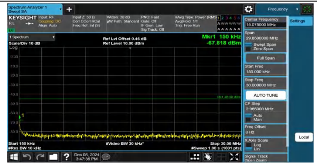
Band7-5MHz-QPSK-21100-1RB#0-0.15~30-PASS
