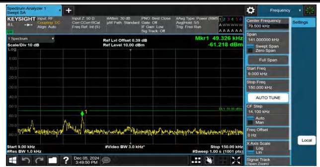
Band7-5MHz-QPSK-21425-1RB#24-0.009~0.15-PASS
