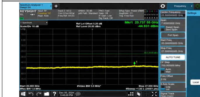
Band7-5MHz-QPSK-21100-1RB#0-20000~27000-PASS
