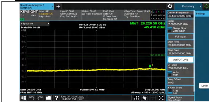
Band7-5MHz-QPSK-21425-1RB#0-20000~27000-PASS
