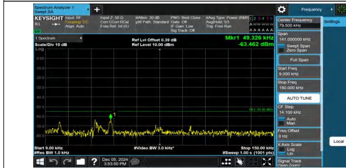
Band7-10MHz-QPSK-21400-1RB#0-0.009~0.15-PASS
