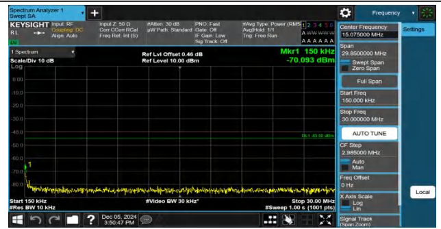
Band7-10MHz-QPSK-20800-1RB#0-0.15~30-PASS
