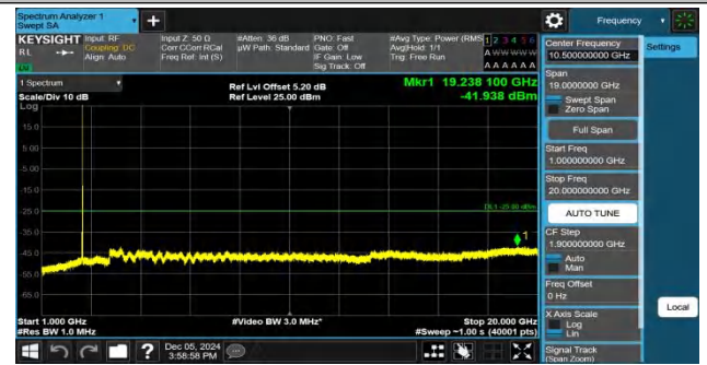
Band7-15MHz-QPSK-21375-1RB#0-1000~20000-PASS
