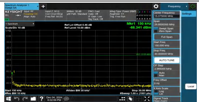
Band4-15MHz-QPSK-20175-1RB#74-0.15~30-PASS
