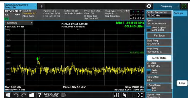
Band4-15MHz-QPSK-20175-75RB#0-0.009~0.15-PASS
