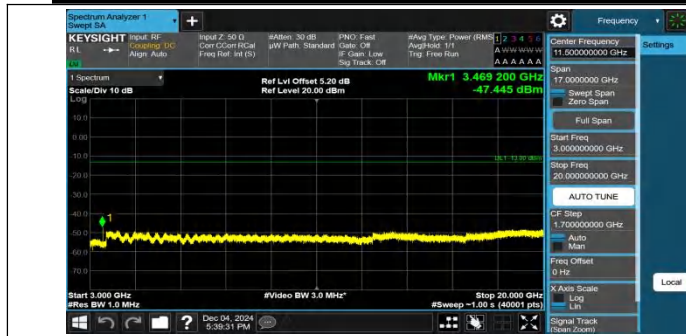
Band4-5MHz-QPSK-20175-1RB#24-3000~20000-PASS
