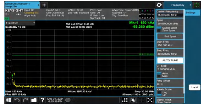
Band4-20MHz-QPSK-20300-1RB#99-0.15~30-PASS
