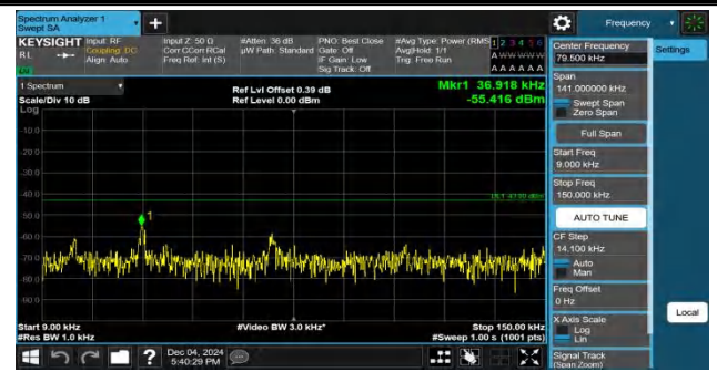
Band4-5MHz-QPSK-20375-1RB#0-0.009~0.15-PASS
