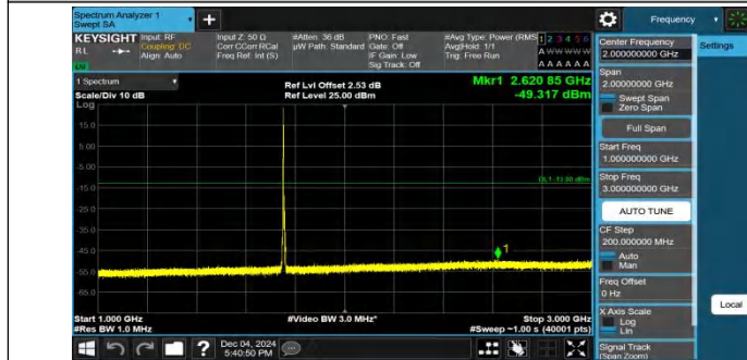
Band4-5MHz-QPSK-20375-1RB#0-1000~3000-PASS
