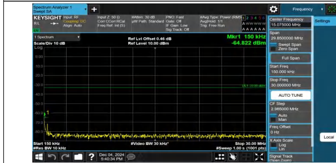
Band4-5MHz-QPSK-20375-1RB#0-0.15~30-PASS
