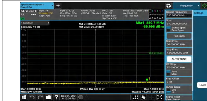
Band4-20MHz-QPSK-20300-1RB#0-30~1000-PASS
