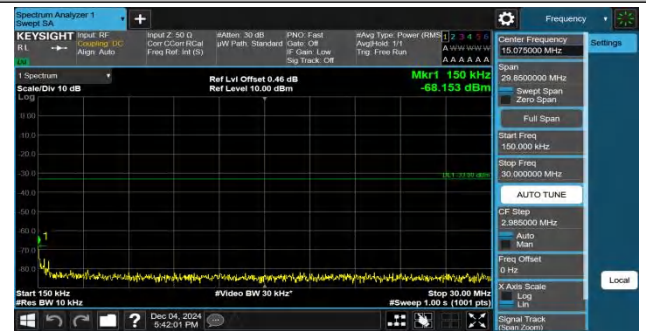
Band4-5MHz-QPSK-20375-25RB#0-0.15~30-PASS
