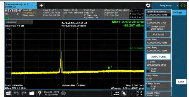
Band4-20MHz-QPSK-20300-1RB#0-1000~3000-PASS
