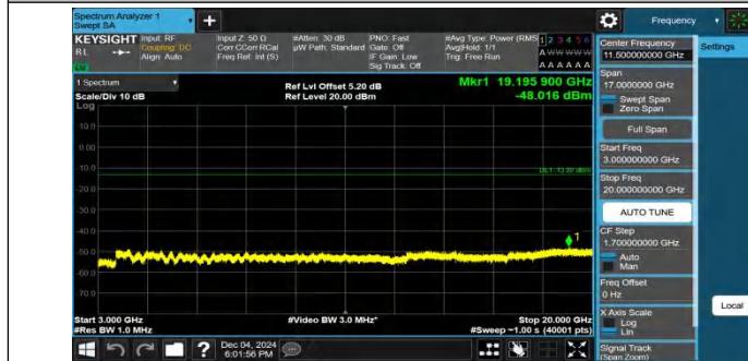
Band4-15MHz-QPSK-20025-75RB#0-3000~20000-PASS
