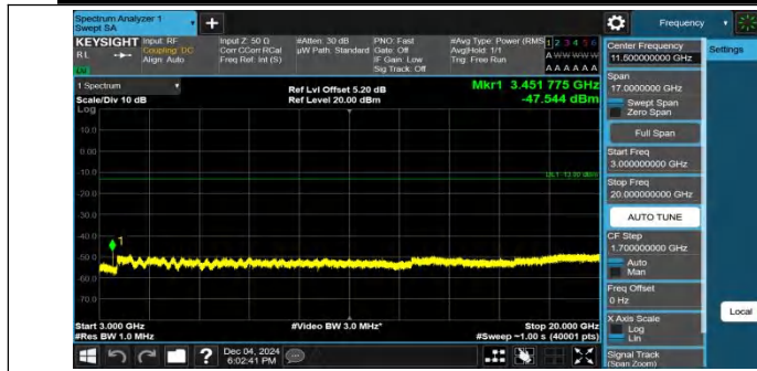
Band4-15MHz-QPSK-20175-1RB#0-3000~20000-PASS
