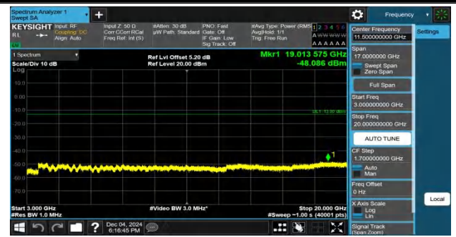
Band4-20MHz-QPSK-20300-100RB#0-3000~20000-PASS
