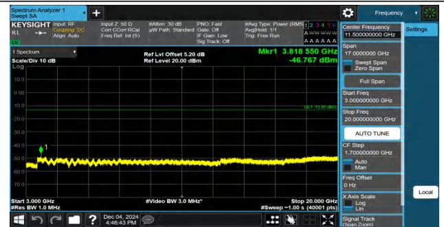
Band2-10MHz-QPSK-19150-1RB#49-3000~20000-PASS
