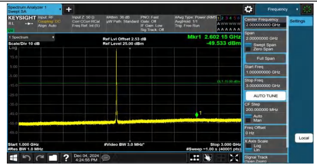
Band2-3MHz-QPSK-18900-1RB#0-1000~3000-PASS
