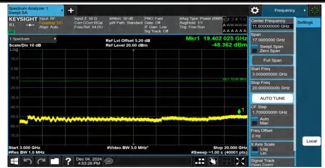
Band2-15MHz-QPSK-18675-1RB#74-3000~20000-PASS
