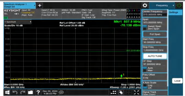
Band2-15MHz-QPSK-19125-1RB#74-30~1000-PASS
