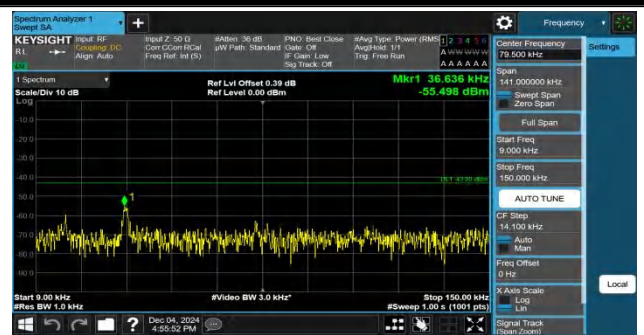
Band2-15MHz-QPSK-19125-1RB#74-0.009~0.15-PASS
