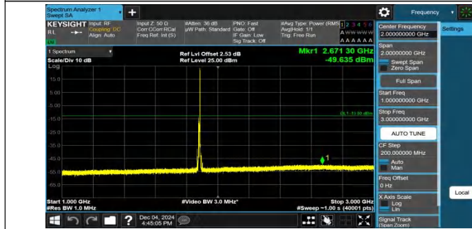
Band2-10MHz-QPSK-18900-1RB#49-1000~3000-PASS
