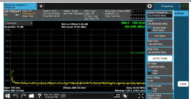
Band2-20MHz-QPSK-18700-1RB#0-0.15~30-PASS
