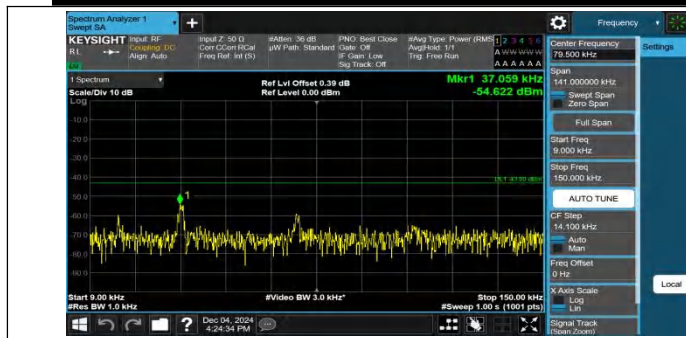
Band2-3MHz-QPSK-18900-1RB#0-0.009~0.15-PASS
