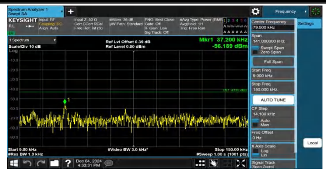
Band2-5MHz-QPSK-18625-1RB#24-0.009~0.15-PASS
