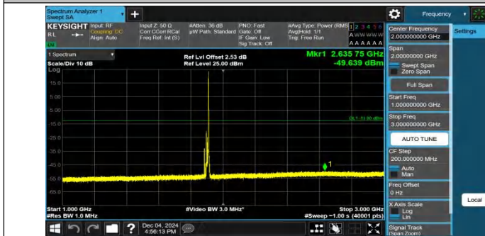
Band2-15MHz-QPSK-19125-1RB#74-1000~3000-PASS
