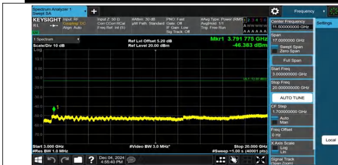
Band2-15MHz-QPSK-19125-1RB#0-3000~20000-PASS
