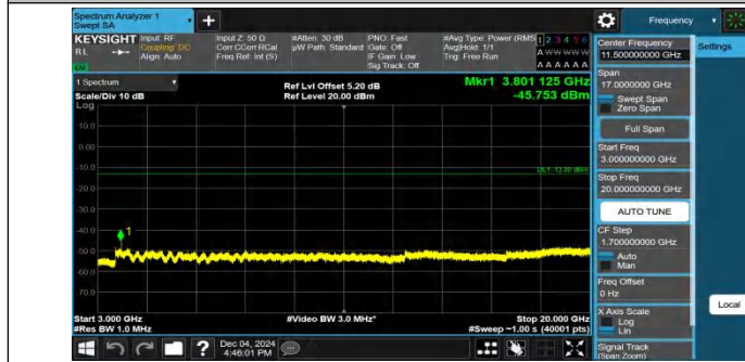
Band2-10MHz-QPSK-19150-1RB#0-3000~20000-PASS
