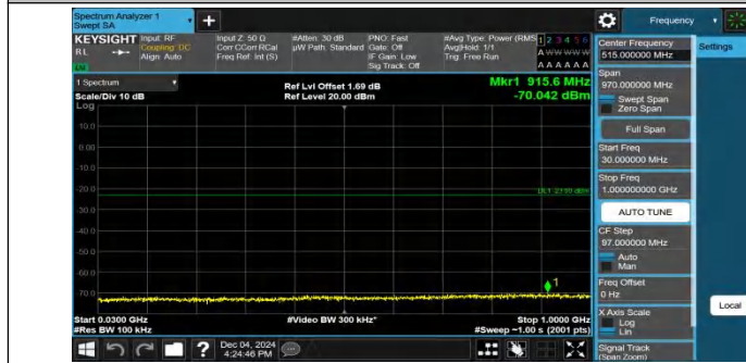
Band2-3MHz-QPSK-18900-1RB#0-30~1000-PASS
