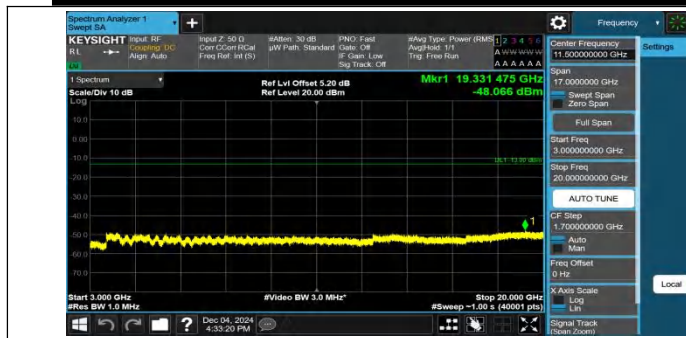
Band2-5MHz-QPSK-18625-1RB#0-3000~20000-PASS
