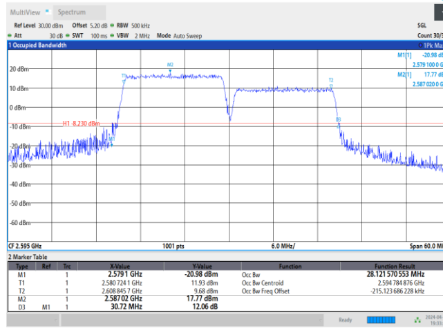
38-38-15MHz-15MHz-16QAM-16QAM-37925-38075-75RB#0-75RB#0
