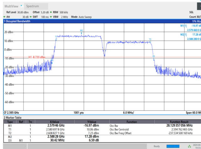
38-38-15MHz-15MHz-64QAM-64QAM-37925-38075-75RB#0-75RB#0
