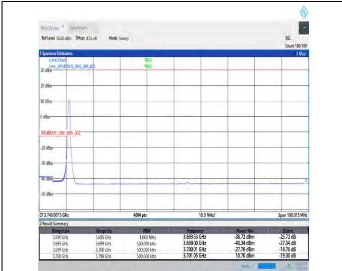
1-N78-3700-3800-30-90-L-1-DFT-PI2BPSK-Edge_1RB_Left-1@0-Ant1-1--PASS-see graph
