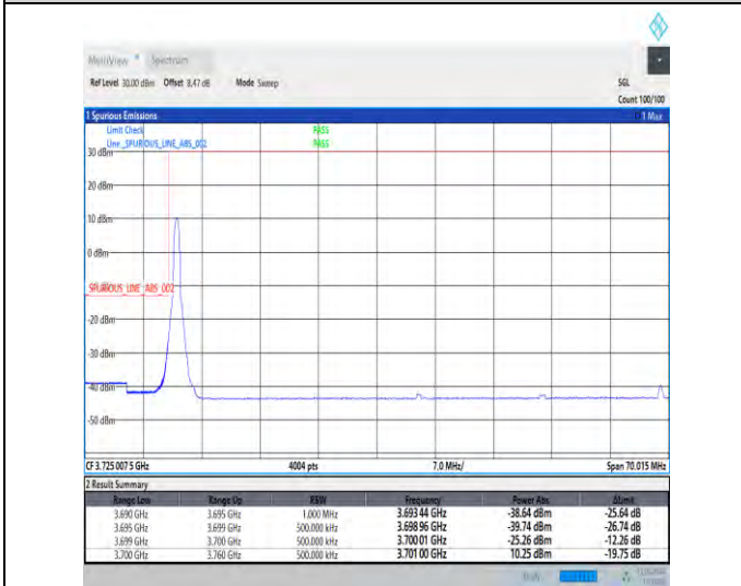
1-N78-3700-3800-30-60-L-4-CP-QPSK-Edge_1RB_Lef t-1@0-Ant1-1--PASS-see graph
