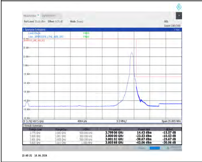
1-N78-3700-3800-N78-3700-380030-25-H-5-CP-QPS K-Edge_1RB_Right-1@64-Ant1-1--PASS-see graph
