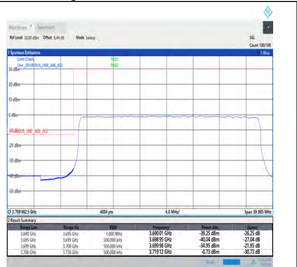
1-N78-3700-3800-30-30-L-3-DFT-PI2BPSK-Outer _Full-75@0-Ant1-1--PASS-see graph
