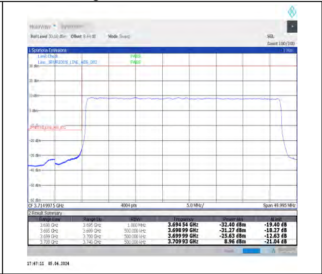
1-N78-3700-3800-N78-3700-380030-40-L-3-DFT-P I2BPSK-Outer_Full-100@0-Ant1-1--PASS-see graph
