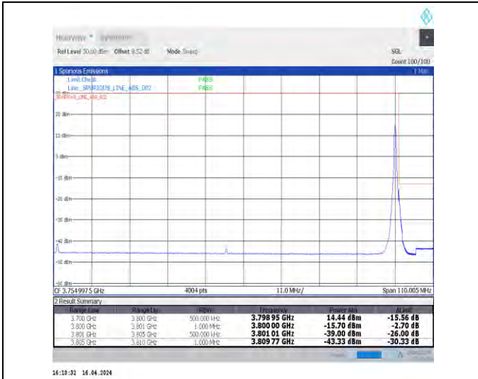
1-N78-3700-3800-N78-3700-380030-100-H-2-DFT-PI2 BPSK-Edge_1RB_Right-1@272-Ant1-1--PASS-see graph
