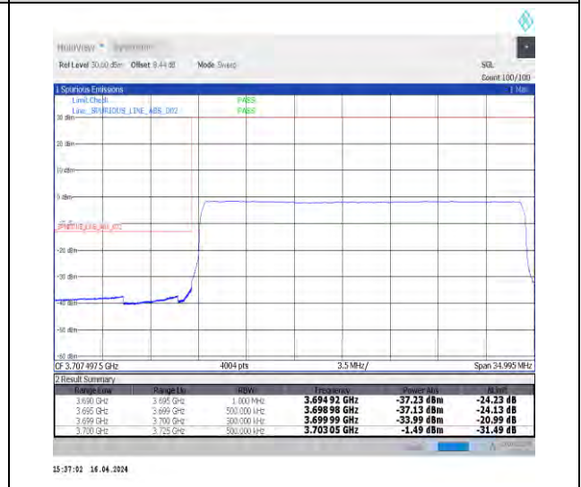
1-N78-3700-3800-N78-3700-380030-25-L-6-CP-Q PSK-Outer_Full-65@0-Ant1-1--PASS-see graph
