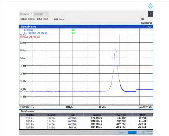
1-N78-3700-3800-30-30-H-2-DFT-PI2BPSK-Edge_1R_B_Right-1@77-Ant1-1--PASS-see graph
