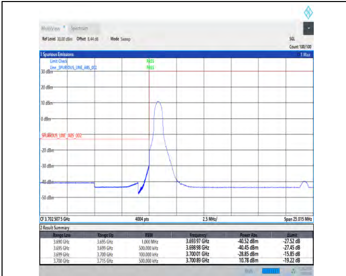
1-N78-3700-3800-30-15-L-1-DFT-PI2BPSK-Edge_1RB _Left-1@0-Ant1-1--PASS-see graph
