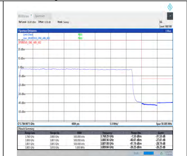
1-N78-3700-3800-30-40-H-3-DFT-PI2BPSK-Outer_Full-100@0-Ant1-1--PASS-see graph
