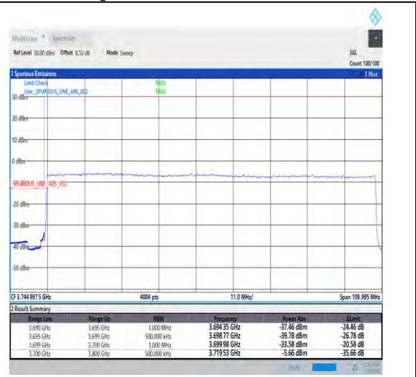
1-N78-3700-3800-30-100-L-3-DFT-PI2BPSK-Outer_Full-270@0-Ant1-1--PASS-see graph
