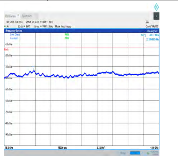
1-N78-3700-3800-30-100-H-1-DFT-QPSK-Edge_1RB _Left-1@0-18000-40000-Ant1-22185.96--33.27--13-P ASS
