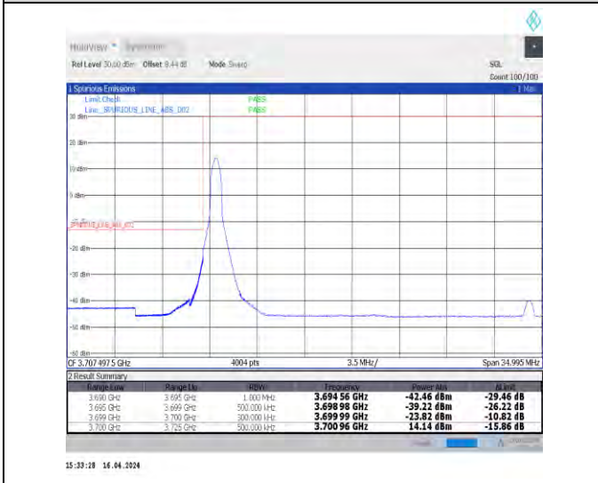
1-N78-3700-3800-N78-3700-380030-25-L-4-CP-QPSK -Edge_1RB_Left-1@0-Ant1-1--PASS-see graph
