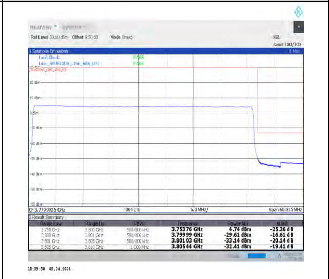
1-N78-3700-3800-N78-3700-380030-50-H-6-CP-Q PSK-Outer_Full-133@0-Ant1-1--PASS-see graph
