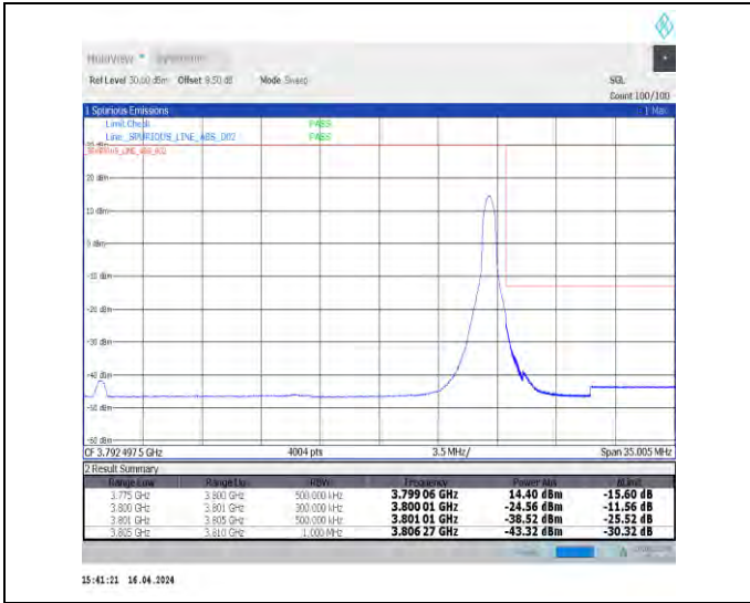
1-N78-3700-3800-N78-3700-380030-25-H-2-DFT-PI2 BPSK-Edge_1RB_Right-1@64-Ant1-1--PASS-see graph
