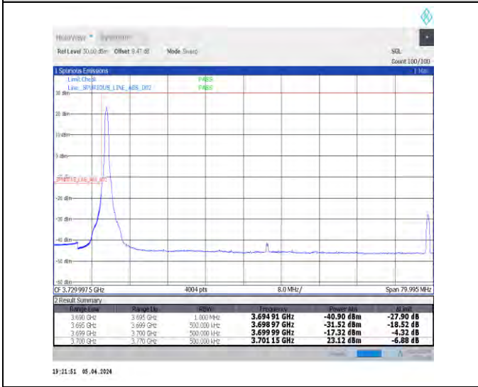
1-N78-3700-3800-N78-3700-380030-70-L-4-CP-QPSK -Edge_1RB_Left-1@0-Ant1-1--PASS-see graph
