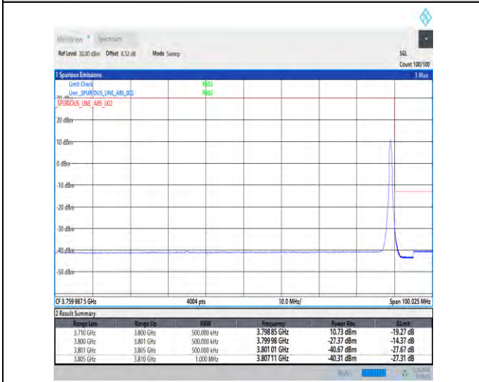
1-N78-3700-3800-30-90-H-5-CP-QPSK-Edge_1RB_Right-1@244-Ant1-1--PASS-see graph
