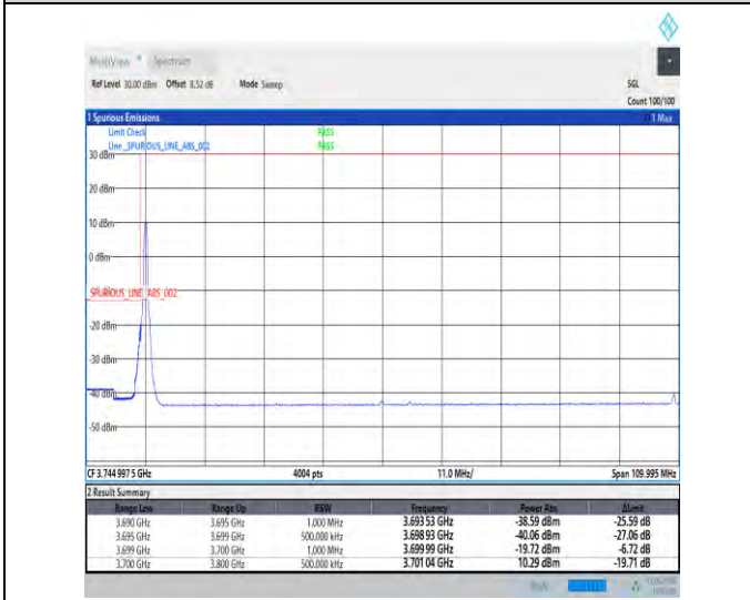
1-N78-3700-3800-30-100-L-4-CP-QPSK-Edge_1RB_Left-1@0-Ant1-1--PASS-see graph
