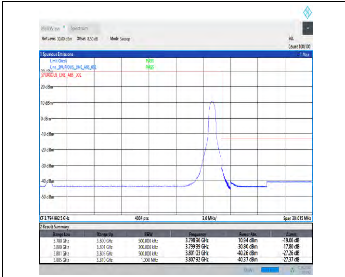
1-N78-3700-3800-30-20-H-2-DFT-PI2BPSK-Edge_1R_B_Right-1@50-Ant1-1--PASS-see graph
