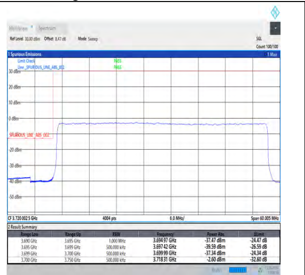
1-N78-3700-3800-30-50-L-3-DFT-PI2BPSK-Outer_Full-128@0-Ant1-1--PASS-see graph
