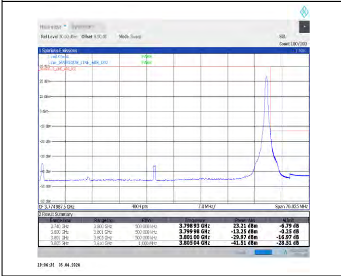
1-N78-3700-3800-N78-3700-380030-60-H-5-CP-QPS K-Edge_1RB_Right-1@161-Ant1-1--PASS-see graph
