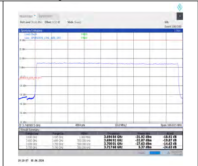
1-N78-3700-3800-N78-3700-380030-90-L-3-DFT-P I2BPSK-Outer_Full-240@0-Ant1-1--PASS-see graph
