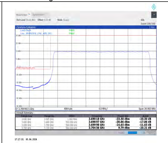
1-N78-3700-3800-N78-3700-380030-30-L-3-DFT-P I2BPSK-Outer_Full-75@0-Ant1-1--PASS-see graph
