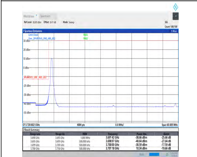
1-N78-3700-3800-30-50-L-4-CP-QPSK-Edge_1RB_Lef t-1@0-Ant1-1--PASS-see graph
