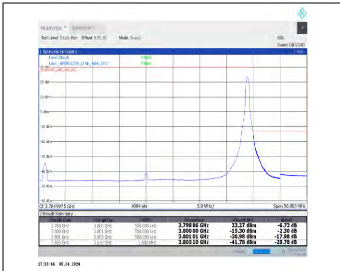
1-N78-3700-3800-N78-3700-380030-40-H-2-DFT-PI2 BPSK-Edge_1RB_Right-1@105-Ant1-1--PASS-see graph
