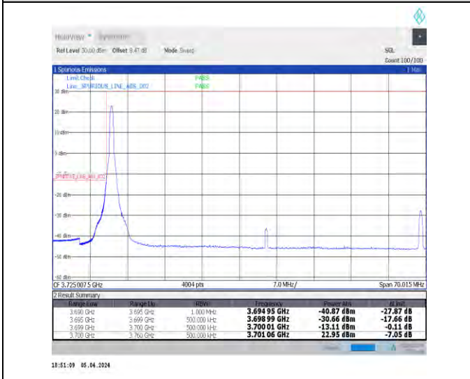
1-N78-3700-3800-N78-3700-380030-60-L-4-CP-QPSK -Edge_1RB_Left-1@0-Ant1-1--PASS-see graph
