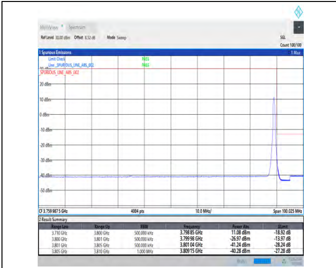
1-N78-3700-3800-30-90-H-2-DFT-PI2BPSK-Edge_1R_B_Right-1@244-Ant1-1--PASS-see graph
