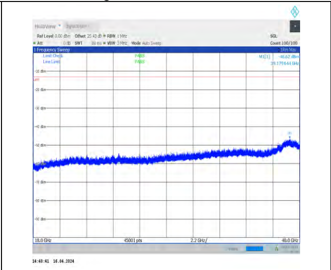
1-N78-3700-3800-N78-3700-380030-100-L-1-DFT-PI 2BPSK-Inner_1RB_Left-1@1-18000-40000-Ant1-185 06.49--46.62--13-PASS
