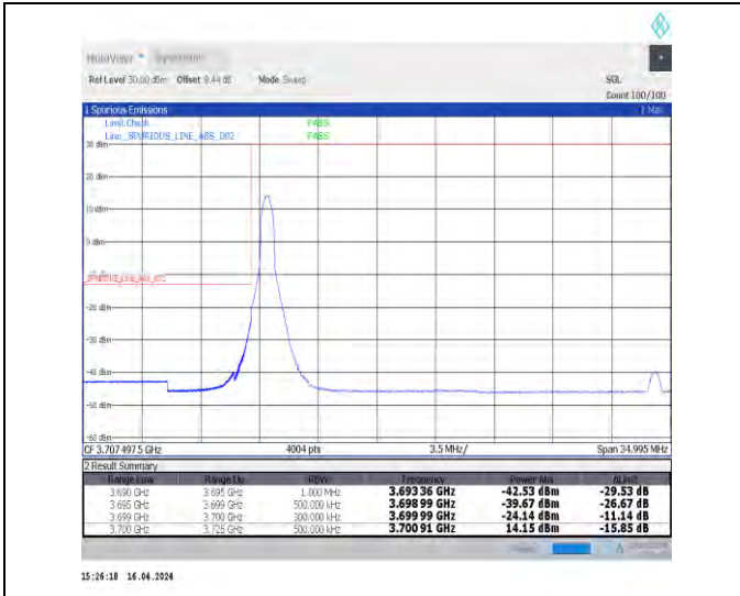
1-N78-3700-3800-N78-3700-380030-25-L-1-DFT-PI2B PSK-Edge_1RB_Left-1@0-Ant1-1--PASS-see graph
