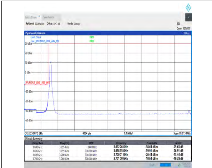
1-N78-3700-3800-30-60-L-1-DFT-PI2BPSK-Edge_1RB_Left-1@0-Ant1-1--PASS-see graph
