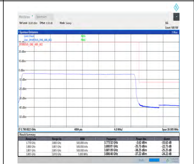
1-N78-3700-3800-30-30-H-6-CP-QPSK-Outer_Full-78@0-Ant1-1--PASS-see graph
