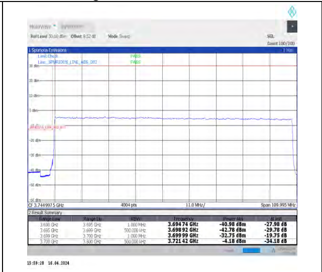
1-N78-3700-3800-N78-3700-380030-100-L-3-DFT-PI2BPSK-Outer_Full-270@0-Ant1-1--PASS-see graph
