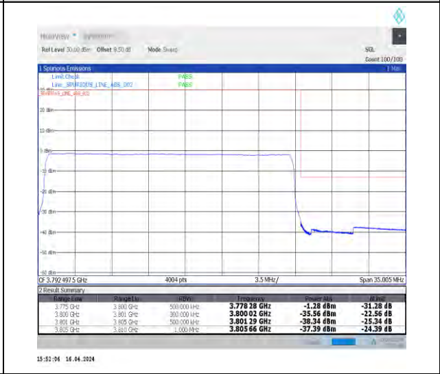
1-N78-3700-3800-N78-3700-380030-25-H-6-CP-Q PSK-Outer_Full-65@0-Ant1-1--PASS-see graph
