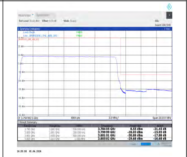
1-N78-3700-3800-N78-3700-380030-20-H-6-CP-Q PSK-Outer_Full-51@0-Ant1-1--PASS-see graph
