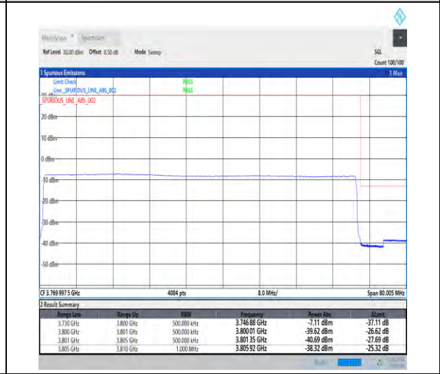
1-N78-3700-3800-30-70-H-6-CP-QPSK-Outer_Full-189@0-Ant1-1--PASS-see graph
