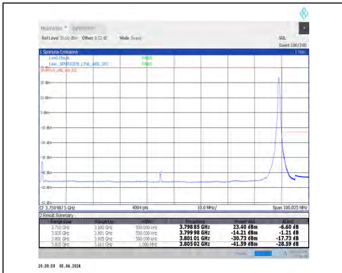
1-N78-3700-3800-N78-3700-380030-90-H-2-DFT-PI2 BPSK-Edge_1RB_Right-1@244-Ant1-1--PASS-see graph
