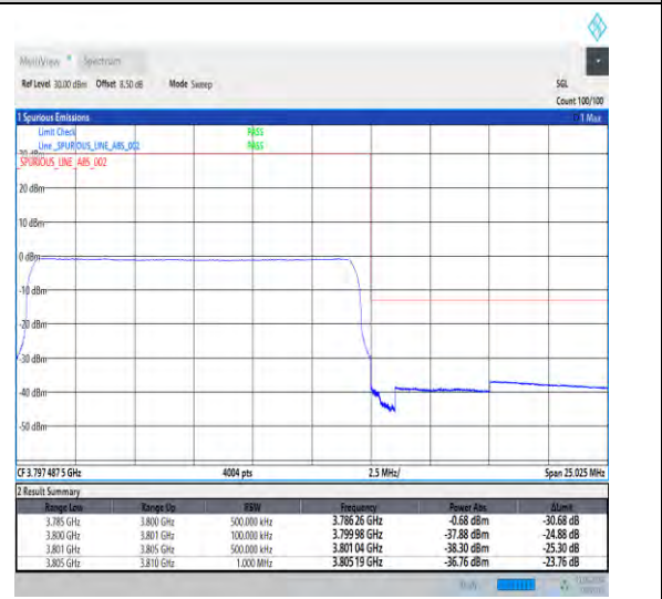
1-N78-3700-3800-30-15-H-6-CP-QPSK-Outer_Full-38@0-Ant1-1--PASS-see graph
