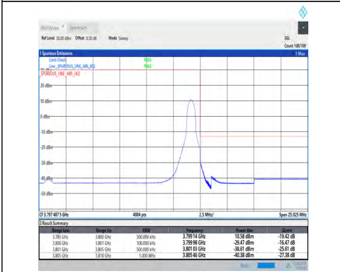
1-N78-3700-3800-30-15-H-5-CP-QPSK-Edge_1RB_Right-1@37-Ant1-1--PASS-see graph
