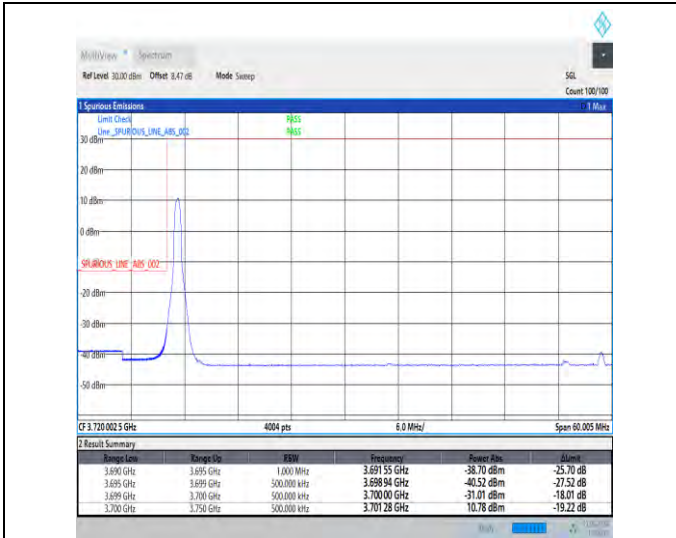
1-N78-3700-3800-30-50-L-1-DFT-PI2BPSK-Edge_1RB_Left-1@0-Ant1-1--PASS-see graph
