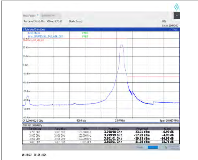
1-N78-3700-3800-N78-3700-380030-20-H-2-DFT-PI2 BPSK-Edge_1RB_Right-1@50-Ant1-1--PASS-see graph
