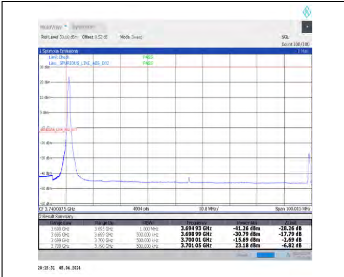
1-N78-3700-3800-N78-3700-380030-90-L-1-DFT-PI2B PSK-Edge_1RB_Left-1@0-Ant1-1--PASS-see graph
