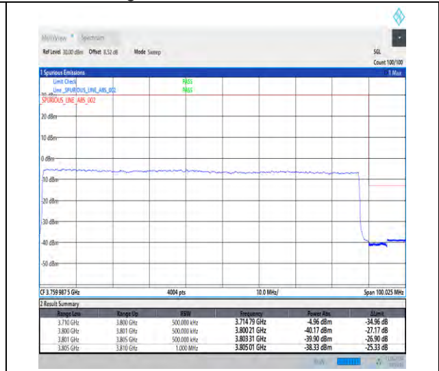
1-N78-3700-3800-30-90-H-3-DFT-PI2BPSK-Outer_Full-240@0-Ant1-1--PASS-see graph
