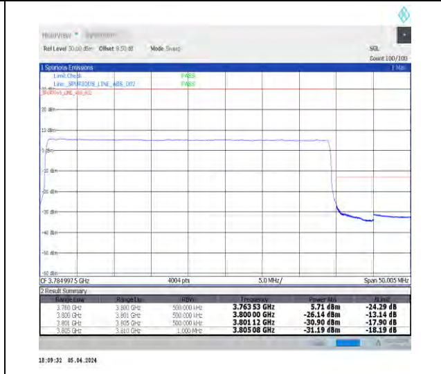
1-N78-3700-3800-N78-3700-380030-40-H-6-CP-Q PSK-Outer_Full-106@0-Ant1-1--PASS-see graph
