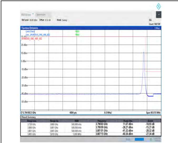
1-N78-3700-3800-30-80-H-2-DFT-PI2BPSK-Edge_1R_B_Right-1@216-Ant1-1--PASS-see graph
