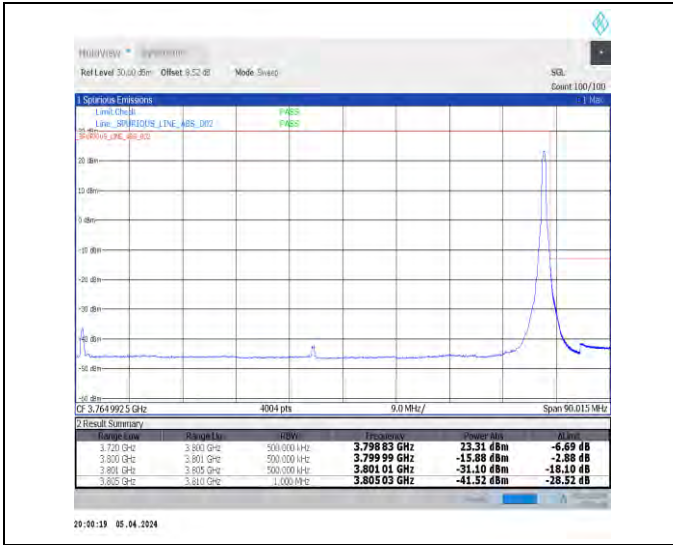
1-N78-3700-3800-N78-3700-380030-80-H-2-DFT-PI2 BPSK-Edge_1RB_Right-1@216-Ant1-1--PASS-see graph
