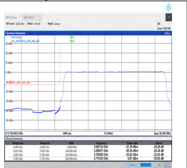
1-N78-3700-3800-30-20-L-3-DFT-PI2BPSK-Outer _Full-50@0-Ant1-1--PASS-see graph
