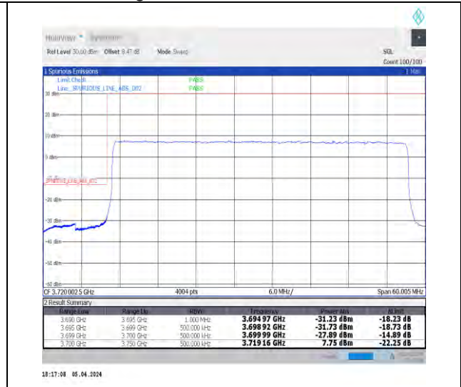
1-N78-3700-3800-N78-3700-380030-50-L-3-DFT-P I2BPSK-Outer_Full-128@0-Ant1-1--PASS-see graph
