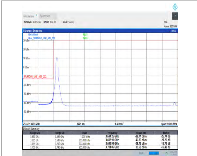
1-N78-3700-3800-30-40-L-1-DFT-PI2BPSK-Edge_1RB_Left-1@0-Ant1-1--PASS-see graph
