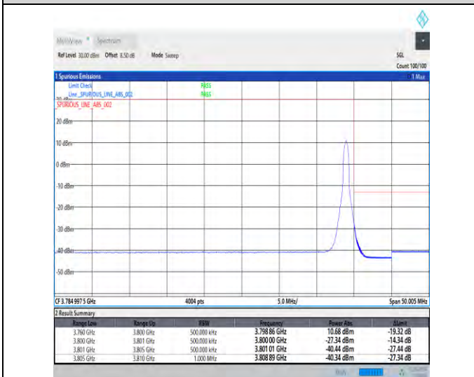
1-N78-3700-3800-30-40-H-5-CP-QPSK-Edge_1RB_Right-1@105-Ant1-1--PASS-see graph
