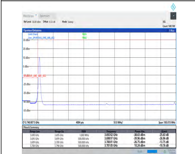
1-N78-3700-3800-30-90-L-4-CP-QPSK-Edge_1RB_Lef t-1@0-Ant1-1--PASS-see graph
