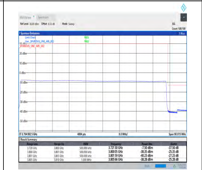
1-N78-3700-3800-30-80-H-6-CP-QPSK-Outer_Full-217@0-Ant1-1--PASS-see graph
