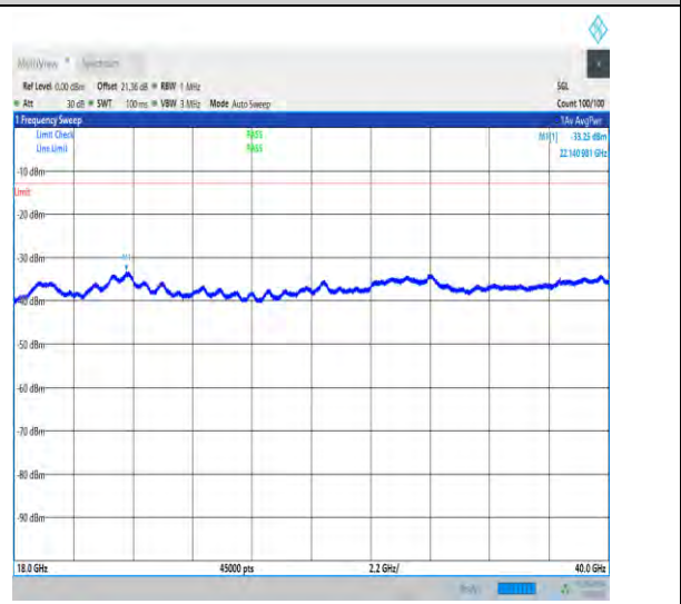
1-N78-3700-3800-30-100-M-1-DFT-QPSK-Edge_1R B_Left-1@0-18000-40000-Ant1-22140.98--33.25--13- PASS
