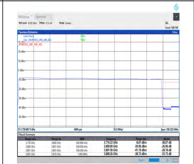
1-N78-3700-3800-30-90-H-6-CP-QPSK-Outer_Full-245@0-Ant1-1--PASS-see graph
