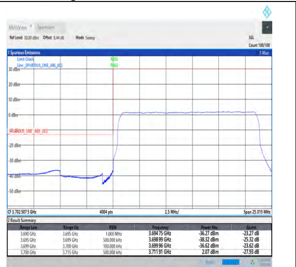
1-N78-3700-3800-30-15-L-3-DFT-PI2BPSK-Outer _Full-36@0-Ant1-1--PASS-see graph
