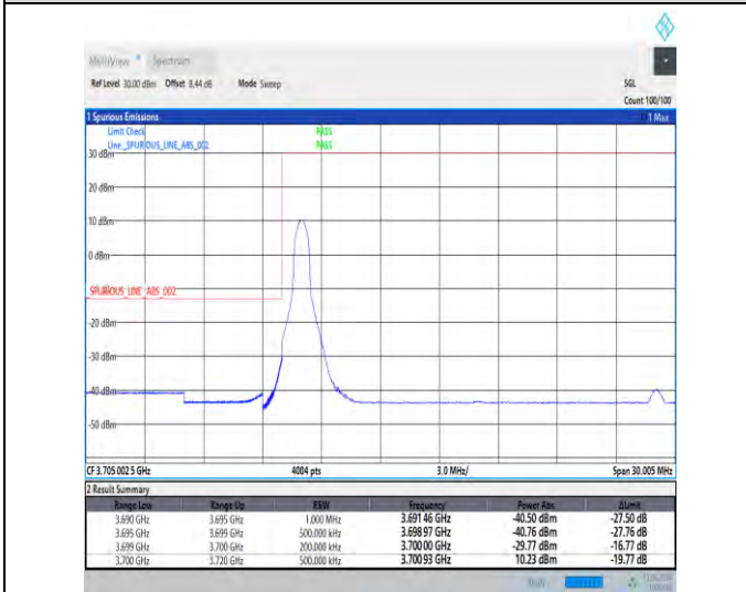
1-N78-3700-3800-30-20-L-4-CP-QPSK-Edge_1RB_Lef t-1@0-Ant1-1--PASS-see graph
