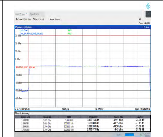
1-N78-3700-3800-30-90-L-6-CP-QPSK-Outer_Full -245@0-Ant1-1--PASS-see graph
