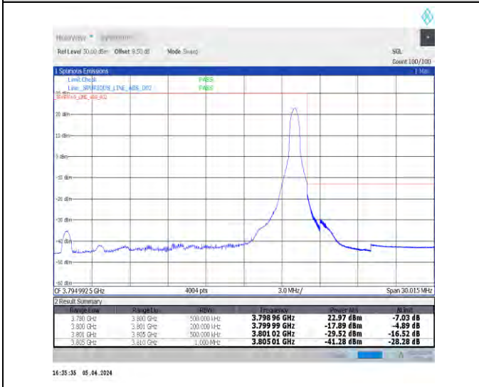
1-N78-3700-3800-N78-3700-380030-20-H-5-CP-QPS K-Edge_1RB_Right-1@50-Ant1-1--PASS-see graph
