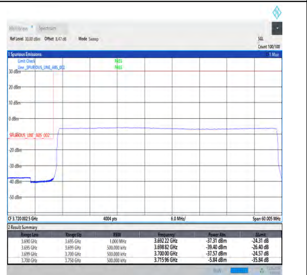
1-N78-3700-3800-30-50-L-6-CP-QPSK-Outer_Full -133@0-Ant1-1--PASS-see graph
