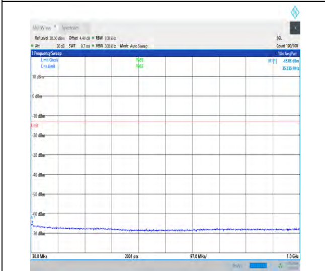
1-N78-3700-3800-30-100-H-1-DFT-QPSK-Edge_1R B_Left-1@0-30-1000-Ant1-35.34--65.08--13-PASS
