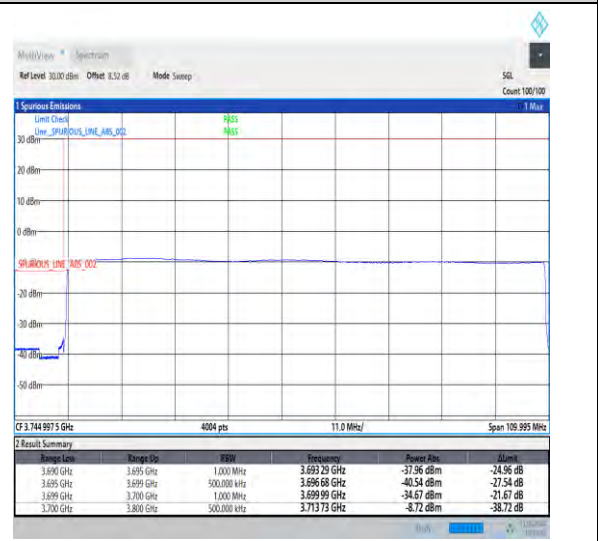
1-N78-3700-3800-30-100-L-6-CP-QPSK-Outer_Full-273@0-Ant1-1--PASS-see graph
