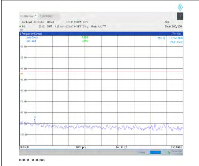
1-N78-3700-3800-N78-3700-380030-100-M-1-DFT-P I2BPSK-Inner_1RB_Left-1@1-0.009-0.15-Ant1-0.0 1--87.56--43-PASS
