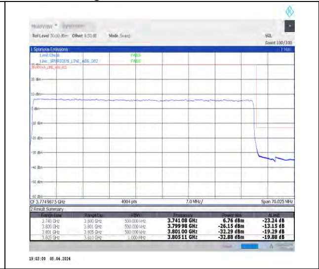
1-N78-3700-3800-N78-3700-380030-60-H-3-DFT-PI2BPSK-Outer_Full-162@0-Ant1-1--PASS-see graph
