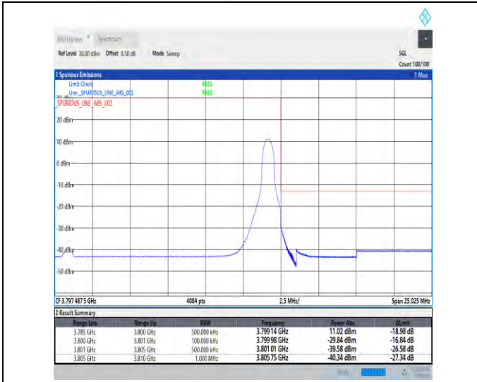
1-N78-3700-3800-30-15-H-2-DFT-PI2BPSK-Edge_1R_B_Right-1@37-Ant1-1--PASS-see graph
