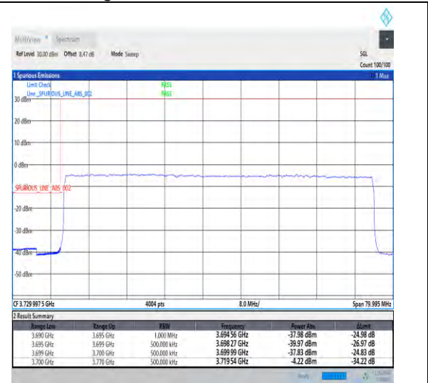
1-N78-3700-3800-30-70-L-3-DFT-PI2BPSK-Outer _Full-180@0-Ant1-1--PASS-see graph
