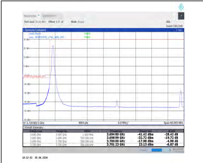
1-N78-3700-3800-N78-3700-380030-50-L-1-DFT-PI2B PSK-Edge_1RB_Left-1@0-Ant1-1--PASS-see graph
