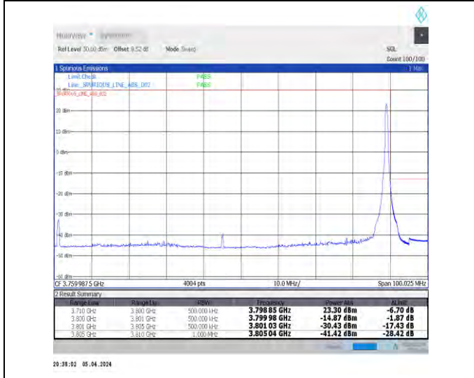
1-N78-3700-3800-N78-3700-380030-90-H-5-CP-QPS K-Edge_1RB_Right-1@244-Ant1-1--PASS-see graph
