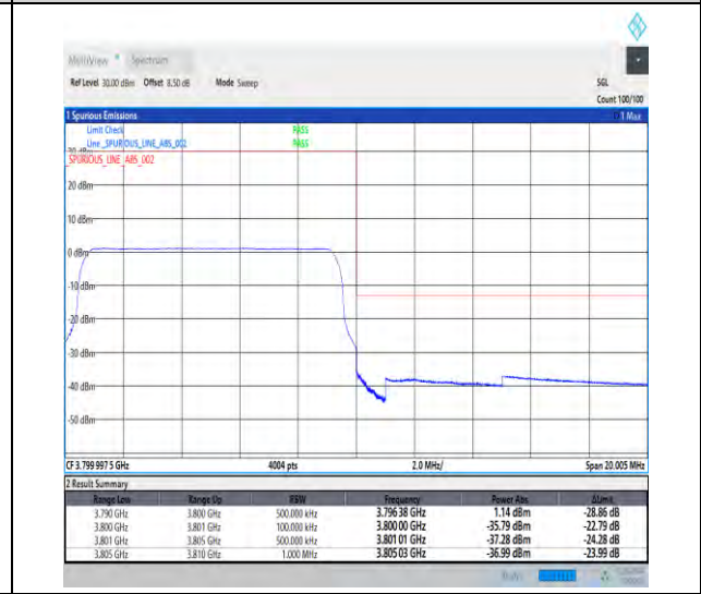
1-N78-3700-3800-30-10-H-6-CP-QPSK-Outer_Full-24@0-Ant1-1--PASS-see graph
