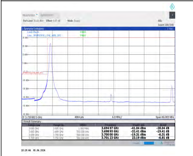
1-N78-3700-3800-N78-3700-380030-50-L-4-CP-QPSK -Edge_1RB_Left-1@0-Ant1-1--PASS-see graph
