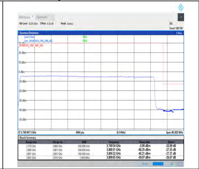
1-N78-3700-3800-30-70-H-3-DFT-PI2BPSK-Outer_Full-180@0-Ant1-1--PASS-see graph
