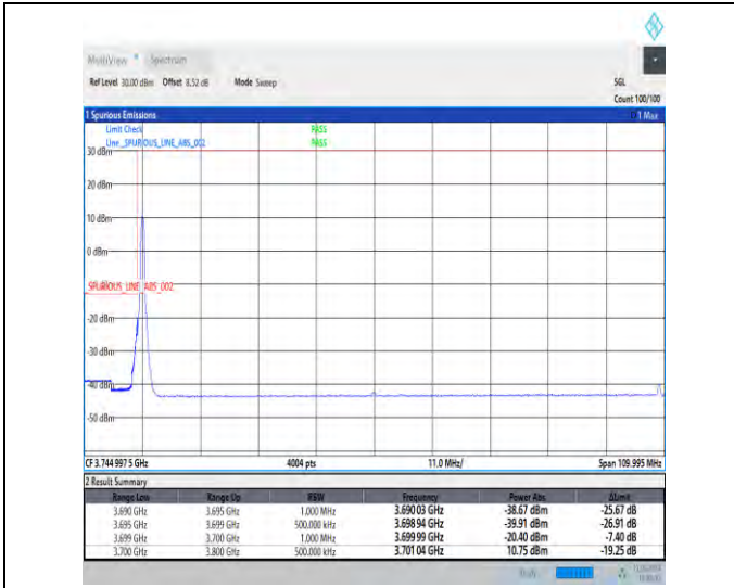
1-N78-3700-3800-100-L-1-DFT-PI2BPSK-Edge_1R_B_Left-1@0-Ant1-1--PASS-see graph
