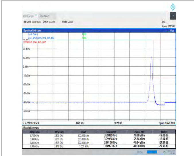
1-N78-3700-3800-30-60-H-2-DFT-PI2BPSK-Edge_1R_B_Right-1@161-Ant1-1--PASS-see graph
