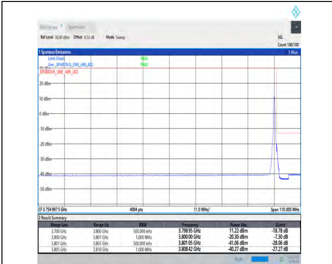
1-N78-3700-3800-30-100-H-2-DFT-PI2BPSK-Edge_1R_B_Right-1@272-Ant1-1--PASS-see graph
