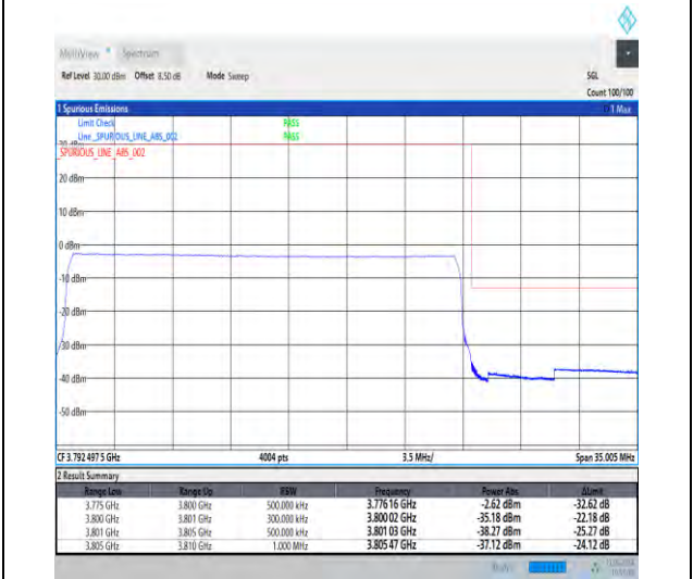
1-N78-3700-3800-30-25-H-6-CP-QPSK-Outer_Full-65@0-Ant1-1--PASS-see graph
