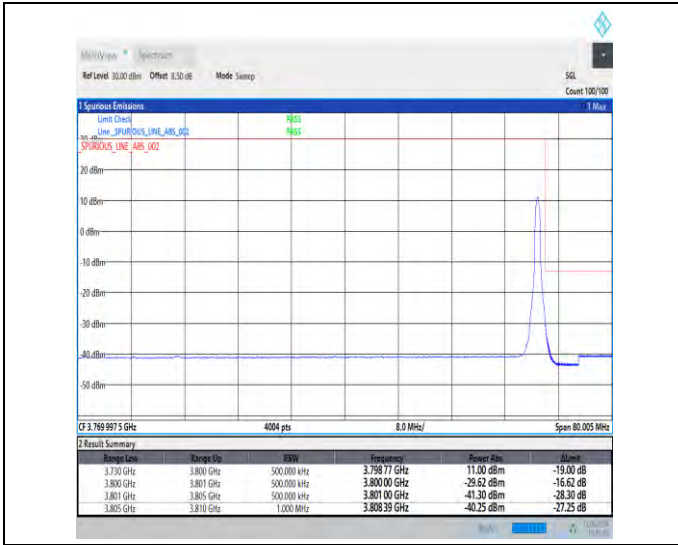
1-N78-3700-3800-30-70-H-2-DFT-PI2BPSK-Edge_1R_B_Right-1@188-Ant1-1--PASS-see graph
