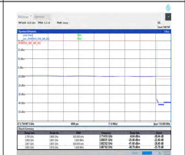
1-N78-3700-3800-30-100-H-6-CP-QPSK-Outer_Full-273@0-Ant1-1--PASS-see graph
