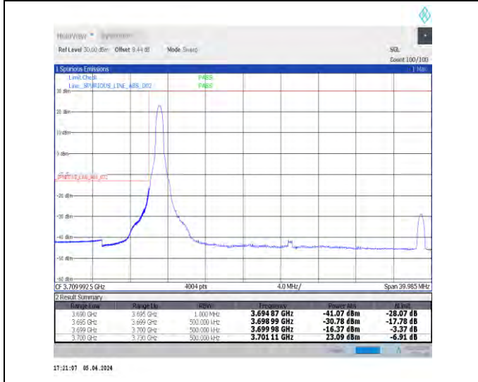
1-N78-3700-3800-N78-3700-380030-30-L-4-CP-QPSK -Edge_1RB_Left-1@0-Ant1-1--PASS-see graph
