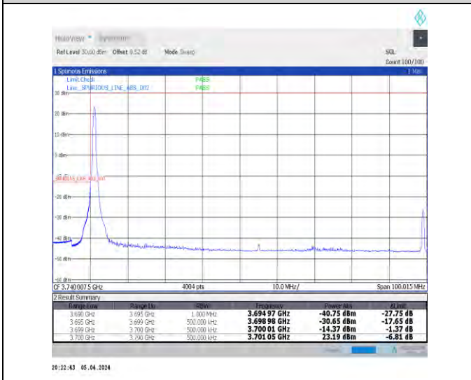
1-N78-3700-3800-N78-3700-380030-90-L-4-CP-QPSK -Edge_1RB_Left-1@0-Ant1-1--PASS-see graph
