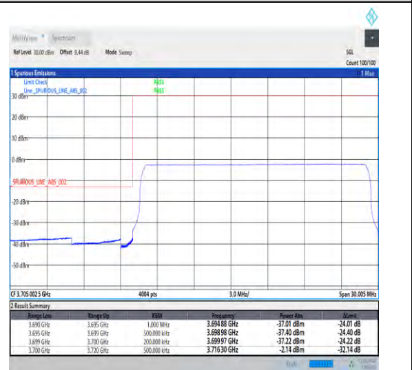
1-N78-3700-3800-30-20-L-6-CP-QPSK-Outer_Full -51@0-Ant1-1--PASS-see graph
