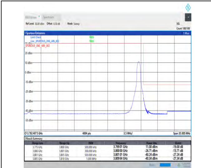
1-N78-3700-3800-30-25-H-2-DFT-PI2BPSK-Edge_1R_B_Right-1@64-Ant1-1--PASS-see graph
