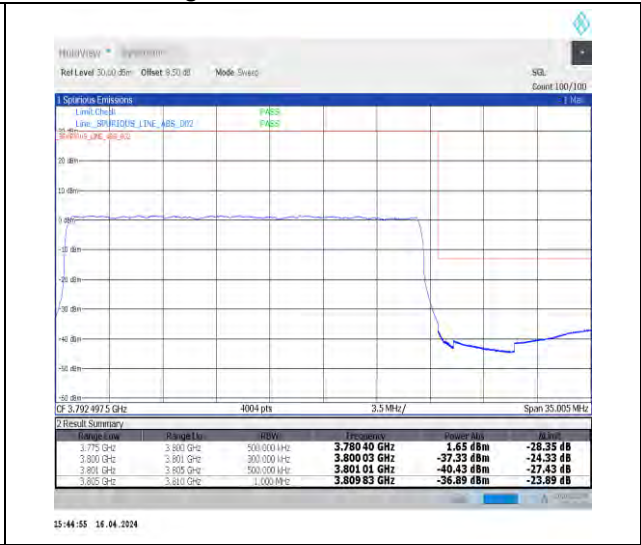
1-N78-3700-3800-N78-3700-380030-25-H-3-DFT-PI2 BPSK-Outer_Full-64@0-Ant1-1--PASS-see graph
