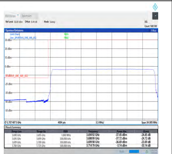
1-N78-3700-3800-30-25-L-6-CP-QPSK-Outer_Full -65@0-Ant1-1--PASS-see graph
