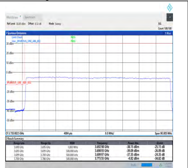
1-N78-3700-3800-30-80-L-3-DFT-PI2BPSK-Outer_Full-216@0-Ant1-1--PASS-see graph
