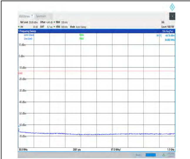
1-N78-3700-3800-30-100-M-1-DFT-QPSK-Edge_1R B_Left-1@0-30-1000-Ant1-34.85--64.76--13-PASS
