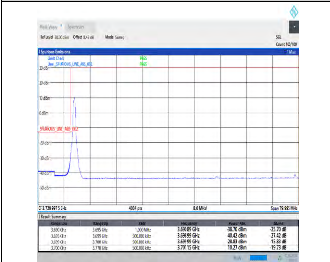
1-N78-3700-3800-30-70-L-4-CP-QPSK-Edge_1RB_Lef t-1@0-Ant1-1--PASS-see graph
