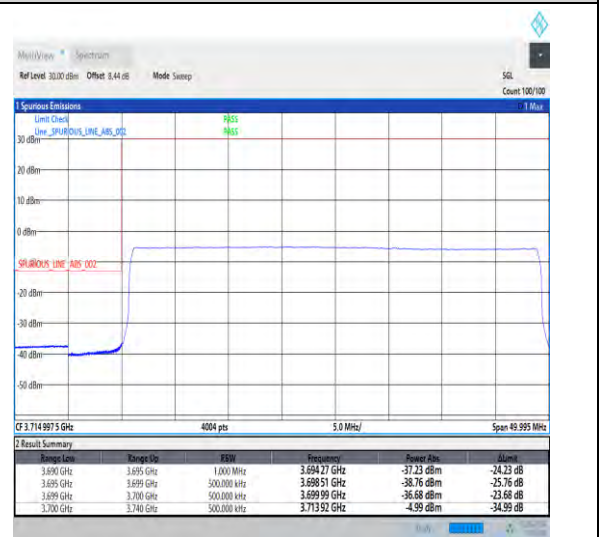
1-N78-3700-3800-30-40-L-6-CP-QPSK-Outer_Full -106@0-Ant1-1--PASS-see graph
