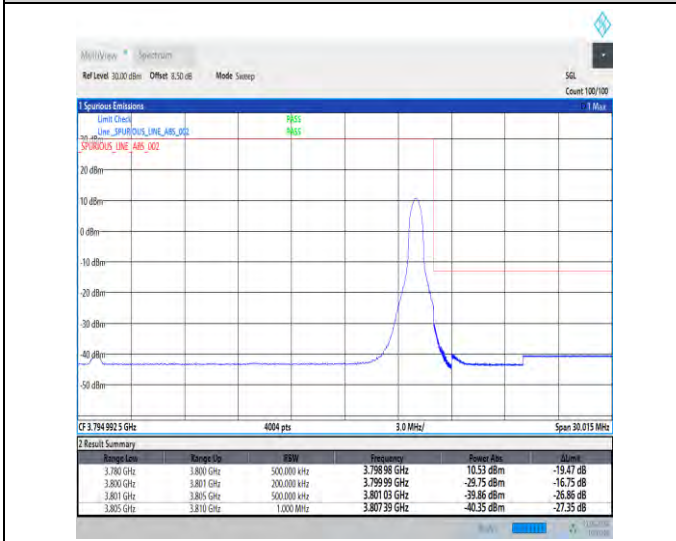
1-N78-3700-3800-30-20-H-5-CP-QPSK-Edge_1RB_Right-1@50-Ant1-1--PASS-see graph
