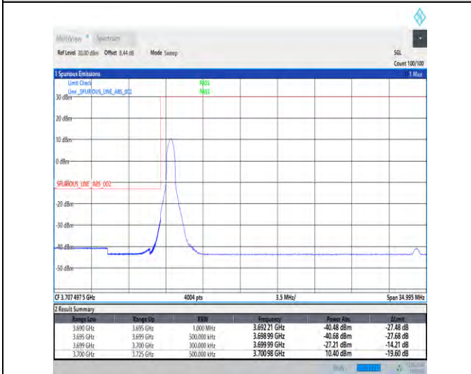
1-N78-3700-3800-30-25-L-4-CP-QPSK-Edge_1RB_Lef t-1@0-Ant1-1--PASS-see graph
