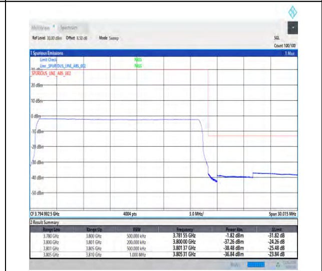
1-N78-3700-3800-30-20-H-6-CP-QPSK-Outer_Full-51@0-Ant1-1--PASS-see graph
