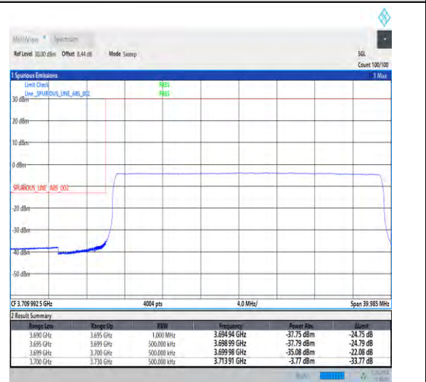
1-N78-3700-3800-30-30-L-6-CP-QPSK-Outer_Full -78@0-Ant1-1--PASS-see graph
