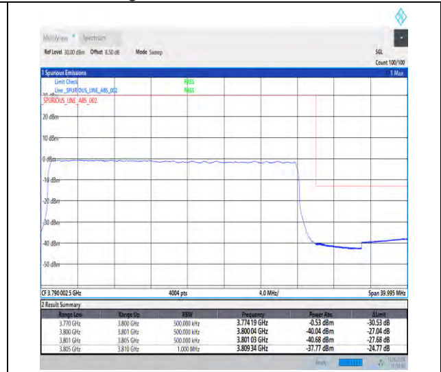
1-N78-3700-3800-30-30-H-3-DFT-PI2BPSK-Outer_Full-75@0-Ant1-1--PASS-see graph
