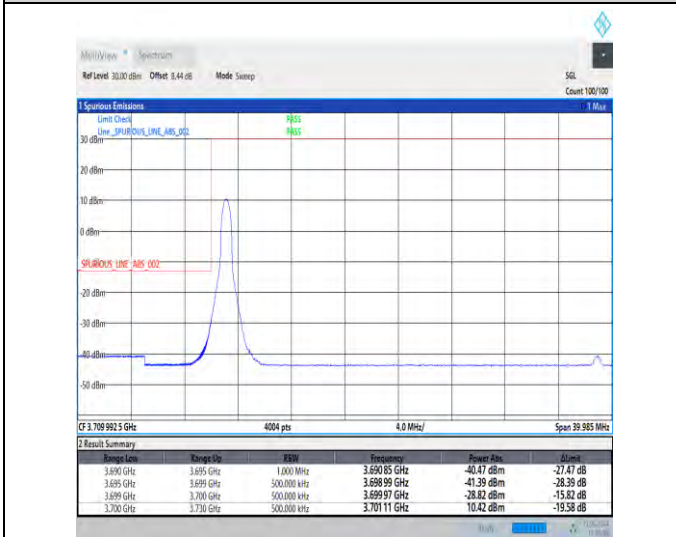
1-N78-3700-3800-30-30-L-4-CP-QPSK-Edge_1RB_Lef t-1@0-Ant1-1--PASS-see graph
