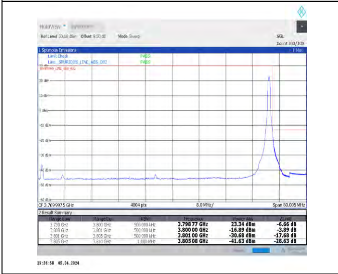
1-N78-3700-3800-N78-3700-380030-70-H-5-CP-QPS K-Edge_1RB_Right-1@188-Ant1-1--PASS-see graph
