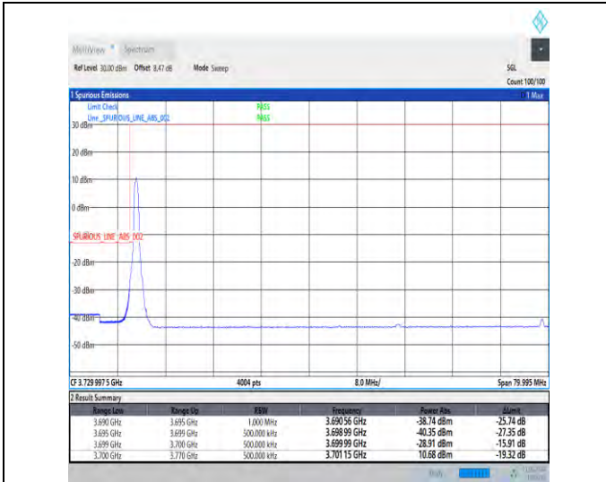
1-N78-3700-3800-30-70-L-1-DFT-PI2BPSK-Edge_1RB _Left-1@0-Ant1-1--PASS-see graph
