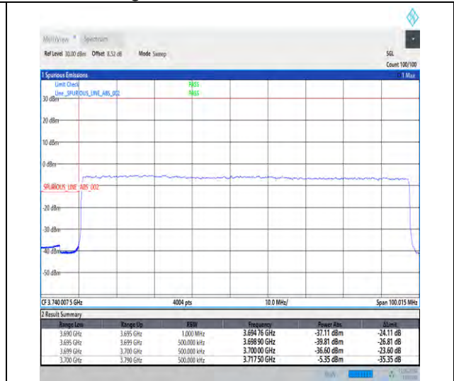
1-N78-3700-3800-30-90-L-3-DFT-PI2BPSK-Outer_Full-240@0-Ant1-1--PASS-see graph
