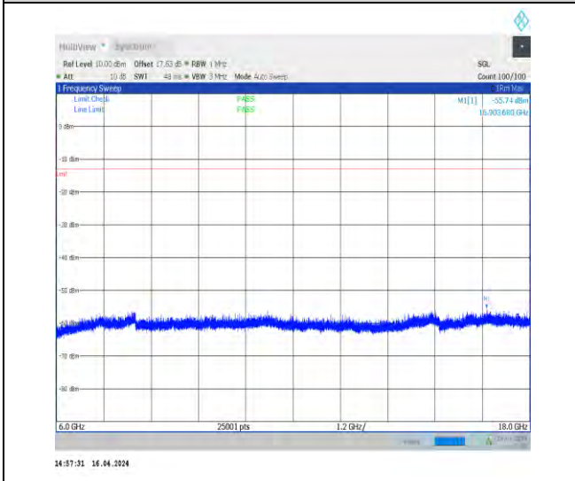
1-N78-3700-3800-N78-3700-380030-100-M-1-DFT-PI2BPSK-Inner_1RB_Left-1@1-6000-18000-Ant1-11 104.32--55.74--13-PASS
