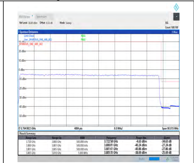
1-N78-3700-3800-30-80-H-3-DFT-PI2BPSK-Outer_Full-216@0-Ant1-1--PASS-see graph
