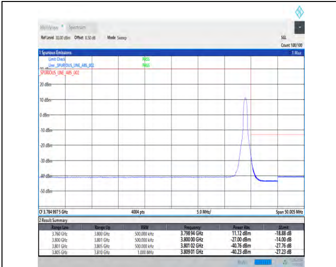
1-N78-3700-3800-30-40-H-2-DFT-PI2BPSK-Edge_1R_B_Right-1@105-Ant1-1--PASS-see graph
