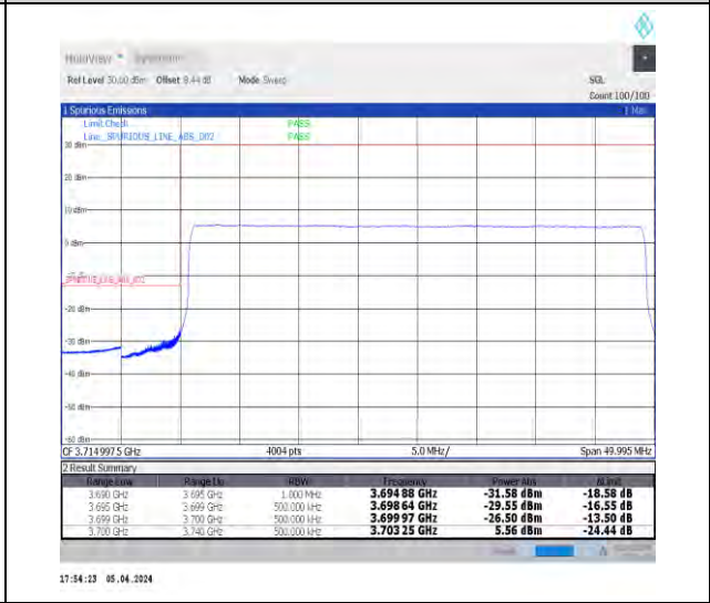
1-N78-3700-3800-N78-3700-380030-40-L-6-CP-Q PSK-Outer_Full-106@0-Ant1-1--PASS-see graph
