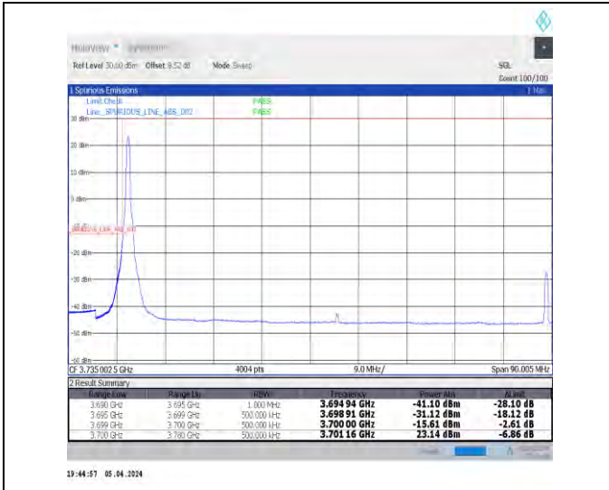
1-N78-3700-3800-N78-3700-380030-80-L-1-DFT-PI2B PSK-Edge_1RB_Left-1@0-Ant1-1--PASS-see graph
