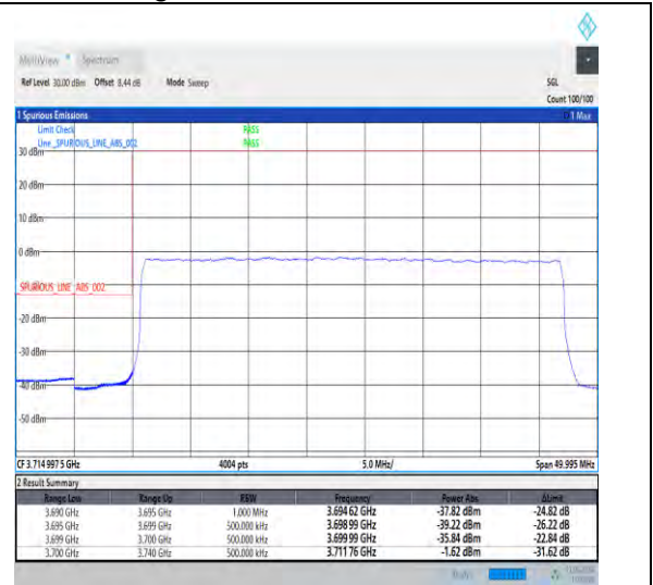
1-N78-3700-3800-30-40-L-3-DFT-PI2BPSK-Outer_Full-100@0-Ant1-1--PASS-see graph
