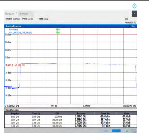
1-N78-3700-3800-30-80-L-6-CP-QPSK-Outer_Full -217@0-Ant1-1--PASS-see graph
