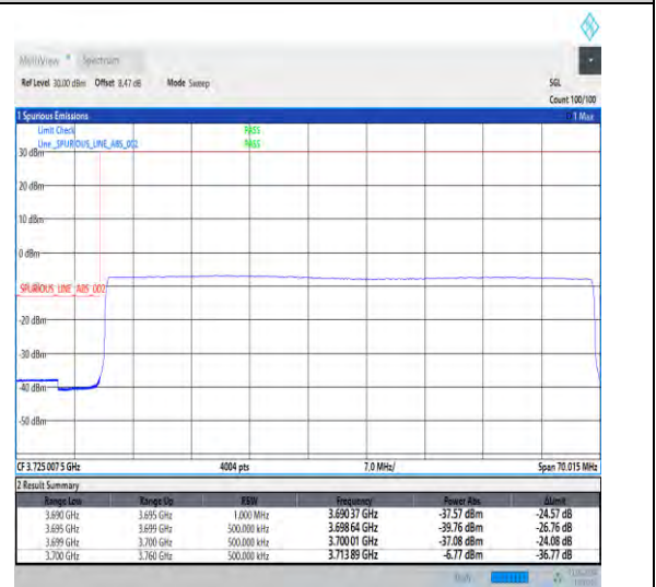
1-N78-3700-3800-30-60-L-6-CP-QPSK-Outer_Full -162@0-Ant1-1--PASS-see graph
