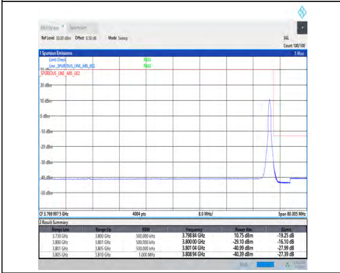
1-N78-3700-3800-30-70-H-5-CP-QPSK-Edge_1RB_Right-1@188-Ant1-1--PASS-see graph
