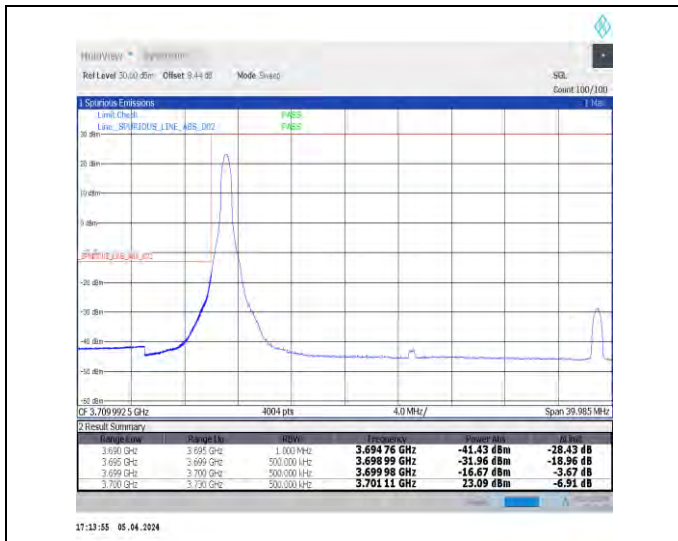
1-N78-3700-3800-N78-3700-380030-30-L-1-DFT-PI2B PSK-Edge_1RB_Left-1@0-Ant1-1--PASS-see graph
