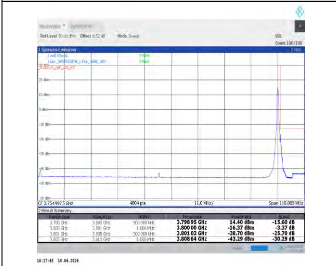
1-N78-3700-3800-N78-3700-380030-100-H-5-CP-QP SK-Edge_1RB_Right-1@272-Ant1-1--PASS-see graph
