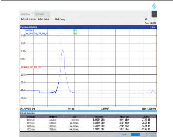
1-N78-3700-3800-30-25-L-1-DFT-PI2BPSK-Edge_1RB _Left-1@0-Ant1-1--PASS-see graph
