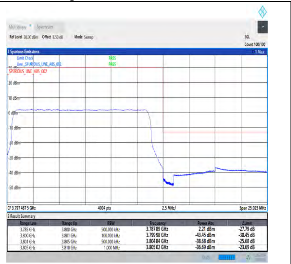
1-N78-3700-3800-30-15-H-3-DFT-PI2BPSK-Outer_Full-36@0-Ant1-1--PASS-see graph
