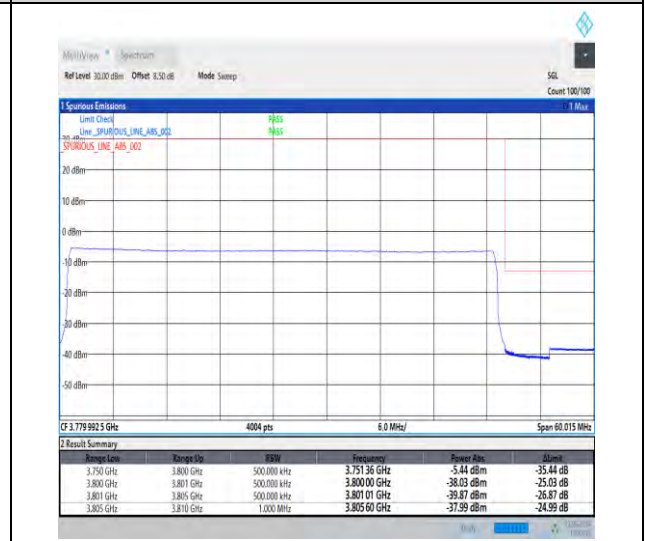
1-N78-3700-3800-30-50-H-6-CP-QPSK-Outer_Full-133@0-Ant1-1--PASS-see graph
