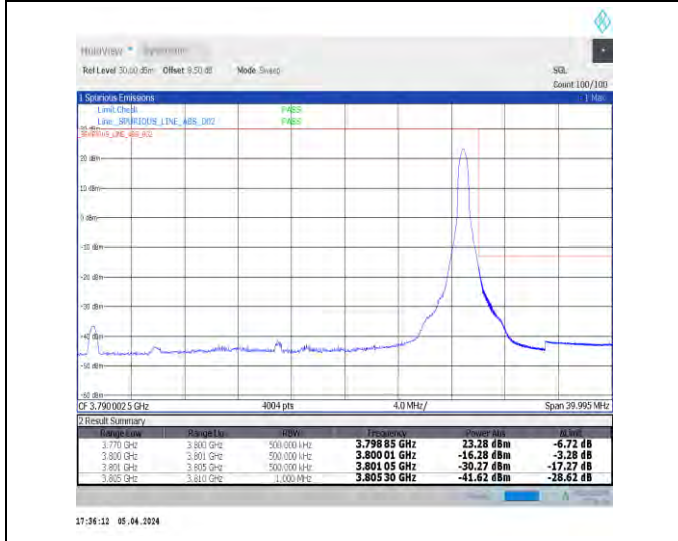
1-N78-3700-3800-N78-3700-380030-30-H-5-CP-QPS K-Edge_1RB_Right-1@77-Ant1-1--PASS-see graph
