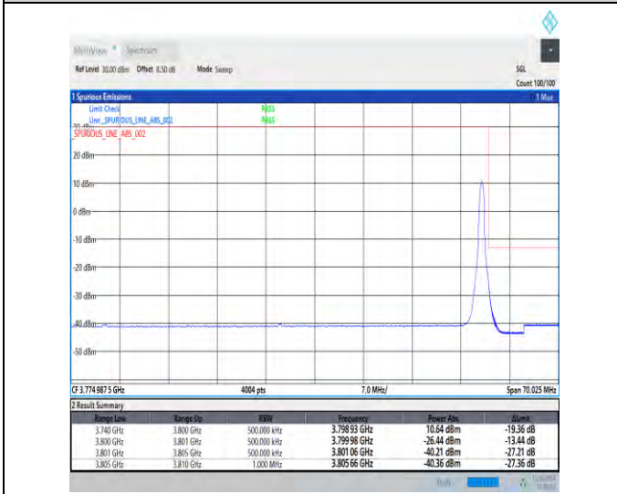
1-N78-3700-3800-30-60-H-5-CP-QPSK-Edge_1RB_Right-1@161-Ant1-1--PASS-see graph
