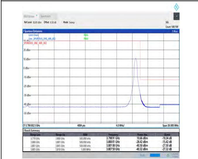
1-N78-3700-3800-30-30-H-5-CP-QPSK-Edge_1RB_Right-1@77-Ant1-1--PASS-see graph
