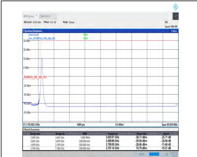
1-N78-3700-3800-30-80-L-1-DFT-PI2BPSK-Edge_1RB_Left-1@0-Ant1-1--PASS-see graph
