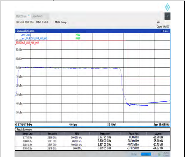
1-N78-3700-3800-30-25-H-3-DFT-PI2BPSK-Outer_Full-64@0-Ant1-1--PASS-see graph
