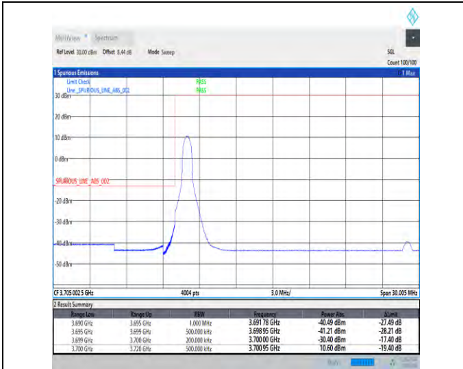
1-N78-3700-3800-30-20-L-1-DFT-PI2BPSK-Edge_1RB _Left-1@0-Ant1-1--PASS-see graph
