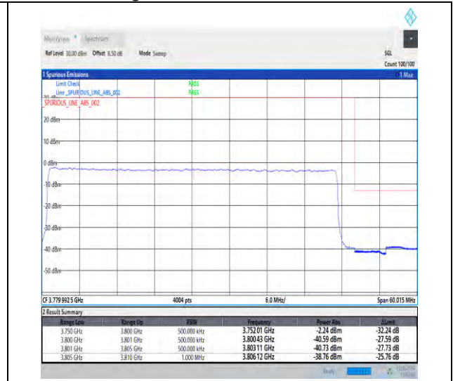
1-N78-3700-3800-30-50-H-3-DFT-PI2BPSK-Outer_Full-128@0-Ant1-1--PASS-see graph
