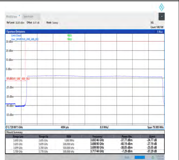
1-N78-3700-3800-30-70-L-6-CP-QPSK-Outer_Full -189@0-Ant1-1--PASS-see graph
