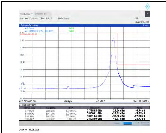
1-N78-3700-3800-N78-3700-380030-30-H-2-DFT-PI2 BPSK-Edge_1RB_Right-1@77-Ant1-1--PASS-see graph
