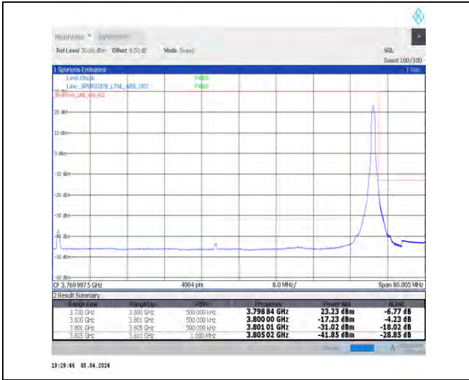
1-N78-3700-3800-N78-3700-380030-70-H-2-DFT-PI2 BPSK-Edge_1RB_Right-1@188-Ant1-1--PASS-see graph
