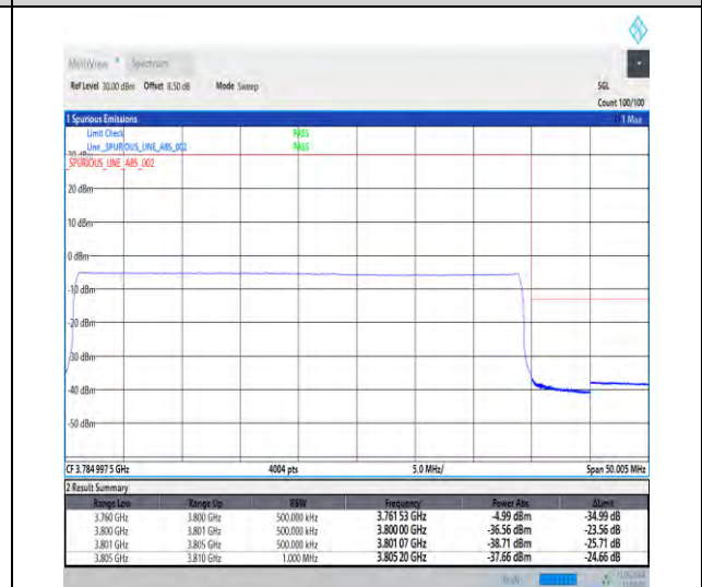
1-N78-3700-3800-30-40-H-6-CP-QPSK-Outer_Full-106@0-Ant1-1--PASS-see graph
