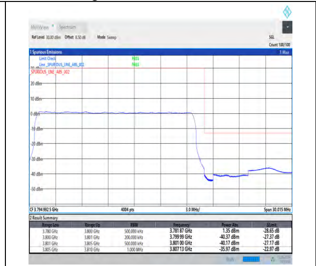
1-N78-3700-3800-30-20-H-3-DFT-PI2BPSK-Outer_Full-50@0-Ant1-1--PASS-see graph
