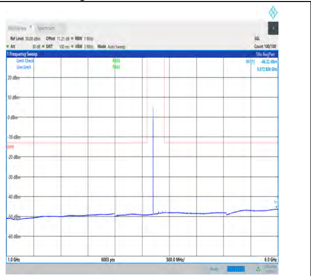
1-N78-3700-3800-30-100-M-1-DFT-QPSK-Edge_1R B_Left-1@0-1000-6000-Ant1-5972.51--46.22--13-PA SS
