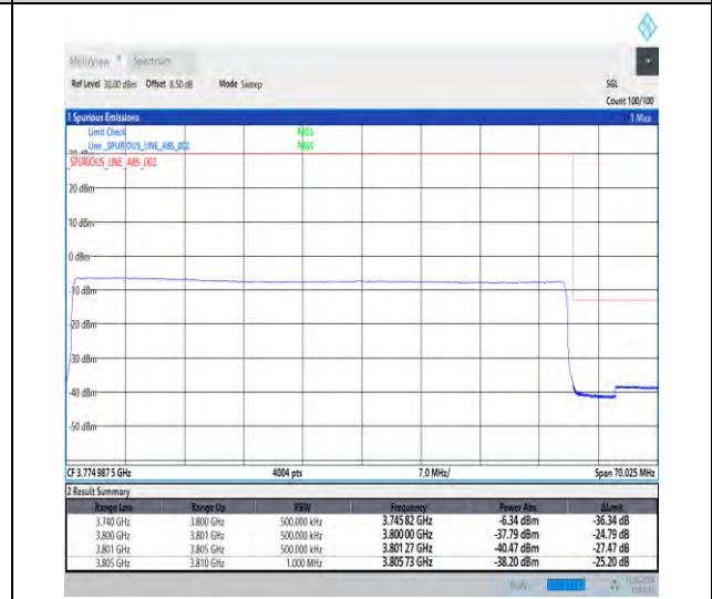
1-N78-3700-3800-30-60-H-6-CP-QPSK-Outer_Full-162@0-Ant1-1--PASS-see graph
