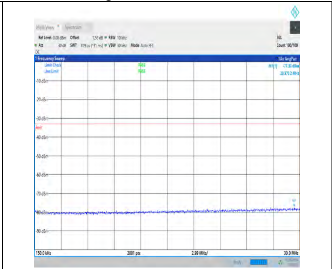
1-N78-3700-3800-30-100-H-1-DFT-QPSK-Edge_1RB _Left-1@0-0.15-30-Ant1-29.37--77.33--33-PASS
