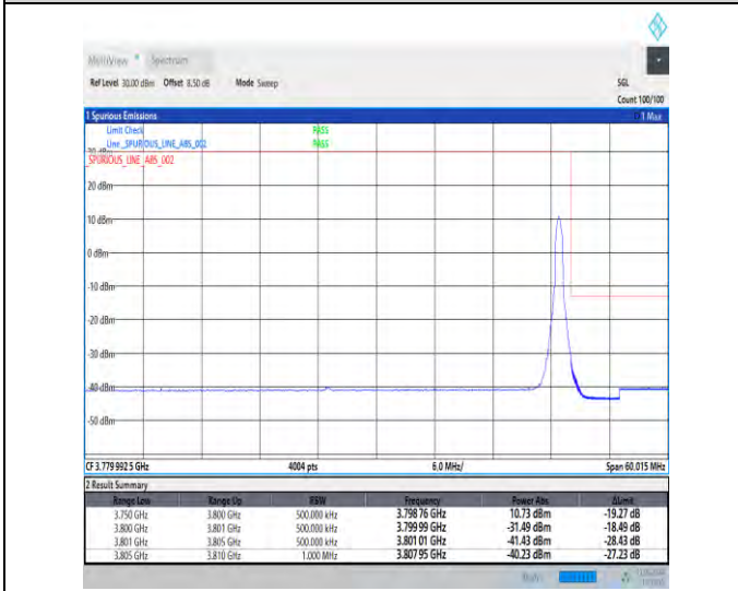
1-N78-3700-3800-30-50-H-5-CP-QPSK-Edge_1RB_Right-1@132-Ant1-1--PASS-see graph
