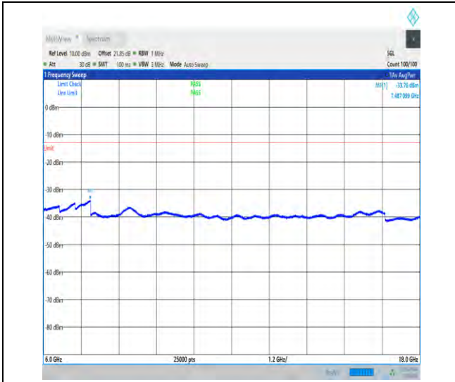
1-N78-3700-3800-30-100-H-1-DFT-QPSK-Edge_1R B_Left-1@0-6000-18000-Ant1-7487.10--33.76--13-P ASS
