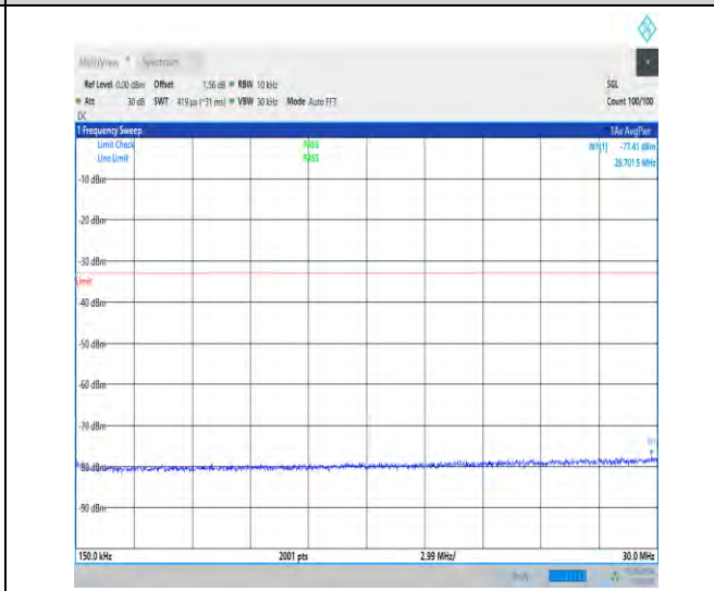
1-N78-3700-3800-30-100-M-1-DFT-QPSK-Edge_1R B_Left-1@0-0.15-30-Ant1-29.70--77.41--33-PASS
