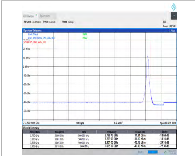
1-N78-3700-3800-30-50-H-2-DFT-PI2BPSK-Edge_1R_B_Right-1@132-Ant1-1--PASS-see graph
