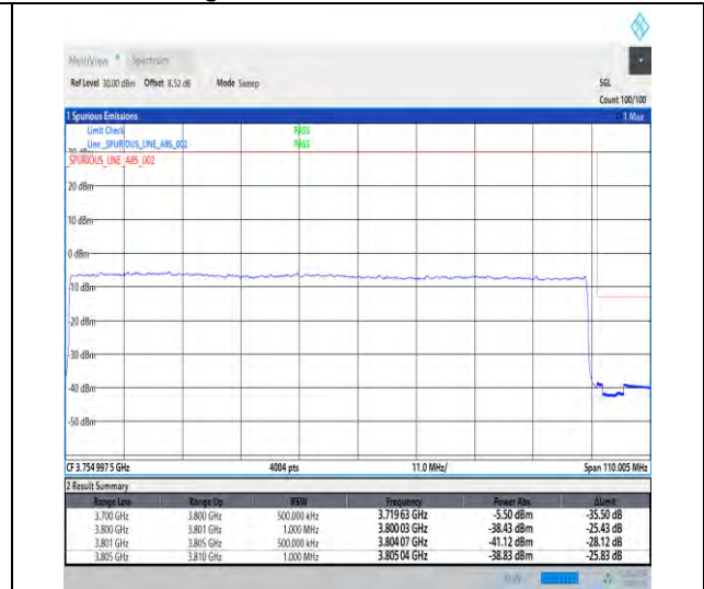
1-N78-3700-3800-30-100-H-3-DFT-PI2BPSK-Outer_Full-270@0-Ant1-1--PASS-see graph
