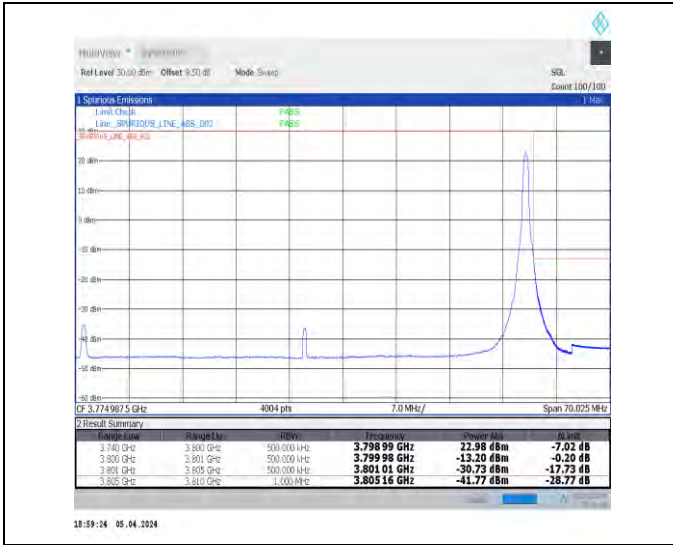
1-N78-3700-3800-N78-3700-380030-60-H-2-DFT-PI2 BPSK-Edge_1RB_Right-1@161-Ant1-1--PASS-see graph
