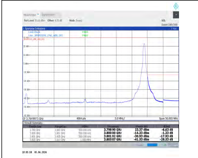
1-N78-3700-3800-N78-3700-380030-40-H-5-CP-QPS K-Edge_1RB_Right-1@105-Ant1-1--PASS-see graph
