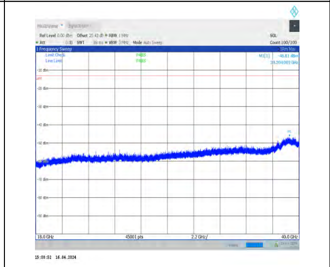
1-N78-3700-3800-N78-3700-380030-100-M-1-DFT-PI2BPSK-Inner_1RB_Left-1@1-18000-40000-Ant1-18 506.49--46.81--13-PASS
