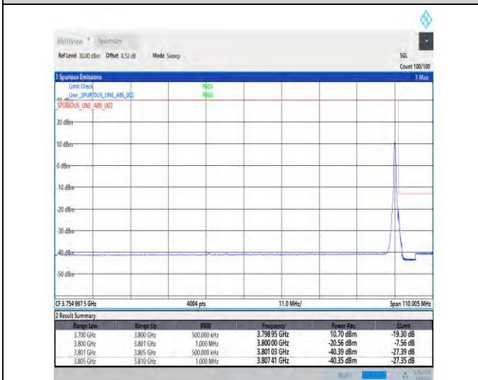
1-N78-3700-3800-30-100-H-5-CP-QPSK-Edge_1RB_Right-1@272-Ant1-1--PASS-see graph
