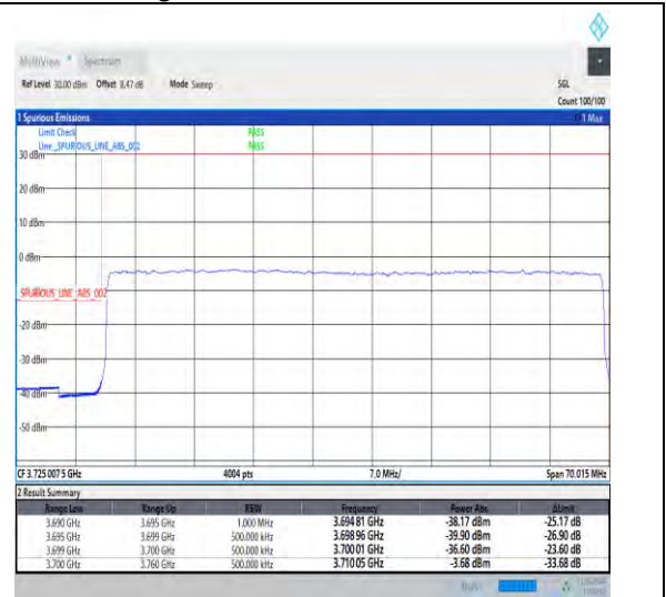
1-N78-3700-3800-30-60-L-3-DFT-PI2BPSK-Outer_Full-162@0-Ant1-1--PASS-see graph
