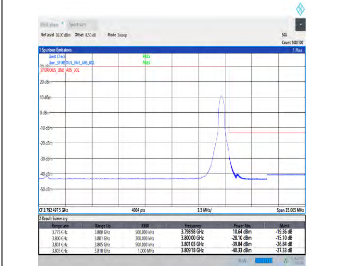
1-N78-3700-3800-30-25-H-5-CP-QPSK-Edge_1RB_Right-1@64-Ant1-1--PASS-see graph
