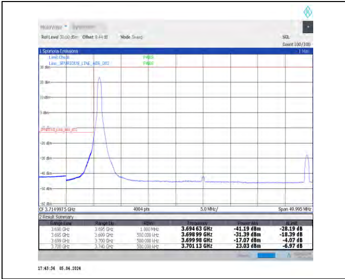
1-N78-3700-3800-N78-3700-380030-40-L-1-DFT-PI2B PSK-Edge_1RB_Left-1@0-Ant1-1--PASS-see graph
