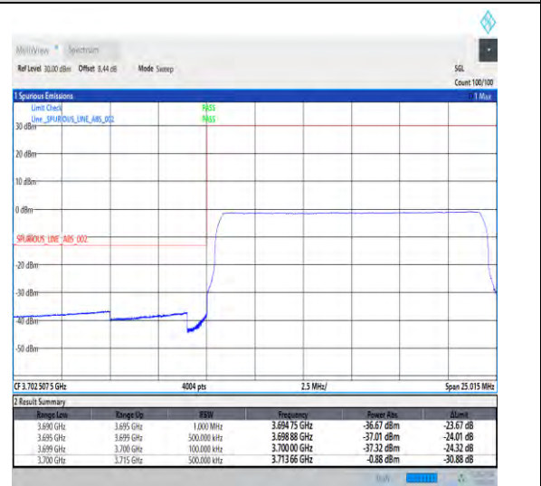
1-N78-3700-3800-30-15-L-6-CP-QPSK-Outer_Full -38@0-Ant1-1--PASS-see graph
