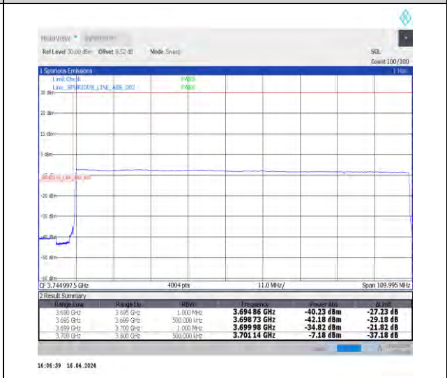
1-N78-3700-3800-N78-3700-380030-100-L-6-CP-QPSK-Outer_Full-273@0-Ant1-1--PASS-see graph
