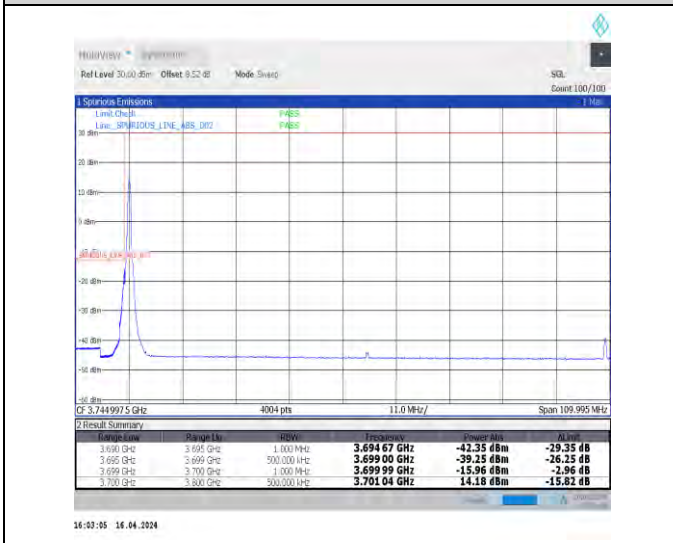
1-N78-3700-3800-N78-3700-380030-100-L-4-CP-QPS K-Edge_1RB_Left-1@0-Ant1-1--PASS-see graph
