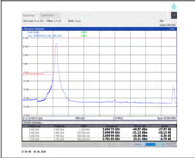
1-N78-3700-3800-N78-3700-380030-40-L-4-CP-QPSK -Edge_1RB_Left-1@0-Ant1-1--PASS-see graph
