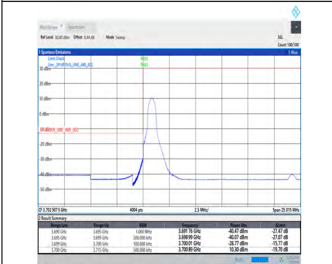
1-N78-3700-3800-30-15-L-4-CP-QPSK-Edge_1RB_Lef t-1@0-Ant1-1--PASS-see graph
