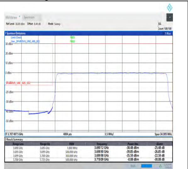
1-N78-3700-3800-30-25-L-3-DFT-PI2BPSK-Outer _Full-64@0-Ant1-1--PASS-see graph
