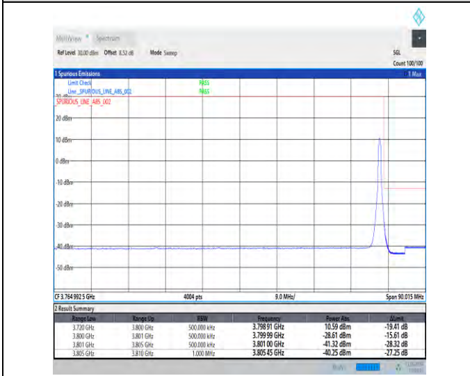
1-N78-3700-3800-30-80-H-5-CP-QPSK-Edge_1RB_Right-1@216-Ant1-1--PASS-see graph
