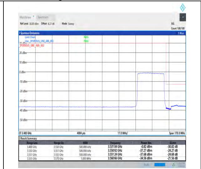
1-N78-3450-3550-30-30-H-3-DFT-PI2BPSK-Outer_Full-75@0-Ant1-1--PASS-see graph
