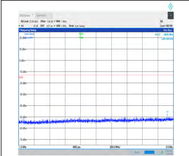
1-N78-3450-3550-30-100-M-1-DFT-QPSK-Edge_1R B_Left-1@0-1000-3000-Ant1-2921.52--48.95--13-PA
