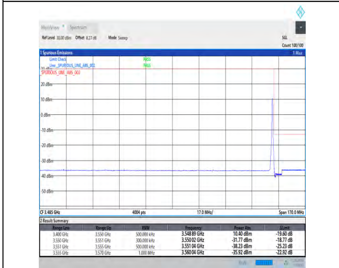
1-N78-3450-3550-30-40-H-5-CP-QPSK-Edge_1RB_Right-1@105-Ant1-1--PASS-see graph
