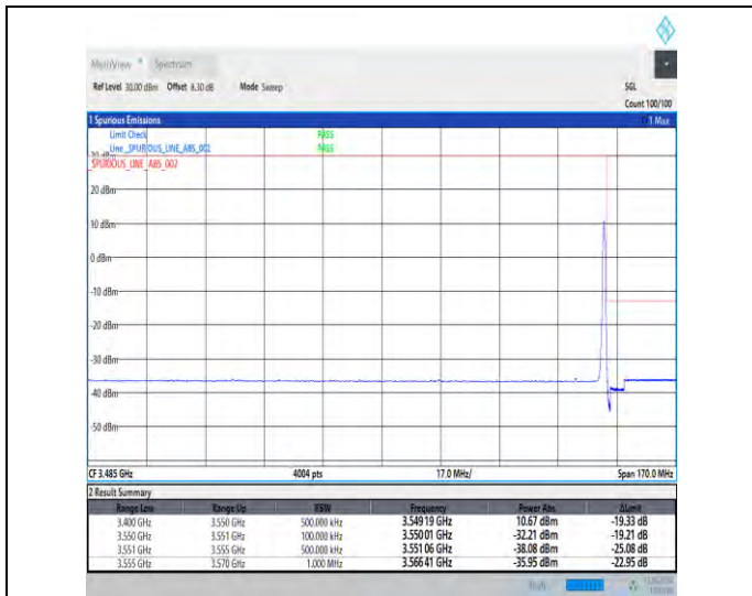
1-N78-3450-3550-30-10-H-2-DFT-PI2BPSK-Edge_1R_B_Right-1@23-Ant1-1--PASS-see graph
