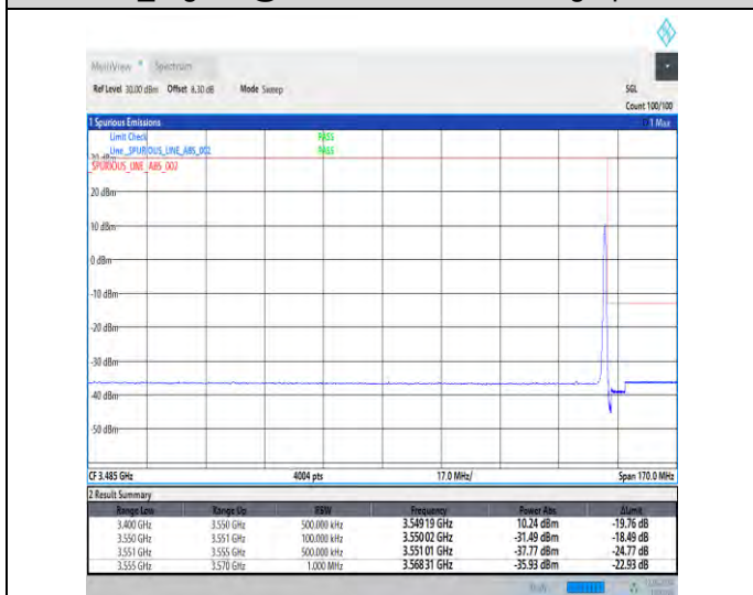
1-N78-3450-3550-30-10-H-5-CP-QPSK-Edge_1RB_Right-1@23-Ant1-1--PASS-see graph
