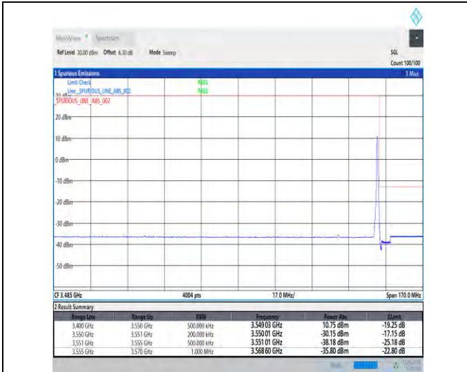
1-N78-3450-3550-30-20-H-2-DFT-PI2BPSK-Edge_1R_B_Right-1@50-Ant1-1--PASS-see graph
