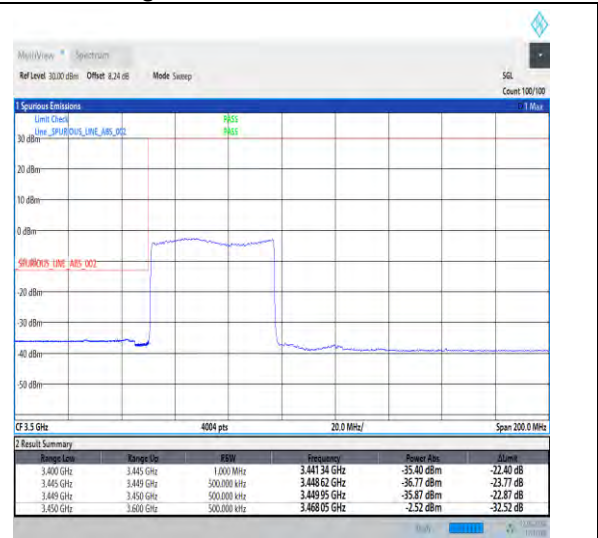
1-N78-3450-3550-30-50-L-3-DFT-PI2BPSK-Outer_Full-128@0-Ant1-1--PASS-see graph
