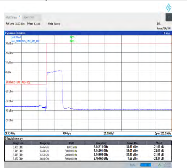
1-N78-3450-3550-30-20-L-3-DFT-PI2BPSK-Outer_Full-50@0-Ant1-1--PASS-see graph
