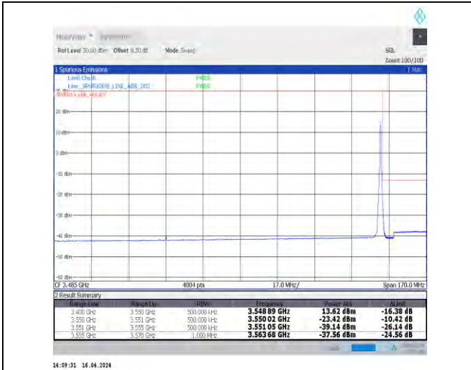
1-N78-3450-3550-30-100-H-2-DFT-PI2BPSK-Edge_1R_B_Right-1@272-Ant1-1--PASS-see graph
