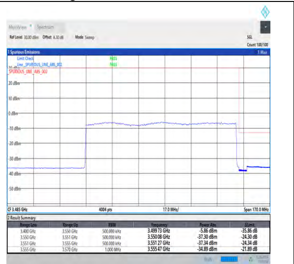
1-N78-3450-3550-30-100-H-3-DFT-PI2BPSK-Outer_Full-270@0-Ant1-1--PASS-see graph
