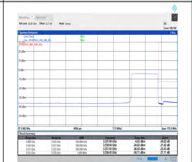
1-N78-3450-3550-30-30-H-6-CP-QPSK-Outer_Full-78@0-Ant1-1--PASS-see graph
