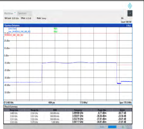
1-N78-3450-3550-30-100-H-6-CP-QPSK-Outer_Full-273@0-Ant1-1--PASS-see graph
