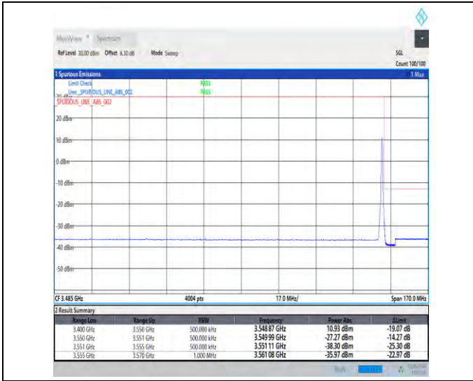
1-N78-3450-3550-30-90-H-2-DFT-PI2BPSK-Edge_1R_B_Right-1@244-Ant1-1--PASS-see graph
