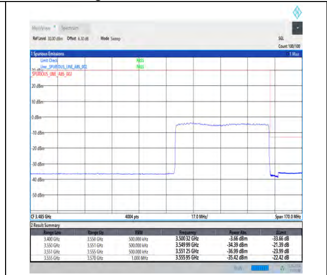
1-N78-3450-3550-30-60-H-3-DFT-PI2BPSK-Outer_Full-162@0-Ant1-1--PASS-see graph
