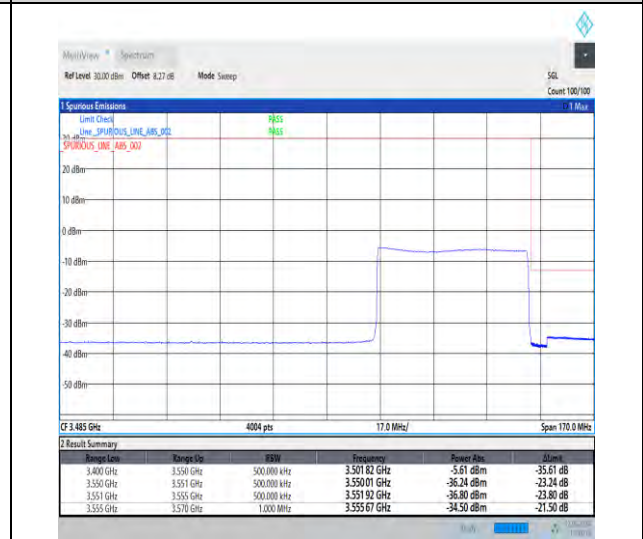
1-N78-3450-3550-30-50-H-6-CP-QPSK-Outer_Full-133@0-Ant1-1--PASS-see graph
