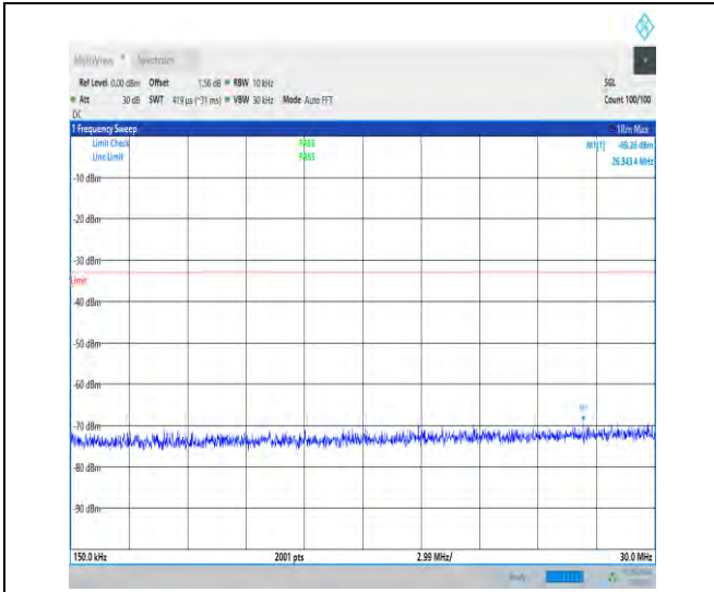
1-N78-3450-3550-30-100-M-1-DFT-QPSK-Edge_1R B_Left-1@0-0.15-30-Ant1-26.34--69.26--33-PASS
