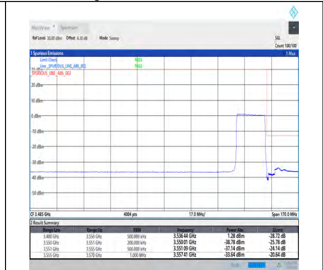
1-N78-3450-3550-30-20-H-3-DFT-PI2BPSK-Outer_Full-50@0-Ant1-1--PASS-see graph
