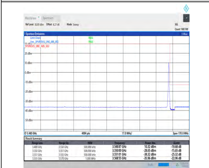
1-N78-3450-3550-30-30-H-5-CP-QPSK-Edge_1RB_Right-1@77-Ant1-1--PASS-see graph
