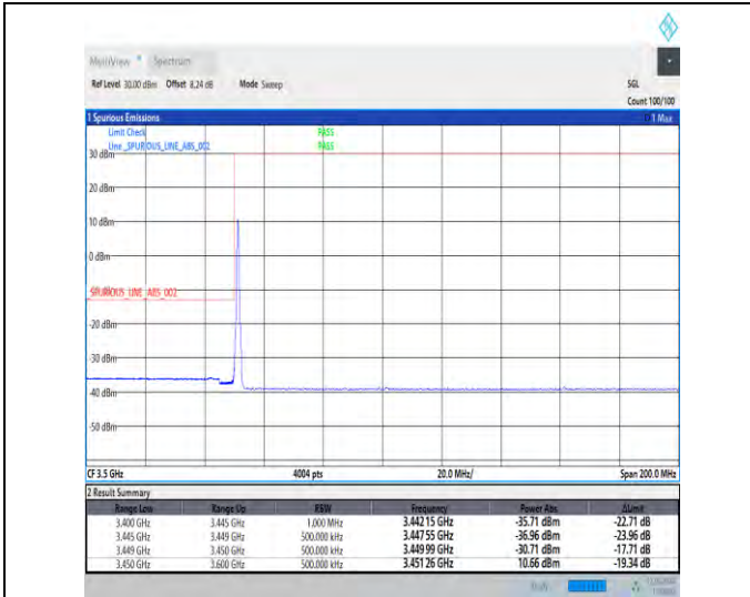
1-N78-3450-3550-30-50-L-1-DFT-PI2BPSK-Edge_1RB_Left-1@0-Ant1-1--PASS-see graph
