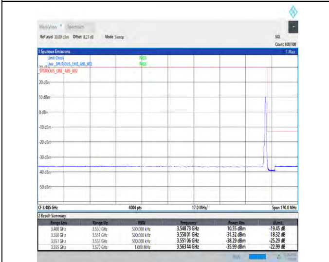
1-N78-3450-3550-30-50-H-5-CP-QPSK-Edge_1RB_Right-1@132-Ant1-1--PASS-see graph
