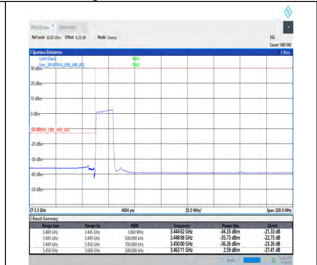
1-N78-3450-3550-30-15-L-3-DFT-PI2BPSK-Outer _Full-36@0-Ant1-1--PASS-see graph
