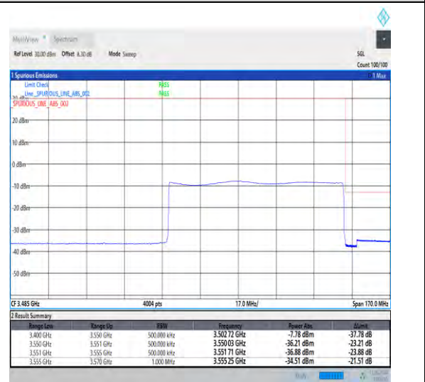
1-N78-3450-3550-30-80-H-6-CP-QPSK-Outer_Full-217@0-Ant1-1--PASS-see graph
