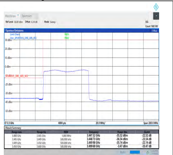
1-N78-3450-3550-30-60-L-3-DFT-PI2BPSK-Outer_Full-162@0-Ant1-1--PASS-see graph
