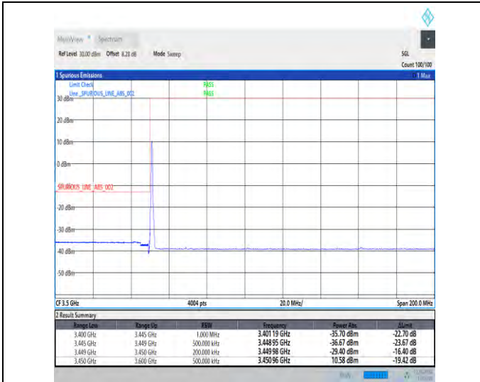
1-N78-3450-3550-30-20-L-1-DFT-PI2BPSK-Edge_1RB_Left-1@0-Ant1-1--PASS-see graph
