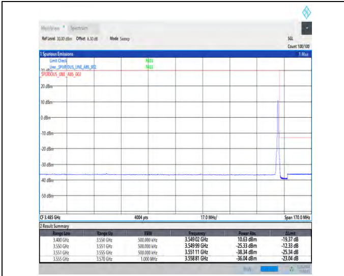
1-N78-3450-3550-30-60-H-2-DFT-PI2BPSK-Edge_1R_B_Right-1@161-Ant1-1--PASS-see graph
