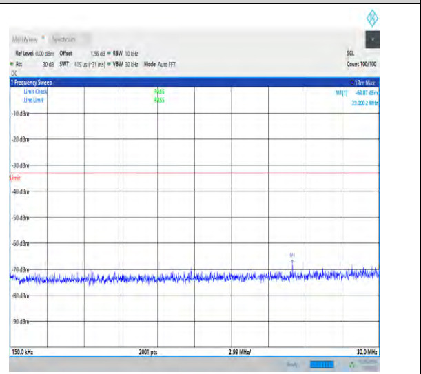
1-N78-3450-3550-30-100-H-1-DFT-QPSK-Edge_1R B_Left-1@0-0.15-30-Ant1-23.00--68.07--33-PASS
