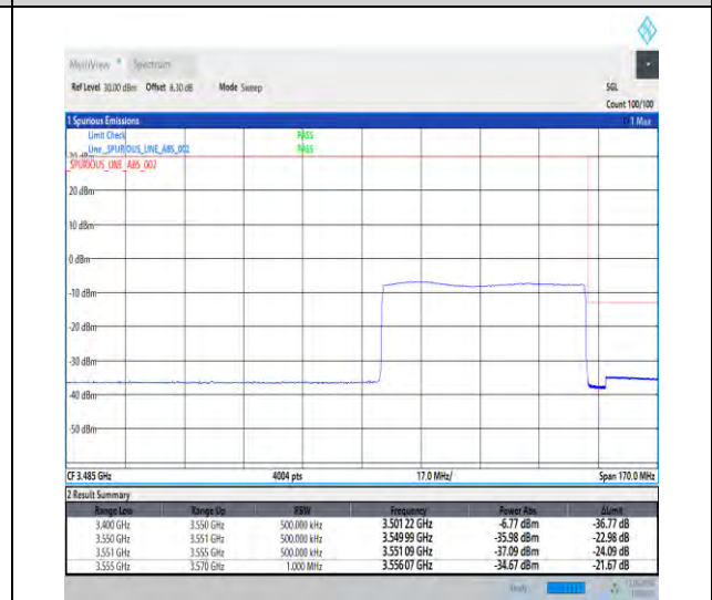
1-N78-3450-3550-30-60-H-6-CP-QPSK-Outer_Full-162@0-Ant1-1--PASS-see graph
