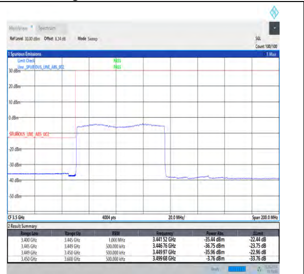
1-N78-3450-3550-30-70-L-3-DFT-PI2BPSK-Outer_Full-180@0-Ant1-1--PASS-see graph
