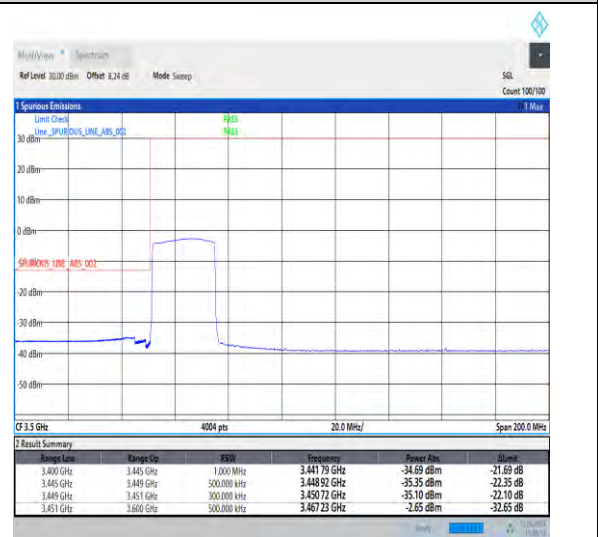
1-N78-3450-3550-30-25-L-6-CP-QPSK-Outer_Full -65@0-Ant1-1--PASS-see graph
