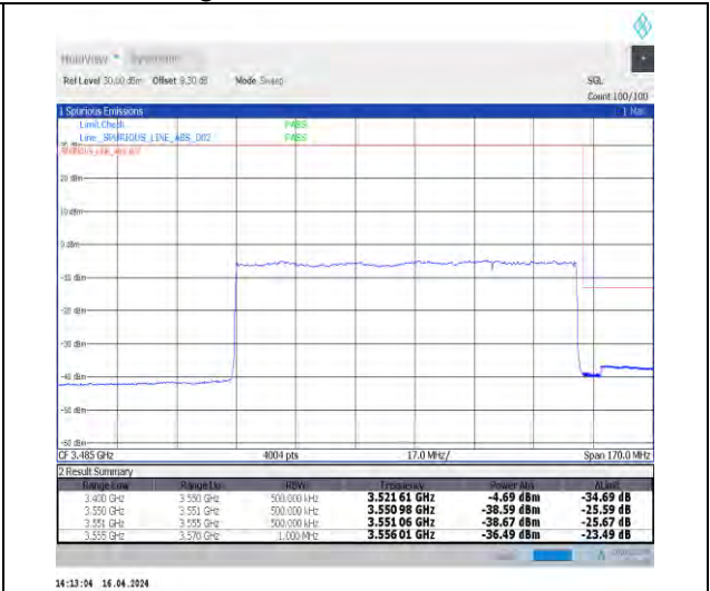
1-N78-3450-3550-30-100-H-3-DFT-PI2BPSK-Outer_Full-270@0-Ant1-1--PASS-see graph
