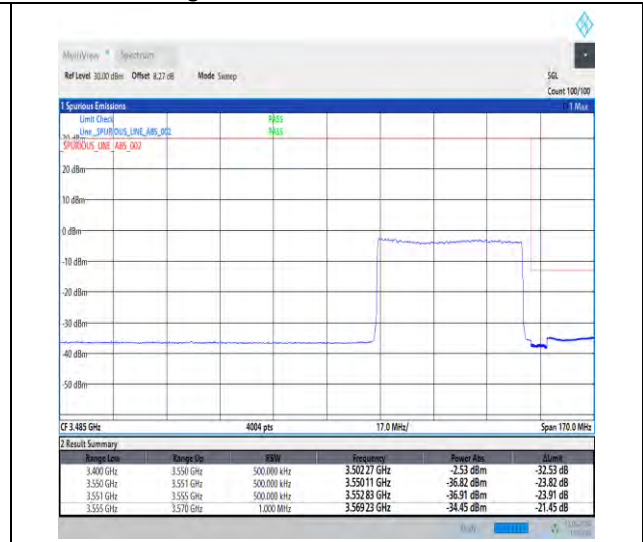
1-N78-3450-3550-30-50-H-3-DFT-PI2BPSK-Outer_Full-128@0-Ant1-1--PASS-see graph
