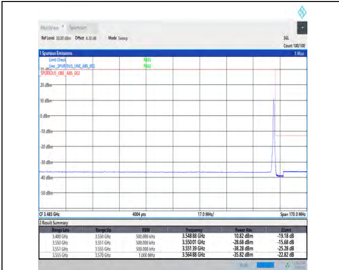
1-N78-3450-3550-30-80-H-2-DFT-PI2BPSK-Edge_1R_B_Right-1@216-Ant1-1--PASS-see graph
