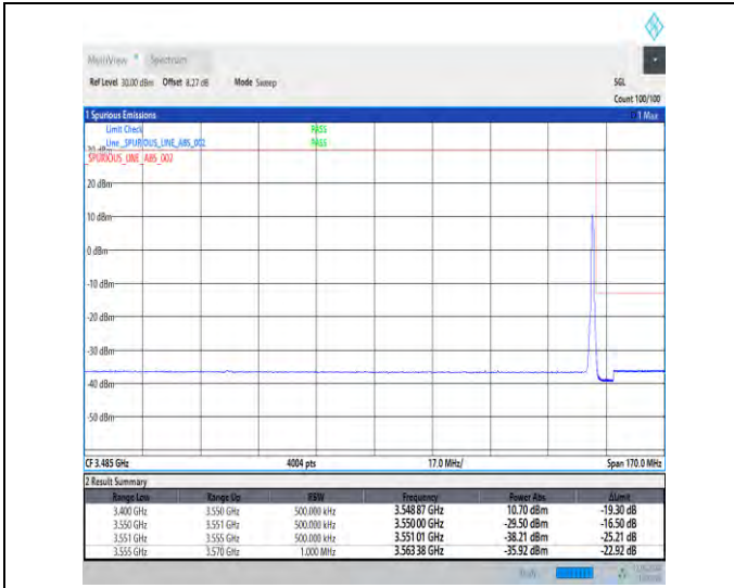
1-N78-3450-3550-30-30-H-2-DFT-PI2BPSK-Edge_1R_B_Right-1@77-Ant1-1--PASS-see graph
