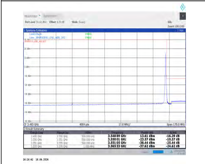
1-N78-3450-3550-30-100-H-5-CP-QPSK-Edge_1RB_Right-1@272-Ant1-1--PASS-see graph
