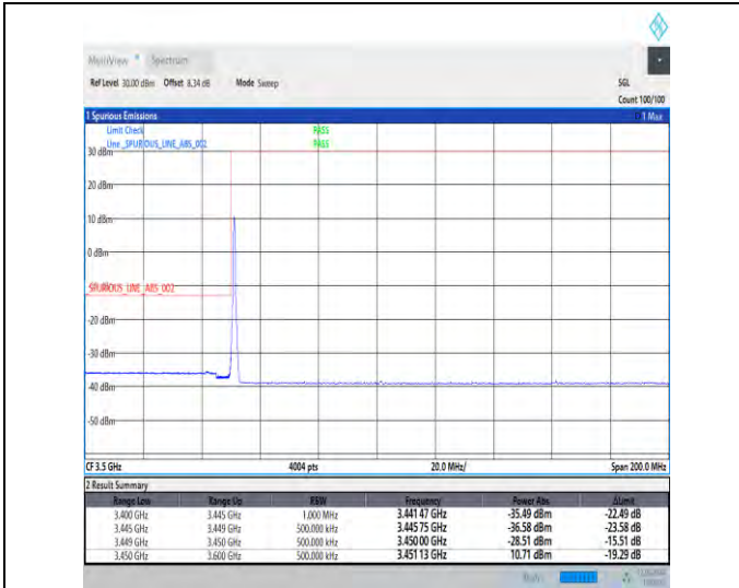
1-N78-3450-3550-30-70-L-1-DFT-PI2BPSK-Edge_1RB_Left-1@0-Ant1-1--PASS-see graph
