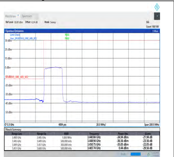
1-N78-3450-3550-30-25-L-3-DFT-PI2BPSK-Outer _Full-64@0-Ant1-1--PASS-see graph
