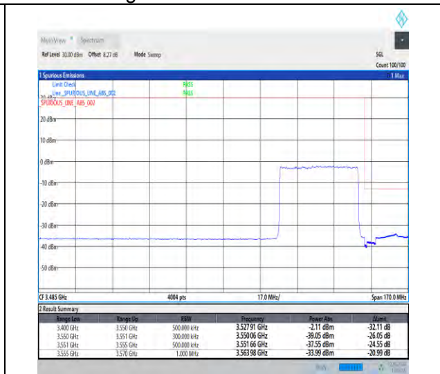
1-N78-3450-3550-30-40-H-3-DFT-PI2BPSK-Outer_Full-100@0-Ant1-1--PASS-see graph
