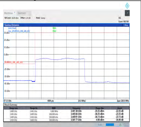
1-N78-3450-3550-30-80-L-3-DFT-PI2BPSK-Outer_Full-216@0-Ant1-1--PASS-see graph
