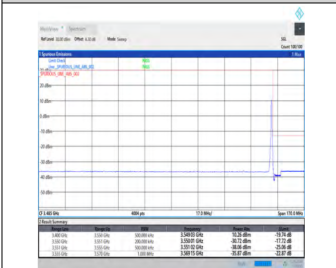
1-N78-3450-3550-30-20-H-5-CP-QPSK-Edge_1RB_Right-1@50-Ant1-1--PASS-see graph
