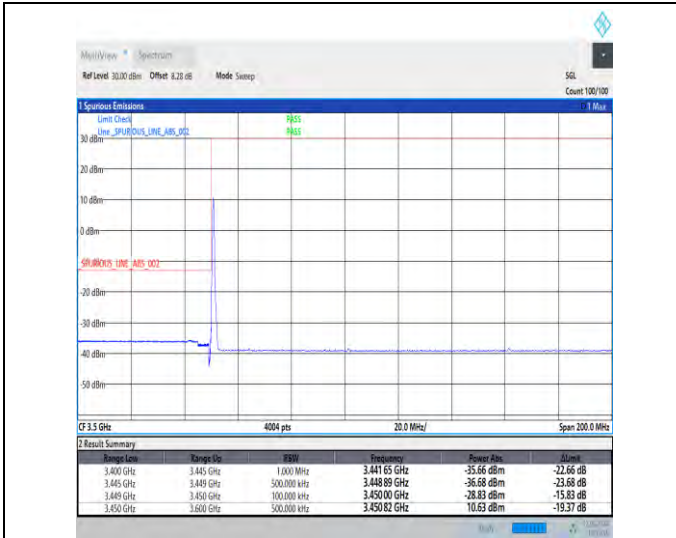
1-N78-3450-3550-30-15-L-1-DFT-PI2BPSK-Edge_1RB _Left-1@0-Ant1-1--PASS-see graph
