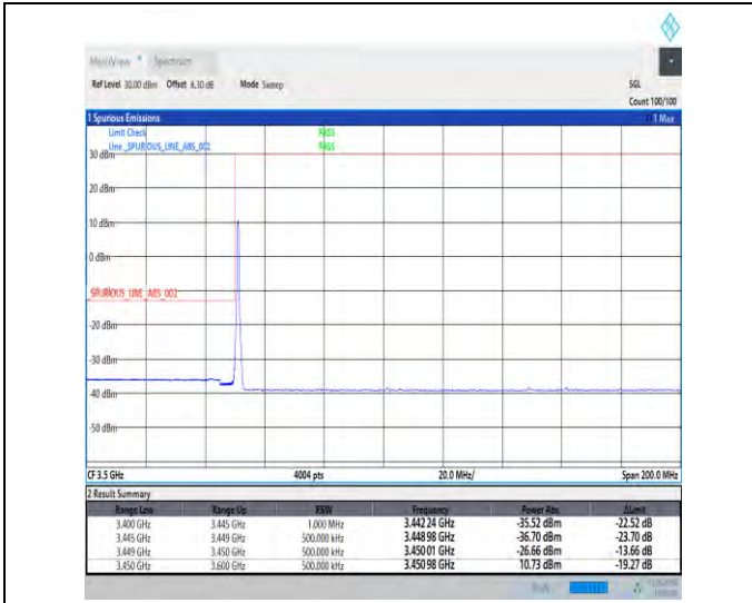
1-N78-3450-3550-30-100-L-1-DFT-PI2BPSK-Edge_1R_B_Left-1@0-Ant1-1--PASS-see graph
