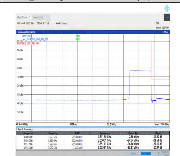
1-N78-3450-3550-30-25-H-6-CP-QPSK-Outer_Full-65@0-Ant1-1--PASS-see graph
