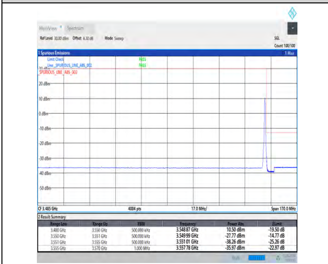
1-N78-3450-3550-30-90-H-5-CP-QPSK-Edge_1RB_Right-1@244-Ant1-1--PASS-see graph
