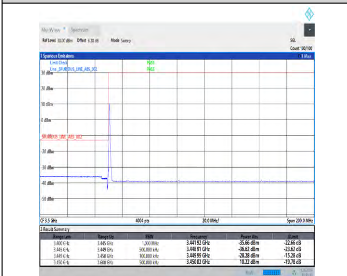
1-N78-3450-3550-30-15-L-4-CP-QPSK-Edge_1RB_Lef t-1@0-Ant1-1--PASS-see graph
