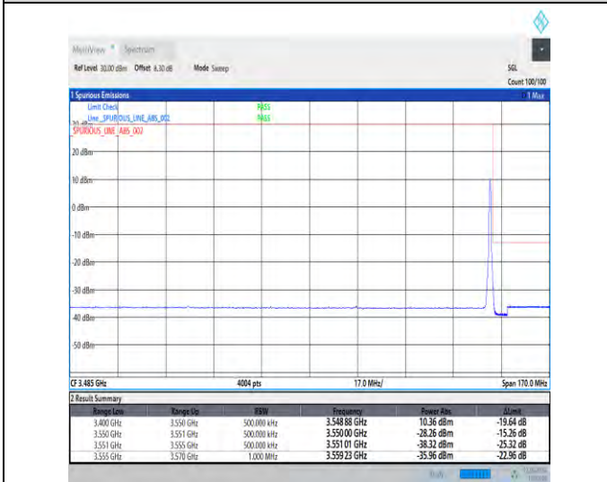
1-N78-3450-3550-30-80-H-5-CP-QPSK-Edge_1RB_Right-1@216-Ant1-1--PASS-see graph
