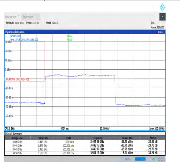
1-N78-3450-3550-30-90-L-3-DFT-PI2BPSK-Outer_Full-240@0-Ant1-1--PASS-see graph
