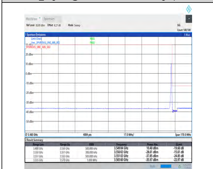
1-N78-3450-3550-30-25-H-5-CP-QPSK-Edge_1RB_Right-1@64-Ant1-1--PASS-see graph
