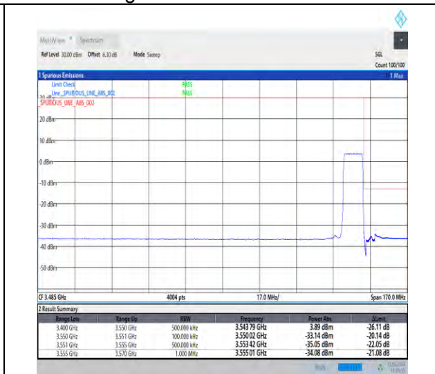
1-N78-3450-3550-30-10-H-3-DFT-PI2BPSK-Outer_Full-24@0-Ant1-1--PASS-see graph
