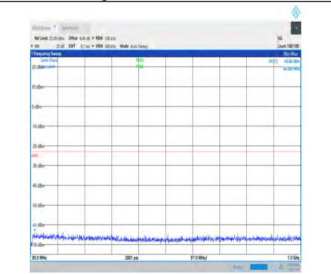
1-N78-3450-3550-30-100-M-1-DFT-QPSK-Edge_1R B_Left-1@0-30-1000-Ant1-44.55--63.66--23-PASS
