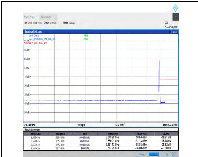
1-N78-3450-3550-30-40-H-2-DFT-PI2BPSK-Edge_1R_B_Right-1@105-Ant1-1--PASS-see graph
