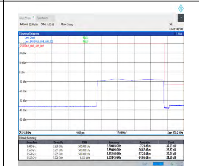
1-N78-3450-3550-30-70-H-6-CP-QPSK-Outer_Full-189@0-Ant1-1--PASS-see graph
