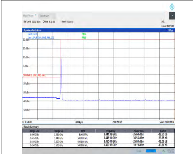
1-N78-3450-3550-30-100-L-4-CP-QPSK-Edge_1RB_Left-1@0-Ant1-1--PASS-see graph
