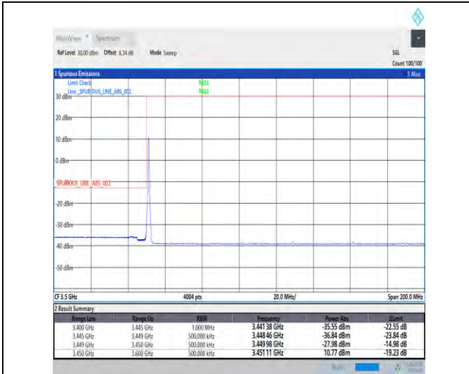
1-N78-3450-3550-30-80-L-1-DFT-PI2BPSK-Edge_1RB_Left-1@0-Ant1-1--PASS-see graph
