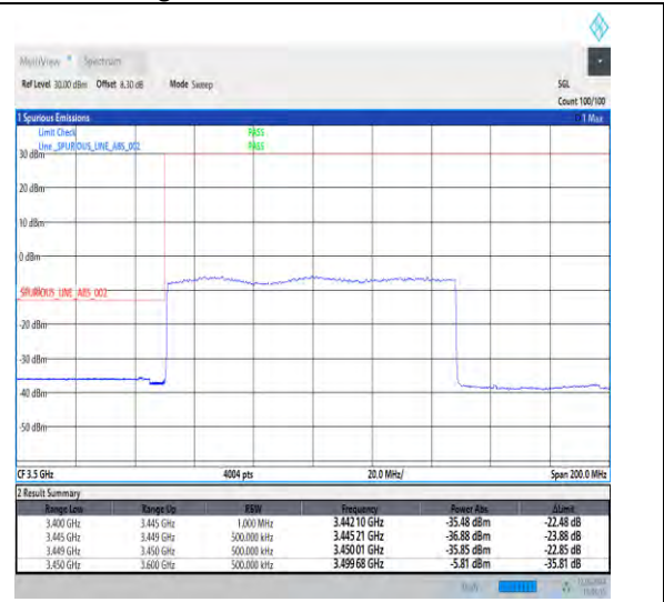
1-N78-3450-3550-30-100-L-3-DFT-PI2BPSK-Outer_Full-270@0-Ant1-1--PASS-see graph
