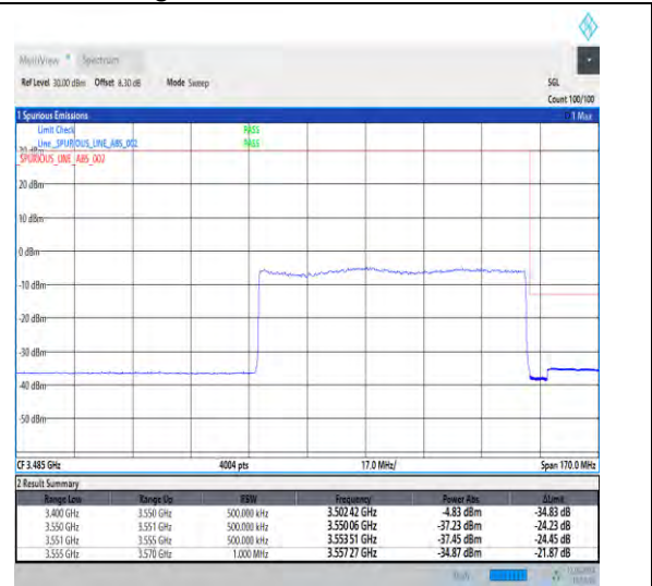
1-N78-3450-3550-30-80-H-3-DFT-PI2BPSK-Outer_Full-216@0-Ant1-1--PASS-see graph
