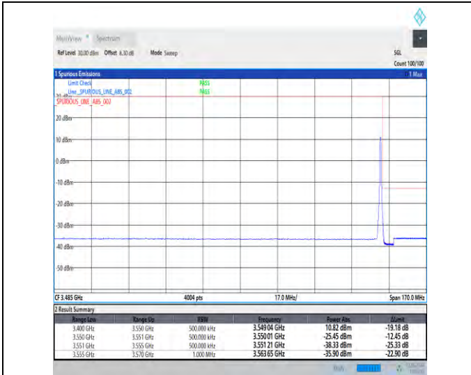
1-N78-3450-3550-30-100-H-2-DFT-PI2BPSK-Edge_1R_B_Right-1@272-Ant1-1--PASS-see graph
