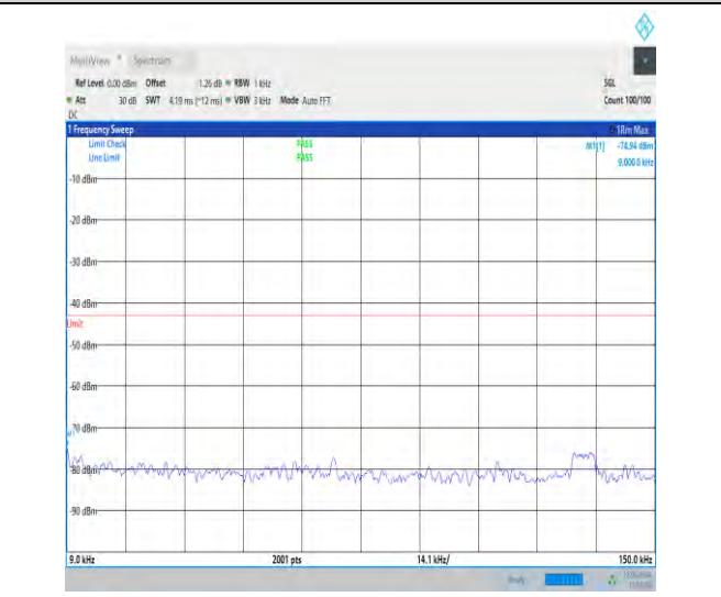
1-N78-3450-3550-30-100-M-1-DFT-QPSK-Edge_1R B_Left-1@0-0.009-0.15-Ant1-0.01--74.94--43-PASS
