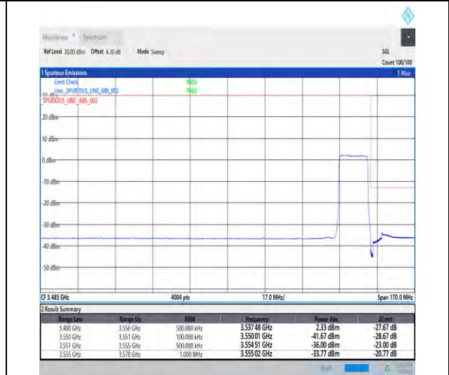
1-N78-3450-3550-30-15-H-3-DFT-PI2BPSK-Outer_Full-36@0-Ant1-1--PASS-see graph
