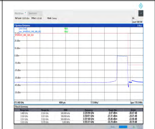
1-N78-3450-3550-30-15-H-6-CP-QPSK-Outer_Full-38@0-Ant1-1--PASS-see graph
