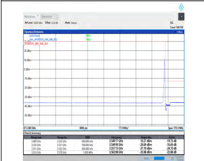
1-N78-3450-3550-30-15-H-5-CP-QPSK-Edge_1RB_Right-1@37-Ant1-1--PASS-see graph
