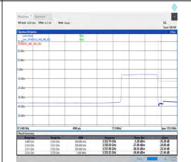
1-N78-3450-3550-30-40-H-6-CP-QPSK-Outer_Full-106@0-Ant1-1--PASS-see graph
