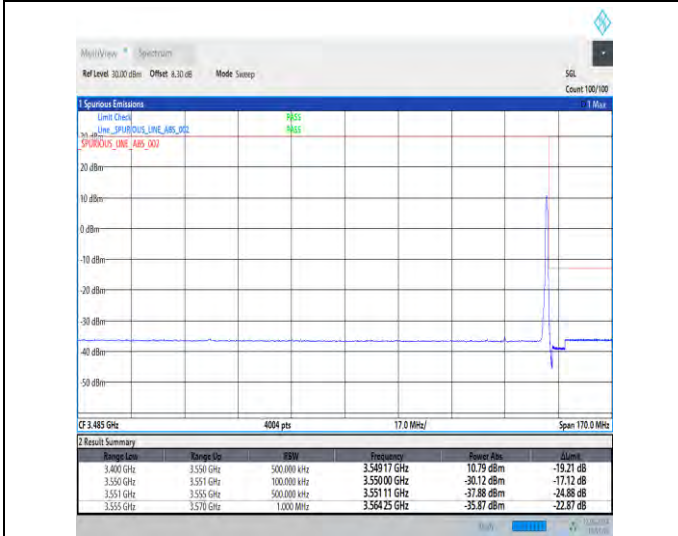
1-N78-3450-3550-30-15-H-2-DFT-PI2BPSK-Edge_1R_B_Right-1@37-Ant1-1--PASS-see graph
