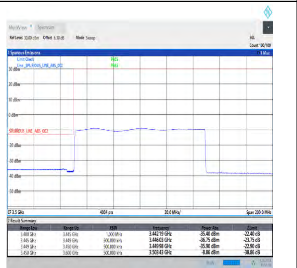
1-N78-3450-3550-30-100-L-6-CP-QPSK-Outer_Full-273@0-Ant1-1--PASS-see graph
