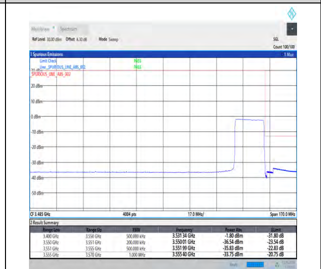
1-N78-3450-3550-30-20-H-6-CP-QPSK-Outer_Full-51@0-Ant1-1--PASS-see graph
