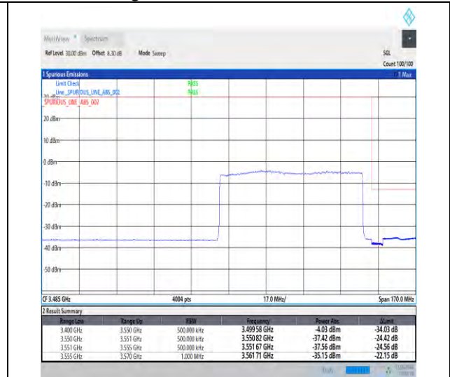
1-N78-3450-3550-30-70-H-3-DFT-PI2BPSK-Outer_Full-180@0-Ant1-1--PASS-see graph
