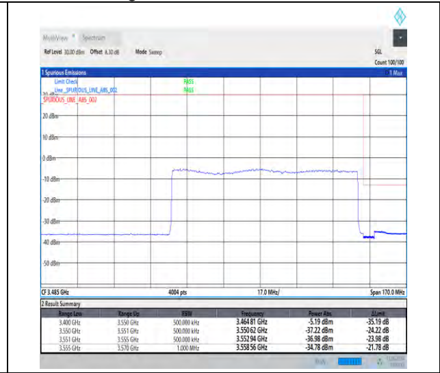
1-N78-3450-3550-30-90-H-3-DFT-PI2BPSK-Outer_Full-240@0-Ant1-1--PASS-see graph
