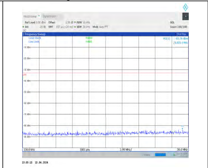
1-N78-3450-3550-30-100-H-1-DFT-PI2BPSK-Inner_1 RB_Left-1@1-0.15-30-Ant1-20.42--83.76--33-PASS
