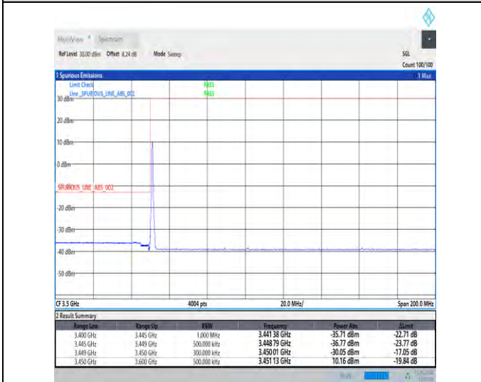
1-N78-3450-3550-30-40-L-4-CP-QPSK-Edge_1RB_Lef t-1@0-Ant1-1--PASS-see graph
