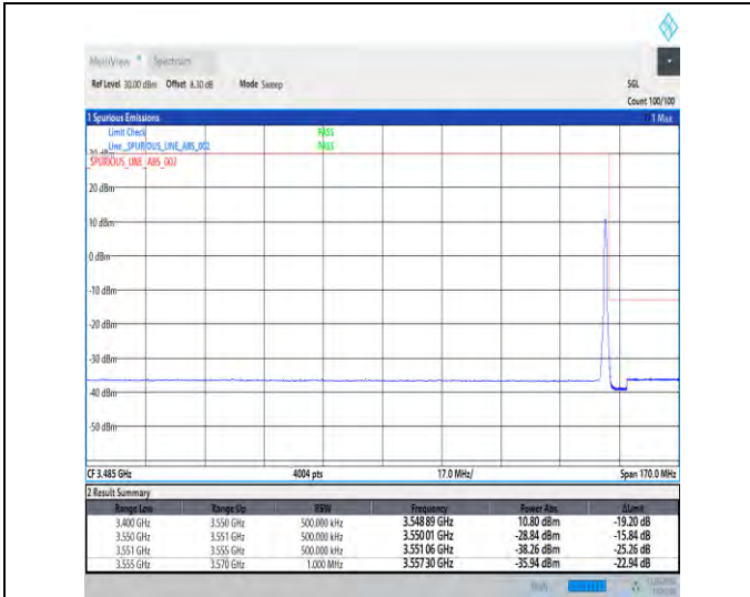
1-N78-3450-3550-30-70-H-2-DFT-PI2BPSK-Edge_1R_B_Right-1@188-Ant1-1--PASS-see graph
