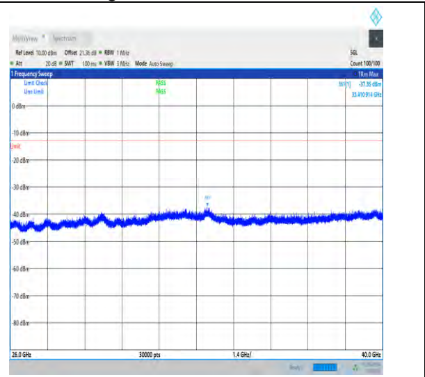
1-N78-3450-3550-30-100-M-1-DFT-QPSK-Edge_1R B_Left-1@0-26000-40000-Ant1-33410.91--37.35--13 -PASS
