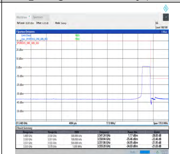
1-N78-3450-3550-30-10-H-6-CP-QPSK-Outer_Full-24@0-Ant1-1--PASS-see graph
