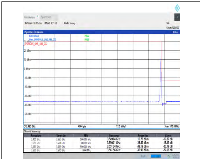
1-N78-3450-3550-30-25-H-2-DFT-PI2BPSK-Edge_1R_B_Right-1@64-Ant1-1--PASS-see graph
