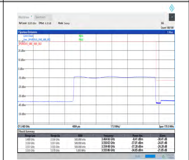
1-N78-3450-3550-30-90-H-6-CP-QPSK-Outer_Full-245@0-Ant1-1--PASS-see graph
