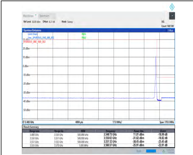
1-N78-3450-3550-30-50-H-2-DFT-PI2BPSK-Edge_1R_B_Right-1@132-Ant1-1--PASS-see graph
