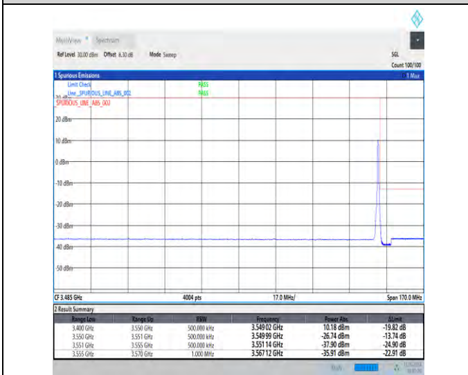
1-N78-3450-3550-30-60-H-5-CP-QPSK-Edge_1RB_Right-1@161-Ant1-1--PASS-see graph
