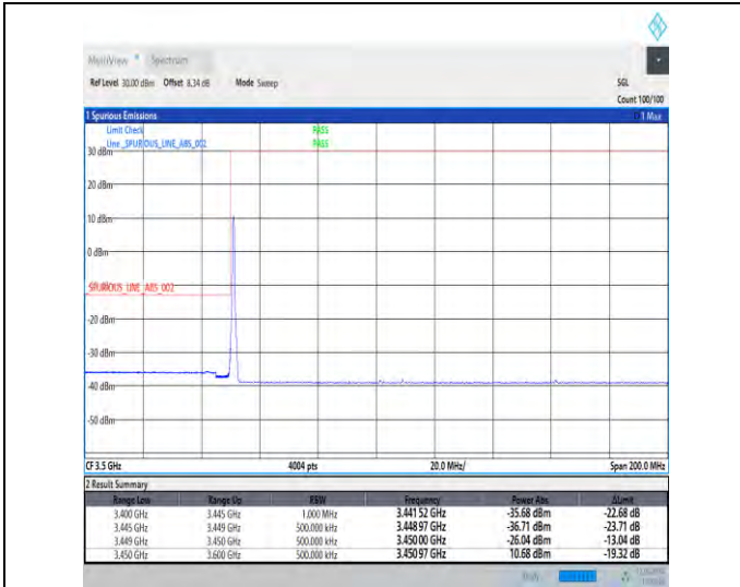
1-N78-3450-3550-30-60-L-1-DFT-PI2BPSK-Edge_1RB_Left-1@0-Ant1-1--PASS-see graph
