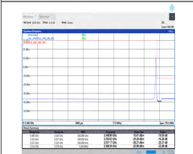
1-N78-3450-3550-30-70-H-5-CP-QPSK-Edge_1RB_Right-1@188-Ant1-1--PASS-see graph
