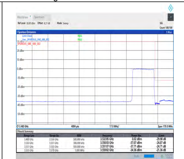
1-N78-3450-3550-30-25-H-3-DFT-PI2BPSK-Outer_Full-64@0-Ant1-1--PASS-see graph
