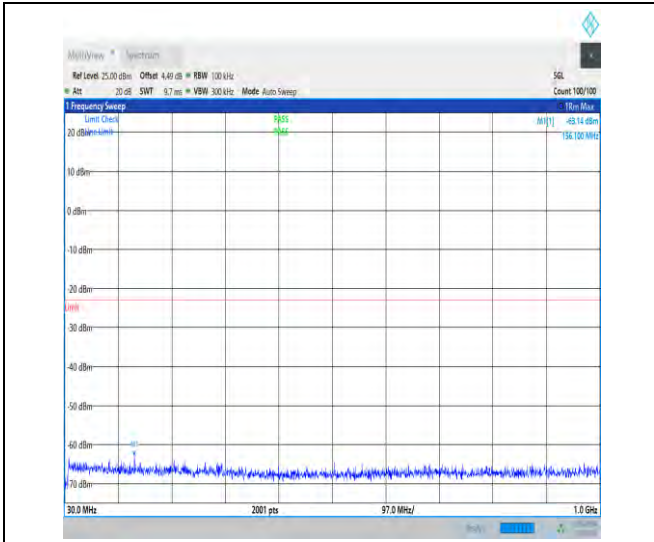
1-N78-3450-3550-30-100-H-1-DFT-QPSK-Edge_1R B_Left-1@0-30-1000-Ant1-156.10--63.14--23-PASS
