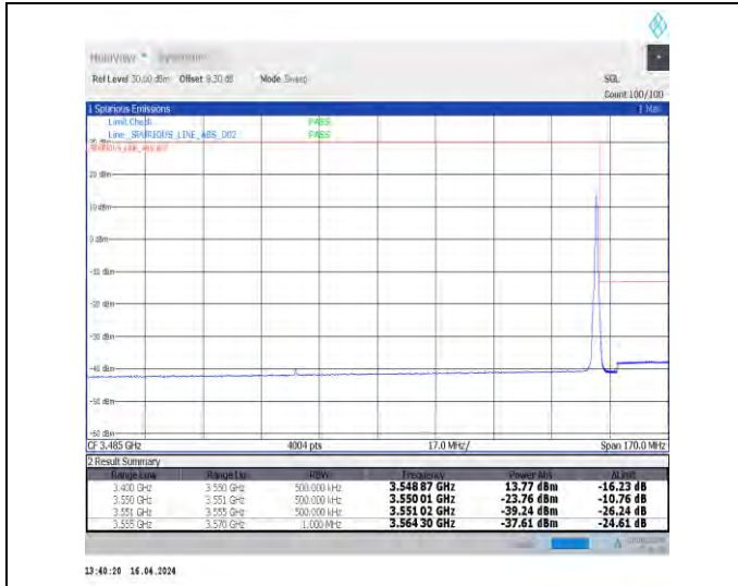
1-N78-3450-3550-30-90-H-2-DFT-PI2BPSK-Edge_1R_B_Right-1@244-Ant1-1--PASS-see graph
