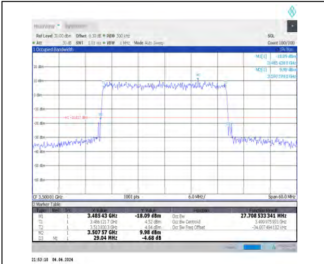
1-N78-3450-3550-30-30-M-9-CP-256QAM-Outer_Full I-78@0-Ant1-27.709-29.040-≤30-PASS
