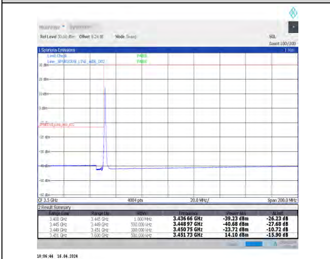
1-N78-3450-3550-30-25-L-4-CP-QPSK-Edge_1RB_Lef t-1@0-Ant1-1--PASS-see graph
