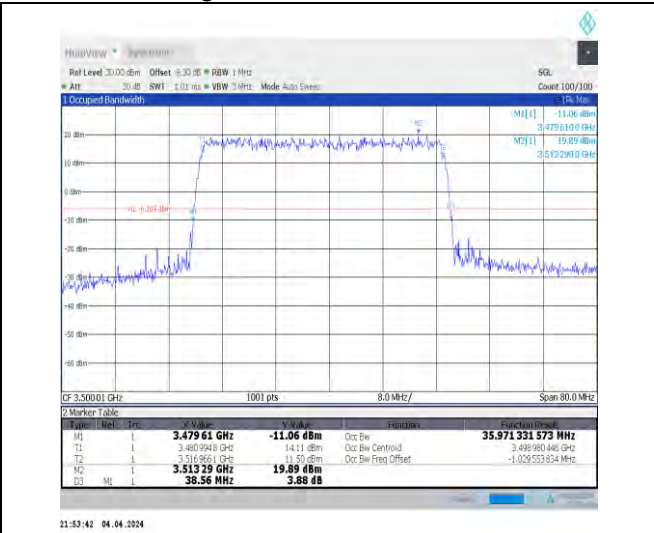
1-N78-3450-3550-30-40-M-1-DFT-QPSK-Outer_Full 100@0-Ant1-35.971-38.560-≤40-PASS
