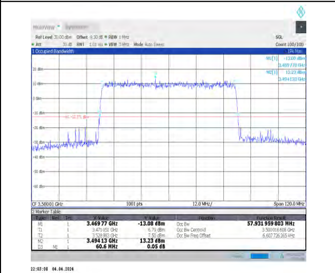
1-N78-3450-3550-30-60-M-9-CP-256QAM-Outer_Full-1 162@0-Ant1-57.932-60.600≤60-PASS
