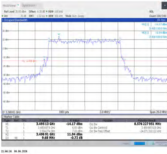
1-N78-3450-3550-30-10-M-5-DFT-256QAM-Outer_Full-24@0-Ant1-8.576-9.680-≤10-PASS
