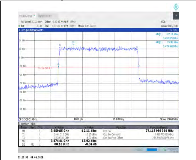
1-N78-3450-3550-30-80-M-5-DFT-256QAM-Outer_Full ull-216@0-Ant1-77.117-80.160-≤80-PASS
