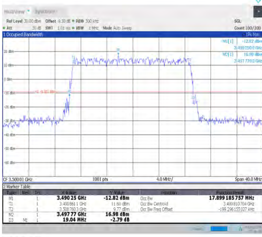
1-N78-3450-3550-30-20-M-3-DFT-16QAM-Outer_Full I-50@0-Ant1-17.899-19.040-≤20-PASS
