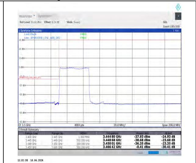
1-N78-3450-3550-30-40-L-3-DFT-PI2BPSK-Outer_Full-100@0-Ant1-1--PASS-see graph
