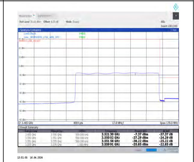
1-N78-3450-3550-30-90-H-6-CP-QPSK-Outer_Full-245@0-Ant1-1--PASS-see graph
