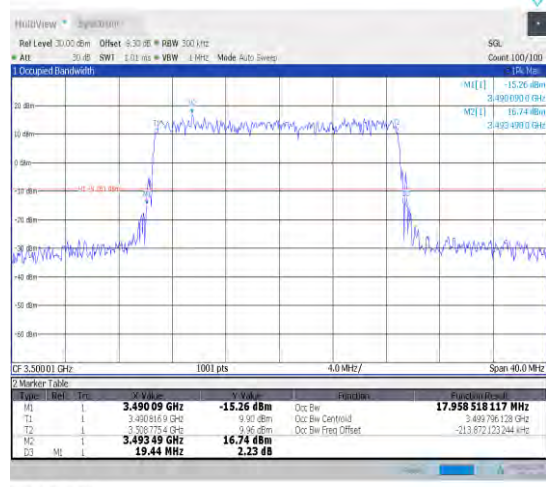
1-N78-3450-3550-30-20-M-4-DFT-64QAM-Outer_Full I-50@0-Ant1-17.959-19.440-≤20-PASS
