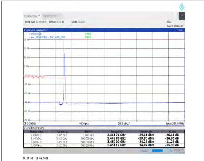
1-N78-3450-3550-30-30-L-1-DFT-PI2BPSK-Edge_1RB _Left-1@0-Ant1-1--PASS-see graph
