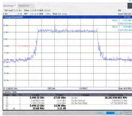
1-N78-3450-3550-30-20-M-6-CP-QPSK-Outer_Full-5 1@0-Ant1-18.263-19.680-≤20-PASS
