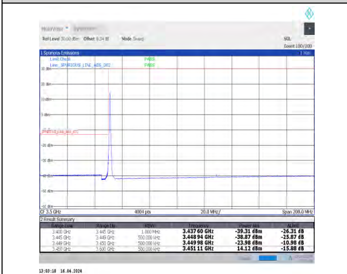
1-N78-3450-3550-30-80-L-4-CP-QPSK-Edge_1RB_Lef t-1@0-Ant1-1--PASS-see graph
