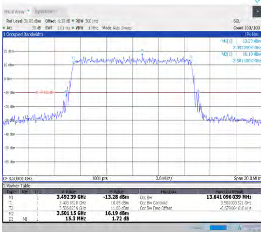
1-N78-3450-3550-30-15-M-6-CP-QPSK-Outer_Full-3 8@0-Ant1-13.641-15.300-≤15-PASS
