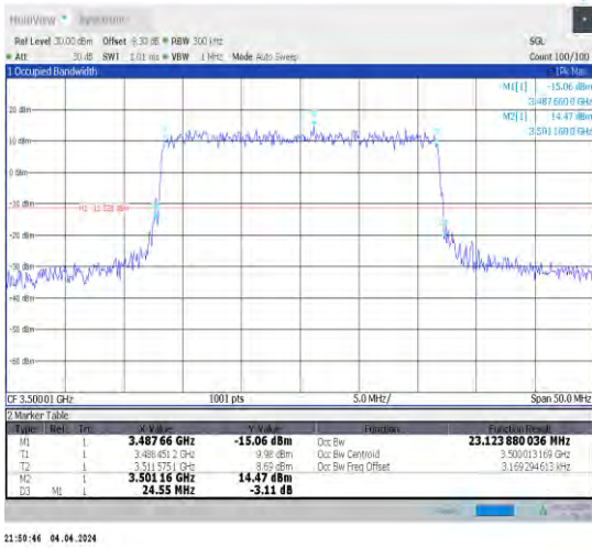
1-N78-3450-3550-30-25-M-6-CP-QPSK-Outer_Full-6 5@0-Ant1-23.124-24.550-≤25-PASS
