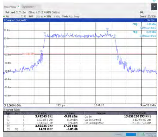
1-N78-3450-3550-30-15-M-7-CP-16QAM-Outer_Full -38@0-Ant1-13.659-14.910-≤15-PASS
