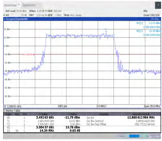
1-N78-3450-3550-30-15-M-5-DFT-256QAM-Outer_Full ull-36@0-Ant1-12.861-14.340-≤15-PASS
