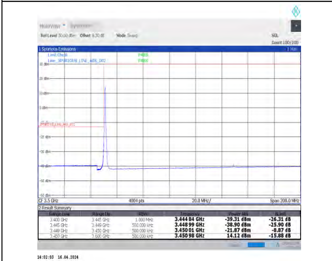
1-N78-3450-3550-30-100-L-4-CP-QPSK-Edge_1RB_Left-1@0-Ant1-1--PASS-see graph
