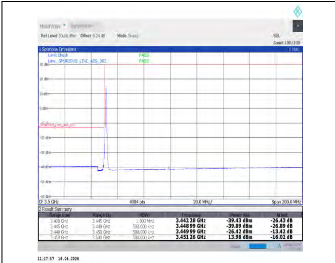
1-N78-3450-3550-30-50-L-1-DFT-PI2BPSK-Edge_1RB_Left-1@0-Ant1-1--PASS-see graph
