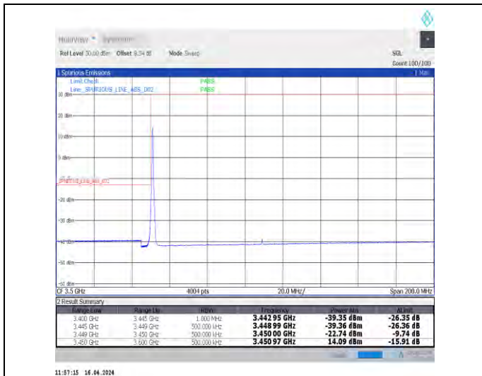
1-N78-3450-3550-30-60-L-1-DFT-PI2BPSK-Edge_1RB _Left-1@0-Ant1-1--PASS-see graph
