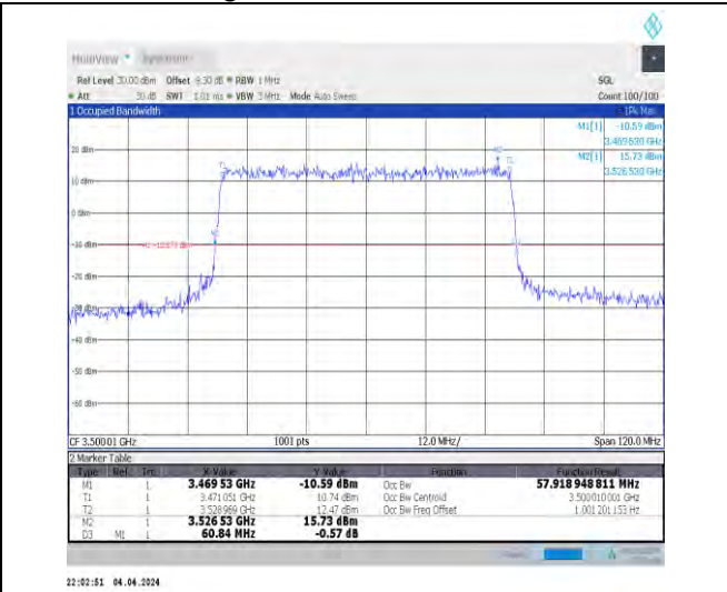
1-N78-3450-3550-30-60-M-7-CP-16QAM-Outer_Full -162@0-Ant1-57.919-60.840≤60-PASS
