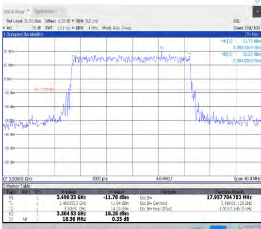
1-N78-3450-3550-30-20-M-1-DFT-QPSK-Outer_Full-50@0-Ant1-17.958-18.960-≤20-PASS
