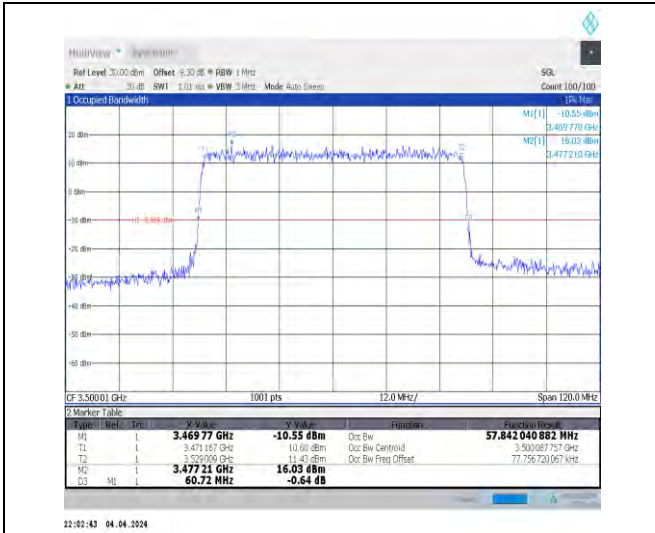
1-N78-3450-3550-30-60-M-6-CP-QPSK-Outer_Full-1 62@0-Ant1-57.842-60.720≤60-PASS
