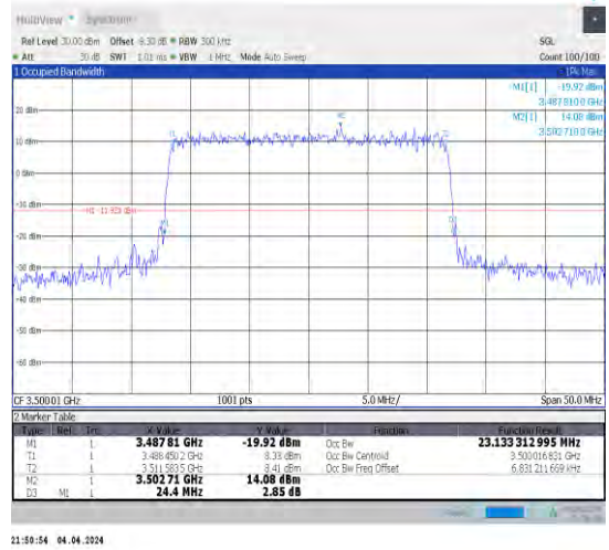
1-N78-3450-3550-30-25-M-7-CP-16QAM-Outer_Full-65@0-Ant1-23.133-24.400-≤25-PASS
