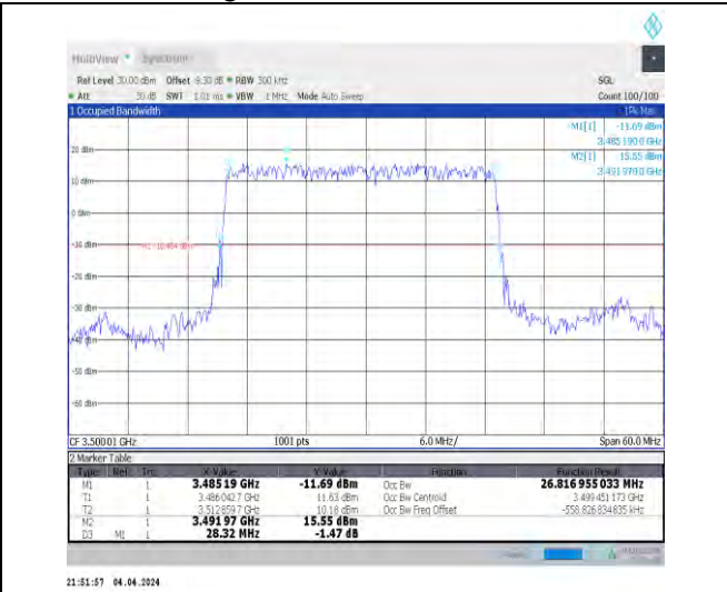
1-N78-3450-3550-30-30-M-2-DFT-PI2BPSK-Outer_Full-75@0-Ant1-26.822-28.320-≤30-PASS
