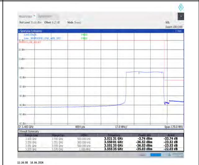
1-N78-3450-3550-30-40-H-6-CP-QPSK-Outer_Full-106@0-Ant1-1--PASS-see graph
