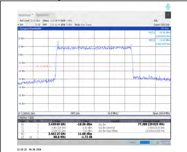
1-N78-3450-3550-30-80-M-9-CP-256QAM-Outer_Fu ll-217@0-Ant1-77.388-80.800-≤80-PASS
