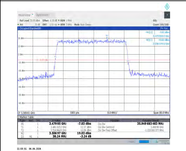
1-N78-3450-3550-30-40-M-3-DFT-16QAM-Outer_Full I-100@0-Ant1-35.95-38.240-≤40-PASS
