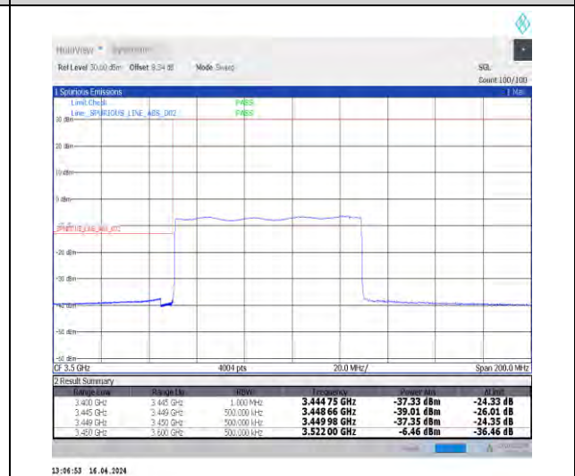
1-N78-3450-3550-30-80-L-6-CP-QPSK-Outer_Full -217@0-Ant1-1--PASS-see graph
