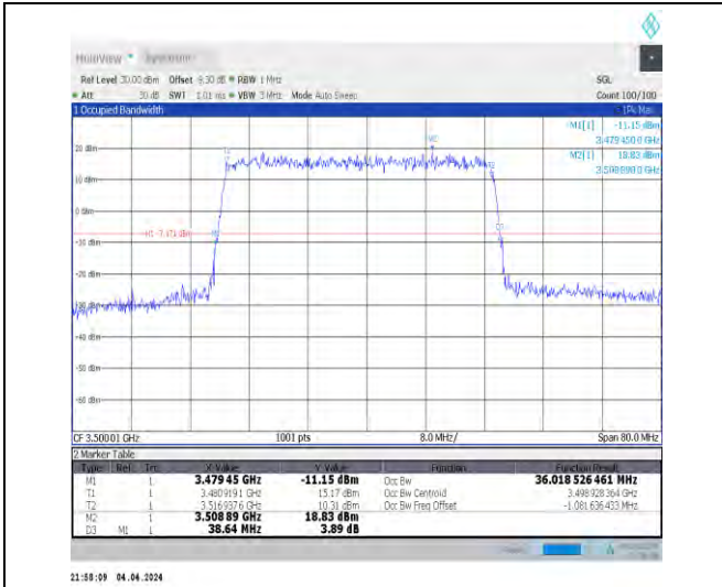
1-N78-3450-3550-30-40-M-4-DFT-64QAM-Outer_Full-100@0-Ant1-36.019-38.640-≤40-PASS
