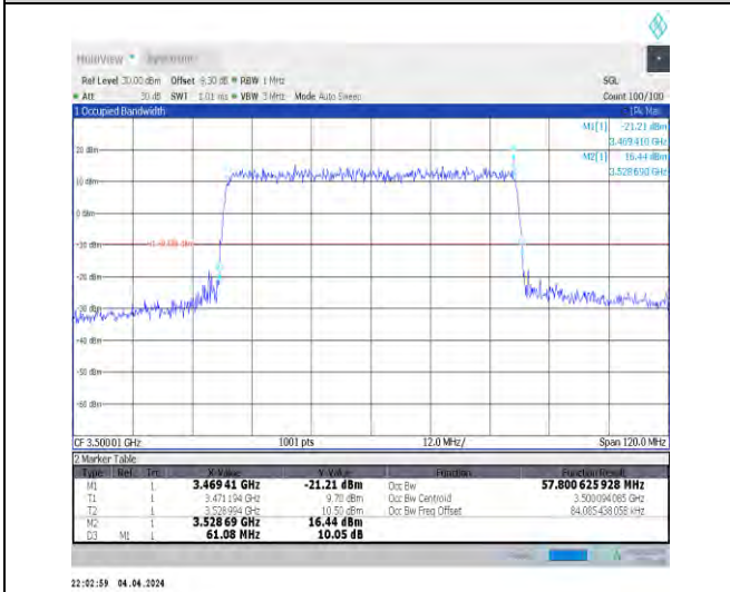
1-N78-3450-3550-30-60-M-8-CP-64QAM-Outer_Full-1 162@0-Ant1-57.801-61.080≤60-PASS
