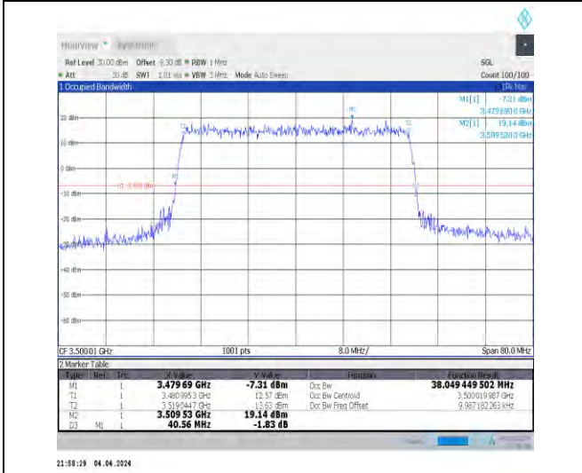
1-N78-3450-3550-30-40-M-6-CP-QPSK-Outer_Full-106@0-Ant1-38.049-40.560-≤40-PASS
