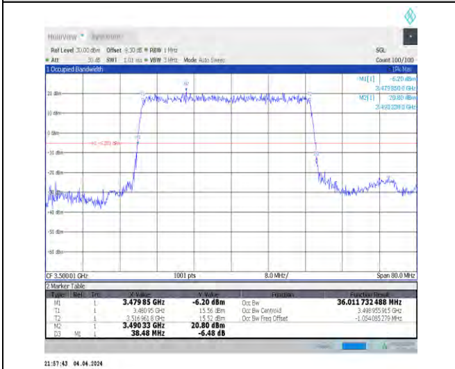
1-N78-3450-3550-30-40-M-2-DFT-PI2BPSK-Outer_Full ull-100@0-Ant1-36.012-38.480-≤40-PASS
