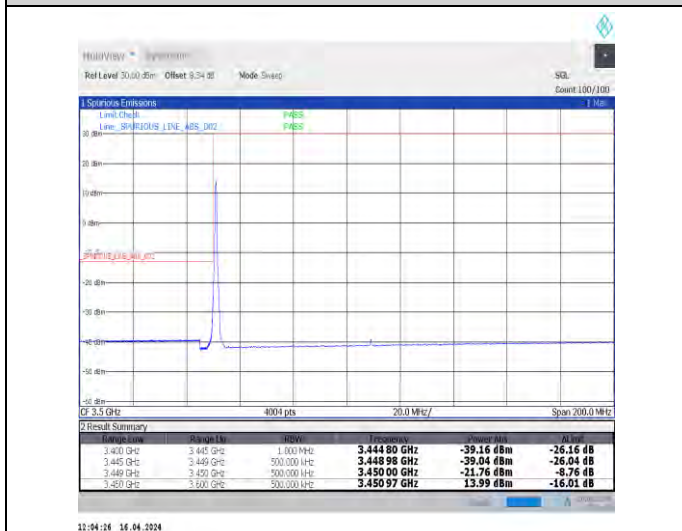
1-N78-3450-3550-30-60-L-4-CP-QPSK-Edge_1RB_Lef t-1@0-Ant1-1--PASS-see graph
