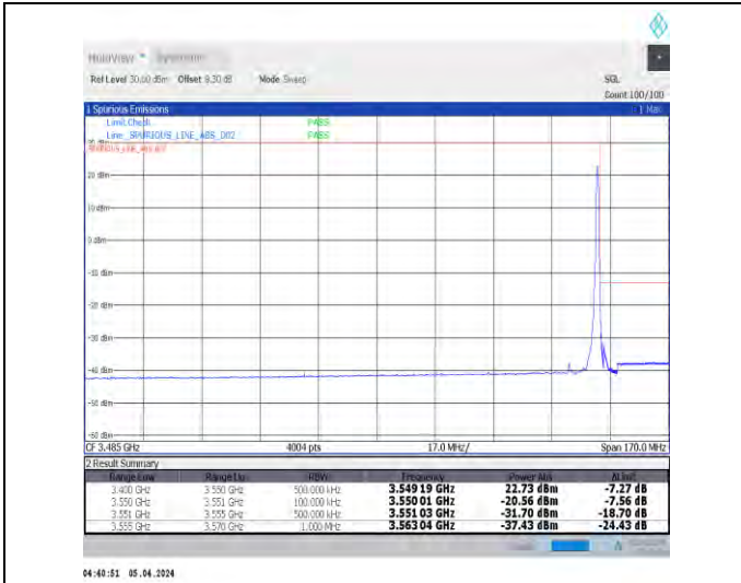
1-N78-3450-3550-30-10-H-2-DFT-PI2BPSK-Edge_1R_B_Right-1@23-Ant1-1--PASS-see graph
