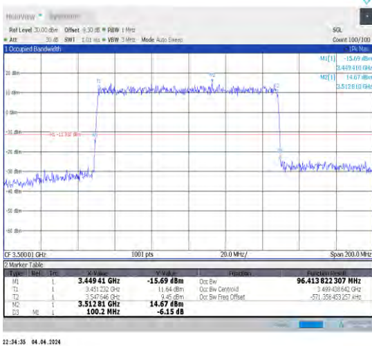
1-N78-3450-3550-30-100-M-4-DFT-64QAM-Outer_Full-270@0-Ant1-96.414-100.200-≤100-PASS
