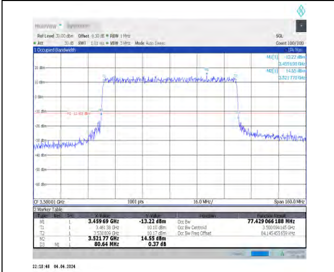
1-N78-3450-3550-30-80-M-6-CP-QPSK-Outer_Full-2 17@0-Ant1-77.429-80.640-≤80-PASS
