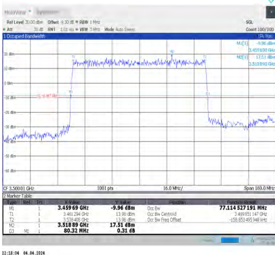
1-N78-3450-3550-30-80-M-2-DFT-PI2BPSK-Outer_Full-216@0-Ant1-77.115-80.320-≤80-PASS
