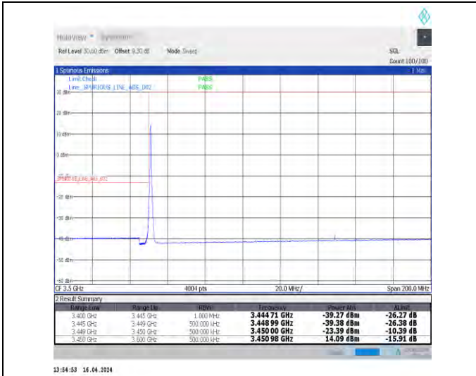
1-N78-3450-3550-30-100-L-1-DFT-PI2BPSK-Edge_1R_B_Left-1@0-Ant1-1--PASS-see graph
