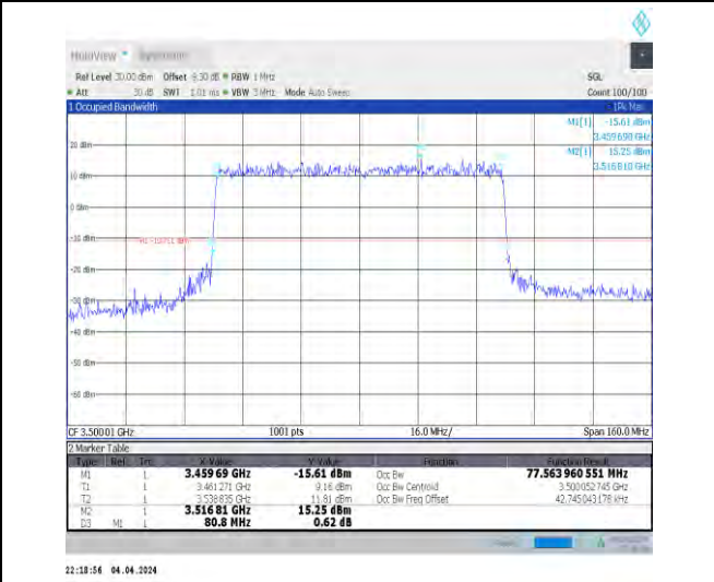
1-N78-3450-3550-30-80-M-7-CP-16QAM-Outer_Full -217@0-Ant1-77.564-80.800-≤80-PASS
