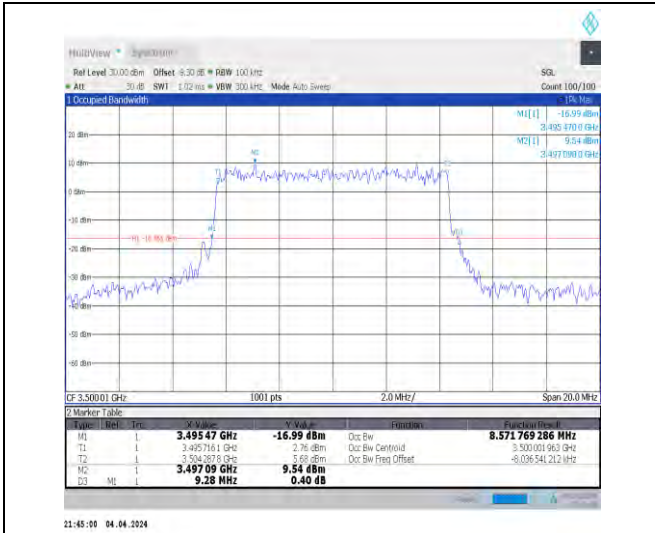
1-N78-3450-3550-30-10-M-9-CP-256QAM-Outer_Full-I-24@0-Ant1-8.572-9.280-≤10-PASS
