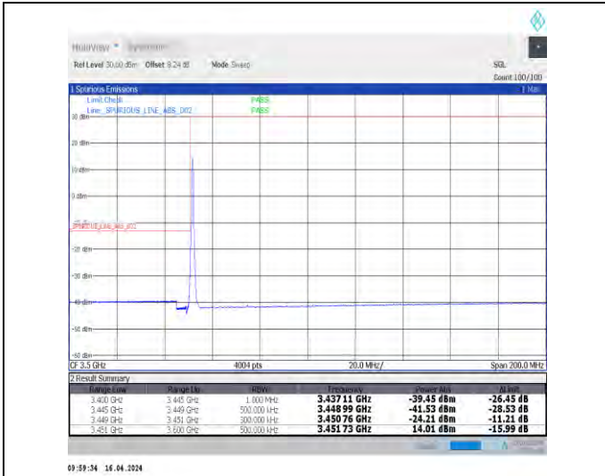
1-N78-3450-3550-30-25-L-1-DFT-PI2BPSK-Edge_1RB _Left-1@0-Ant1-1--PASS-see graph
