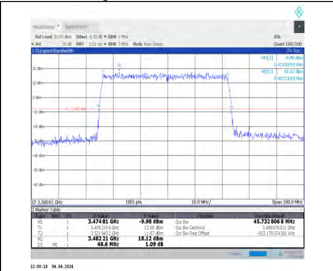
1-N78-3450-3550-30-50-M-4-DFT-64QAM-Outer_Full-128@0-Ant1-45.733-48.600-≤50-PASS
