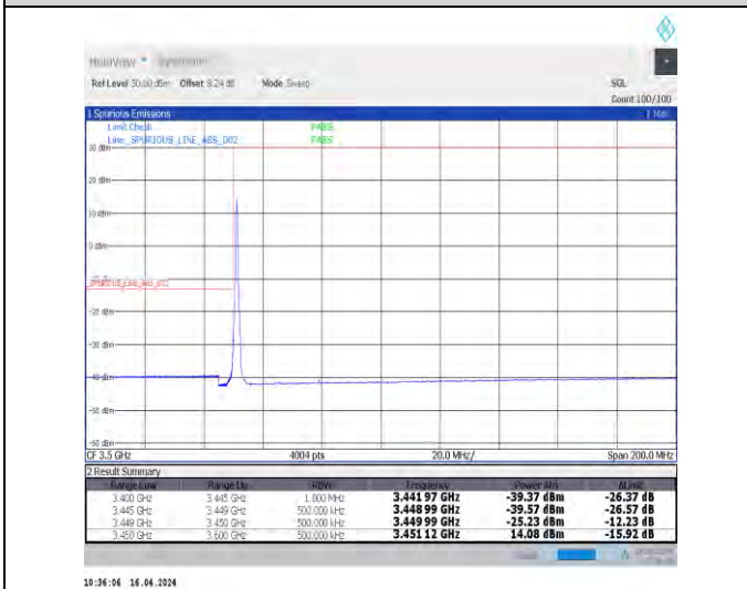
1-N78-3450-3550-30-30-L-4-CP-QPSK-Edge_1RB_Lef t-1@0-Ant1-1--PASS-see graph
