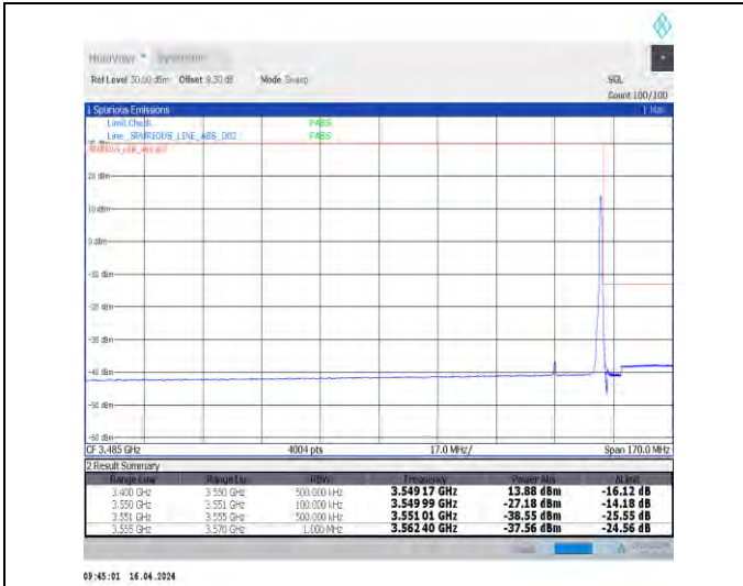
1-N78-3450-3550-30-15-H-2-DFT-PI2BPSK-Edge_1R_B_Right-1@37-Ant1-1--PASS-see graph
