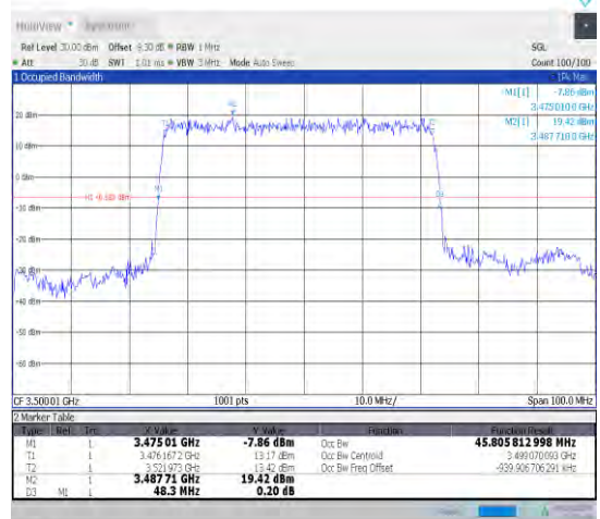
1-N78-3450-3550-30-50-M-2-DFT-PI2BPSK-Outer_Full-128@0-Ant1-45.806-48.300-≤50-PASS
