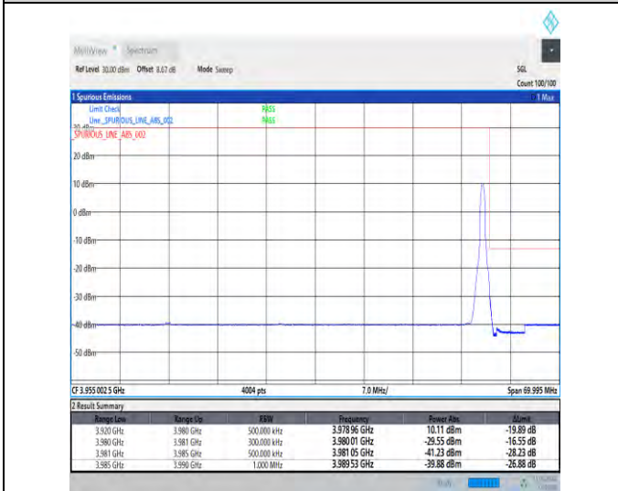
1-N77-3700-3980-30-60-H-5-CP-QPSK-Edge_1RB_Right-1@161-Ant1-1--PASS-see graph
