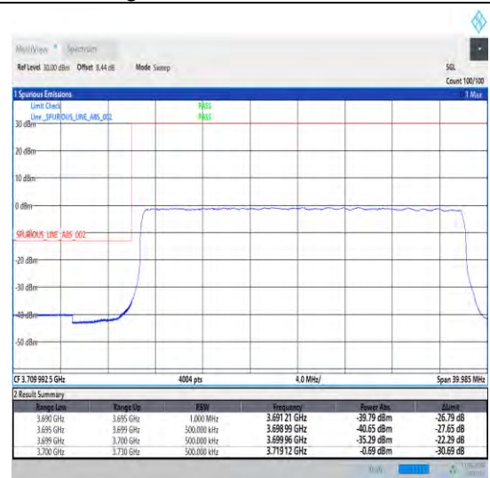
1-N77-3700-3980-30-30-L-3-DFT-PI2BPSK-Outer _Full-75@0-Ant1-1--PASS-see graph
