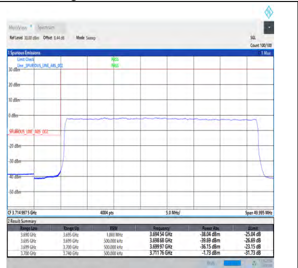
1-N77-3700-3980-30-40-L-3-DFT-PI2BPSK-Outer_Full-100@0-Ant1-1--PASS-see graph
