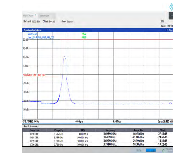
1-N77-3700-3980-30-30-L-1-DFT-PI2BPSK-Edge_1RB _Left-1@0-Ant1-1--PASS-see graph
