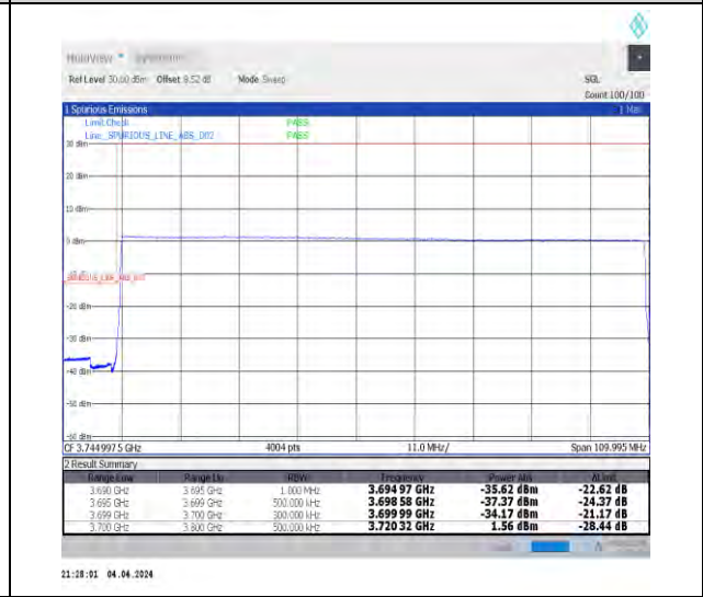
1-N77-3700-3980-30-100-L-6-CP-QPSK-Outer_Full-273@0-Ant1-1--PASS-see graph
