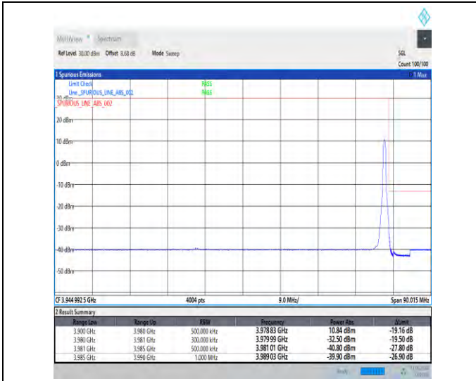
1-N77-3700-3980-30-80-H-2-DFT-PI2BPSK-Edge_1R_B_Right-1@216-Ant1-1--PASS-see graph
