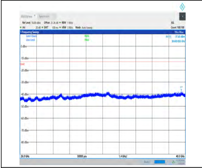
1-N77-3700-3980-30-100-L-1-DFT-QPSK-Edge_1R B_Left-1@0-26000-40000-Ant1-39663.06--37.43--13 -PASS
