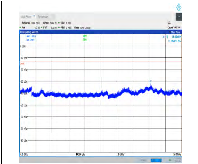
1-N77-3700-3980-30-100-M-1-DFT-QPSK-Edge_1R B_Left-1@0-6000-26000-Ant1-22156.28--33.05--13- PASS
