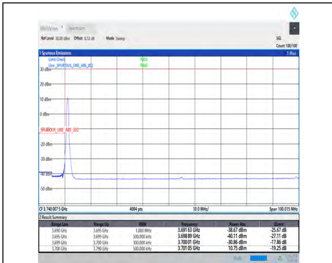
1-N77-3700-3980-30-90-L-1-DFT-PI2BPSK-Edge_1RB_Left-1@0-Ant1-1--PASS-see graph
