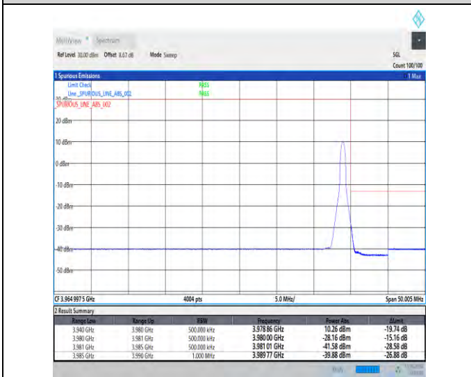
1-N77-3700-3980-30-40-H-5-CP-QPSK-Edge_1RB_Right-1@105-Ant1-1--PASS-see graph
