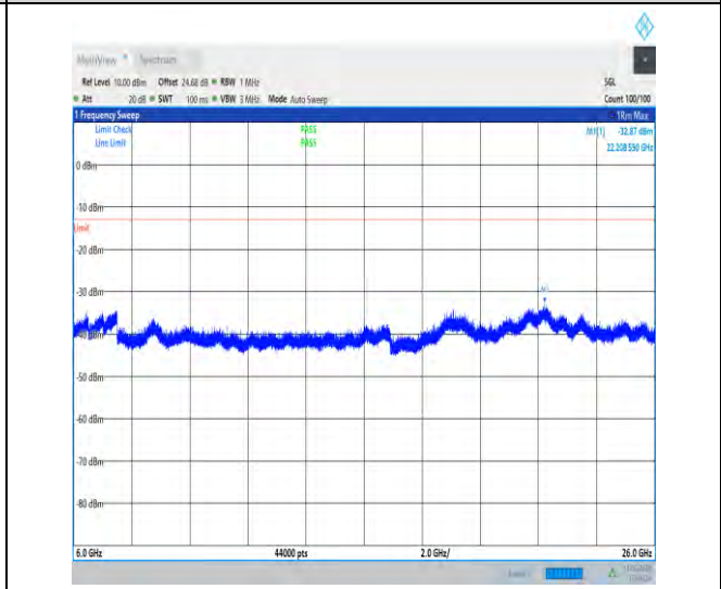
1-N77-3700-3980-30-100-H-1-DFT-QPSK-Edge_1R B_Left-1@0-6000-26000-Ant1-22208.55--32.87--13- PASS
