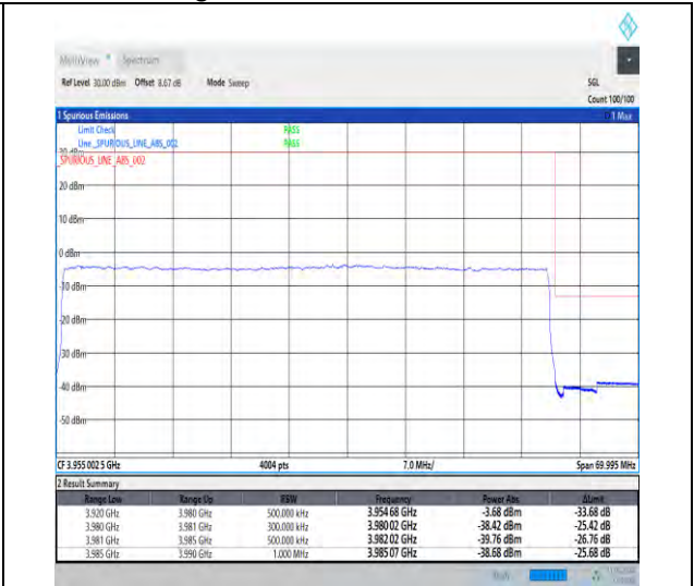
1-N77-3700-3980-30-60-H-3-DFT-PI2BPSK-Outer_Full-162@0-Ant1-1--PASS-see graph
