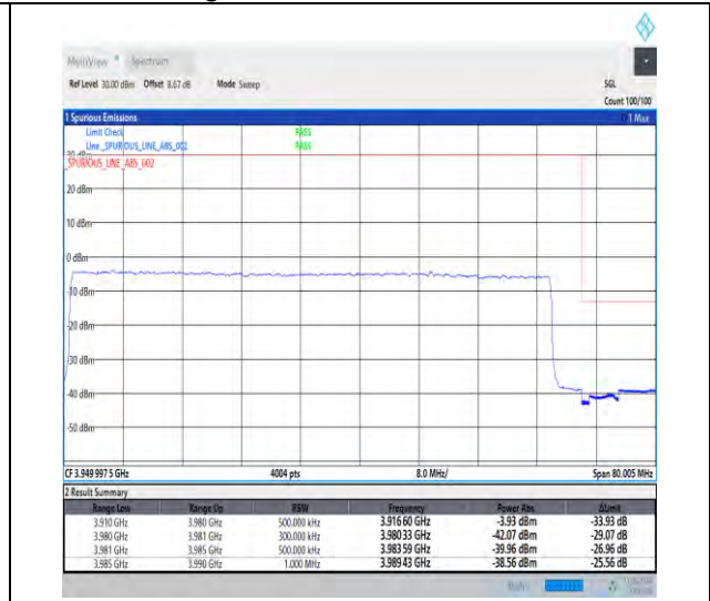
1-N77-3700-3980-30-70-H-3-DFT-PI2BPSK-Outer_Full-180@0-Ant1-1--PASS-see graph
