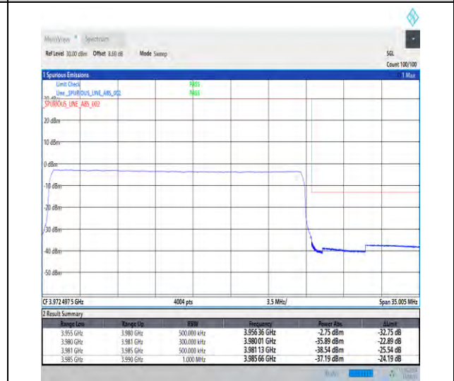
1-N77-3700-3980-30-25-H-6-CP-QPSK-Outer_Full-65@0-Ant1-1--PASS-see graph
