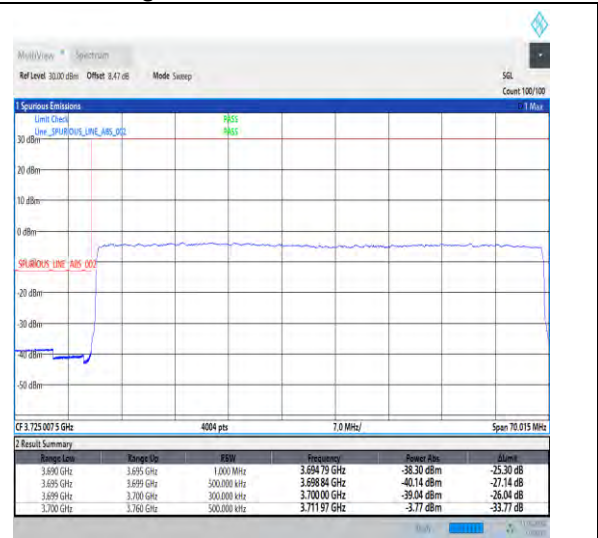
1-N77-3700-3980-30-60-L-3-DFT-PI2BPSK-Outer_Full-162@0-Ant1-1--PASS-see graph
