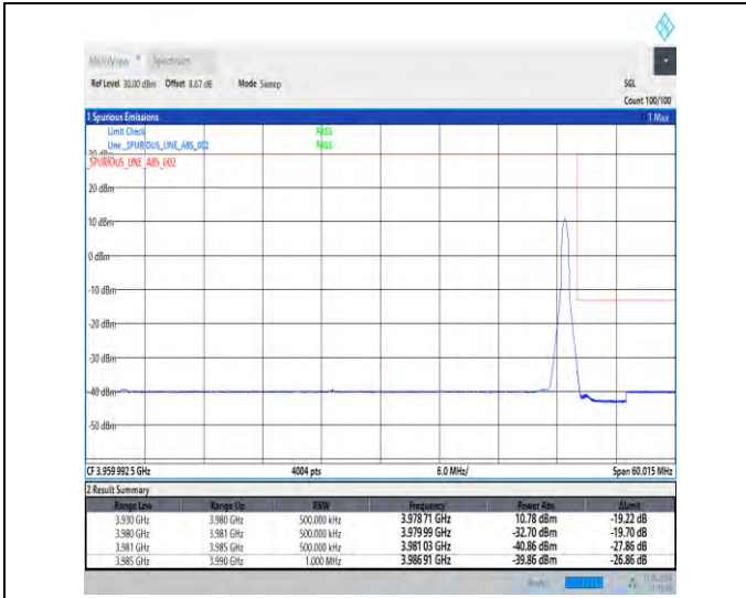
1-N77-3700-3980-30-50-H-2-DFT-PI2BPSK-Edge_1R_B_Right-1@132-Ant1-1--PASS-see graph
