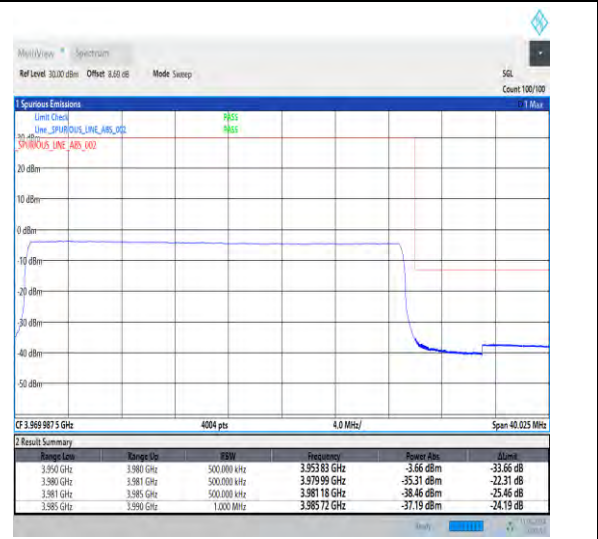
1-N77-3700-3980-30-30-H-6-CP-QPSK-Outer_Full-78@0-Ant1-1--PASS-see graph
