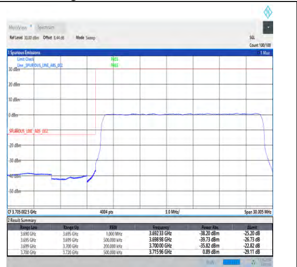
1-N77-3700-3980-30-20-L-3-DFT-PI2BPSK-Outer _Full-50@0-Ant1-1--PASS-see graph
