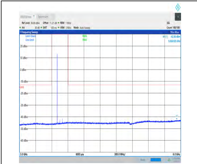
1-N77-3700-3980-30-100-L-1-DFT-QPSK-Edge_1R B_Left-1@0-3000-6000-Ant1-5926.02--42.58--13-PA SS
