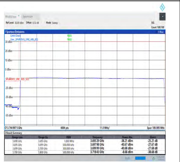
1-N77-3700-3980-30-100-L-6-CP-QPSK-Outer_Full-273@0-Ant1-1--PASS-see graph
