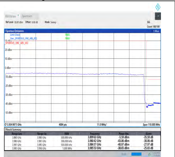
1-N77-3700-3980-30-100-H-3-DFT-PI2BPSK-Outer_Full-270@0-Ant1-1--PASS-see graph
