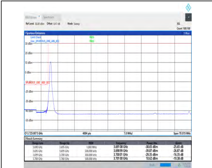
1-N77-3700-3980-30-60-L-1-DFT-PI2BPSK-Edge_1RB_Left-1@0-Ant1-1--PASS-see graph
