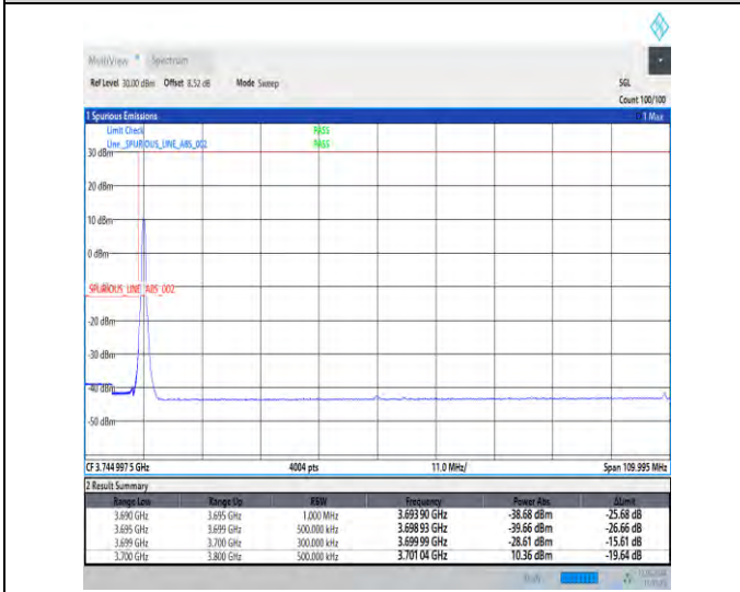
1-N77-3700-3980-30-100-L-4-CP-QPSK-Edge_1RB_Left-1@0-Ant1-1--PASS-see graph
