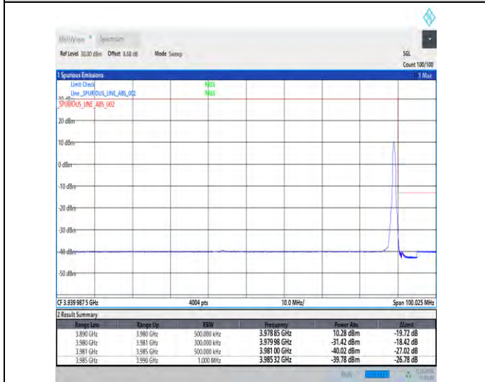
1-N77-3700-3980-30-90-H-5-CP-QPSK-Edge_1RB_Right-1@244-Ant1-1--PASS-see graph
