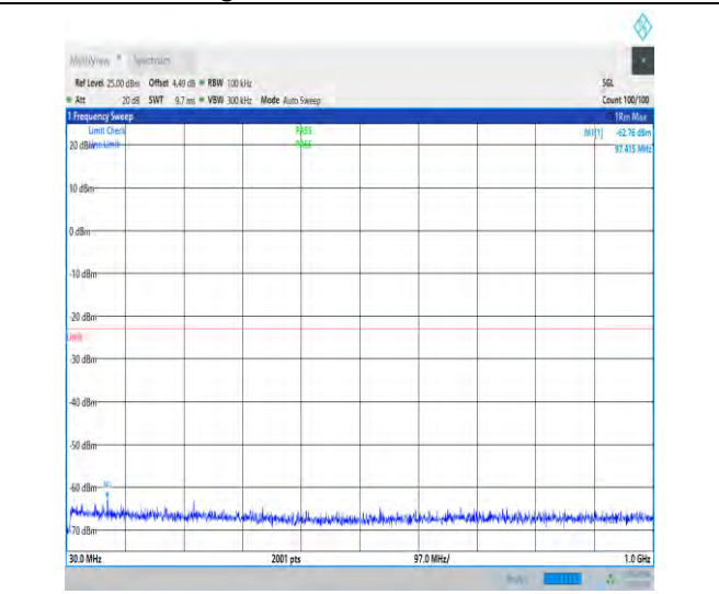
1-N77-3700-3980-30-100-M-1-DFT-QPSK-Edge_1R B_Left-1@0-30-1000-Ant1-97.42--62.76--23-PASS
