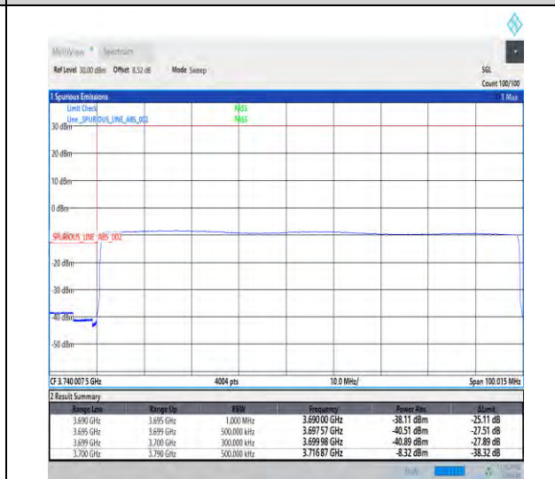
1-N77-3700-3980-30-90-L-6-CP-QPSK-Outer_Full -245@0-Ant1-1--PASS-see graph
