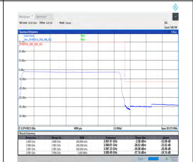
1-N77-3700-3980-30-20-H-6-CP-QPSK-Outer_Full-51@0-Ant1-1--PASS-see graph
