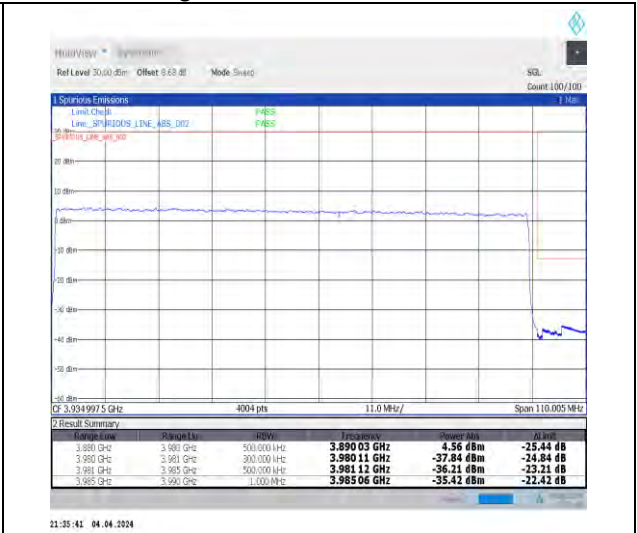
1-N77-3700-3980-30-100-H-3-DFT-PI2BPSK-Outer_Full-270@0-Ant1-1--PASS-see graph
