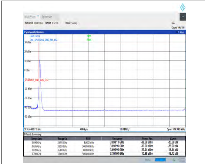
1-N77-3700-3980-100-L-1-DFT-PI2BPSK-Edge_1R_B_Left-1@0-Ant1-1--PASS-see graph
