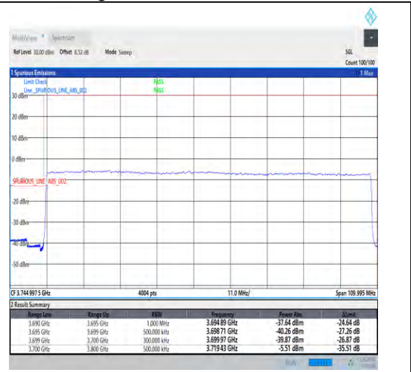
1-N77-3700-3980-30-100-L-3-DFT-PI2BPSK-Outer_Full-270@0-Ant1-1--PASS-see graph
