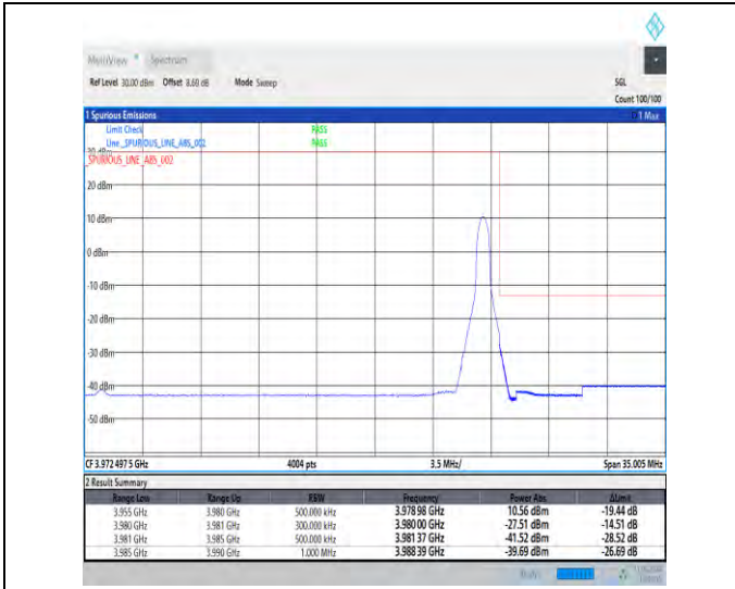
1-N77-3700-3980-30-25-H-2-DFT-PI2BPSK-Edge_1R_B_Right-1@64-Ant1-1--PASS-see graph
