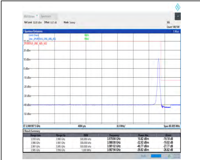
1-N77-3700-3980-30-70-H-2-DFT-PI2BPSK-Edge_1R_B_Right-1@188-Ant1-1--PASS-see graph
