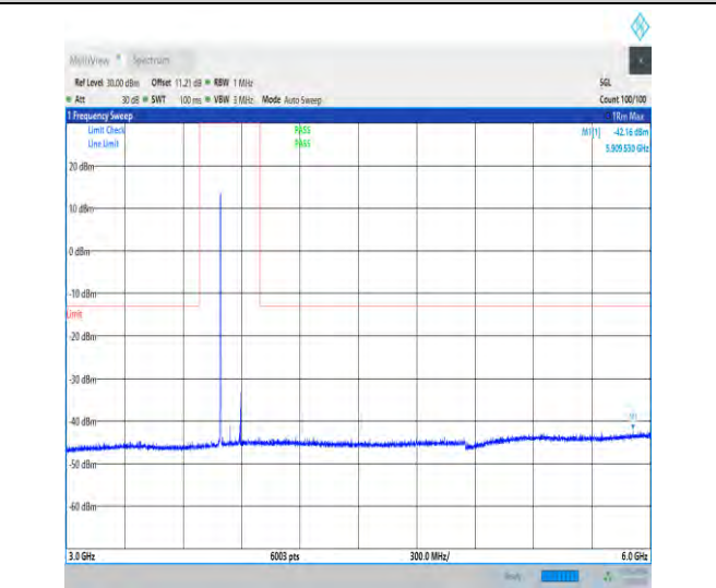
1-N77-3700-3980-30-100-M-1-DFT-QPSK-Edge_1R B_Left-1@0-3000-6000-Ant1-5909.53--42.16--13-PA
