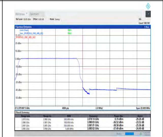
1-N77-3700-3980-30-10-H-6-CP-QPSK-Outer_Full-24@0-Ant1-1--PASS-see graph
