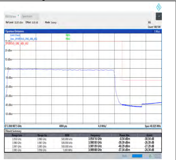
1-N77-3700-3980-30-30-H-3-DFT-PI2BPSK-Outer_Full-75@0-Ant1-1--PASS-see graph
