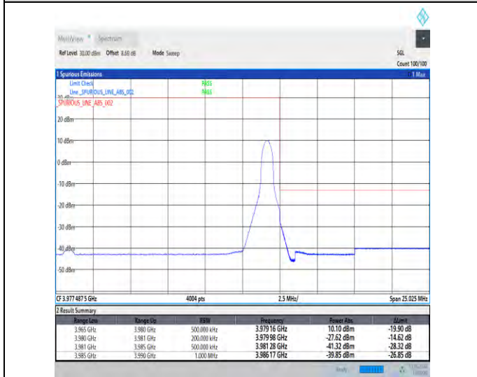
1-N77-3700-3980-30-15-H-5-CP-QPSK-Edge_1RB_Right-1@37-Ant1-1--PASS-see graph
