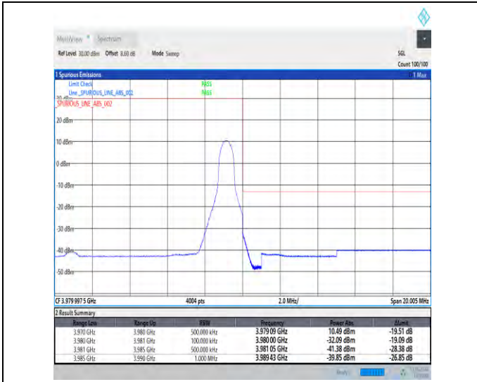
1-N77-3700-3980-30-10-H-2-DFT-PI2BPSK-Edge_1R_B_Right-1@23-Ant1-1--PASS-see graph
