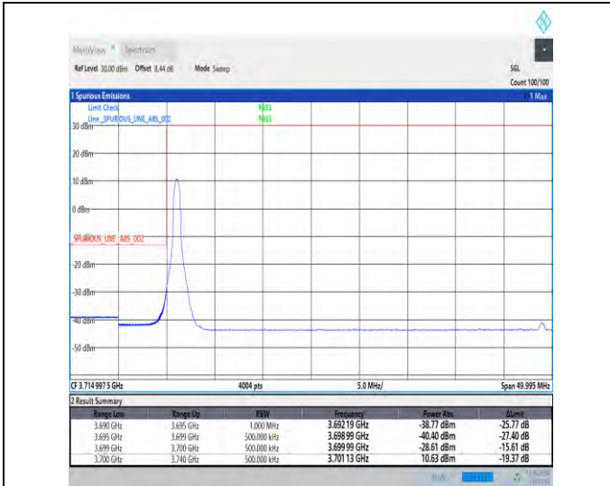
1-N77-3700-3980-30-40-L-1-DFT-PI2BPSK-Edge_1RB_Left-1@0-Ant1-1--PASS-see graph
