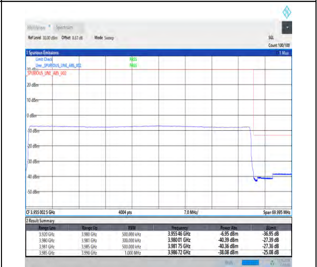
1-N77-3700-3980-30-60-H-6-CP-QPSK-Outer_Full-162@0-Ant1-1--PASS-see graph
