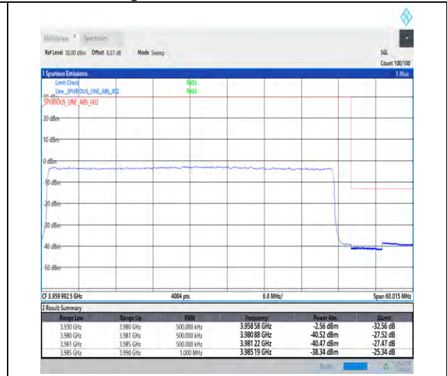
1-N77-3700-3980-30-50-H-3-DFT-PI2BPSK-Outer_Full-128@0-Ant1-1--PASS-see graph
