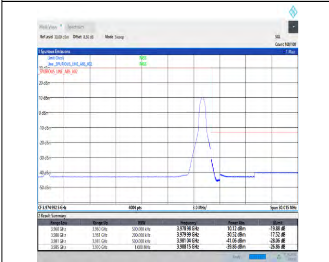
1-N77-3700-3980-30-20-H-5-CP-QPSK-Edge_1RB_Right-1@50-Ant1-1--PASS-see graph
