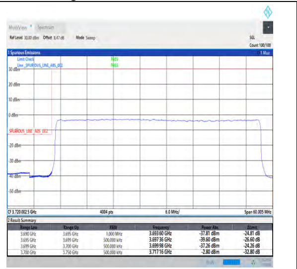
1-N77-3700-3980-30-50-L-3-DFT-PI2BPSK-Outer_Full-128@0-Ant1-1--PASS-see graph
