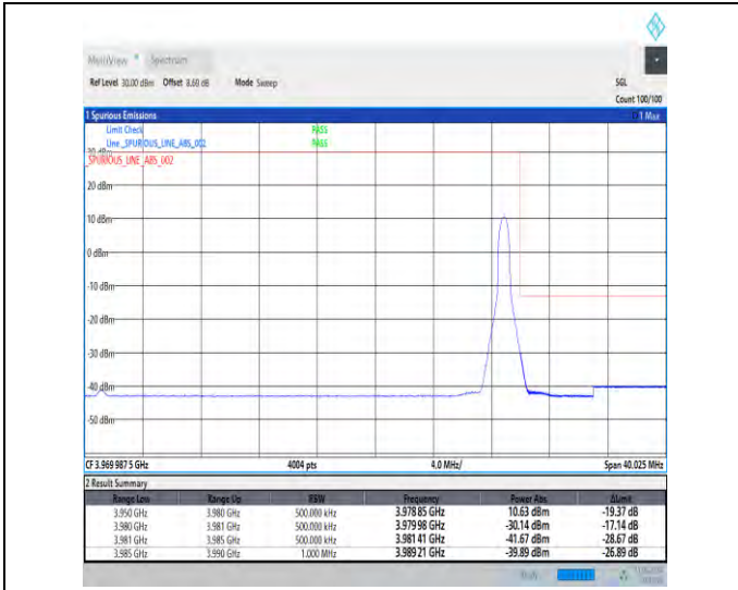
1-N77-3700-3980-30-30-H-2-DFT-PI2BPSK-Edge_1R_B_Right-1@77-Ant1-1--PASS-see graph
