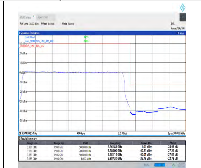
1-N77-3700-3980-30-20-H-3-DFT-PI2BPSK-Outer_Full-50@0-Ant1-1--PASS-see graph
