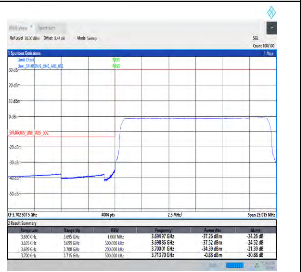
1-N77-3700-3980-30-15-L-6-CP-QPSK-Outer_Full -38@0-Ant1-1--PASS-see graph
