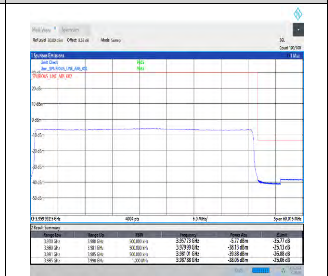
1-N77-3700-3980-30-50-H-6-CP-QPSK-Outer_Full-133@0-Ant1-1--PASS-see graph
