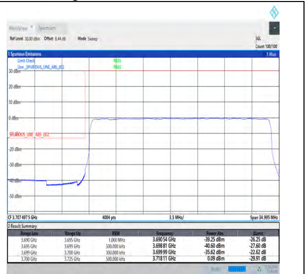
1-N77-3700-3980-30-25-L-3-DFT-PI2BPSK-Outer _Full-64@0-Ant1-1--PASS-see graph
