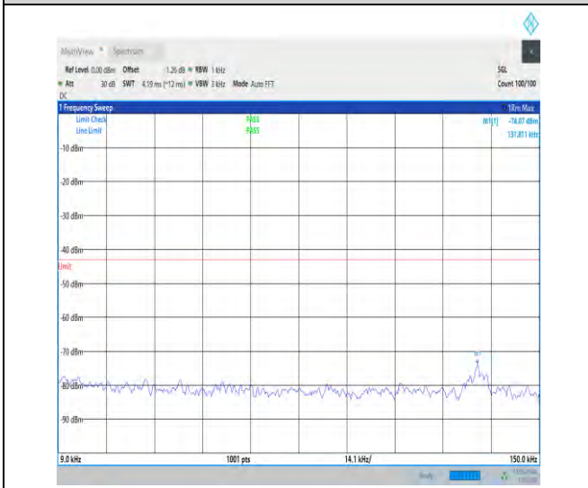
1-N77-3700-3980-30-100-H-1-DFT-QPSK-Edge_1R B_Left-1@0-0.009-0.15-Ant1-0.13--74.07--43-PASS
