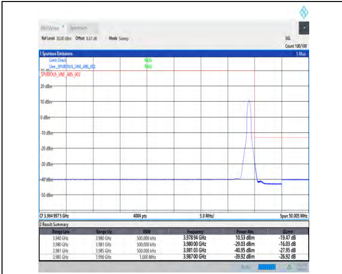
1-N77-3700-3980-30-40-H-2-DFT-PI2BPSK-Edge_1R_B_Right-1@105-Ant1-1--PASS-see graph
