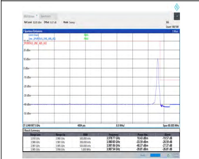
1-N77-3700-3980-30-70-H-5-CP-QPSK-Edge_1RB_Right-1@188-Ant1-1--PASS-see graph
