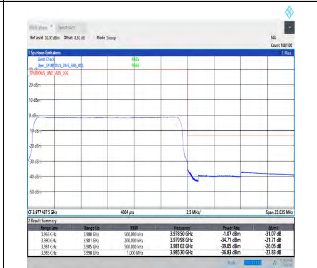
1-N77-3700-3980-30-15-H-6-CP-QPSK-Outer_Full-38@0-Ant1-1--PASS-see graph
