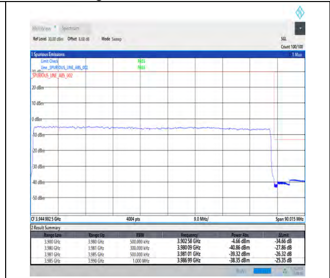
1-N77-3700-3980-30-80-H-3-DFT-PI2BPSK-Outer_Full-216@0-Ant1-1--PASS-see graph
