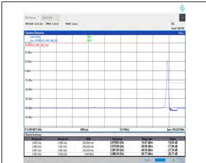
1-N77-3700-3980-30-90-H-2-DFT-PI2BPSK-Edge_1R_B_Right-1@244-Ant1-1--PASS-see graph
