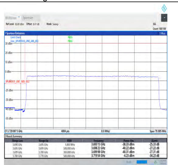
1-N77-3700-3980-30-70-L-3-DFT-PI2BPSK-Outer _Full-180@0-Ant1-1--PASS-see graph
