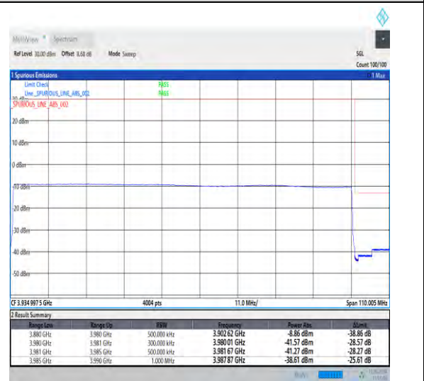
1-N77-3700-3980-30-100-H-6-CP-QPSK-Outer_Full-273@0-Ant1-1--PASS-see graph
