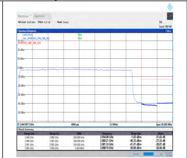
1-N77-3700-3980-30-40-H-3-DFT-PI2BPSK-Outer_Full-100@0-Ant1-1--PASS-see graph
