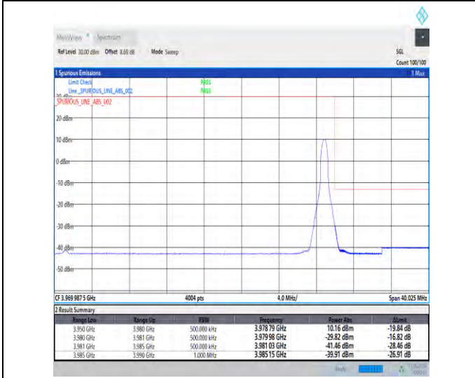
1-N77-3700-3980-30-30-H-5-CP-QPSK-Edge_1RB_Right-1@77-Ant1-1--PASS-see graph
