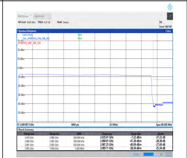
1-N77-3700-3980-30-70-H-6-CP-QPSK-Outer_Full-189@0-Ant1-1--PASS-see graph
