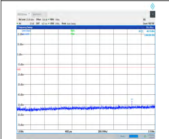
1-N77-3700-3980-30-100-M-1-DFT-QPSK-Edge_1R B_Left-1@0-1000-3000-Ant1-2664.58--48.10--13-PA
