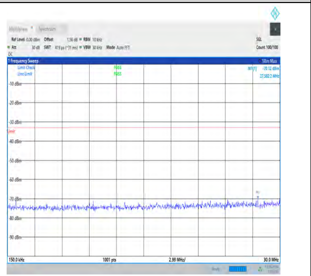
1-N77-3700-3980-30-100-H-1-DFT-QPSK-Edge_1R B_Left-1@0-0.15-30-Ant1-27.58--70.12--33-PASS
