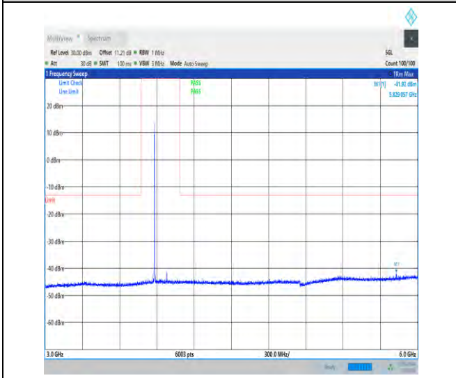
1-N77-3700-3980-30-100-H-1-DFT-QPSK-Edge_1R B_Left-1@0-3000-6000-Ant1-5829.06--41.92--13-PA SS
