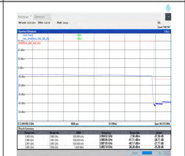
1-N77-3700-3980-30-80-H-6-CP-QPSK-Outer_Full-217@0-Ant1-1--PASS-see graph
