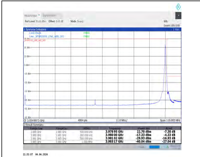
1-N77-3700-3980-30-100-H-2-DFT-PI2BPSK-Edge_1R_B_Right-1@272-Ant1-1--PASS-see graph
