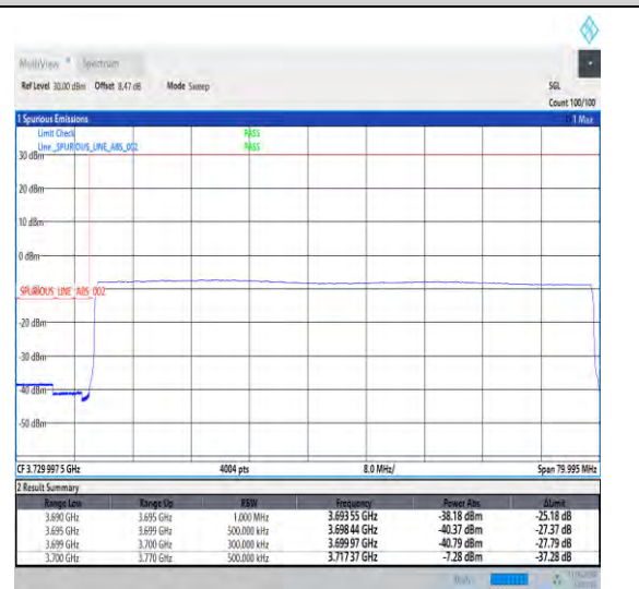
1-N77-3700-3980-30-70-L-6-CP-QPSK-Outer_Full -189@0-Ant1-1--PASS-see graph
