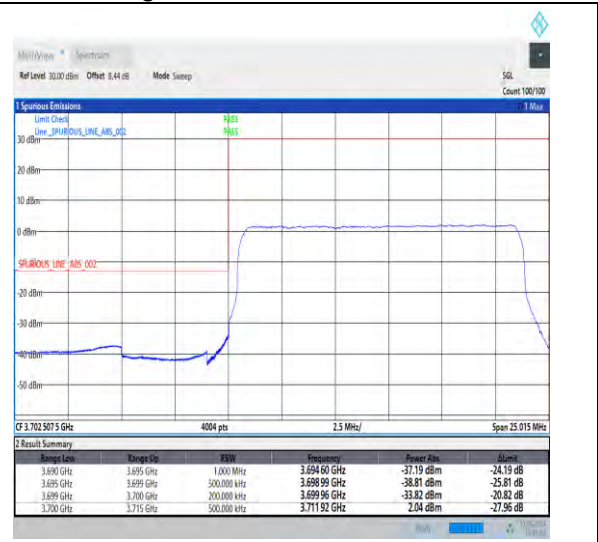
1-N77-3700-3980-30-15-L-3-DFT-PI2BPSK-Outer _Full-36@0-Ant1-1--PASS-see graph
