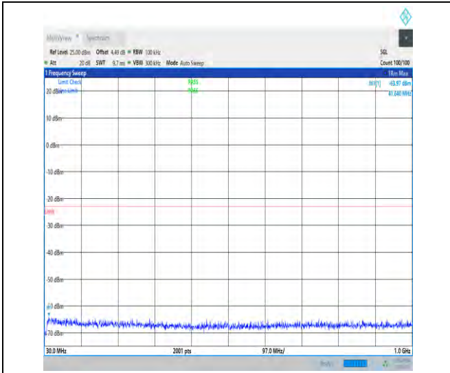
1-N77-3700-3980-30-100-H-1-DFT-QPSK-Edge_1R B_Left-1@0-30-1000-Ant1-41.64--63.97--23-PASS
