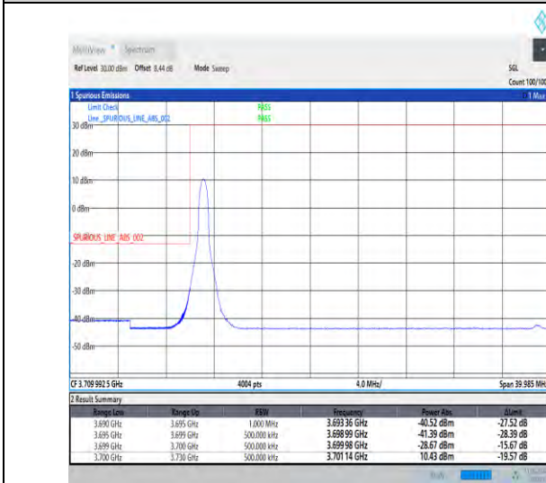
1-N77-3700-3980-30-30-L-4-CP-QPSK-Edge_1RB_Lef t-1@0-Ant1-1--PASS-see graph
