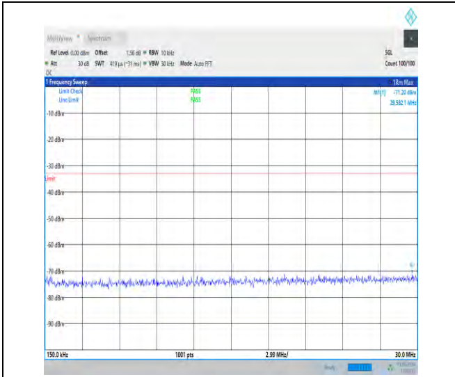
1-N77-3700-3980-30-100-M-1-DFT-QPSK-Edge_1R B_Left-1@0-0.15-30-Ant1-29.58--71.20--33-PASS
