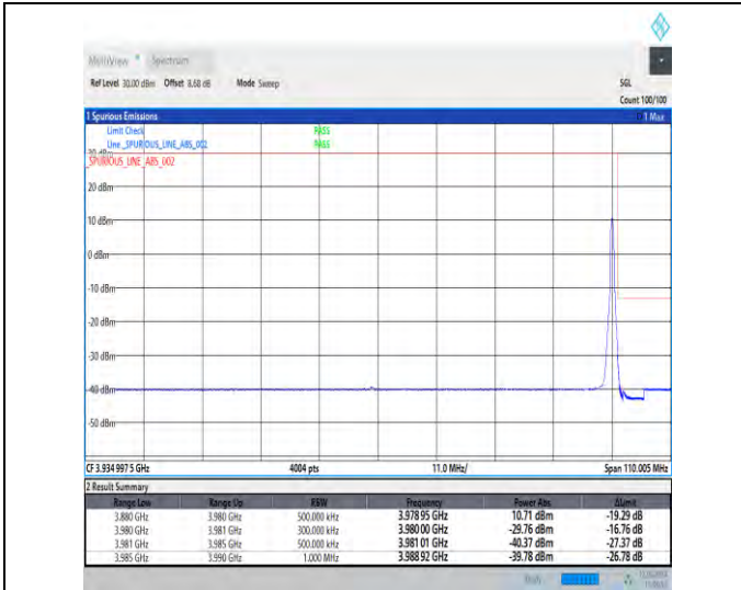
1-N77-3700-3980-100-H-2-DFT-PI2BPSK-Edge_1R_B_Right-1@272-Ant1-1--PASS-see graph
