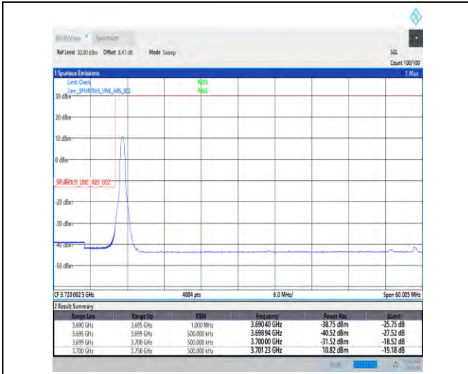
1-N77-3700-3980-30-50-L-1-DFT-PI2BPSK-Edge_1RB_Left-1@0-Ant1-1--PASS-see graph
