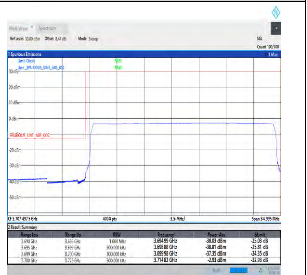
1-N77-3700-3980-30-25-L-6-CP-QPSK-Outer_Full -65@0-Ant1-1--PASS-see graph
