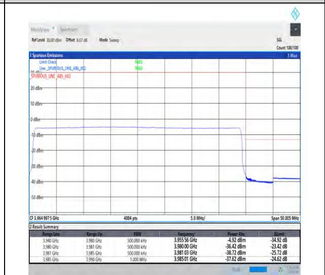
1-N77-3700-3980-30-40-H-6-CP-QPSK-Outer_Full-106@0-Ant1-1--PASS-see graph
