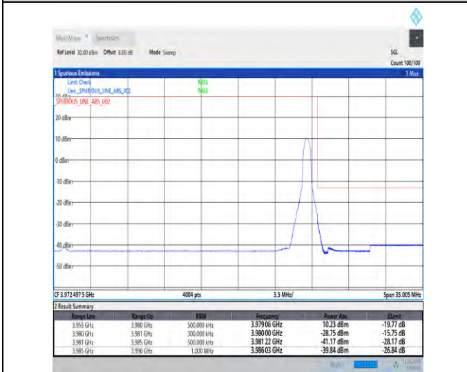
1-N77-3700-3980-30-25-H-5-CP-QPSK-Edge_1RB_Right-1@64-Ant1-1--PASS-see graph
