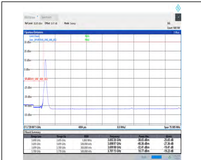
1-N77-3700-3980-30-70-L-1-DFT-PI2BPSK-Edge_1RB _Left-1@0-Ant1-1--PASS-see graph
