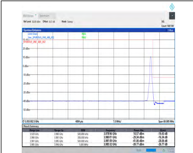
1-N77-3700-3980-30-60-H-2-DFT-PI2BPSK-Edge_1R_B_Right-1@161-Ant1-1--PASS-see graph
