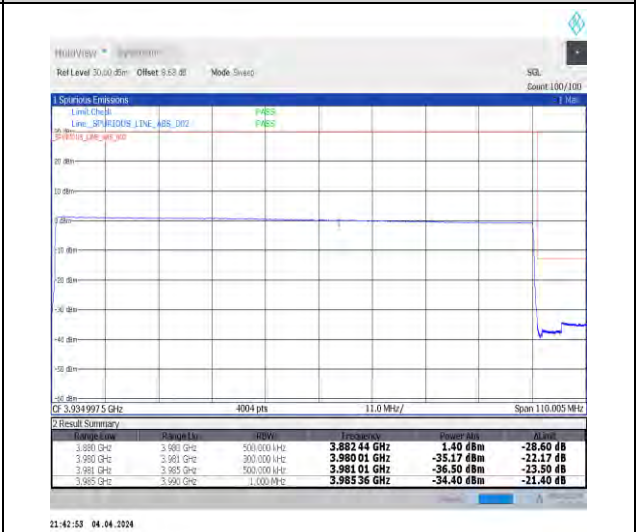
1-N77-3700-3980-30-100-H-6-CP-QPSK-Outer_Full-273@0-Ant1-1--PASS-see graph
