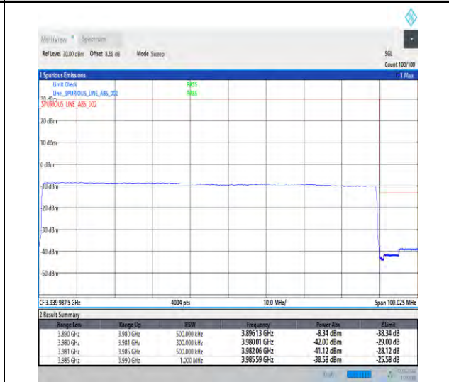
1-N77-3700-3980-30-90-H-6-CP-QPSK-Outer_Full-245@0-Ant1-1--PASS-see graph
