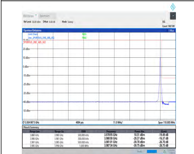
1-N77-3700-3980-30-100-H-5-CP-QPSK-Edge_1RB_Right-1@272-Ant1-1--PASS-see graph
