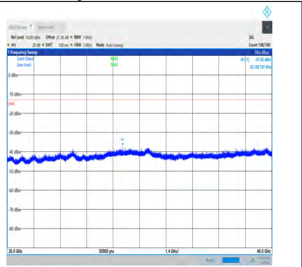
1-N77-3700-3980-30-100-M-1-DFT-QPSK-Edge_1R B_Left-1@0-26000-40000-Ant1-32105.14--37.03--13 -PASS
