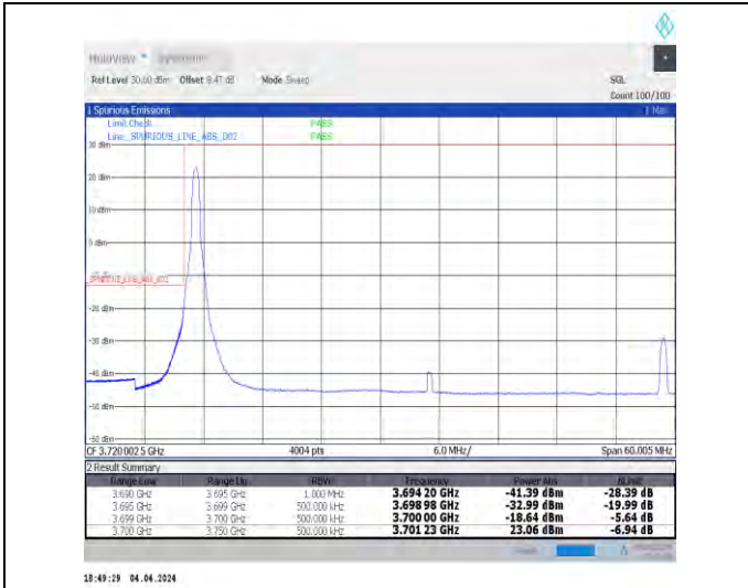
1-N77-3700-3980-30-50-L-1-DFT-PI2BPSK-Edge_1RB_Left-1@0-Ant1-1--PASS-see graph
