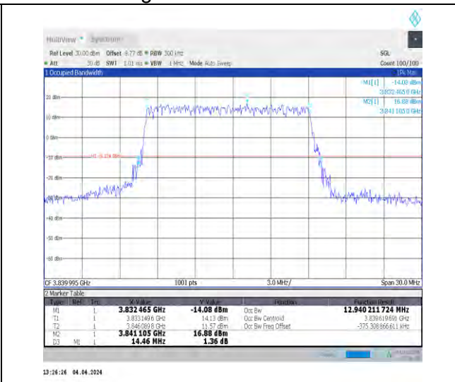
1-N77-3700-3980-30-15-M-4-DFT-64QAM-Outer_Fu II-36@0-Ant1-12.94-14.460-≤15-PASS
