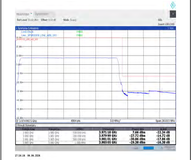
1-N77-3700-3980-30-20-H-6-CP-QPSK-Outer_Full-51@0-Ant1-1--PASS-see graph
