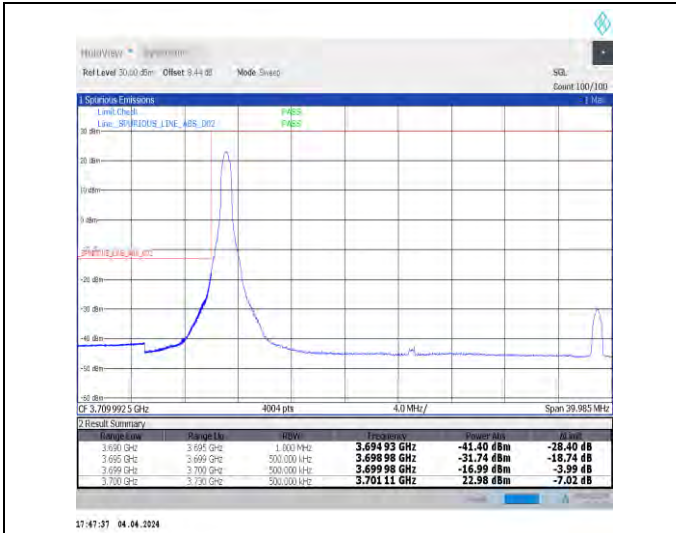
1-N77-3700-3980-30-30-L-1-DFT-PI2BPSK-Edge_1RB _Left-1@0-Ant1-1--PASS-see graph
