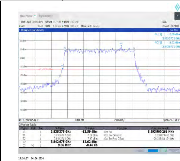
1-N77-3700-3980-30-10-M-5-DFT-256QAM-Outer_F ull-24@0-Ant1-8.594-9.360-≤10-PASS
