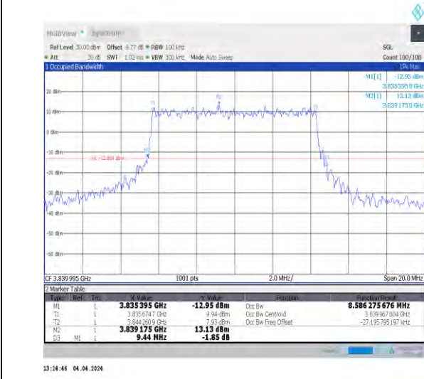
1-N77-3700-3980-30-10-M-7-CP-16QAM-Outer_Full -24@0-Ant1-8.586-9.440-≤10-PASS
