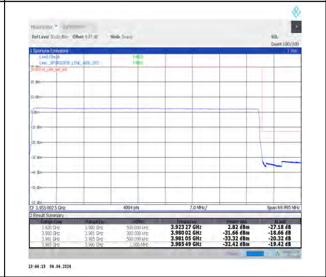
1-N77-3700-3980-30-60-H-6-CP-QPSK-Outer_Full-162@0-Ant1-1--PASS-see graph
