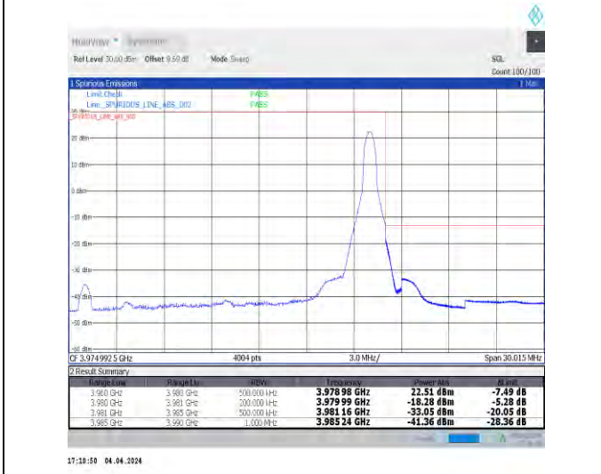
1-N77-3700-3980-30-20-H-5-CP-QPSK-Edge_1RB_Right-1@50-Ant1-1--PASS-see graph
