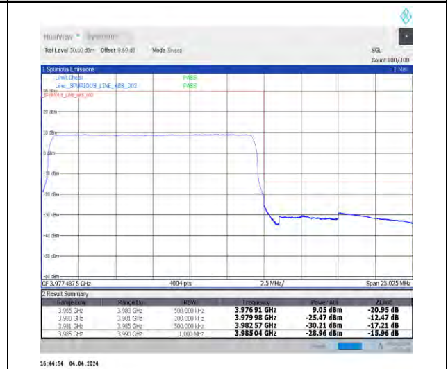
1-N77-3700-3980-30-15-H-6-CP-QPSK-Outer_Full-38@0-Ant1-1--PASS-see graph
