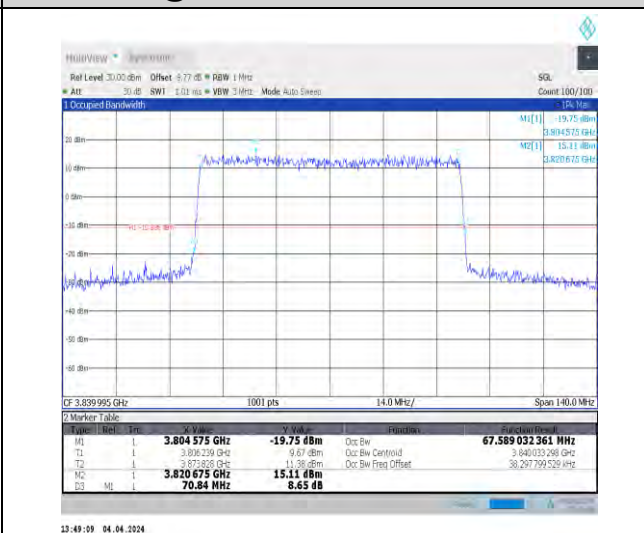
1-N77-3700-3980-30-70-M-7-CP-16QAM-Outer_Full I-189@0-Ant1-67.589-70.840-≤70-PASS
