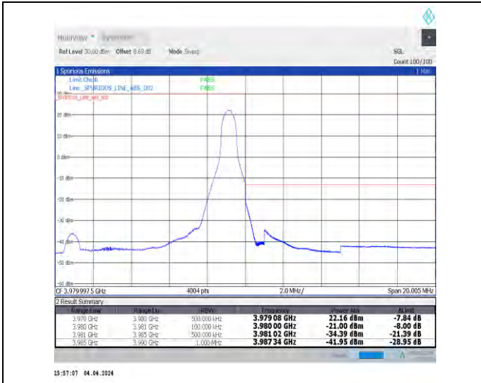
1-N77-3700-3980-30-10-H-2-DFT-PI2BPSK-Edge_1R_B_Right-1@23-Ant1-1--PASS-see graph
