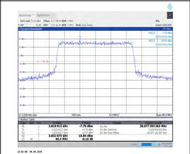
1-N77-3700-3980-30-40-M-6-CP-QPSK-Outer_Full- 106@0-Ant1-38.077-40.400-≤40-PASS
