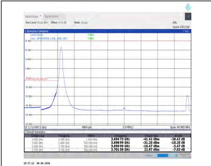
1-N77-3700-3980-30-40-L-1-DFT-PI2BPSK-Edge_1RB_Left-1@0-Ant1-1--PASS-see graph
