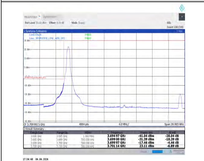
1-N77-3700-3980-30-30-L-4-CP-QPSK-Edge_1RB_Lef t-1@0-Ant1-1--PASS-see graph
