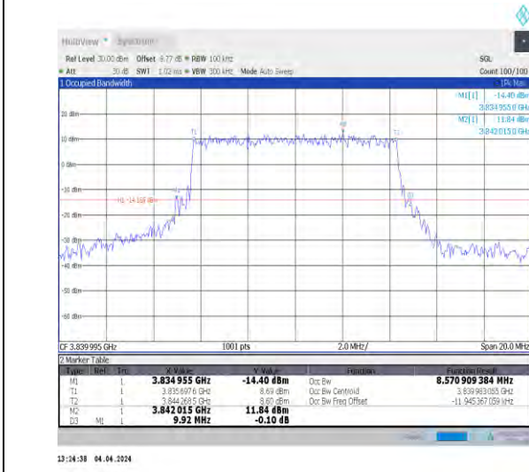
1-N77-3700-3980-30-10-M-6-CP-QPSK-Outer_Full-2 4@0-Ant1-8.571-9.920-≤10-PASS
