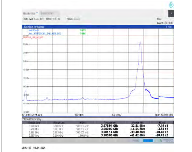
1-N77-3700-3980-30-40-H-5-CP-QPSK-Edge_1RB_Ri ght-1@105-Ant1-1--PASS-see graph
