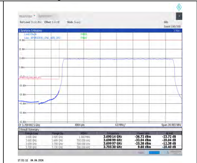
1-N77-3700-3980-30-30-L-3-DFT-PI2BPSK-Outer _Full-75@0-Ant1-1--PASS-see graph
