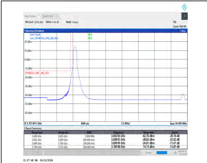
1-N77-3700-3980-30-25-L-1-DFT-PI2BPSK-Edge_1RB _Left-1@0-Ant1-1--PASS-see graph
