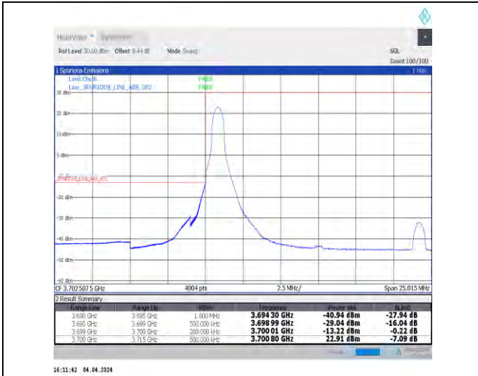
1-N77-3700-3980-30-15-L-1-DFT-PI2BPSK-Edge_1RB_Left-1@0-Ant1-1--PASS-see graph
