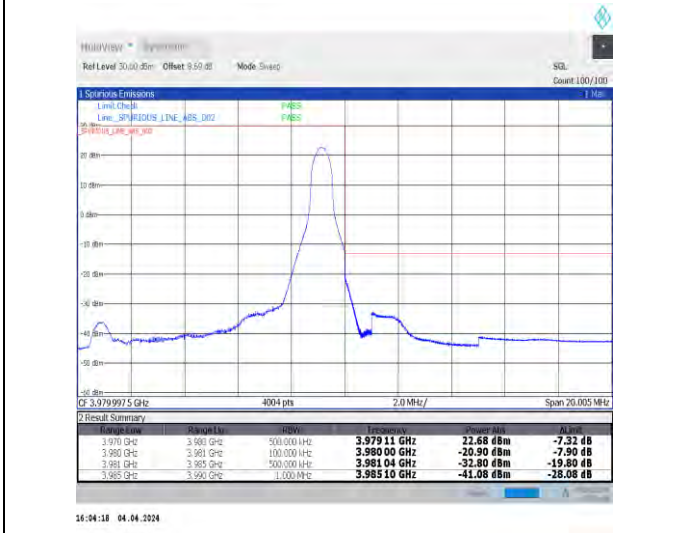
1-N77-3700-3980-30-10-H-5-CP-QPSK-Edge_1RB_Right-1@23-Ant1-1--PASS-see graph
