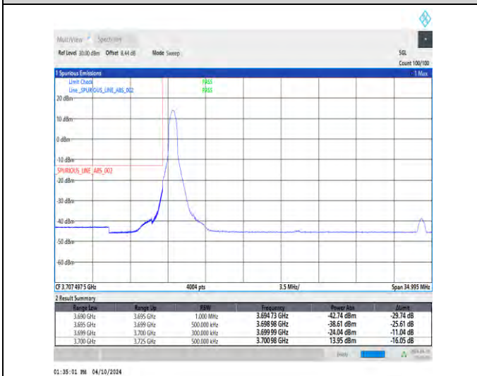
1-N77-3700-3980-30-25-L-4-CP-QPSK-Edge_1RB_Lef t-1@0-Ant1-1--PASS-see graph
