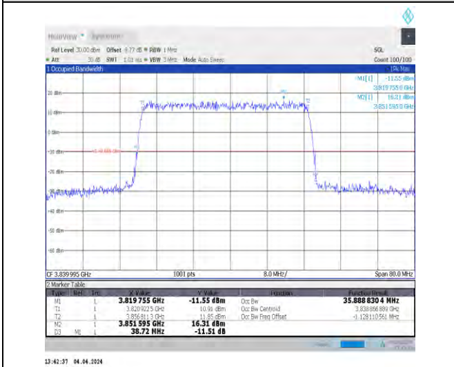
1-N77-3700-3980-30-40-M-5-DFT-256QAM-Outer_F ull-100@0-Ant1-35.889-38.720-≤40-PASS
