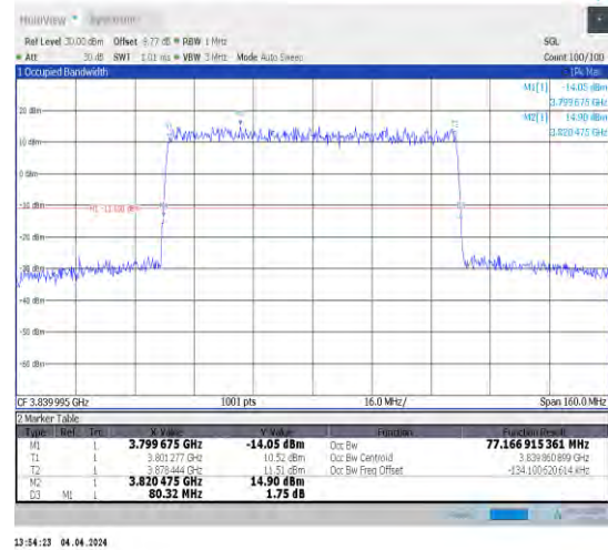
1-N77-3700-3980-30-80-M-4-DFT-64QAM-Outer_Full II-216@0-Ant1-77.167-80.320-≤80-PASS
