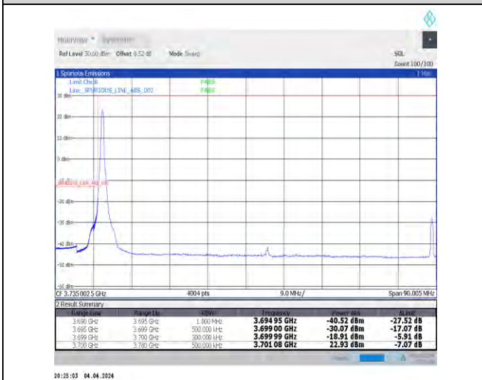
1-N77-3700-3980-30-80-L-4-CP-QPSK-Edge_1RB_Lef t-1@0-Ant1-1--PASS-see graph
