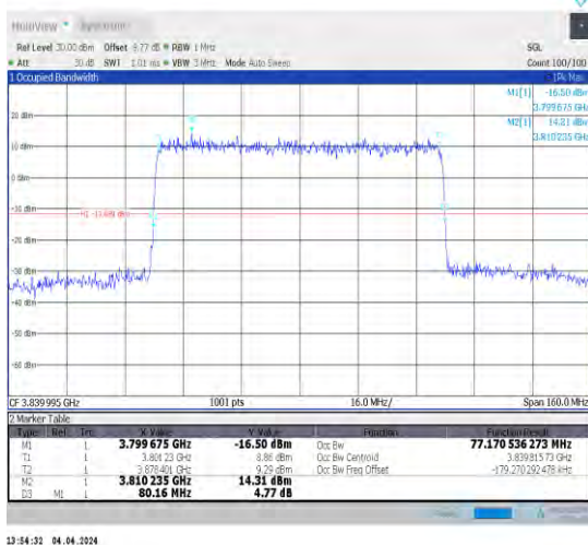
1-N77-3700-3980-30-80-M-5-DFT-256QAM-Outer_Full ull-216@0-Ant1-77.171-80.160-≤80-PASS
