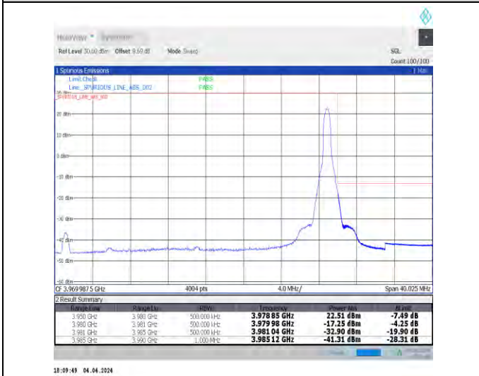
1-N77-3700-3980-30-30-H-5-CP-QPSK-Edge_1RB_Right-1@77-Ant1-1--PASS-see graph
