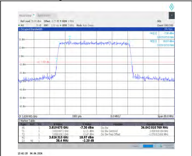
1-N77-3700-3980-30-40-M-4-DFT-64QAM-Outer_Fu II-100@0-Ant1-36.042-38.400-≤40-PASS
