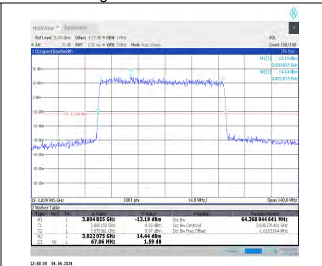
1-N77-3700-3980-30-70-M-5-DFT-256QAM-Outer_Full I-180@0-Ant1-64.369-67.060-≤70-PASS
