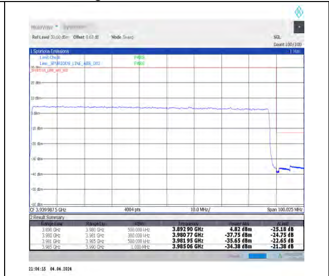
1-N77-3700-3980-30-90-H-3-DFT-PI2BPSK-Outer_Full-240@0-Ant1-1--PASS-see graph
