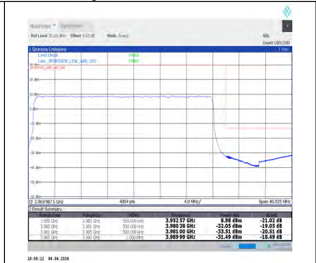
1-N77-3700-3980-30-30-H-3-DFT-PI2BPSK-Outer_Full-75@0-Ant1-1--PASS-see graph
