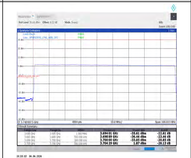
1-N77-3700-3980-30-90-L-6-CP-QPSK-Outer_Full -245@0-Ant1-1--PASS-see graph
