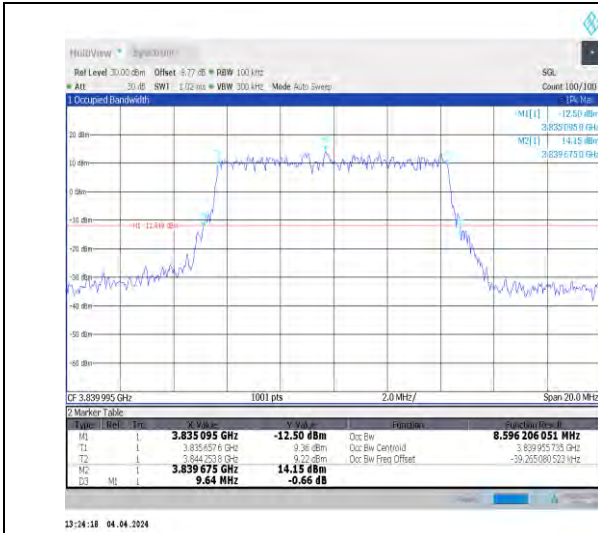
1-N77-3700-3980-30-10-M-4-DFT-64QAM-Outer_Ful I-24@0-Ant1-8.596-9.640-≤10-PASS
