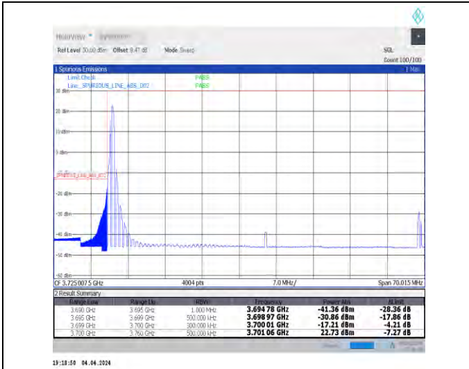
1-N77-3700-3980-30-60-L-1-DFT-PI2BPSK-Edge_1RB_Left-1@0-Ant1-1--PASS-see graph
