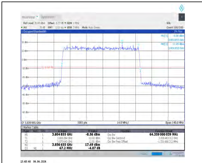
1-N77-3700-3980-30-70-M-4-DFT-64QAM-Outer_Full I-180@0-Ant1-64.359-67.200-≤70-PASS
