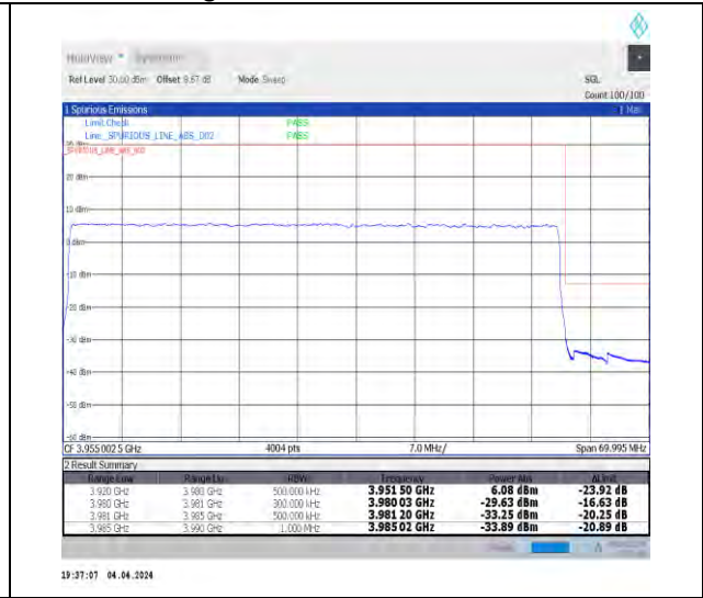
1-N77-3700-3980-30-60-H-3-DFT-PI2BPSK-Outer_Full-162@0-Ant1-1--PASS-see graph
