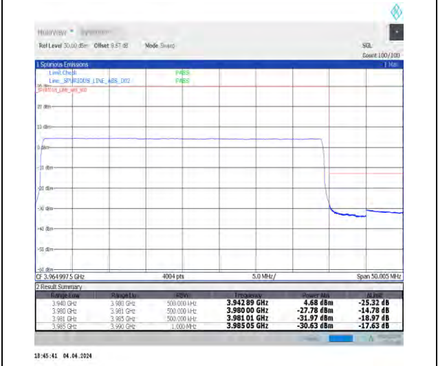
1-N77-3700-3980-30-40-H-6-CP-QPSK-Outer_Full -106@0-Ant1-1--PASS-see graph
