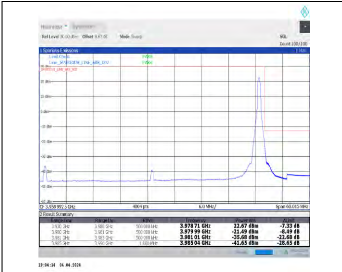
1-N77-3700-3980-30-50-H-2-DFT-PI2BPSK-Edge_1R B_Right-1@132-Ant1-1--PASS-see graph
