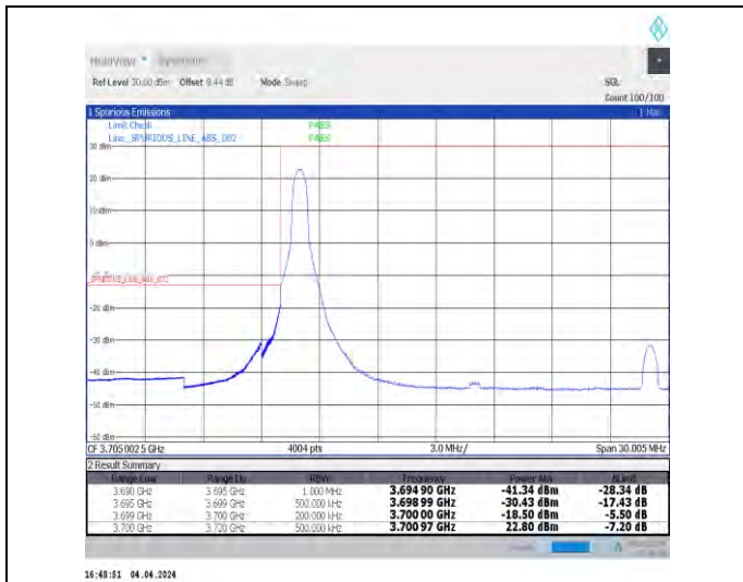
1-N77-3700-3980-30-20-L-1-DFT-PI2BPSK-Edge_1RB_Left-1@0-Ant1-1--PASS-see graph
