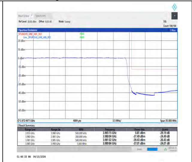
1-N77-3700-3980-30-25-H-3-DFT-PI2BPSK-Outer_Full-64@0-Ant1-1--PASS-see graph
