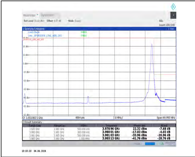
1-N77-3700-3980-30-60-H-2-DFT-PI2BPSK-Edge_1R B_Right-1@161-Ant1-1--PASS-see graph
