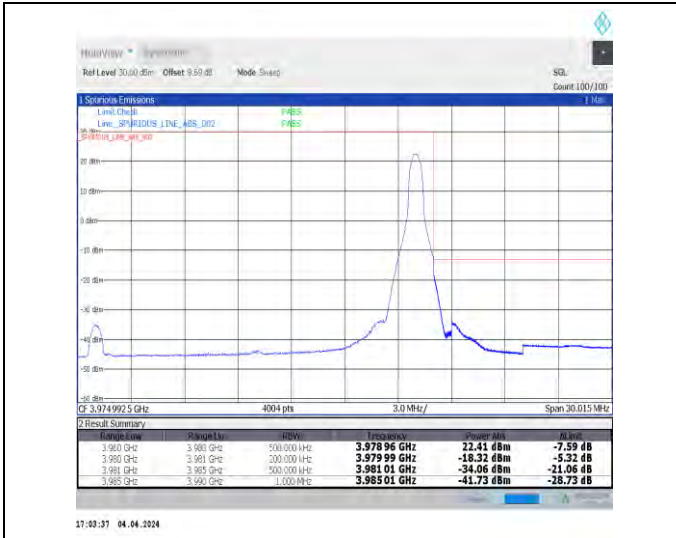
1-N77-3700-3980-30-20-H-2-DFT-PI2BPSK-Edge_1R_B_Right-1@50-Ant1-1--PASS-see graph
