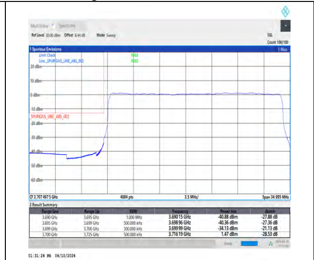
1-N77-3700-3980-30-25-L-3-DFT-PI2BPSK-Outer _Full-64@0-Ant1-1--PASS-see graph
