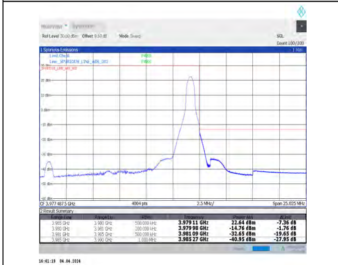
1-N77-3700-3980-30-15-H-5-CP-QPSK-Edge_1RB_Right-1@37-Ant1-1--PASS-see graph
