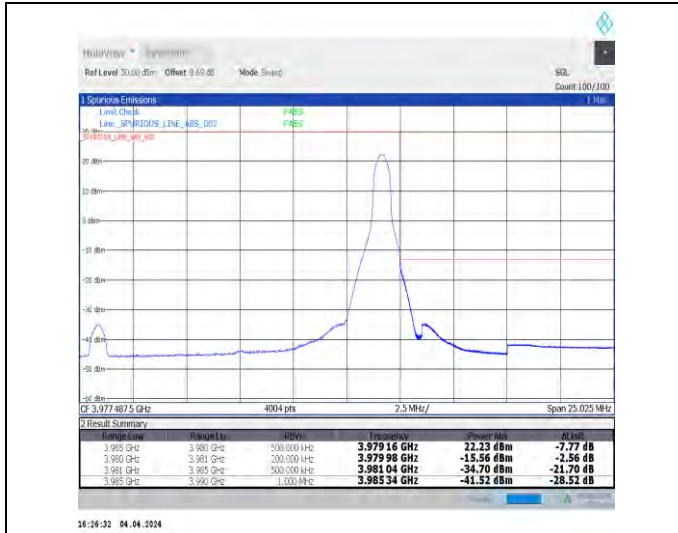
1-N77-3700-3980-30-15-H-2-DFT-PI2BPSK-Edge_1R_B_Right-1@37-Ant1-1--PASS-see graph
