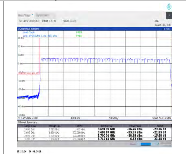
1-N77-3700-3980-30-60-L-3-DFT-PI2BPSK-Outer_Full-162@0-Ant1-1--PASS-see graph
