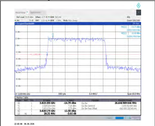
1-N77-3700-3980-30-30-M-5-DFT-256QAM-Outer_Full ull-75@0-Ant1-26.648-28.320-≤30-PASS
