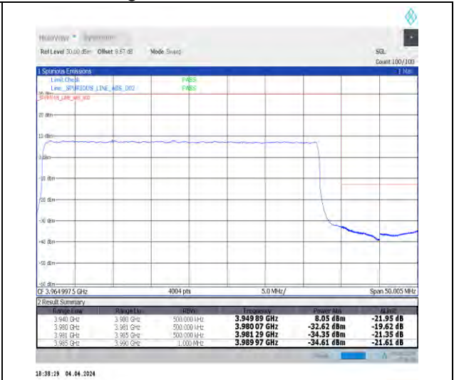
1-N77-3700-3980-30-40-H-3-DFT-PI2BPSK-Outer _Full-100@0-Ant1-1--PASS-see graph
