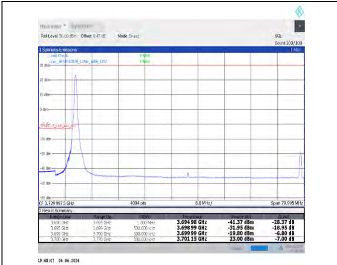
1-N77-3700-3980-30-70-L-1-DFT-PI2BPSK-Edge_1RB_Left-1@0-Ant1-1--PASS-see graph
