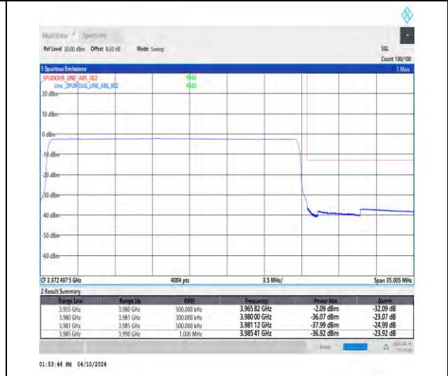
1-N77-3700-3980-30-25-H-6-CP-QPSK-Outer_Full-65@0-Ant1-1--PASS-see graph
