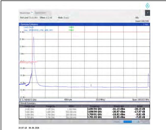
1-N77-3700-3980-30-90-L-1-DFT-PI2BPSK-Edge_1RB_Left-1@0-Ant1-1--PASS-see graph
