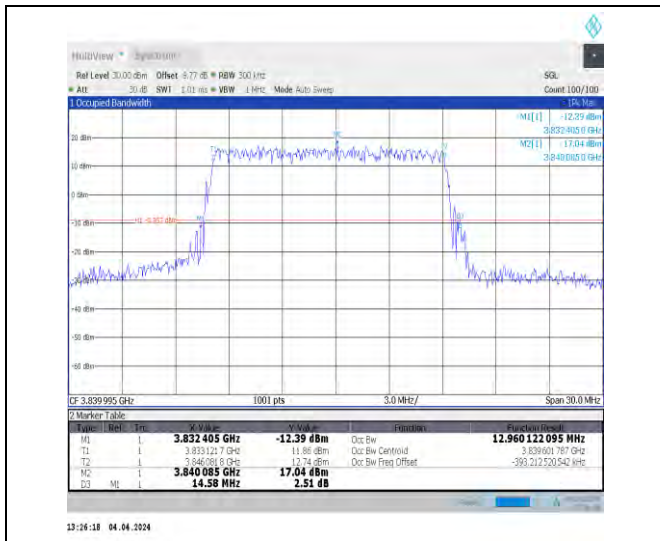
1-N77-3700-3980-30-15-M-3-DFT-16QAM-Outer_Ful I-36@0-Ant1-12.96-14.580-≤15-PASS
