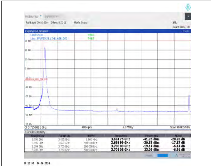
1-N77-3700-3980-30-80-L-1-DFT-PI2BPSK-Edge_1RB _Left-1@0-Ant1-1--PASS-see graph
