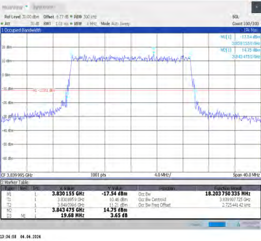
1-N77-3700-3980-30-20-M-6-CP-QPSK-Outer_Full-5 1@0-Ant1-18.204-19.680-≤20-PASS
