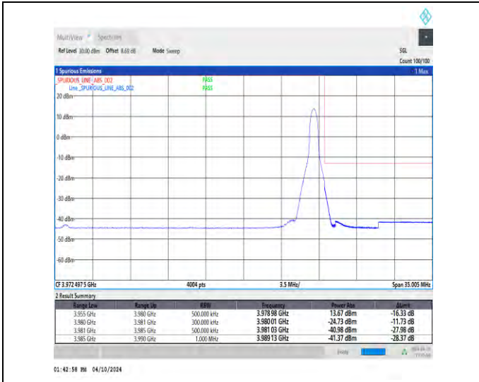
1-N77-3700-3980-30-25-H-2-DFT-PI2BPSK-Edge_1R_B_Right-1@64-Ant1-1--PASS-see graph
