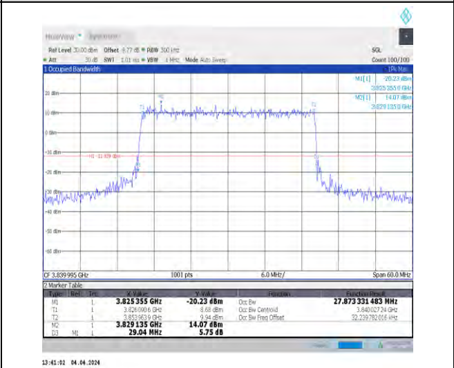
1-N77-3700-3980-30-30-M-7-CP-16QAM-Outer_Full -78@0-Ant1-27.875-29.040-≤30-PASS
