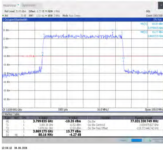
1-N77-3700-3980-30-80-M-3-DFT-16QAM-Outer_Full I-216@0-Ant1-77.031-80.160-≤80-PASS
