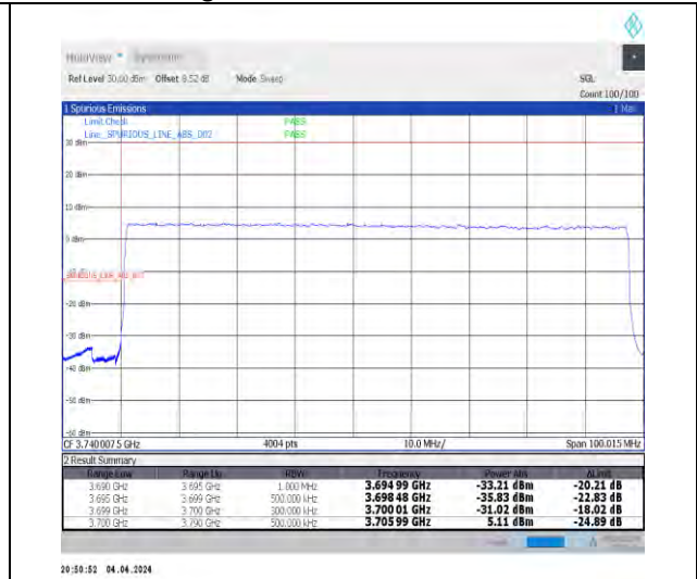
1-N77-3700-3980-30-90-L-3-DFT-PI2BPSK-Outer_Full-240@0-Ant1-1--PASS-see graph
