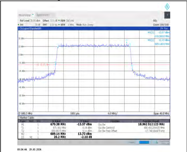
1-N71-15-20-M-7-CP-16QAM-Outer_Full-106@0-Ant1 t1-18.962-20.200-≤20-PASS
