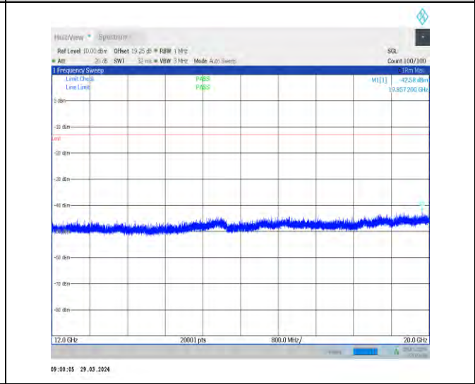
1-N71-15-20-M-1-DFT-PI2BPSK-Inner_1RB_Left-1@ 1-12000-20000-Ant1-19857.20--42.58--13-PASS
