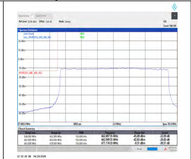
1-N71-15-15-L-3-DFT-PI2BPSK-Outer_Full-75@0-Ant1-1--PASS-see graph
