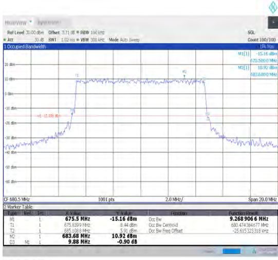
1-N71-15-10-M-8-CP-64QAM-Outer_Full-52@0-Ant1 -9.269-9.880-≤10-PASS
