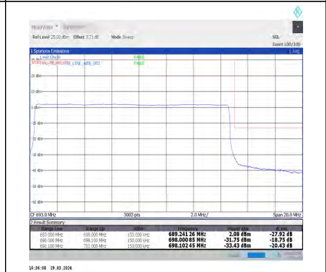
1-N71-15-15-H-6-CP-QPSK-Outer_Full-79@0-Ant1-1--PASS-see graph
