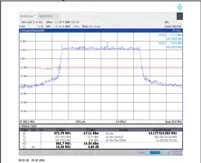
1-N71-15-15-M-8-CP-64QAM-Outer_Full-79@0-Ant1 1-14.178-15.360-≤15-PASS
