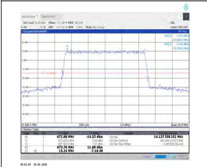
1-N71-15-15-M-9-CP-256QAM-Outer_Full-79@0-Ant1 1-14.137-15.240-≤15-PASS
