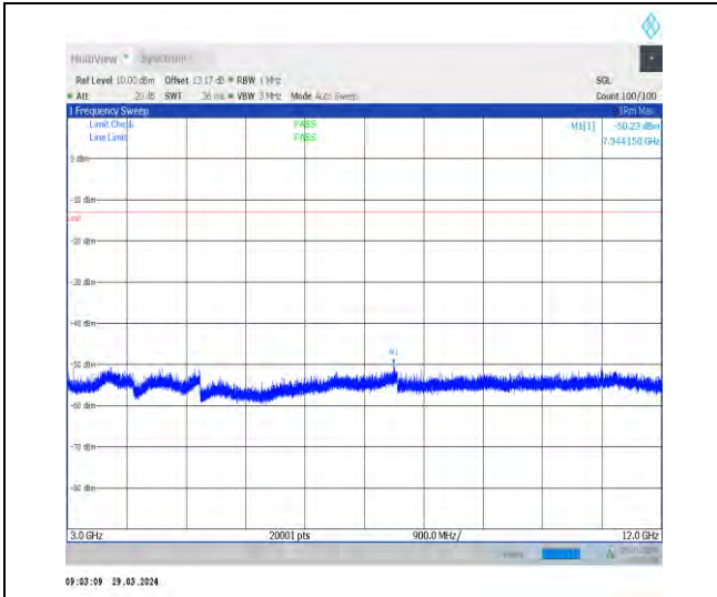
1-N71-15-20-H-1-DFT-PI2BPSK-Inner_1RB_Left-1 @1-3000-12000-Ant1-7944.15--50.23--13-PASS
