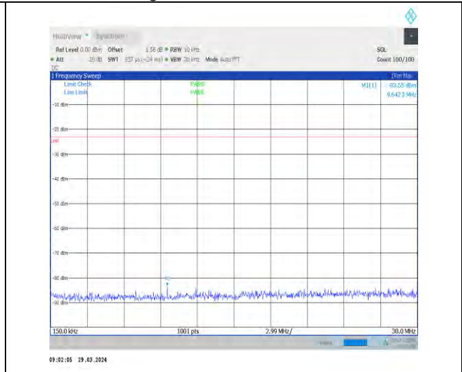
1-N71-15-20-H-1-DFT-PI2BPSK-Inner_1RB_Left-1@ 1-0.15-30-Ant1-9.64--83.55--23-PASS
