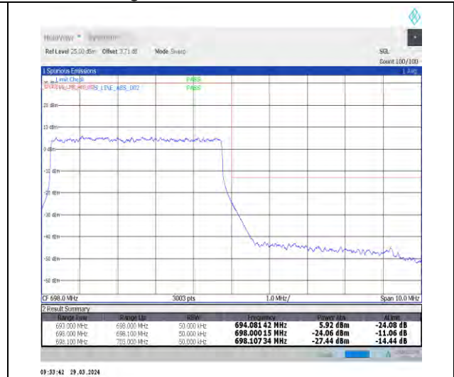
1-N71-15-5-H-3-DFT-PI2BPSK-Outer_Full-25@0-Ant1-1--PASS-see graph
