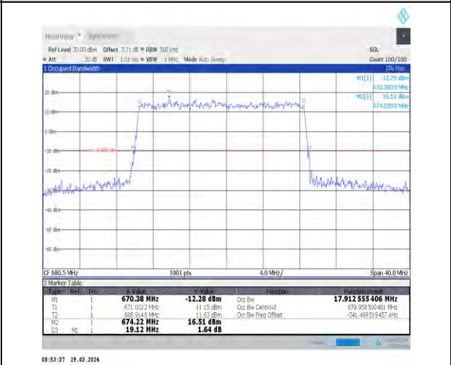
1-N71-15-20-M-1-DFT-QPSK-Outer_Full-100@0-Ant1 1-17.913-19.120-≤20-PASS
