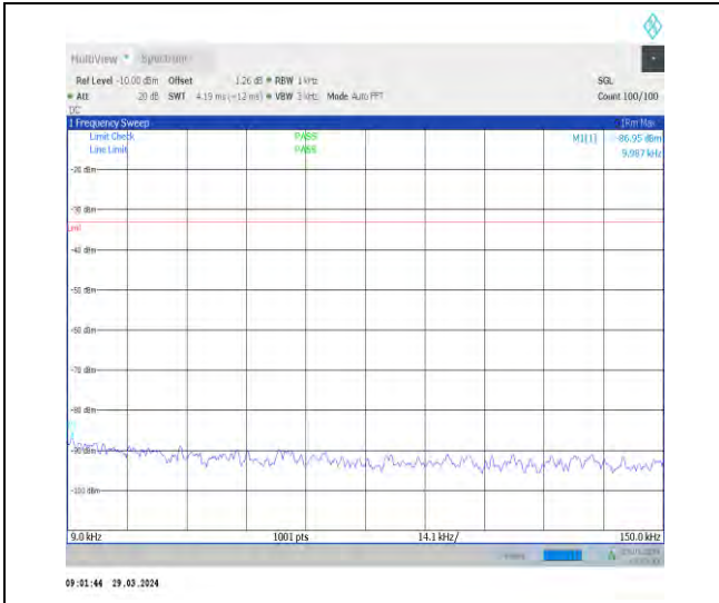
1-N71-15-20-H-1-DFT-PI2BPSK-Inner_1RB_Left-1 @1-0.009-0.15-Ant1-0.01--86.95--33-PASS
