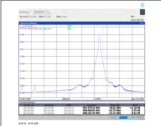
1-N71-15-10-H-5-CP-QPSK-Edge_1RB_Right-1@51-Ant1-1--PASS-see graph
