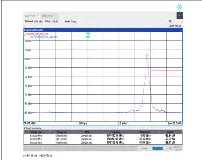
1-N71-15-20-H-5-CP-QPSK-Edge_1RB_Right-1@105-Ant1-1--PASS-see graph
