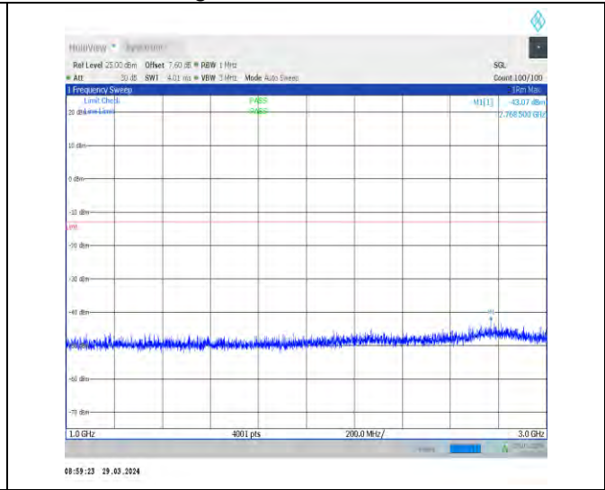
1-N71-15-20-M-1-DFT-PI2BPSK-Inner_1RB_Left-1@ 1-1000-3000-Ant1-2768.50--43.07--13-PASS
