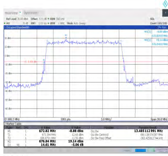
1-N71-15-15-M-2-DFT-PI2BPSK-Outer_Full-75@0-A nt1-13.485-14.610-≤15-PASS
