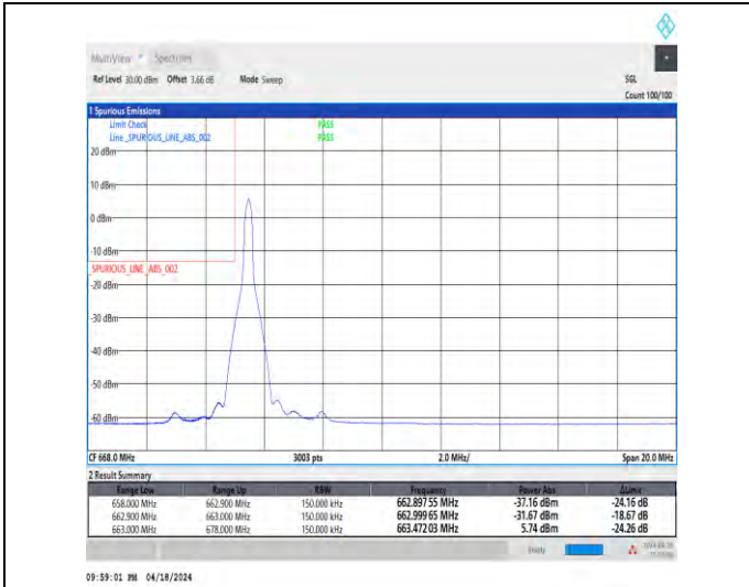
1-N71-15-15-L-1-DFT-PI2BPSK-Edge_1RB_Left-1@0-Ant1-1--PASS-see graph
