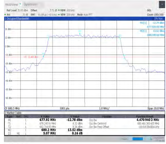
1-N71-15-5-M-6-CP-QPSK-Outer_Full-25@0-Ant1-4 .471-5.070-≤5-PASS
