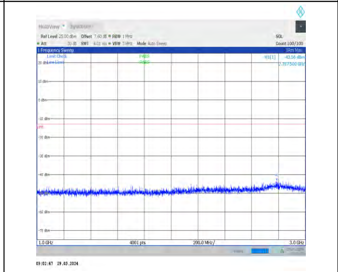
1-N71-15-20-H-1-DFT-PI2BPSK-Inner_1RB_Left-1@ 1-1000-3000-Ant1-2787.50--43.56--13-PASS
