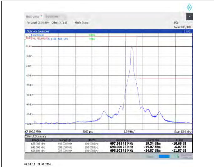
1-N71-15-10-H-2-DFT-PI2BPSK-Edge_1RB_Right-1@51-Ant1-1--PASS-see graph
