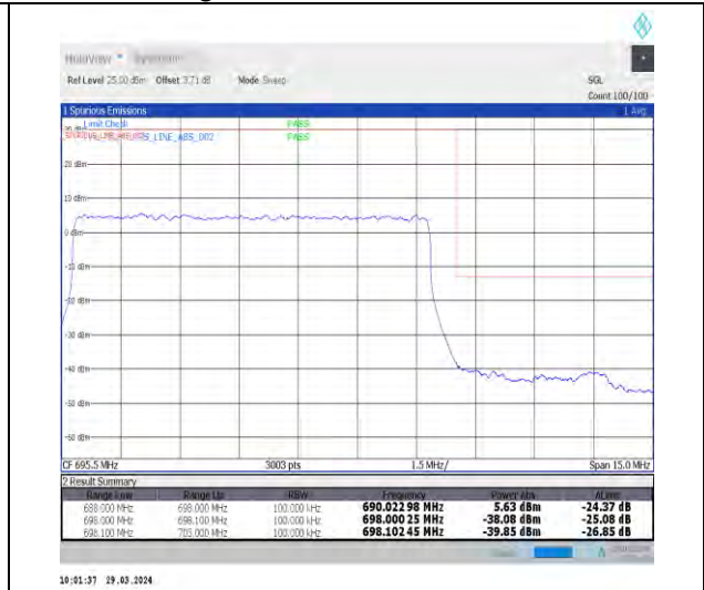
1-N71-15-10-H-3-DFT-PI2BPSK-Outer_Full-50@0-Ant1-1--PASS-see graph
