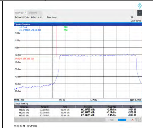
1-N71-15-10-L-3-DFT-PI2BPSK-Outer_Full-50@0-Ant1-1--PASS-see graph
