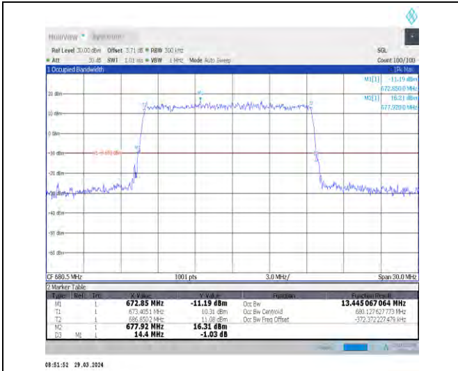
1-N71-15-15-M-3-DFT-16QAM-Outer_Full-75@0-Ant 1-13.445-14.400-≤15-PASS
