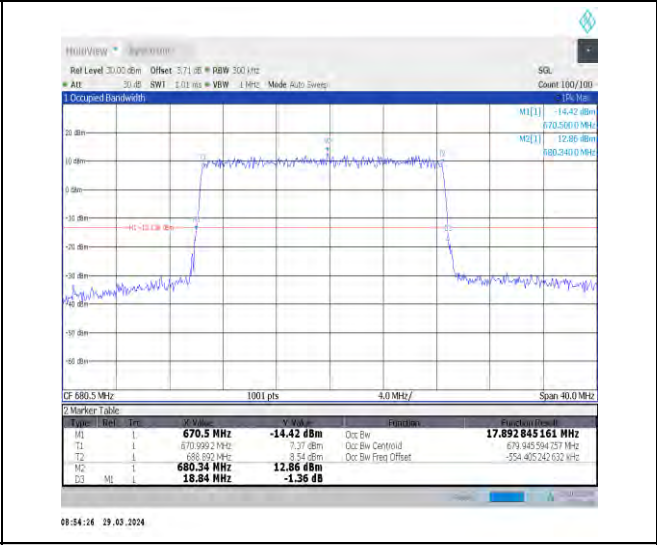
1-N71-15-20-M-5-DFT-256QAM-Outer_Full-100@0-Ant1-17.893-18.840-≤20-PASS
