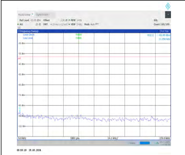
1-N71-15-20-M-1-DFT-PI2BPSK-Inner_1RB_Left-1 @ 1-0.009-0.15-Ant1-0.01--85.90--33-PASS
