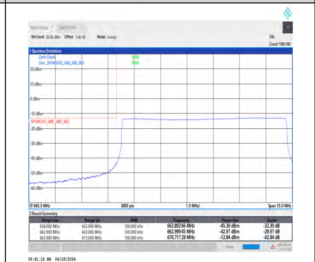
1-N71-15-10-L-6-CP-QPSK-Outer_Full-52@0-Ant1-1--PASS-see graph
