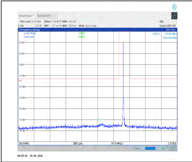
1-N71-15-20-M-1-DFT-PI2BPSK-Inner_1RB_Left-1 @1-30-1000-Ant1-526.64--52.83--13-PASS
