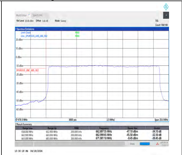
1-N71-15-20-L-3-DFT-PI2BPSK-Outer_Full-100@0-Ant1-1--PASS-see graph
