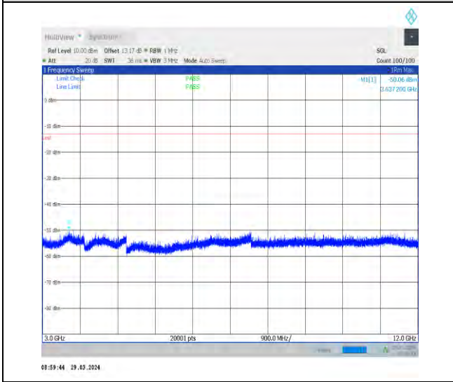
1-N71-15-20-M-1-DFT-PI2BPSK-Inner_1RB_Left-1 @1-3000-12000-Ant1-3637.20--50.06--13-PASS
