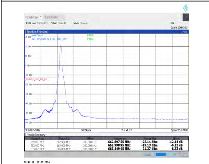
1-N71-15-20-L-4-CP-QPSK-Edge_1RB_Left-1@0-Ant1-1--PASS-see graph
