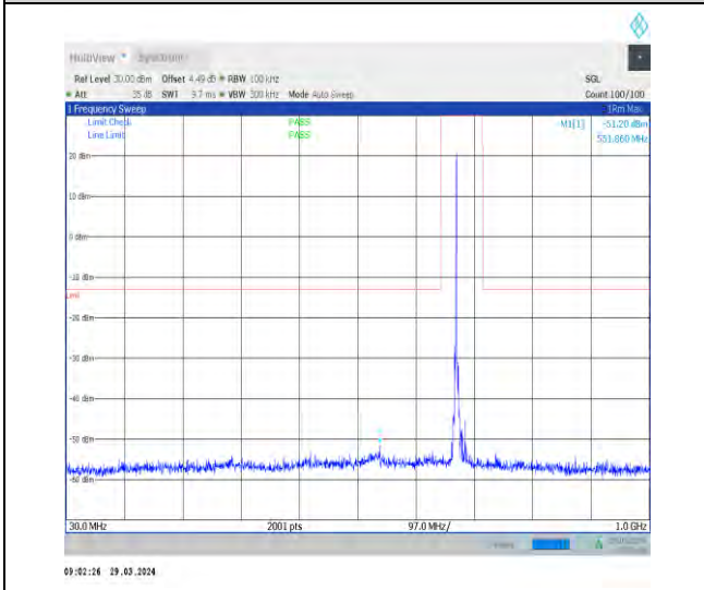
1-N71-15-20-H-1-DFT-PI2BPSK-Inner_1RB_Left-1 @1-30-1000-Ant1-551.86--51.20--13-PASS
