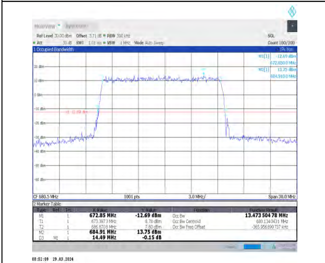
1-N71-15-15-M-5-DFT-256QAM-Outer_Full-75@0-A nt1-13.474-14.490-≤15-PASS
