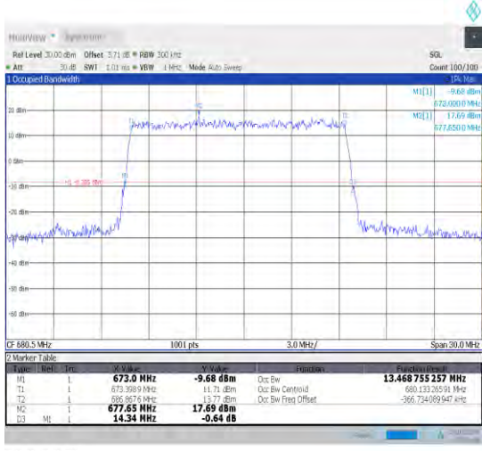
1-N71-15-15-M-1-DFT-QPSK-Outer_Full-75@0-Ant1 -13.469-14.340-≤15-PASS
