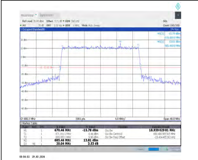
1-N71-15-20-M-8-CP-64QAM-Outer_Full-106@0-Ant1 1-18.939-20.040-≤20-PASS
