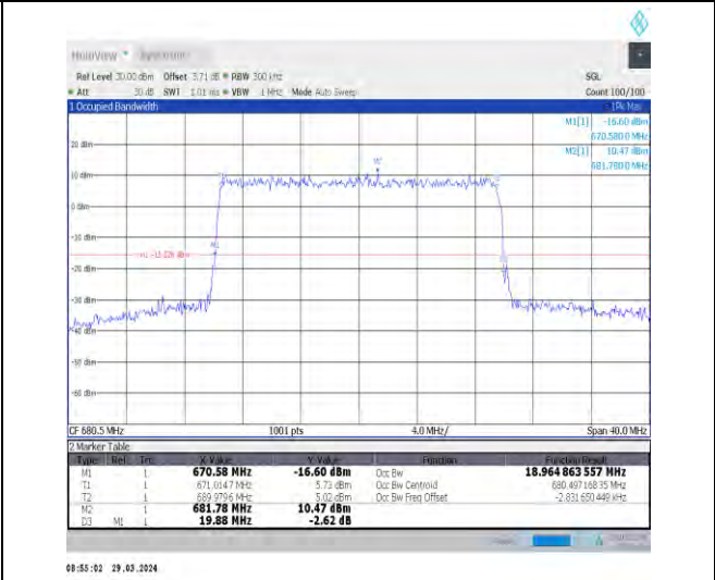
1-N71-15-20-M-9-CP-256QAM-Outer_Full-106@0-Ant1 nt1-18.965-19.880-≤20-PASS
