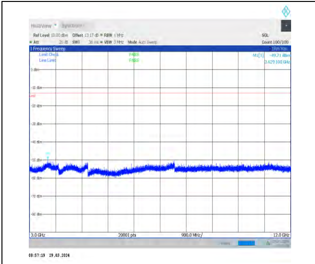
1-N71-15-20-L-1-DFT-PI2BPSK-Inner_1RB_Left-1 @ 1-3000-12000-Ant1-3629.10--49.71--13-PASS
