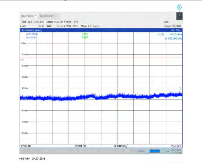
1-N71-15-20-L-1-DFT-PI2BPSK-Inner_1RB_Left-1 @ 1-12000-20000-Ant1-19895.60--42.65--13-PASS
