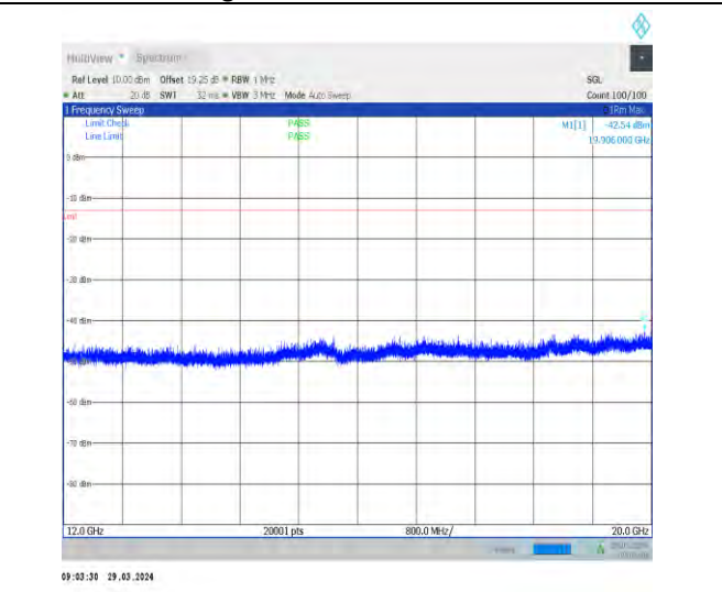
1-N71-15-20-H-1-DFT-PI2BPSK-Inner_1RB_Left-1@ 1-12000-20000-Ant1-19906.00--42.54--13-PASS
