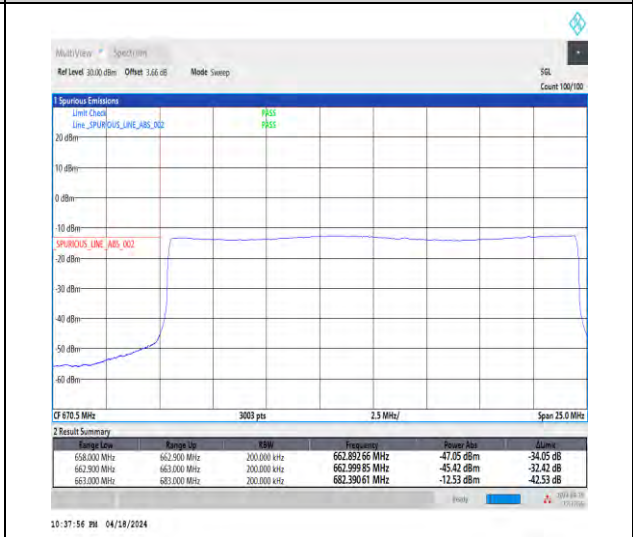
1-N71-15-20-L-6-CP-QPSK-Outer_Full-106@0-Ant1-1--PASS-see graph
