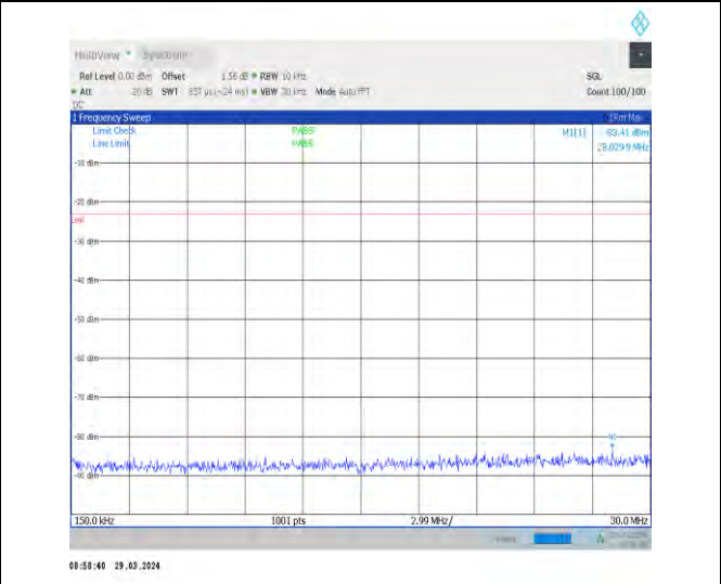
1-N71-15-20-M-1-DFT-PI2BPSK-Inner_1RB_Left-1 @ 1-0.15-30-Ant1-28.03--83.41--23-PASS
