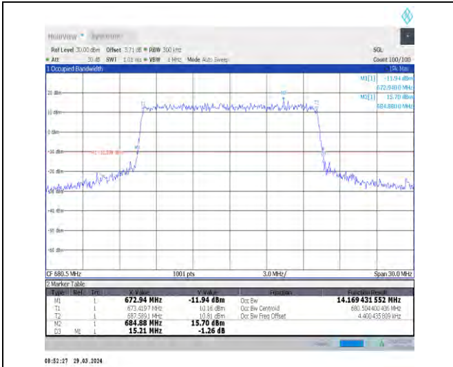
1-N71-15-15-M-7-CP-16QAM-Outer_Full-79@0-Ant1 -14.169-15.210-≤15-PASS
