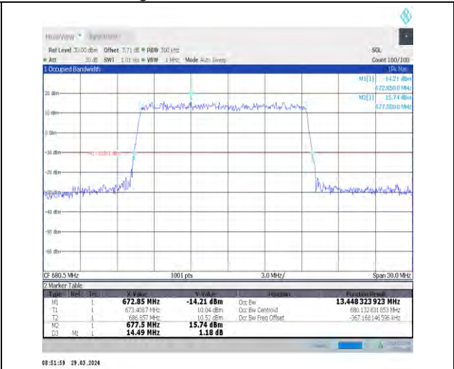
1-N71-15-15-M-4-DFT-64QAM-Outer_Full-75@0-Ant 1-13.448-14.490-≤15-PASS
