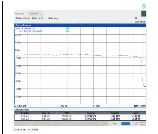
1-N66-15-40-H-3-DFT-PI2BPSK-Outer_Full-216@0-Ant1-1-seegraph-PASS-see graph
