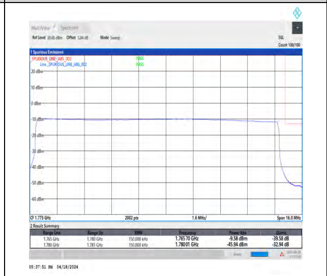
1-N66-15-15-H-6-CP-QPSK-Outer_Full-79@0-Ant1-1-seegraph-PASS-see graph
