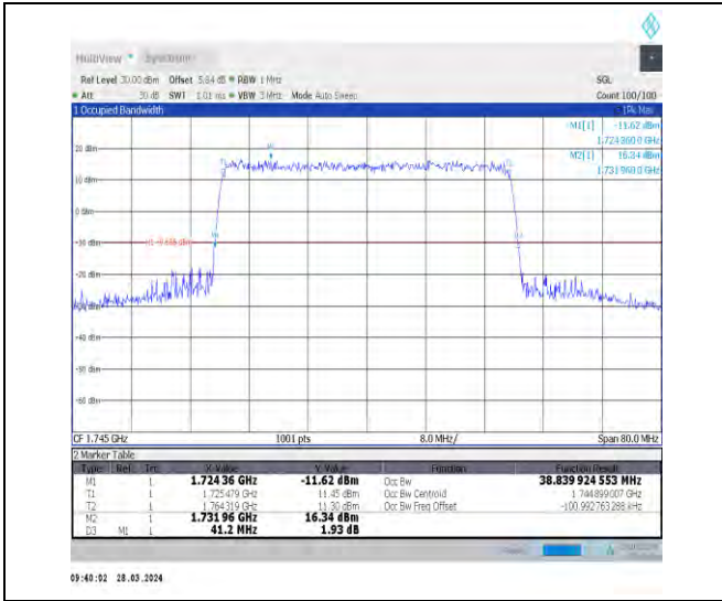
1-N66-15-40-M-3-DFT-16QAM-Outer_Full-216@0-A nt1-38.84-41.200-≤40-PASS
