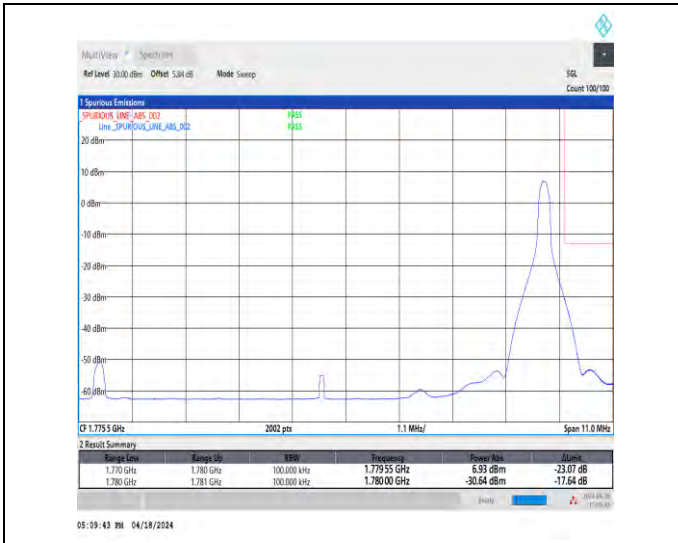
1-N66-15-10-H-2-DFT-PI2BPSK-Edge_1RB_Right-1@51-Ant1-1-seegraph-PASS-see graph
