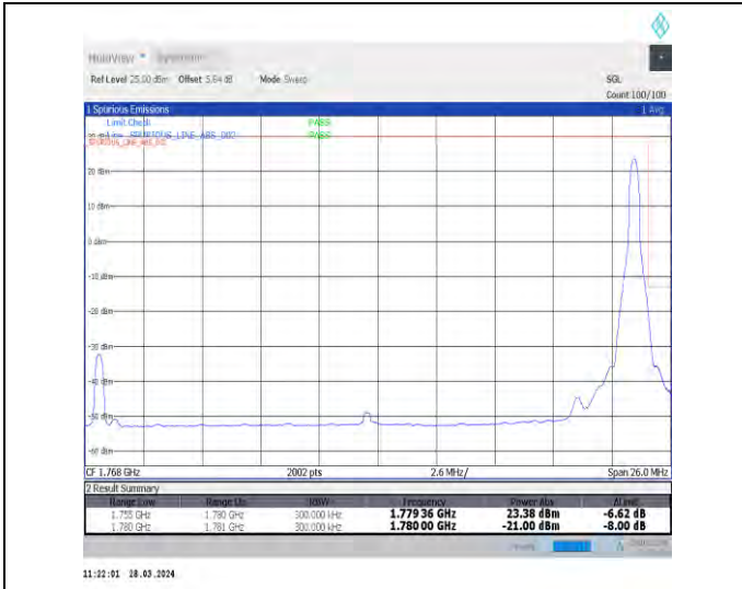
1-N66-15-25-H-2-DFT-PI2BPSK-Edge_1RB_Right-1@132-Ant1-1-seegraph-PASS-see graph
