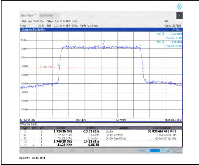
1-N66-15-40-M-5-DFT-256QAM-Outer_Full-216@0-A nt1-38.83-41.280-≤40-PASS
