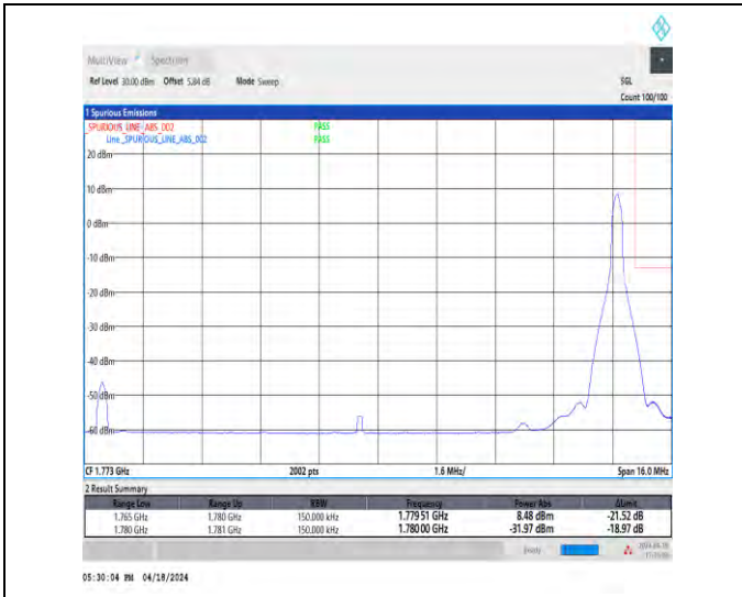
1-N66-15-15-H-2-DFT-PI2BPSK-Edge_1RB_Right-1@78-Ant1-1-seegraph-PASS-see graph
