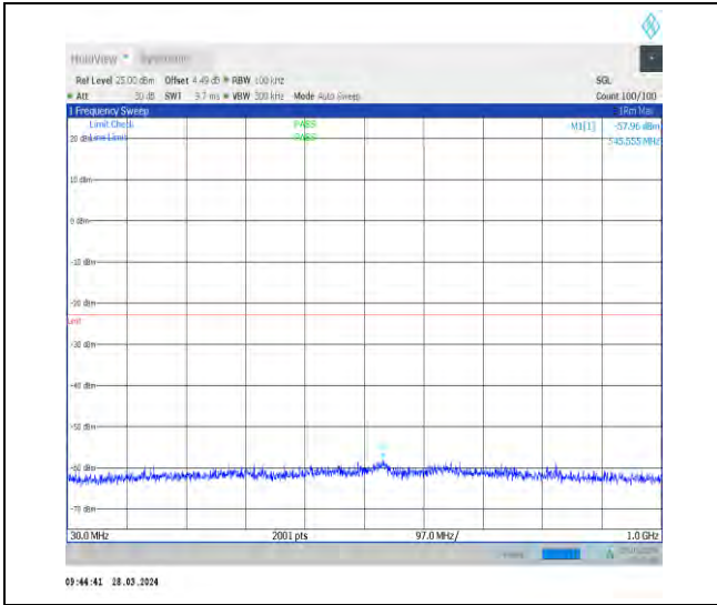
1-N66-15-40-M-1-DFT-PI2BPSK-Inner_1RB_Left-1 @ 1-30-1000-Ant1-545.56--57.96--23-PASS
