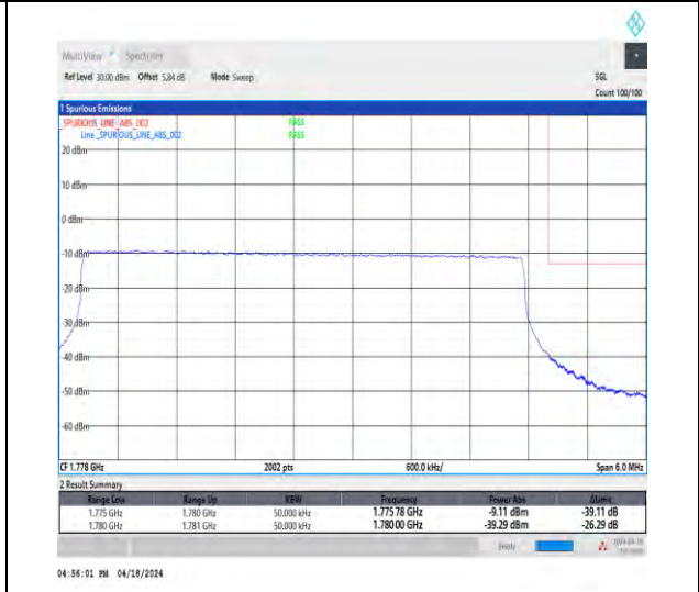
1-N66-15-5-H-6-CP-QPSK-Outer_Full-25@0-Ant1-1-seegraph-PASS-see graph
