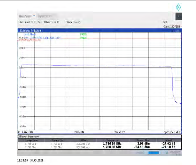
1-N66-15-25-H-6-CP-QPSK-Outer_Full-133@0-Ant1-1-seegraph-PASS-see graph
