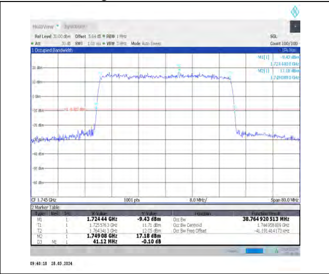
1-N66-15-40-M-4-DFT-64QAM-Outer_Full-216@0-A nt1-38.765-41.120-≤40-PASS
