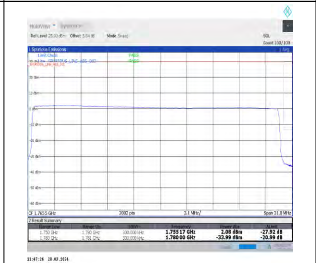
1-N66-15-30-H-6-CP-QPSK-Outer_Full-160@0-Ant1-1-seegraph-PASS-see graph
