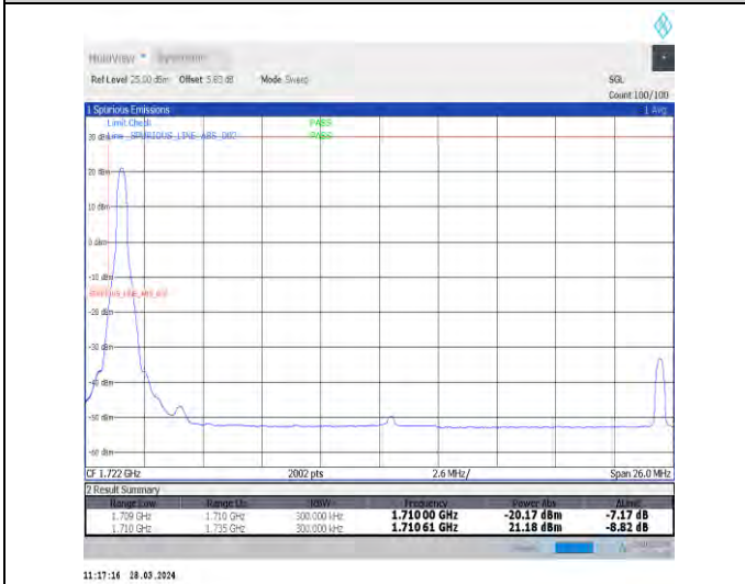
1-N66-15-25-L-4-CP-QPSK-Edge_1RB_Left-1@0-Ant1-1-seegraph-PASS-see graph
