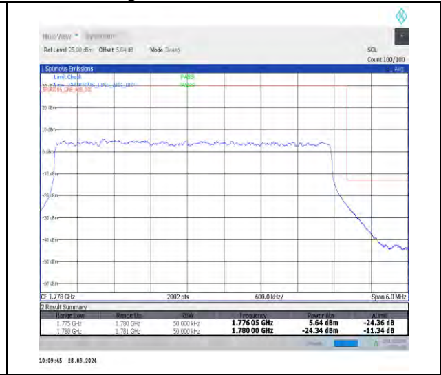
1-N66-15-5-H-3-DFT-PI2BPSK-Outer_Full-25@0-Ant1-1-seegraph-PASS-see graph
