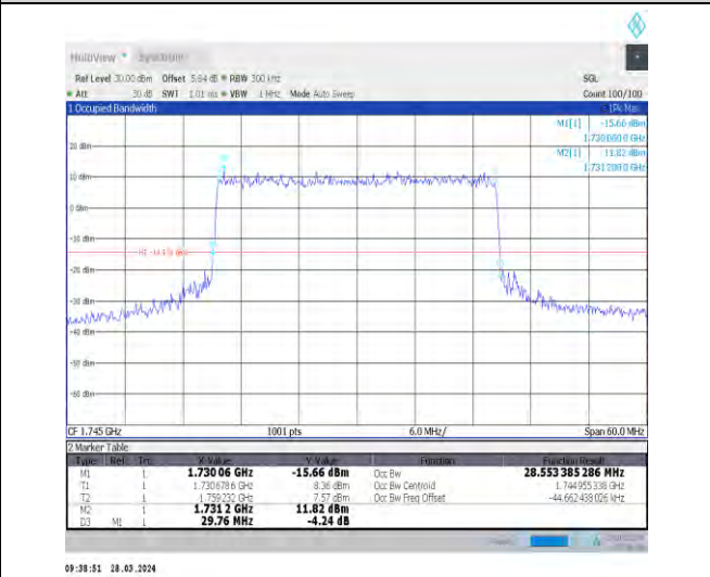
1-N66-15-30-M-7-CP-16QAM-Outer_Full-160@0-Ant1-28.554-29.760-≤30-PASS
