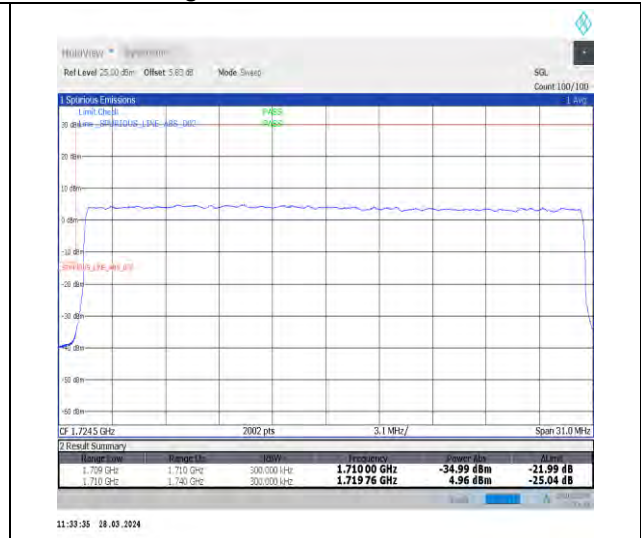
1-N66-15-30-L-3-DFT-PI2BPSK-Outer_Full-160@0-Ant1-1-seegraph-PASS-see graph
