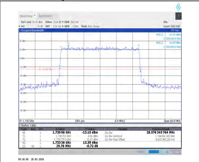
1-N66-15-30-M-1-DFT-QPSK-Outer_Full-160@0-Ant 1-28.577-29.760-≤30-PASS
