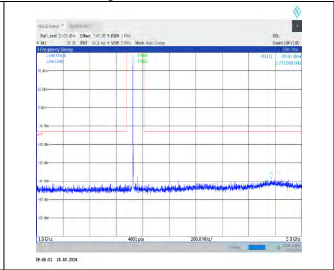
1-N66-15-40-M-1-DFT-PI2BPSK-Inner_1RB_Left-1 @ 1-1000-3000-Ant1-2771.00--39.01--13-PASS
