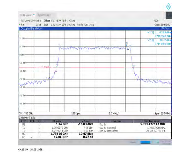
1-N66-15-10-M-8-CP-64QAM-Outer_Full-52@0-Ant1 -9.283-10.060-≤10-PASS
