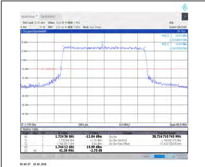
1-N66-15-40-M-7-CP-16QAM-Outer_Full-216@0-Ant 1-38.717-41.360-≤40-PASS
