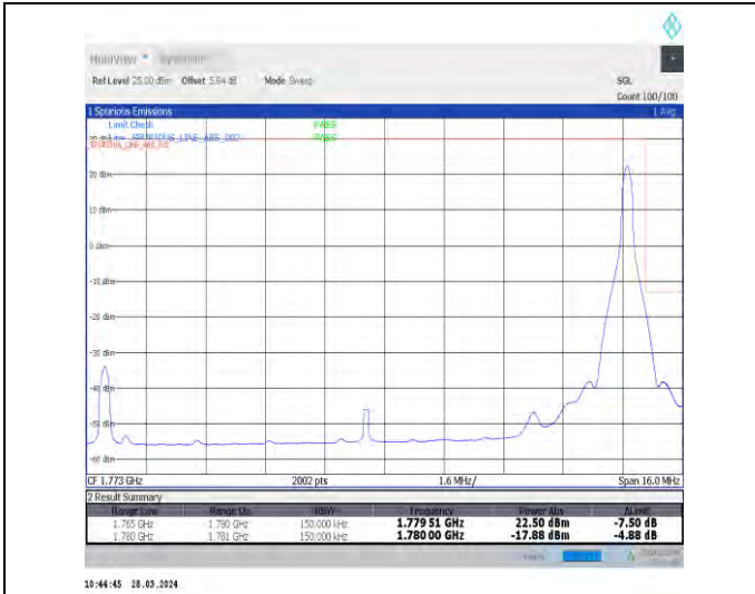
1-N66-15-15-H-2-DFT-PI2BPSK-Edge_1RB_Right-1@78-Ant1-1-seegraph-PASS-see graph
