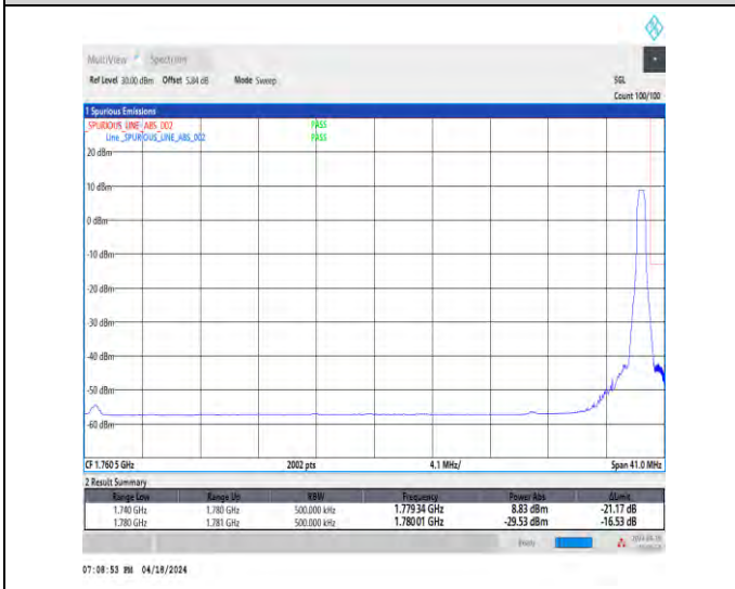
1-N66-15-40-H-5-CP-QPSK-Edge_1RB_Right-1@215-Ant1-1-seegraph-PASS-see graph
