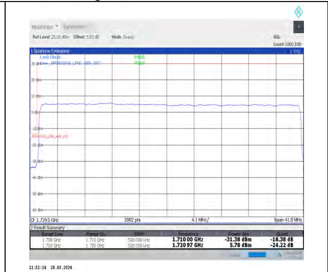
1-N66-15-40-L-3-DFT-PI2BPSK-Outer_Full-216@0-Ant1-1-seegraph-PASS-see graph
