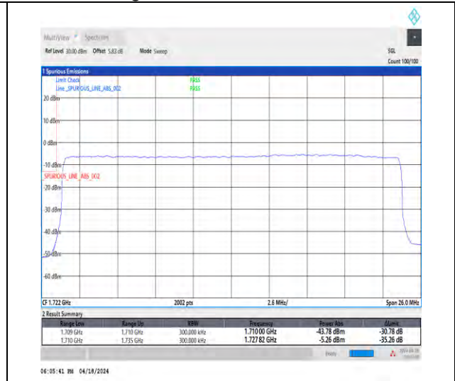
1-N66-15-25-L-3-DFT-PI2BPSK-Outer_Full-128@0-Ant1-1-seegraph-PASS-see graph
