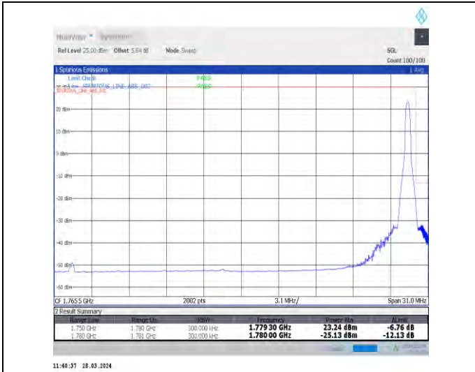
1-N66-15-30-H-2-DFT-PI2BPSK-Edge_1RB_Right-1@159-Ant1-1-seegraph-PASS-see graph
