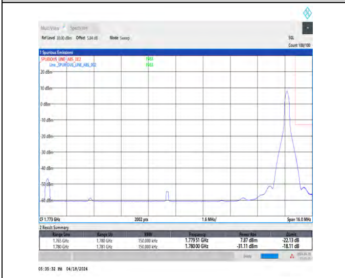
1-N66-15-15-H-5-CP-QPSK-Edge_1RB_Right-1@78-Ant1-1-seegraph-PASS-see graph
