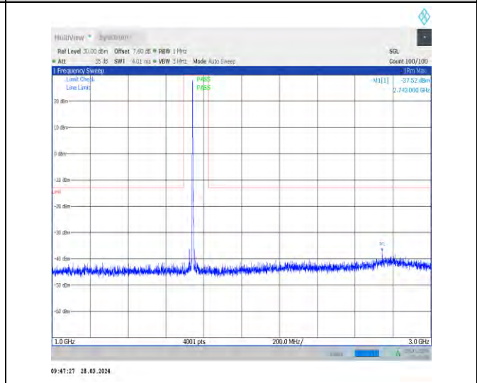
1-N66-15-40-H-1-DFT-PI2BPSK-Inner_1RB_Left-1 @ 1-1000-3000-Ant1-2743.00--37.52--13-PASS
