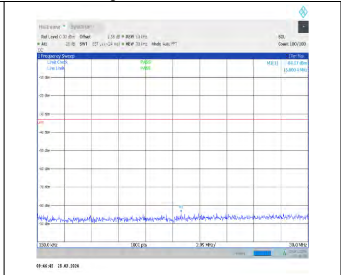
1-N66-15-40-H-1-DFT-PI2BPSK-Inner_1RB_Left-1 @ 1-0.15-30-Ant1-16.00--84.17--33-PASS
