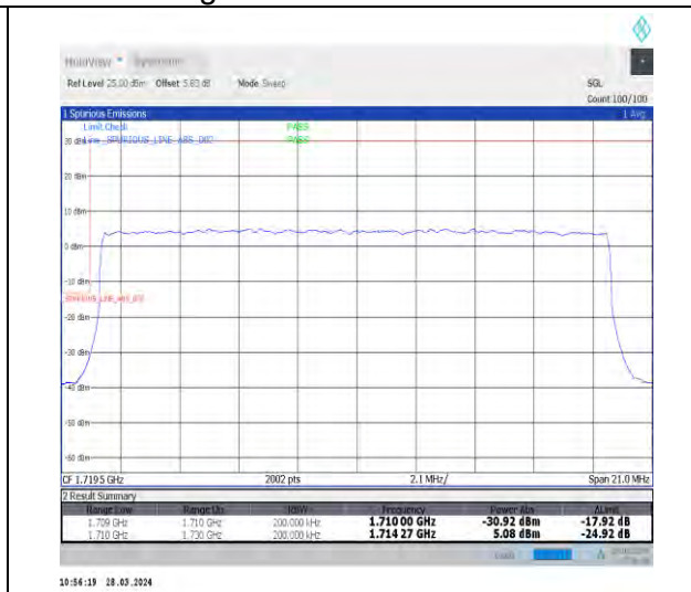
1-N66-15-20-L-3-DFT-PI2BPSK-Outer_Full-100@0-Ant1-1-seegraph-PASS-see graph
