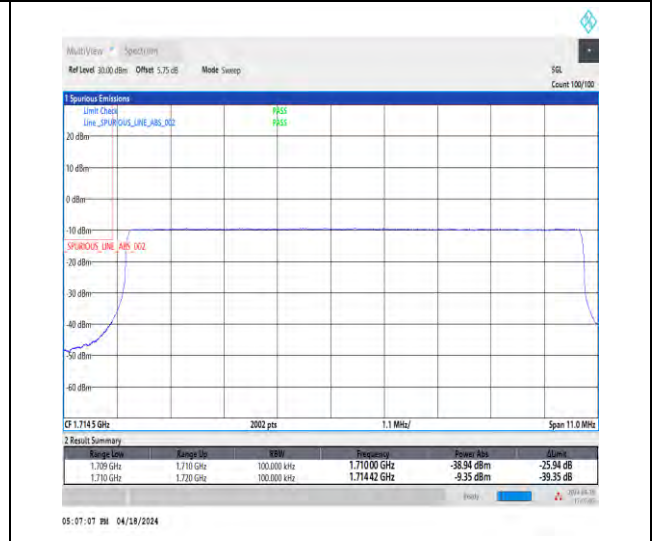
1-N66-15-10-L-6-CP-QPSK-Outer_Full-52@0-Ant1 -1-seegraph-PASS-see graph
