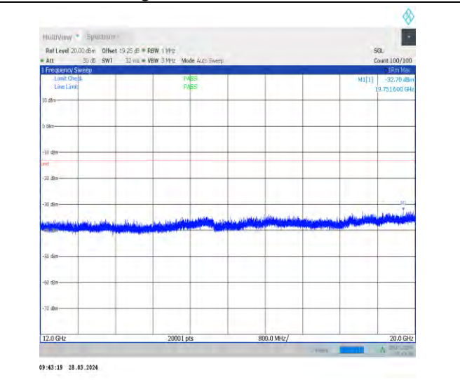
1-N66-15-40-L-1-DFT-PI2BPSK-Inner_1RB_Left-1@ 1-12000-20000-Ant1-19751.60--32.70--13-PASS
