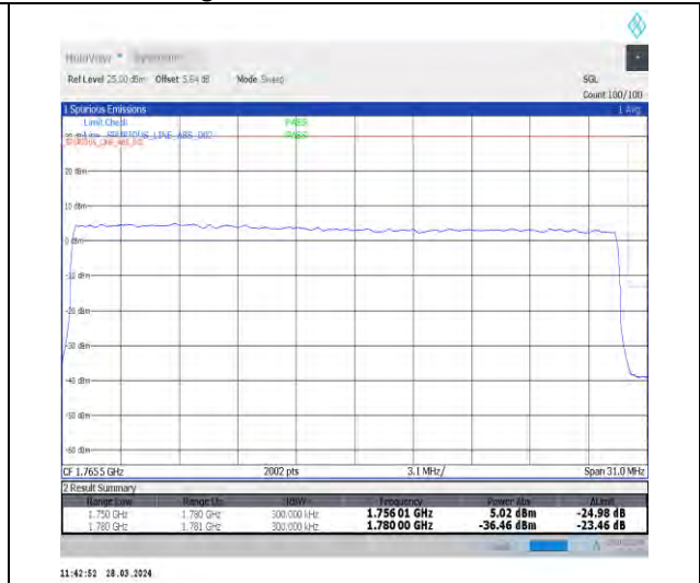
1-N66-15-30-H-3-DFT-PI2BPSK-Outer_Full-160@0-Ant1-1-seegraph-PASS-see graph
