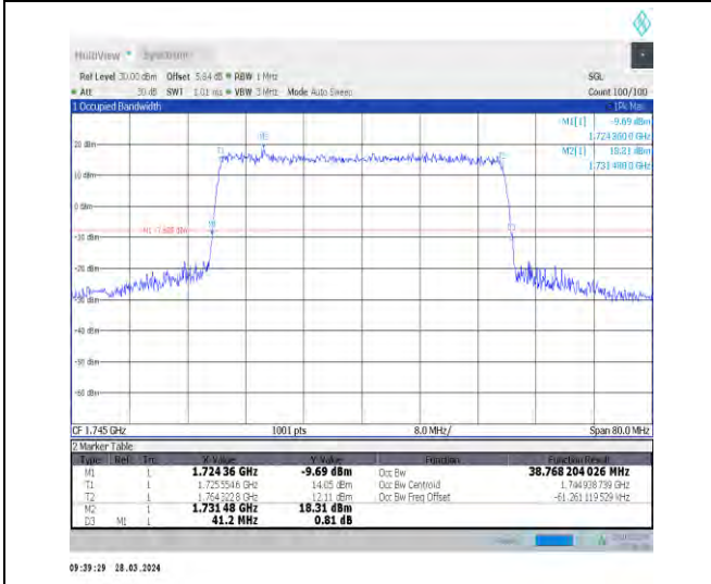
1-N66-15-40-M-1-DFT-QPSK-Outer_Full-216@0-Ant 1-38.768-41.200-≤40-PASS
