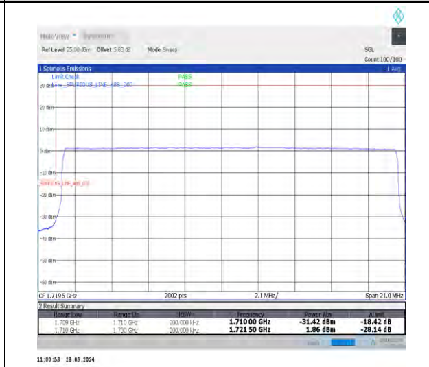
1-N66-15-20-L-6-CP-QPSK-Outer_Full-106@0-Ant1-1-seegraph-PASS-see graph
