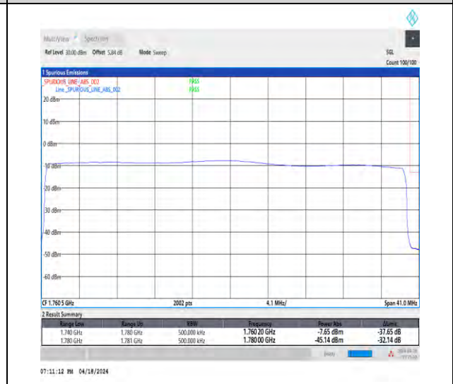
1-N66-15-40-H-6-CP-QPSK-Outer_Full-216@0-Ant1-1-seegraph-PASS-see graph
