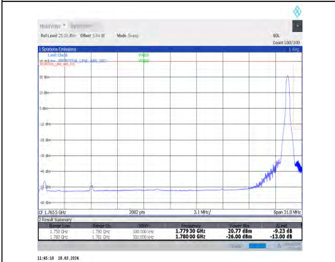
1-N66-15-30-H-5-CP-QPSK-Edge_1RB_Right-1@159-Ant1-1-seegraph-PASS-see graph
