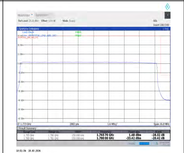
1-N66-15-15-H-6-CP-QPSK-Outer_Full-79@0-Ant1-1-seegraph-PASS-see graph
