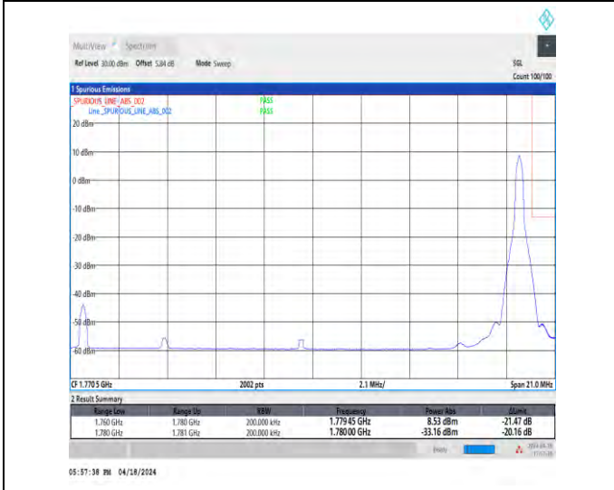
1-N66-15-20-H-5-CP-QPSK-Edge_1RB_Right-1@105-Ant1-1-seegraph-PASS-see graph
