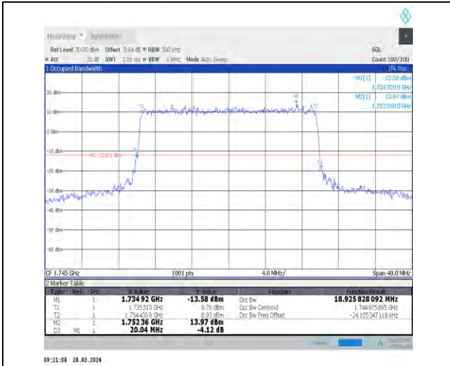
1-N66-15-20-M-6-CP-QPSK-Outer_Full-106@0-Ant1 -18.926-20.040-≤20-PASS
