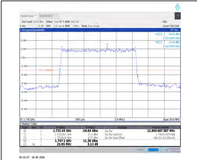
1-N66-15-25-M-5-DFT-256QAM-Outer_Full-128@0-Ant1-22.906-23.950-≤25-PASS
