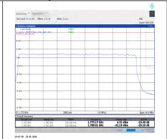
1-N66-15-15-H-3-DFT-PI2BPSK-Outer_Full-75@0-Ant1-1-seegraph-PASS-see graph
