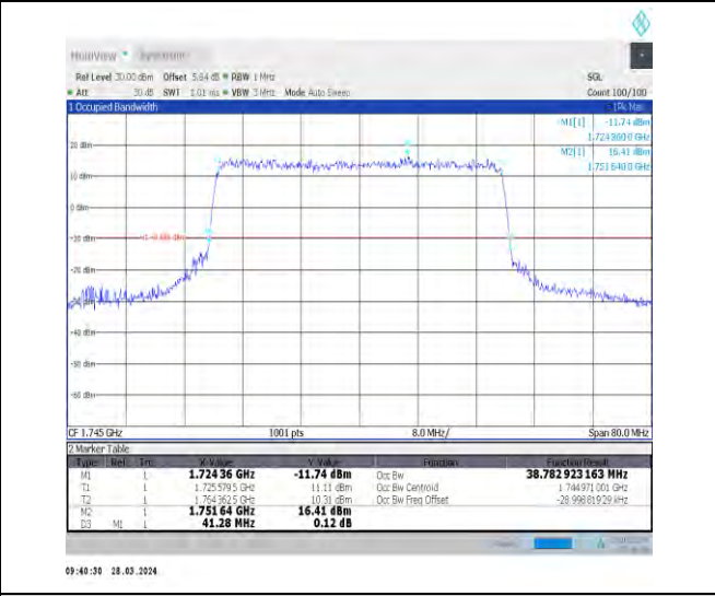
1-N66-15-40-M-6-CP-QPSK-Outer_Full-216@0-A nt1-38.783-41.280-≤40-PASS
