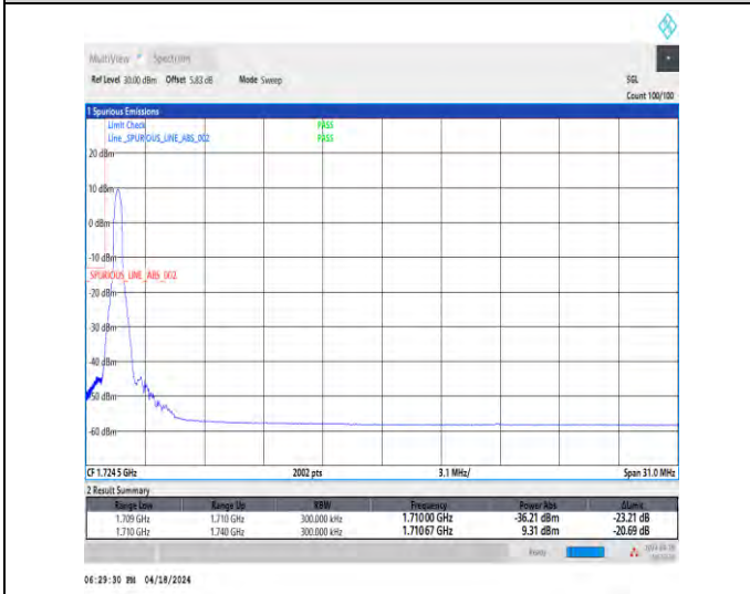
1-N66-15-30-L-4-CP-QPSK-Edge_1RB_Left-1@0-Ant1-1-seegraph-PASS-see graph
