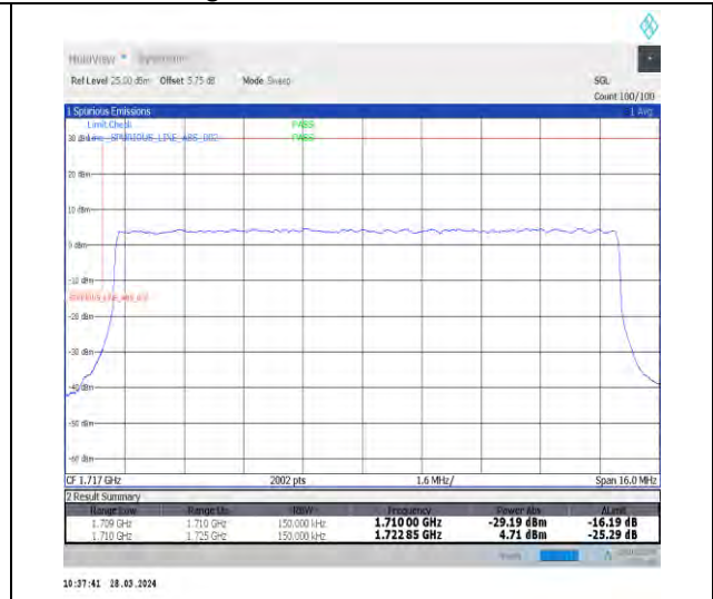
1-N66-15-15-L-3-DFT-PI2BPSK-Outer_Full-75@0-Ant1-1-see graph-PASS-see graph
