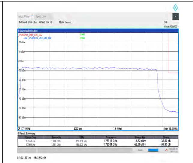
1-N66-15-15-H-3-DFT-PI2BPSK-Outer_Full-75@0-Ant1-1-seegraph-PASS-see graph
