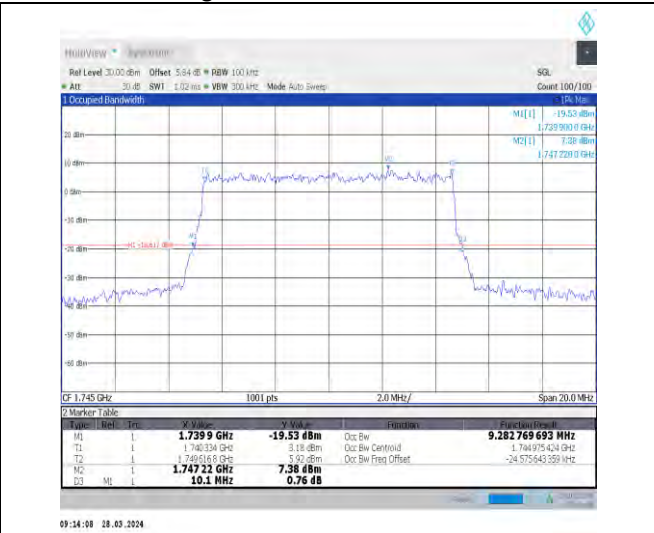
1-N66-15-10-M-9-CP-256QAM-Outer_Full-52@0-Ant1 1-9.283-10.100-≤10-PASS
