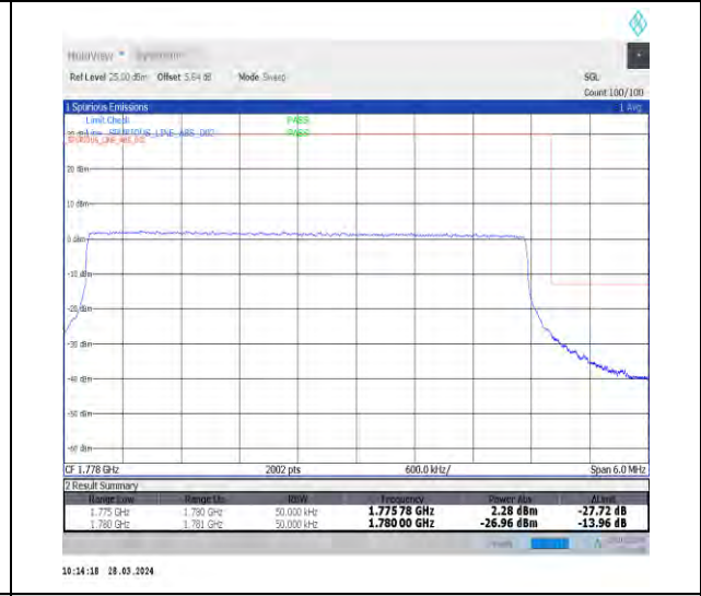
1-N66-15-5-H-6-CP-QPSK-Outer_Full-25@0-Ant1-1-seegraph-PASS-see graph
