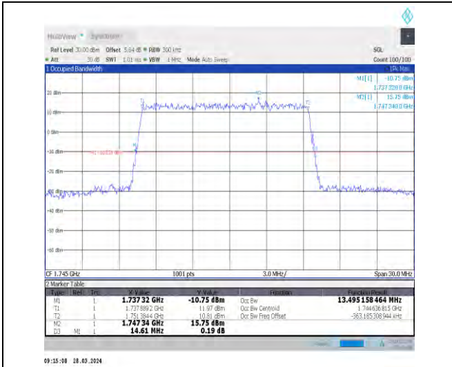
1-N66-15-15-M-3-DFT-16QAM-Outer_Full-75@0-Ant 1-13.495-14.610-≤15-PASS
