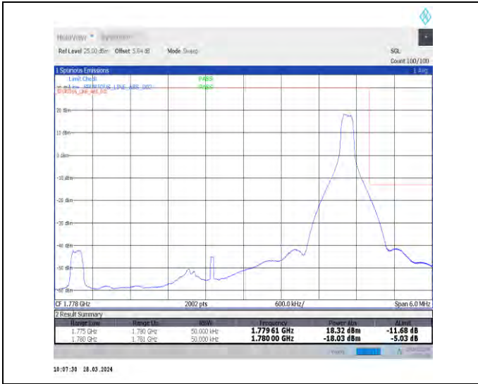
1-N66-15-5-H-2-DFT-PI2BPSK-Edge_1RB_Right-1@2-4-Ant1-1-seegraph-PASS-see graph
