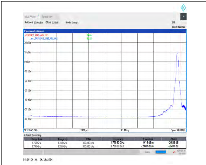
1-N66-15-30-H-2-DFT-PI2BPSK-Edge_1RB_Right-1@159-Ant1-1-seegraph-PASS-see graph
