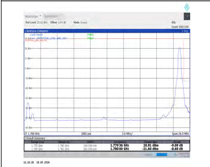
1-N66-15-25-H-5-CP-QPSK-Edge_1RB_Right-1@132-Ant1-1-seegraph-PASS-see graph
