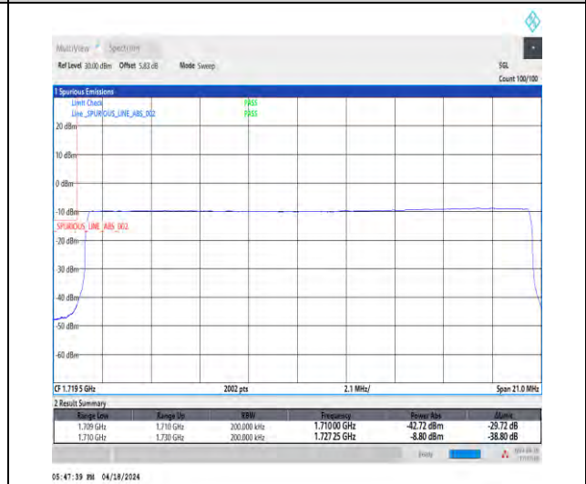
1-N66-15-20-L-6-CP-QPSK-Outer_Full-106@0-Ant1-1-seegraph-PASS-see graph
