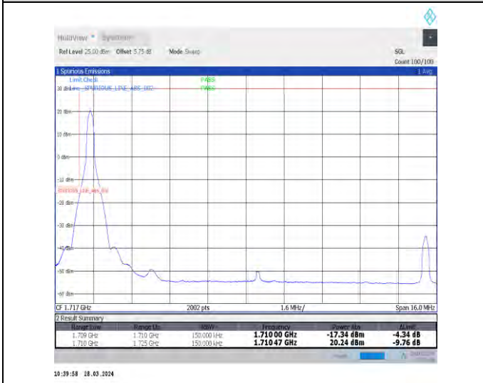
1-N66-15-15-L-4-CP-QPSK-Edge_1RB_Left-1@0-Ant1-1-see graph-PASS-see graph
