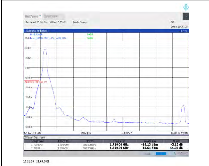
1-N66-15-10-L-4-CP-QPSK-Edge_1RB_Left-1@0-Ant1-1-seegraph-PASS-see graph
