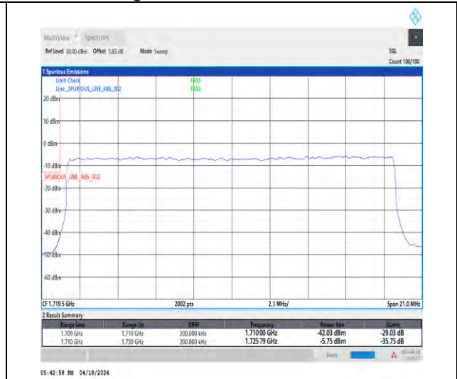
1-N66-15-20-L-3-DFT-PI2BPSK-Outer_Full-100@0-Ant1-1-seegraph-PASS-see graph
