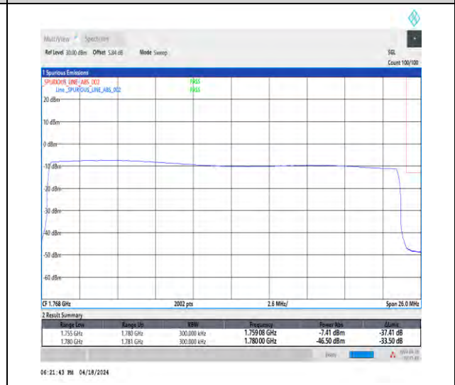
1-N66-15-25-H-6-CP-QPSK-Outer_Full-133@0-Ant1-1-seegraph-PASS-see graph
