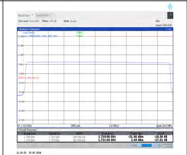
1-N66-15-25-L-6-CP-QPSK-Outer_Full-133@0-Ant1-1-seegraph-PASS-see graph
