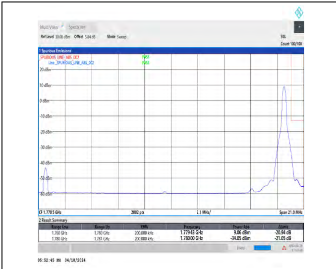
1-N66-15-20-H-2-DFT-PI2BPSK-Edge_1RB_Right-1@105-Ant1-1-seegraph-PASS-see graph
