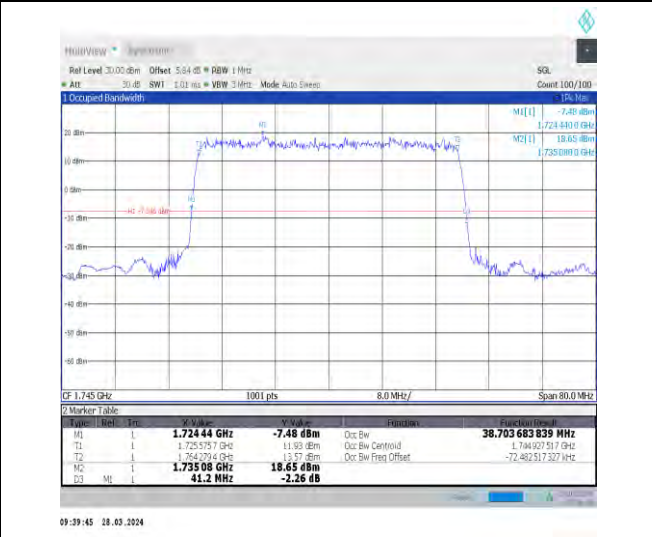
1-N66-15-40-M-2-DFT-PI2BPSK-Outer_Full-216@0-Ant 1-38.704-41.200-≤40-PASS
