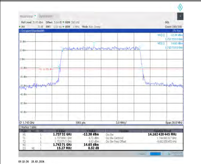
1-N66-15-15-M-6-CP-QPSK-Outer_Full-79@0-Ant1 14.162-15.270-≤15-PASS
