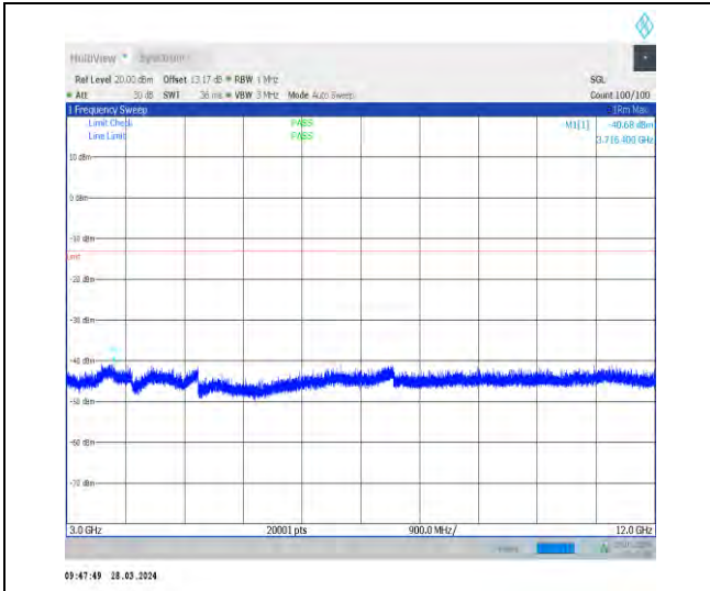
1-N66-15-40-H-1-DFT-PI2BPSK-Inner_1RB_Left-1 @1-3000-12000-Ant1-3716.40--40.68--13-PASS
