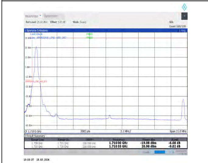
1-N66-15-20-L-4-CP-QPSK-Edge_1RB_Left-1@0-Ant1-1-seegraph-PASS-see graph
