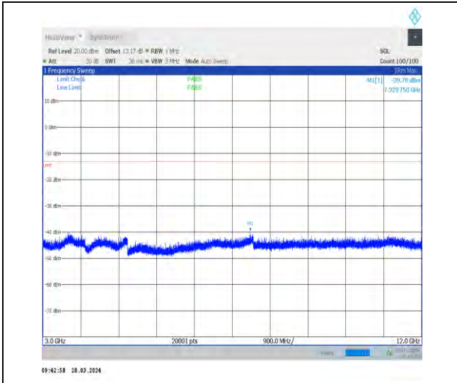
1-N66-15-40-L-1-DFT-PI2BPSK-Inner_1RB_Left-1 @1-3000-12000-Ant1-7929.75--39.78--13-PASS
