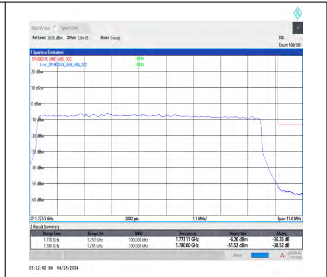
1-N66-15-10-H-3-DFT-PI2BPSK-Outer_Full-50@0-Ant1-1-seegraph-PASS-see graph
