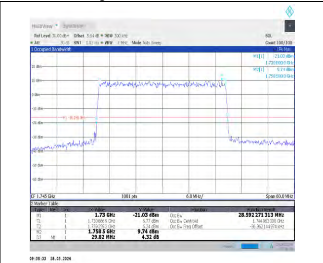
1-N66-15-30-M-5-DFT-256QAM-Outer_Full-160@0-Ant1-28.595-29.820-≤30-PASS
