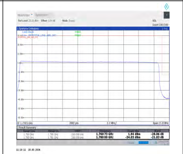
1-N66-15-20-H-6-CP-QPSK-Outer_Full-106@0-Ant1-1-seegraph-PASS-see graph
