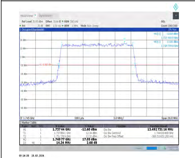
1-N66-15-15-M-1-DFT-QPSK-Outer_Full-75@0-Ant1 -13.493-14.340-≤15-PASS
