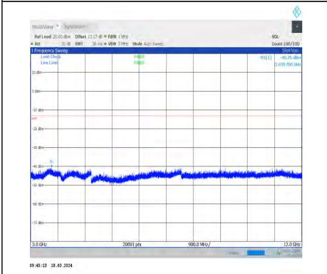
1-N66-15-40-M-1-DFT-PI2BPSK-Inner_1RB_Left-1 @ 1-3000-12000-Ant1-3695.70--40.76--13-PASS
