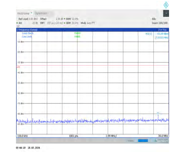
1-N66-15-40-M-1-DFT-PI2BPSK-Inner_1RB_Left-1@ 1-0.15-30-Ant1-27.91--82.50--33-PASS
