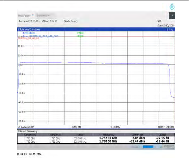
1-N66-15-40-H-6-CP-QPSK-Outer_Full-216@0-Ant1-1-seegraph-PASS-see graph
