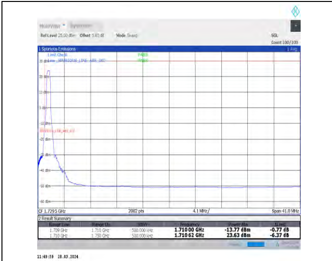
1-N66-15-40-L-1-DFT-PI2BPSK-Edge_1RB_Left-1@0-Ant1-1-seegraph-PASS-see graph
