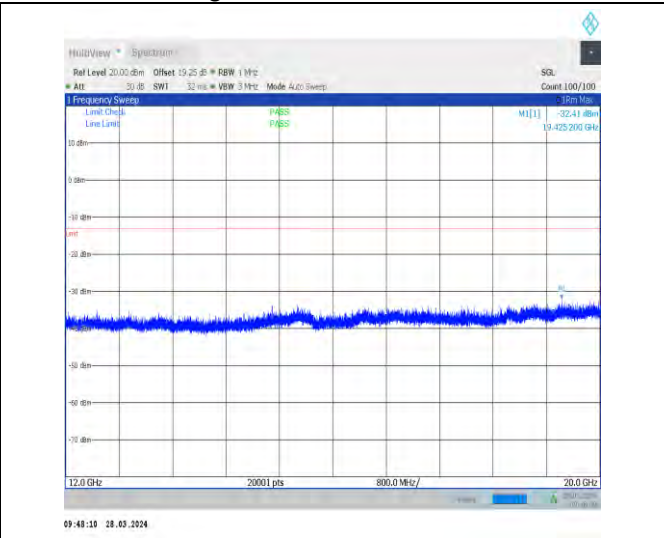
1-N66-15-40-H-1-DFT-PI2BPSK-Inner_1RB_Left-1@ 1-12000-20000-Ant1-19425.20--32.41--13-PASS
