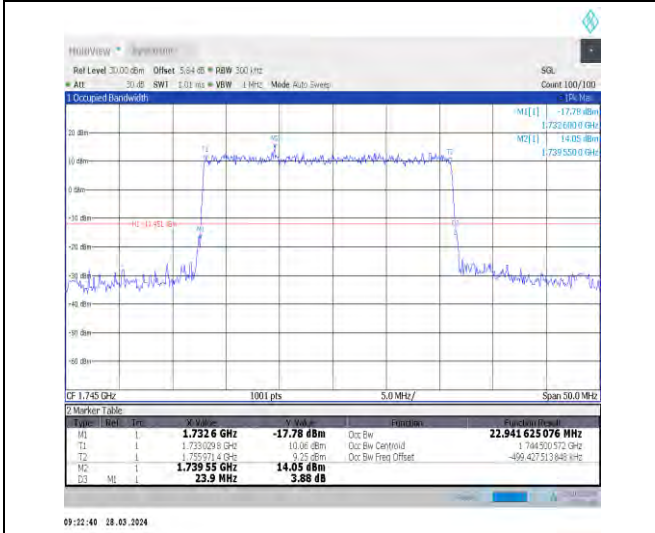
1-N66-15-25-M-3-DFT-16QAM-Outer_Full-128@0-Ant 1-22.942-23.900-≤25-PASS
