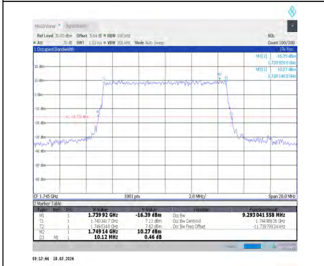
1-N66-15-10-M-6-CP-QPSK-Outer_Full-52@0-Ant1 9.293-10.120-≤10-PASS
