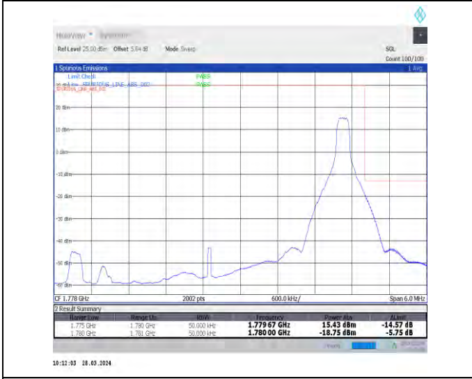
1-N66-15-5-H-5-CP-QPSK-Edge_1RB_Right-1@24-Ant1-1-seegraph-PASS-see graph
