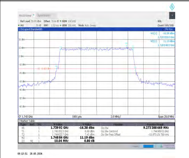
1-N66-15-10-M-7-CP-16QAM-Outer_Full-52@0-Ant1 -9.273-10.040-≤10-PASS
