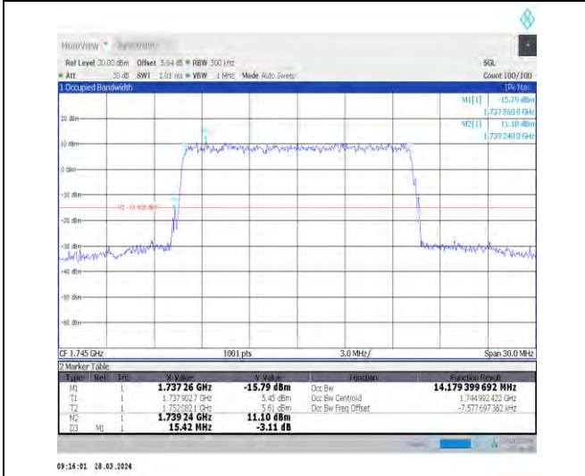
1-N66-15-15-M-9-CP-256QAM-Outer_Full-79@0-Ant 1-14.179-15.420-≤15-PASS
