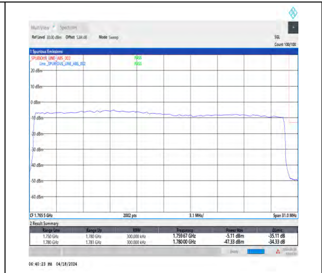
1-N66-15-30-H-3-DFT-PI2BPSK-Outer_Full-160@0-Ant1-1-seegraph-PASS-see graph
