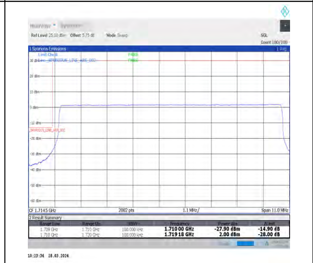
1-N66-15-10-L-6-CP-QPSK-Outer_Full-52@0-Ant1-1-seegraph-PASS-see graph
