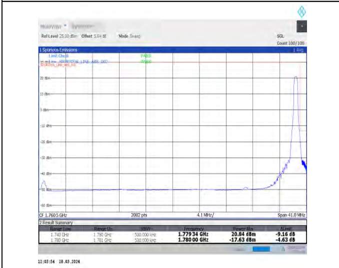
1-N66-15-40-H-5-CP-QPSK-Edge_1RB_Right-1@215-Ant1-1-seegraph-PASS-see graph
