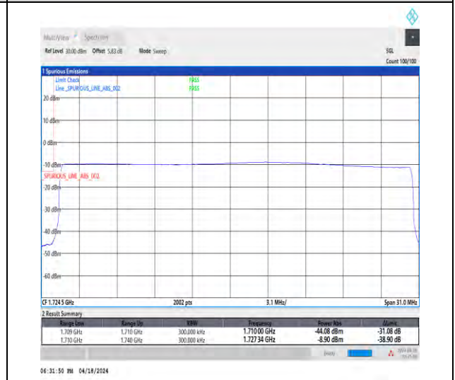
1-N66-15-30-L-6-CP-QPSK-Outer_Full-160@0-Ant1-1-seegraph-PASS-see graph
