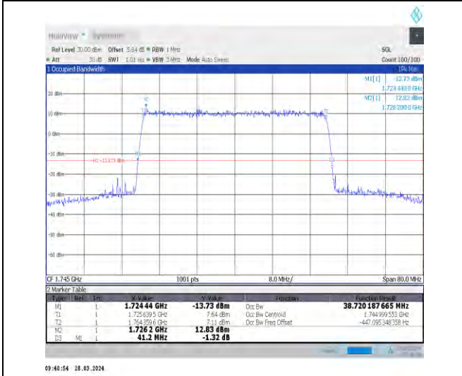
1-N66-15-40-M-9-CP-256QAM-Outer_Full-216@0-Ant nt1-38.72-41.200-≤40-PASS
