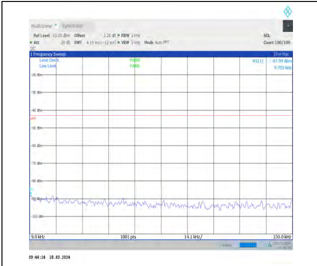
1-N66-15-40-H-1-DFT-PI2BPSK-Inner_1RB_Left-1 @ 1-0.009-0.15-Ant1-0.01--87.99--43-PASS
