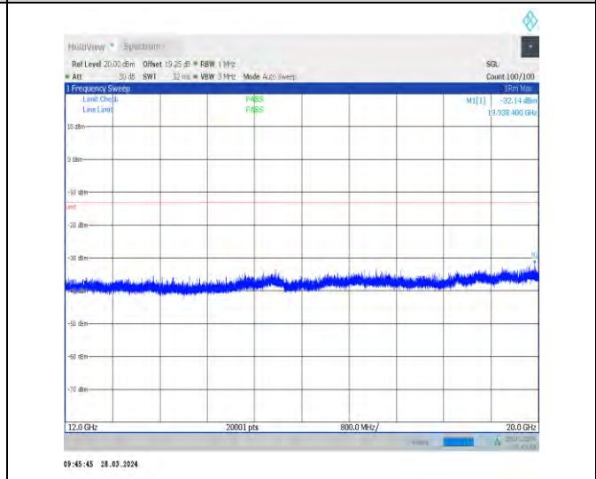
1-N66-15-40-M-1-DFT-PI2BPSK-Inner_1RB_Left-1 @ 1-12000-20000-Ant1-19938.40--32.14--13-PASS
