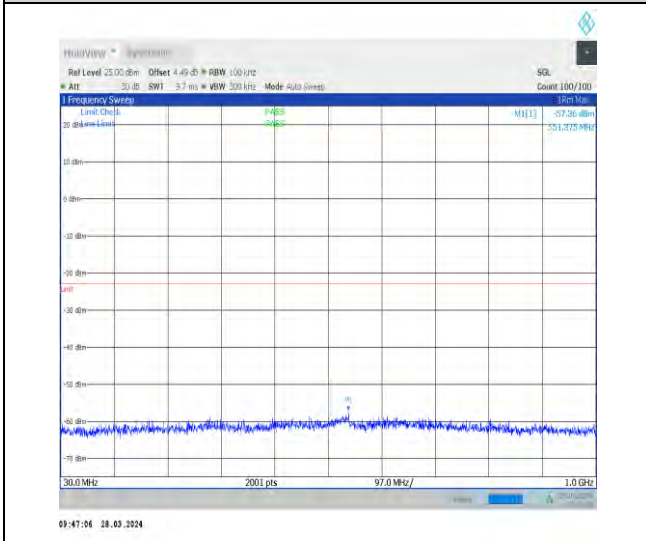
1-N66-15-40-H-1-DFT-PI2BPSK-Inner_1RB_Left-1 @ 1-30-1000-Ant1-551.38--57.36--23-PASS
