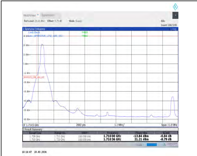
1-N66-15-10-L-1-DFT-PI2BPSK-Edge_1RB_Left-1@0-Ant1-1-seegraph-PASS-see graph
