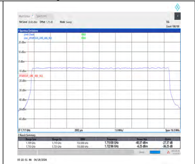
1-N66-15-15-L-3-DFT-PI2BPSK-Outer_Full-75@0-Ant1-1-seegraph-PASS-see graph
