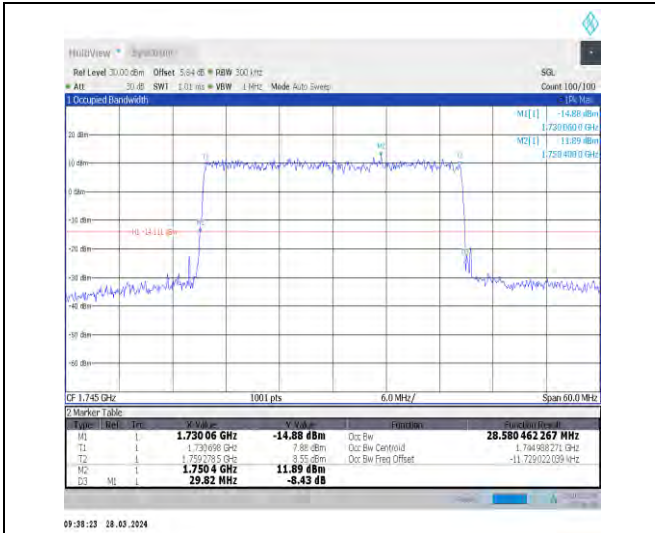
1-N66-15-30-M-4-DFT-64QAM-Outer_Full-160@0-Ant1-28.582-29.820-≤30-PASS
