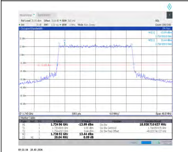
1-N66-15-20-M-8-CP-64QAM-Outer_Full-106@0-Ant1 1-18.939-20.040-≤20-PASS
