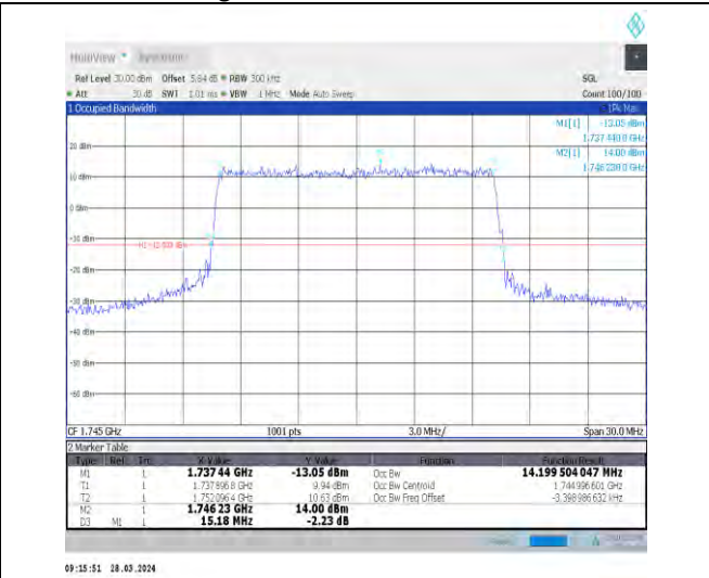
1-N66-15-15-M-8-CP-64QAM-Outer_Full-79@0-Ant1 -14.2-15.180-≤15-PASS
