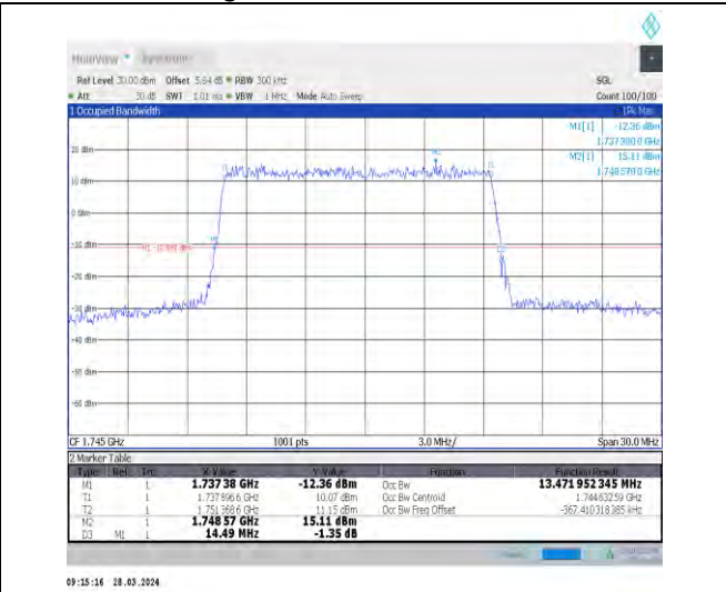
1-N66-15-15-M-4-DFT-64QAM-Outer_Full-75@0-Ant 1-13.472-14.490-≤15-PASS
