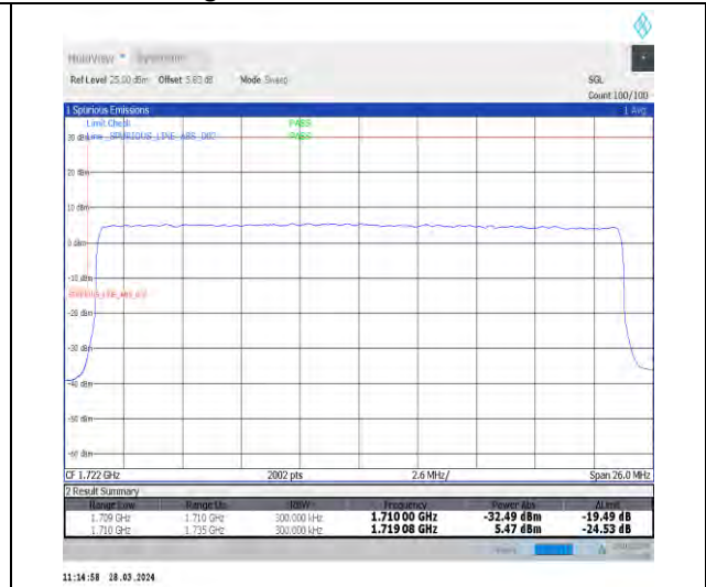
1-N66-15-25-L-3-DFT-PI2BPSK-Outer_Full-128@0-Ant1-1-seegraph-PASS-see graph
