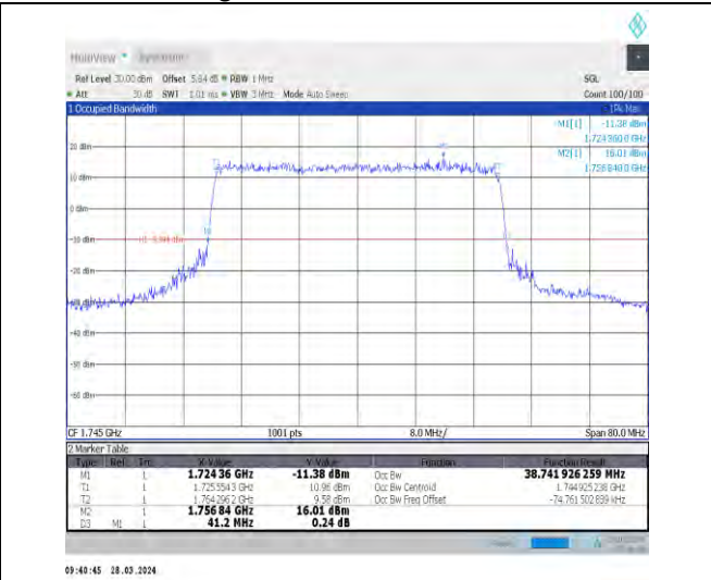
1-N66-15-40-M-8-CP-64QAM-Outer_Full-216@0-Ant 1-38.742-41.200-≤40-PASS
