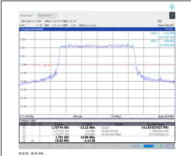
1-N66-15-15-M-7-CP-16QAM-Outer_Full-79@0-Ant1 -14.154-15.030-≤15-PASS
