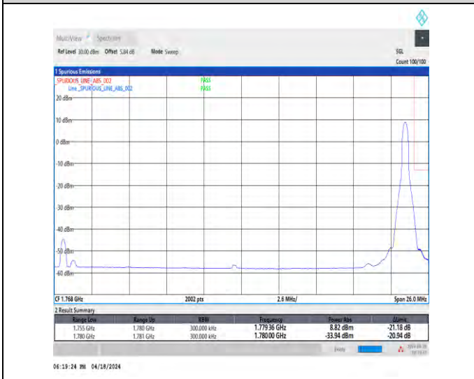
1-N66-15-25-H-5-CP-QPSK-Edge_1RB_Right-1@132-Ant1-1-seegraph-PASS-see graph
