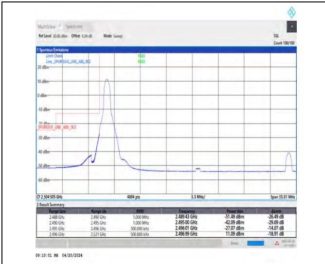
1-N41-30-25-L-1-DFT-PI2BPSK-Edge_1RB_Left-1@0-Ant1-1--PASS-see graph
