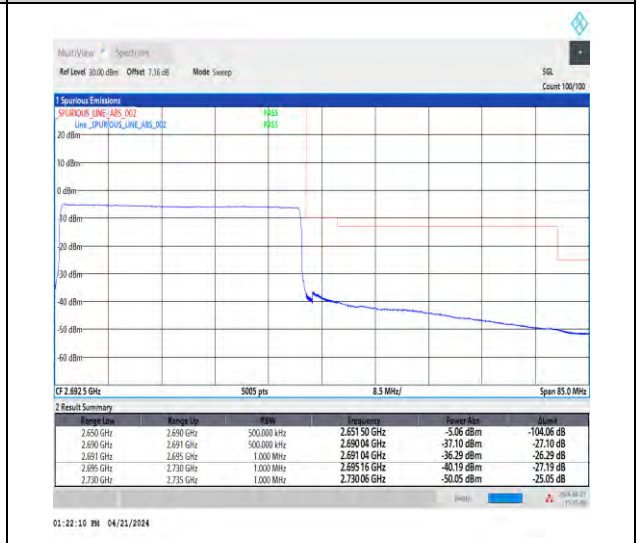
1-N41-30-40-H-6-CP-QPSK-Outer_Full-106@0-Ant1-1--PASS-see graph
