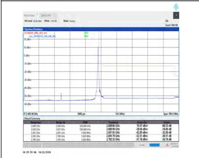
1-N41-30-90-H-5-CP-QPSK-Edge_1RB_Right-1@244-Ant1-1--PASS-see graph
