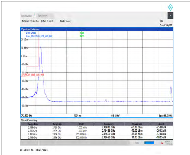
1-N41-30-60-L-1-DFT-PI2BPSK-Edge_1RB_Left-1@0-Ant1-1--PASS-see graph
