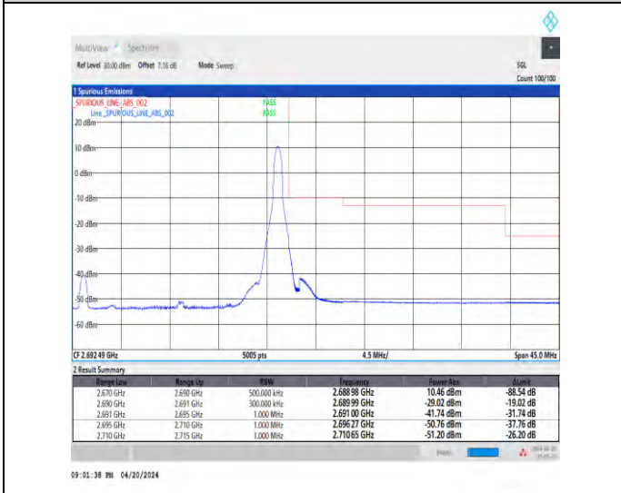
1-N41-30-20-H-5-CP-QPSK-Edge_1RB_Right-1@50-Ant1-1--PASS-see graph
