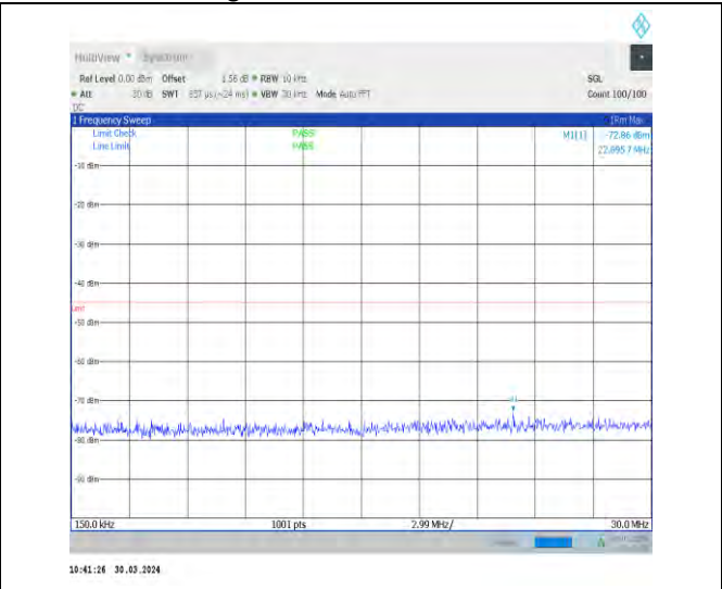
1-N41-30-100-H-1-DFT-PI2BPSK-Inner_1RB_Left-1 @1-0.15-30-Ant1-27.58--72.86--45-PASS
