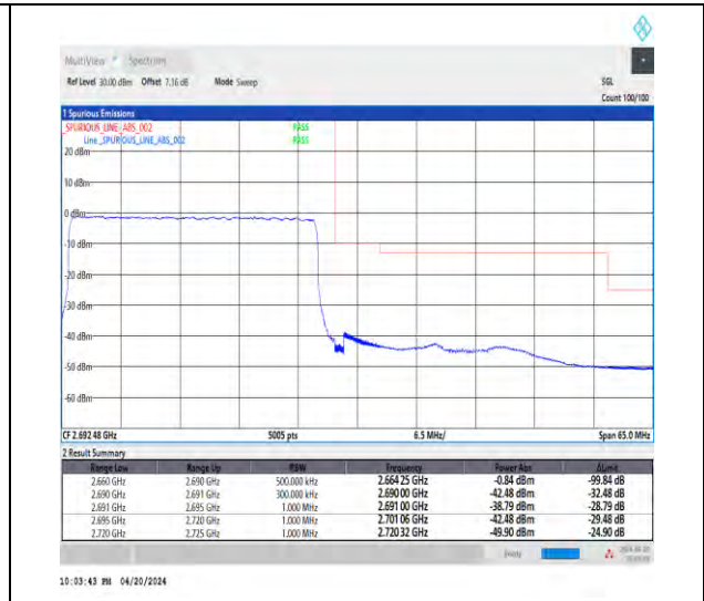
1-N41-30-30-H-3-DFT-PI2BPSK-Outer_Full-75@0-Ant1-1--PASS-see graph
