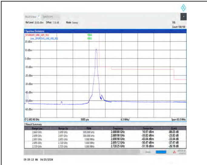
1-N41-30-30-H-2-DFT-PI2BPSK-Edge_1RB_Right-1@77-Ant1-1--PASS-see graph
