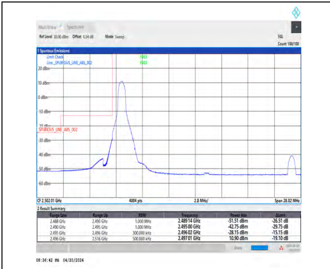
1-N41-30-20-L-1-DFT-PI2BPSK-Edge_1RB_Left-1@0-Ant1-1--PASS-see graph
