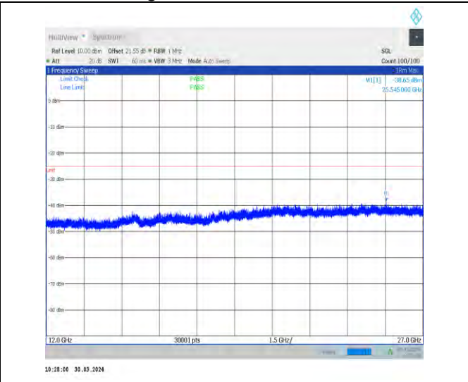
1-N41-30-100-L-1-DFT-PI2BPSK-Inner_1RB_Left-1 @1-12000-27000-Ant1-21117.50--38.65--25-PASS
