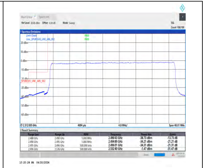
1-N41-30-40-L-3-DFT-PI2BPSK-Outer_Full-100@0-Ant1-1--PASS-see graph
