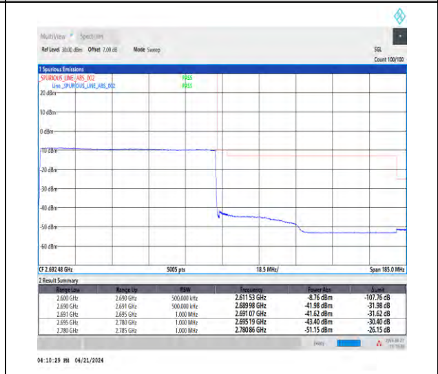
1-N41-30-90-H-6-CP-QPSK-Outer_Full-245@0-Ant1-1--PASS-see graph
