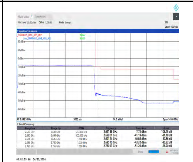
1-N41-30-70-H-6-CP-QPSK-Outer_Full-189@0-Ant1-1--PASS-see graph
