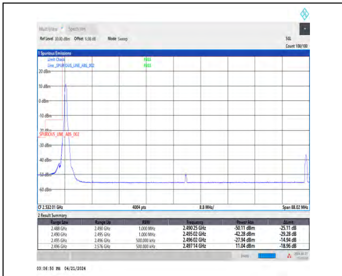
1-N41-30-80-L-1-DFT-PI2BPSK-Edge_1RB_Left-1@0-Ant1-1--PASS-see graph
