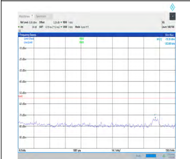
1-N41-30-100-M-1-DFT-PI2BPSK-Inner_1RB_Left-1 @1-0.009-0.15-Ant1-0.13--73.29--55-PASS
