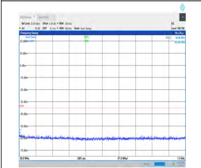
1-N41-30-100-H-1-DFT-PI2BPSK-Inner_1RB_Left-1 @1-30-1000-Ant1-35.34--56.46--35-PASS
