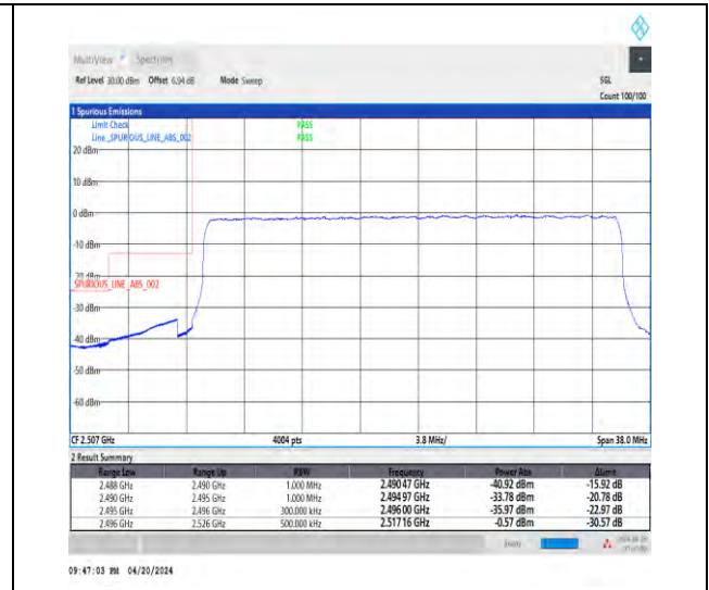
1-N41-30-30-L-3-DFT-PI2BPSK-Outer_Full-75@0-Ant1-1--PASS-see graph
