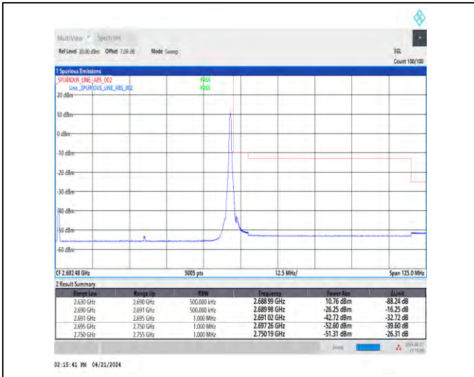
1-N41-30-60-H-2-DFT-PI2BPSK-Edge_1RB_Right-1@161-Ant1-1--PASS-see graph
