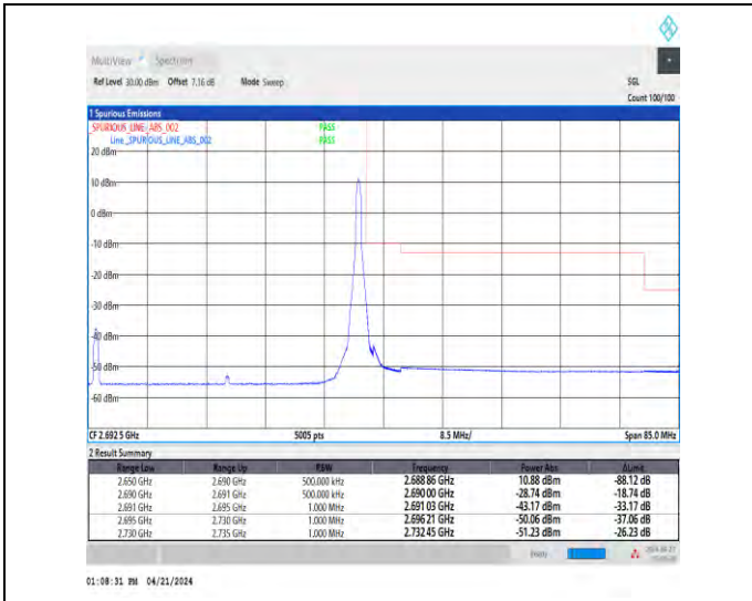
1-N41-30-40-H-2-DFT-PI2BPSK-Edge_1RB_Right-1@105-Ant1-1--PASS-see graph
