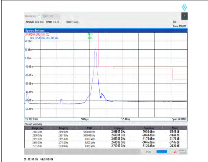
1-N41-30-25-H-5-CP-QPSK-Edge_1RB_Right-1@64-Ant1-1--PASS-see graph
