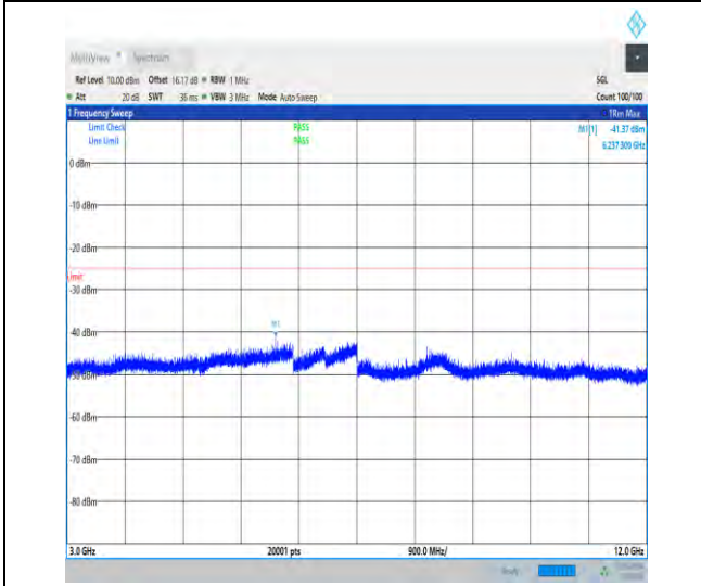
1-N41-30-100-H-1-DFT-PI2BPSK-Inner_1RB_Left-1 @1-3000-12000-Ant1-6237.30--41.37--25-PASS
