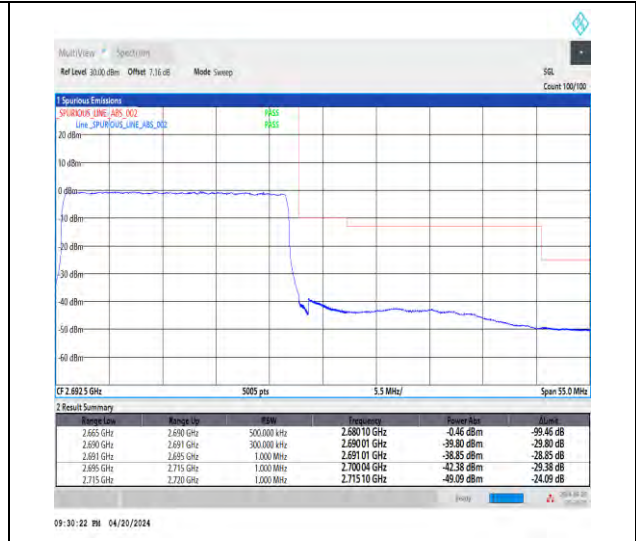
1-N41-30-25-H-3-DFT-PI2BPSK-Outer_Full-64@0-Ant1-1--PASS-see graph
