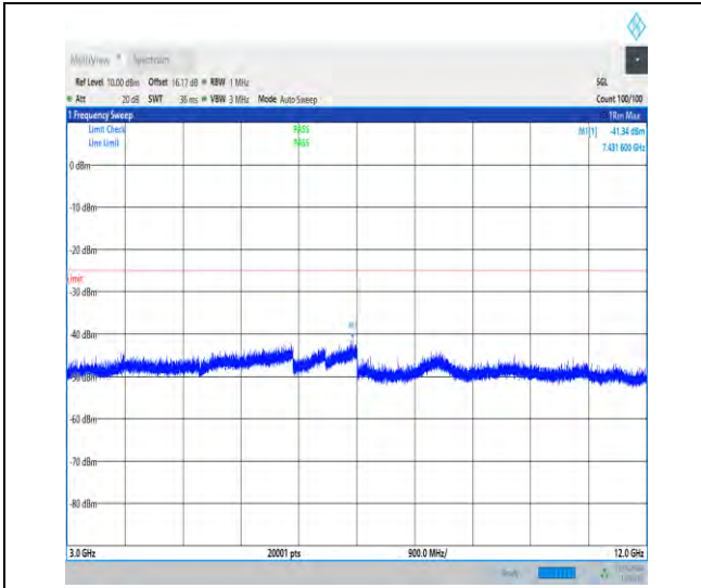
1-N41-30-100-L-1-DFT-PI2BPSK-Inner_1RB_Left-1 @1-3000-12000-Ant1-7431.60--41.34--25-PASS
