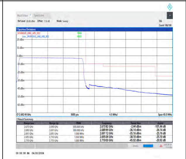
1-N41-30-20-H-6-CP-QPSK-Outer_Full-51@0-Ant1-1--PASS-see graph
