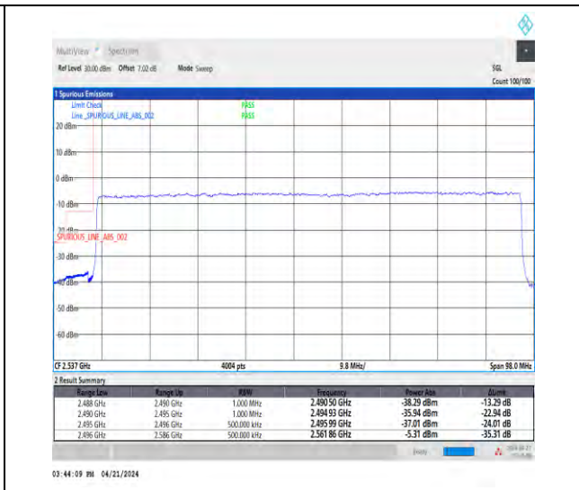
1-N41-30-90-L-3-DFT-PI2BPSK-Outer_Full-240@0-Ant1-1--PASS-see graph
