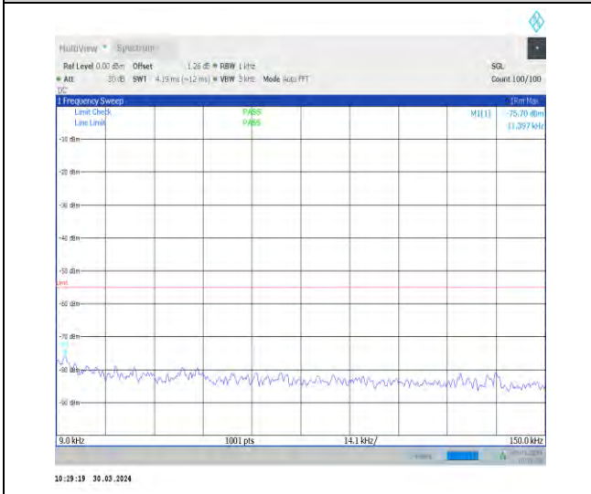
1-N41-30-100-M-1-DFT-PI2BPSK-Inner_1RB_Left-1 @1-0.009-0.15-Ant1-0.01--75.70--55-PASS
