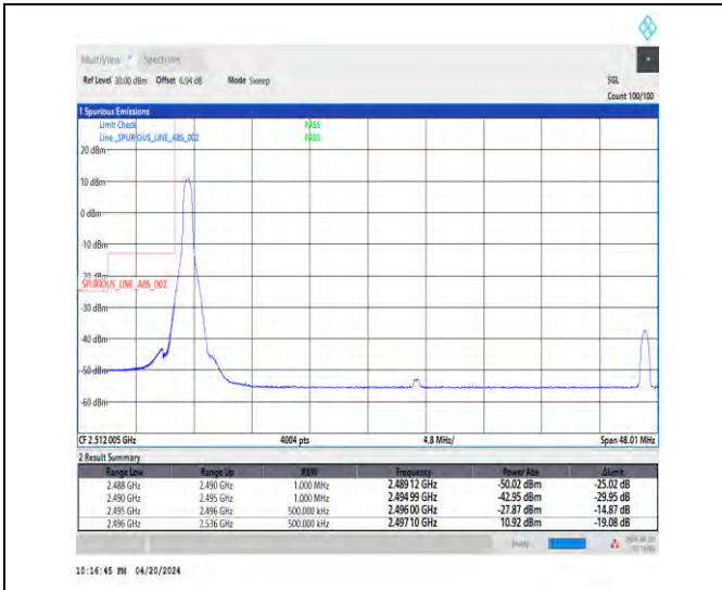
1-N41-30-40-L-1-DFT-PI2BPSK-Edge_1RB_Left-1@0-Ant1-1--PASS-see graph
