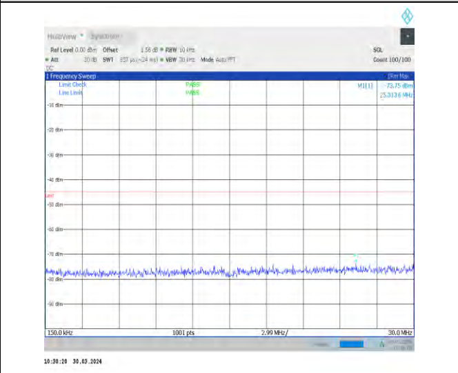
1-N41-30-100-M-1-DFT-PI2BPSK-Inner_1RB_Left-1 @1-0.15-30-Ant1-27.28--73.75--45-PASS
