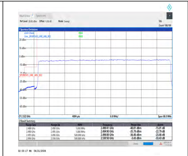
1-N41-30-60-L-3-DFT-PI2BPSK-Outer_Full-162@0-Ant1-1--PASS-see graph
