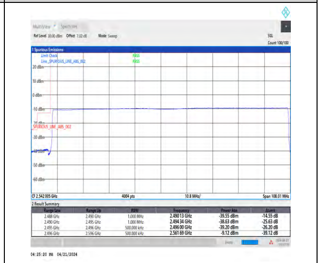
1-N41-30-100-L-6-CP-QPSK-Outer_Full-273@0-Ant1-1--PASS-see graph
