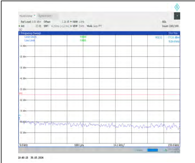
1-N41-30-100-H-1-DFT-PI2BPSK-Inner_1RB_Left-1 @1-0.009-0.15-Ant1-0.01--77.31--55-PASS
