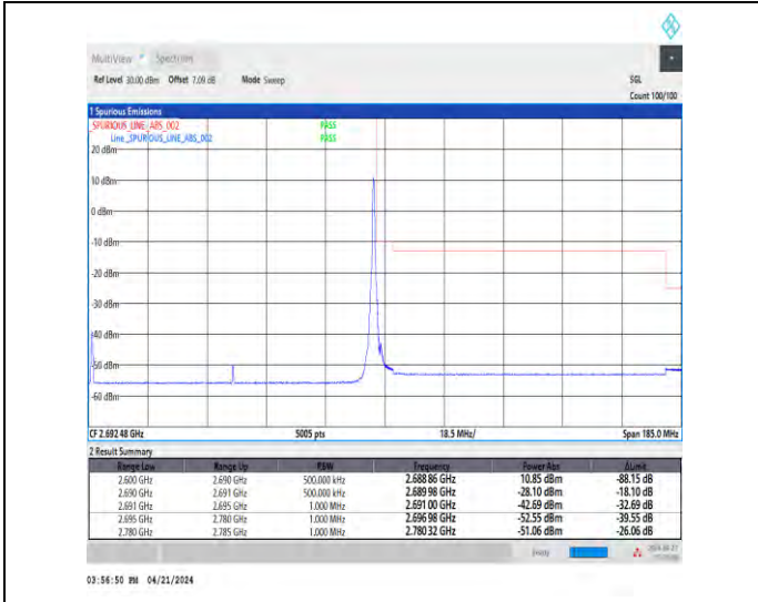
1-N41-30-90-H-2-DFT-PI2BPSK-Edge_1RB_Right-1@244-Ant1-1--PASS-see graph
