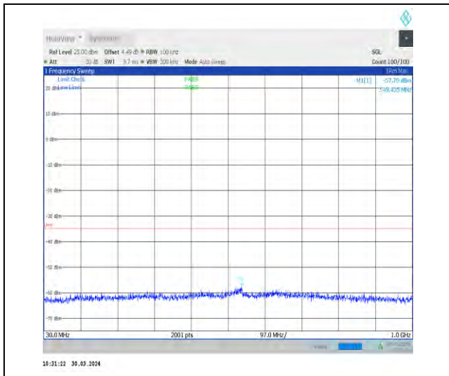
1-N41-30-100-M-1-DFT-PI2BPSK-Inner_1RB_Left-1 @1-30-1000-Ant1-528.10--57.70--35-PASS
