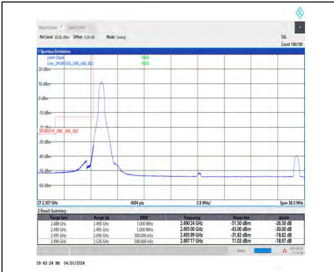
1-N41-30-30-L-1-DFT-PI2BPSK-Edge_1RB_Left-1@0-Ant1-1--PASS-see graph
