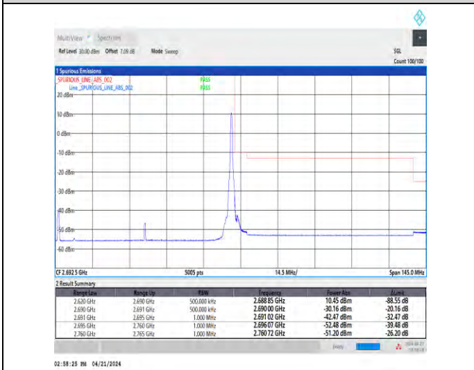
1-N41-30-70-H-5-CP-QPSK-Edge_1RB_Right-1@188-Ant1-1--PASS-see graph
