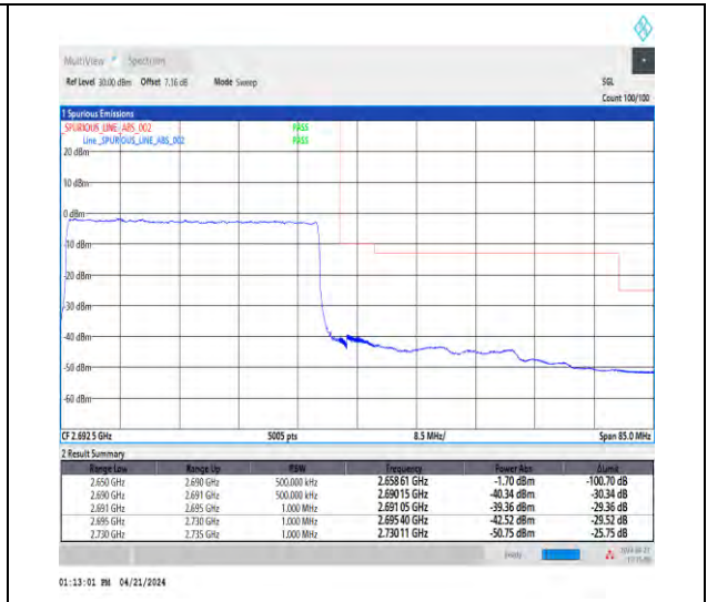
1-N41-30-40-H-3-DFT-PI2BPSK-Outer_Full-100@0-Ant1-1--PASS-see graph
