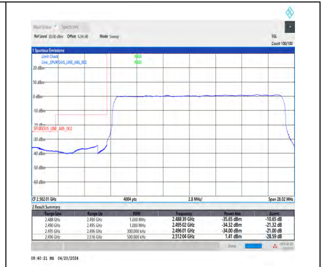
1-N41-30-20-L-3-DFT-PI2BPSK-Outer_Full-50@0-Ant1-1--PASS-see graph
