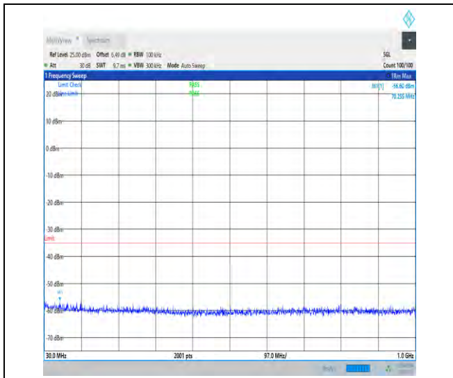
1-N41-30-100-M-1-DFT-PI2BPSK-Inner_1RB_Left-1 @1-30-1000-Ant1-70.26--56.60--35-PASS
