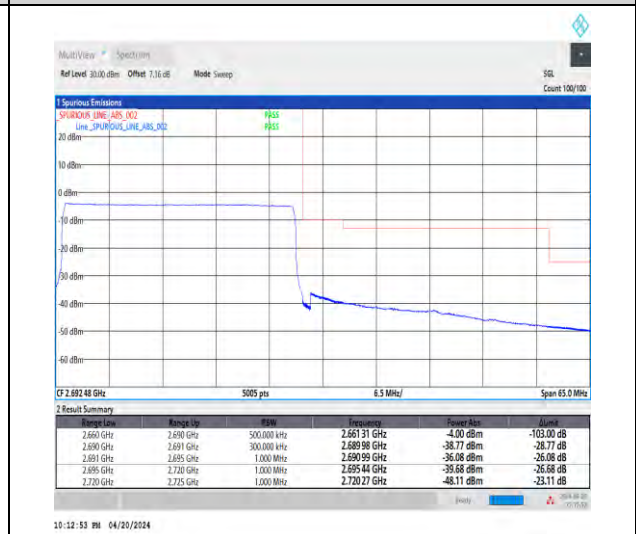
1-N41-30-30-H-6-CP-QPSK-Outer_Full-78@0-Ant1-1--PASS-see graph
