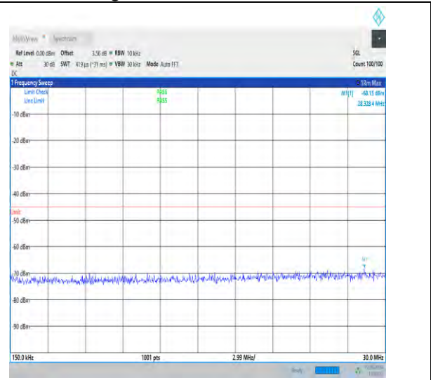
1-N41-30-100-H-1-DFT-PI2BPSK-Inner_1RB_Left-1 @1-0.15-30-Ant1-28.33--68.15--45-PASS
