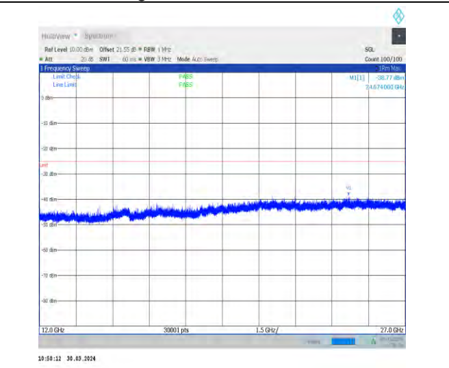
1-N41-30-100-H-1-DFT-PI2BPSK-Inner_1RB_Left-1 @1-12000-27000-Ant1-21015.00--38.77--25-PASS
