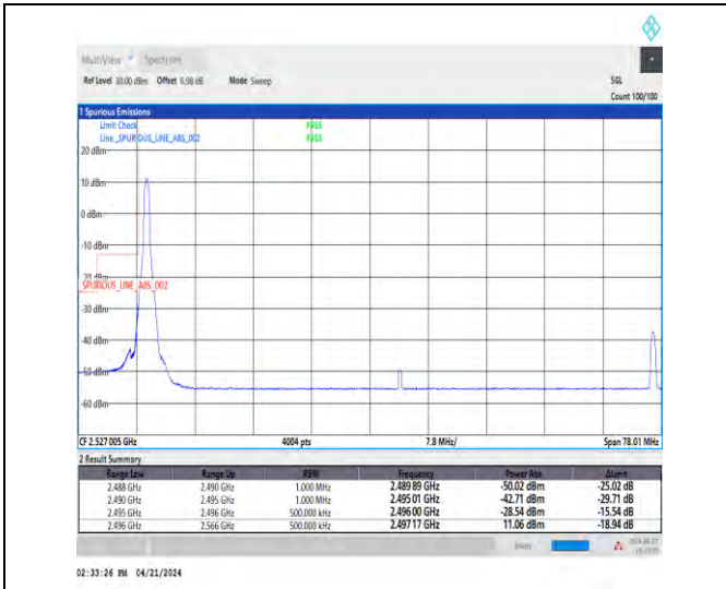
1-N41-30-70-L-1-DFT-PI2BPSK-Edge_1RB_Left-1@0-Ant1-1--PASS-see graph
