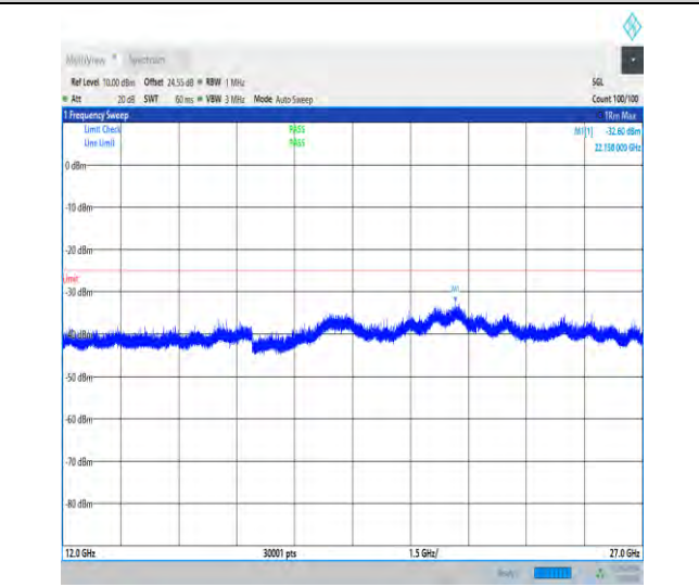
1-N41-30-100-M-1-DFT-PI2BPSK-Inner_1RB_Left-1 @1-12000-27000-Ant1-22158.00--32.60--25-PASS
