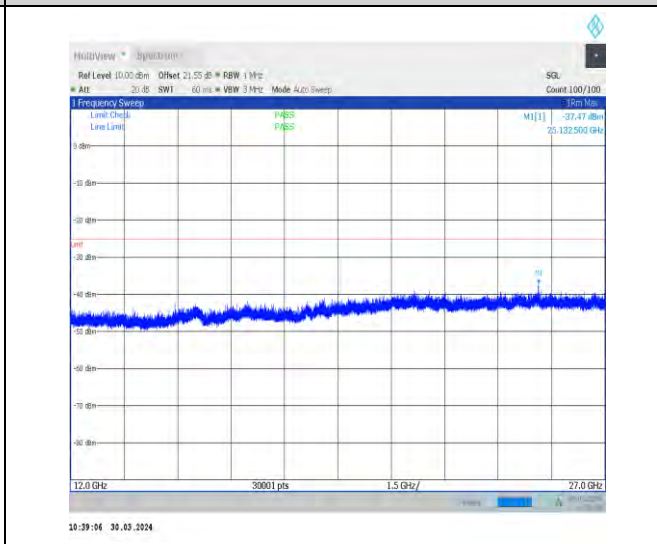
1-N41-30-100-M-1-DFT-PI2BPSK-Inner_1RB_Left-1 @1-12000-27000-Ant1-19449.50--37.47--25-PASS
