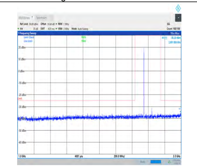
1-N41-30-100-M-1-DFT-PI2BPSK-Inner_1RB_Left-1 @1-1000-3000-Ant1-2991.00--35.23--25-PASS
