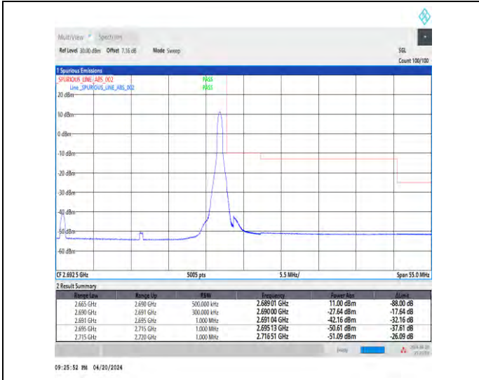
1-N41-30-25-H-2-DFT-PI2BPSK-Edge_1RB_Right-1@64-Ant1-1--PASS-see graph
