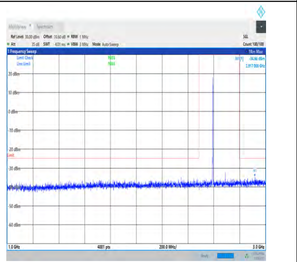
1-N41-30-100-H-1-DFT-PI2BPSK-Inner_1RB_Left-1 @1-1000-3000-Ant1-2917.00--34.66--25-PASS
