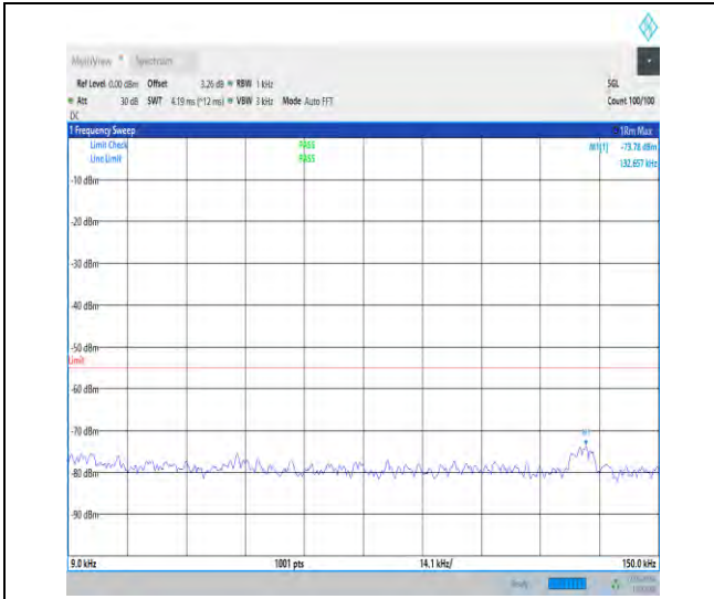
1-N41-30-100-H-1-DFT-PI2BPSK-Inner_1RB_Left-1 @1-0.009-0.15-Ant1-0.13--73.78--55-PASS
