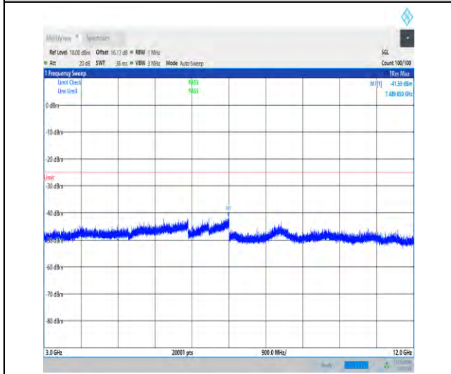
1-N41-30-100-M-1-DFT-PI2BPSK-Inner_1RB_Left-1 @1-3000-12000-Ant1-7489.65--41.59--25-PASS
