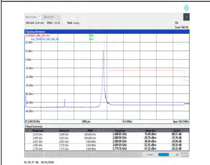
1-N41-30-80-H-5-CP-QPSK-Edge_1RB_Right-1@216-Ant1-1--PASS-see graph
