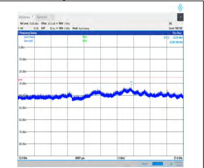
1-N41-30-100-L-1-DFT-PI2BPSK-Inner_1RB_Left-1 @1-12000-27000-Ant1-22301.50--32.29--25-PASS
