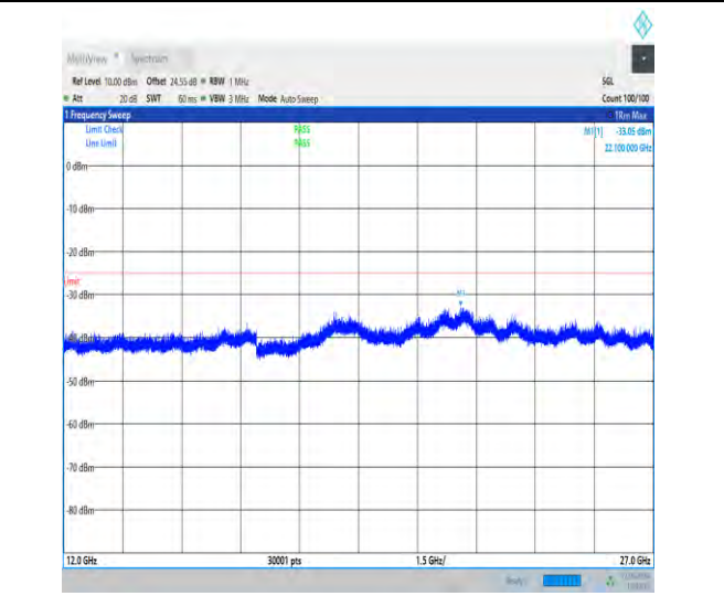
1-N41-30-100-H-1-DFT-PI2BPSK-Inner_1RB_Left-1 @1-12000-27000-Ant1-22100.00--33.05--25-PASS
