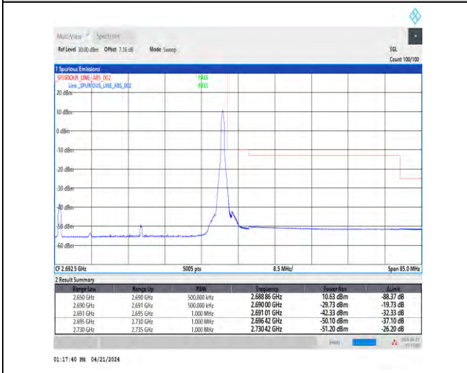
1-N41-30-40-H-5-CP-QPSK-Edge_1RB_Right-1@105-Ant1-1--PASS-see graph
