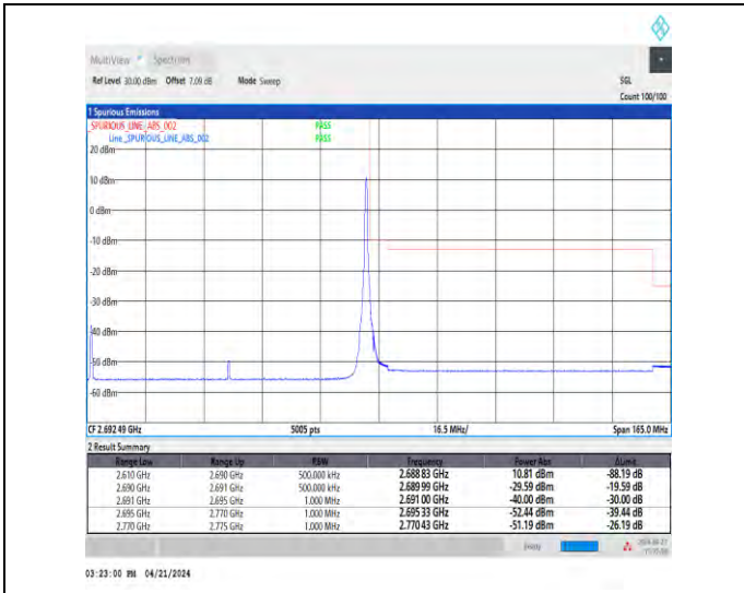
1-N41-30-80-H-2-DFT-PI2BPSK-Edge_1RB_Right-1@216-Ant1-1--PASS-see graph
