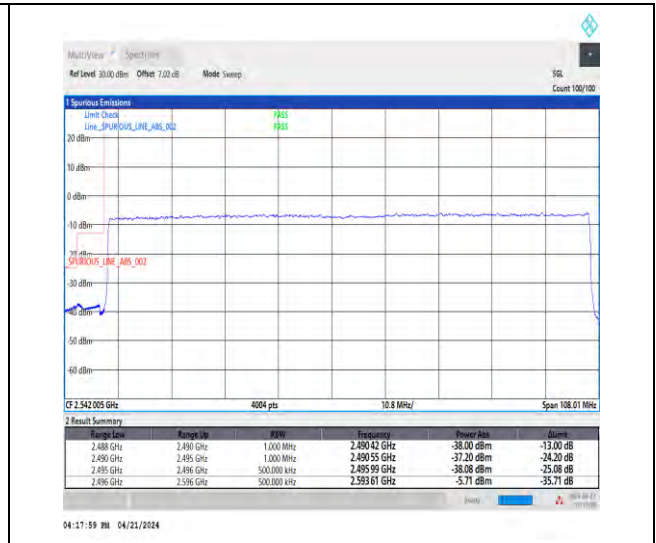
1-N41-30-100-L-3-DFT-PI2BPSK-Outer_Full-270@0-Ant1-1--PASS-see graph
