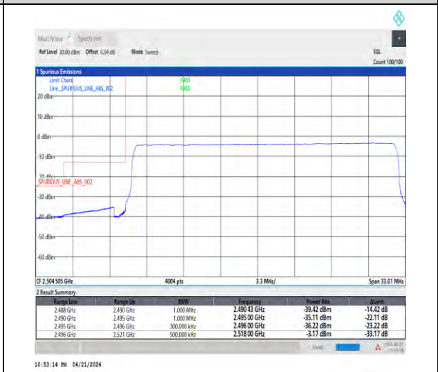
1-N41-30-25-L-6-CP-QPSK-Outer_Full-65@0-Ant1-1--PASS-see graph
