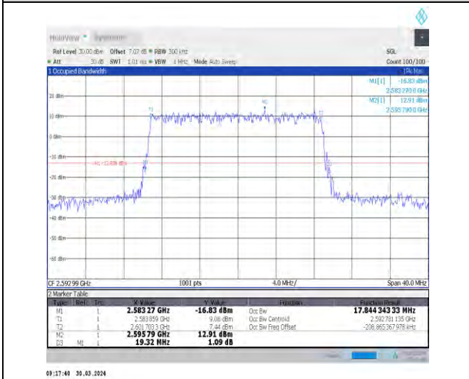
1-N41-30-20-M-5-DFT-256QAM-Outer_Full-50@0-Ant 1-17.844-19.320-≤20-PASS
