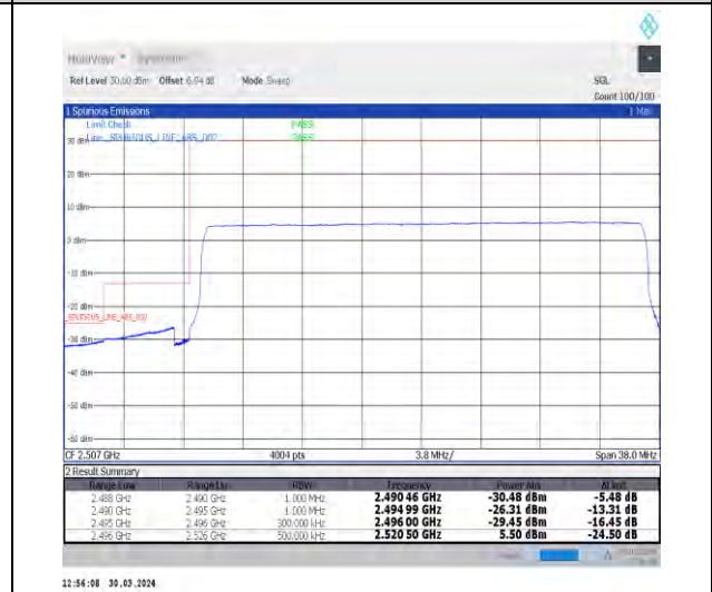
1-N41-30-30-L-6-CP-QPSK-Outer_Full-78@0-Ant1-1--PASS-see graph
