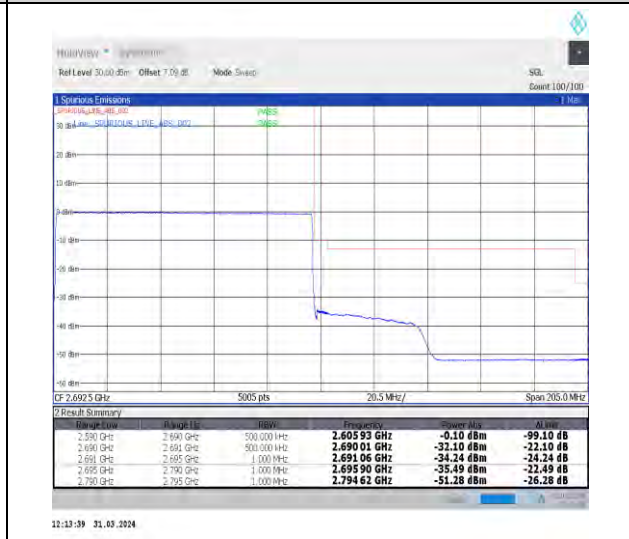
1-N41-30-100-H-6-CP-QPSK-Outer_Full-273@0-Ant1-1--PASS-see graph
