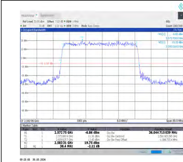
1-N41-30-40-M-2-DFT-PI2BPSK-Outer_Full-100@0-Ant1 1-36.045-38.400-≤40-PASS
