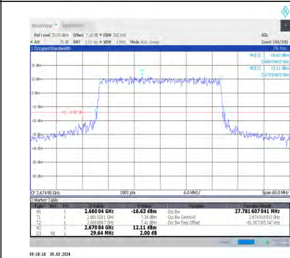
1-N41-30-30-H-8-CP-64QAM-Outer_Full-78@0-Ant1 -27.784-29.640-≤30-PASS
