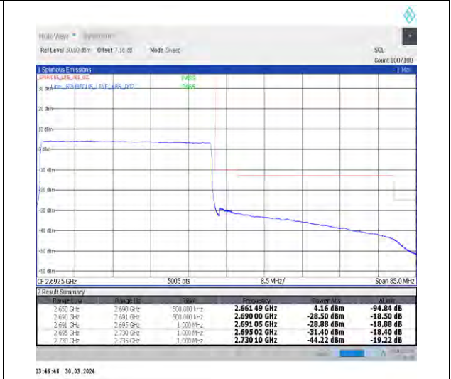
1-N41-30-40-H-6-CP-QPSK-Outer_Full-106@0-Ant1-1--PASS-see graph
