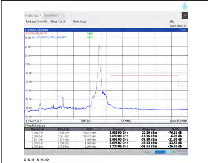
1-N41-30-40-H-5-CP-QPSK-Edge_1RB_Right-1@105-Ant1-1--PASS-see graph
