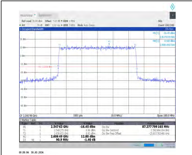
1-N41-30-90-M-7-CP-16QAM-Outer_Full-245@0-Ant 1-87.378-90.900-≤90-PASS
