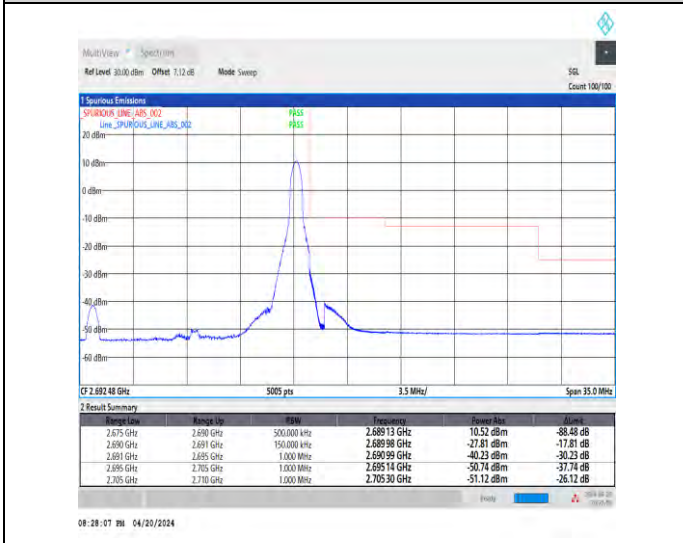
1-N41-30-15-H-5-CP-QPSK-Edge_1RB_Right-1@37-Ant1-1--PASS-see graph
