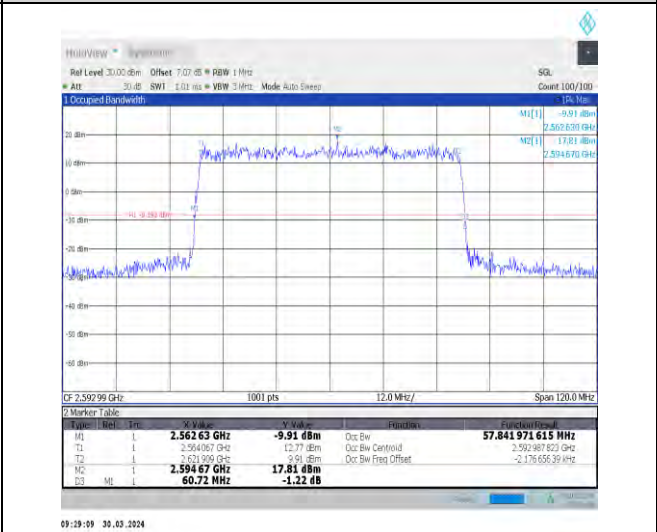
1-N41-30-60-M-1-DFT-QPSK-Outer_Full-162@0-Ant 1-57.842-60.720-≤60-PASS
