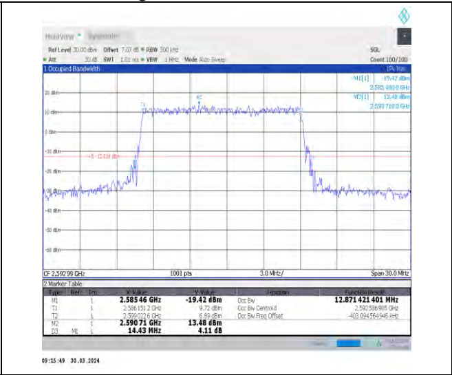
1-N41-30-15-M-5-DFT-256QAM-Outer_Full-36@0-A nt1-12.871-14.430-≤15-PASS
