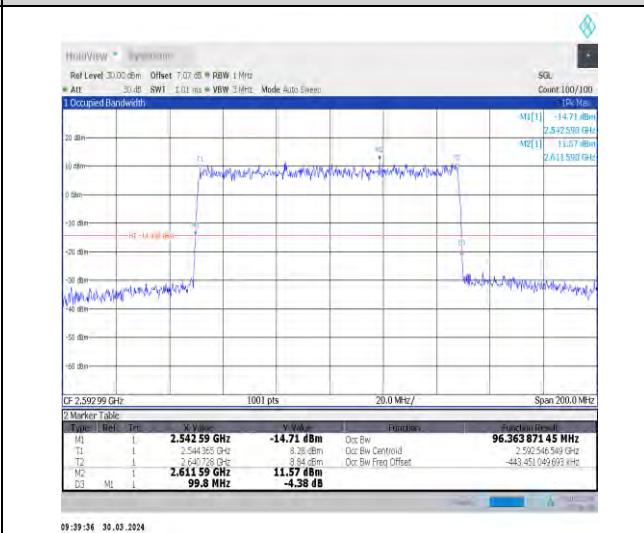
1-N41-30-100-M-5-DFT-256QAM-Outer_Full-270@0-Ant1-96.364-99.800-≤100-PASS
