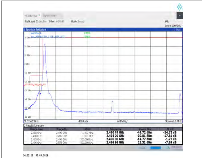
1-N41-30-60-L-1-DFT-PI2BPSK-Edge_1RB_Left-1@0-Ant1-1--PASS-see graph
