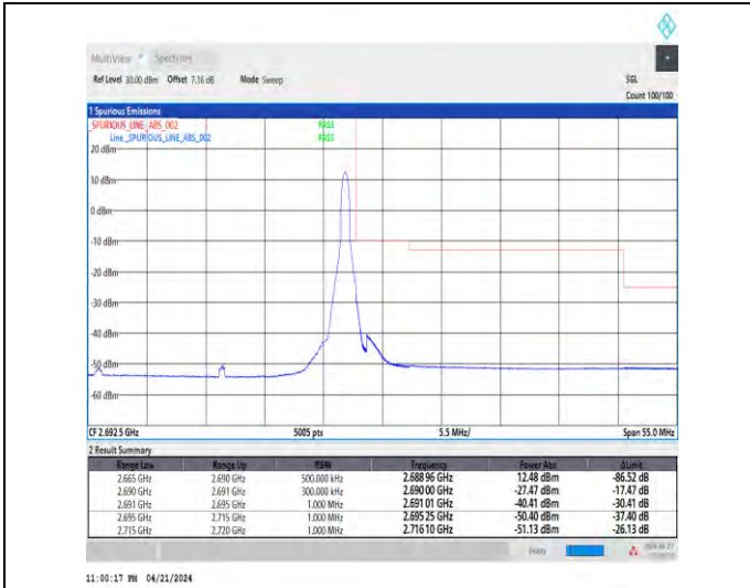
1-N41-30-25-H-2-DFT-PI2BPSK-Edge_1RB_Right-1@64-Ant1-1--PASS-see graph
