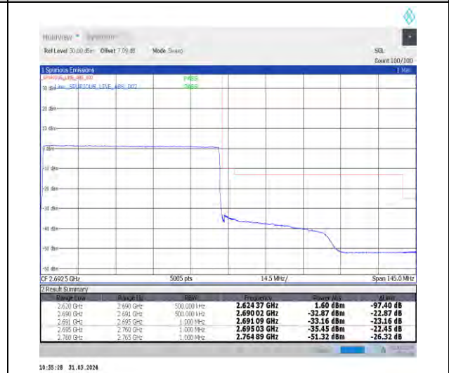
1-N41-30-70-H-6-CP-QPSK-Outer_Full-189@0-Ant1-1--PASS-see graph
