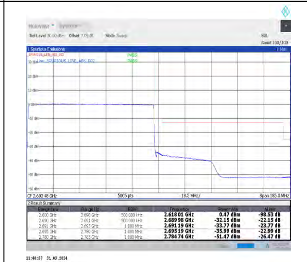
1-N41-30-90-H-6-CP-QPSK-Outer_Full-245@0-Ant1-1--PASS-see graph
