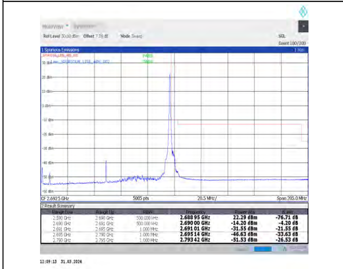
1-N41-30-100-H-5-CP-QPSK-Edge_1RB_Right-1@272 -Ant1-1--PASS-see graph
