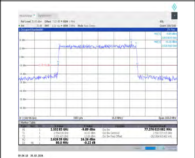
1-N41-30-80-M-3-DFT-16QAM-Outer_Full-216@0-A nt1-77.376-80.000-≤80-PASS
