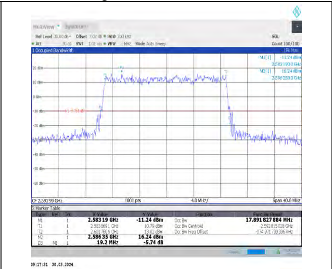
1-N41-30-20-M-4-DFT-64QAM-Outer_Full-50@0-Ant 1-17.892-19.200-≤20-PASS
