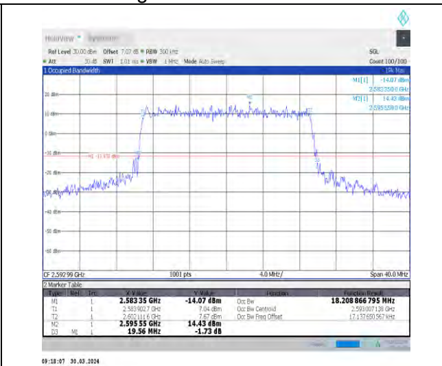
1-N41-30-20-M-8-CP-64QAM-Outer_Full-51@0-Ant1 1-18.209-19.560-<=20-PASS
