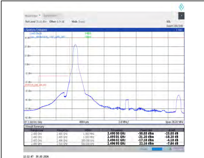
1-N41-30-20-L-1-DFT-PI2BPSK-Edge_1RB_Left-1@0-Ant1-1--PASS-see graph
