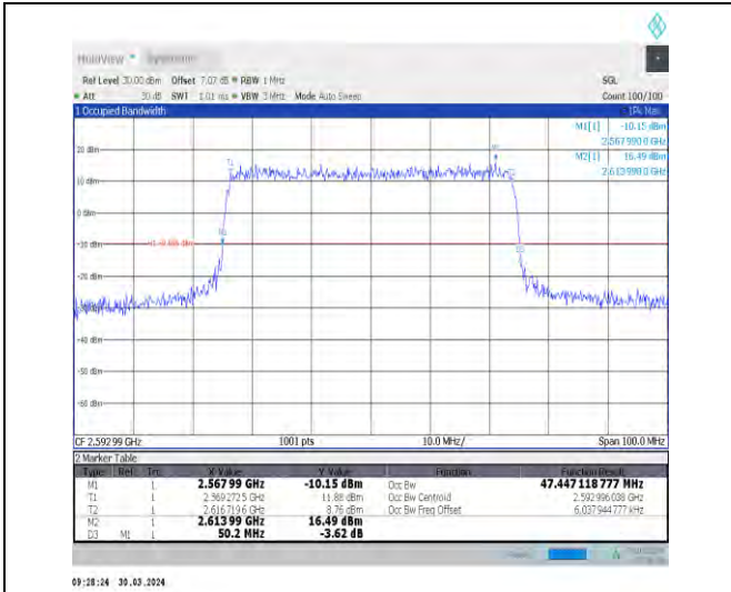
1-N41-30-50-M-7-CP-16QAM-Outer_Full-133@0-Ant 1-47.447-50.200-≤50-PASS
