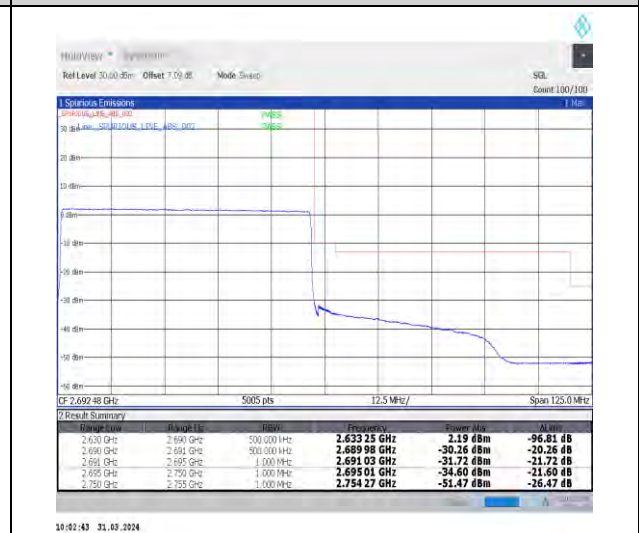
1-N41-30-60-H-6-CP-QPSK-Outer_Full-162@0-Ant1-1--PASS-see graph
