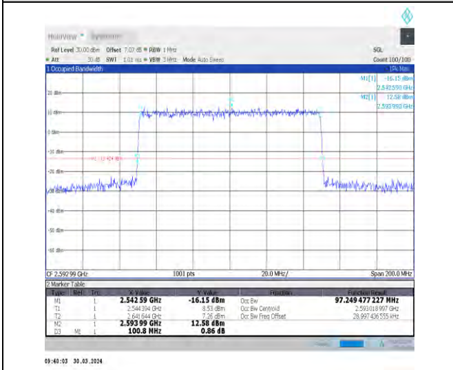
1-N41-30-100-M-8-CP-64QAM-Outer_Full-273@0-Ant nt1-97.249-100.800≤100-PASS
