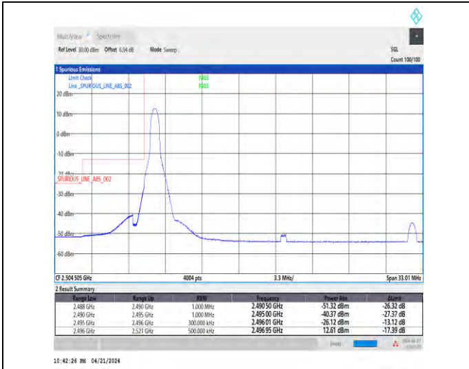
1-N41-30-25-L-1-DFT-PI2BPSK-Edge_1RB_Left-1@0-Ant1-1--PASS-see graph
