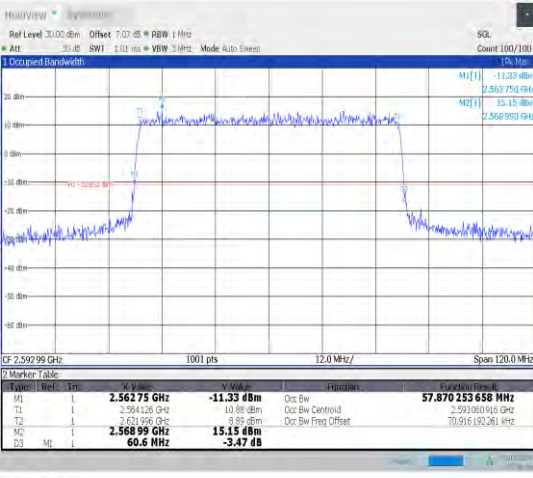
1-N41-30-60-M-6-CP-QPSK-Outer_Full-162@0-Ant1 -57.87-60.600-≤60-PASS
