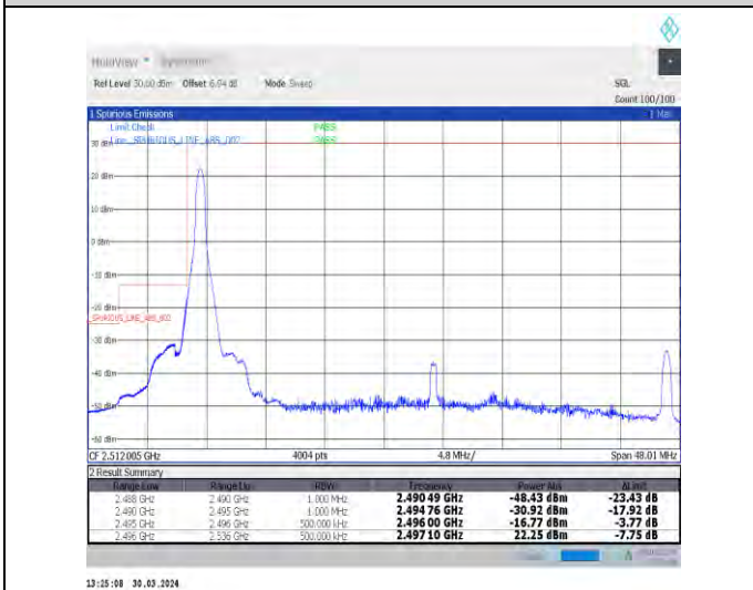
1-N41-30-40-L-4-CP-QPSK-Edge_1RB_Left-1@0-Ant1-1--PASS-see graph
