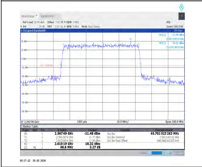
1-N41-30-50-M-1-DFT-QPSK-Outer_Full-128@0-Ant 1-45.703-48.600-≤50-PASS
