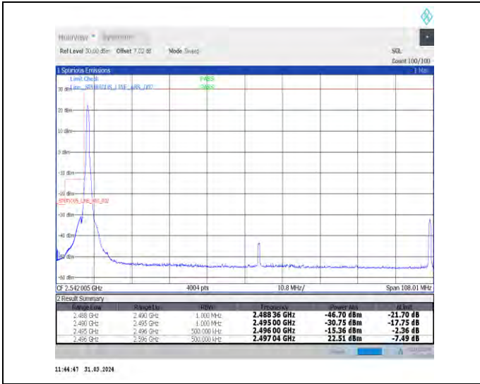
1-N41-30-100-L-1-DFT-PI2BPSK-Edge_1RB_Left-1@0-Ant1-1--PASS-see graph
