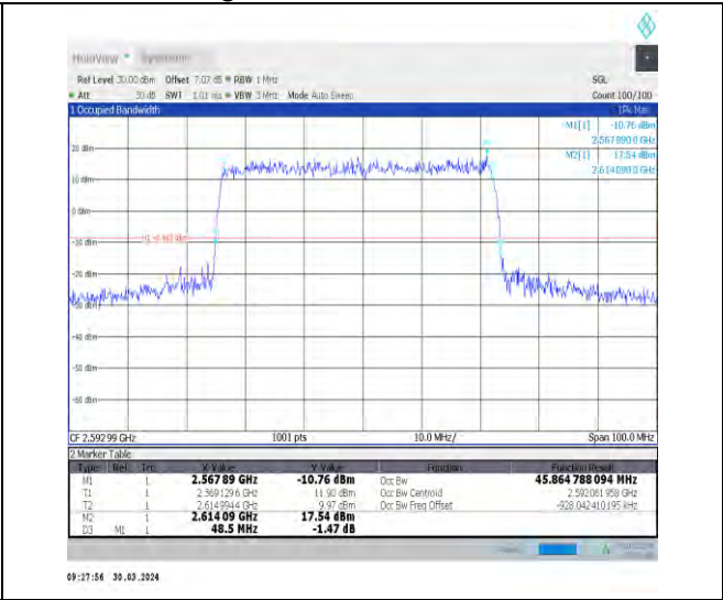
1-N41-30-50-M-4-DFT-64QAM-Outer_Full-128@0-A nt1-45.865-48.500-≤50-PASS
