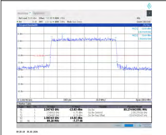
1-N41-30-90-M-1-DFT-QPSK-Outer_Full-240@0-Ant 1-85.275-89.280-≤90-PASS
