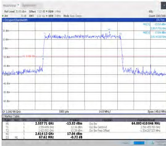
1-N41-30-70-M-1-DFT-QPSK-Outer_Full-180@0-Ant 1-64.093-67.620-≤70-PASS
