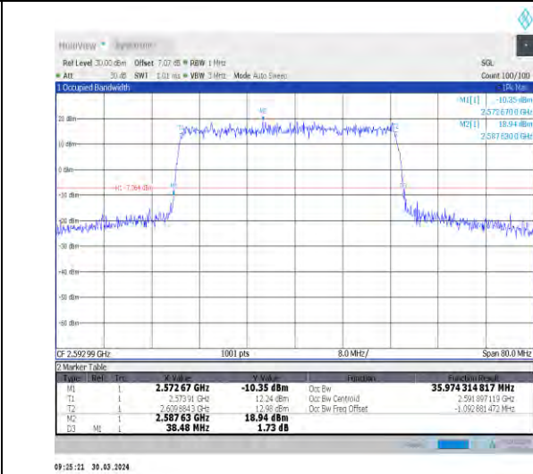
1-N41-30-40-M-3-DFT-16QAM-Outer_Full-100@0-Ant1 1-35.974-38.480-≤40-PASS
