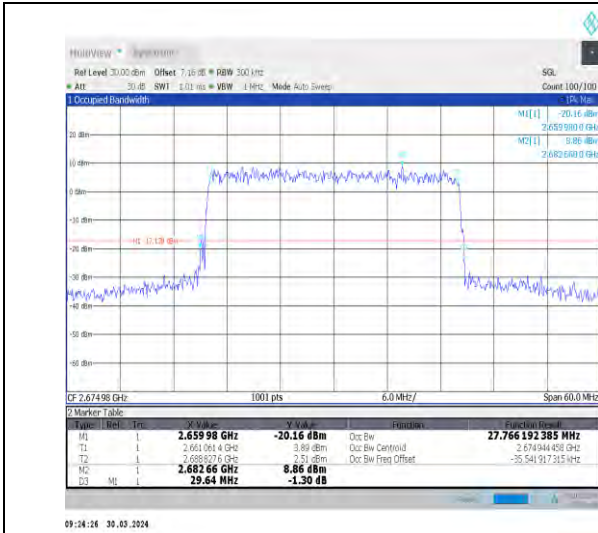
1-N41-30-30-H-9-CP-256QAM-Outer_Full-78@0-Ant 1-27.77-29.640-≤30-PASS
