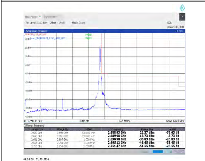
1-N41-30-60-H-5-CP-QPSK-Edge_1RB_Right-1@161-Ant1-1--PASS-see graph
