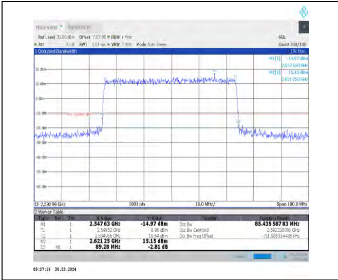
1-N41-30-90-M-3-DFT-16QAM-Outer_Full-240@0-A Ant1-85.436-89.280-≤90-PASS
