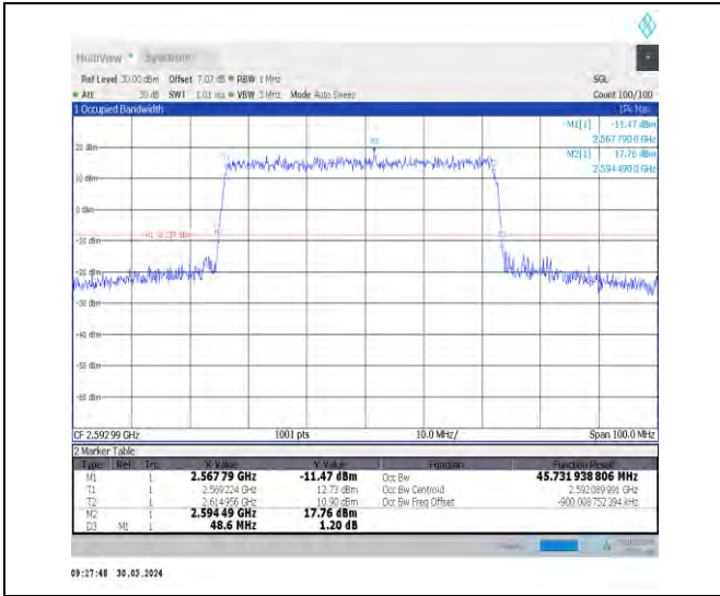
1-N41-30-50-M-3-DFT-16QAM-Outer_Full-128@0-A nt1-45.732-48.600-≤50-PASS
