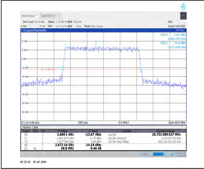
1-N41-30-30-H-3-DFT-16QAM-Outer_Full-75@0-Ant1 1-26.752-28.800-≤30-PASS
