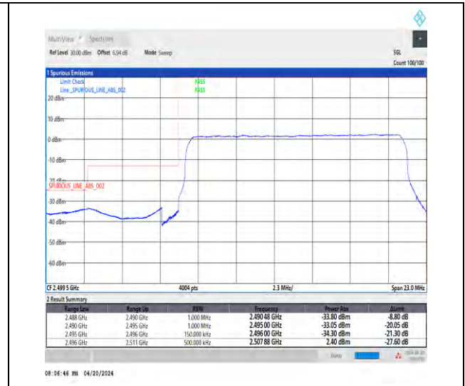
1-N41-30-15-L-3-DFT-PI2BPSK-Outer_Full-36@0-Ant1-1--PASS-see graph
