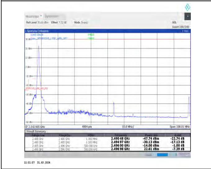
1-N41-30-100-L-4-CP-QPSK-Edge_1RB_Left-1@0-Ant1-1--PASS-see graph
