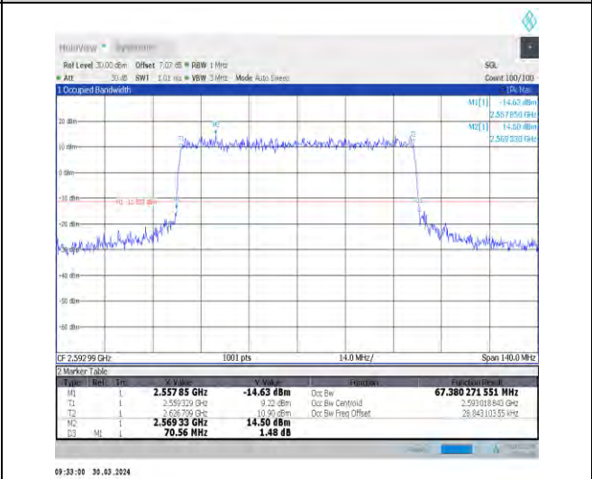
1-N41-30-70-M-8-CP-64QAM-Outer_Full-189@0-Ant1-67.38-70.560-<=70-PASS
