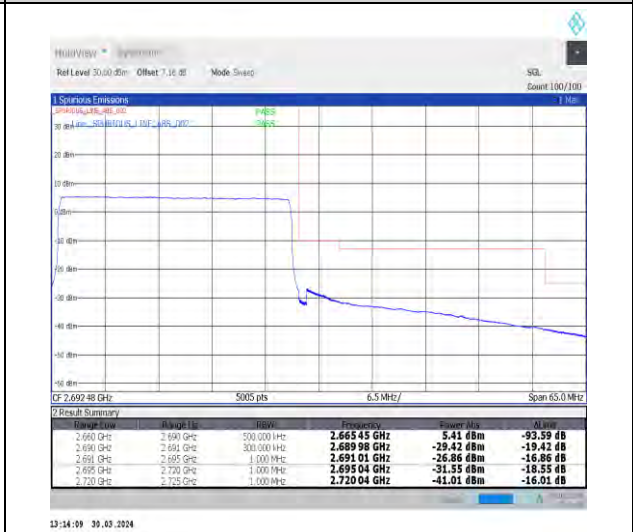
1-N41-30-30-H-6-CP-QPSK-Outer_Full-78@0-Ant1-1--PASS-see graph
