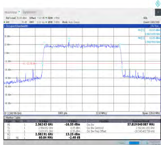
1-N41-30-60-M-9-CP-256QAM-Outer_Full-162@0-Ant1 -57.819-60.840-≤60-PASS
