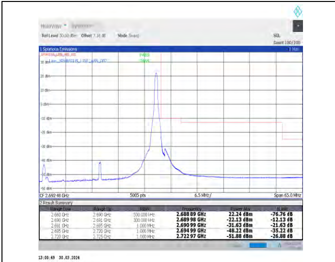
1-N41-30-30-H-2-DFT-PI2BPSK-Edge_1RB_Right-1@77-Ant1-1--PASS-see graph
