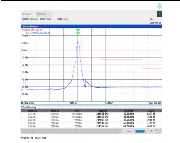
1-N41-30-15-H-2-DFT-PI2BPSK-Edge_1RB_Right-1@37-Ant1-1--PASS-see graph
