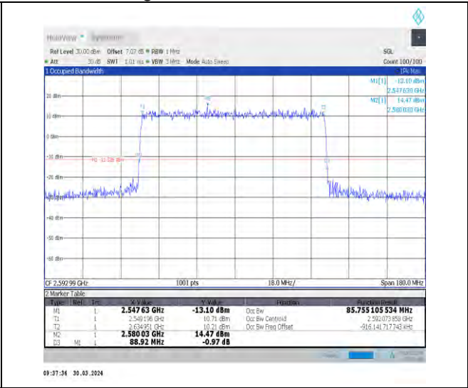
1-N41-30-90-M-4-DFT-64QAM-Outer_Full-240@0-A Ant1-85.755-88.920-≤90-PASS
