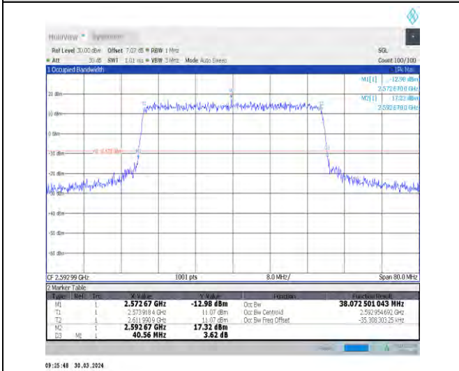
1-N41-30-40-M-6-CP-QPSK-Outer_Full-106@0-Ant1 -38.073-40.560-≤40-PASS
