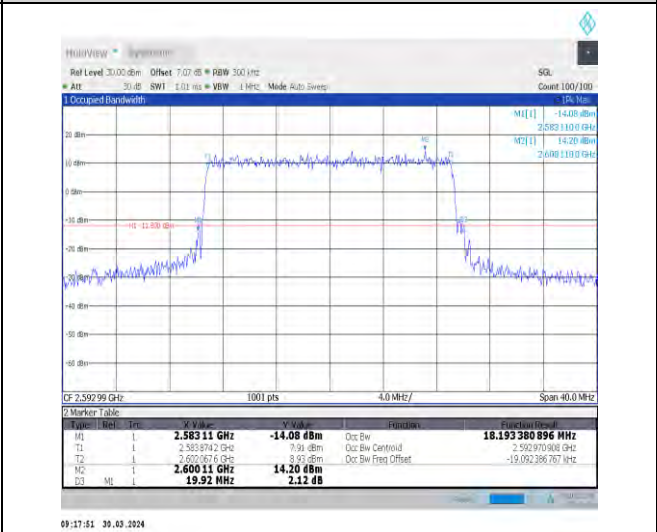
1-N41-30-20-M-6-CP-QPSK-Outer_Full-51@0-Ant 1-18.193-19.920-≤20-PASS
