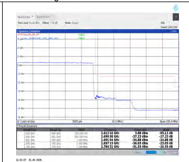
1-N41-30-90-H-3-DFT-PI2BPSK-Outer_Full-240@0-Ant1-1--PASS-see graph
