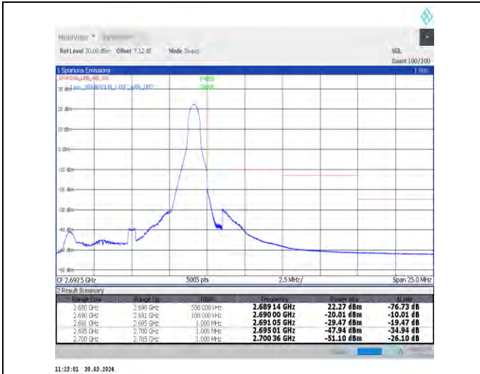
1-N41-30-10-H-2-DFT-PI2BPSK-Edge_1RB_Right-1@23-Ant1-1--PASS-see graph
