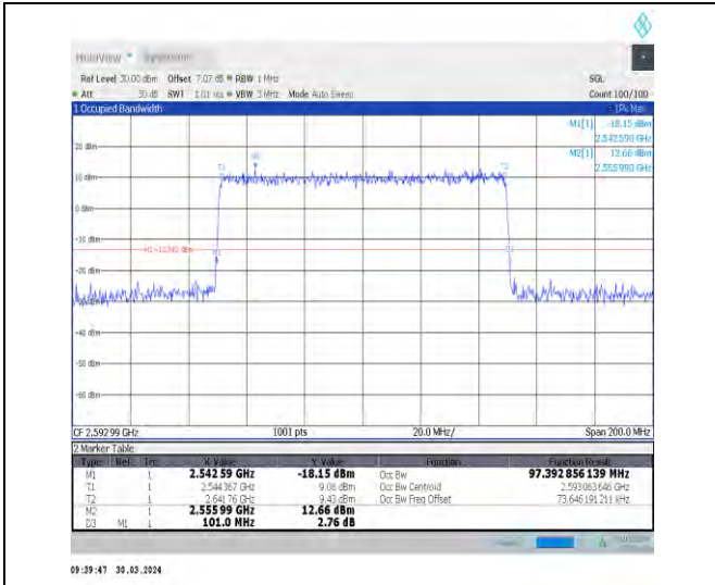
1-N41-30-100-M-6-CP-QPSK-Outer_Full-273@0-Ant 1-97.393-101.000≤100-PASS
