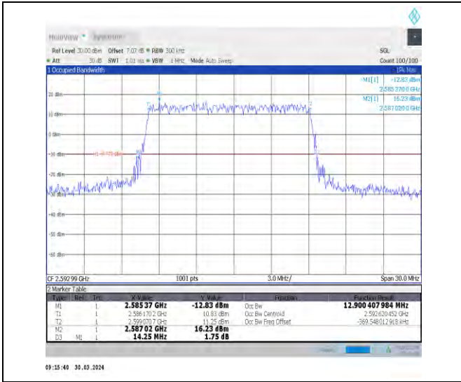
1-N41-30-15-M-4-DFT-64QAM-Outer_Full-36@0-Ant 1-12.9-14.250-≤15-PASS
