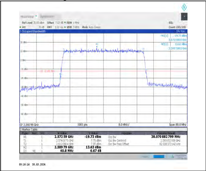
1-N41-30-40-M-9-CP-256QAM-Outer_Full-106@0-Ant 1-38.071-40.800-≤40-PASS
