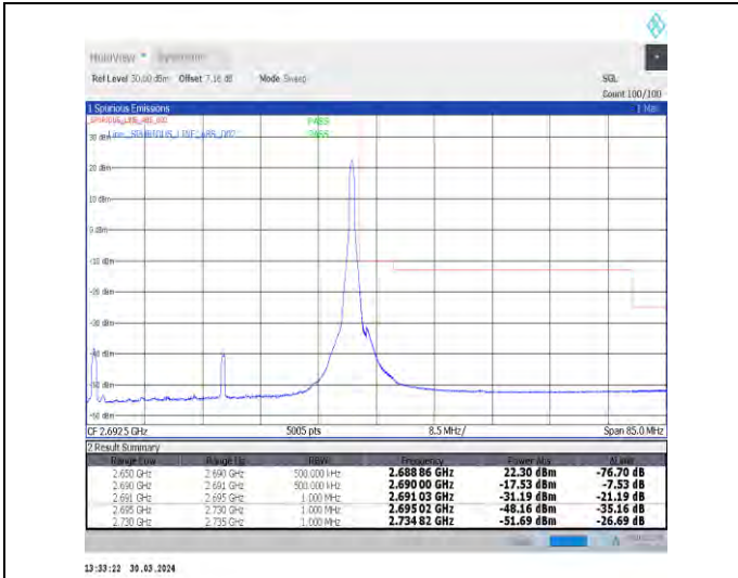
1-N41-30-40-H-2-DFT-PI2BPSK-Edge_1RB_Right-1@105-Ant1-1--PASS-see graph
