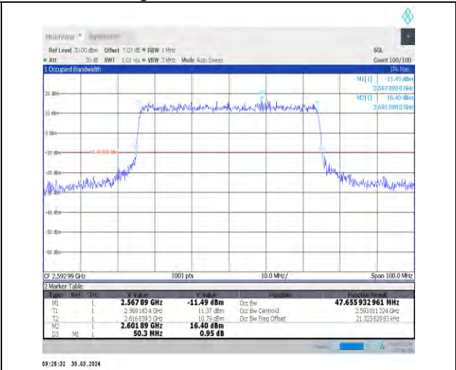
1-N41-30-50-M-8-CP-64QAM-Outer_Full-133@0-Ant t1-47.656-50.300-≤50-PASS
