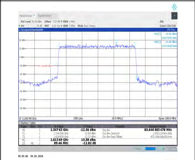
1-N41-30-90-M-2-DFT-PI2BPSK-Outer_Full-240@0-Ant 1-85.641-89.460-≤90-PASS
