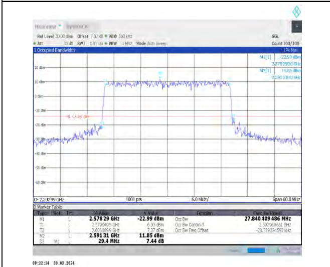
1-N41-30-30-M-8-CP-64QAM-Outer_Full-78@0-Ant1-27.844-29.400-≤30-PASS
