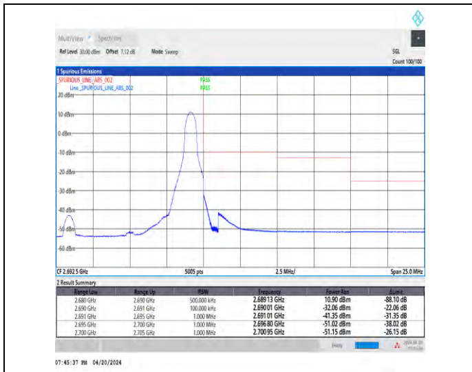
1-N41-30-10-H-2-DFT-PI2BPSK-Edge_1RB_Right-1@23-Ant1-1--PASS-see graph
