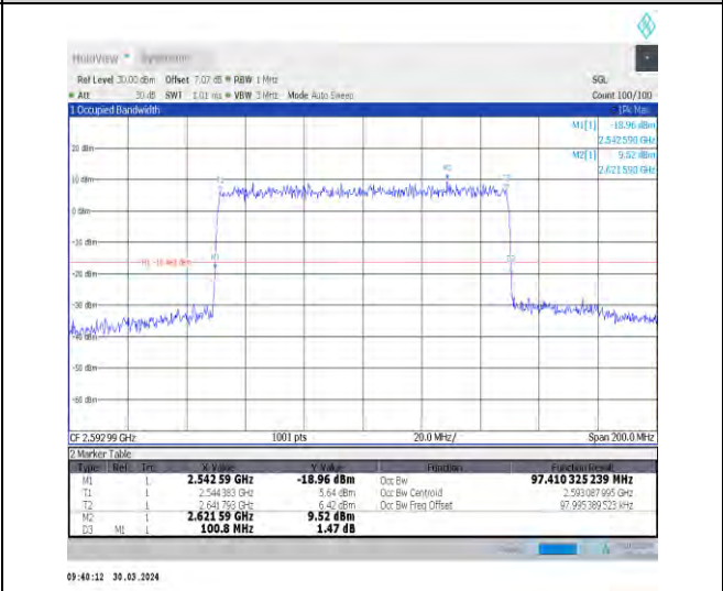
1-N41-30-100-M-9-CP-256QAM-Outer_Full-273@0-Ant nt1-97.41-100.800≤100-PASS
