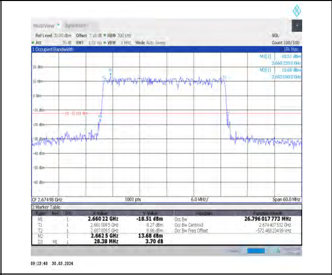
1-N41-30-30-H-4-DFT-64QAM-Outer_Full-75@0-Ant1 1-26.796-28.380-≤30-PASS
