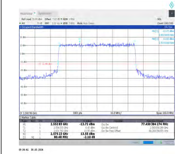
1-N41-30-80-M-6-CP-QPSK-Outer_Full-217@0-Ant1 -77.45-80.480-≤80-PASS
