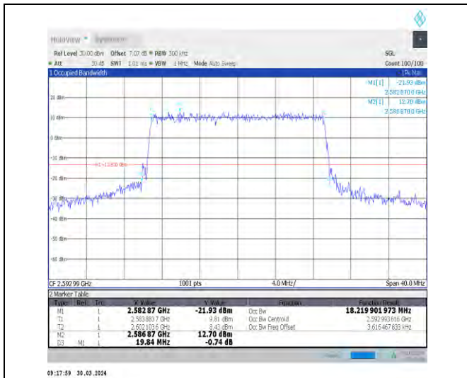
1-N41-30-20-M-7-CP-16QAM-Outer_Full-51@0-Ant1 -18.22-19.840-<=20-PASS
