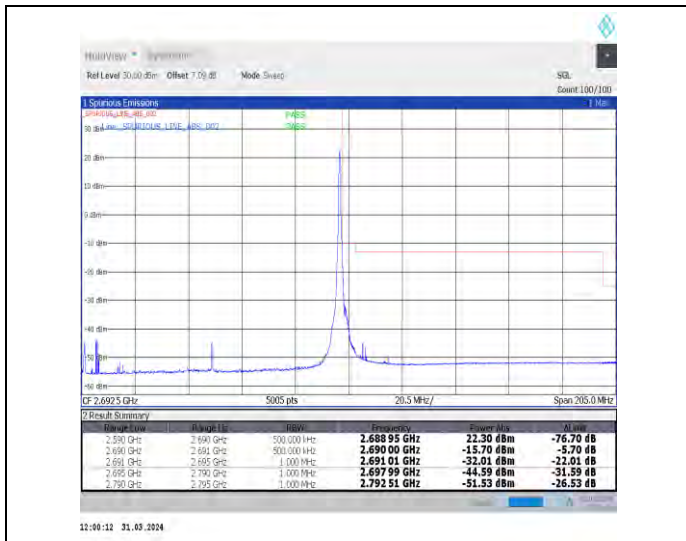
1-N41-30-100-H-2-DFT-PI2BPSK-Edge_1RB_Right-1 @272-Ant1-1--PASS-see graph
