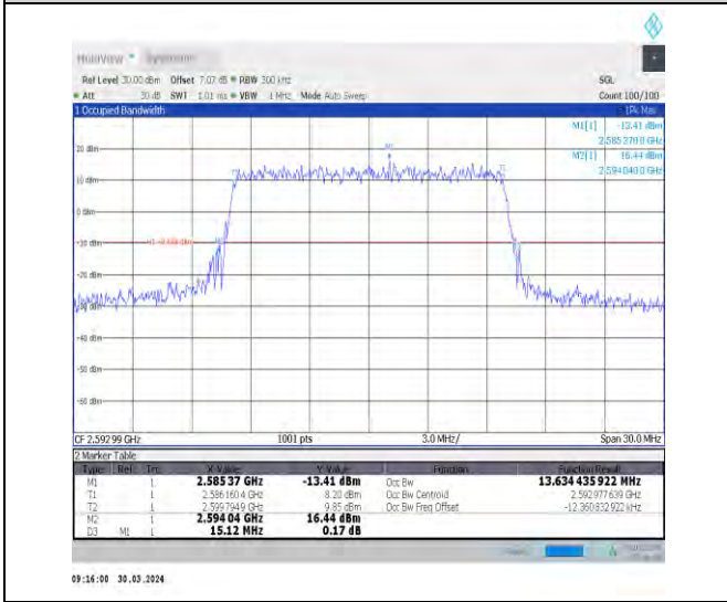
1-N41-30-15-M-6-CP-QPSK-Outer_Full-38@0-Ant1 13.634-15.120-≤15-PASS
