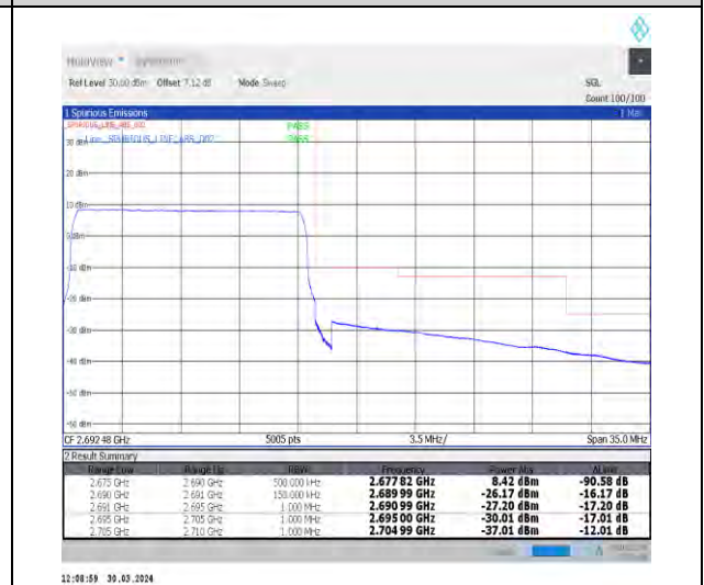
1-N41-30-15-H-6-CP-QPSK-Outer_Full-38@0-Ant1-1--PASS-see graph
