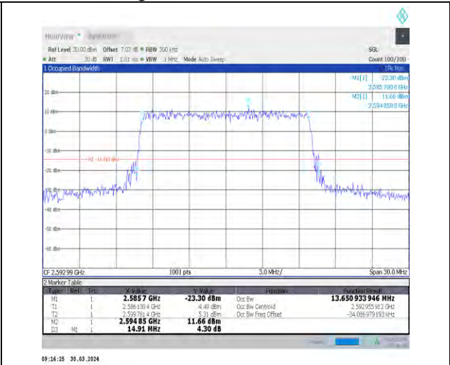
1-N41-30-15-M-9-CP-256QAM-Outer_Full-38@0-Ant1 -13.651-14.910-≤15-PASS
