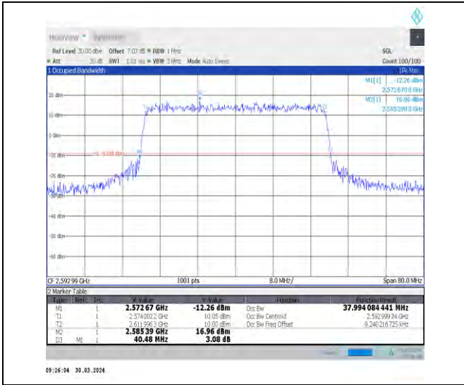
1-N41-30-40-M-8-CP-64QAM-Outer_Full-106@0-Ant 1-37.994-40.480-≤40-PASS
