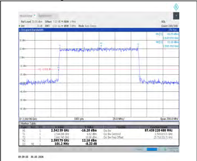
1-N41-30-100-M-7-CP-16QAM-Outer_Full-273@0-Ant nt1-97.459-101.200≤100-PASS
