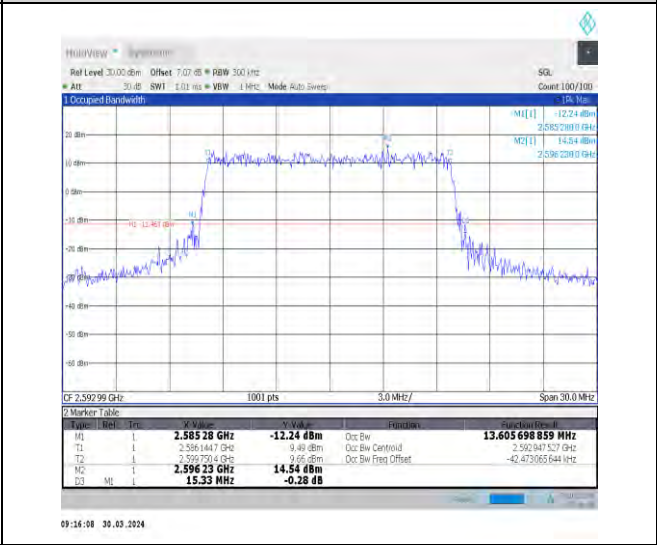
1-N41-30-15-M-7-CP-16QAM-Outer_Full-38@0-Ant 1-13.606-15.330-≤15-PASS
