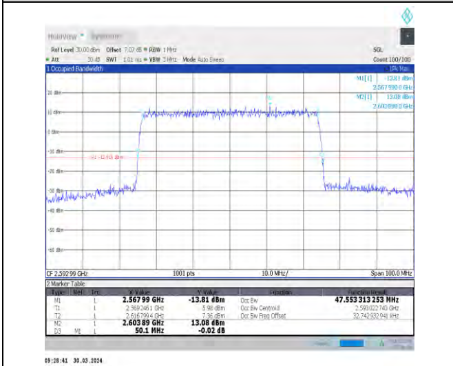
1-N41-30-50-M-9-CP-256QAM-Outer_Full-133@0-Ant nt1-47.553-50.100-≤50-PASS
