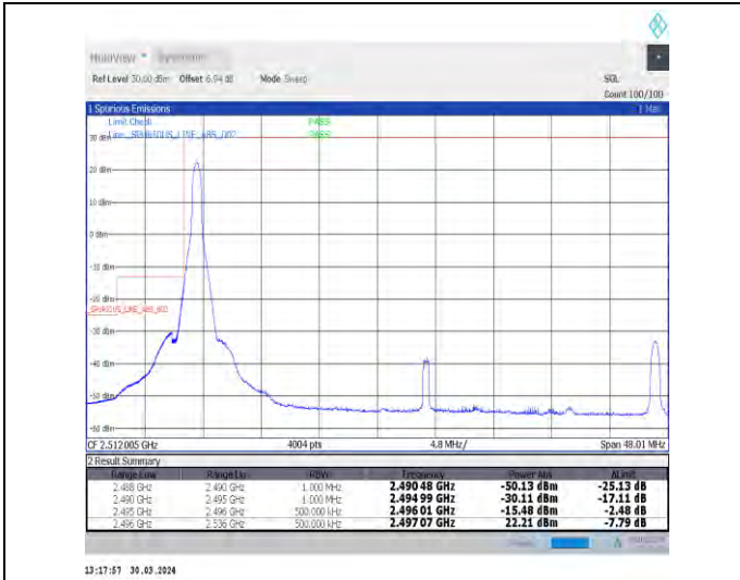
1-N41-30-40-L-1-DFT-PI2BPSK-Edge_1RB_Left-1@0-Ant1-1--PASS-see graph
