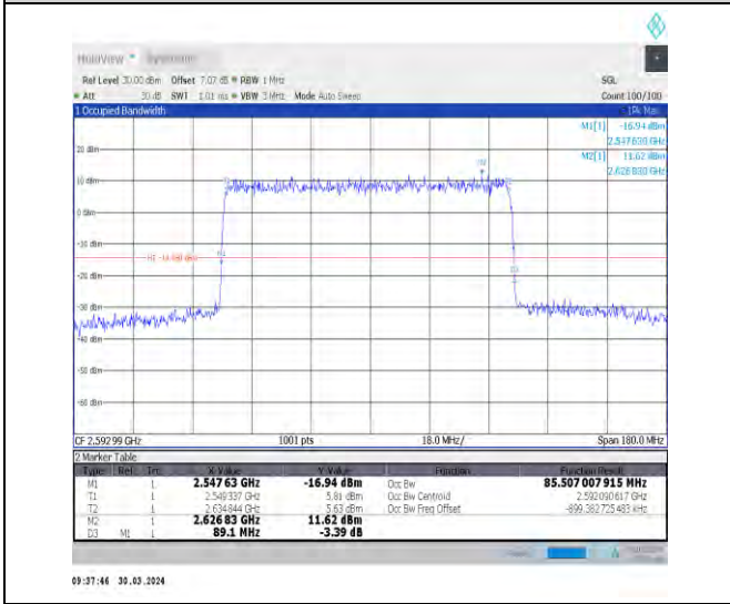
1-N41-30-90-M-5-DFT-256QAM-Outer_Full-240@0-A Ant1-85.507-89.100-≤90-PASS
