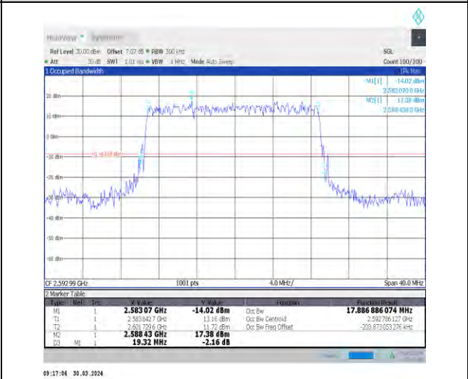
1-N41-30-20-M-2-DFT-PI2BPSK-Outer_Full-50@0-Ant1 -17.887-19.320-≤20-PASS
