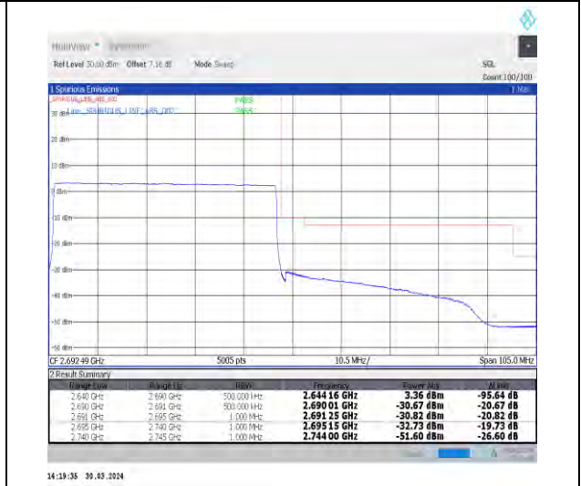
1-N41-30-50-H-6-CP-QPSK-Outer_Full-133@0-Ant1-1--PASS-see graph
