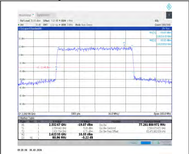
1-N41-30-80-M-9-CP-256QAM-Outer_Full-217@0-Ant 1-77.262-80.960-≤80-PASS
