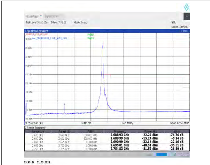
1-N41-30-60-H-2-DFT-PI2BPSK-Edge_1RB_Right-1@161-Ant1-1--PASS-see graph
