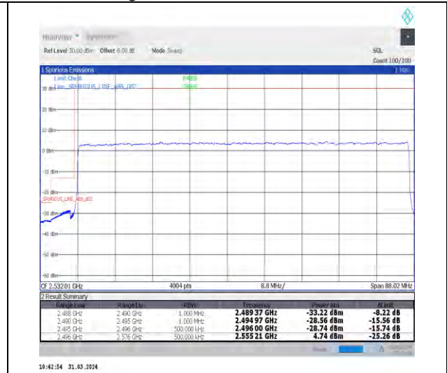
1-N41-30-80-L-3-DFT-PI2BPSK-Outer_Full-216@0-Ant1-1--PASS-see graph
