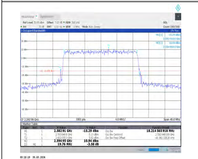
1-N41-30-20-M-9-CP-256QAM-Outer_Full-51@0-Ant1 1-18.215-19.760-<=20-PASS
