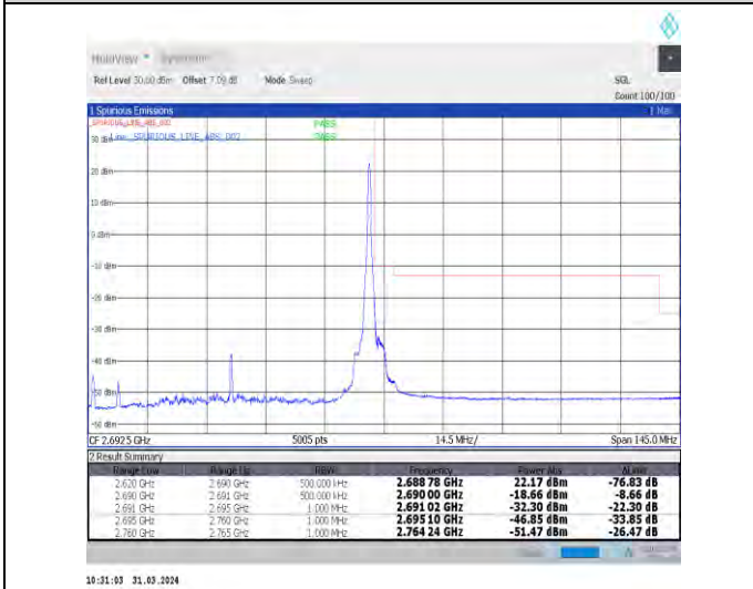
1-N41-30-70-H-5-CP-QPSK-Edge_1RB_Right-1@188-Ant1-1--PASS-see graph
