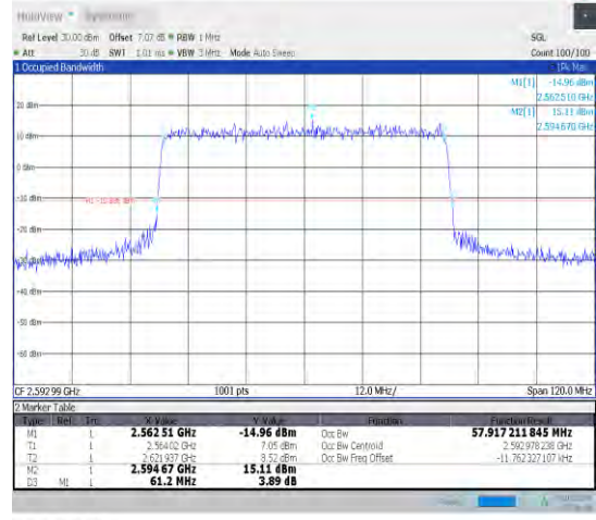
1-N41-30-60-M-7-CP-16QAM-Outer_Full-162@0-Ant1 -57.917-61.200-≤60-PASS
