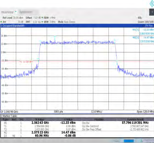
1-N41-30-60-M-8-CP-64QAM-Outer_Full-162@0-Ant1 1-57.796-60.960-≤60-PASS
