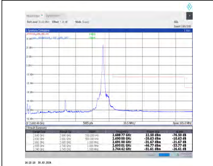
1-N41-30-50-H-5-CP-QPSK-Edge_1RB_Right-1@132-Ant1-1--PASS-see graph
