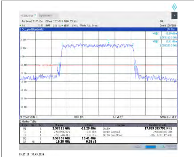
1-N41-30-20-M-3-DFT-16QAM-Outer_Full-50@0-Ant 1-17.889-19.280-≤20-PASS
