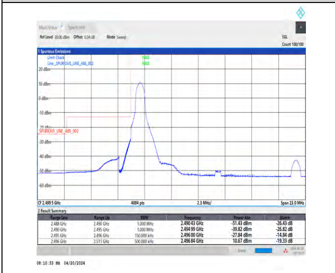
1-N41-30-15-L-4-CP-QPSK-Edge_1RB_Left-1@0-Ant1-1--PASS-see graph
