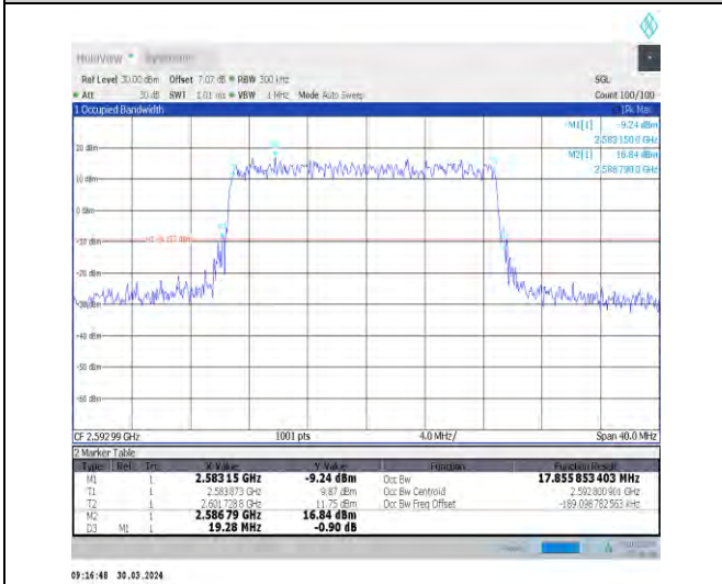
1-N41-30-20-M-1-DFT-QPSK-Outer_Full-50@0-Ant1 -17.856-19.280-≤20-PASS
