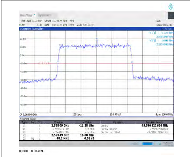
1-N41-30-50-M-5-DFT-256QAM-Outer_Full-128@0-A Ant1-45.591-48.200-≤50-PASS
