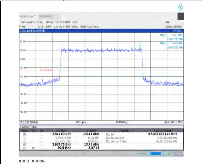
1-N41-30-90-M-8-CP-64QAM-Outer_Full-245@0-An t1-87.337-90.900-≤90-PASS
