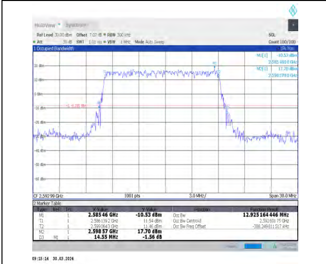
1-N41-30-15-M-2-DFT-PI2BPSK-Outer_Full-36@0-A nt1-12.925-14.550-≤15-PASS
