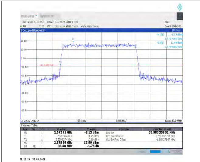
1-N41-30-40-M-4-DFT-64QAM-Outer_Full-100@0-A nt1-35.983-38.480-≤40-PASS
