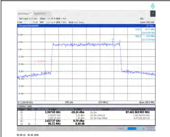
1-N41-30-90-M-9-CP-256QAM-Outer_Full-245@0-A nt1-87.463-90.720-≤90-PASS
