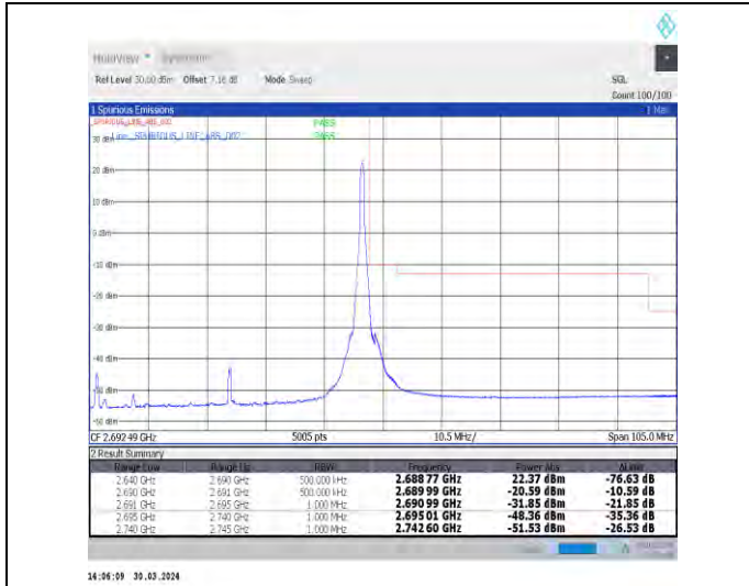
1-N41-30-50-H-2-DFT-PI2BPSK-Edge_1RB_Right-1@132-Ant1-1--PASS-see graph
