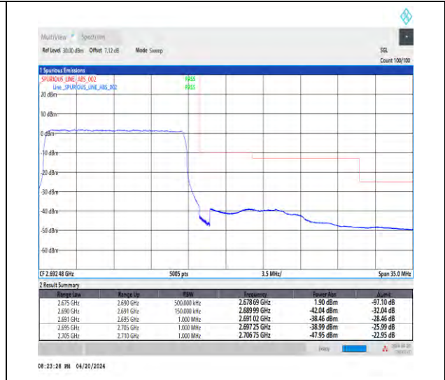
1-N41-30-15-H-3-DFT-PI2BPSK-Outer_Full-36@0-Ant1-1--PASS-see graph
