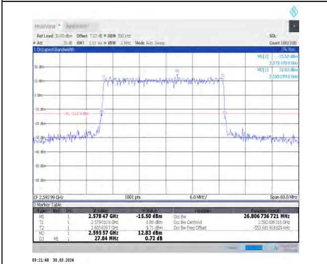
1-N41-30-30-M-4-DFT-64QAM-Outer_Full-75@0-Ant 1-26.808-27.840-≤30-PASS
