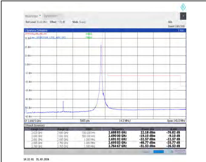
1-N41-30-70-H-2-DFT-PI2BPSK-Edge_1RB_Right-1@188-Ant1-1--PASS-see graph
