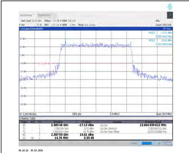
1-N41-30-15-M-8-CP-64QAM-Outer_Full-38@0-Ant1 -13.604-14.760-≤15-PASS
