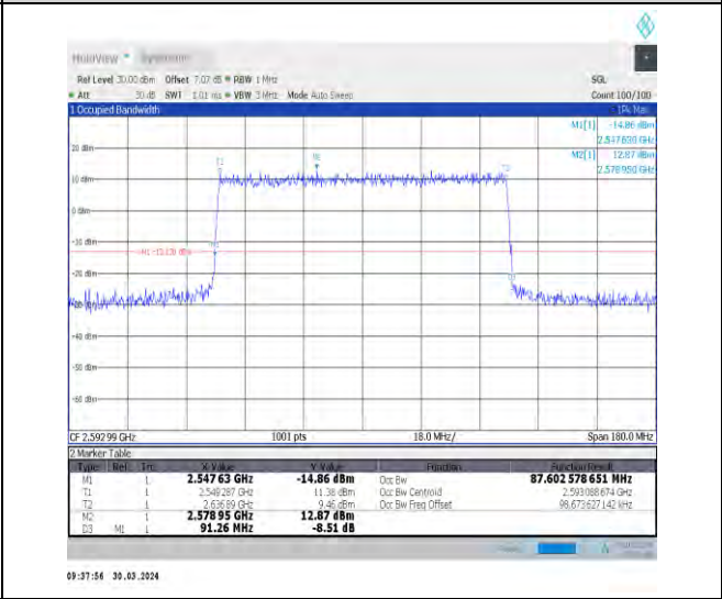
1-N41-30-90-M-6-CP-QPSK-Outer_Full-245@0-Ant1 -87.603-91.260-≤90-PASS
