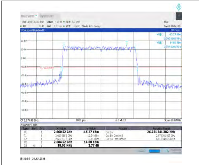
1-N41-30-30-H-1-DFT-QPSK-Outer_Full-75@0-Ant1 -26.752-28.020-≤30-PASS
