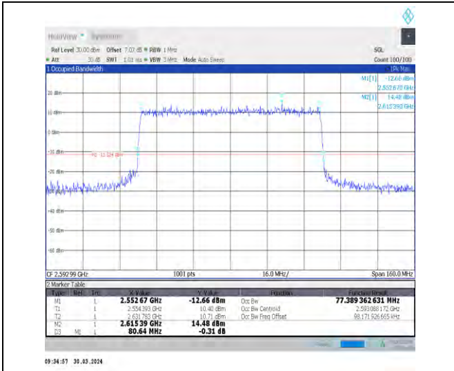
1-N41-30-80-M-8-CP-64QAM-Outer_Full-217@0-Ant 1-77.389-80.640-≤80-PASS
