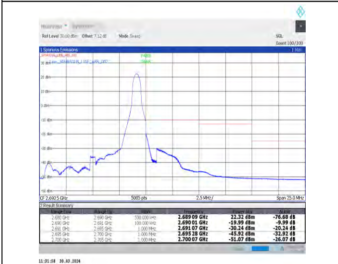
1-N41-30-10-H-5-CP-QPSK-Edge_1RB_Right-1@23-Ant1-1--PASS-see graph
