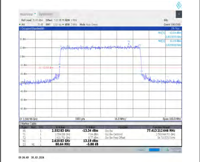
1-N41-30-80-M-7-CP-16QAM-Outer_Full-217@0-Ant1 t1-77.413-80.640-≤80-PASS
