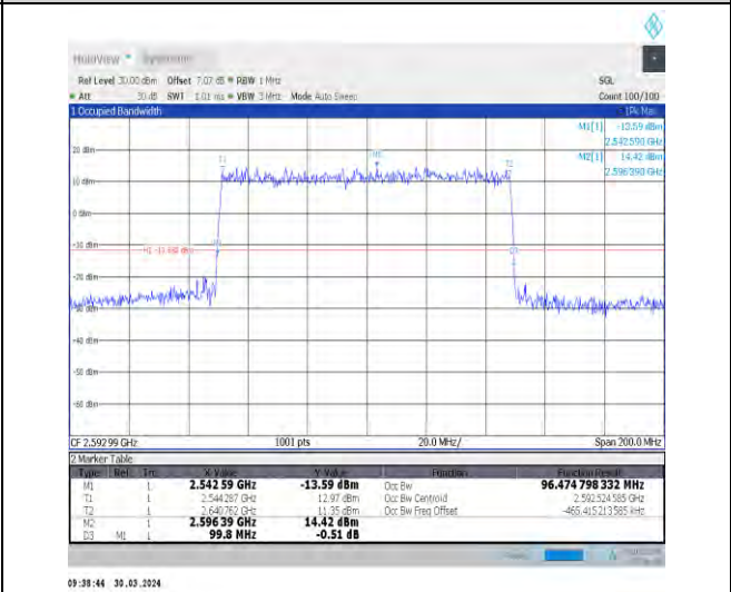
1-N41-30-100-M-1-DFT-QPSK-Outer_Full-270@0-A nt1-96.475-99.800-≤100-PASS
