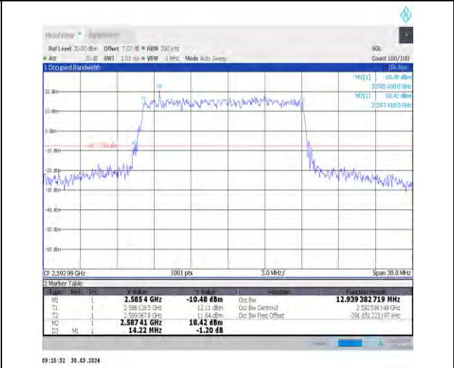
1-N41-30-15-M-3-DFT-16QAM-Outer_Full-36@0-Ant 1-12.939-14.220-≤15-PASS
