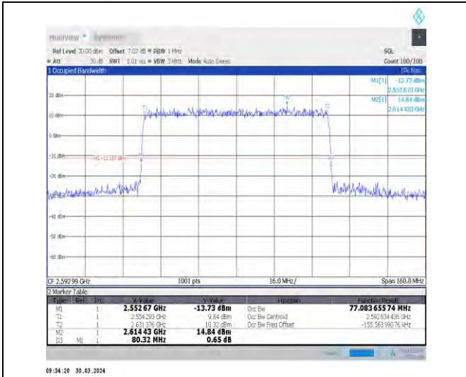
1-N41-30-80-M-4-DFT-64QAM-Outer_Full-216@0-A nt1-77.084-80.320-≤80-PASS
