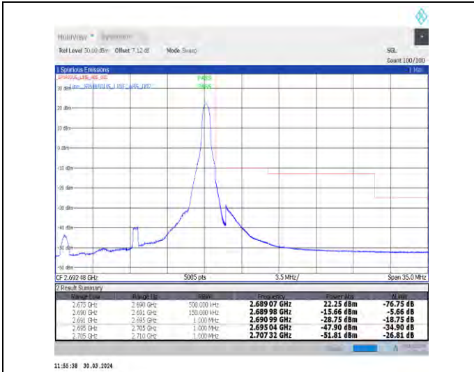
1-N41-30-15-H-2-DFT-PI2BPSK-Edge_1RB_Right-1@37-Ant1-1--PASS-see graph
