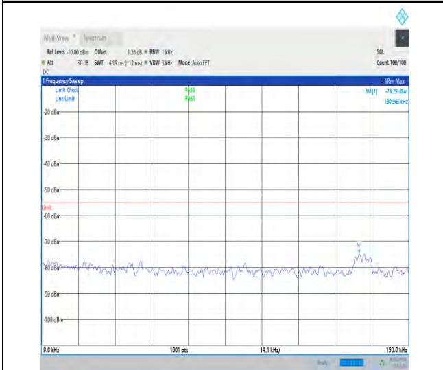
1-N38-30-40-M-1-DFT-PI2BPSK-Inner_1RB_Left-1 @ 1-0.009-0.15-Ant1-0.01--74.79--55-PASS
