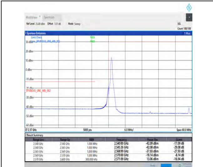
1-N38-30-30-L-1-DFT-PI2BPSK-Edge_1RB_Left-1@0-Ant1-1--PASS-see graph
