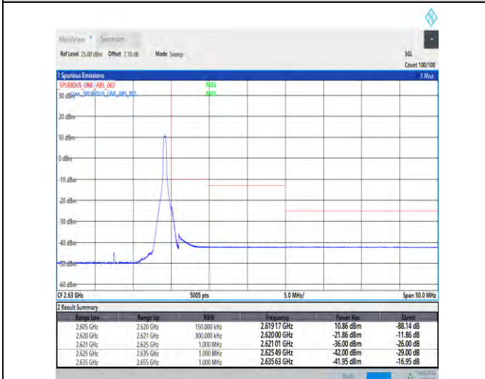
1-N38-30-15-H-5-CP-QPSK-Edge_1RB_Right-1@37-Ant1-1--PASS-see graph
