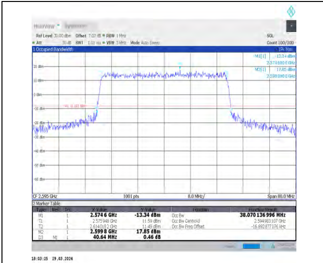
1-N38-30-40-M-8-CP-64QAM-Outer_Full-106@0-Ant 1-38.07-40.640-≤40-PASS
