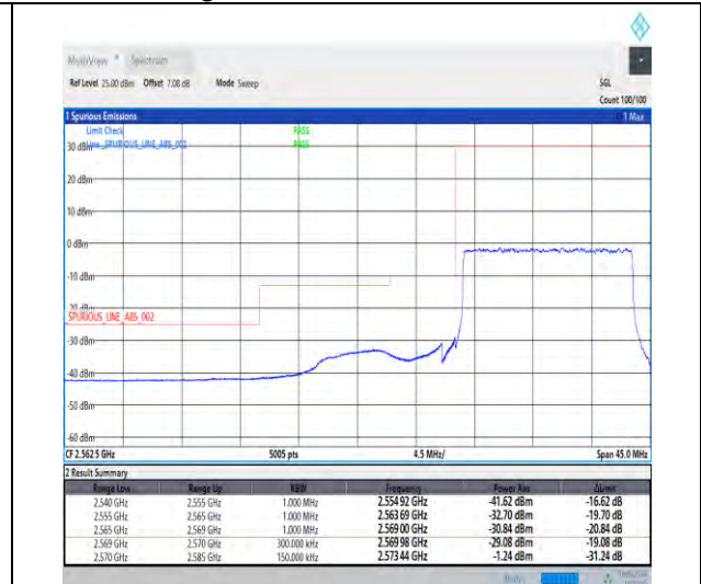
1-N38-30-15-L-3-DFT-PI2BPSK-Outer_Full-36@0-Ant1-1--PASS-see graph
