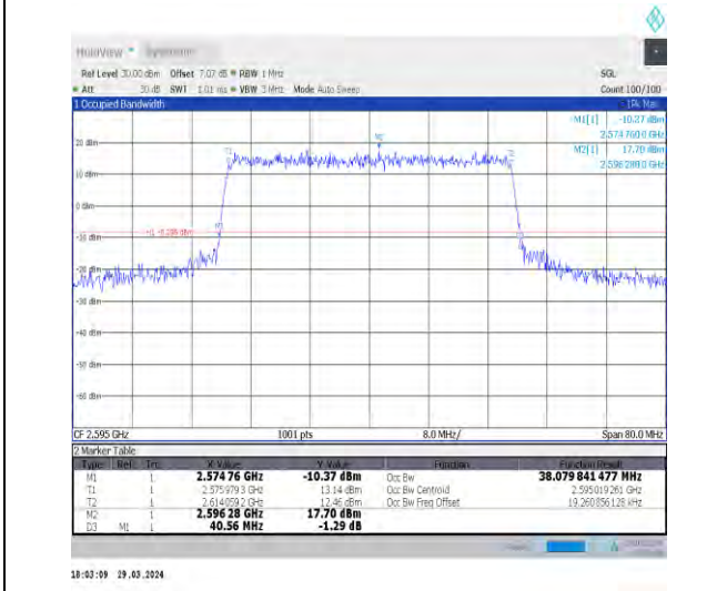
1-N38-30-40-M-6-CP-QPSK-Outer_Full-106@0-Ant1 -38.08-40.560-≤40-PASS
