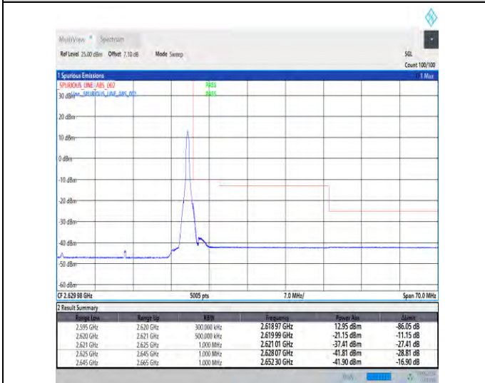
1-N38-30-25-H-5-CP-QPSK-Edge_1RB_Right-1@64-Ant1-1--PASS-see graph
