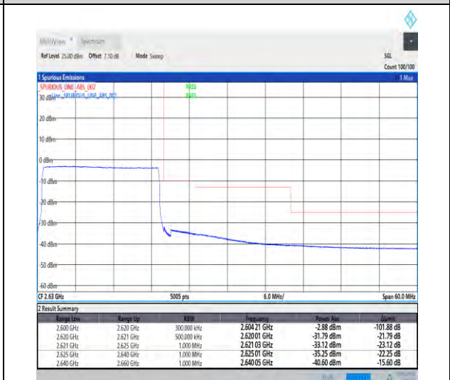
1-N38-30-20-H-6-CP-QPSK-Outer_Full-51@0-Ant1-1--PASS-see graph
