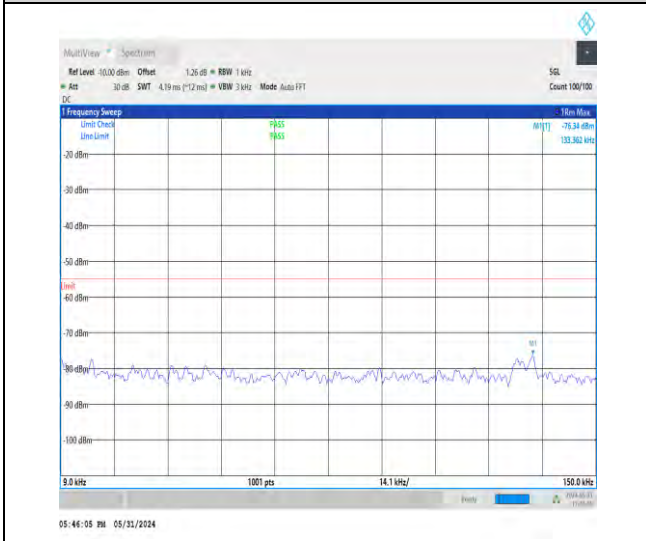
1-N38-30-40-M-1-DFT-PI2BPSK-Inner_1RB_Left-1 @ 1-0.009-0.15-Ant1-0.13--76.34--55-PASS
