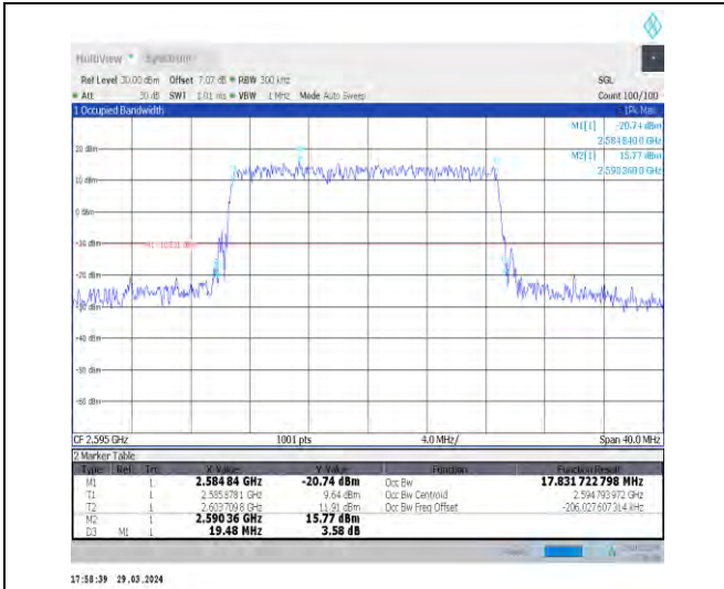
1-N38-30-20-M-3-DFT-16QAM-Outer_Full-50@0-Ant 1-17.832-19.480-≤20-PASS
