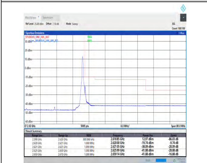
1-N38-30-30-H-5-CP-QPSK-Edge_1RB_Right-1@77-Ant1-1--PASS-see graph
