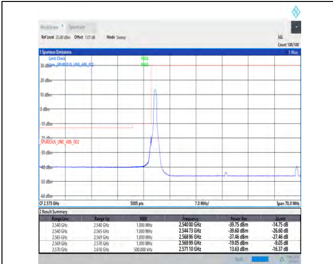
1-N38-30-40-L-1-DFT-PI2BPSK-Edge_1RB_Left-1@0-Ant1-1--PASS-see graph
