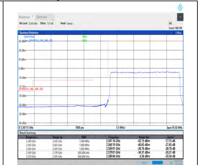
1-N38-30-25-L-3-DFT-PI2BPSK-Outer_Full-64@0-Ant1-1--PASS-see graph
