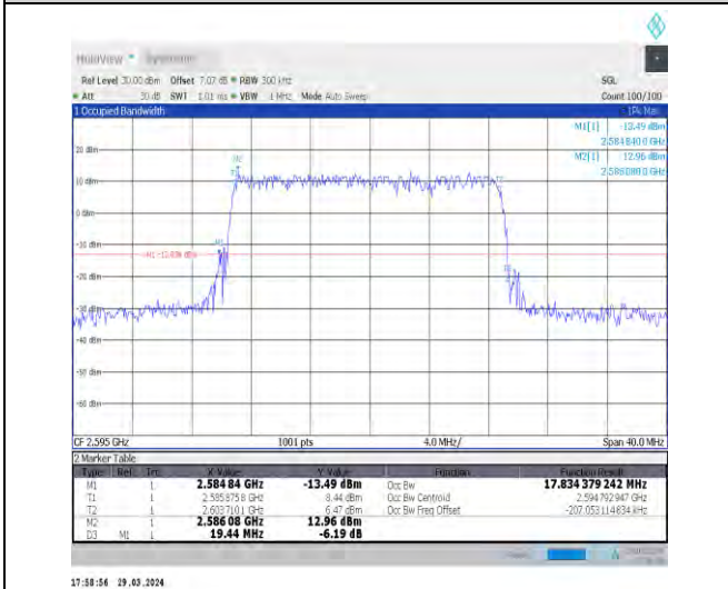
1-N38-30-20-M-5-DFT-256QAM-Outer_Full-50@0-A nt1-17.834-19.440-≤20-PASS
