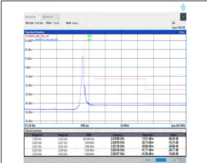
1-N38-30-30-H-2-DFT-PI2BPSK-Edge_1RB_Right-1@77-Ant1-1--PASS-see graph
