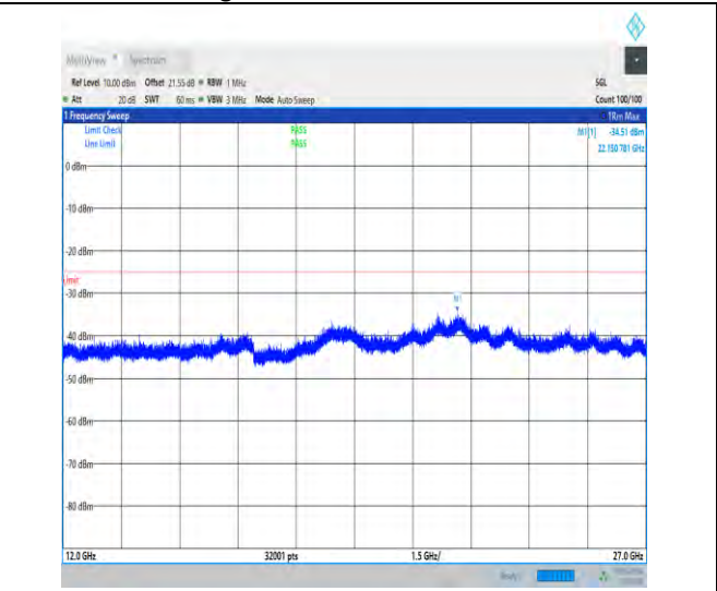
1-N38-30-40-L-1-DFT-PI2BPSK-Inner_1RB_Left-1 @ 1-12000-27000-Ant1-22150.78--34.51--25-PASS
