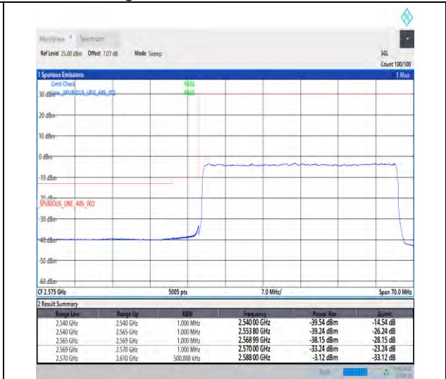
1-N38-30-40-L-3-DFT-PI2BPSK-Outer_Full-100@0-Ant1-1--PASS-see graph
