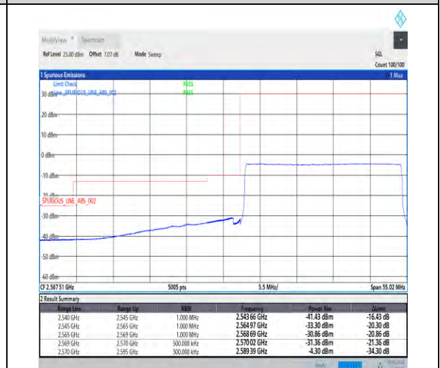
1-N38-30-25-L-6-CP-QPSK-Outer_Full-65@0-Ant1-1--PASS-see graph
