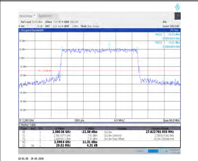
1-N38-30-30-M-8-CP-64QAM-Outer_Full-106@0-Ant 1-38.07-40.640-≤40-PASS
