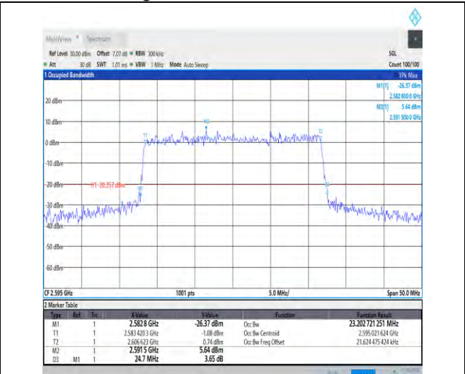
1-N38-30-25-M-7-CP-16QAM-Outer_Full-78@0-Ant1-27.87-29.160-≤30-PASS
