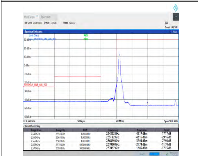
1-N38-30-20-L-4-CP-QPSK-Edge_1RB_Left-1@0-Ant1-1--PASS-see graph
