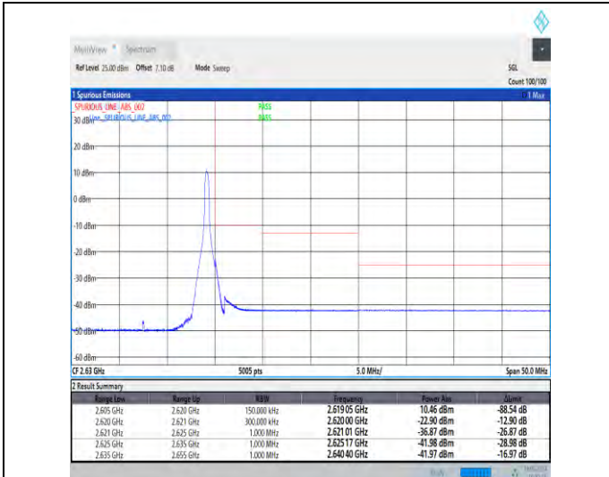
1-N38-30-15-H-2-DFT-PI2BPSK-Edge_1RB_Right-1@37-Ant1-1--PASS-see graph
