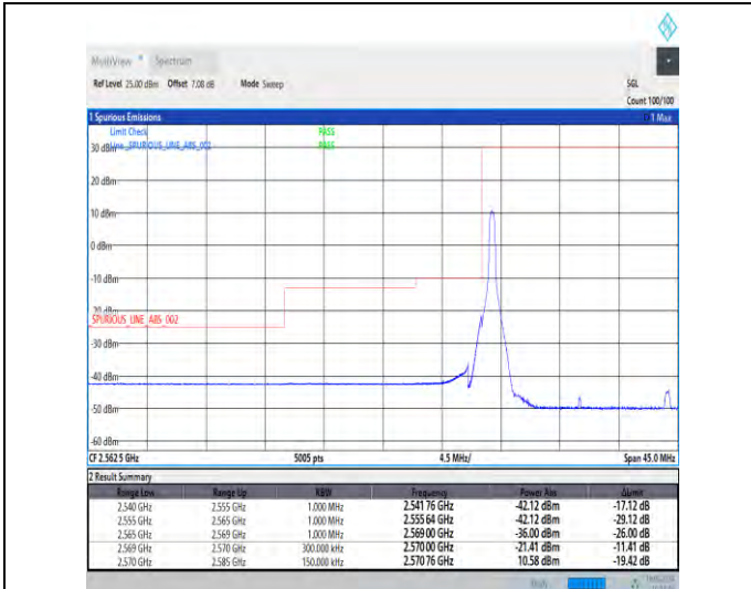
1-N38-30-15-L-1-DFT-PI2BPSK-Edge_1RB_Left-1@0-Ant1-1--PASS-see graph
