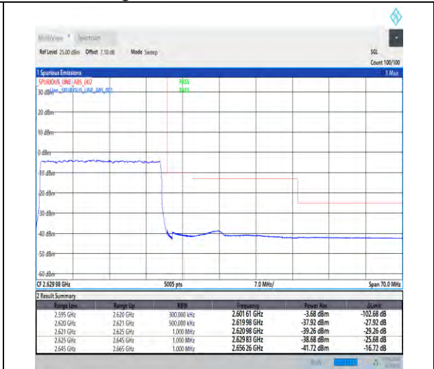
1-N38-30-25-H-3-DFT-PI2BPSK-Outer_Full-64@0-Ant1-1--PASS-see graph
