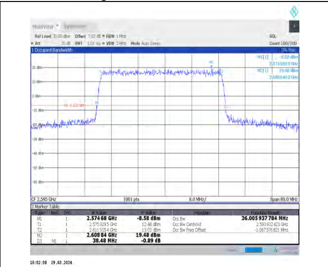
1-N38-30-40-M-1-DFT-QPSK-Outer_Full-100@0-Ant 1-36.006-38.480-≤40-PASS
