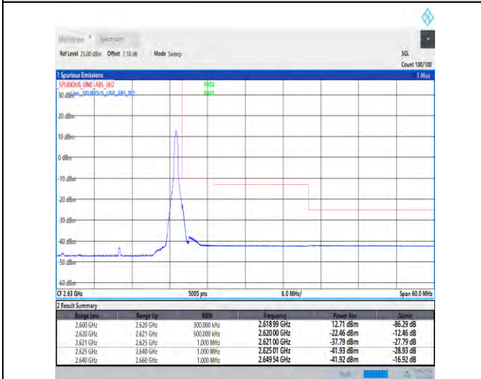
1-N38-30-20-H-5-CP-QPSK-Edge_1RB_Right-1@50-Ant1-1--PASS-see graph
