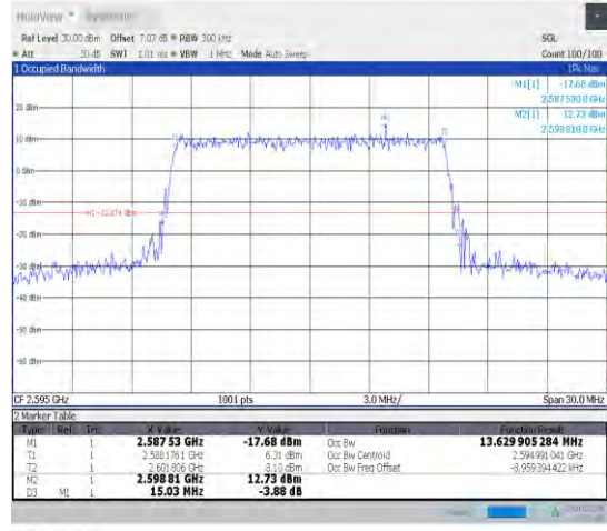
1-N38-30-15-M-9-CP-256QAM-Outer_Full-38@0-Ant1 1-13.63-15.030-≤15-PASS
