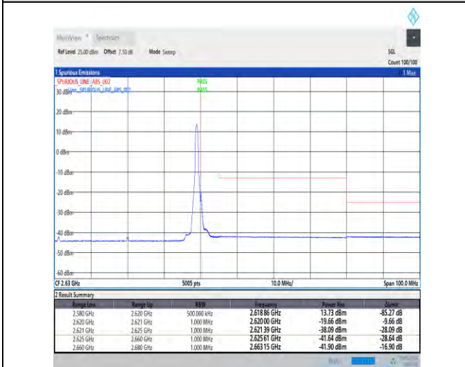
1-N38-30-40-H-5-CP-QPSK-Edge_1RB_Right-1@105-Ant1-1--PASS-see graph
