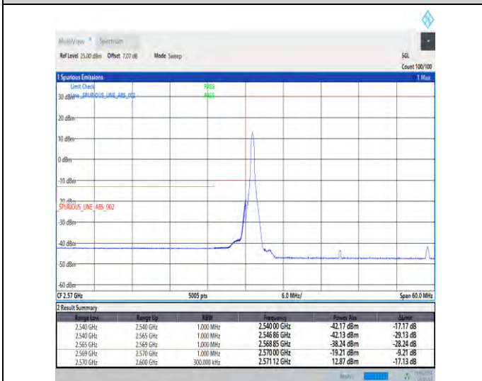
1-N38-30-30-L-4-CP-QPSK-Edge_1RB_Left-1@0-Ant1-1--PASS-see graph
