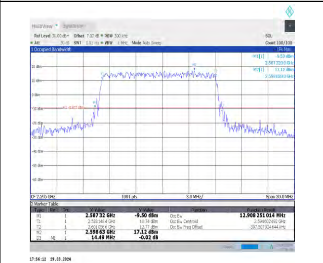
1-N38-30-15-M-3-DFT-16QAM-Outer_Full-36@0-Ant 1-12.908-14.490-≤15-PASS
