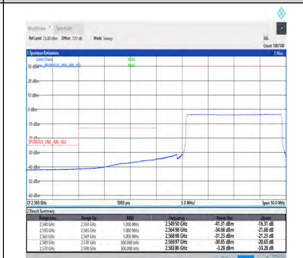
1-N38-30-20-L-6-CP-QPSK-Outer_Full-51@0-Ant1-1--PASS-see graph
