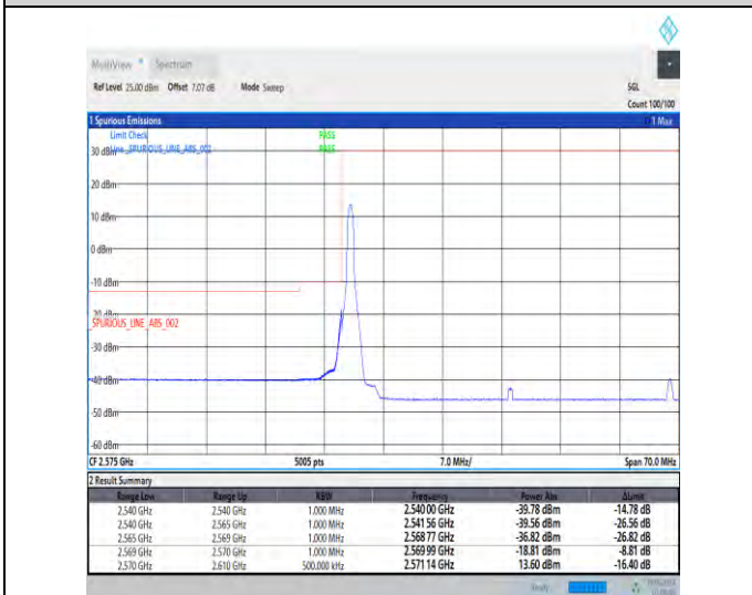
1-N38-30-40-L-4-CP-QPSK-Edge_1RB_Left-1@0-Ant1-1--PASS-see graph
