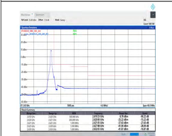
1-N38-30-10-H-5-CP-QPSK-Edge_1RB_Right-1@23-Ant1-1--PASS-see graph
