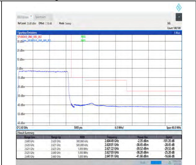
1-N38-30-20-H-3-DFT-PI2BPSK-Outer_Full-50@0-Ant1-1--PASS-see graph
