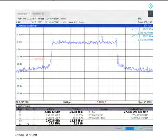
1-N38-30-330-M-6-CP-QPSK-Outer_Full-106@0-Ant 1-38.08-40.560-≤40-PASS
