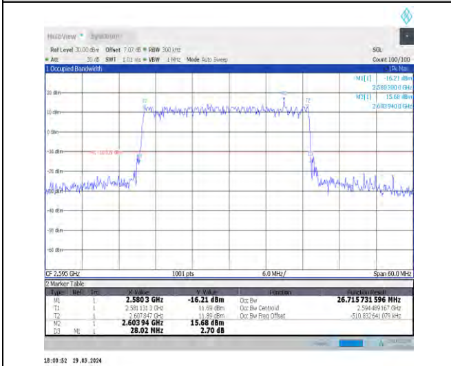
1-N38-30-30-M-3-DFT-16QAM-Outer_Full-100@0-A nt1-35.94-38.640-≤40-PASS
