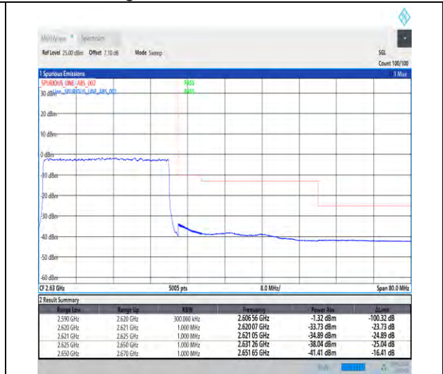
1-N38-30-30-H-3-DFT-PI2BPSK-Outer_Full-75@0-Ant1-1--PASS-see graph
