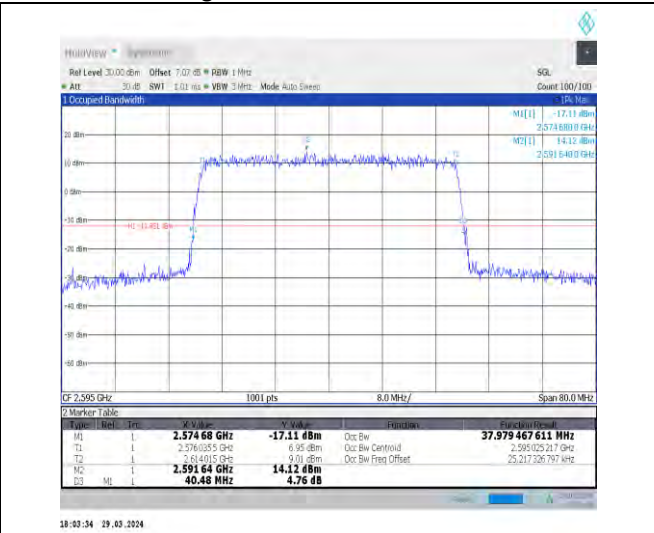
1-N38-30-40-M-9-CP-256QAM-Outer_Full-106@0-Ant nt1-37.979-40.480-≤40-PASS
