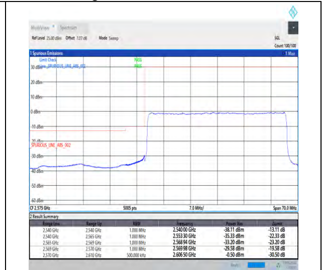
1-N38-30-40-L-3-DFT-PI2BPSK-Outer_Full-100@0-Ant1-1--PASS-see graph
