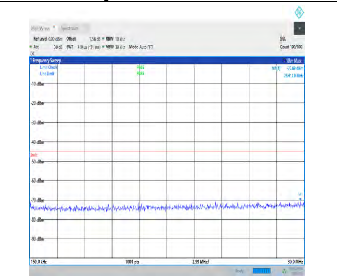
1-N38-30-40-H-1-DFT-PI2BPSK-Inner_1RB_Left-1 @ 1-0.15-30-Ant1-23.43--70.69--45-PASS
