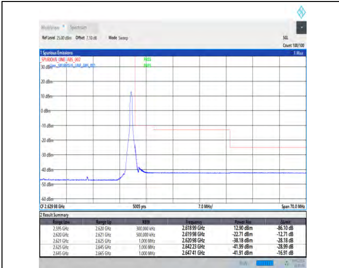
1-N38-30-25-H-2-DFT-PI2BPSK-Edge_1RB_Right-1@64-Ant1-1--PASS-see graph
