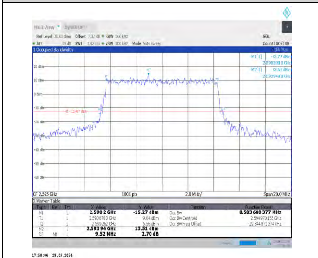
1-N38-30-10-M-7-CP-16QAM-Outer_Full-24@0-Ant1 -8.584-9.520-≤10-PASS
