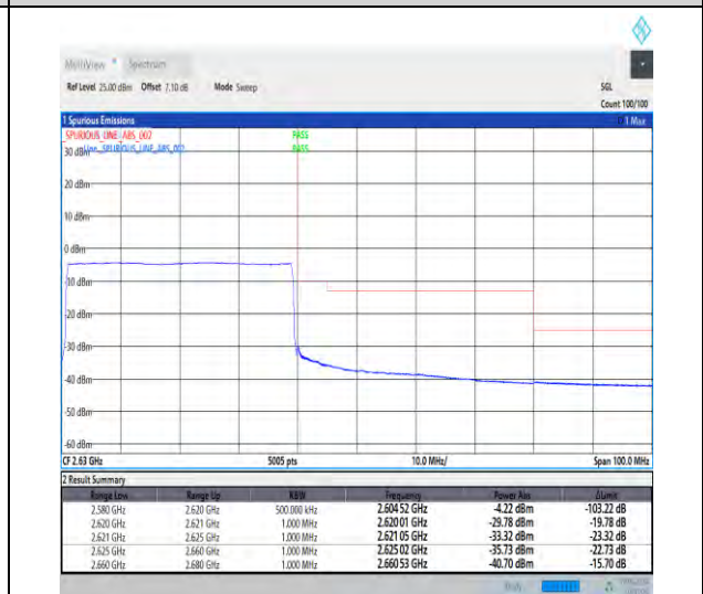
1-N38-30-40-H-6-CP-QPSK-Outer_Full-106@0-Ant1-1--PASS-see graph
