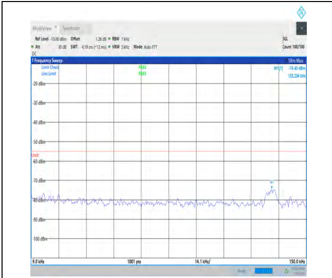
1-N38-30-40-H-1-DFT-PI2BPSK-Inner_1RB_Left-1 @ 1-0.009-0.15-Ant1-0.01--74.45--55-PASS
