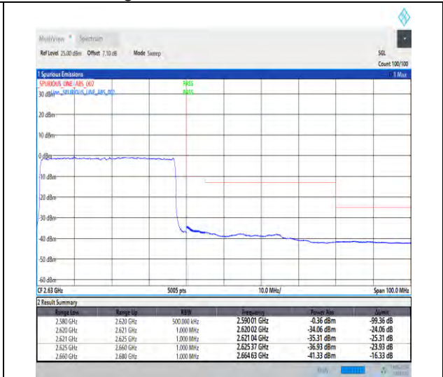
1-N38-30-40-H-3-DFT-PI2BPSK-Outer_Full-100@0-Ant1-1--PASS-see graph
