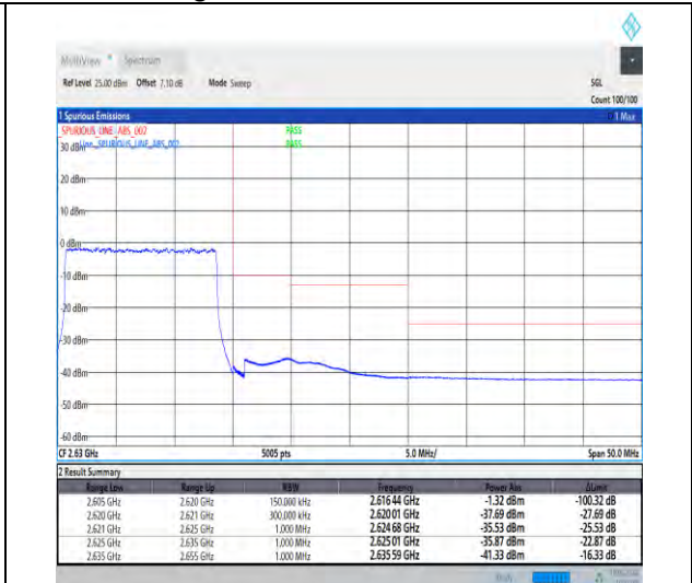
1-N38-30-15-H-3-DFT-PI2BPSK-Outer_Full-36@0-Ant1-1--PASS-see graph
