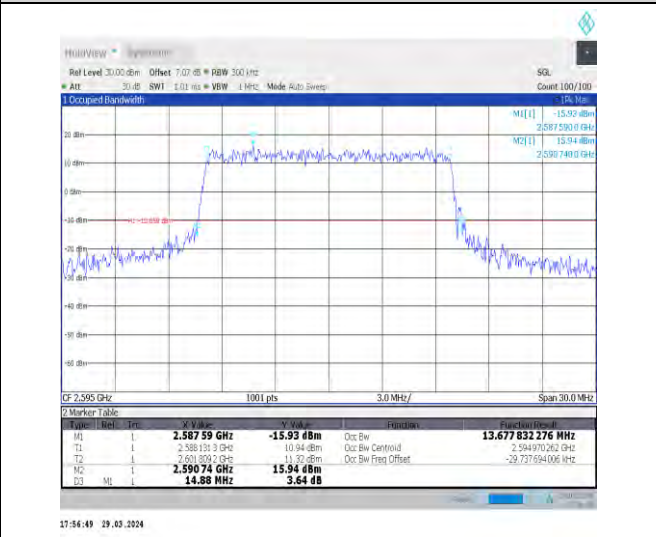
1-N38-30-15-M-7-CP-16QAM-Outer_Full-38@0-Ant1 -13.678-14.880-≤15-PASS
