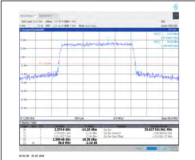
1-N38-30-40-M-4-DFT-64QAM-Outer_Full-100@0-A nt1-35.928-38.800-≤40-PASS
