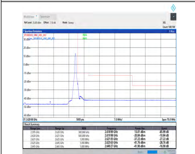
1-N38-30-25-H-5-CP-QPSK-Edge_1RB_Right-1@64-Ant1-1--PASS-see graph
