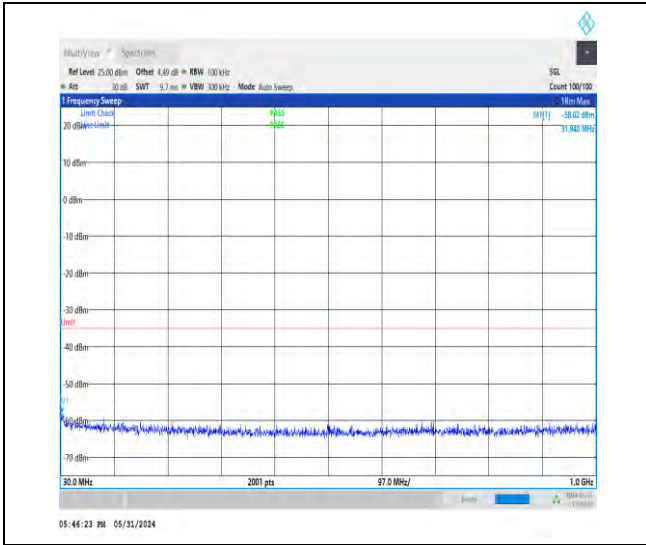
1-N38-30-40-M-1-DFT-PI2BPSK-Inner_1RB_Left-1 @1-30-1000-Ant1-33.88--58.02--35-PASS
