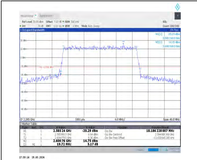
1-N38-30-20-M-7-CP-16QAM-Outer_Full-51@0-Ant1 -18.186-19.720-≤20-PASS
