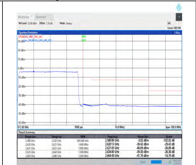
1-N38-30-40-H-3-DFT-PI2BPSK-Outer_Full-100@0-Ant1-1--PASS-see graph
