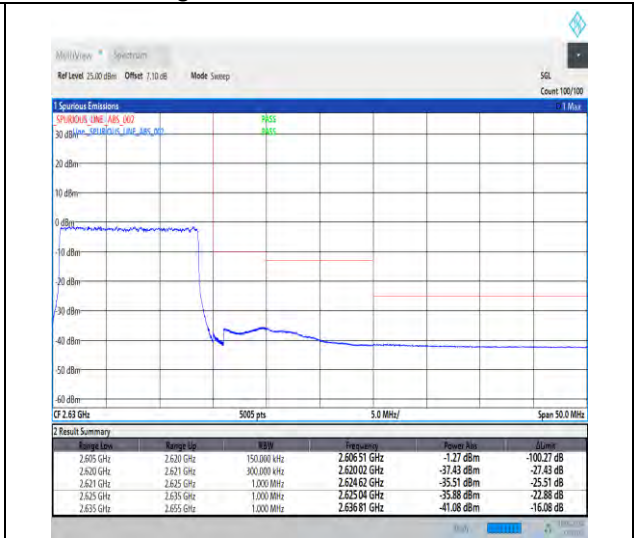
1-N38-30-15-H-3-DFT-PI2BPSK-Outer_Full-36@0-Ant1-1--PASS-see graph
