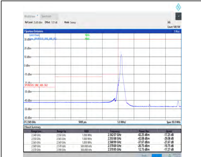
1-N38-30-20-L-1-DFT-PI2BPSK-Edge_1RB_Left-1@0-Ant1-1--PASS-see graph
