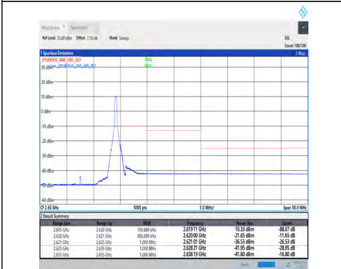
1-N38-30-15-H-5-CP-QPSK-Edge_1RB_Right-1@37-Ant1-1--PASS-see graph
