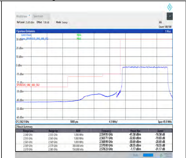
1-N38-30-15-L-3-DFT-PI2BPSK-Outer_Full-36@0-Ant1-1--PASS-see graph
