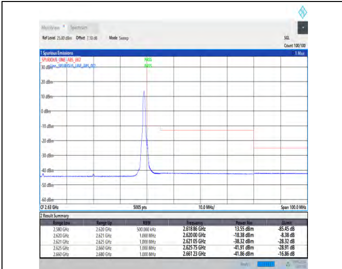
1-N38-30-40-H-2-DFT-PI2BPSK-Edge_1RB_Right-1@105-Ant1-1--PASS-see graph
