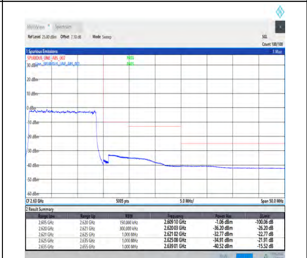
1-N38-30-15-H-6-CP-QPSK-Outer_Full-38@0-Ant1-1--PASS-see graph
