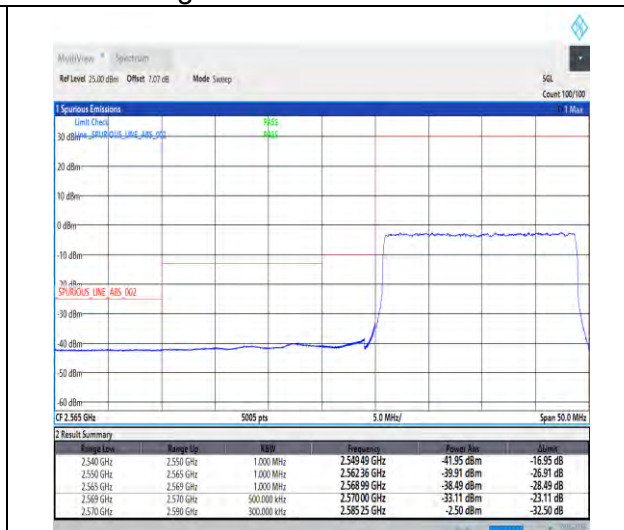
1-N38-30-20-L-3-DFT-PI2BPSK-Outer_Full-50@0-Ant1-1--PASS-see graph
