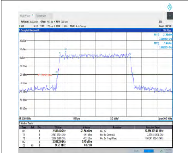
1-N38-30-25-M-4-DFT-64QAM-Outer_Full-75@0-Ant 1-26.738-28.200-≤30-PASS
