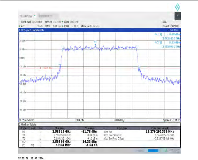
1-N38-30-20-M-6-CP-QPSK-Outer_Full-51@0-Ant1 18.279-19.640-≤20-PASS
