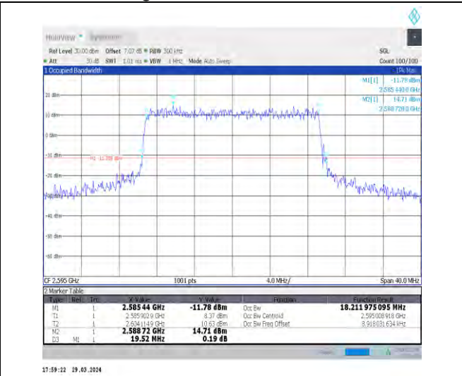
1-N38-30-20-M-8-CP-64QAM-Outer_Full-51@0-Ant1 -18.212-19.520-≤20-PASS
