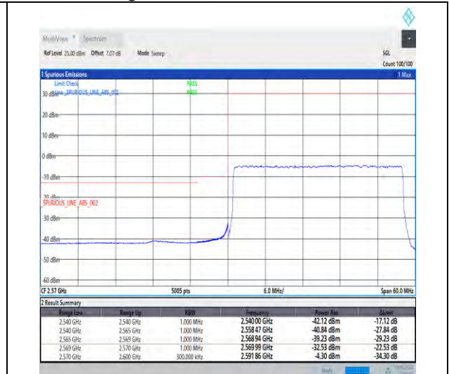
1-N38-30-30-L-3-DFT-PI2BPSK-Outer_Full-75@0-Ant1-1--PASS-see graph
