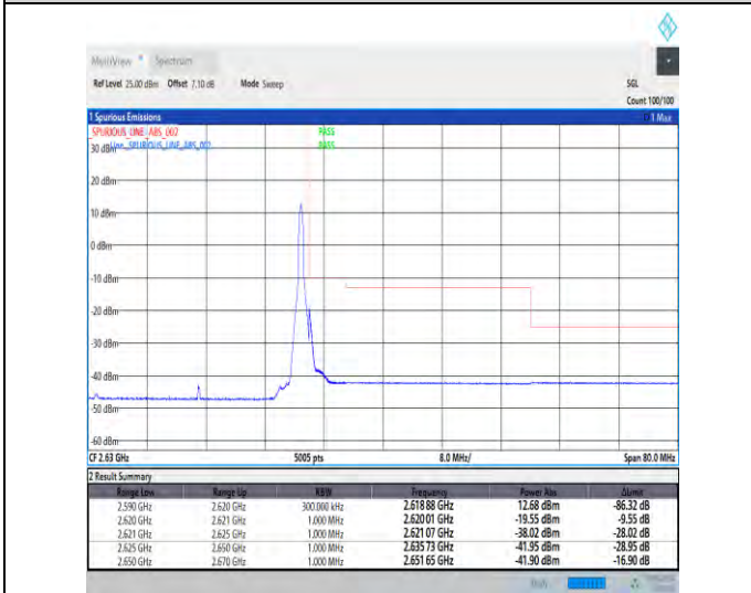
1-N38-30-30-H-5-CP-QPSK-Edge_1RB_Right-1@77-Ant1-1--PASS-see graph
