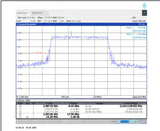
1-N38-30-15-M-4-DFT-64QAM-Outer_Full-36@0-Ant 1-12.914-14.280-≤15-PASS
