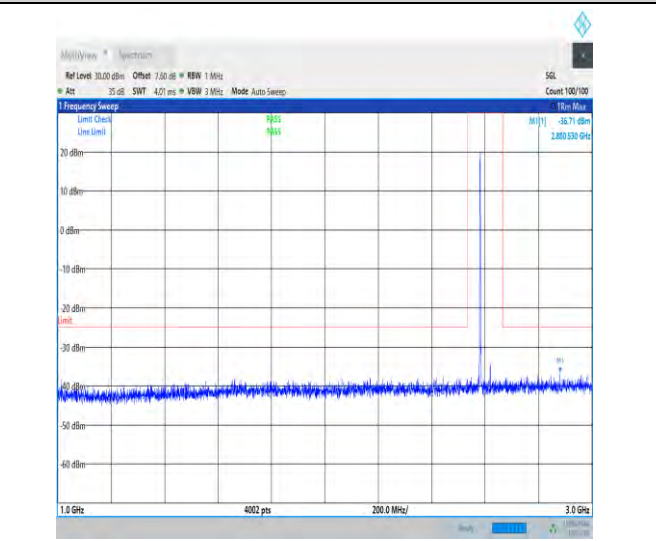
1-N38-30-40-H-1-DFT-PI2BPSK-Inner_1RB_Left-1 @ 1-1000-3000-Ant1-2778.00--36.71--25-PASS
