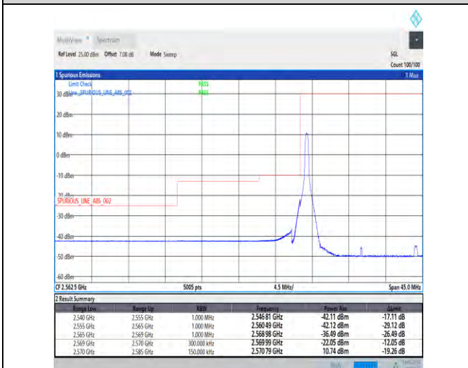
1-N38-30-15-L-4-CP-QPSK-Edge_1RB_Left-1@0-Ant1-1--PASS-see graph
