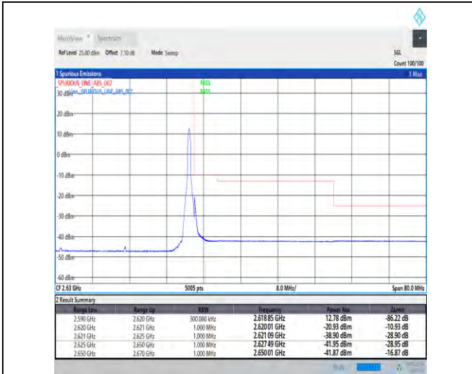
1-N38-30-30-H-2-DFT-PI2BPSK-Edge_1RB_Right-1@77-Ant1-1--PASS-see graph
