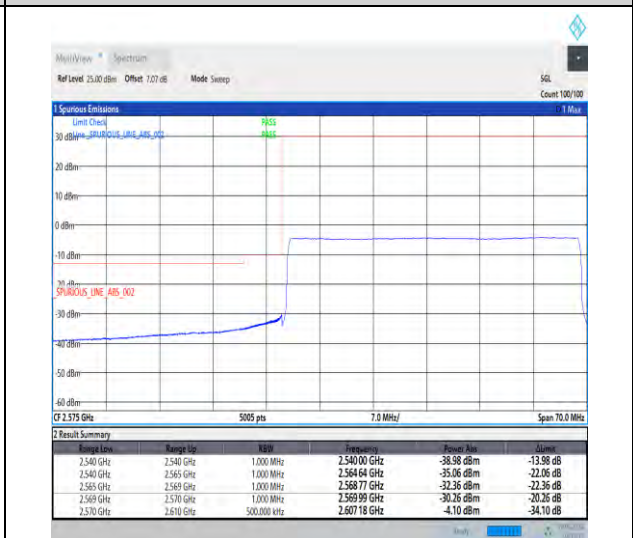
1-N38-30-40-L-6-CP-QPSK-Outer_Full-106@0-Ant1-1--PASS-see graph
