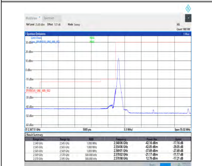
1-N38-30-25-L-4-CP-QPSK-Edge_1RB_Left-1@0-Ant1-1--PASS-see graph
