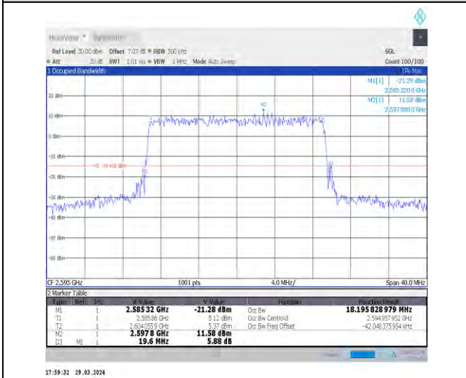
1-N38-30-20-M-9-CP-256QAM-Outer_Full-51@0-Ant 1-18.196-19.600-≤20-PASS
