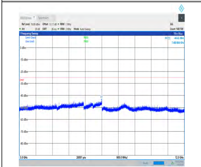
1-N38-30-40-M-1-DFT-PI2BPSK-Inner_1RB_Left-1 @ 1-3000-12000-Ant1-3629.55--44.42--25-PASS
