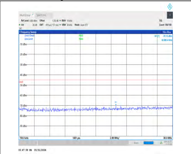
1-N38-30-40-H-1-DFT-PI2BPSK-Inner_1RB_Left-1 @ 1-0.15-30-Ant1-23.97--70.15--45-PASS
