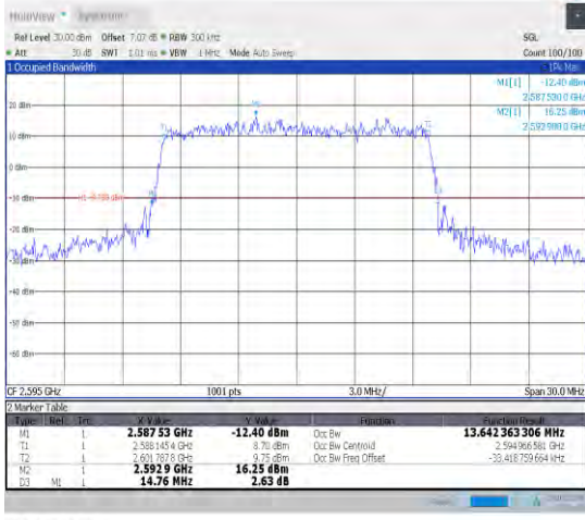
1-N38-30-15-M-8-CP-64QAM-Outer_Full-38@0-Ant1 -13.642-14.760-≤15-PASS
