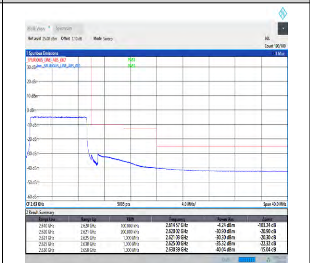
1-N38-30-10-H-6-CP-QPSK-Outer_Full-24@0-Ant1-1--PASS-see graph
