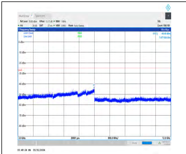
1-N38-30-40-H-1-DFT-PI2BPSK-Inner_1RB_Left-1 @1-3000-12000-Ant1-7477.05--44.40--25-PASS
