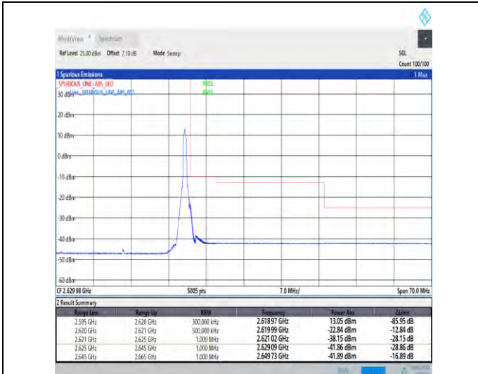
1-N38-30-25-H-2-DFT-PI2BPSK-Edge_1RB_Right-1@64-Ant1-1--PASS-see graph
