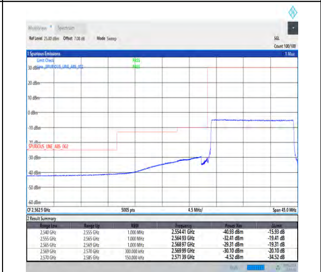
1-N38-30-15-L-6-CP-QPSK-Outer_Full-38@0-Ant1-1--PASS-see graph
