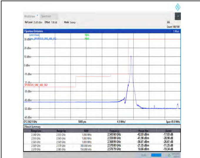
1-N38-30-15-L-1-DFT-PI2BPSK-Edge_1RB_Left-1@0-Ant1-1--PASS-see graph
