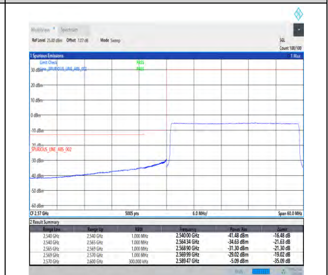
1-N38-30-30-L-6-CP-QPSK-Outer_Full-78@0-Ant1-1--PASS-see graph
