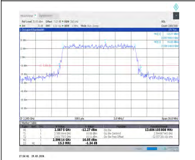
1-N38-30-15-M-6-CP-QPSK-Outer_Full-38@0-Ant1 13.606-15.300-≤15-PASS
