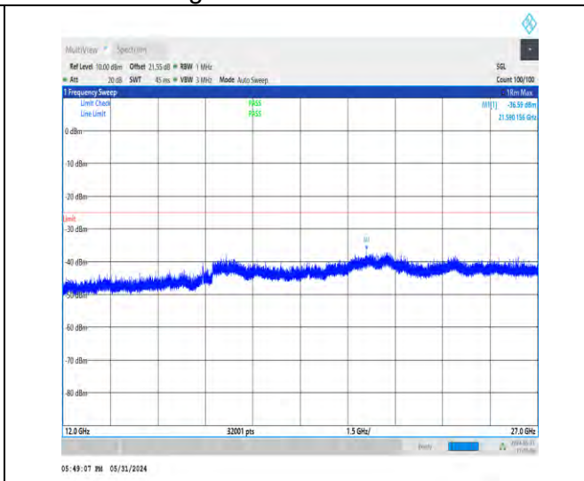
1-N38-30-40-H-1-DFT-PI2BPSK-Inner_1RB_Left-1@ 1-12000-27000-Ant1-21590.16--36.59--25-PASS
