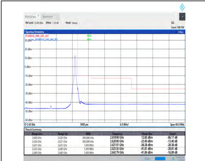
1-N38-30-20-H-2-DFT-PI2BPSK-Edge_1RB_Right-1@50-Ant1-1--PASS-see graph
