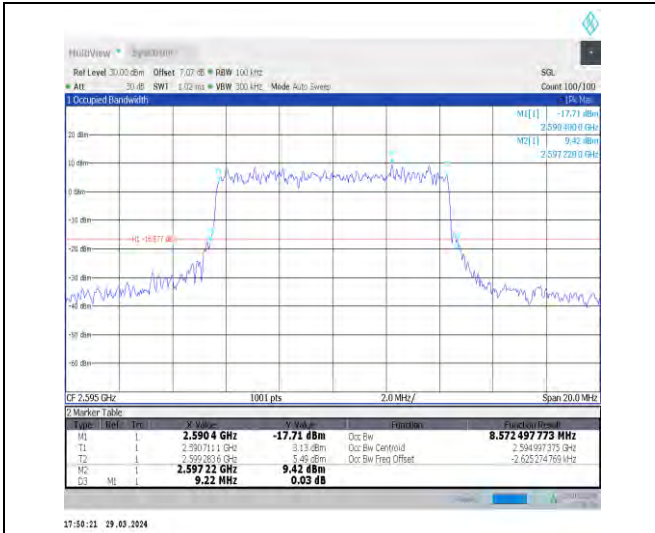
1-N38-30-10-M-9-CP-256QAM-Outer_Full-24@0-Ant 1-8.572-9.220-≤10-PASS
