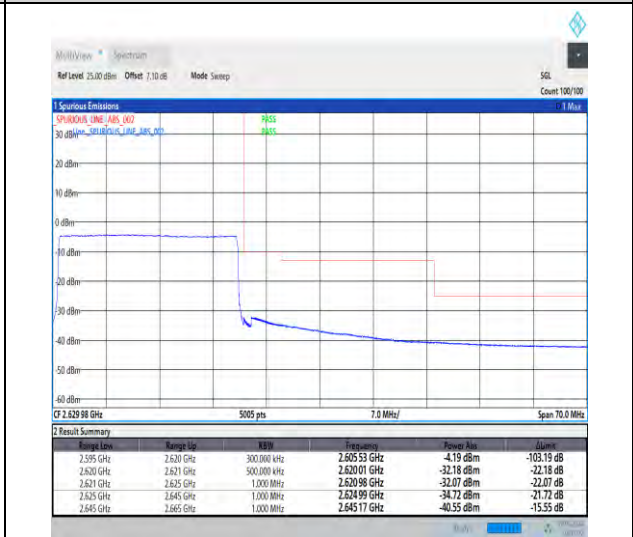
1-N38-30-25-H-6-CP-QPSK-Outer_Full-65@0-Ant1-1--PASS-see graph
