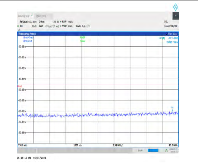
1-N38-30-40-M-1-DFT-PI2BPSK-Inner_1RB_Left-1 @ 1-0.15-30-Ant1-28.39--70.15--45-PASS
