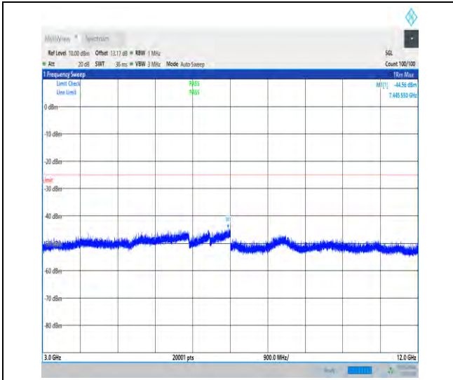
1-N38-30-40-L-1-DFT-PI2BPSK-Inner_1RB_Left-1 @ 1-3000-12000-Ant1-7445.55--44.56--25-PASS
