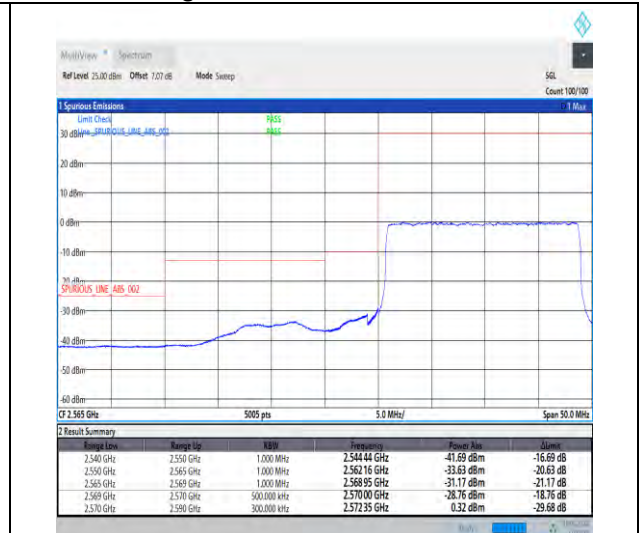
1-N38-30-20-L-3-DFT-PI2BPSK-Outer_Full-50@0-Ant1-1--PASS-see graph
