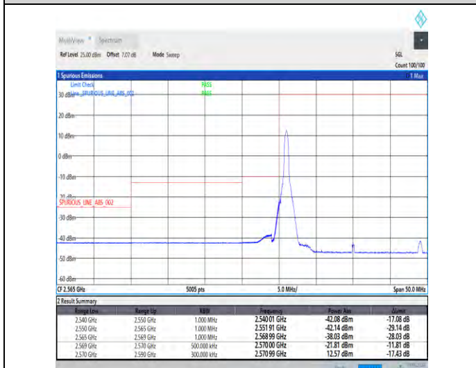
1-N38-30-20-L-4-CP-QPSK-Edge_1RB_Left-1@0-Ant1-1--PASS-see graph
