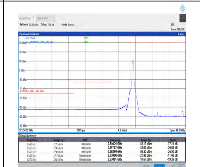
1-N38-30-15-L-6-CP-QPSK-Outer_Full-38@0-Ant1-1--PASS-see graph
