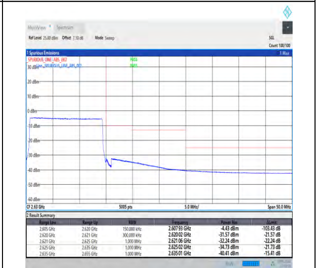
1-N38-30-15-H-6-CP-QPSK-Outer_Full-38@0-Ant1-1--PASS-see graph
