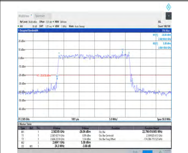
1-N38-30-25-M-1-DFT-QPSK-Outer_Full-75@0-Ant1 -26.785-27.720-≤30-PASS
