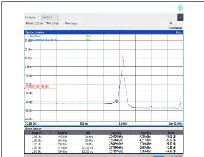
1-N38-30-20-L-1-DFT-PI2BPSK-Edge_1RB_Left-1@0-Ant1-1--PASS-see graph
