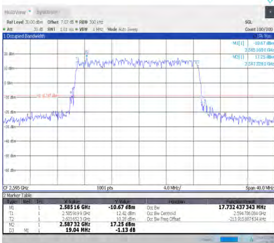
1-N38-30-20-M-1-DFT-QPSK-Outer_Full-50@0-Ant1 -17.732-19.040-≤20-PASS
