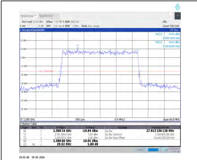
1-N38-30-30-M-9-CP-256QAM-Outer_Full-106@0-A nt1-37.979-40.480-≤40-PASS
