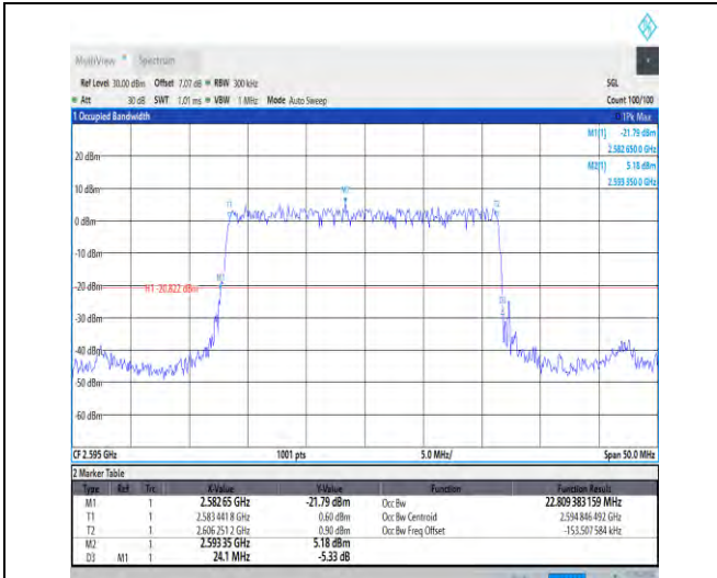
1-N38-30-25-M-2-DFT-PI2BPSK-Outer_Full-75@0-A nt1-26.635-28.380-≤30-PASS
