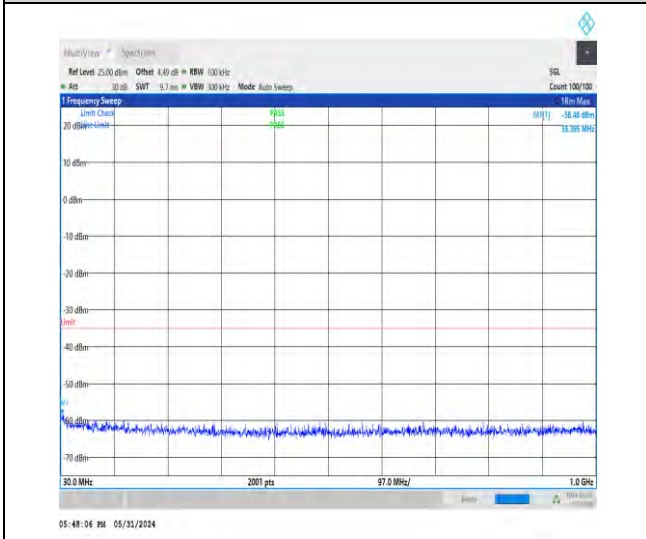
1-N38-30-40-H-1-DFT-PI2BPSK-Inner_1RB_Left-1 @ 1-30-1000-Ant1-32.91--58.48--35-PASS
