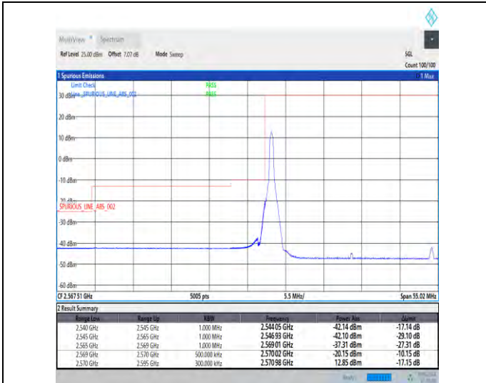
1-N38-30-25-L-1-DFT-PI2BPSK-Edge_1RB_Left-1@0-Ant1-1--PASS-see graph
