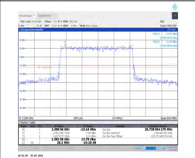
1-N38-30-30-M-4-DFT-64QAM-Outer_Full-100@0-A nt1-35.928-38.800-≤40-PASS
