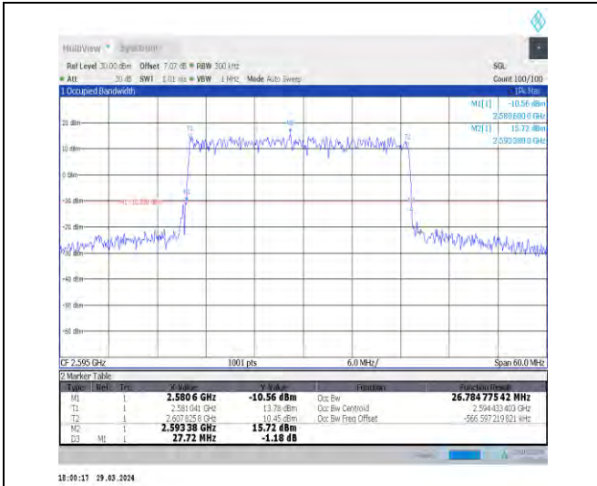
1-N38-30-30-M-1-DFT-QPSK-Outer_Full-100@0-Ant 1-36.006-38.480-≤40-PASS
