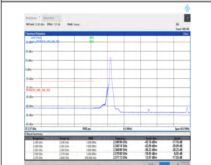
1-N38-30-30-L-4-CP-QPSK-Edge_1RB_Left-1@0-Ant1-1--PASS-see graph
