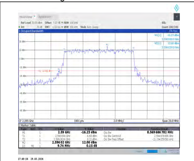
1-N38-30-10-M-6-CP-QPSK-Outer_Full-24@0-Ant1- 8.57-9.740-≤10-PASS
