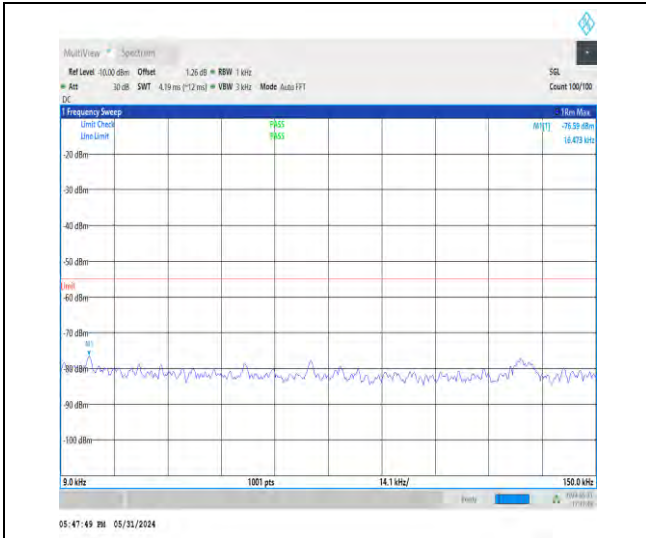
1-N38-30-40-H-1-DFT-PI2BPSK-Inner_1RB_Left-1 @ 1-0.009-0.15-Ant1-0.01--76.59--55-PASS
