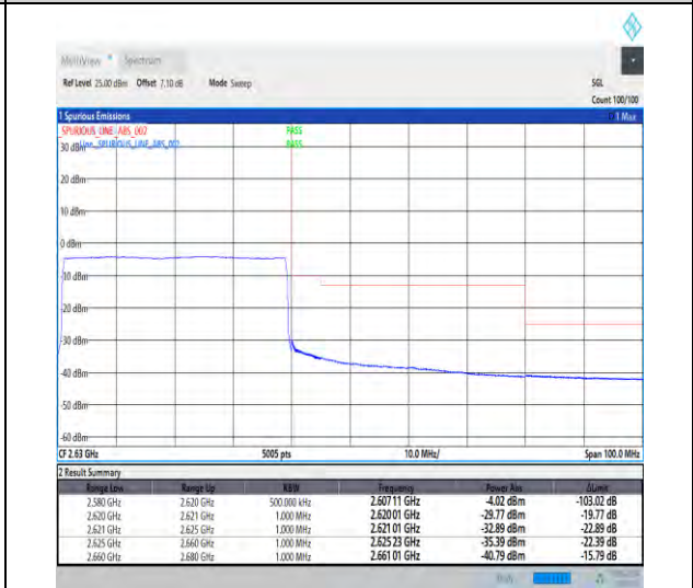
1-N38-30-40-H-6-CP-QPSK-Outer_Full-106@0-Ant1-1--PASS-see graph
