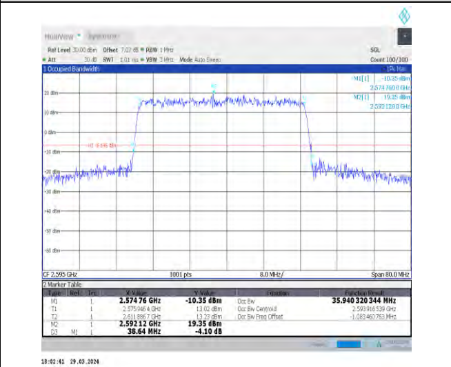
1-N38-30-40-M-3-DFT-16QAM-Outer_Full-100@0-A nt1-35.94-38.640-≤40-PASS
