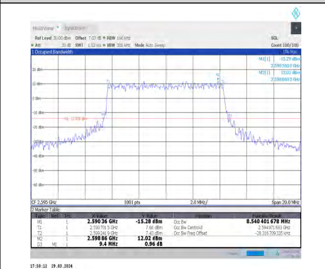
1-N38-30-10-M-8-CP-64QAM-Outer_Full-24@0-Ant1 -8.54-9.400-≤10-PASS
