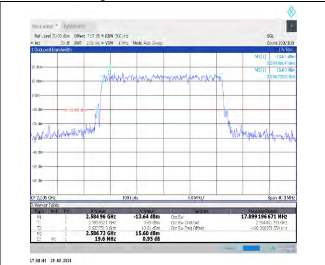
1-N38-30-20-M-4-DFT-64QAM-Outer_Full-50@0-Ant 1-17.899-19.600-≤20-PASS
