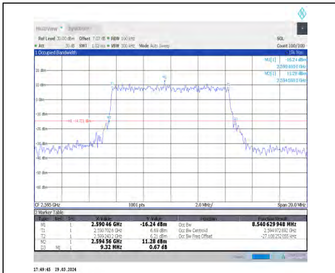
1-N38-30-10-M-5-DFT-256QAM-Outer_Full-24@0-A nt1-8.541-9.320-≤10-PASS
