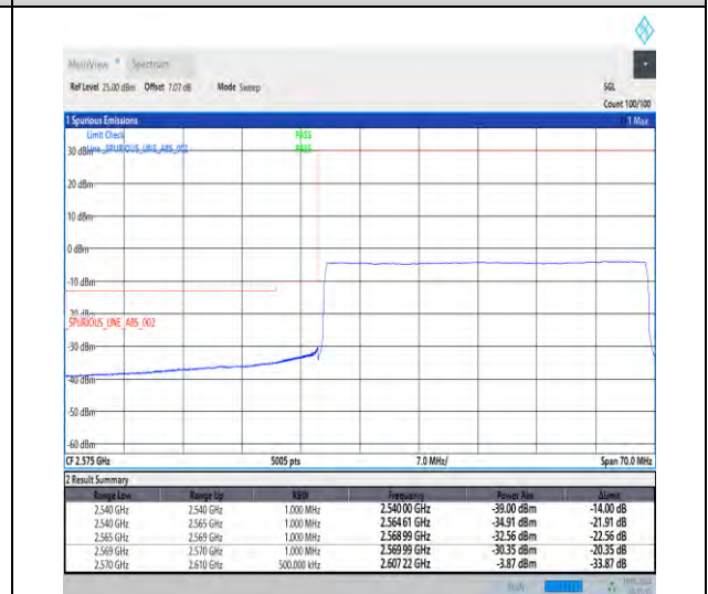
1-N38-30-40-L-6-CP-QPSK-Outer_Full-106@0-Ant1-1--PASS-see graph
