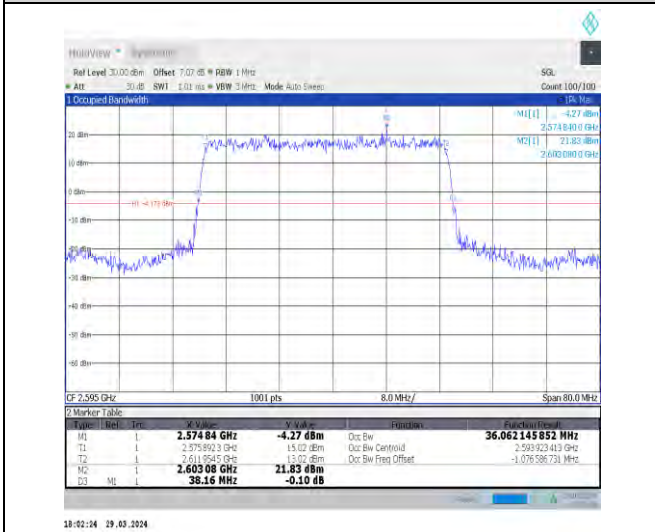
1-N38-30-40-M-2-DFT-PI2BPSK-Outer_Full-100@0-Ant1 Ant1-36.062-38.160-≤40-PASS
