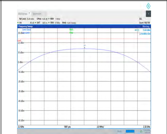
1-N30-15-10-L-3-DFT-PI2BPSK-Outer_Full-50@0-23 00-2320-Ant1-2310.08-13.69-23.98-PASS
