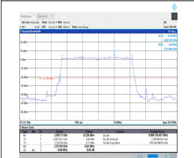
1-N30-15-10-M-2-DFT-PI2BPSK-Outer_Full-50@0-Ant1 -8.907-9.480-≤10-PASS
