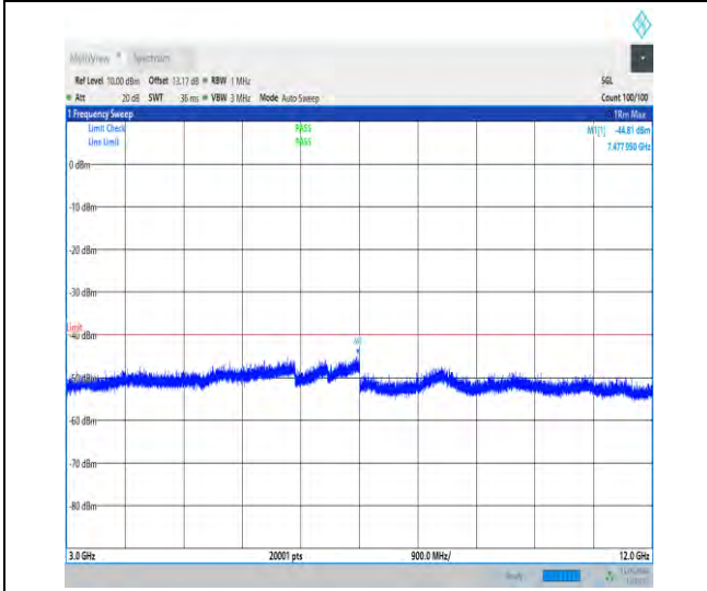
1-N30-15-10-M-1-DFT-PI2BPSK-Inner_1RB_Left-1 @1-3000-12000-Ant1-7477.95--44.81--40-PASS
