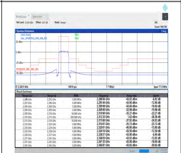
1-N30-15-5-H-6-CP-QPSK-Outer_Full-25@0-Ant1-1--PASS-see graph
