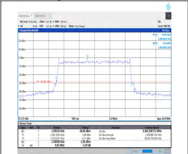
1-N30-15-10-M-9-CP-256QAM-Outer_Full-52@0-An t1-9.302-9.820-≤10-PASS
