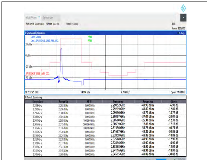
1-N30-15-10-L-1-DFT-PI2BPSK-Edge_1RB_Left-1@0-Ant1-1--PASS-see graph
