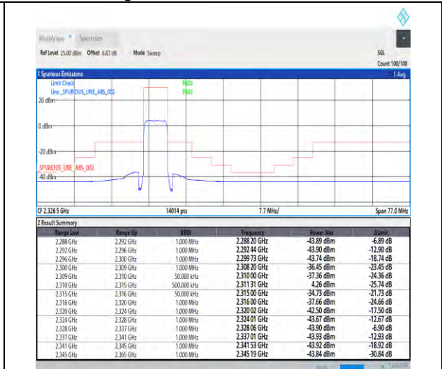
1-N30-15-5-H-3-DFT-PI2BPSK-Outer_Full-25@0-Ant1-1--PASS-see graph
