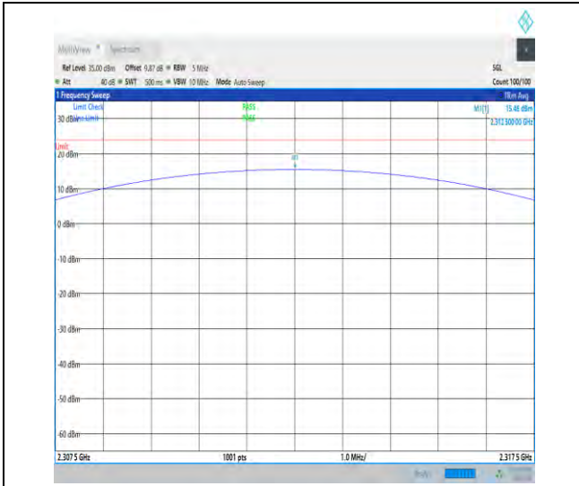
1-N30-15-5-H-3-DFT-PI2BPSK-Outer_Full-25@0-23 07.5-2317.5-Ant1-2312.50-15.48-23.98-PASS
