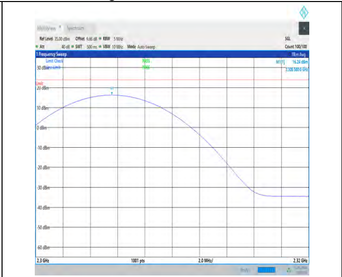
1-N30-15-10-L-1-DFT-PI2BPSK-Inner_1RB_Left-1@ 1-2300-2320-Ant1-2305.58-16.24-23.98-PASS
