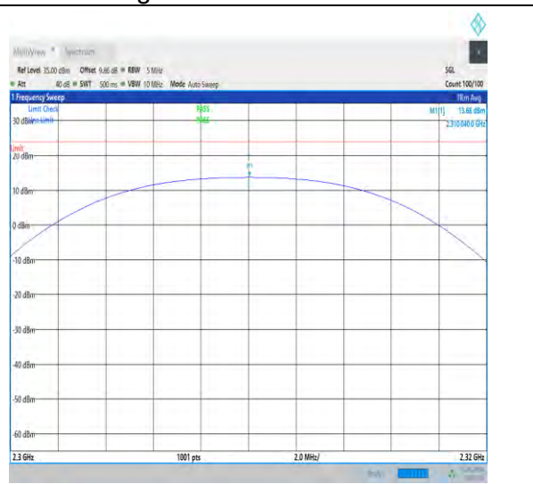
1-N30-15-10-H-3-DFT-PI2BPSK-Outer_Full-50@0-23 00-2320-Ant1-2310.04-13.68-23.98-PASS
