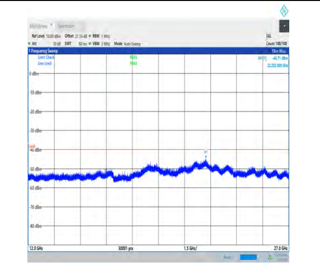
1-N30-15-10-M-1-DFT-PI2BPSK-Inner_1RB_Left-1@ 1-12000-27000-Ant1-22232.00--44.71--40-PASS
