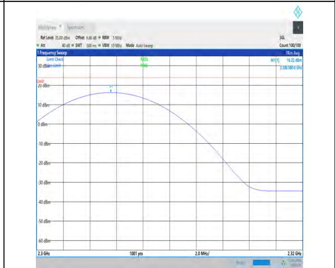
1-N30-15-10-H-1-DFT-PI2BPSK-Inner_1RB_Left-1@ 1-2300-2320-Ant1-2305.58-16.22-23.98-PASS
