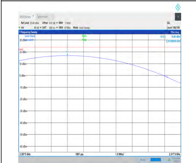
1-N30-15-5-H-1-DFT-PI2BPSK-Inner_1RB_Left-1@ 1-2307.5-2317.5-Ant1-2310.50-16.80-23.98-PASS
