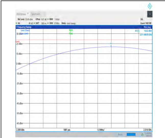
1-N30-15-5-M-2-DFT-PI2BPSK-Inner_1RB_Right-1 @23-2305-2315-Ant1-2311.98-16.82-23.98-PASS
