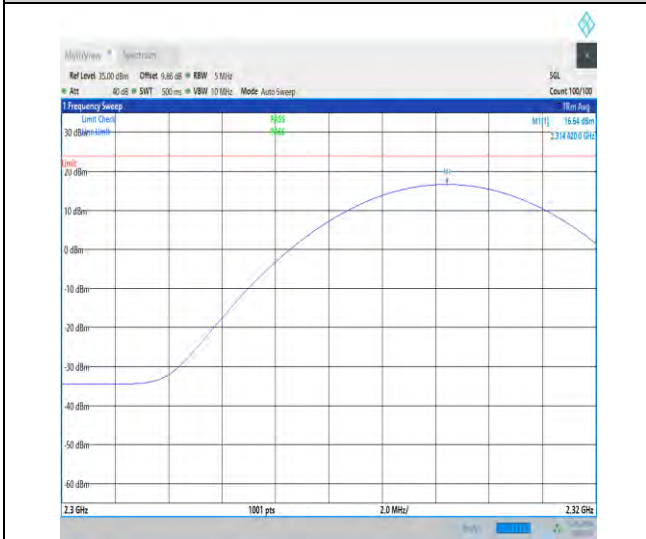
1-N30-15-10-L-2-DFT-PI2BPSK-Inner_1RB_Right-1 @50-2300-2320-Ant1-2314.42-16.64-23.98-PASS
