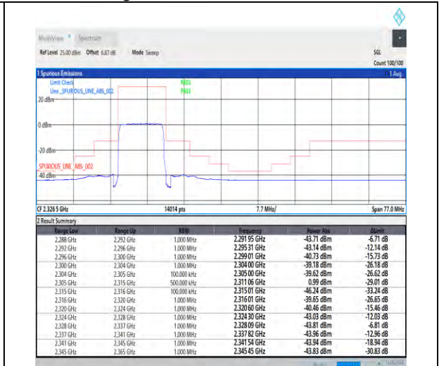
1-N30-15-10-H-3-DFT-PI2BPSK-Outer_Full-50@0-Ant1-1--PASS-see graph
