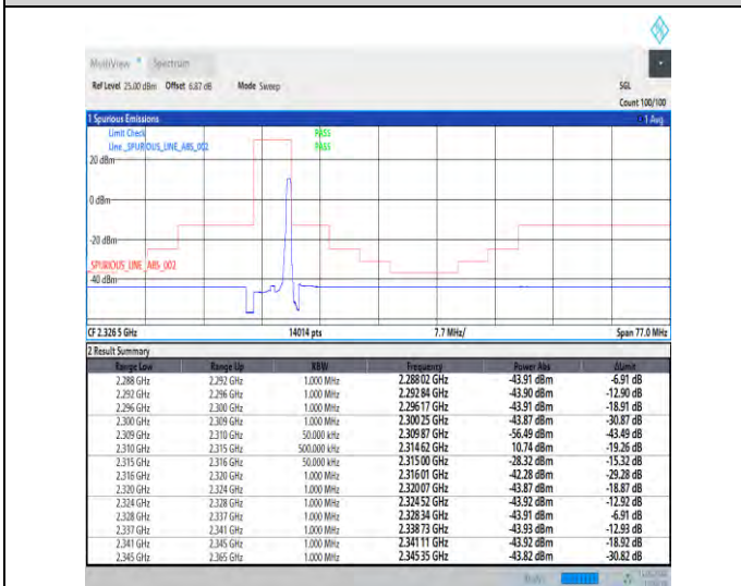
1-N30-15-5-H-5-CP-QPSK-Edge_1RB_Right-1@24-Ant1-1--PASS-see graph
