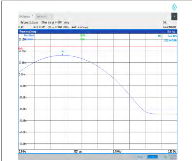
1-N30-15-10-M-1-DFT-PI2BPSK-Inner_1RB_Left-1 @ 2300-2320-Ant1-2305.56-16.22-23.98-PASS
