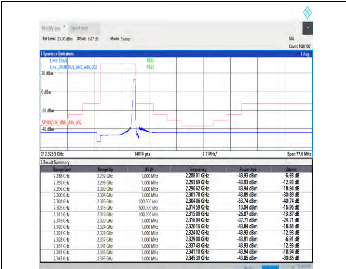
1-N30-15-10-H-2-DFT-PI2BPSK-Edge_1RB_Right-1@51-Ant1-1--PASS-see graph
