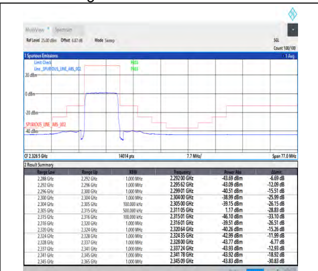
1-N30-15-10-L-3-DFT-PI2BPSK-Outer_Full-50@0-Ant1-1--PASS-see graph
