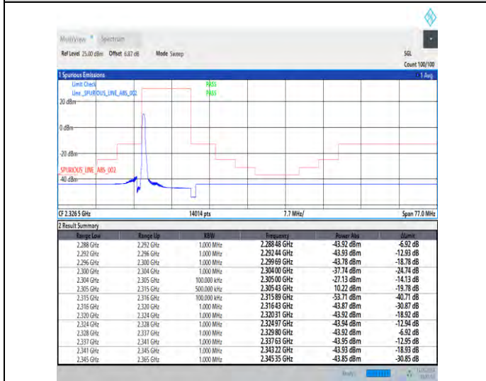
1-N30-15-10-L-4-CP-QPSK-Edge_1RB_Left-1@0-Ant1-1--PASS-see graph
