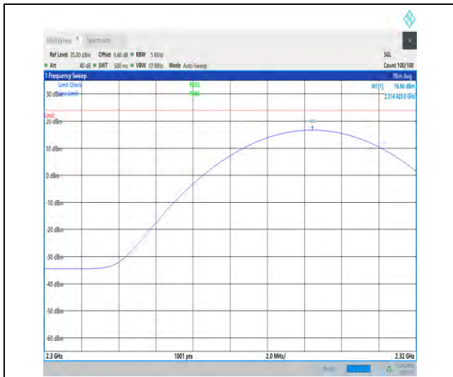
1-N30-15-10-H-2-DFT-PI2BPSK-Inner_1RB_Right-1 @50-2300-2320-Ant1-2314.42-16.66-23.98-PASS
