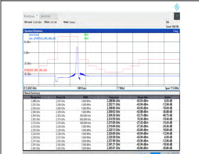
1-N30-15-10-H-5-CP-QPSK-Edge_1RB_Right-1@51-Ant1-1--PASS-see graph
