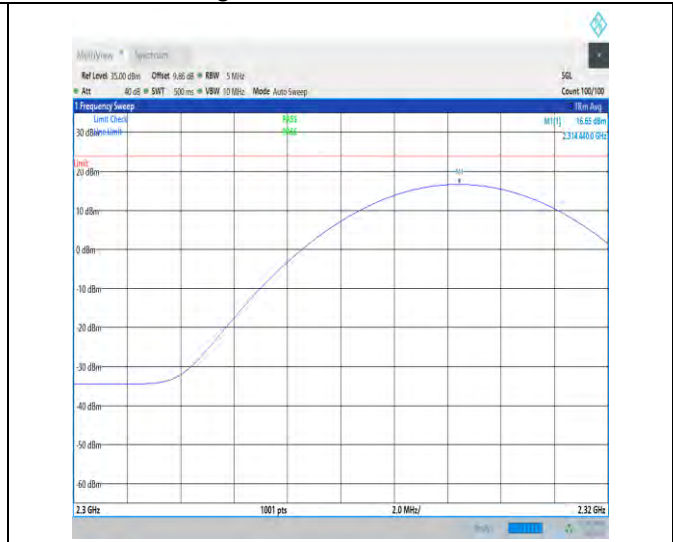
1-N30-15-10-M-2-DFT-PI2BPSK-Inner_1RB_Right-1 @ 50-2300-2320-Ant1-2314.44-16.65-23.98-PASS
