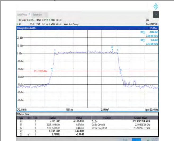
1-N30-15-10-M-1-DFT-QPSK-Outer_Full-50@0-Ant1 -8.914-9.700-≤10-PASS
