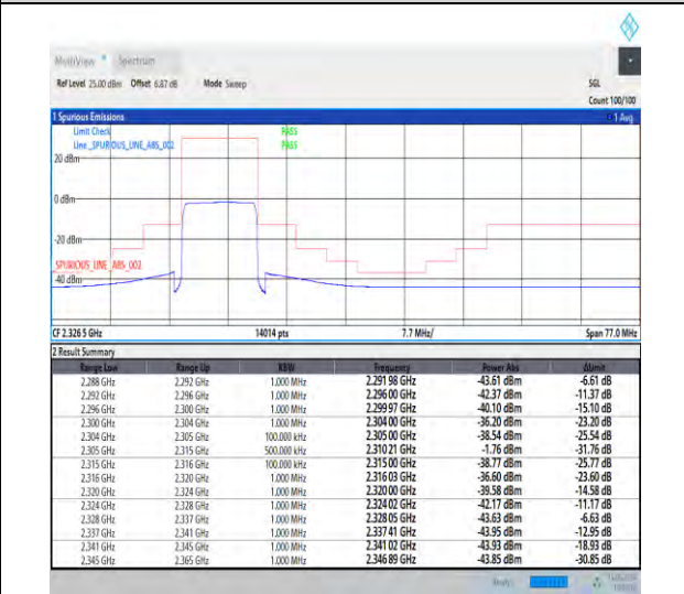
1-N30-15-10-L-6-CP-QPSK-Outer_Full-52@0-Ant1-1--PASS-see graph
