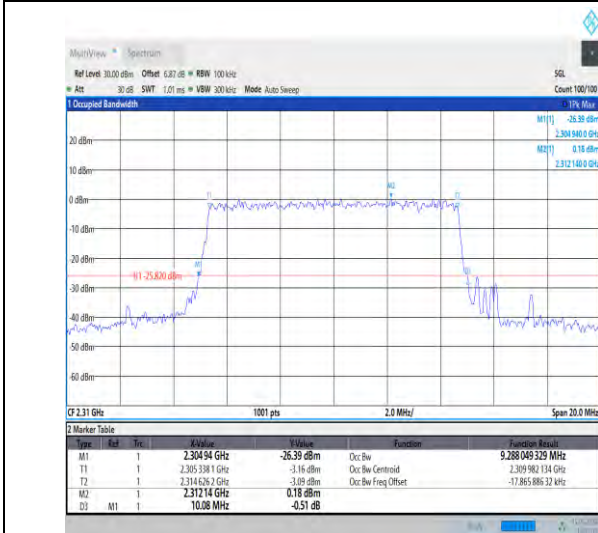
1-N30-15-10-M-6-CP-QPSK-Outer_Full-52@0-Ant1- 9.288-10.080-≤10-PASS
