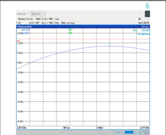
1-N30-15-5-H-2-DFT-PI2BPSK-Inner_1RB_Right-1@ 23-2307.5-2317.5-Ant1-2314.48-16.59-23.98-PASS
