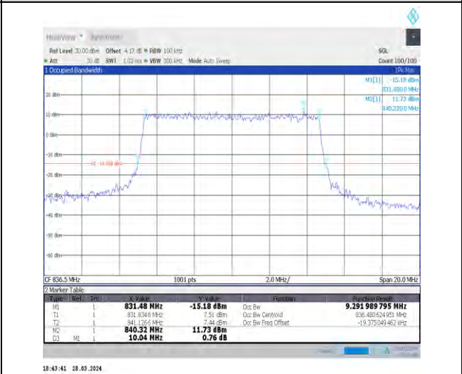
1-N26-824-849-15-10-M-7-CP-16QAM-Outer_Full-52@0-Ant1-9.292-10.040-≤10-PASS
