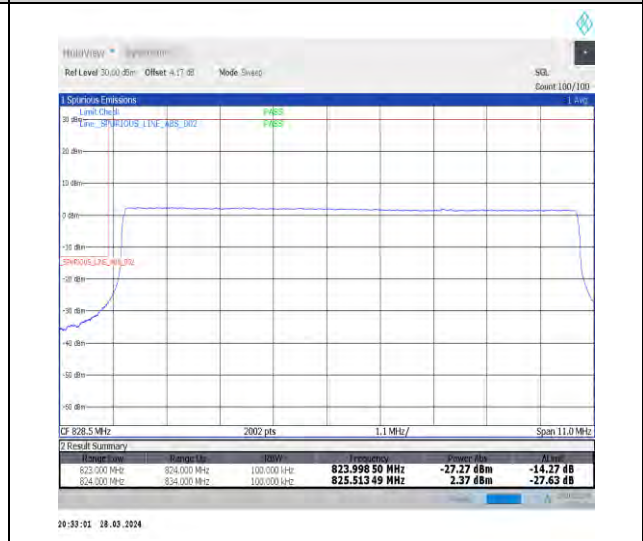
1-N26-824-849-15-10-L-6-CP-QPSK-Outer_Full-52@0-Ant1-1-seegraph-PASS-see graph
