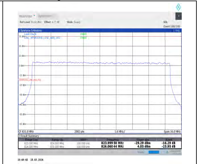
1-N26-824-849-15-15-L-3-DFT-PI2BPSK-Outer_Full-75@0-Ant1-1-seegraph-PASS-see graph
