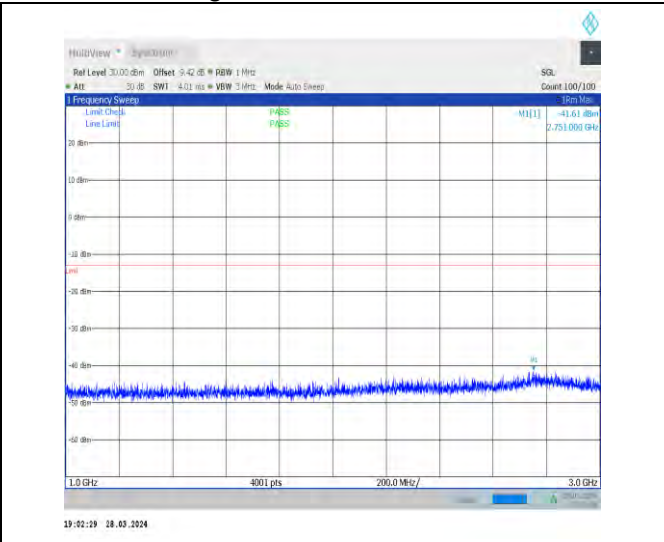
1-N26-824-849-15-20-M-1-DFT-PI2BPSK-Inner_1RB _Left-1@1-1000-3000-Ant1-2751.00--41.61--13-PAS S
