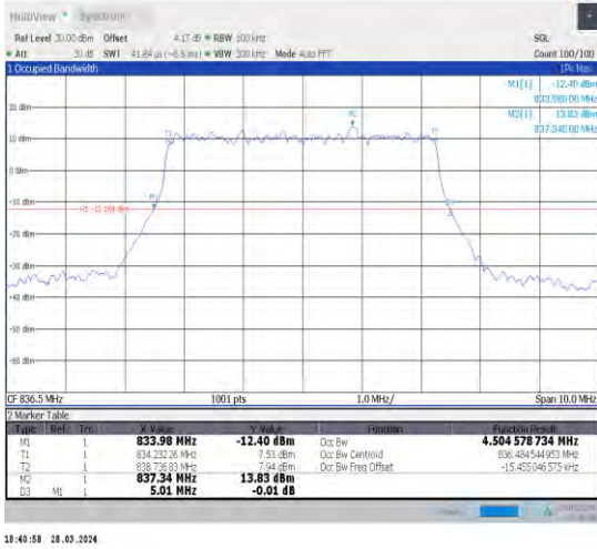
1-N26-824-849-15-5-M-5-DFT-256QAM-Outer_Full-2@0-Ant1-4.505-5.010-≤5-PASS
