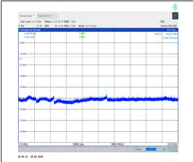
1-N26-824-849-15-20-L-1-DFT-PI2BPSK-Inner_1RB _Left-1@1-3000-12000-Ant1-7965.75--46.25--13-PA SS
