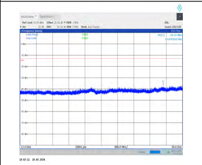
1-N26-824-849-15-20-M-1-DFT-PI2BPSK-Inner_1RB _Left-1@1-12000-20000-Ant1-19049.60--36.43--13-P ASS
