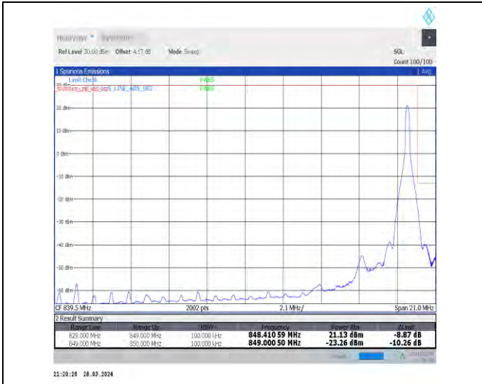
1-N26-824-849-15-20-H-2-DFT-PI2BPSK-Edge_1RB_Right-1@105-Ant1-1-seegraph-PASS-see graph
