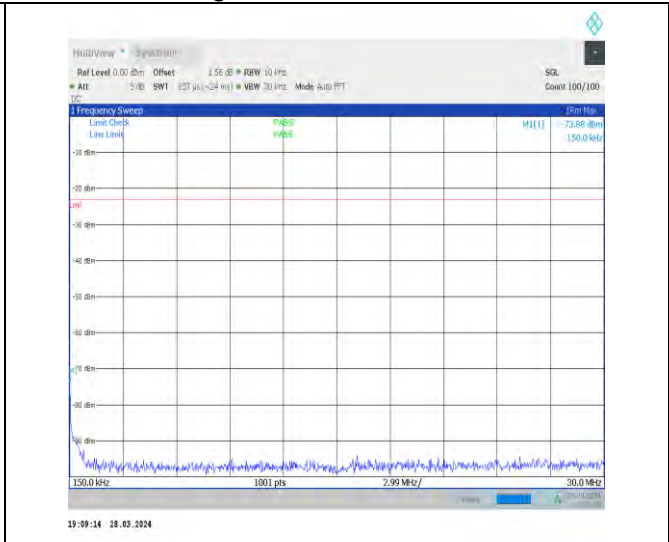
1-N26-824-849-15-20-H-1-DFT-PI2BPSK-Inner_1RB _Left-1@1-0.15-30-Ant1-0.15--73.88--23-PASS
