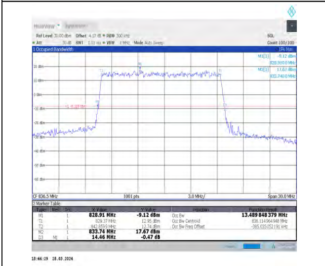
1-N26-824-849-15-15-M-1-DFT-QPSK-Outer_Full-75 @0-Ant1-13.49-14.460-≤15-PASS
