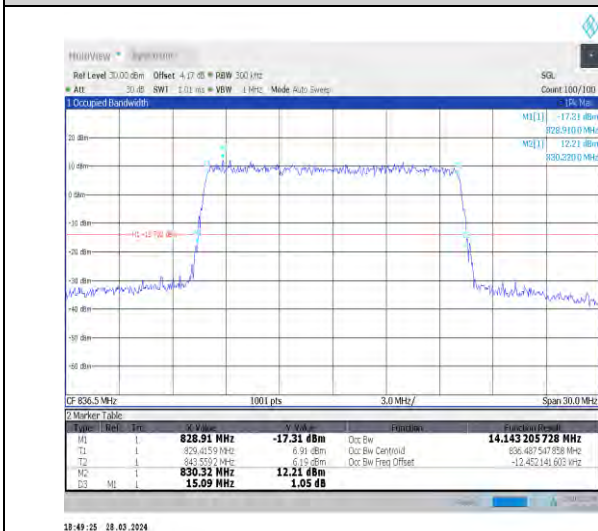
1-N26-824-849-15-15-M-9-CP-256QAM-Outer_Full-7 9@0-Ant1-14.143-15.090-≤15-PASS
