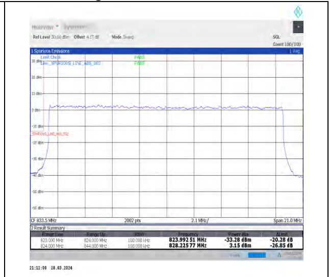
1-N26-824-849-15-20-L-3-DFT-PI2BPSK-Outer_Full-100@0-Ant1-1-seegraph-PASS-see graph
