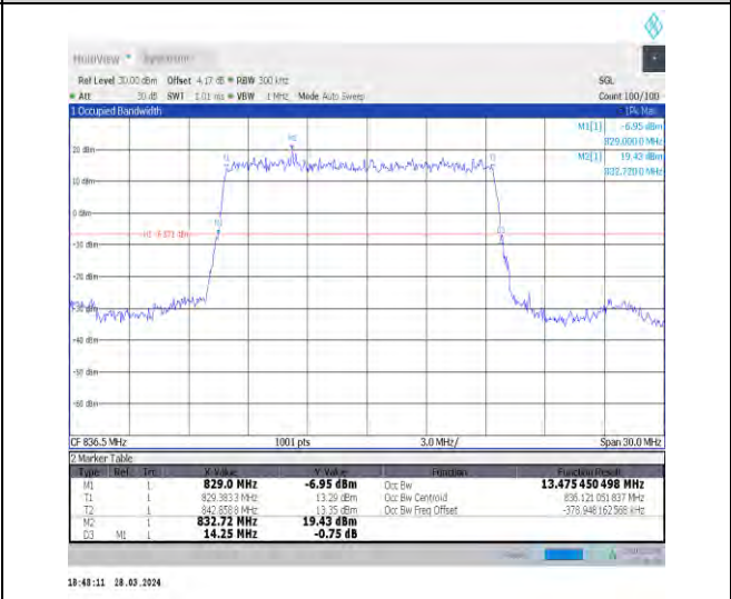
1-N26-824-849-15-15-M-2-DFT-PI2BPSK-Outer_Full-75 @0-Ant1-13.475-14.250-≤15-PASS
