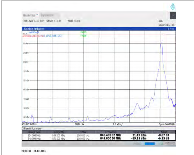
1-N26-824-849-15-15-H-2-DFT-PI2BPSK-Edge_1RB_Right-1@78-Ant1-1-seegraph-PASS-see graph
