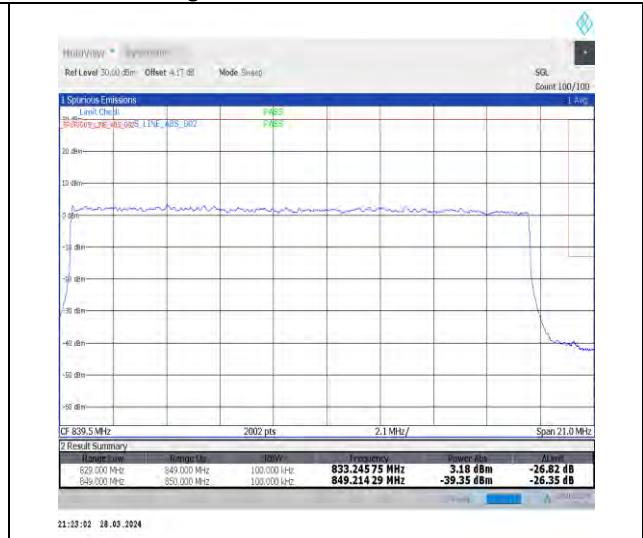
1-N26-824-849-15-20-H-3-DFT-PI2BPSK-Outer_Full-100@0-Ant1-1-seegraph-PASS-see graph
