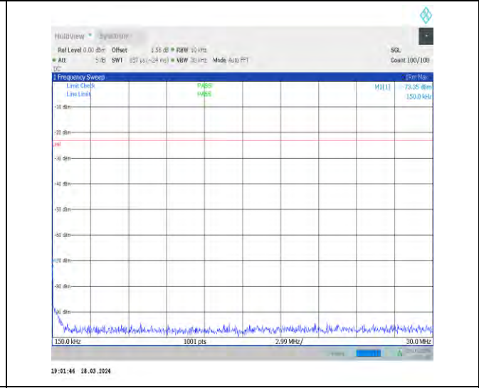
1-N26-824-849-15-20-M-1-DFT-PI2BPSK-Inner_1RB _Left-1@1-0.15-30-Ant1-0.15--73.35--23-PASS
