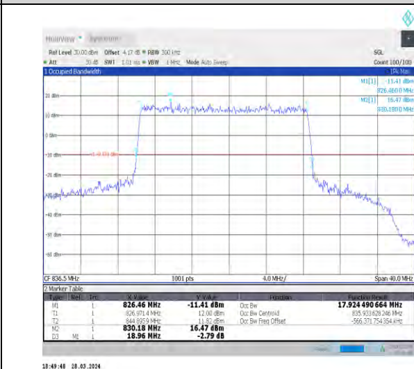
1-N26-824-849-15-20-M-1-DFT-QPSK-Outer_Full-10 0@0-Ant1-17.924-18.960-≤20-PASS
