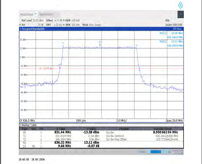
1-N26-824-849-15-10-M-3-DFT-16QAM-Outer_Full-50 @0-Ant1-8.951-9.660-≤10-PASS
