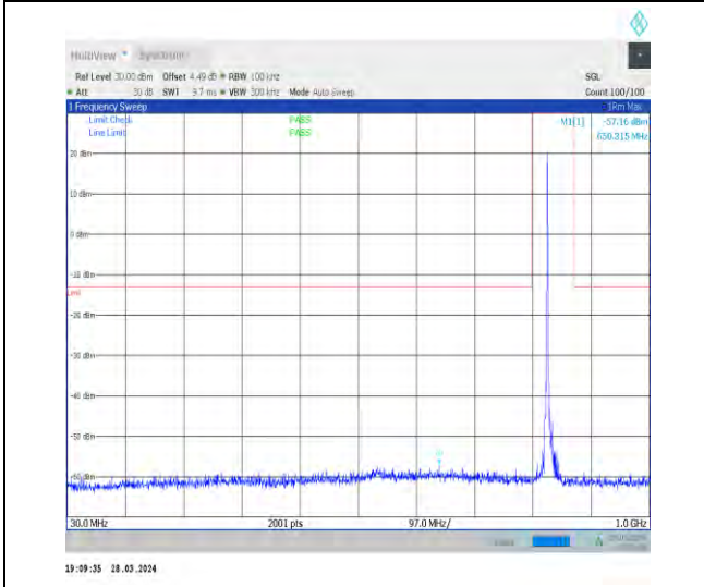
1-N26-824-849-15-20-H-1-DFT-PI2BPSK-Inner_1R B_Left-1@1-30-1000-Ant1-650.32--57.16--13-PASS
