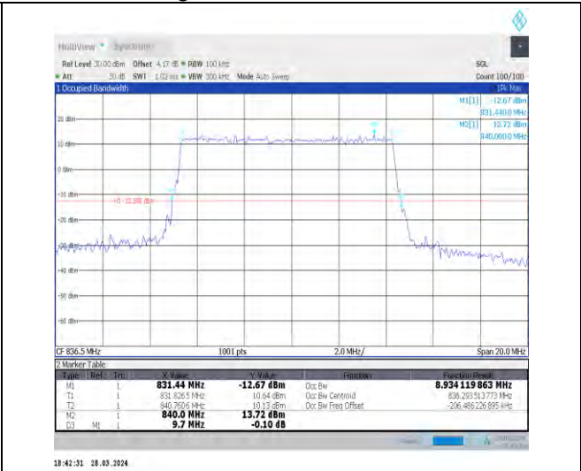
1-N26-824-849-15-10-M-1-DFT-QPSK-Outer_Full-50 @0-Ant1-8.934-9.700-≤10-PASS
