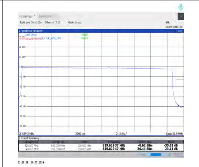
1-N26-824-849-15-20-H-6-CP-QPSK-Outer_Full-106@0-Ant1-1-seegraph-PASS-see graph
