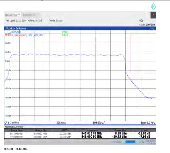
1-N26-824-849-15-5-H-3-DFT-PI2BPSK-Outer_Ful l-25@0-Ant1-1-seegraph-PASS-see graph
