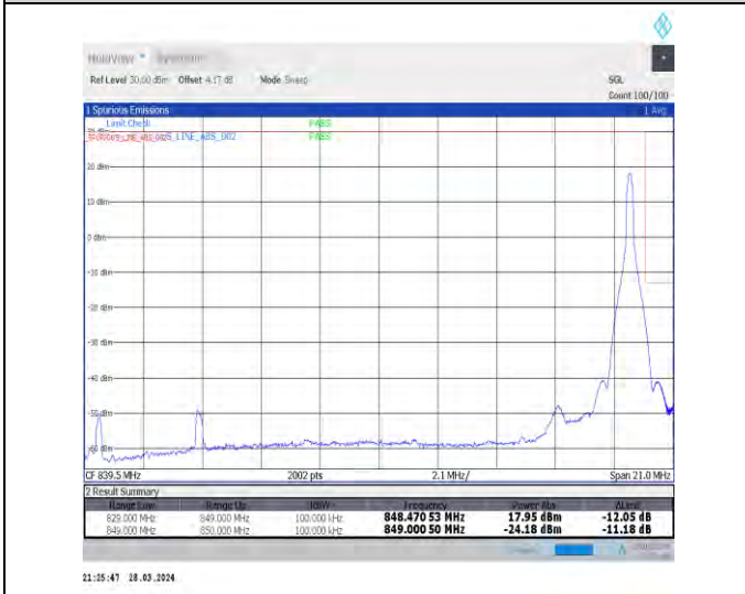
1-N26-824-849-15-20-H-5-CP-QPSK-Edge_1RB_Right-1@105-Ant1-1-seegraph-PASS-see graph
