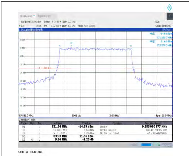
1-N26-824-849-15-10-M-8-CP-64QAM-Outer_Full-52 @0-Ant1-9.285-9.860-≤10-PASS
