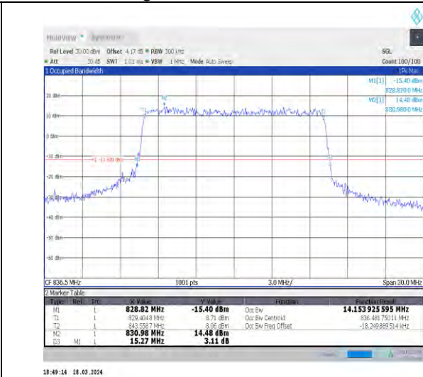
1-N26-824-849-15-15-M-8-CP-64QAM-Outer_Full-7 9@0-Ant1-14.154-15.270-≤15-PASS
