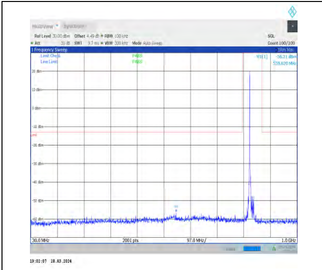
1-N26-824-849-15-20-M-1-DFT-PI2BPSK-Inner_1R B_Left-1@1-30-1000-Ant1-559.62--56.31--13-PASS
