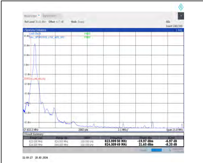
1-N26-824-849-15-20-L-1-DFT-PI2BPSK-Edge_1RB_Left-1@0-Ant1-1-seegraph-PASS-see graph
