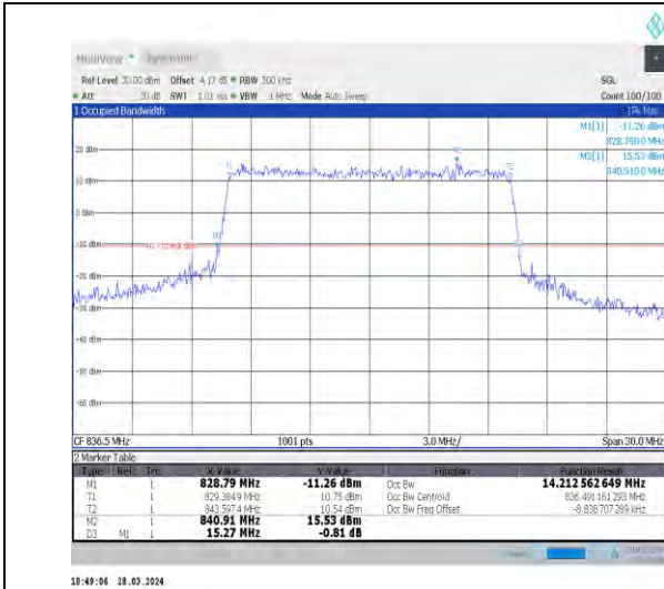
1-N26-824-849-15-15-M-7-CP-16QAM-Outer_Full-79 @0-Ant1-14.213-15.270-≤15-PASS
