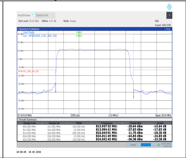
1-N26-814-824-15-10-H-3-DFT-PI2BPSK-Outer_Full-50@0-Ant1-1--PASS-see graph
