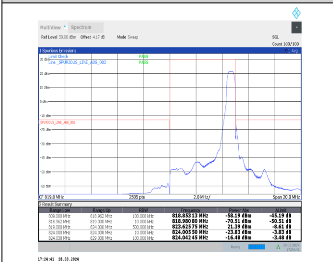
1-N26-814-824-15-5-H-5-CP-QPSK-Edge_1RB_Right-1@24-Ant1-1--PASS-see graph
