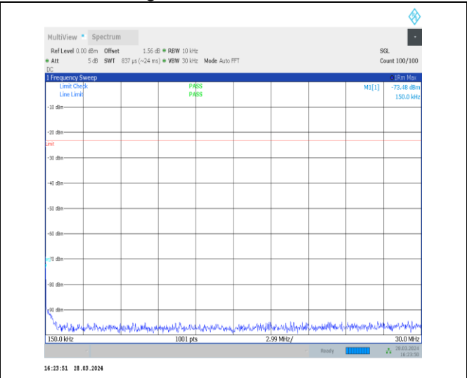
1-N26-814-824-15-10-H-1-DFT-PI2BPSK-Inner_1RB _Left-1@1-0.15-30-Ant1-0.15--73.48--23-PASS
