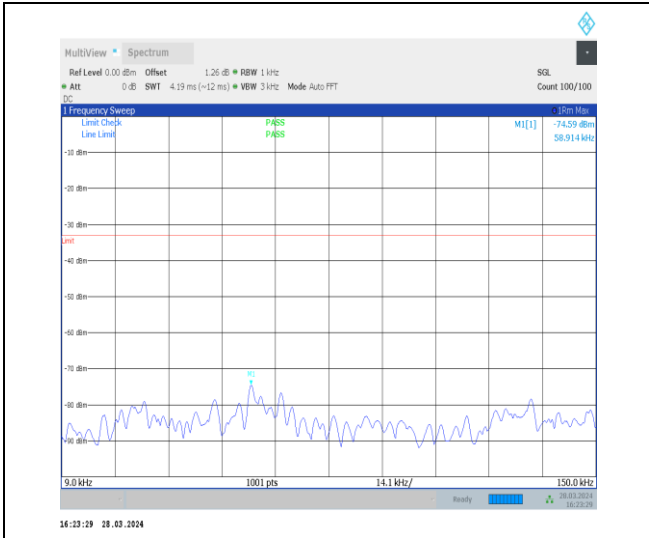
1-N26-814-824-15-10-H-1-DFT-PI2BPSK-Inner_1R B_Left-1@1-0.009-0.15-Ant1-0.06--74.59--33-PASS
