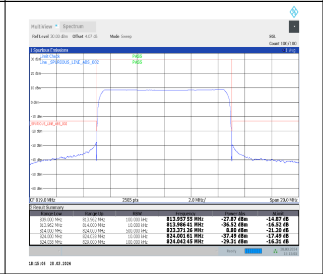
1-N26-814-824-15-10-H-6-CP-QPSK-Outer_Full-52@0-Ant1-1--PASS-see graph
