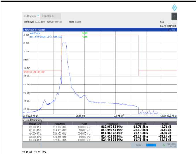
1-N26-814-824-15-10-L-4-CP-QPSK-Edge_1RB_Left-1@0-Ant1-1--PASS-see graph
