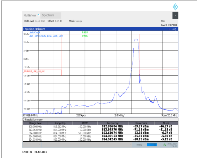
1-N26-814-824-15-10-H-2-DFT-PI2BPSK-Edge_1RB_Right-1@51-Ant1-1--PASS-see graph
