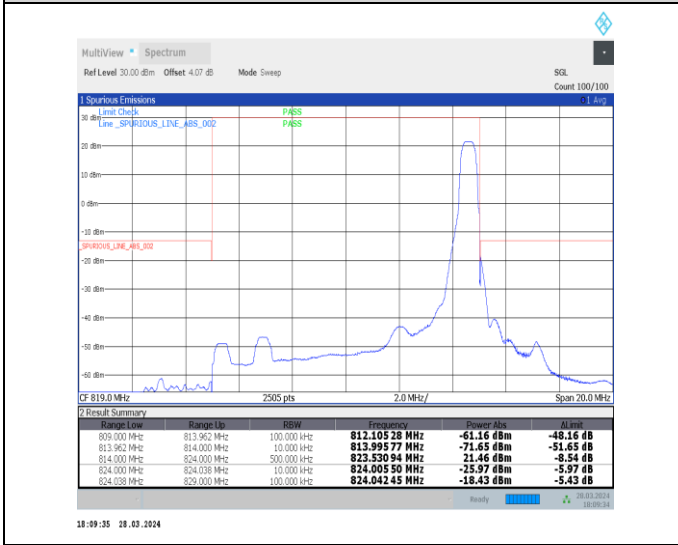
1-N26-814-824-15-10-H-5-CP-QPSK-Edge_1RB_Right-1@51-Ant1-1--PASS-see graph
