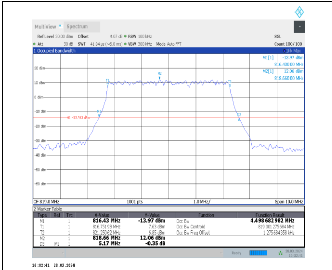
1-N26-814-824-15-5-M-5-DFT-256QAM-Outer_Full-2 5@0-Ant1-4.499-5.170-≤5-PASS
