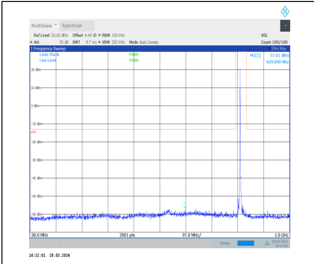
1-N26-814-824-15-10-M-1-DFT-PI2BPSK-Inner_1R B_Left-1@1-30-1000-Ant1-609.09--57.01--13-PASS
