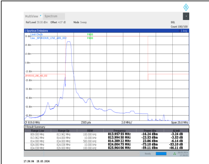
1-N26-814-824-15-10-L-1-DFT-PI2BPSK-Edge_1RB_L-1@0-Ant1-1--PASS-see graph
