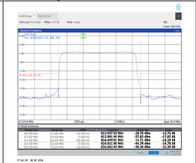
1-N26-814-824-15-10-L-3-DFT-PI2BPSK-Outer_Full-50@0-Ant1-1--PASS-see graph
