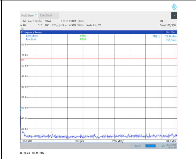
1-N26-814-824-15-10-M-1-DFT-PI2BPSK-Inner_1RB _Left-1@1-0.15-30-Ant1-0.15--73.40--23-PASS
