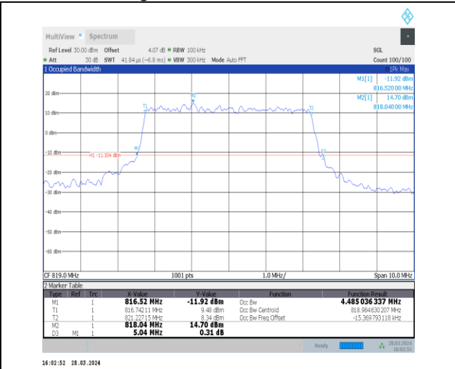
1-N26-814-824-15-5-M-6-CP-QPSK-Outer_Full-25@ 0-Ant1-4.485-5.040-≤5-PASS
