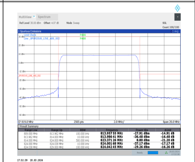
1-N26-814-824-15-10-L-6-CP-QPSK-Outer_Full-52@0-Ant1-1--PASS-see graph
