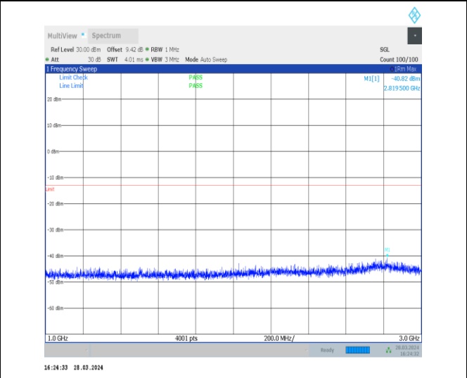
1-N26-814-824-15-10-H-1-DFT-PI2BPSK-Inner_1RB _Left-1@1-1000-3000-Ant1-2819.50--40.82--13-PASS
