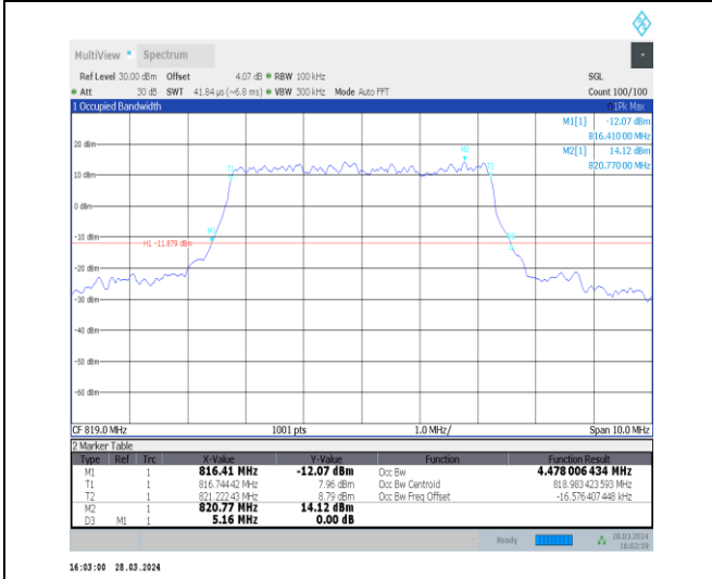
1-N26-814-824-15-5-M-7-CP-16QAM-Outer_Full-25 @0-Ant1-4.478-5.160-≤5-PASS
