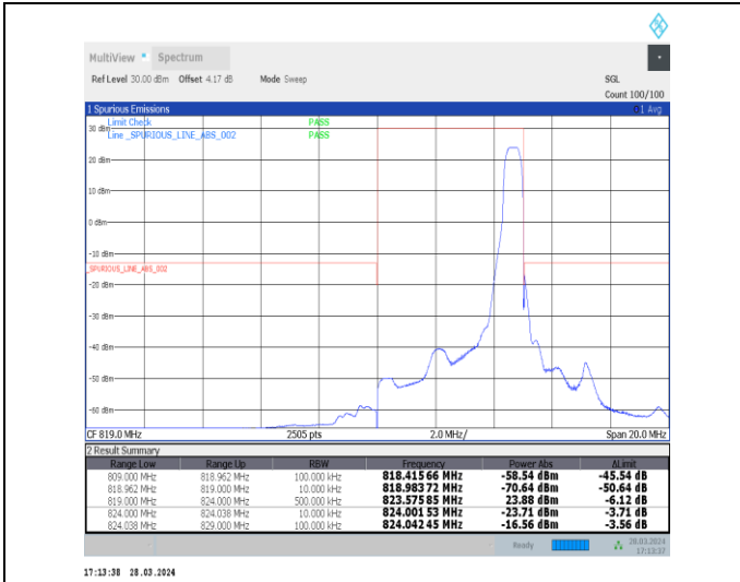
1-N26-814-824-15-5-H-2-DFT-PI2BPSK-Edge_1RB_Right-1@24-Ant1-1--PASS-see graph
