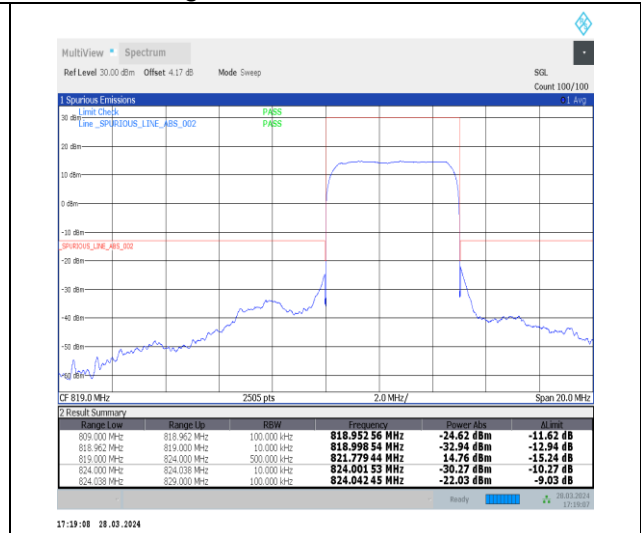
1-N26-814-824-15-5-H-3-DFT-PI2BPSK-Outer_Full-I-25@0-Ant1-1--PASS-see graph
