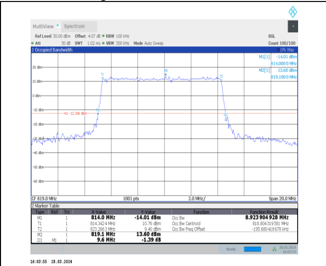
1-N26-814-824-15-10-M-1-DFT-QPSK-Outer_Full-50 @0-Ant1-8.924-9.600-≤10-PASS
