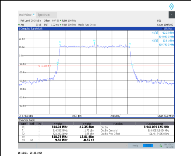
1-N26-814-824-15-10-M-3-DFT-16QAM-Outer_Full-50 @0-Ant1-8.944-9.580-≤10-PASS
