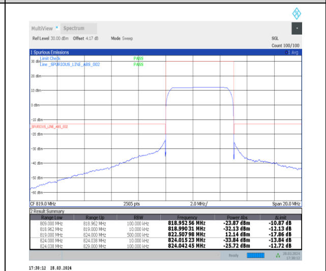
1-N26-814-824-15-5-H-6-CP-QPSK-Outer_Full-25@0-Ant1-1--PASS-see graph
