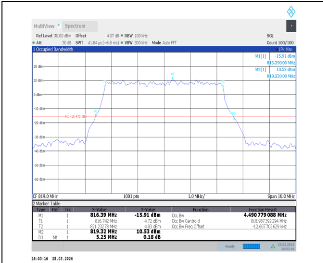
1-N26-814-824-15-5-M-9-CP-256QAM-Outer_Full-25 @0-Ant1-4.491-5.250-≤5-PASS
