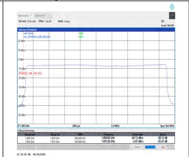
1-N25-15-25-L-3-DFT-PI2BPSK-Outer_Full-128@0-Ant1-1-seegraph-PASS-see graph
