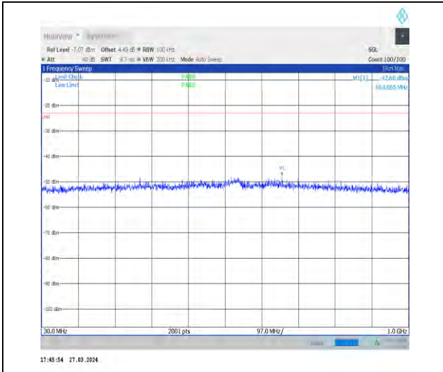
1-N25-15-40-M-1-DFT-PI2BPSK-Inner_1RB_Left-1 @1-30-1000-Ant1-664.87--47.68--23-PASS
