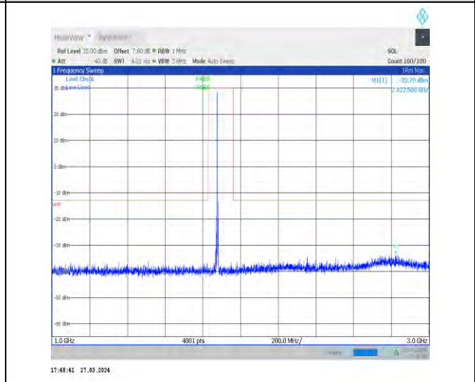
1-N25-15-40-H-1-DFT-PI2BPSK-Inner_1RB_Left-1@ 1-1000-3000-Ant1-2822.50--33.70--13-PASS
