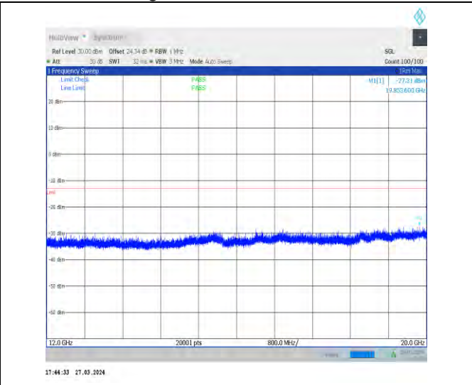
1-N25-15-40-L-1-DFT-PI2BPSK-Inner_1RB_Left-1@ 1-12000-20000-Ant1-19853.60--27.31--13-PASS
