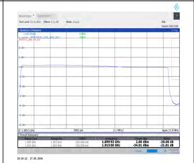
1-N25-15-20-H-6-CP-QPSK-Outer_Full-106@0-Ant1-1-seegraph-PASS-see graph
