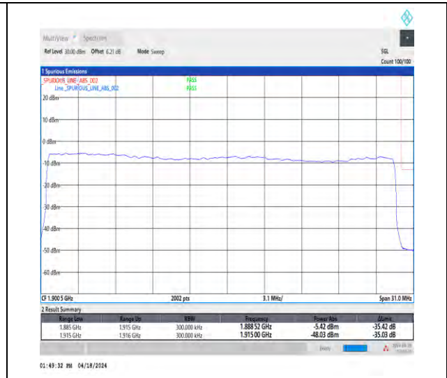
1-N25-15-30-H-3-DFT-PI2BPSK-Outer_Full-160@0-Ant1-1-seegraph-PASS-see graph
