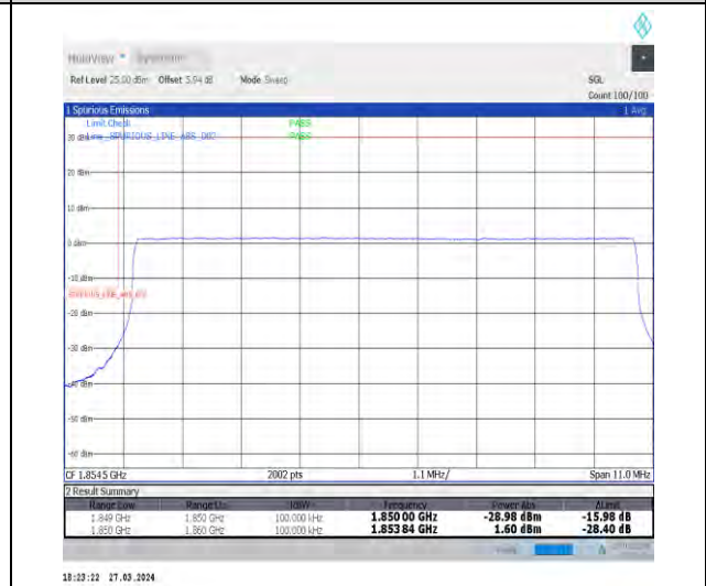
1-N25-15-10-L-6-CP-QPSK-Outer_Full-52@0-Ant1-1-seegraph-PASS-see graph
