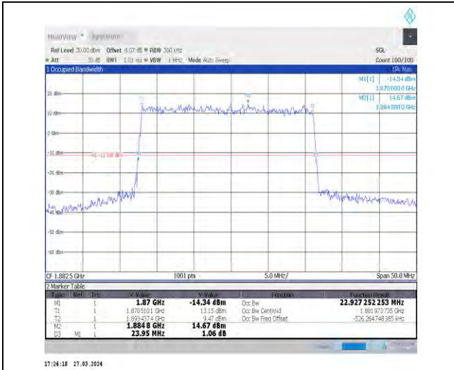
1-N25-15-25-M-1-DFT-QPSK-Outer_Full-128@0-Ant 1-22.927-23.950-≤25-PASS
