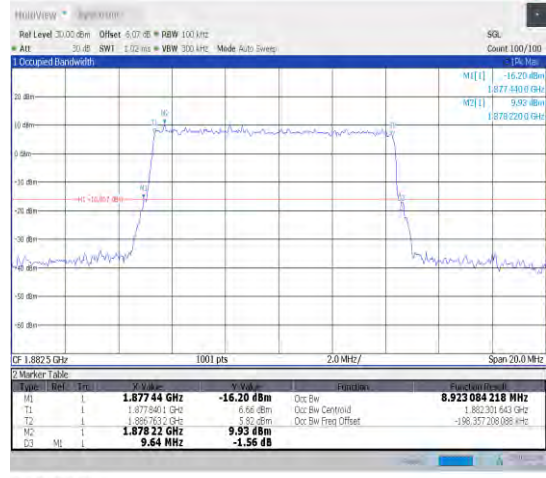
1-N25-15-10-M-5-DFT-256QAM-Outer_Full-50@0-A nt1-8.923-9.640-≤10-PASS
