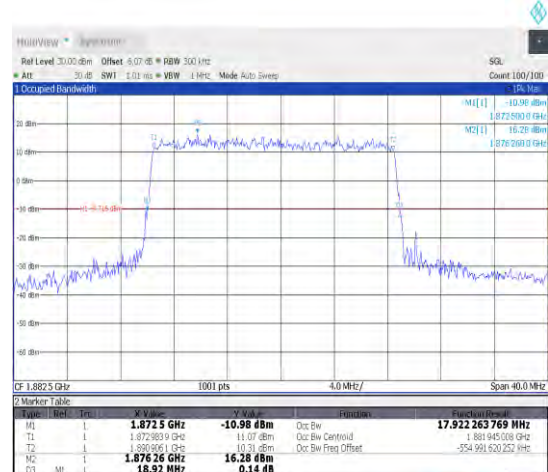
1-N25-15-15-M-8-CP-64QAM-Outer_Full-79@0-Ant1 -14.134-15.210-≤15-PASS
