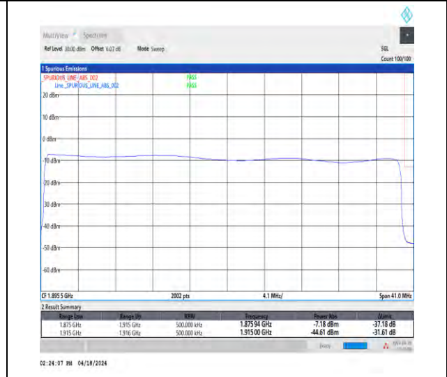
1-N25-15-40-H-6-CP-QPSK-Outer_Full-216@0-Ant1-1-seegraph-PASS-see graph
