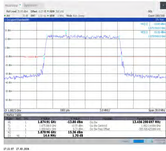
1-N25-15-15-M-4-DFT-64QAM-Outer_Full-75@0-Ant 1-13.456-14.400-≤15-PASS
