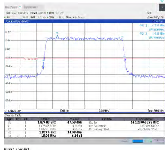
1-N25-15-15-M-6-CP-QPSK-Outer_Full-79@0-Ant1 14.128-15.060-≤15-PASS
