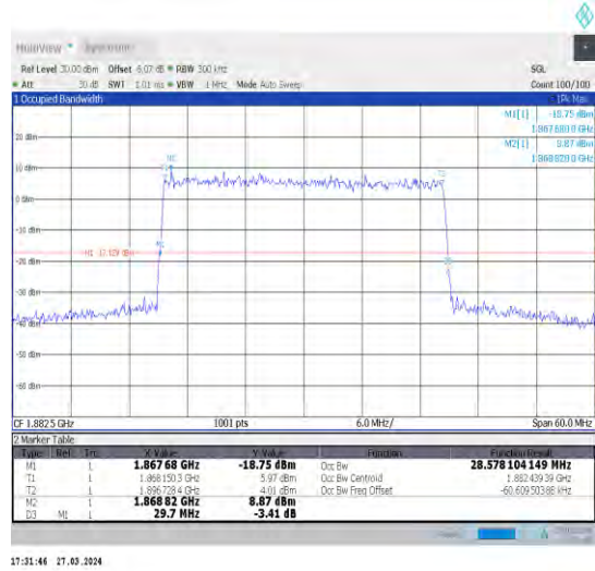
1-N25-15-30-M-9-CP-256QAM-Outer_Full-160@0-A nt1-28.578-29.700-≤30-PASS
