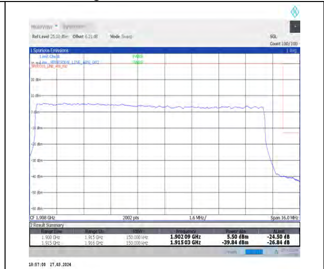
1-N25-15-15-H-3-DFT-PI2BPSK-Outer_Full-75@0-Ant1-1-seegraph-PASS-see graph
