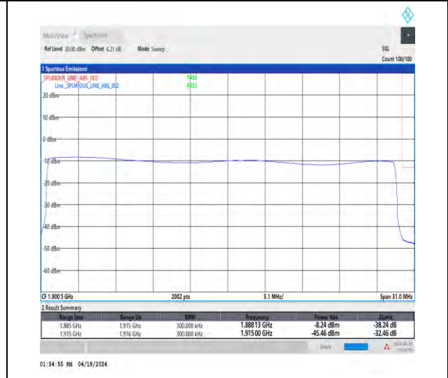
1-N25-15-30-H-6-CP-QPSK-Outer_Full-160@0-Ant1-1-seegraph-PASS-see graph
