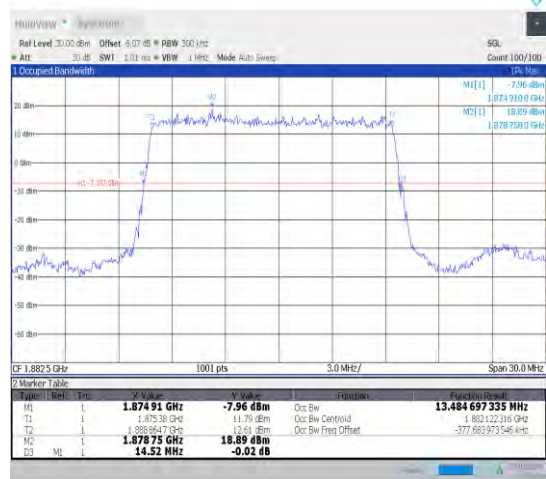
1-N25-15-15-M-2-DFT-PI2BPSK-Outer_Full-75@0-Ant1 -13.485-14.520-≤15-PASS
