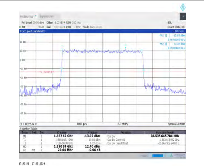
1-N25-15-30-M-3-DFT-16QAM-Outer_Full-160@0-A nt1-28.537-29.640-≤30-PASS
