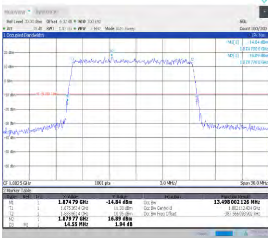
1-N25-15-15-M-1-DFT-QPSK-Outer_Full-75@0-Ant1 -13.498-14.550-≤15-PASS
