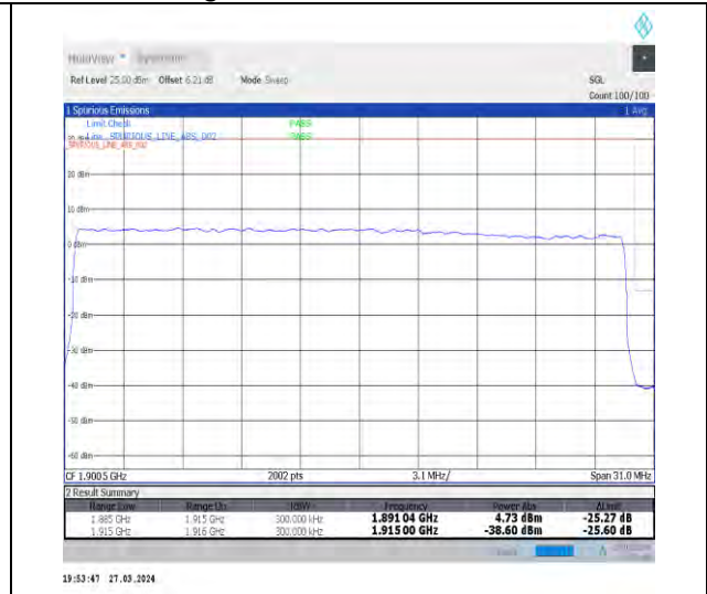
1-N25-15-30-H-3-DFT-PI2BPSK-Outer_Full-160@0-Ant1-1-seegraph-PASS-see graph
