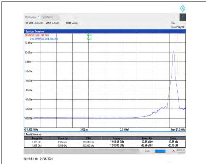
1-N25-15-20-H-2-DFT-PI2BPSK-Edge_1RB_Right-1@105-Ant1-1-seegraph-PASS-see graph
