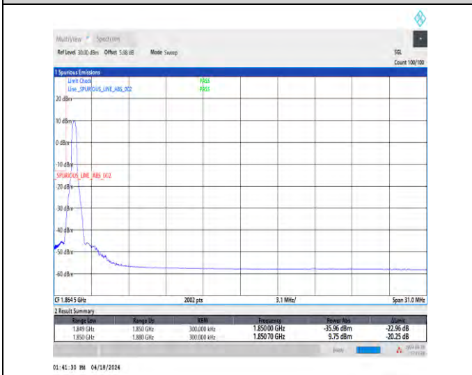
1-N25-15-30-L-4-CP-QPSK-Edge_1RB_Left-1@0-Ant1-1-seegraph-PASS-see graph
