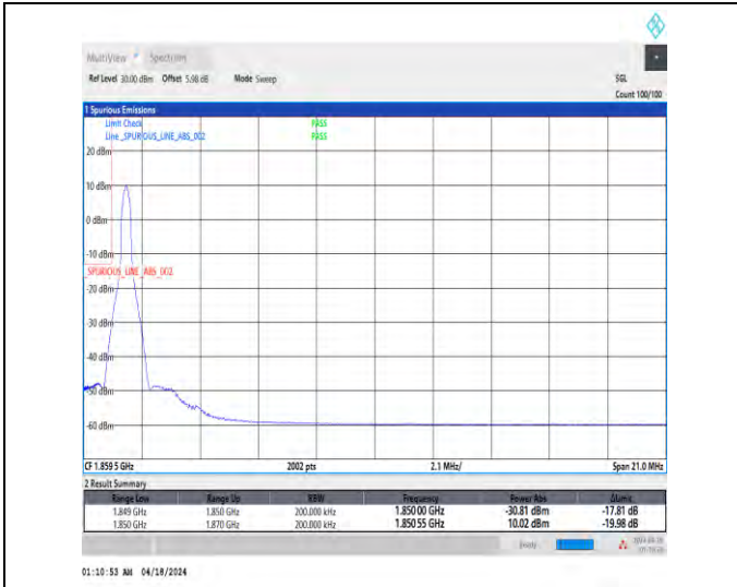
1-N25-15-20-L-1-DFT-PI2BPSK-Edge_1RB_Left-1@0-Ant1-1-seegraph-PASS-see graph
