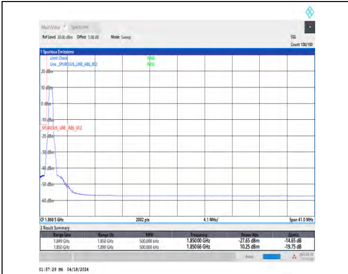
1-N25-15-40-L-1-DFT-PI2BPSK-Edge_1RB_Left-1@0-Ant1-1-seegraph-PASS-see graph
