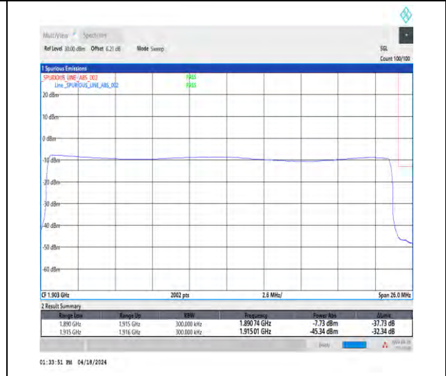
1-N25-15-25-H-6-CP-QPSK-Outer_Full-133@0-Ant1-1-seegraph-PASS-see graph
