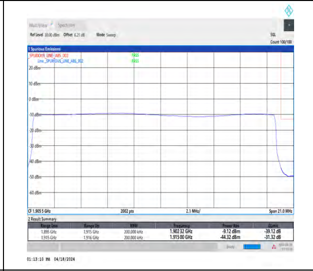
1-N25-15-20-H-6-CP-QPSK-Outer_Full-106@0-Ant1-1-seegraph-PASS-see graph
