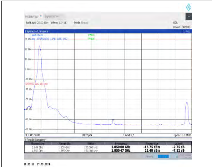
1-N25-15-15-L-1-DFT-PI2BPSK-Edge_1RB_Left-1@0-Ant1-1-seegraph-PASS-see graph
