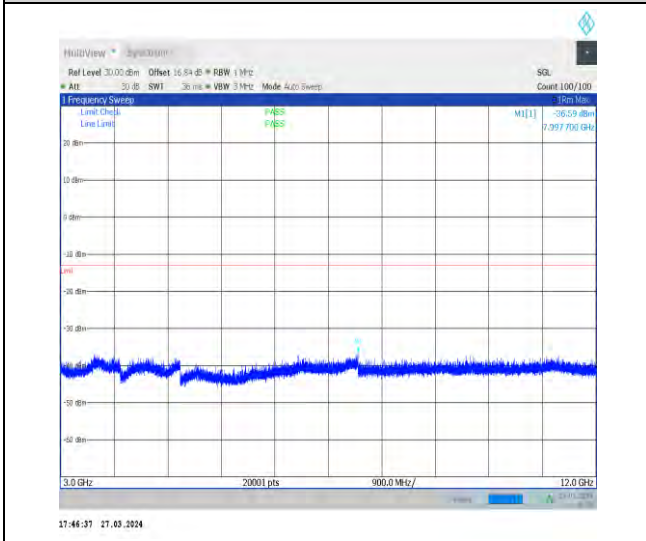
1-N25-15-40-M-1-DFT-PI2BPSK-Inner_1RB_Left-1 @1-3000-12000-Ant1-7997.70--36.59--13-PASS
