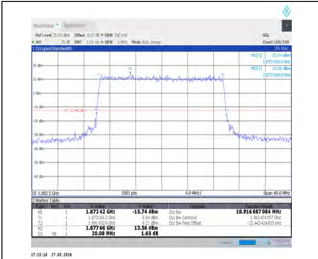
1-N25-15-20-M-6-CP-QPSK-Outer_Full-106@0-Ant1 -18.917-20.080-≤20-PASS
