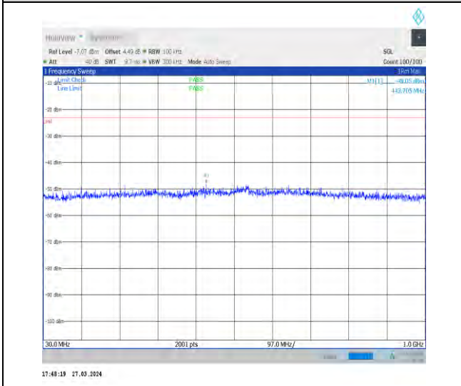
1-N25-15-40-H-1-DFT-PI2BPSK-Inner_1RB_Left-1 @1-30-1000-Ant1-443.71--48.05--23-PASS
