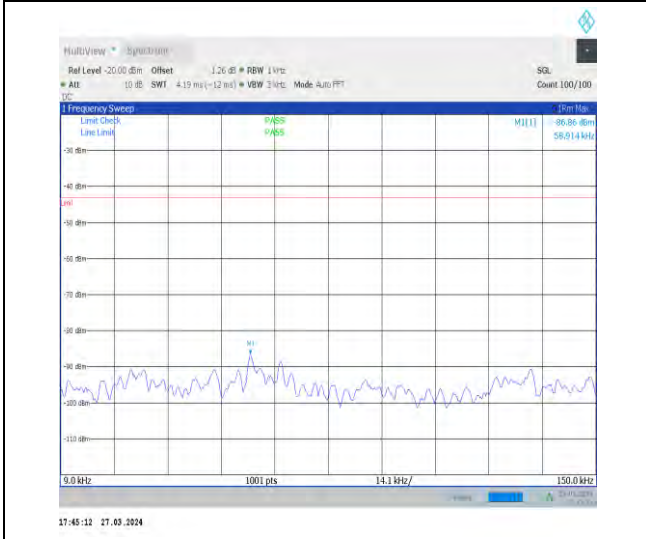
1-N25-15-40-M-1-DFT-PI2BPSK-Inner_1RB_Left-1 @1-0.009-0.15-Ant1-0.06--86.86--43-PASS
