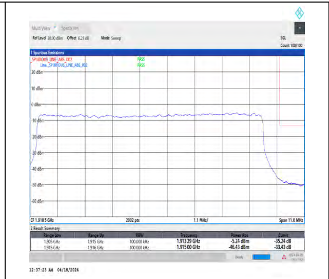
1-N25-15-10-H-3-DFT-PI2BPSK-Outer_Full-50@0-Ant1-1-seegraph-PASS-see graph
