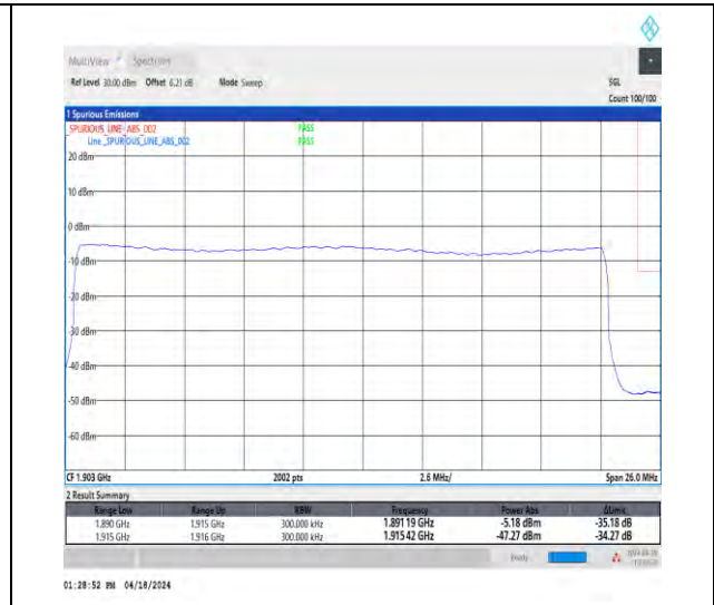
1-N25-15-25-H-3-DFT-PI2BPSK-Outer_Full-128@0-Ant1-1-seegraph-PASS-see graph
