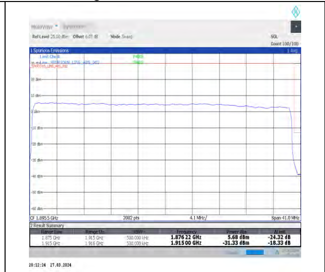
1-N25-15-40-H-3-DFT-PI2BPSK-Outer_Full-216@0-Ant1-1-seegraph-PASS-see graph
