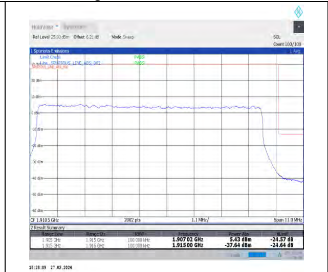
1-N25-15-10-H-3-DFT-PI2BPSK-Outer_Full-50@0-Ant1-1-seegraph-PASS-see graph
