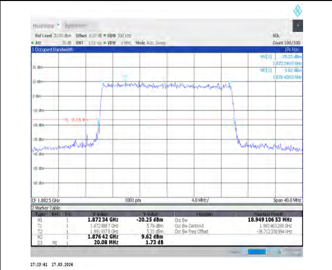
1-N25-15-20-M-9-CP-256QAM-Outer_Full-106@0-A nt1-18.949-20.080-≤20-PASS
