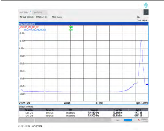
1-N25-15-30-H-5-CP-QPSK-Edge_1RB_Right-1@159-Ant1-1-seegraph-PASS-see graph
