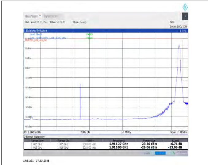
1-N25-15-30-H-2-DFT-PI2BPSK-Edge_1RB_Right-1@159-Ant1-1-seegraph-PASS-see graph
