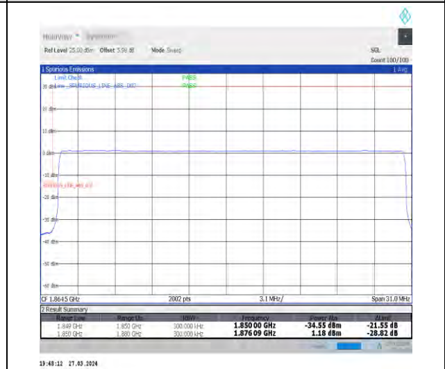
1-N25-15-30-L-6-CP-QPSK-Outer_Full-160@0-Ant1-1-seegraph-PASS-see graph
