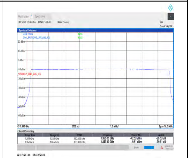
1-N25-15-15-L-6-CP-QPSK-Outer_Full-79@0-Ant1-1-seegraph-PASS-see graph
