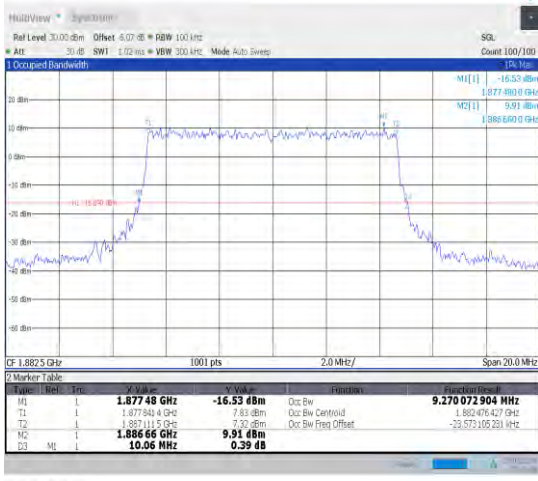
1-N25-15-10-M-8-CP-64QAM-Outer_Full-52@0-Ant1 -9.27-10.060-≤10-PASS
