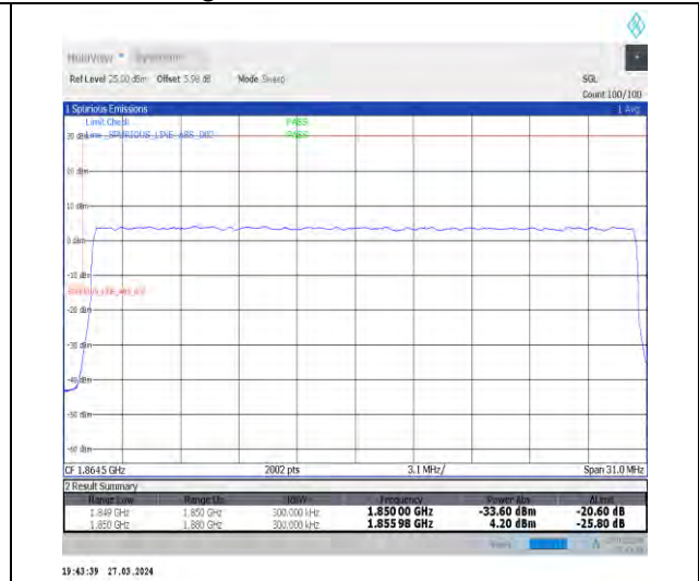
1-N25-15-30-L-3-DFT-PI2BPSK-Outer_Full-160@0-Ant1-1-seegraph-PASS-see graph
