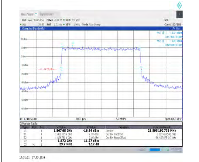
1-N25-15-30-M-6-CP-QPSK-Outer_Full-160@0-Ant1 -28.598-29.700-≤30-PASS
