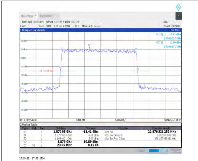
1-N25-15-25-M-5-DFT-256QAM-Outer_Full-128@0-Ant1-22.877-23.950-≤25-PASS
