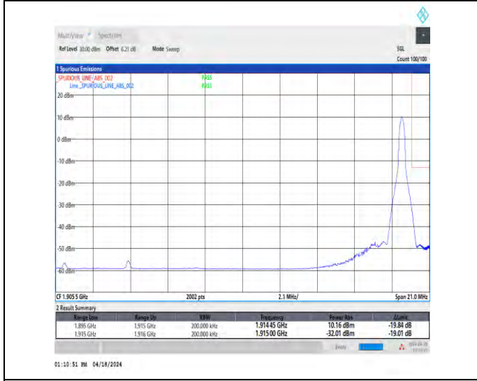
1-N25-15-20-H-5-CP-QPSK-Edge_1RB_Right-1@105-Ant1-1-seegraph-PASS-see graph
