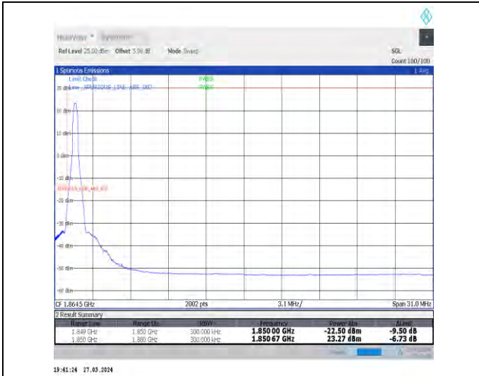
1-N25-15-30-L-1-DFT-PI2BPSK-Edge_1RB_Left-1@0-Ant1-1-seegraph-PASS-see graph
