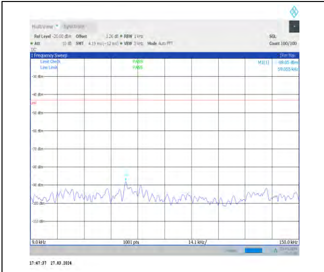
1-N25-15-40-H-1-DFT-PI2BPSK-Inner_1RB_Left-1 @1-0.009-0.15-Ant1-0.06--88.05--43-PASS
