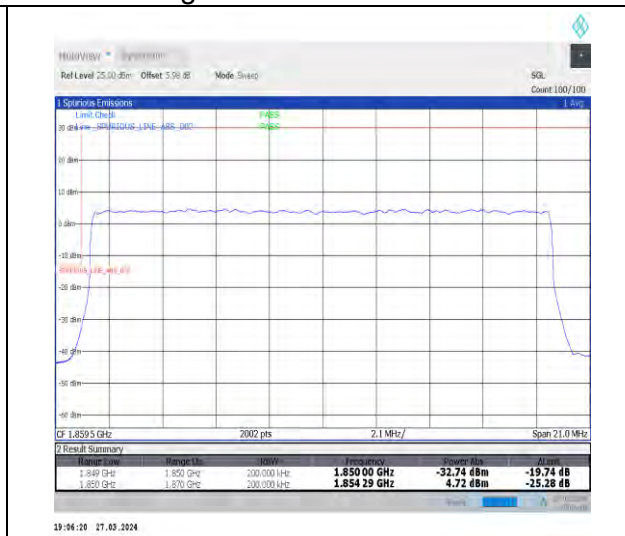
1-N25-15-20-L-3-DFT-PI2BPSK-Outer_Full-100@0-Ant1-1-seegraph-PASS-see graph
