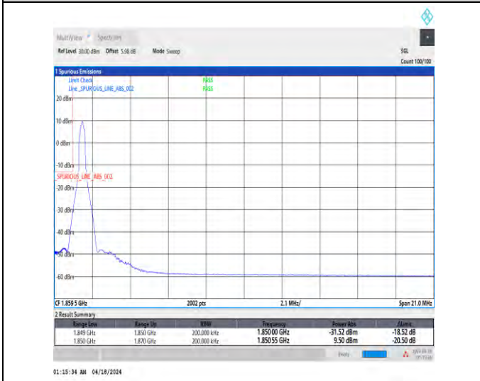
1-N25-15-20-L-4-CP-QPSK-Edge_1RB_Left-1@0-Ant1-1-seegraph-PASS-see graph
