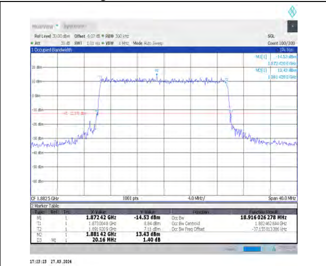
1-N25-15-20-M-7-CP-16QAM-Outer_Full-106@0-Ant 1-18.916-20.160-≤20-PASS
