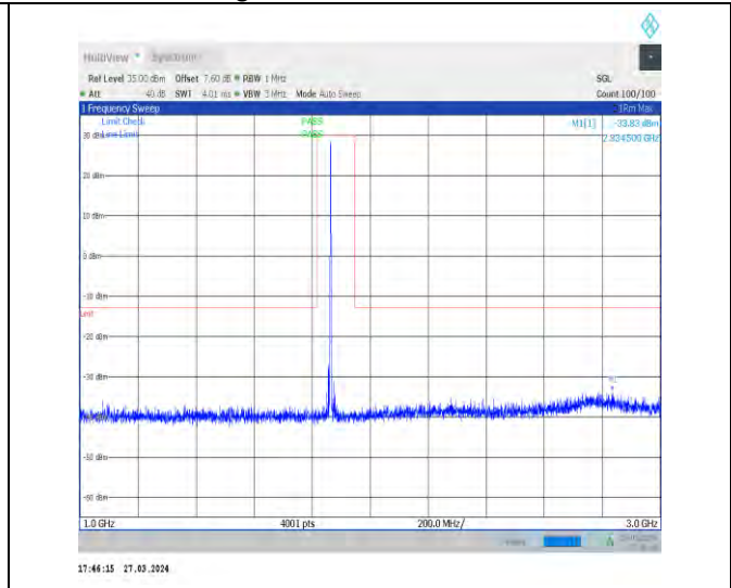
1-N25-15-40-M-1-DFT-PI2BPSK-Inner_1RB_Left-1 @ 1-1000-3000-Ant1-2834.50--33.83--13-PASS
