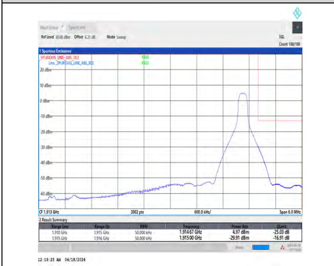
1-N25-15-5-H-5-CP-QPSK-Edge_1RB_Right-1@24-Ant1-1-seegraph-PASS-see graph
