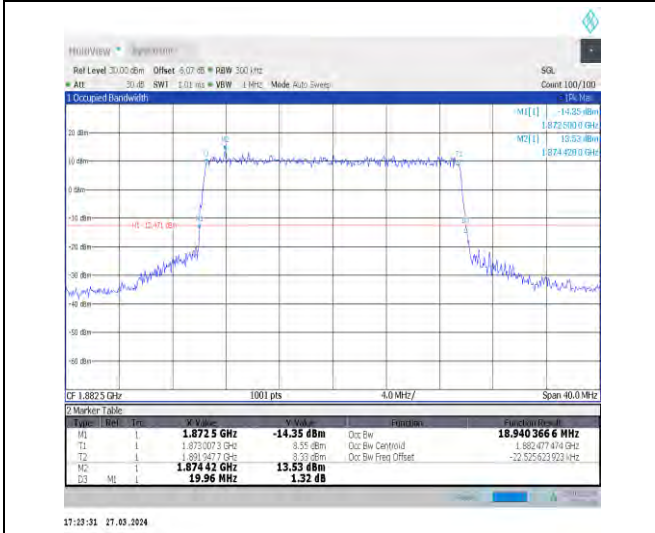
1-N25-15-20-M-8-CP-64QAM-Outer_Full-106@0-Ant 1-18.94-19.960-≤20-PASS
