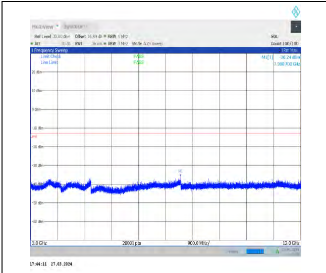
1-N25-15-40-L-1-DFT-PI2BPSK-Inner_1RB_Left-1 @1-3000-12000-Ant1-7988.70--36.24--13-PASS
