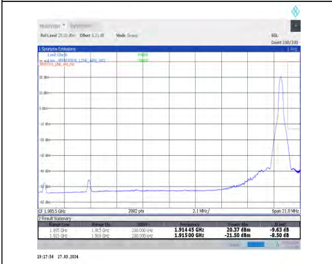
1-N25-15-20-H-5-CP-QPSK-Edge_1RB_Right-1@105-Ant1-1-seegraph-PASS-see graph
