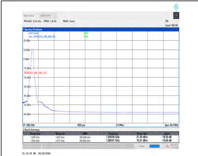
1-N25-15-25-L-1-DFT-PI2BPSK-Edge_1RB_Left-1@0-Ant1-1-seegraph-PASS-see graph
