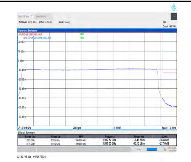
1-N25-15-10-H-6-CP-QPSK-Outer_Full-52@0-Ant1-1-seegraph-PASS-see graph
