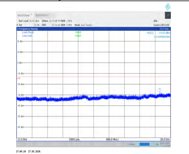
1-N25-15-40-H-1-DFT-PI2BPSK-Inner_1RB_Left-1@ 1-12000-20000-Ant1-19444.80--27.55--13-PASS
