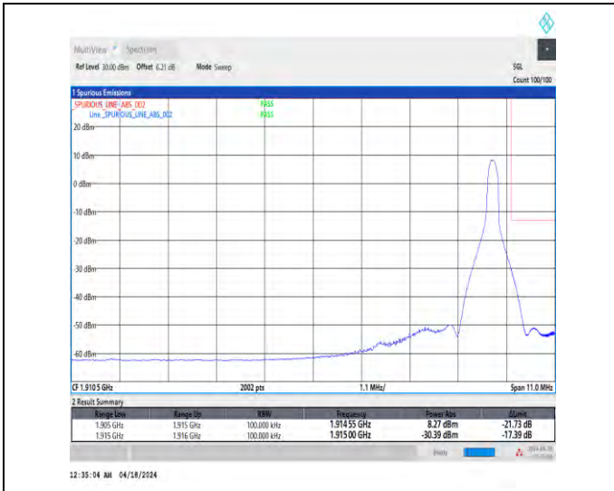
1-N25-15-10-H-2-DFT-PI2BPSK-Edge_1RB_Right-1@51-Ant1-1-seegraph-PASS-see graph
