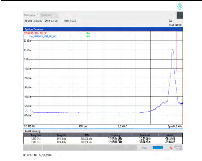
1-N25-15-25-H-5-CP-QPSK-Edge_1RB_Right-1@132-Ant1-1-seegraph-PASS-see graph
