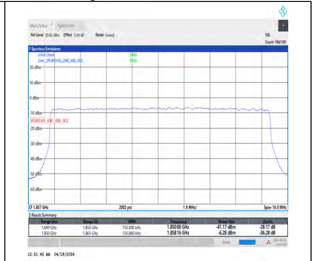
1-N25-15-15-L-3-DFT-PI2BPSK-Outer_Full-75@0-Ant1-1-seegraph-PASS-see graph
