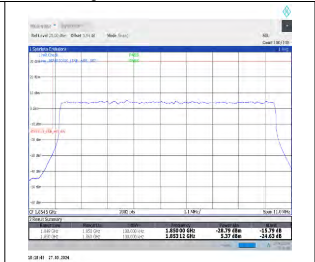
1-N25-15-10-L-3-DFT-PI2BPSK-Outer_Full-50@0-Ant1-1-seegraph-PASS-see graph
