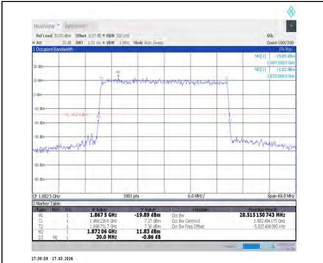
1-N25-15-30-M-4-DFT-64QAM-Outer_Full-160@0-A nt1-28.516-30.000-≤30-PASS
