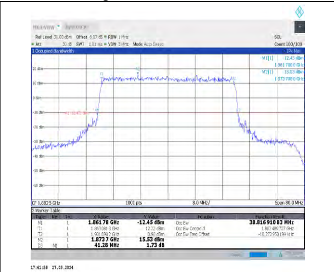
1-N25-15-40-M-8-CP-64QAM-Outer_Full-216@0-Ant 1-38.817-41.280-≤40-PASS
