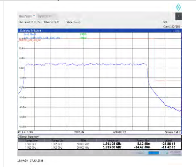
1-N25-15-5-H-3-DFT-PI2BPSK-Outer_Full-25@0-Ant1-1-seegraph-PASS-see graph
