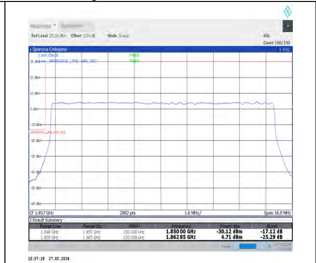
1-N25-15-15-L-3-DFT-PI2BPSK-Outer_Full-75@0-Ant1-1-seegraph-PASS-see graph
