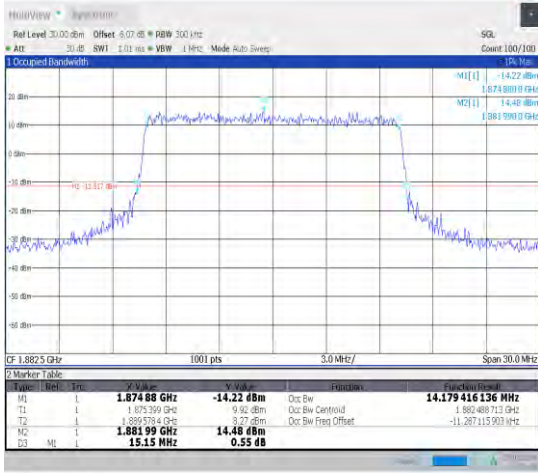
1-N25-15-15-M-7-CP-16QAM-Outer_Full-79@0-Ant1 -14.179-15.150-≤15-PASS
