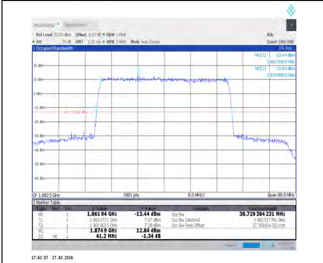
1-N25-15-40-M-9-CP-256QAM-Outer_Full-216@0-Ant nt1-38.729-41.200-≤40-PASS
