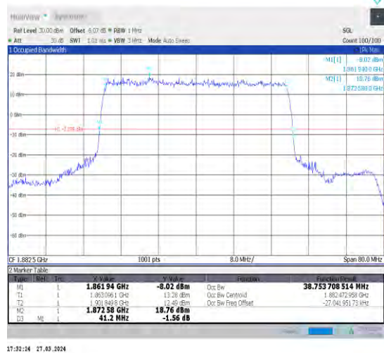
1-N25-15-40-M-2-DFT-PI2BPSK-Outer_Full-216@0- Ant1-38.754-41.200-≤40-PASS
