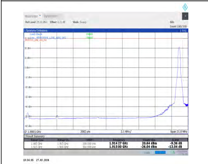
1-N25-15-30-H-5-CP-QPSK-Edge_1RB_Right-1@159-Ant1-1-seegraph-PASS-see graph
