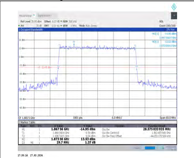
1-N25-15-30-M-1-DFT-QPSK-Outer_Full-160@0-Ant 1-28.576-29.700-≤30-PASS
