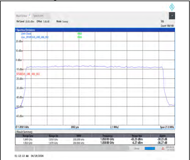
1-N25-15-20-L-3-DFT-PI2BPSK-Outer_Full-100@0-Ant1-1-seegraph-PASS-see graph
