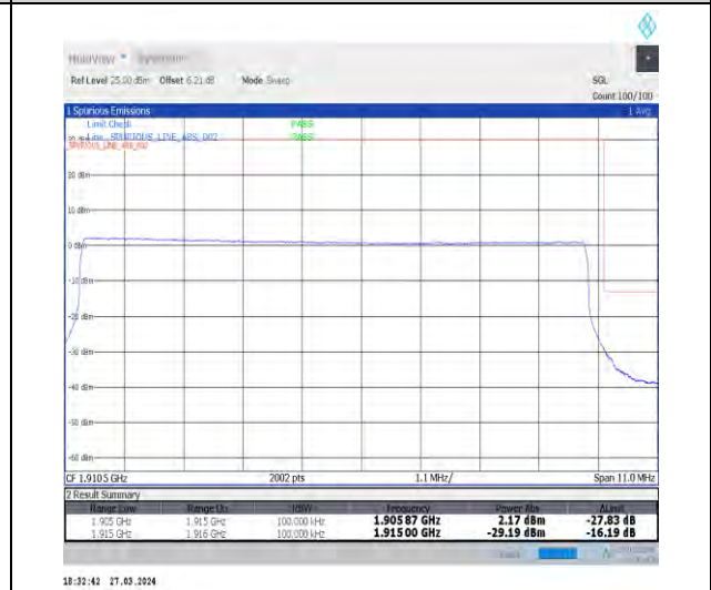
1-N25-15-10-H-6-CP-QPSK-Outer_Full-52@0-Ant1-1-seegraph-PASS-see graph
