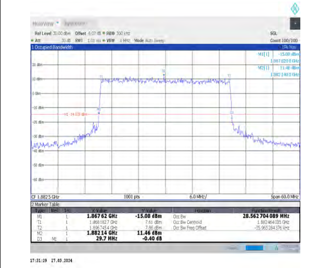
1-N25-15-30-M-7-CP-16QAM-Outer_Full-160@0-Ant1 1-28.563-29.700-≤30-PASS
