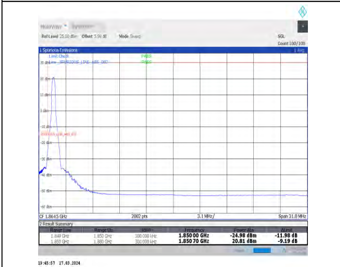
1-N25-15-30-L-4-CP-QPSK-Edge_1RB_Left-1@0-Ant1-1-seegraph-PASS-see graph
