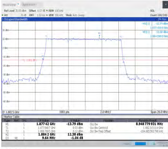
1-N25-15-10-M-4-DFT-64QAM-Outer_Full-50@0-Ant 1-8.949-9.640-≤10-PASS
