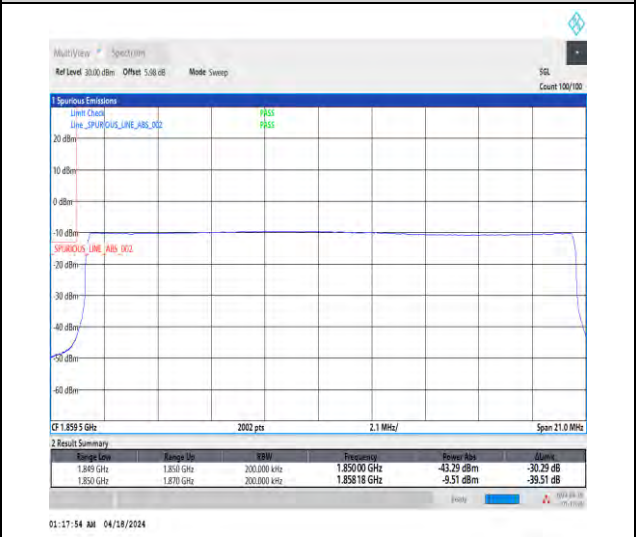
1-N25-15-20-L-6-CP-QPSK-Outer_Full-106@0-Ant1-1-seegraph-PASS-see graph
