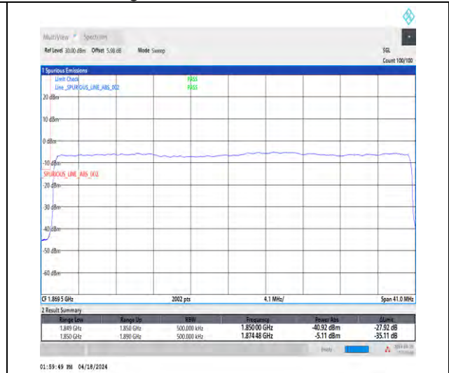
1-N25-15-40-L-3-DFT-PI2BPSK-Outer_Full-216@0-Ant1-1-seegraph-PASS-see graph
