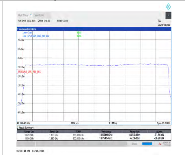
1-N25-15-30-L-3-DFT-PI2BPSK-Outer_Full-160@0-Ant1-1-seegraph-PASS-see graph
