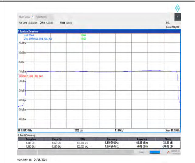
1-N25-15-30-L-6-CP-QPSK-Outer_Full-160@0-Ant1-1-seegraph-PASS-see graph
