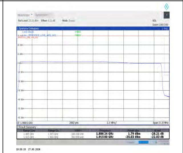
1-N25-15-30-H-6-CP-QPSK-Outer_Full-160@0-Ant1-1-seegraph-PASS-see graph
