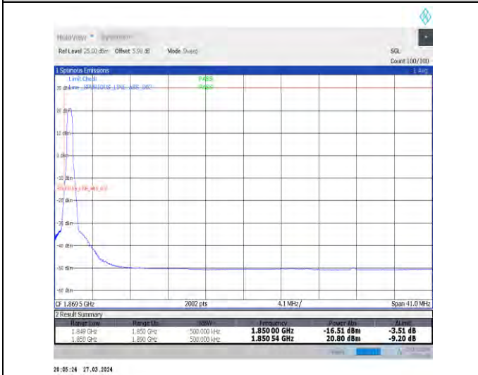
1-N25-15-40-L-4-CP-QPSK-Edge_1RB_Left-1@0-Ant1-1-seegraph-PASS-see graph
