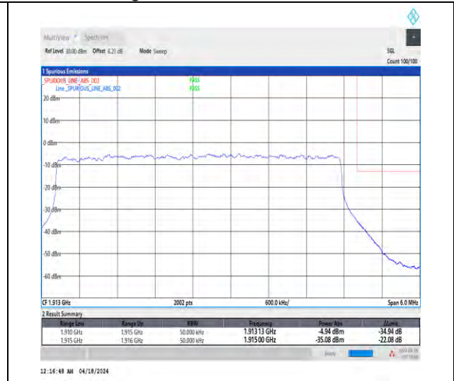
1-N25-15-5-H-3-DFT-PI2BPSK-Outer_Full-25@0-Ant1-1-seegraph-PASS-see graph
