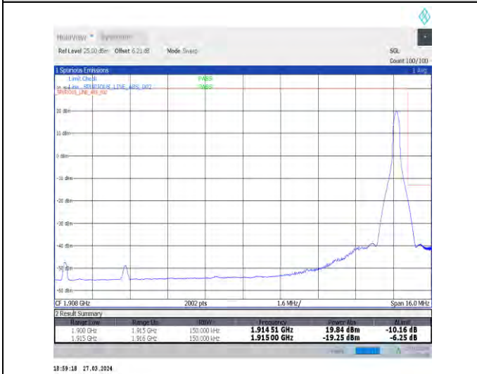
1-N25-15-15-H-5-CP-QPSK-Edge_1RB_Right-1@78-Ant1-1-seegraph-PASS-see graph
