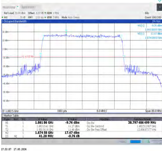
1-N25-15-40-M-1-DFT-QPSK-Outer_Full-216@0-Ant 1-38.797-41.280-≤40-PASS
