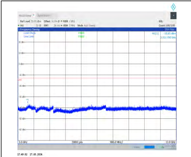
1-N25-15-40-H-1-DFT-PI2BPSK-Inner_1RB_Left-1 @1-3000-12000-Ant1-3551.70--35.85--13-PASS
