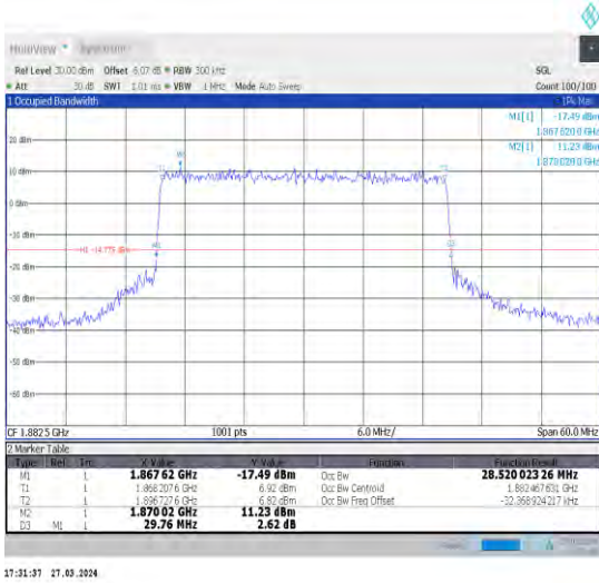
1-N25-15-30-M-8-CP-64QAM-Outer_Full-160@0-Ant 1-28.521-29.760-≤30-PASS
