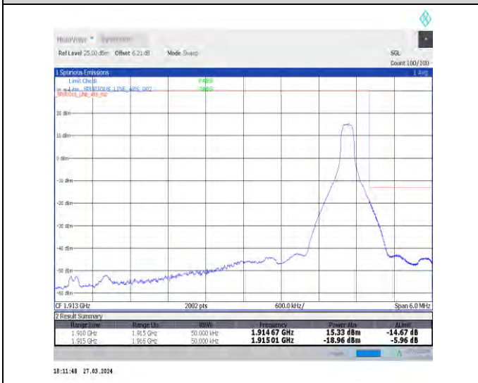
1-N25-15-5-H-5-CP-QPSK-Edge_1RB_Right-1@24-Ant1-1-seegraph-PASS-see graph
