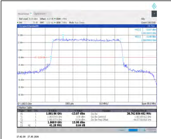
1-N25-15-40-M-7-CP-16QAM-Outer_Full-216@0-Ant 1-38.763-41.280-≤40-PASS
