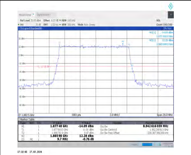
1-N25-15-10-M-3-DFT-16QAM-Outer_Full-50@0-Ant1 1-8.943-9.700-≤10-PASS
