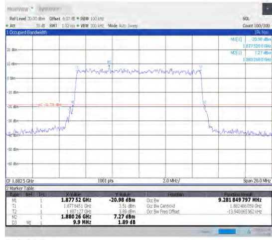
1-N25-15-10-M-9-CP-256QAM-Outer_Full-52@0-Ant1 1-9.282-9.900-≤10-PASS
