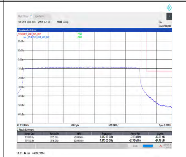
1-N25-15-5-H-6-CP-QPSK-Outer_Full-25@0-Ant1-1-seegraph-PASS-see graph
