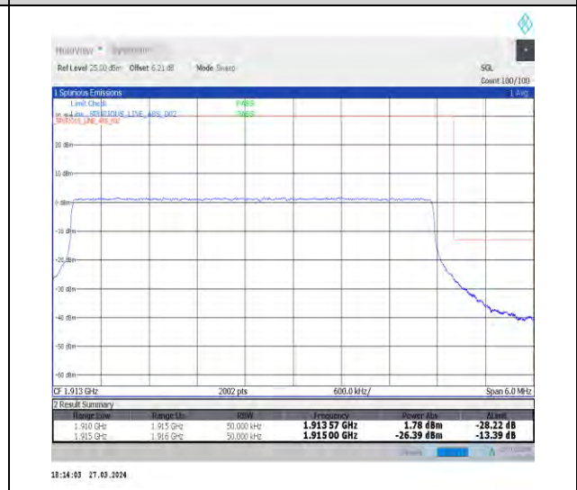
1-N25-15-5-H-6-CP-QPSK-Outer_Full-25@0-Ant1-1-seegraph-PASS-see graph
