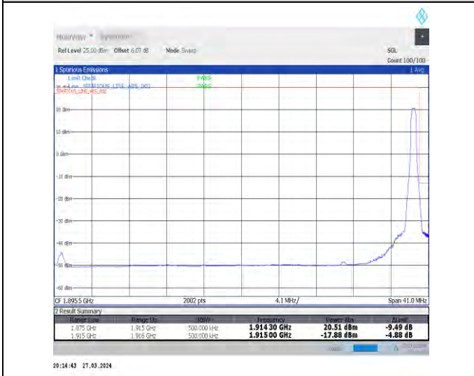
1-N25-15-40-H-5-CP-QPSK-Edge_1RB_Right-1@215-Ant1-1-seegraph-PASS-see graph
