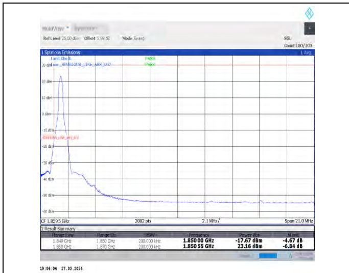
1-N25-15-20-L-1-DFT-PI2BPSK-Edge_1RB_Left-1@0-Ant1-1-seegraph-PASS-see graph
