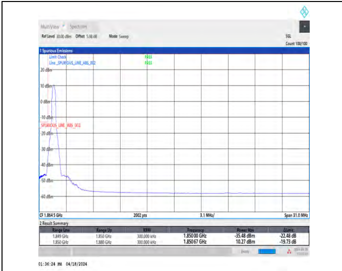
1-N25-15-30-L-1-DFT-PI2BPSK-Edge_1RB_Left-1@0-Ant1-1-seegraph-PASS-see graph
