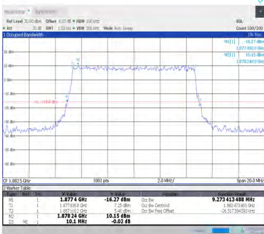
1-N25-15-10-M-6-CP-QPSK-Outer_Full-52@0-Ant1 9.273-10.100-≤10-PASS
