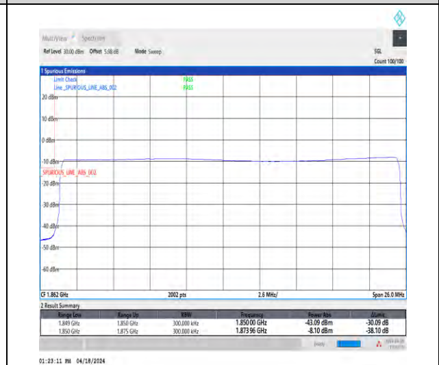
1-N25-15-25-L-6-CP-QPSK-Outer_Full-133@0-Ant1-1-seegraph-PASS-see graph
