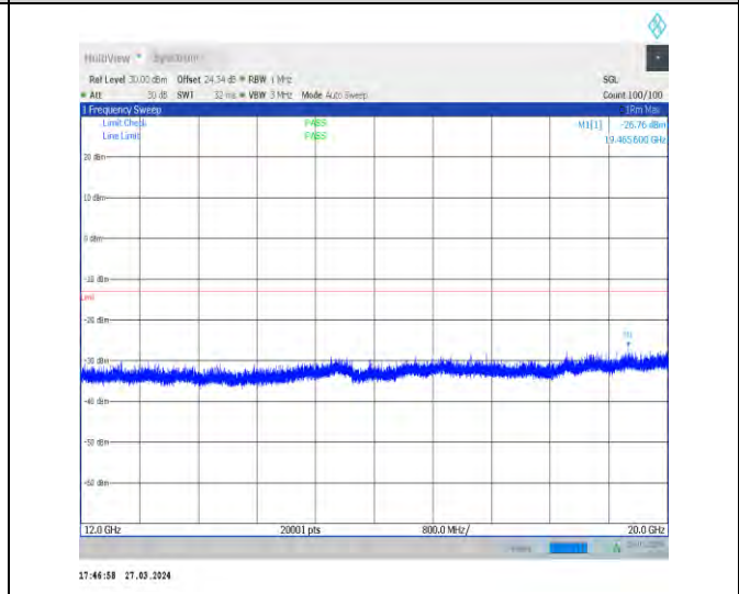
1-N25-15-40-M-1-DFT-PI2BPSK-Inner_1RB_Left-1 @ 1-12000-20000-Ant1-19465.60--26.76--13-PASS
