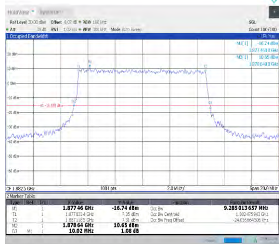
1-N25-15-10-M-7-CP-16QAM-Outer_Full-52@0-Ant1 -9.285-10.020-≤10-PASS
