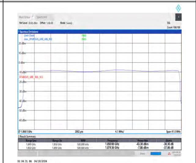
1-N25-15-40-L-6-CP-QPSK-Outer_Full-216@0-Ant1-1-seegraph-PASS-see graph
