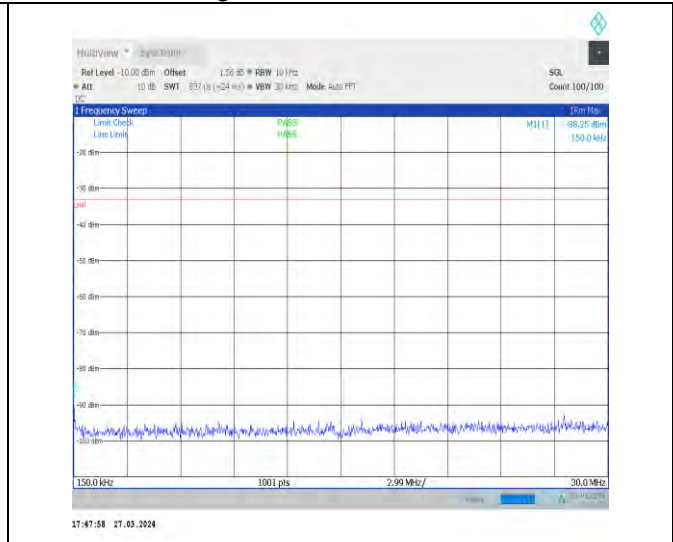
1-N25-15-40-H-1-DFT-PI2BPSK-Inner_1RB_Left-1@ 1-0.15-30-Ant1-0.15--88.25--33-PASS
