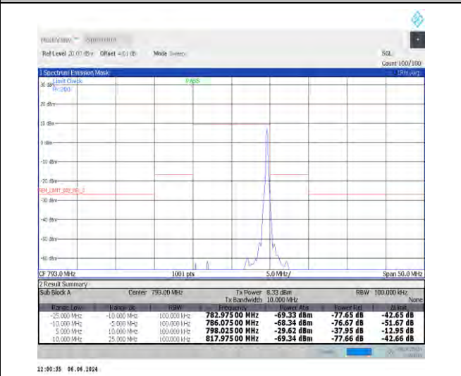
NTNV_N14_15_10_H_TID6_-25.00_-10.00_100.00_#1
