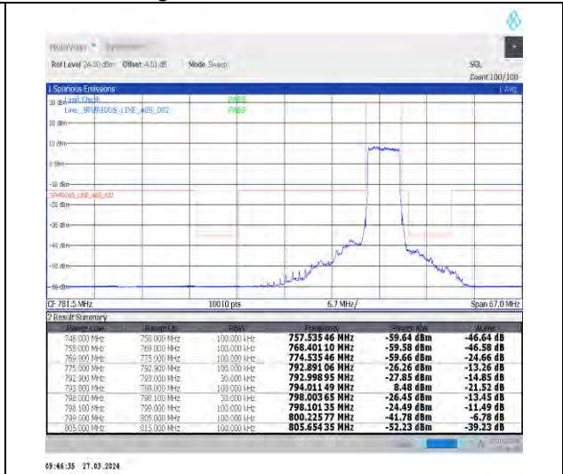
1-N14-15-5-H-3-DFT-PI2BPSK-Outer_Full-25@0-Ant1-1--PASS-see graph
