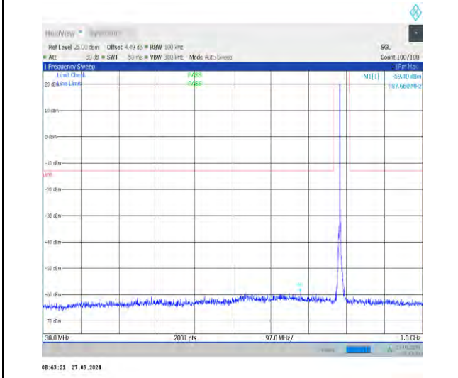
1-N14-15-10-M-1-DFT-PI2BPSK-Inner_1RB_Left-1 @ 1-30-1000-Ant1-687.66--59.40--13-PASS
