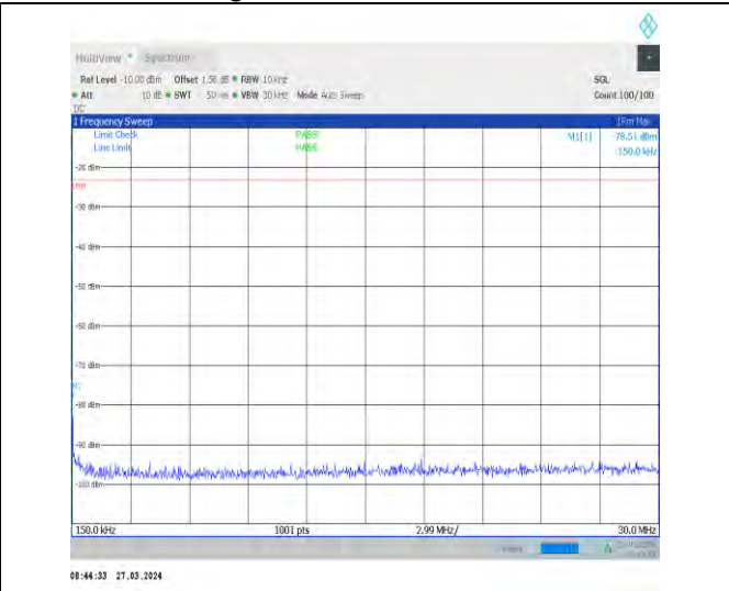
1-N14-15-10-H-1-DFT-PI2BPSK-Inner_1RB_Left-1@ 1-0.15-30-Ant1-0.15--78.51--23-PASS
