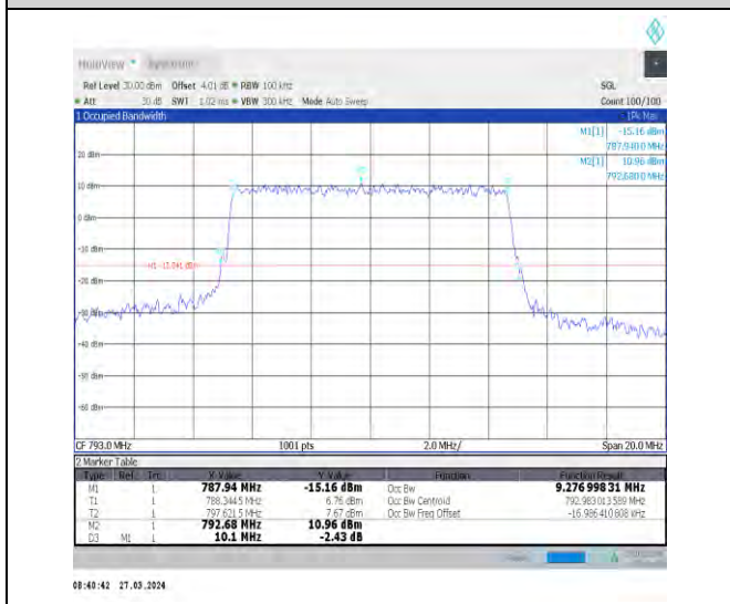
1-N14-15-10-M-6-CP-QPSK-Outer_Full-52@0-Ant1 9.277-10.100-≤10-PASS
