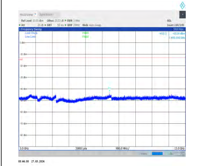
1-N14-15-10-M-1-DFT-PI2BPSK-Inner_1RB_Left-1 @ 1-3000-12000-Ant1-7895.10--42.58--13-PASS
