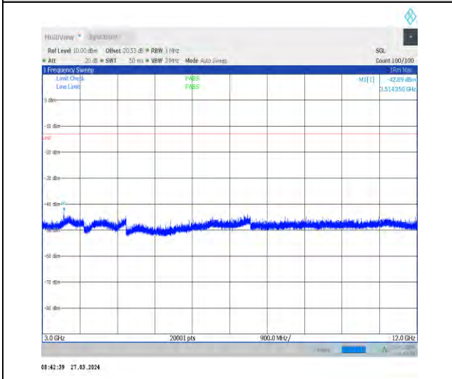
1-N14-15-10-L-1-DFT-PI2BPSK-Inner_1RB_Left-1 @1-3000-12000-Ant1-3514.35--42.89--13-PASS
