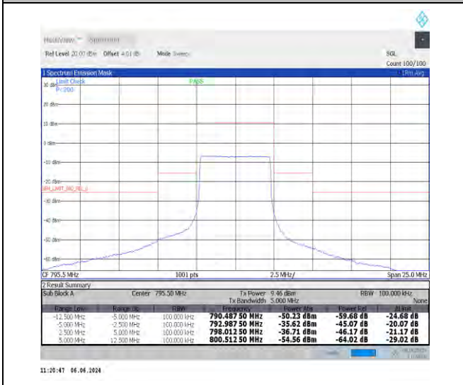
NTNV_N14_15_5_H_TID4_-12.50_-5.00_100.00_#1
