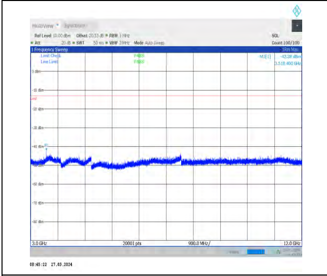
1-N14-15-10-H-1-DFT-PI2BPSK-Inner_1RB_Left-1 @1-3000-12000-Ant1-3518.40--42.38--13-PASS
