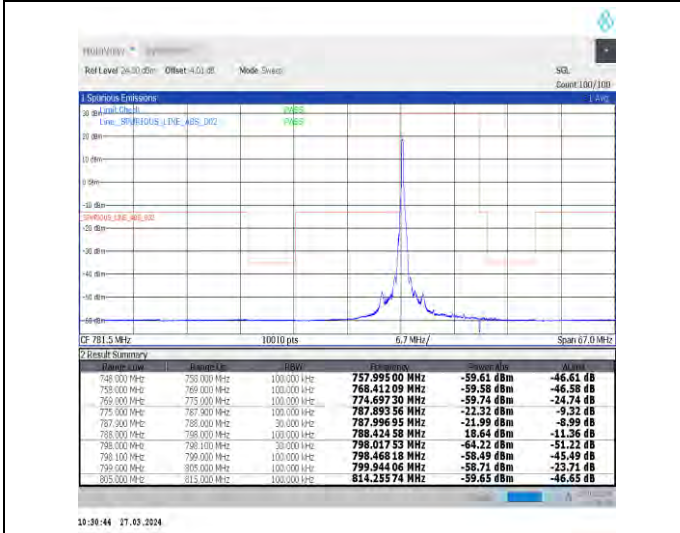
1-N14-15-10-L-4-CP-QPSK-Edge_1RB_Left-1@0-Ant1-1--PASS-see graph
