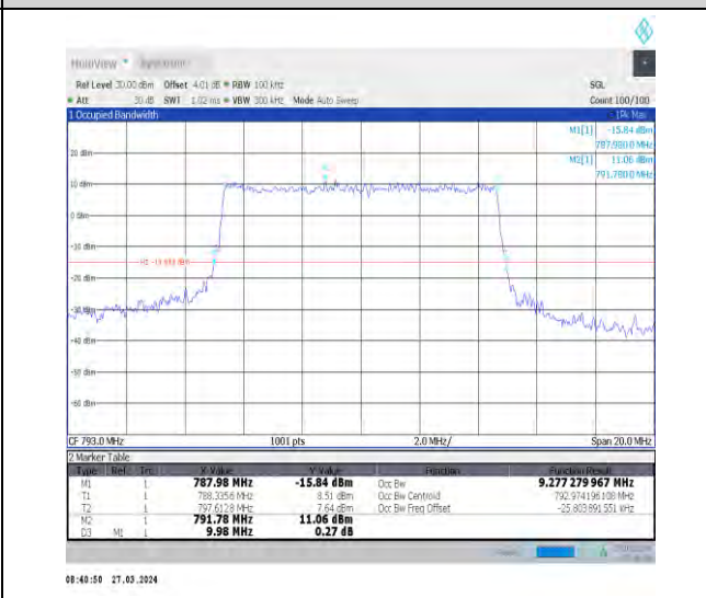
1-N14-15-10-M-7-CP-16QAM-Outer_Full-52@0-Ant 1-9.277-9.980-≤10-PASS
