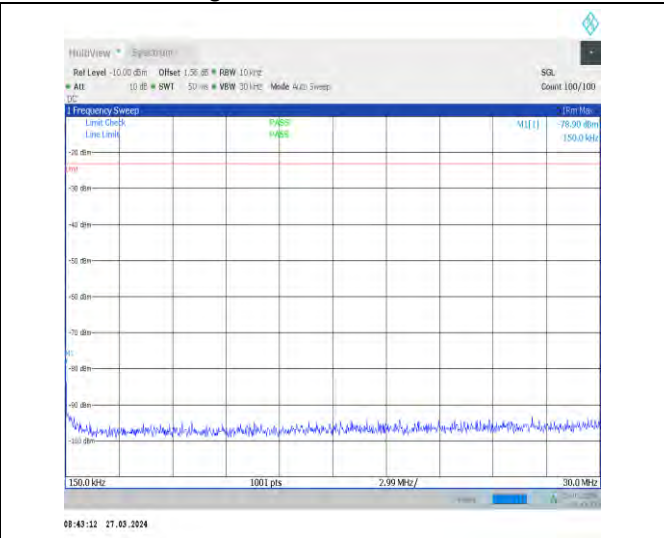
1-N14-15-10-M-1-DFT-PI2BPSK-Inner_1RB_Left-1 @ 1-0.15-30-Ant1-0.15--78.90--23-PASS
