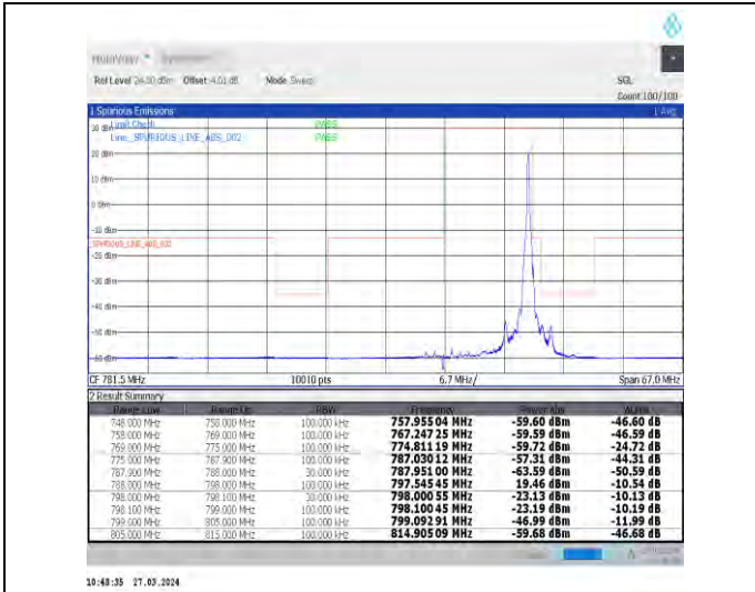
1-N14-15-10-H-2-DFT-PI2BPSK-Edge_1RB_Right-1@51-Ant1-1--PASS-see graph
