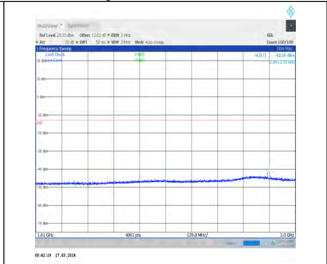
1-N14-15-10-L-1-DFT-PI2BPSK-Inner_1RB_Left-1@ 1-1610-3000-Ant1-2851.27--43.56--13-PASS
