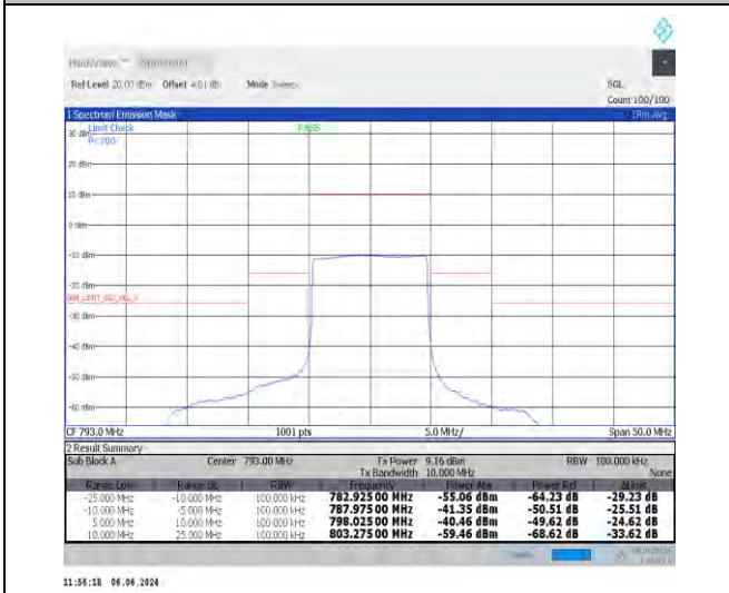
NTNV_N14_15_10_H_TID4_-25.00_-10.00_100.00_#1
