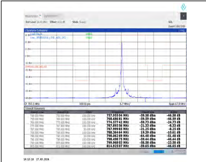
1-N14-15-10-L-1-DFT-PI2BPSK-Edge_1RB_Left-1@0-Ant1-1--PASS-see graph
