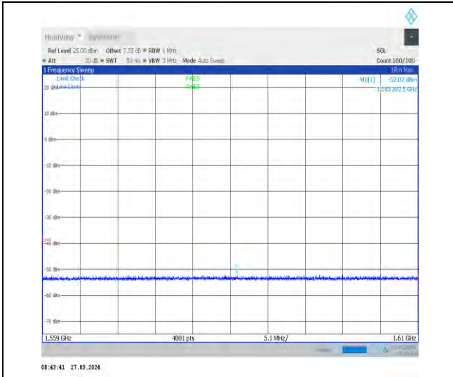
1-N14-15-10-M-1-DFT-PI2BPSK-Inner_1RB_Left-1 @ 1-1559-1610-Ant1-1585.39--52.02--40-PASS
