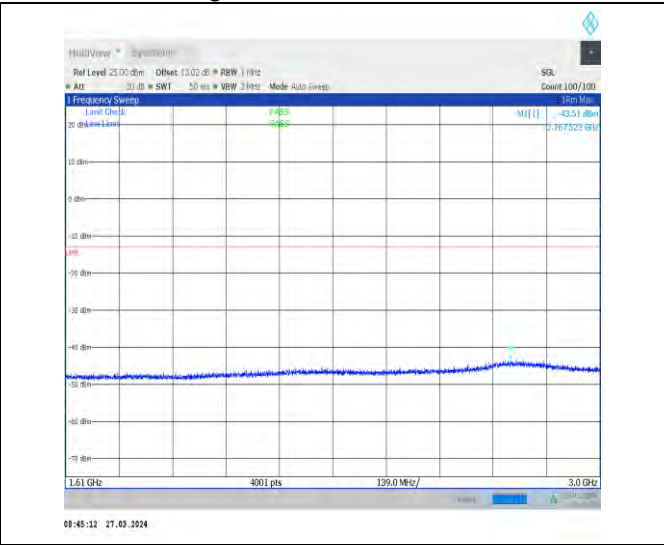
1-N14-15-10-H-1-DFT-PI2BPSK-Inner_1RB_Left-1@ 1-1610-3000-Ant1-2767.52--43.51--13-PASS
