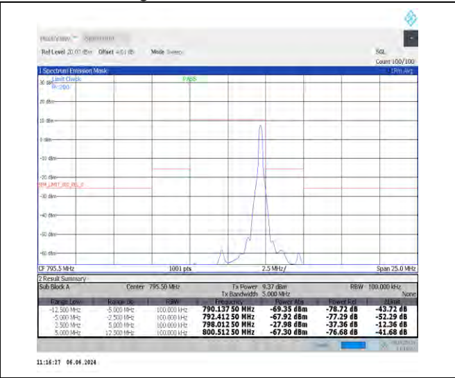
NTNV_N14_15_5_H_TID3_-12.50_-5.00_100.00_#1
