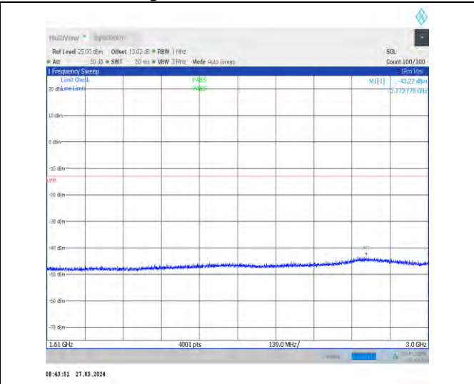
1-N14-15-10-M-1-DFT-PI2BPSK-Inner_1RB_Left-1 @ 1-1610-3000-Ant1-2773.78--43.22--13-PASS
