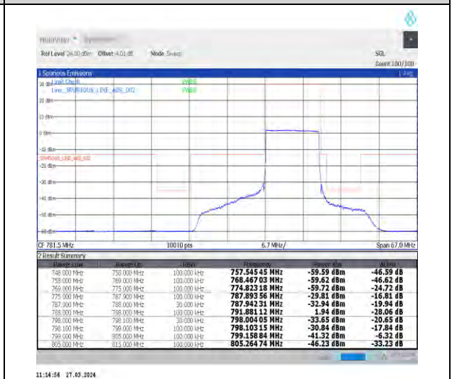
1-N14-15-10-H-6-CP-QPSK-Outer_Full-52@0-Ant1-1--PASS-see graph
