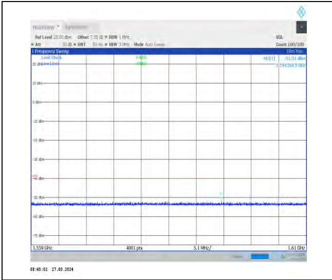
1-N14-15-10-H-1-DFT-PI2BPSK-Inner_1RB_Left-1 @1-1559-1610-Ant1-1594.27--51.31--40-PASS
