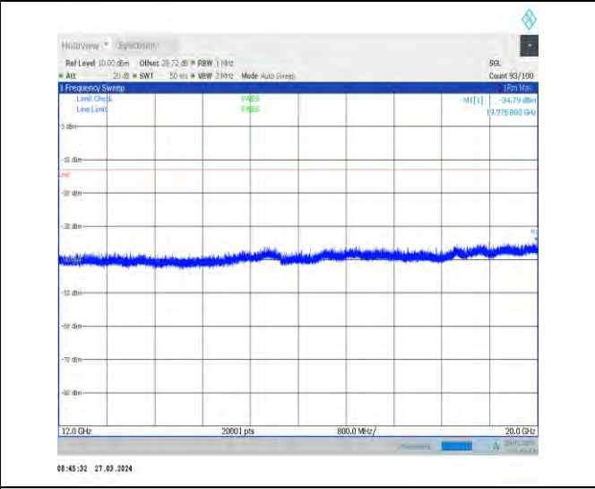
1-N14-15-10-H-1-DFT-PI2BPSK-Inner_1RB_Left-1@ 1-12000-20000-Ant1-19976.80--34.79--13-PASS
