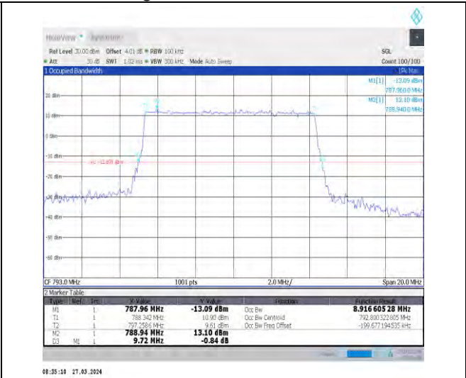
1-N14-15-10-M-1-DFT-QPSK-Outer_Full-50@0-Ant1 -8.917-9.720≤10-PASS
