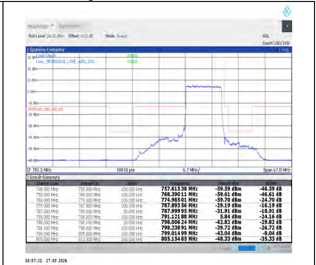
1-N14-15-10-H-3-DFT-PI2BPSK-Outer_Full-50@0-Ant1-1--PASS-see graph
