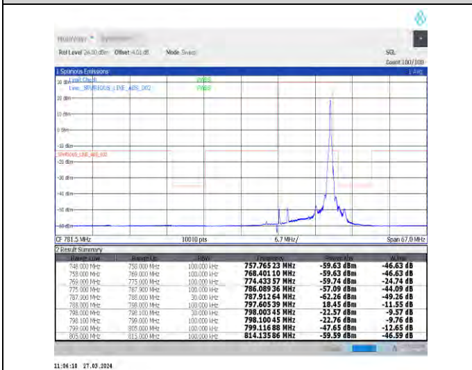
1-N14-15-10-H-5-CP-QPSK-Edge_1RB_Right-1@51-Ant1-1--PASS-see graph
