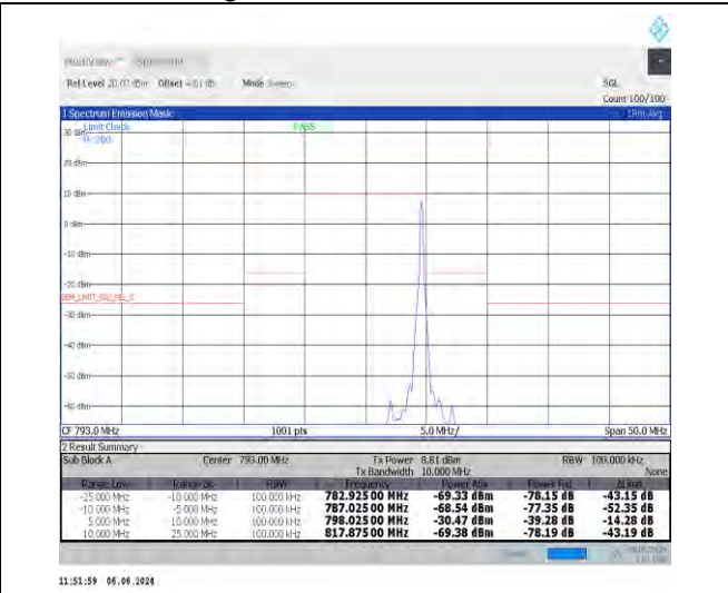
NTNV_N14_15_10_H_TID3_-25.00_-10.00_100.00_#1
