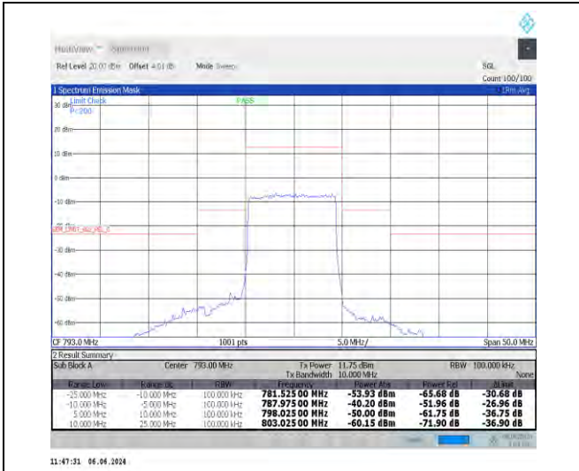
NTNV_N14_15_10_H_TID1_-25.00_-10.00_100.00_#1
