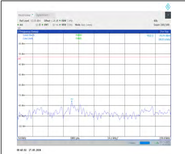
1-N14-15-10-M-1-DFT-PI2BPSK-Inner_1RB_Left-1 @ 1-0.009-0.15-Ant1-0.06--76.94--33-PASS
