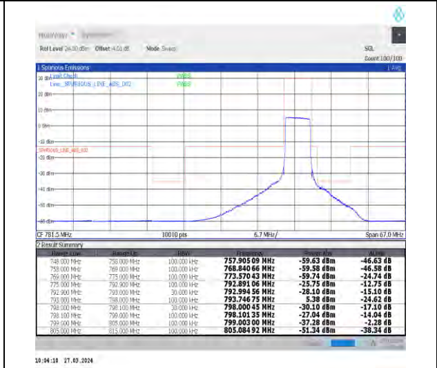
1-N14-15-5-H-6-CP-QPSK-Outer_Full-25@0-Ant1-1--PASS-see graph
