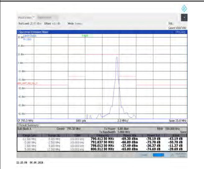
NTNV_N14_15_5_H_TID6_-12.50_-5.00_100.00_#1
