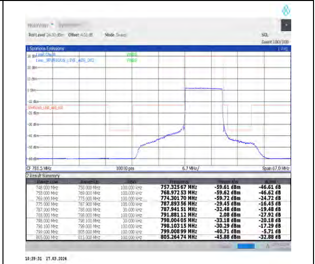
1-N14-15-10-L-6-CP-QPSK-Outer_Full-52@0-Ant1-1--PASS-see graph
