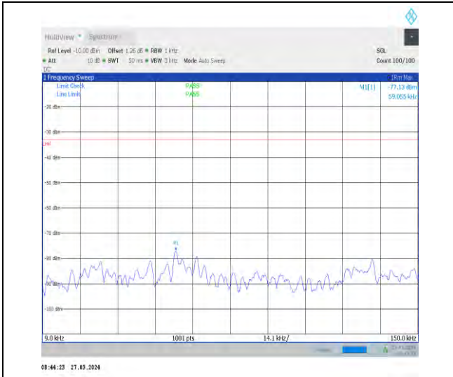
1-N14-15-10-H-1-DFT-PI2BPSK-Inner_1RB_Left-1 @1-0.009-0.15-Ant1-0.06--77.13--33-PASS
