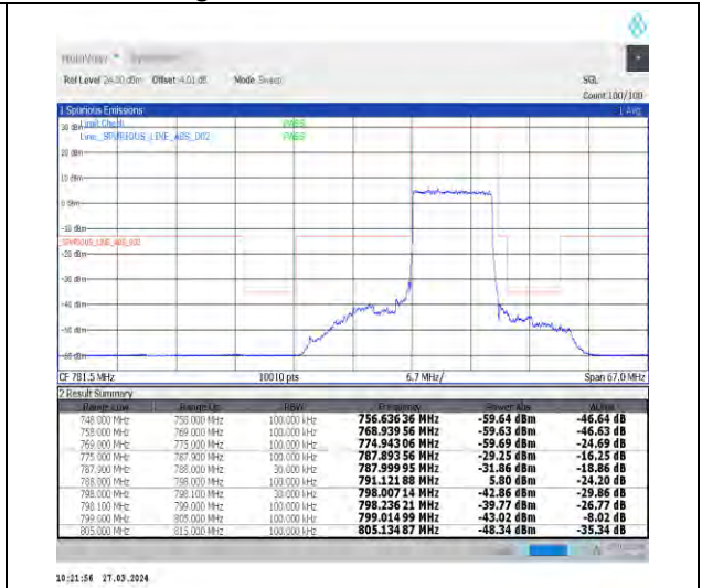
1-N14-15-10-L-3-DFT-PI2BPSK-Outer_Full-50@0-Ant1-1--PASS-see graph
