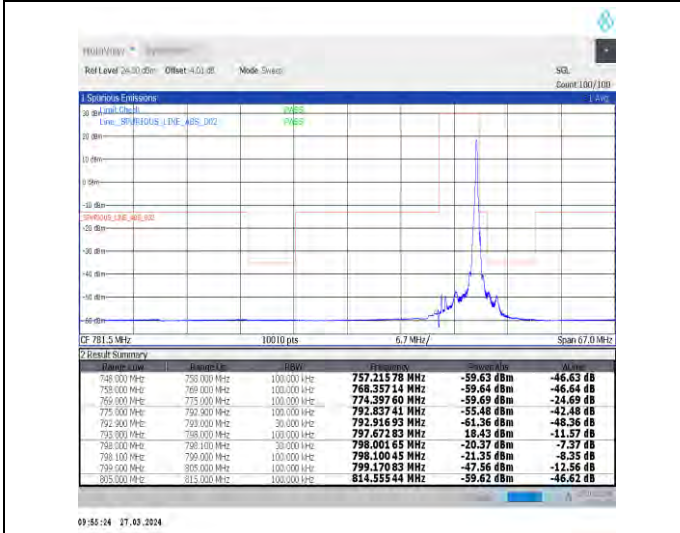
1-N14-15-5-H-5-CP-QPSK-Edge_1RB_Right-1@24-Ant1-1--PASS-see graph
