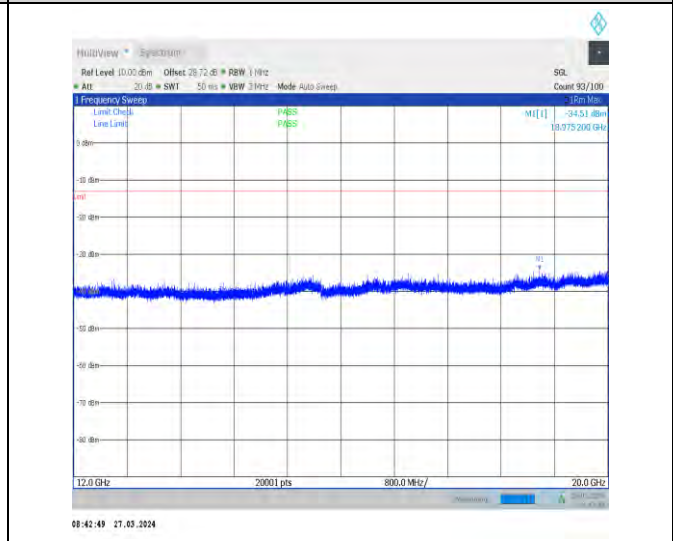
1-N14-15-10-L-1-DFT-PI2BPSK-Inner_1RB_Left-1@ 1-12000-20000-Ant1-18975.20--34.51--13-PASS
