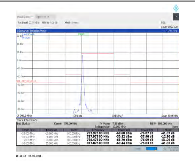
NTNV_N14_15_10_L_TID5_-25.00_-10.00_100.00_#1
