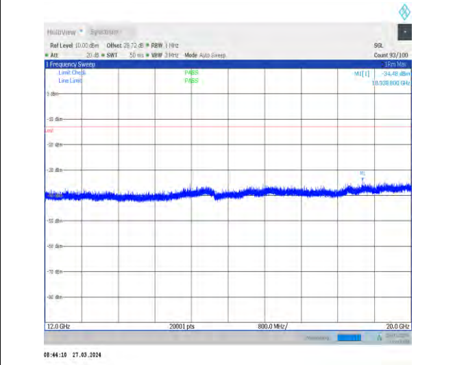
1-N14-15-10-M-1-DFT-PI2BPSK-Inner_1RB_Left-1 @ 1-12000-20000-Ant1-18938.80--34.48--13-PASS
