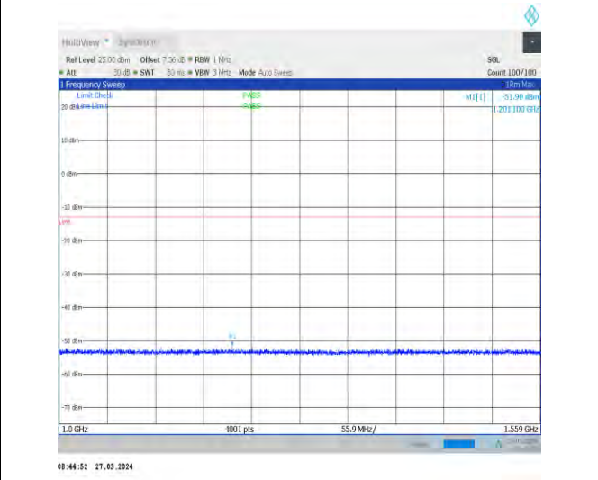
1-N14-15-10-H-1-DFT-PI2BPSK-Inner_1RB_Left-1@ 1-1000-1559-Ant1-1201.10--51.90--13-PASS
